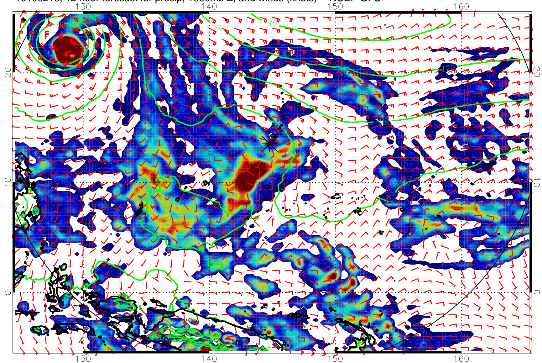
16100218, 12 hour forecast for precip, 1000mb Z, and winds (knots) -- NCEP GFS
