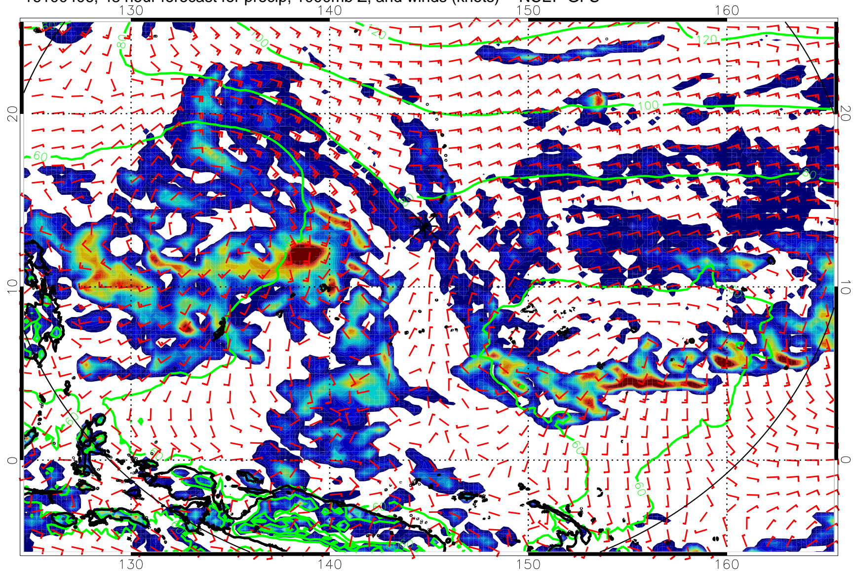
16100406, 48 hour forecast for precip, 1000mb Z, and winds (knots) -- NCEP GFS
