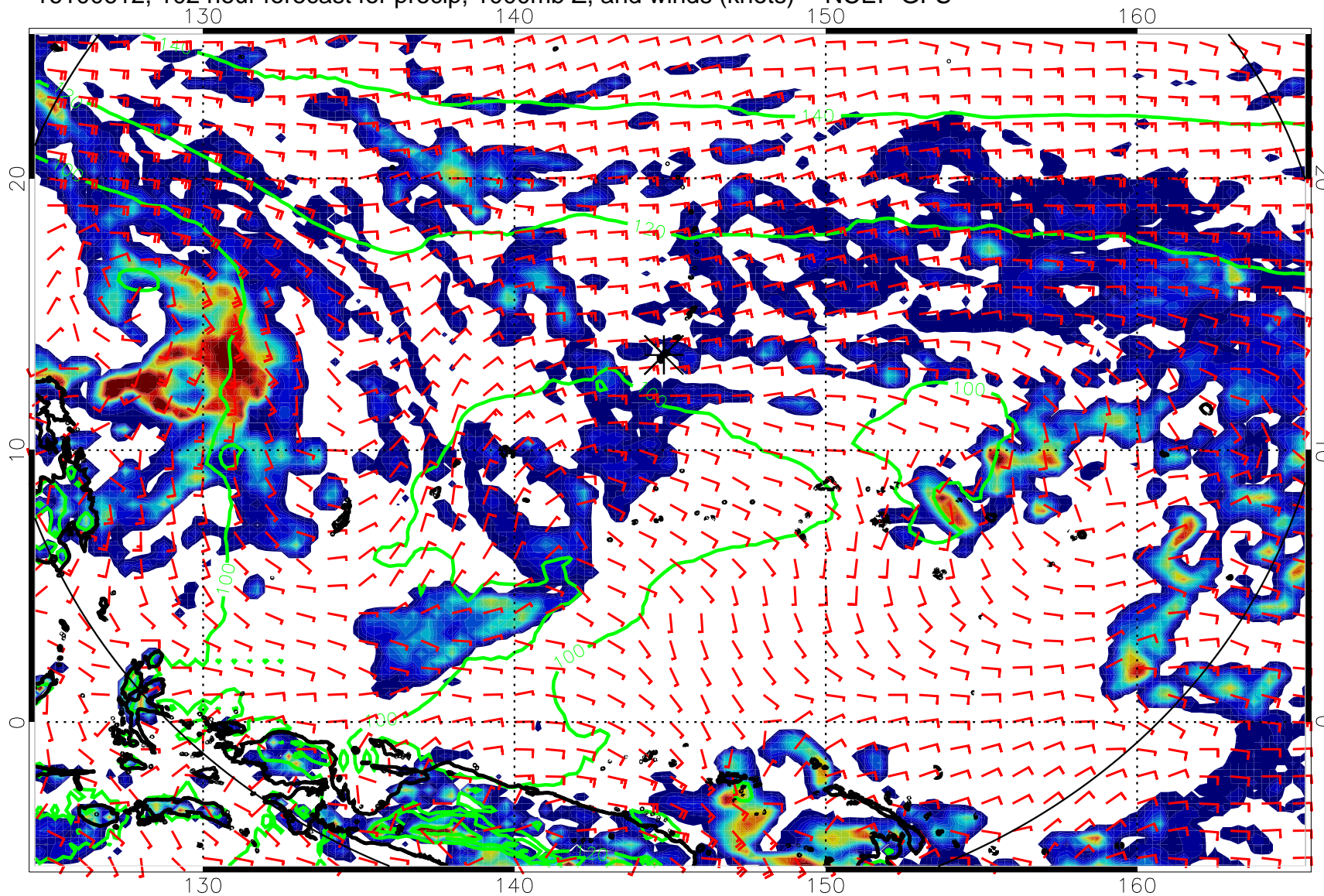
16100612, 102 hour forecast for precip, 1000mb Z, and winds (knots) -- NCEP GFS
