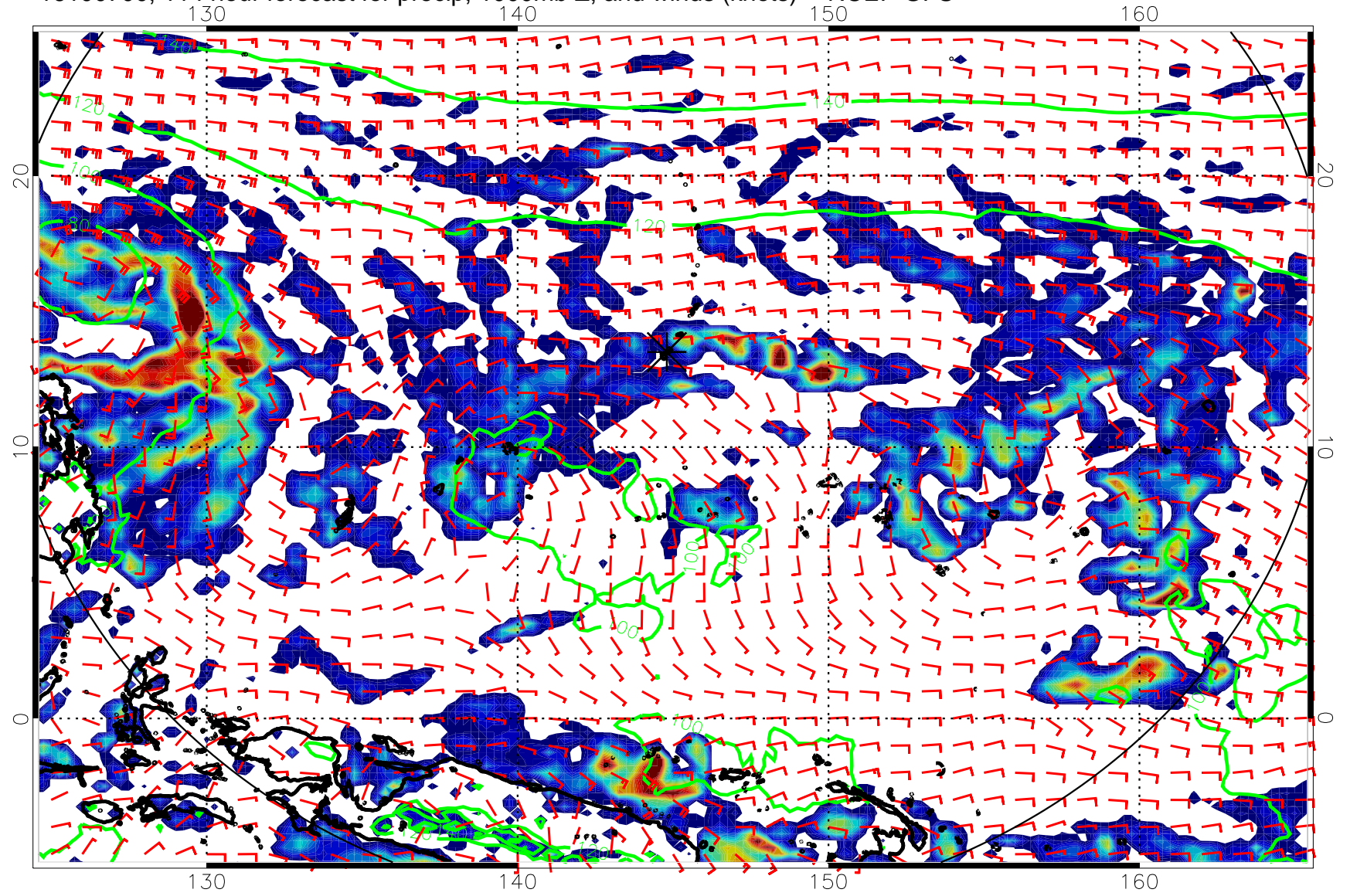
16100700, 114 hour forecast for precip, 1000mb Z, and winds (knots) -- NCEP GFS
