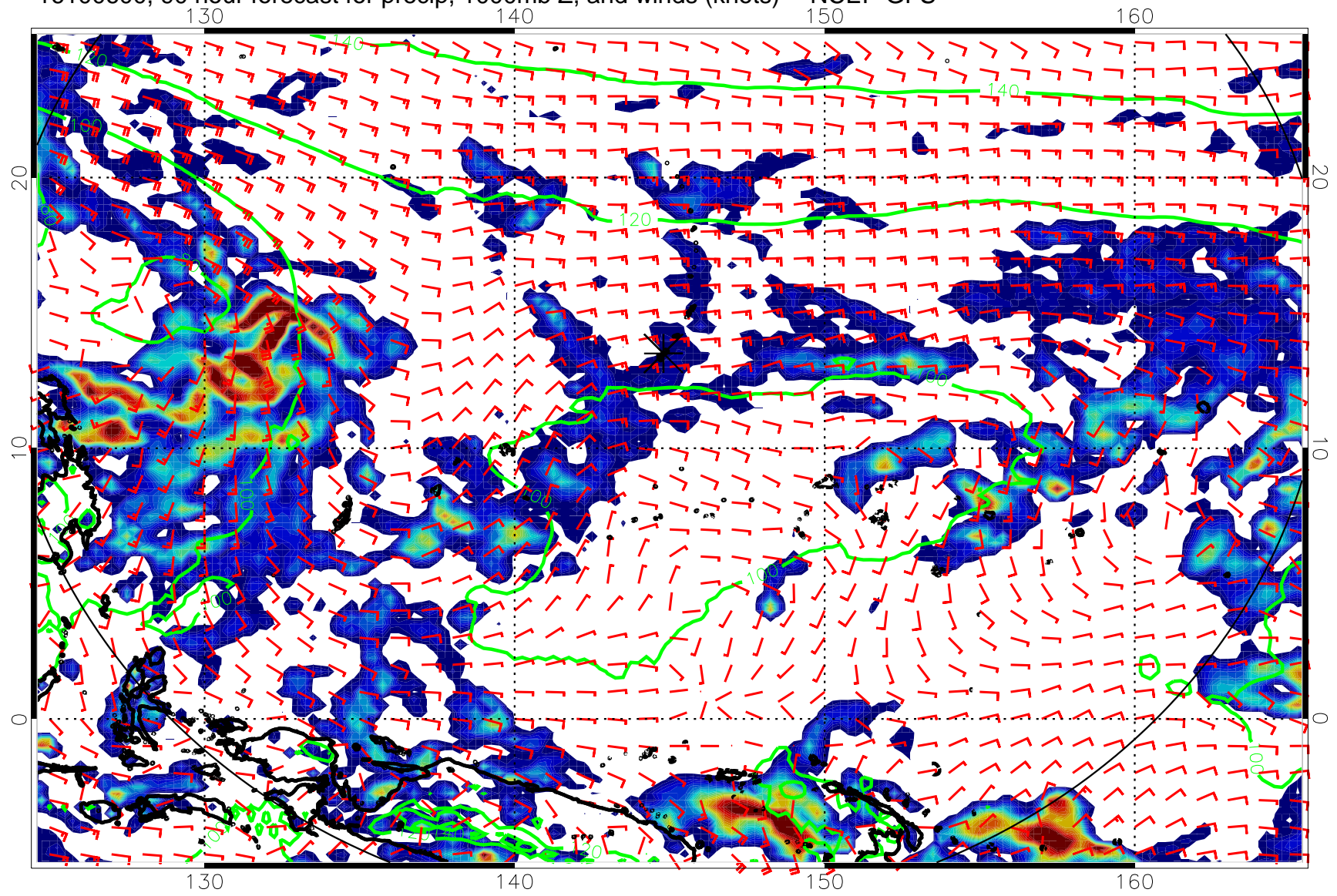
16100600, 90 hour forecast for precip, 1000mb Z, and winds (knots) -- NCEP GFS
