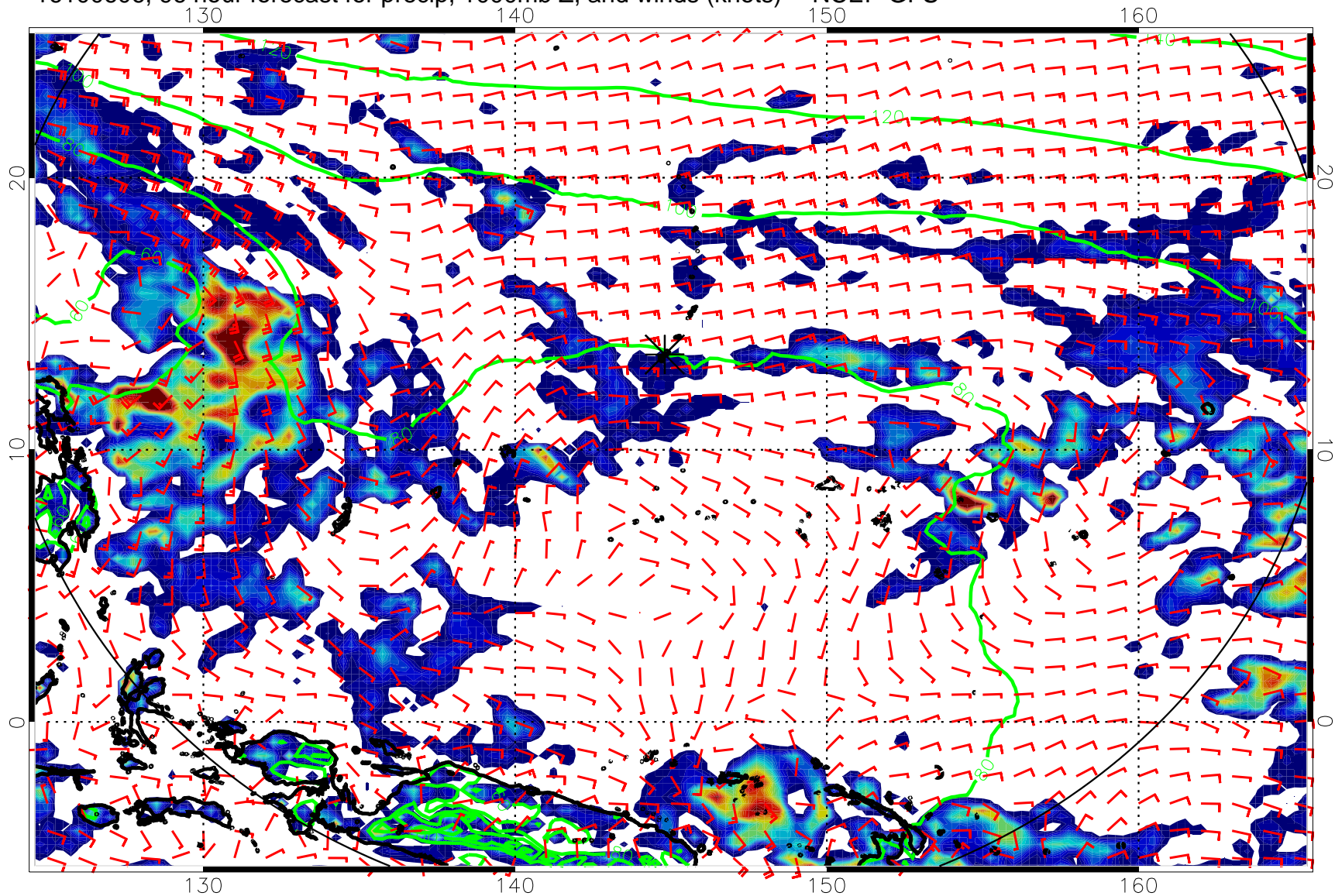
16100606, 96 hour forecast for precip, 1000mb Z, and winds (knots) -- NCEP GFS
