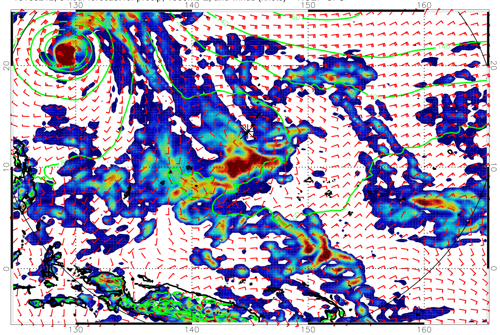
16100212, 6 hour forecast for precip, 1000mb Z, and winds (knots) -- NCEP GFS
