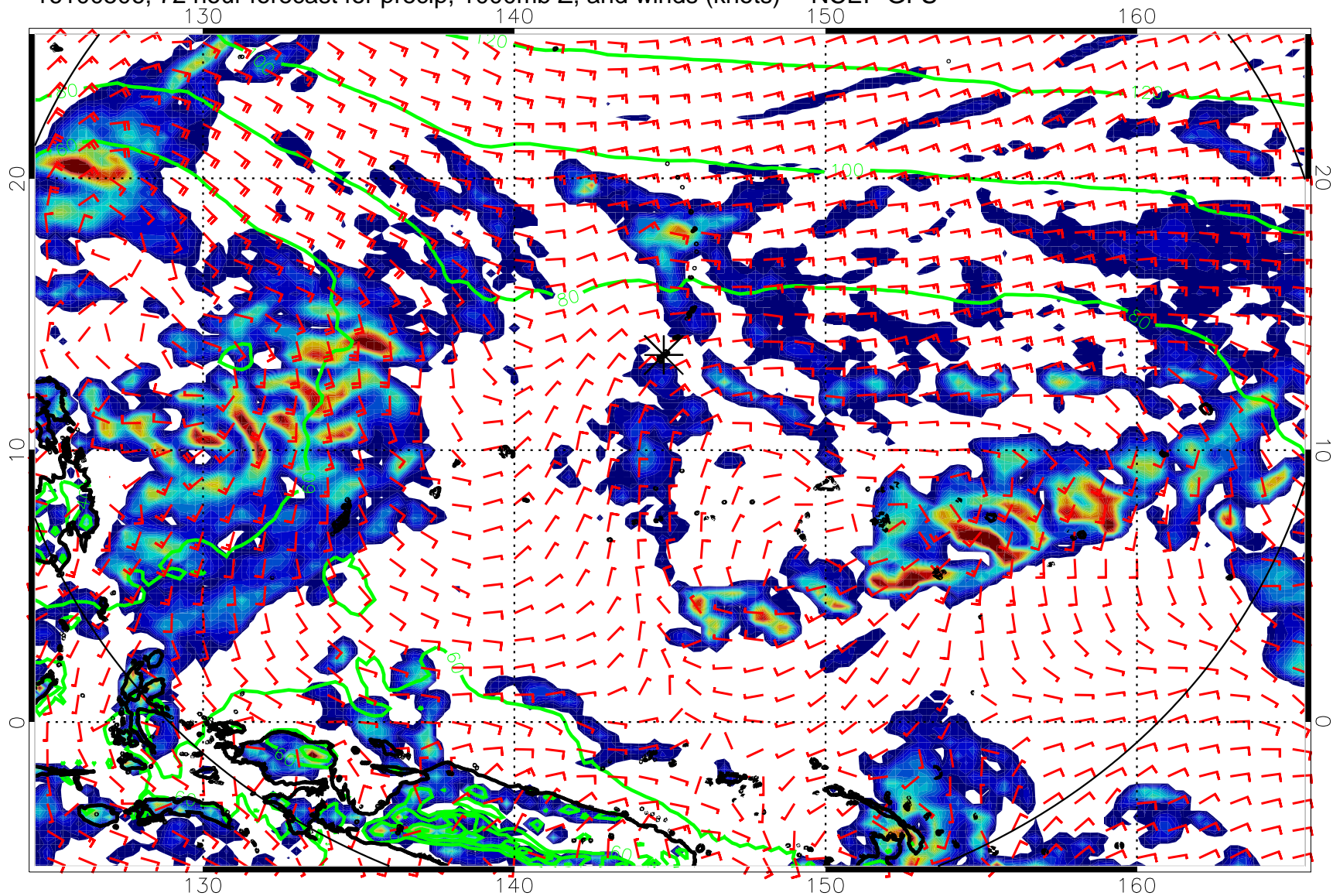
16100506, 72 hour forecast for precip, 1000mb Z, and winds (knots) -- NCEP GFS
