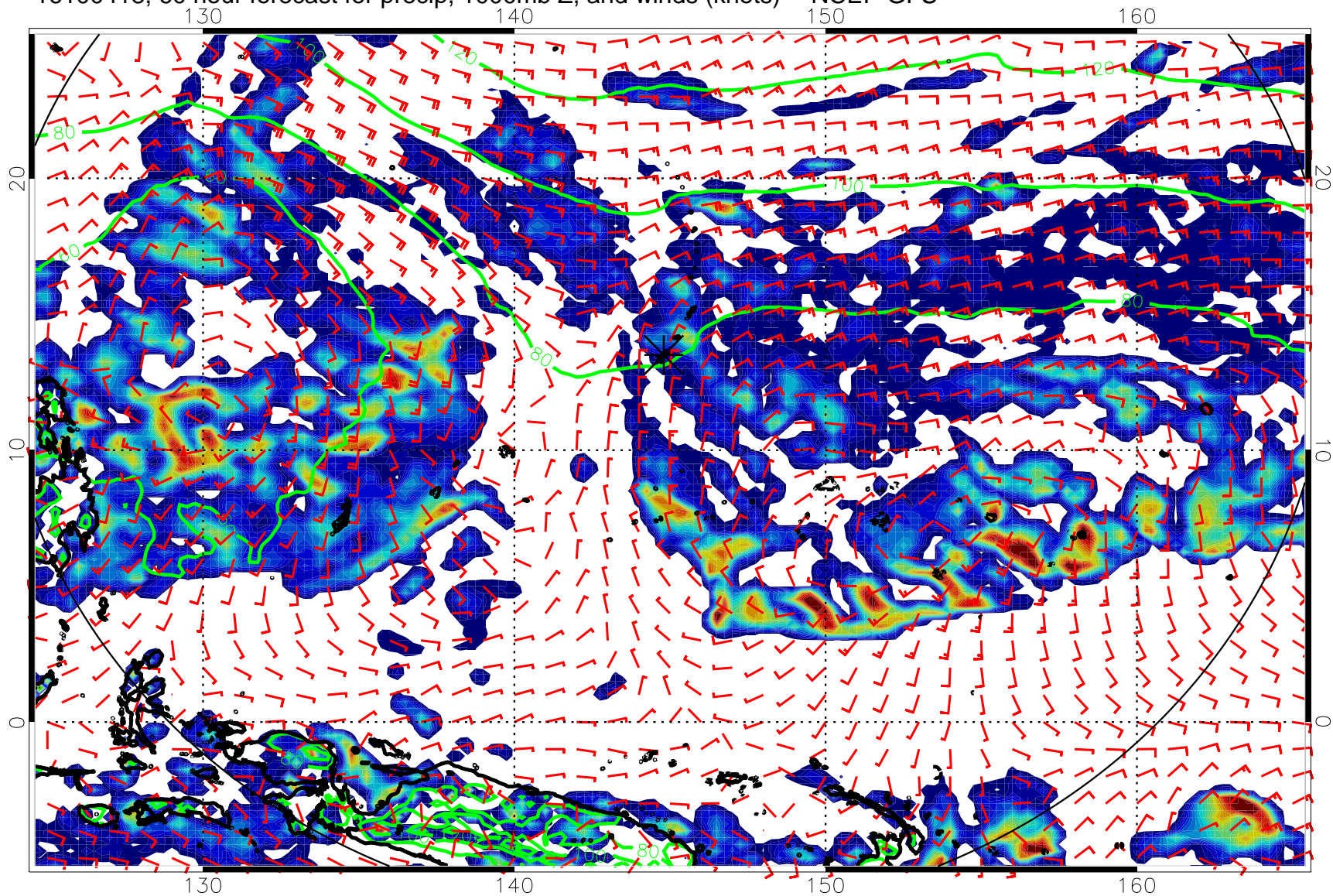
16100418, 60 hour forecast for precip, 1000mb Z, and winds (knots) -- NCEP GFS
