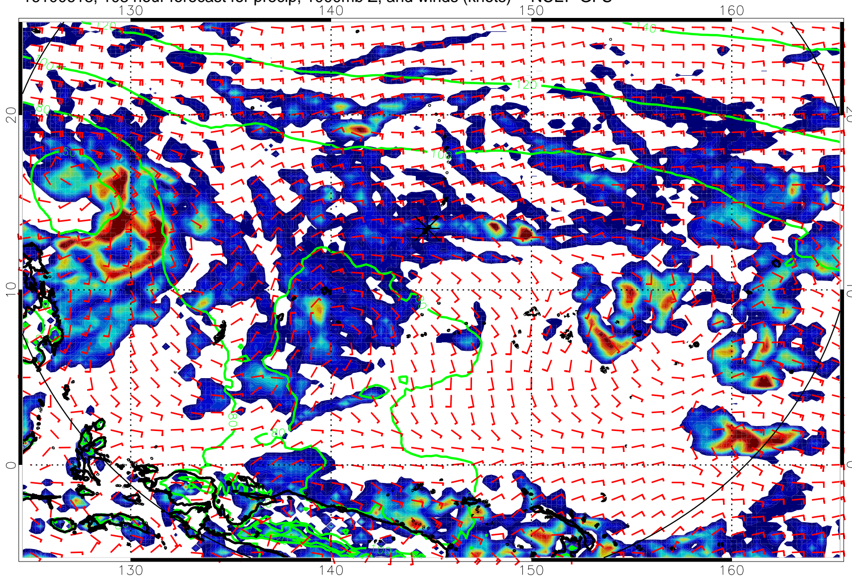
16100618, 108 hour forecast for precip, 1000mb Z, and winds (knots) -- NCEP GFS
