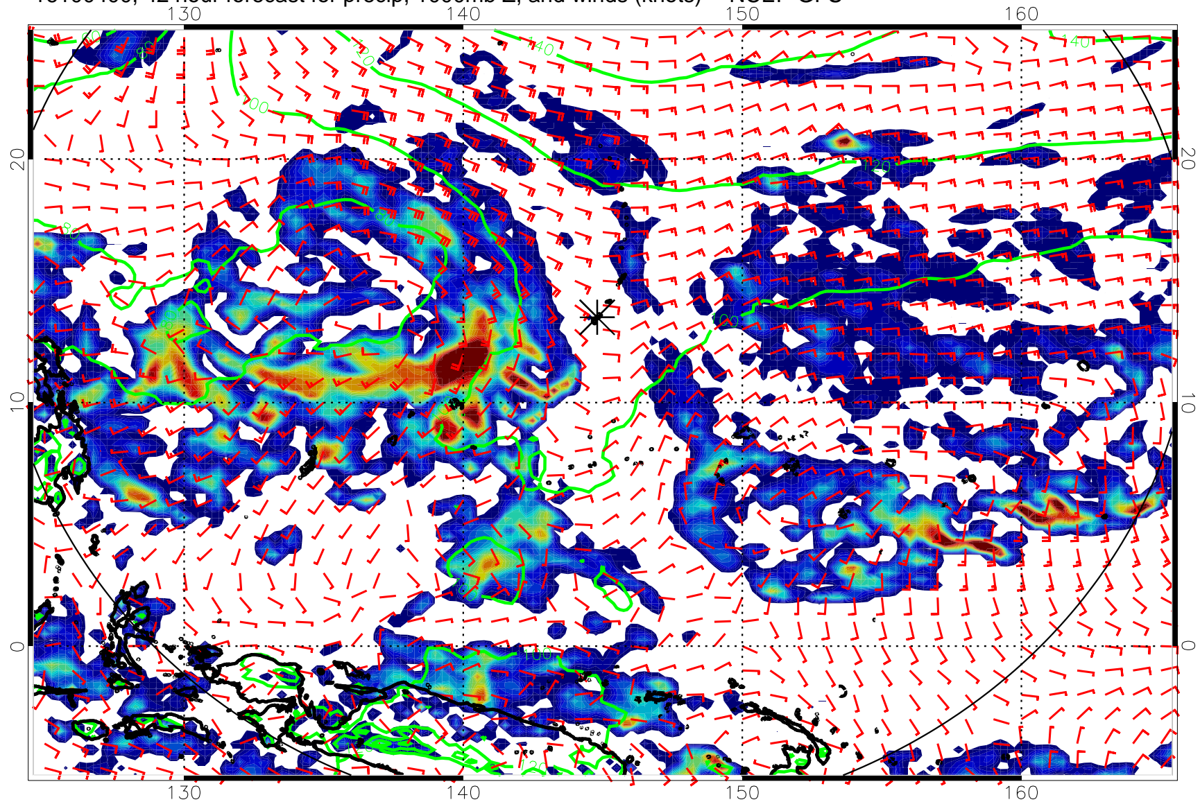
16100400, 42 hour forecast for precip, 1000mb Z, and winds (knots) -- NCEP GFS
