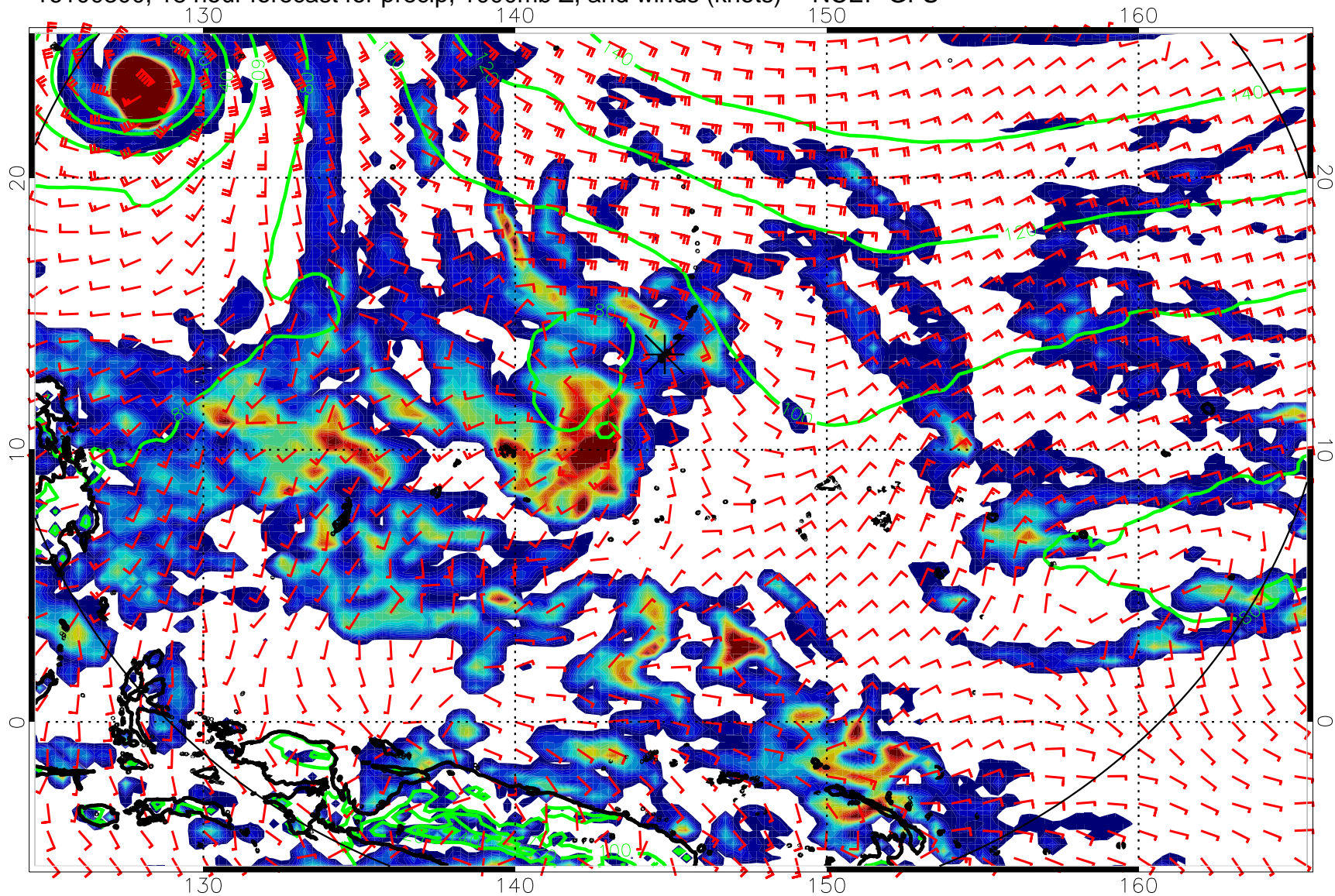
16100300, 18 hour forecast for precip, 1000mb Z, and winds (knots) -- NCEP GFS
