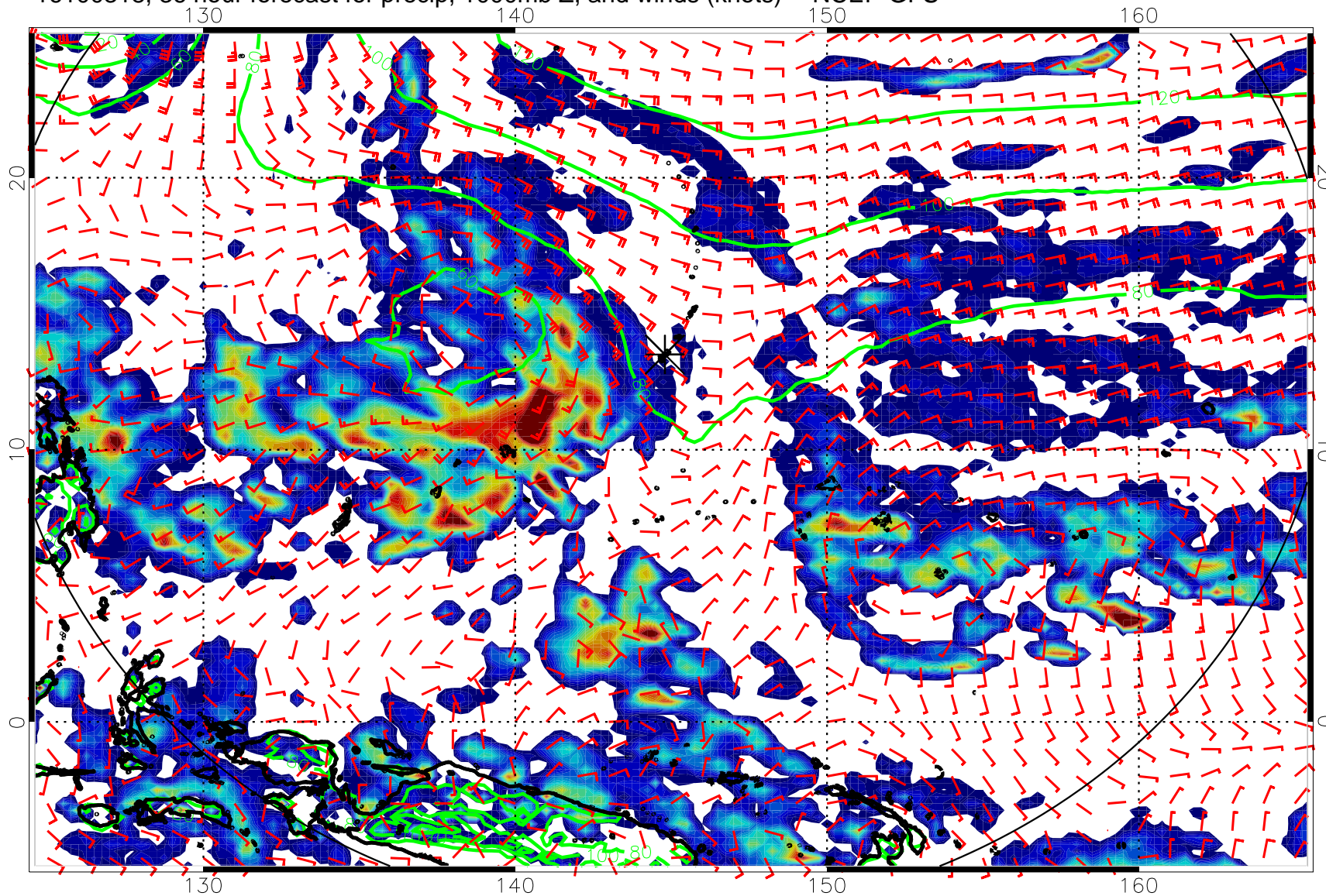
16100318, 36 hour forecast for precip, 1000mb Z, and winds (knots) -- NCEP GFS
