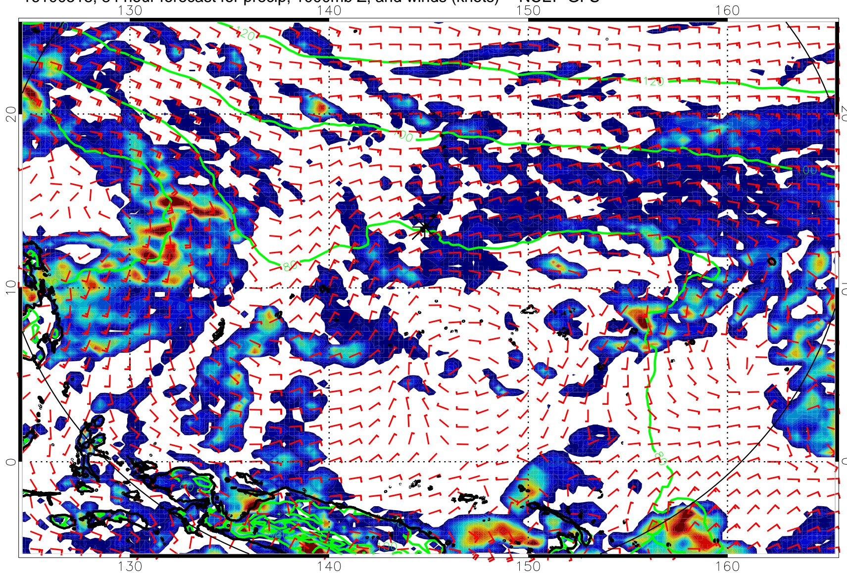
16100518, 84 hour forecast for precip, 1000mb Z, and winds (knots) -- NCEP GFS
