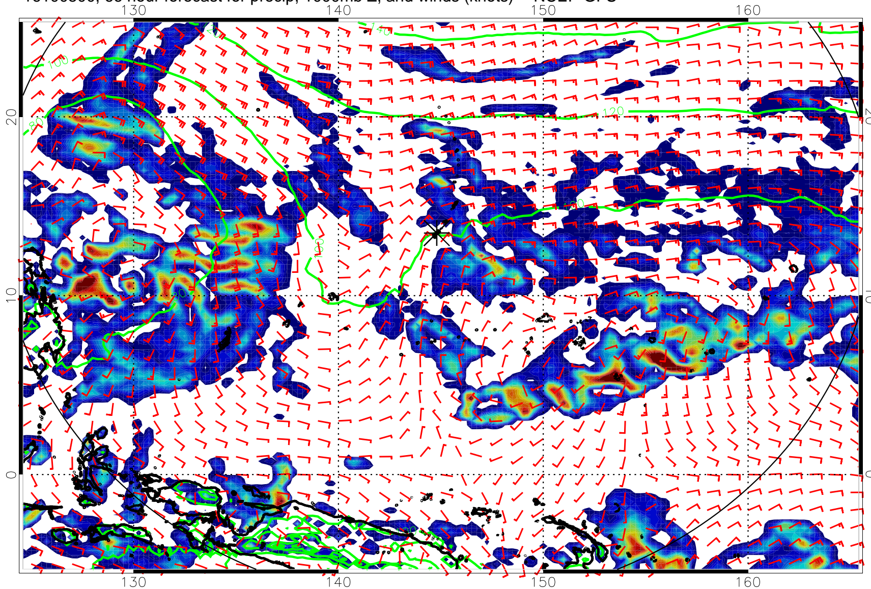
16100500, 66 hour forecast for precip, 1000mb Z, and winds (knots) -- NCEP GFS
