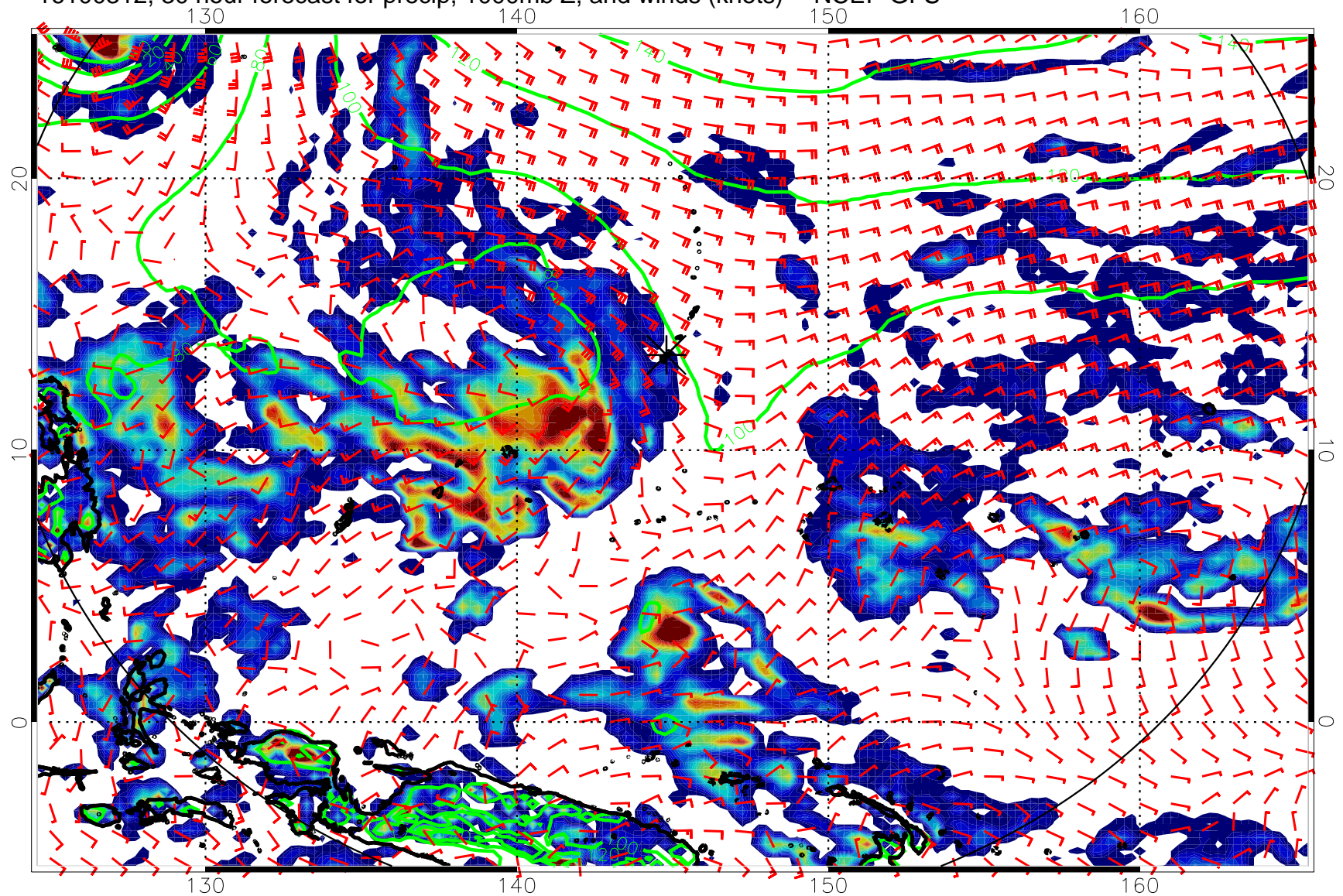
16100312, 30 hour forecast for precip, 1000mb Z, and winds (knots) -- NCEP GFS
