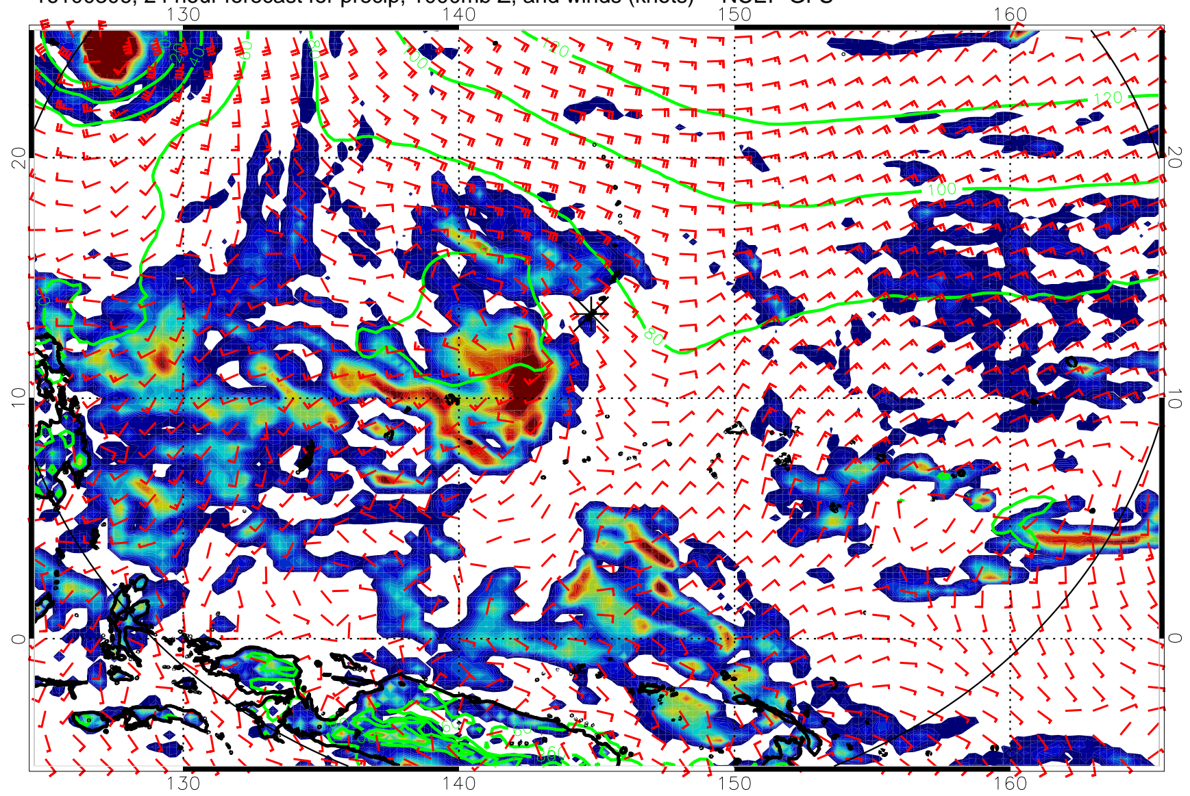
16100306, 24 hour forecast for precip, 1000mb Z, and winds (knots) -- NCEP GFS
