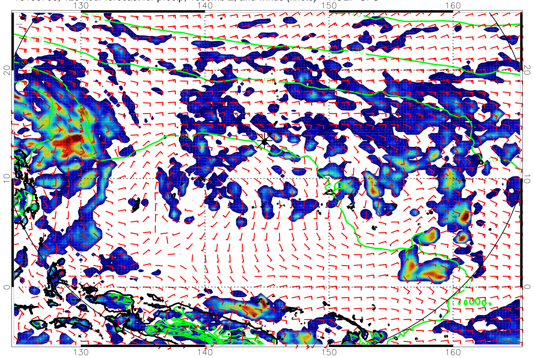
16100706, 120 hour forecast for precip, 1000mb Z, and winds (knots) -- NCEP GFS
