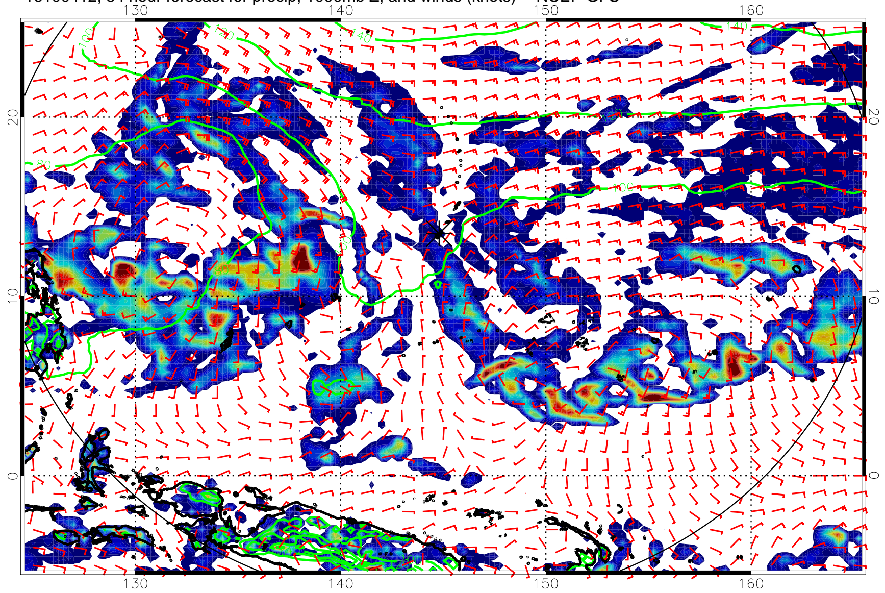
16100412, 54 hour forecast for precip, 1000mb Z, and winds (knots) -- NCEP GFS
