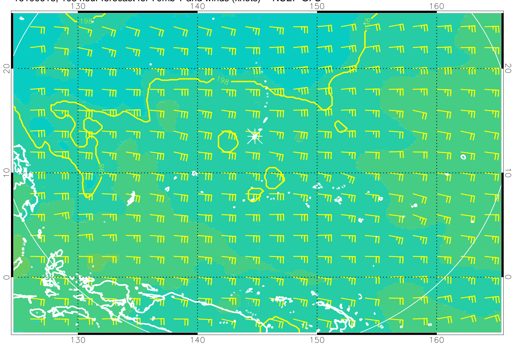
16100618, 108 hour forecast for 70mb T and winds (knots) -- NCEP GFS
