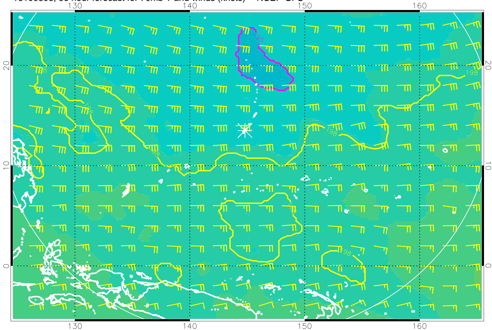
16100606, 96 hour forecast for 70mb T and winds (knots) -- NCEP GFS
