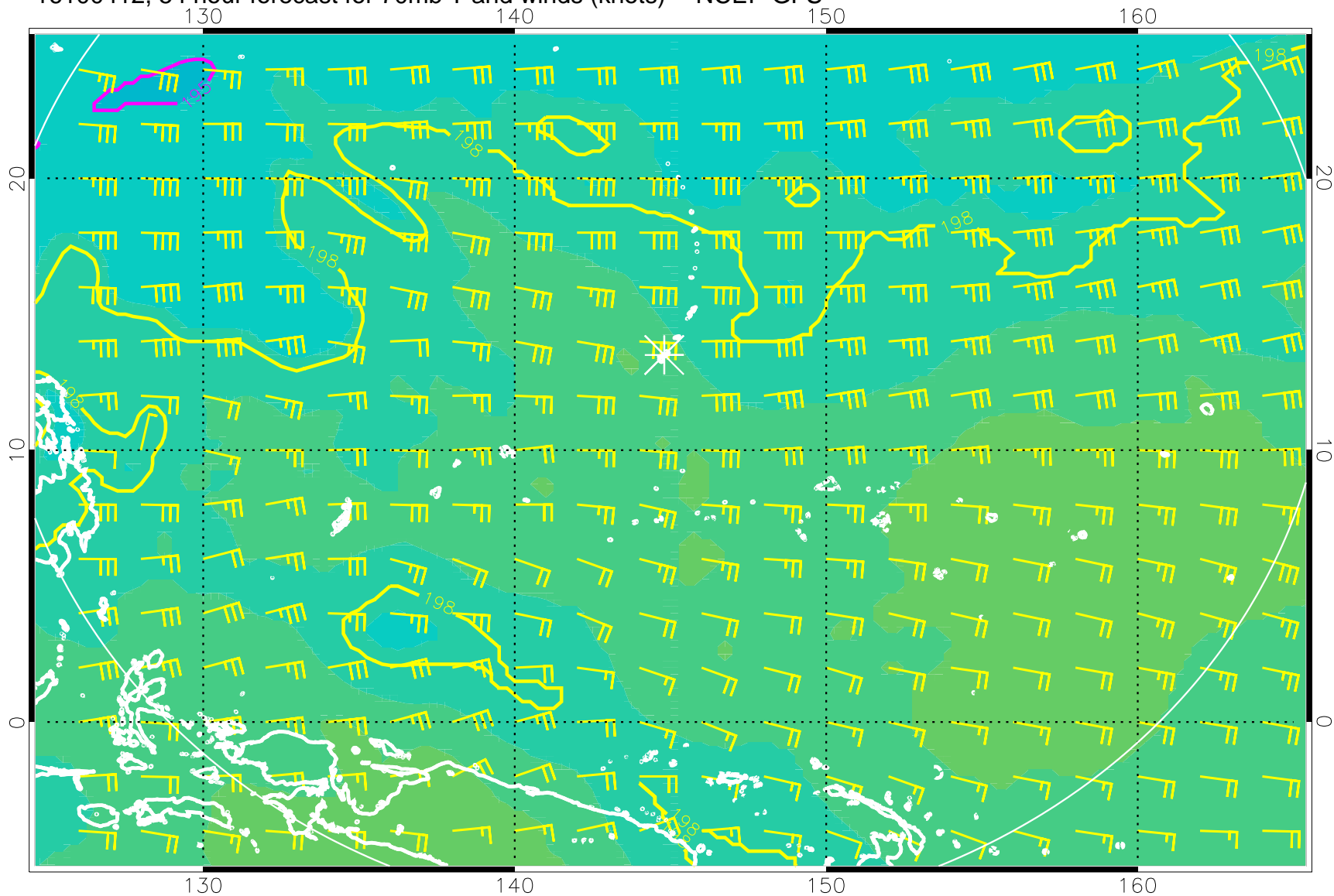
16100412, 54 hour forecast for 70mb T and winds (knots) -- NCEP GFS
