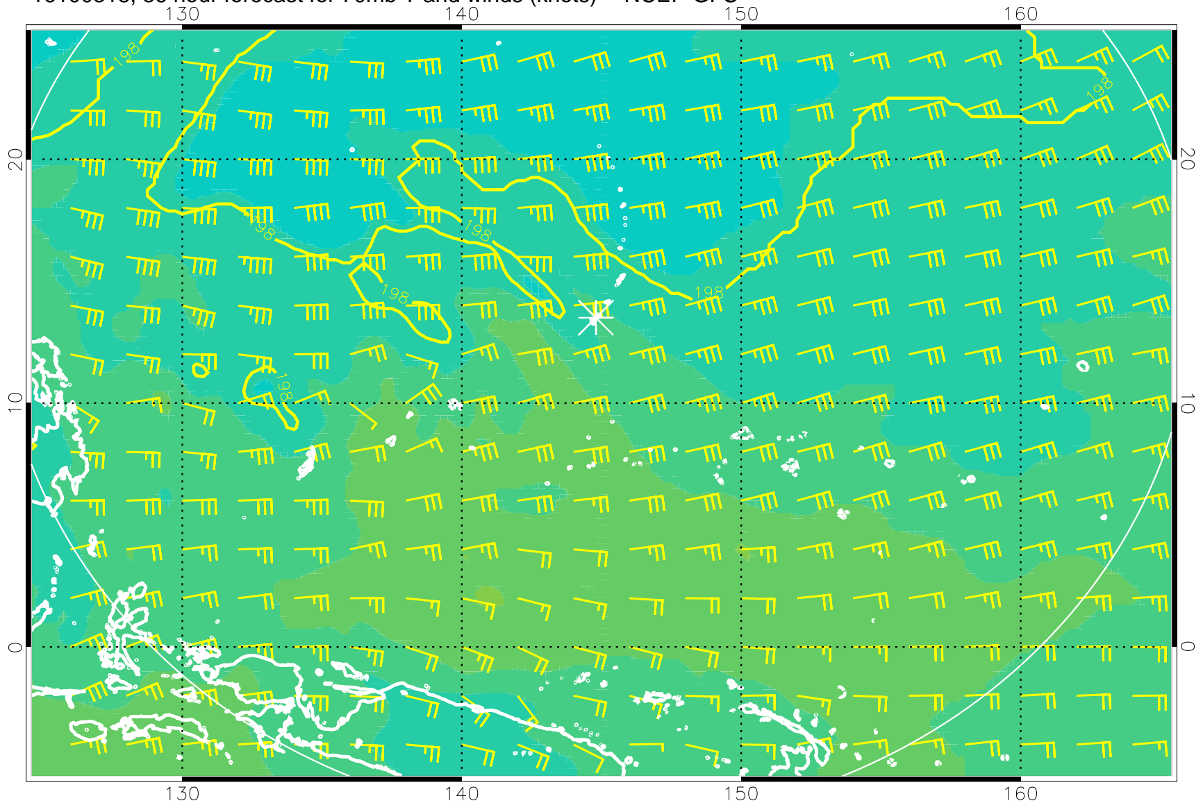
16100318, 36 hour forecast for 70mb T and winds (knots) -- NCEP GFS
