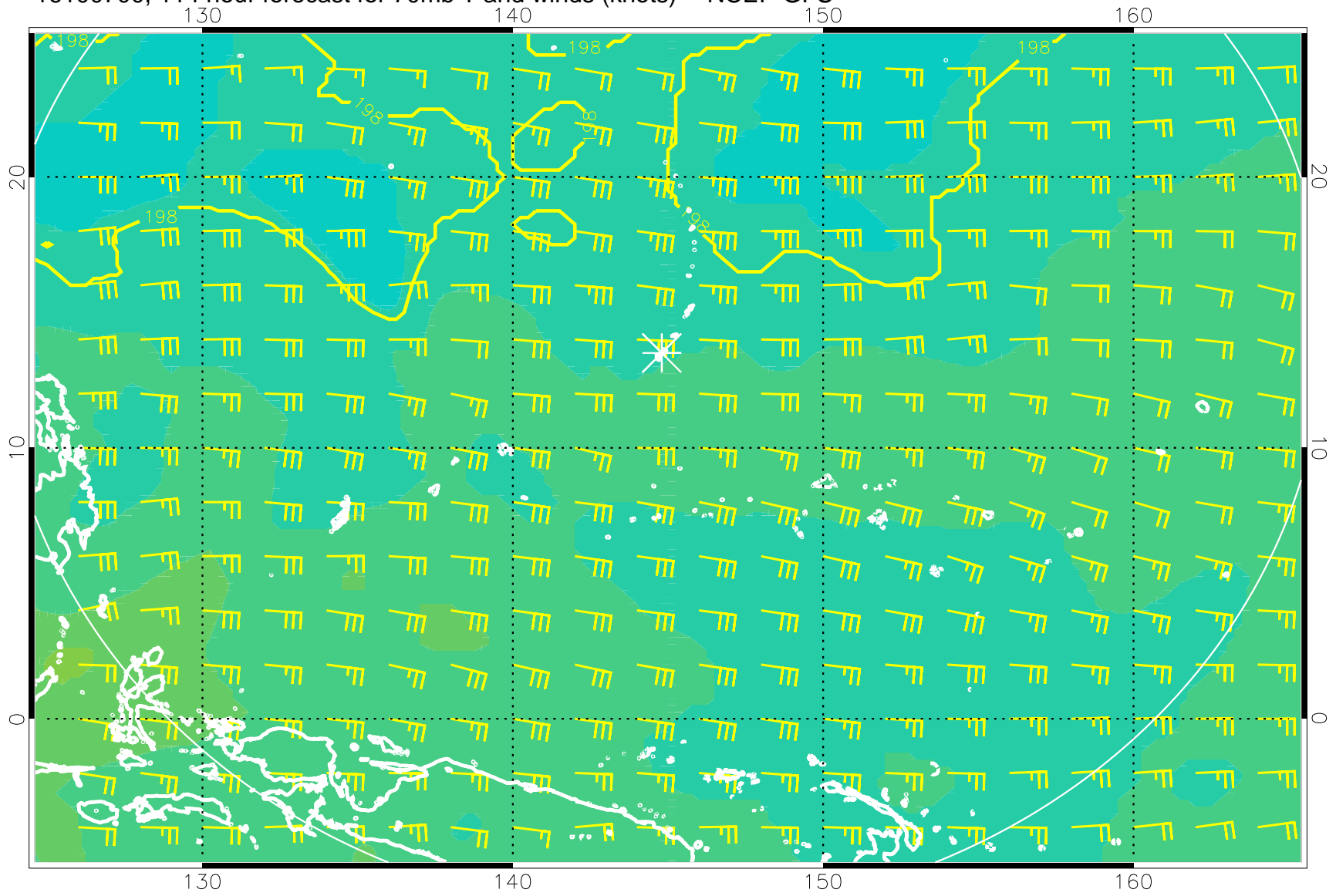
16100700, 114 hour forecast for 70mb T and winds (knots) -- NCEP GFS
