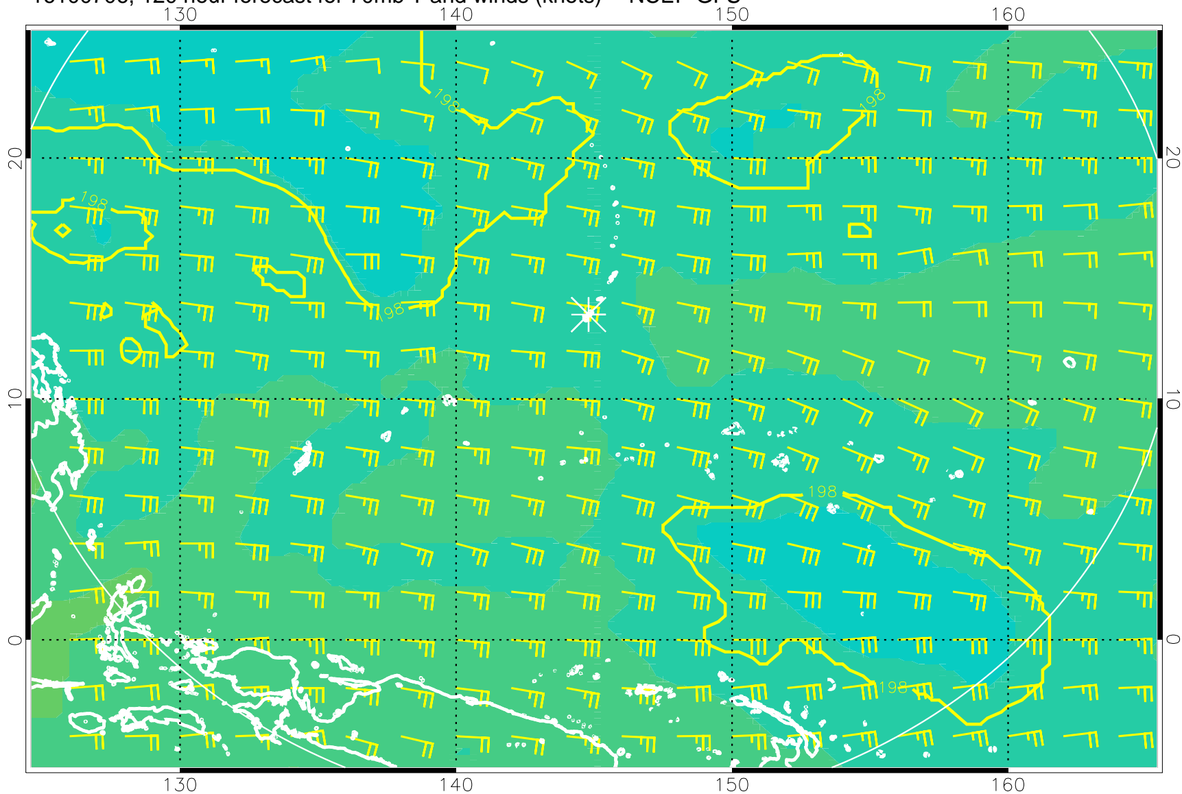
16100706, 120 hour forecast for 70mb T and winds (knots) -- NCEP GFS
