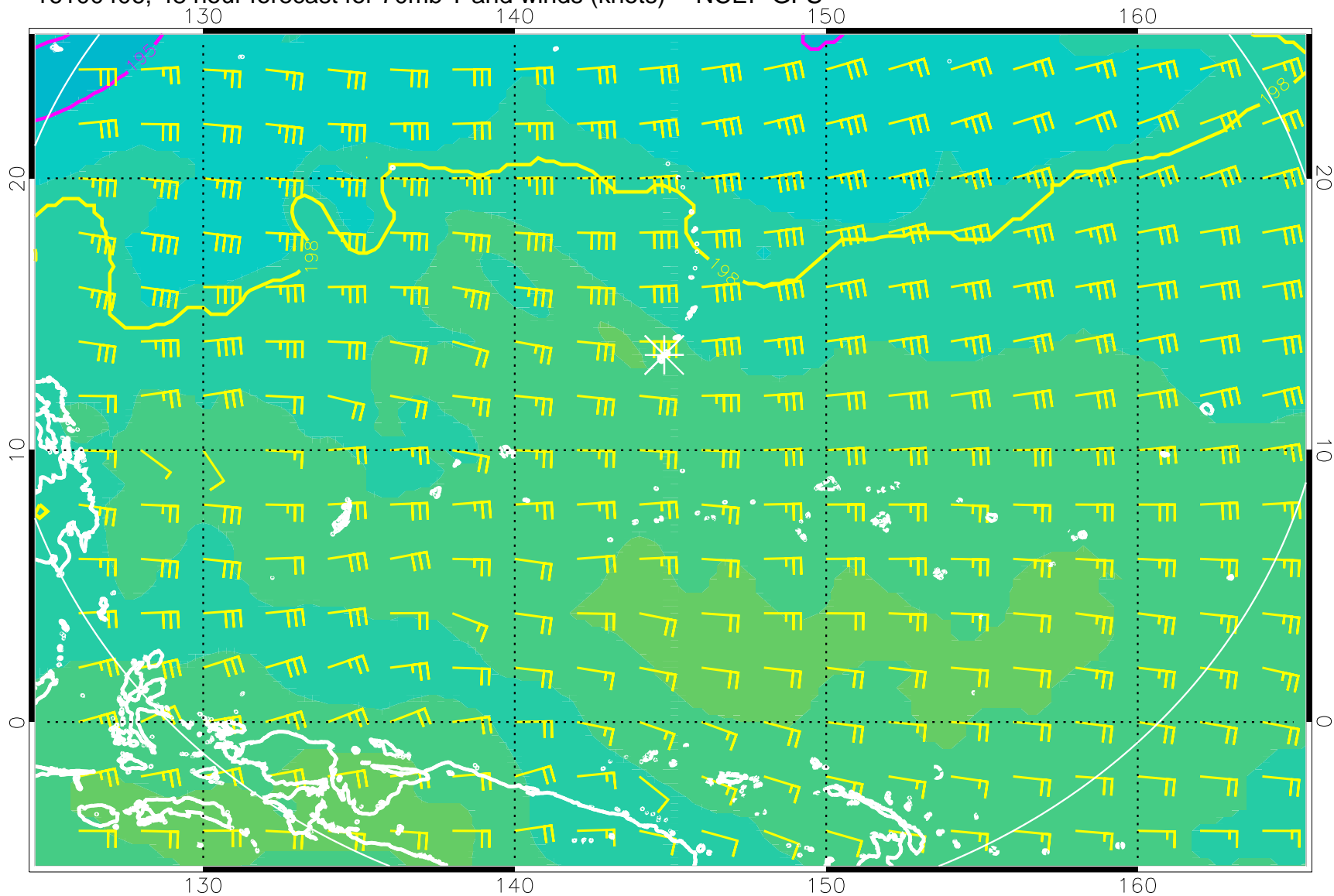
16100406, 48 hour forecast for 70mb T and winds (knots) -- NCEP GFS
