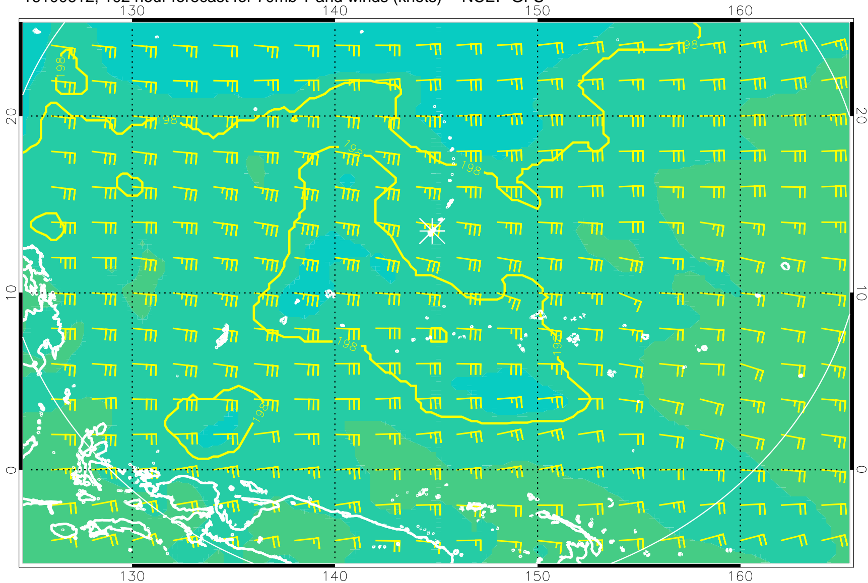
16100612, 102 hour forecast for 70mb T and winds (knots) -- NCEP GFS
