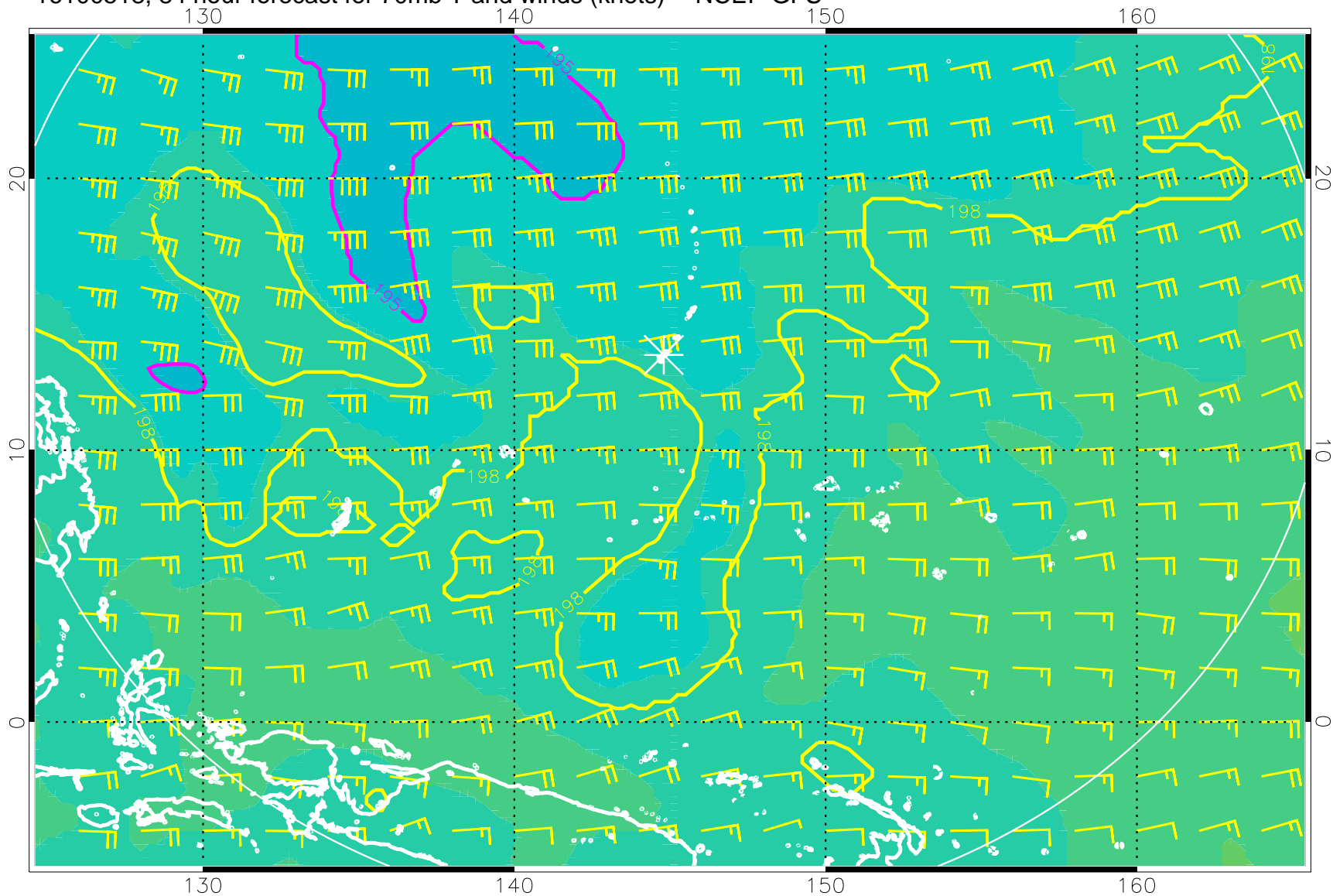
16100518, 84 hour forecast for 70mb T and winds (knots) -- NCEP GFS
