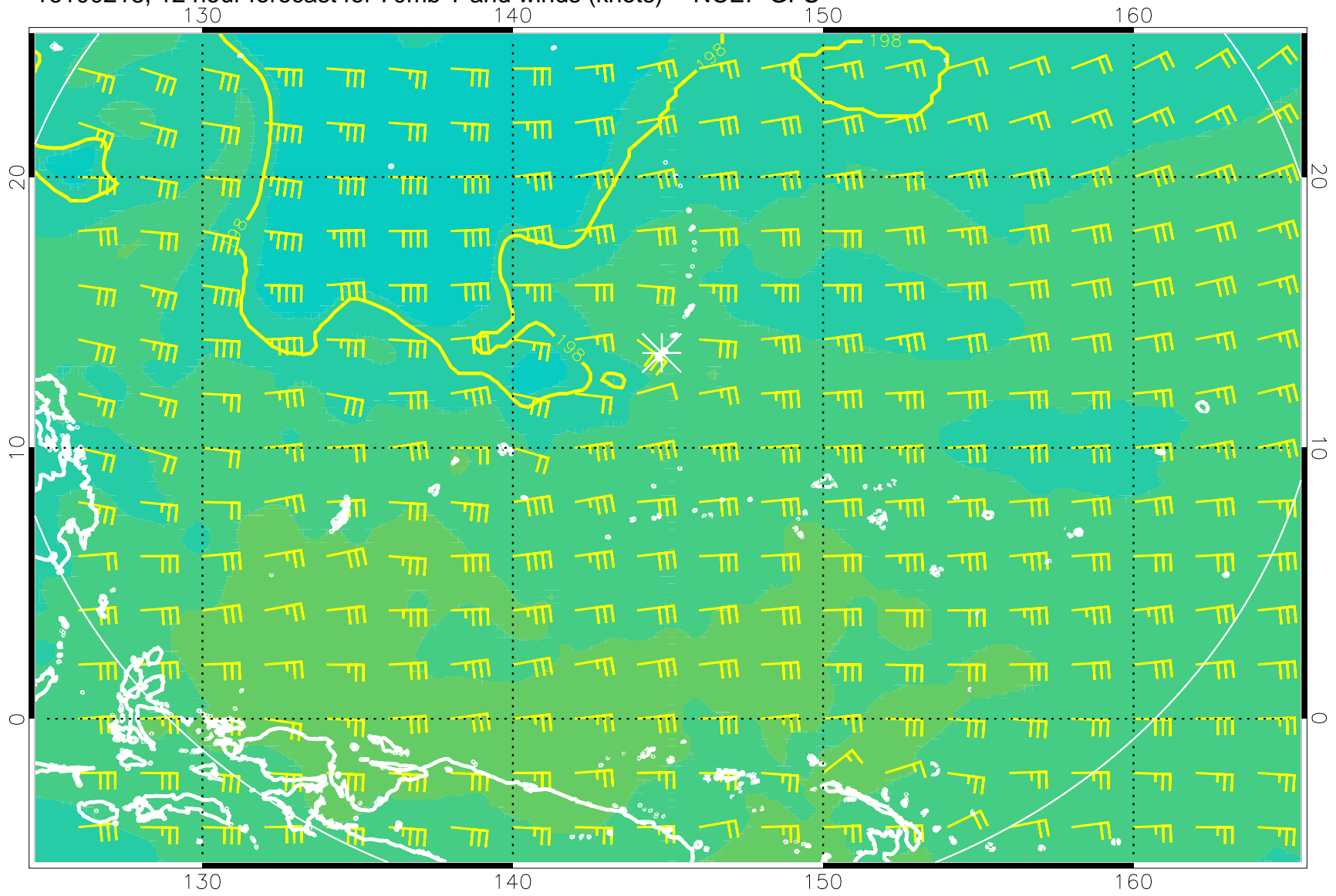
16100218, 12 hour forecast for 70mb T and winds (knots) -- NCEP GFS
