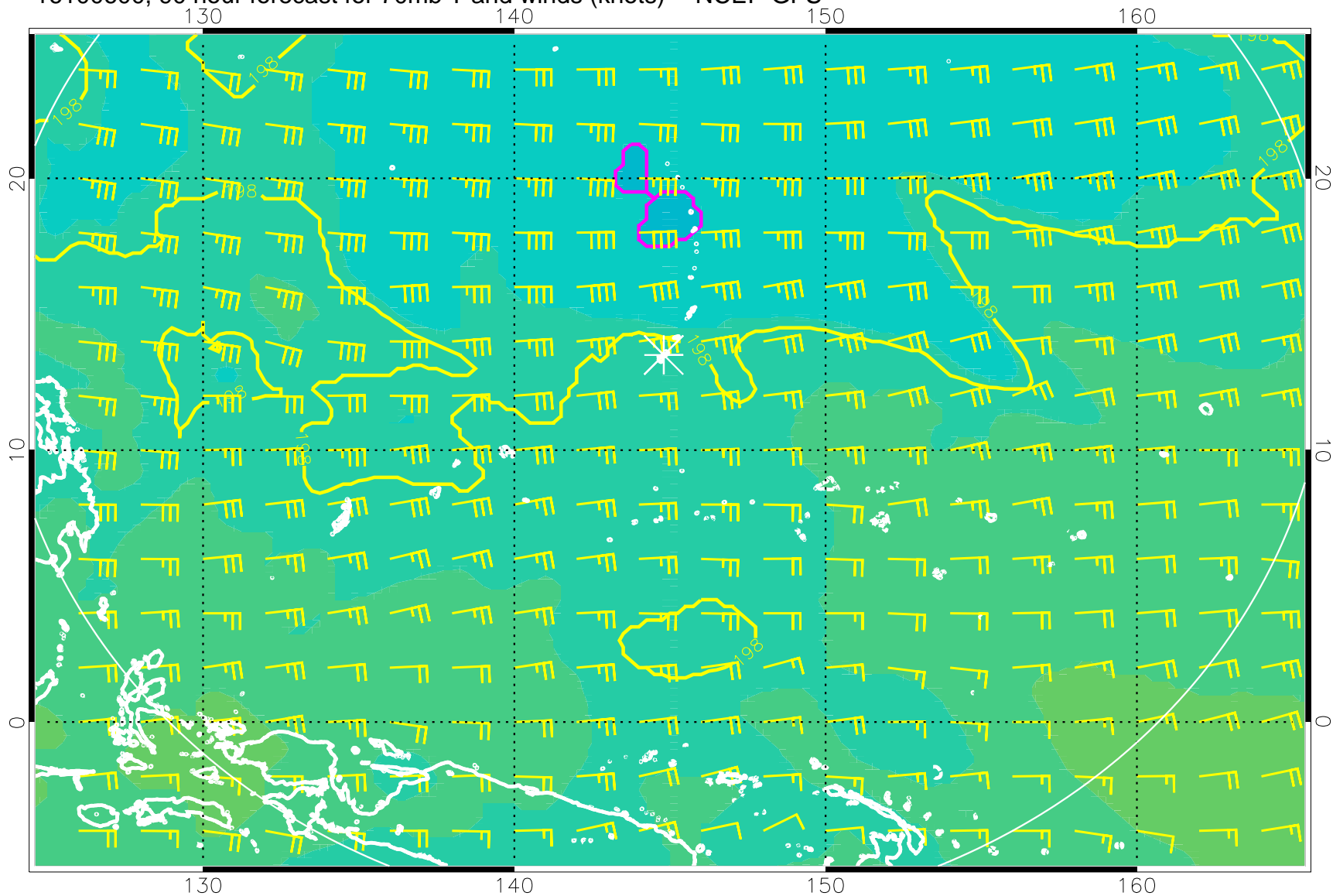
16100600, 90 hour forecast for 70mb T and winds (knots) -- NCEP GFS
