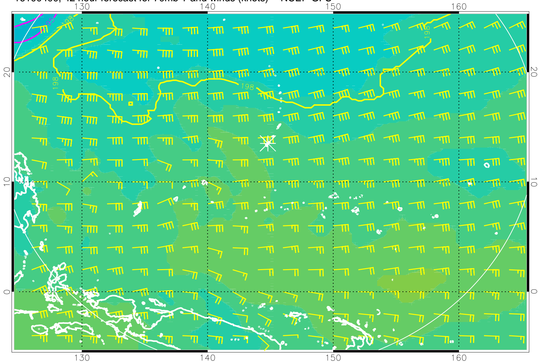
16100400, 42 hour forecast for 70mb T and winds (knots) -- NCEP GFS
