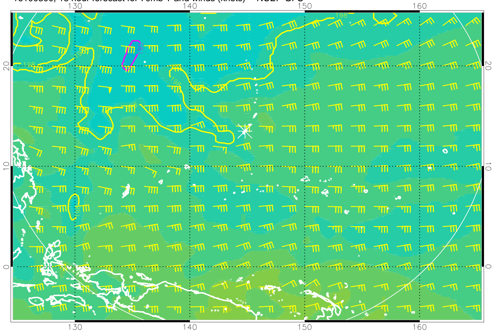
16100300, 18 hour forecast for 70mb T and winds (knots) -- NCEP GFS
