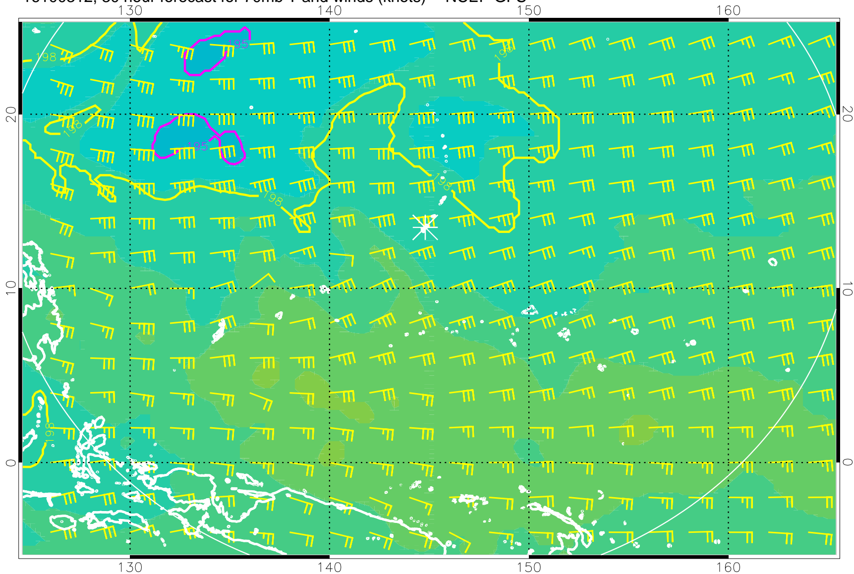
16100312, 30 hour forecast for 70mb T and winds (knots) -- NCEP GFS
