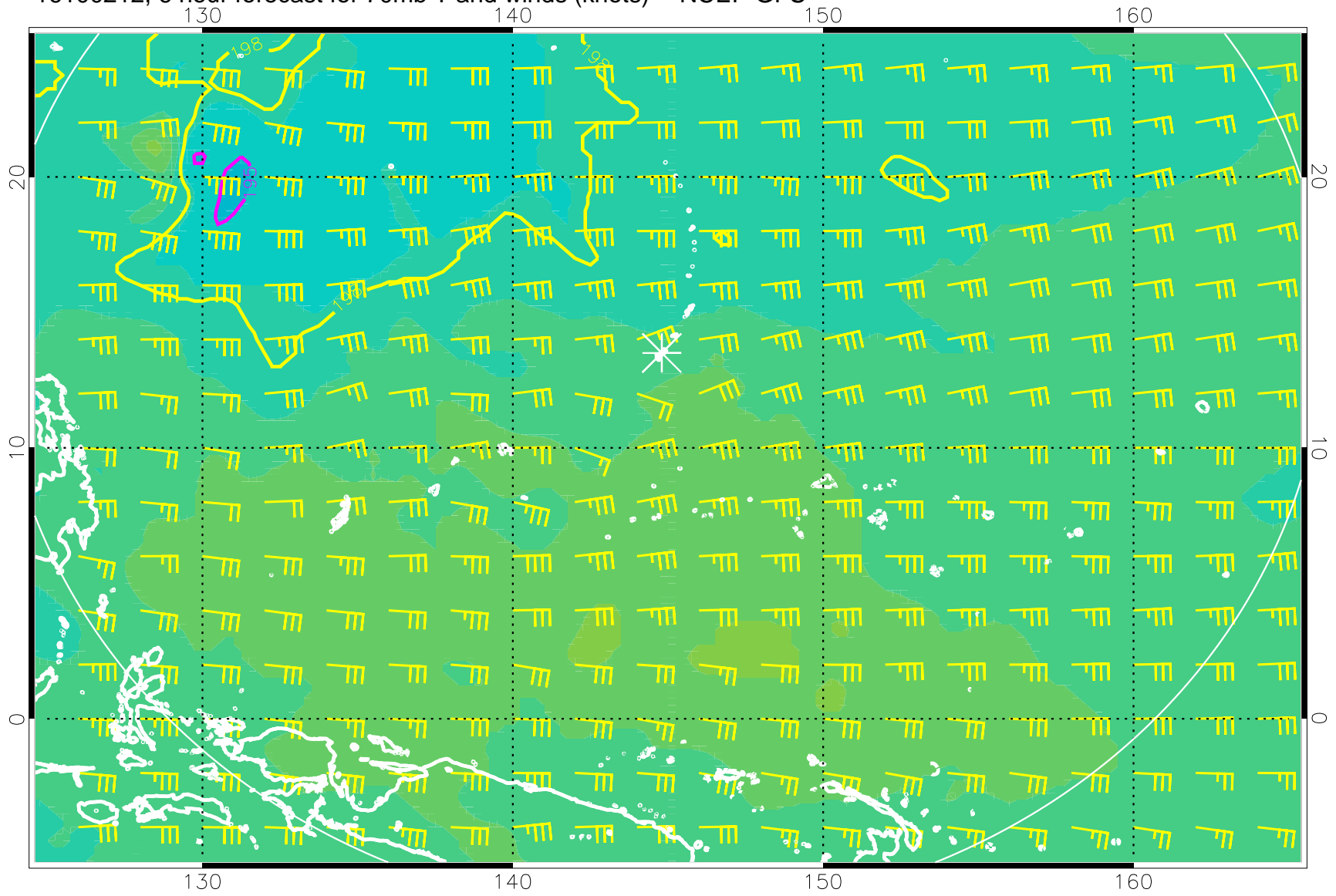
16100212, 6 hour forecast for 70mb T and winds (knots) -- NCEP GFS
