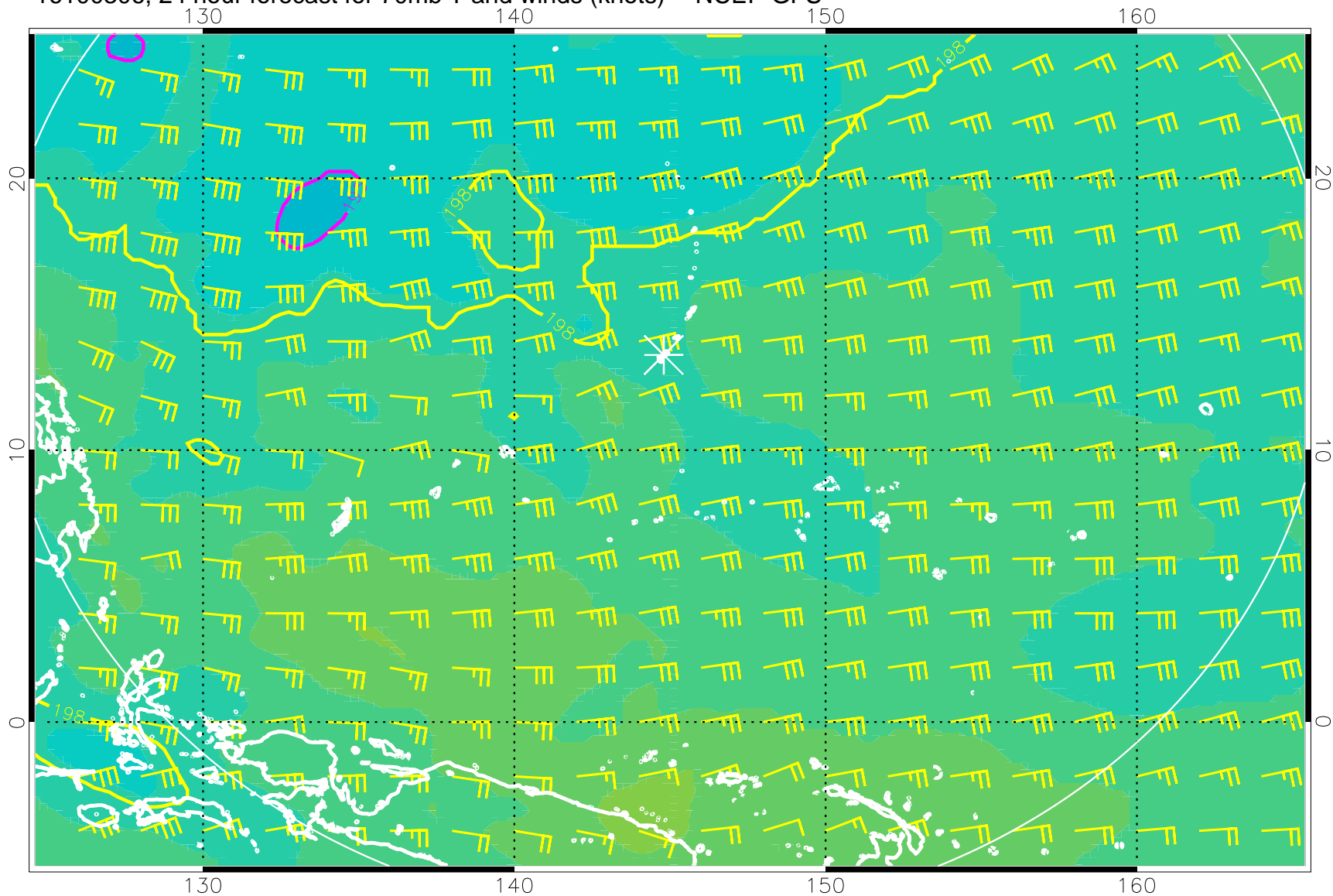
16100306, 24 hour forecast for 70mb T and winds (knots) -- NCEP GFS
