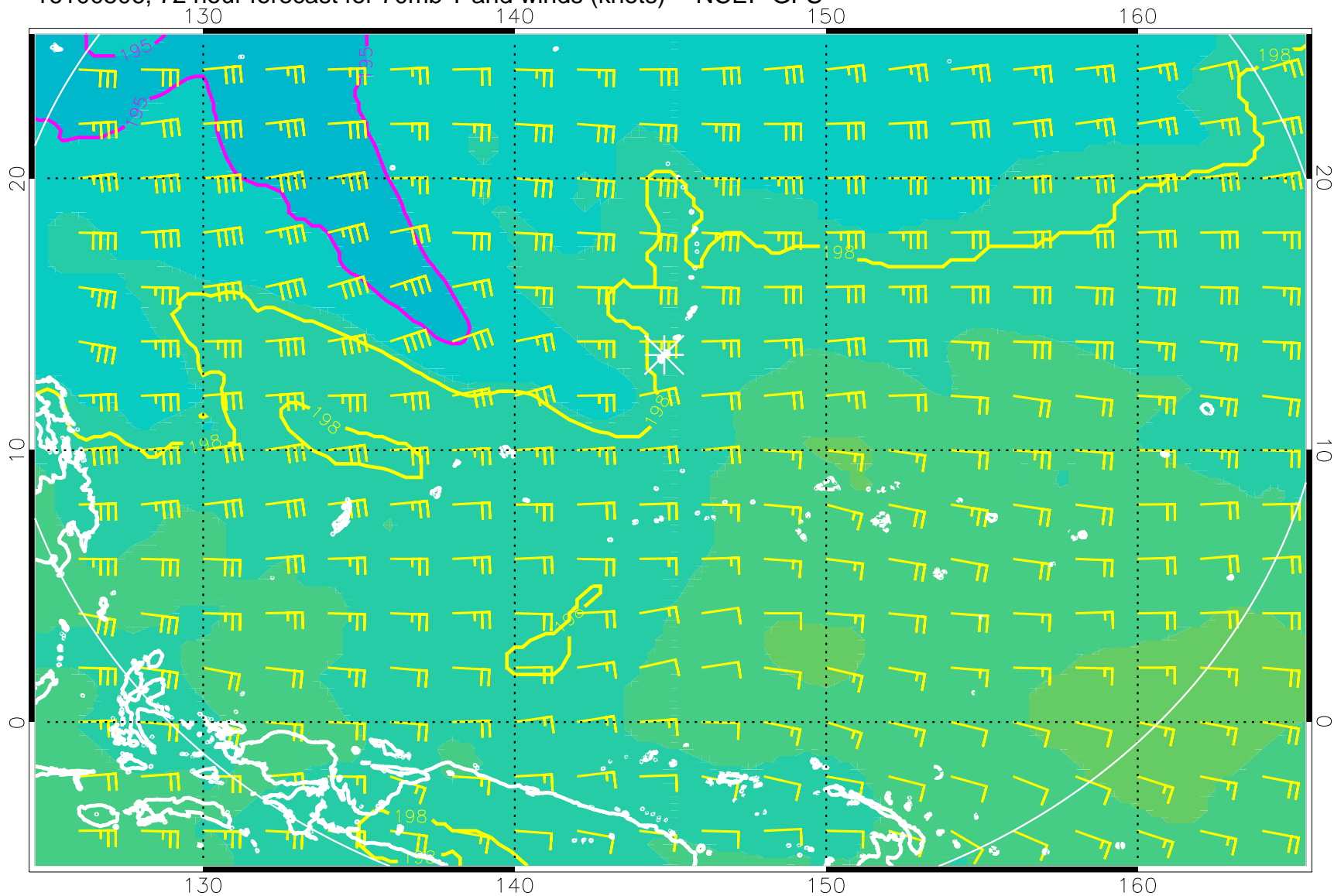
16100506, 72 hour forecast for 70mb T and winds (knots) -- NCEP GFS
