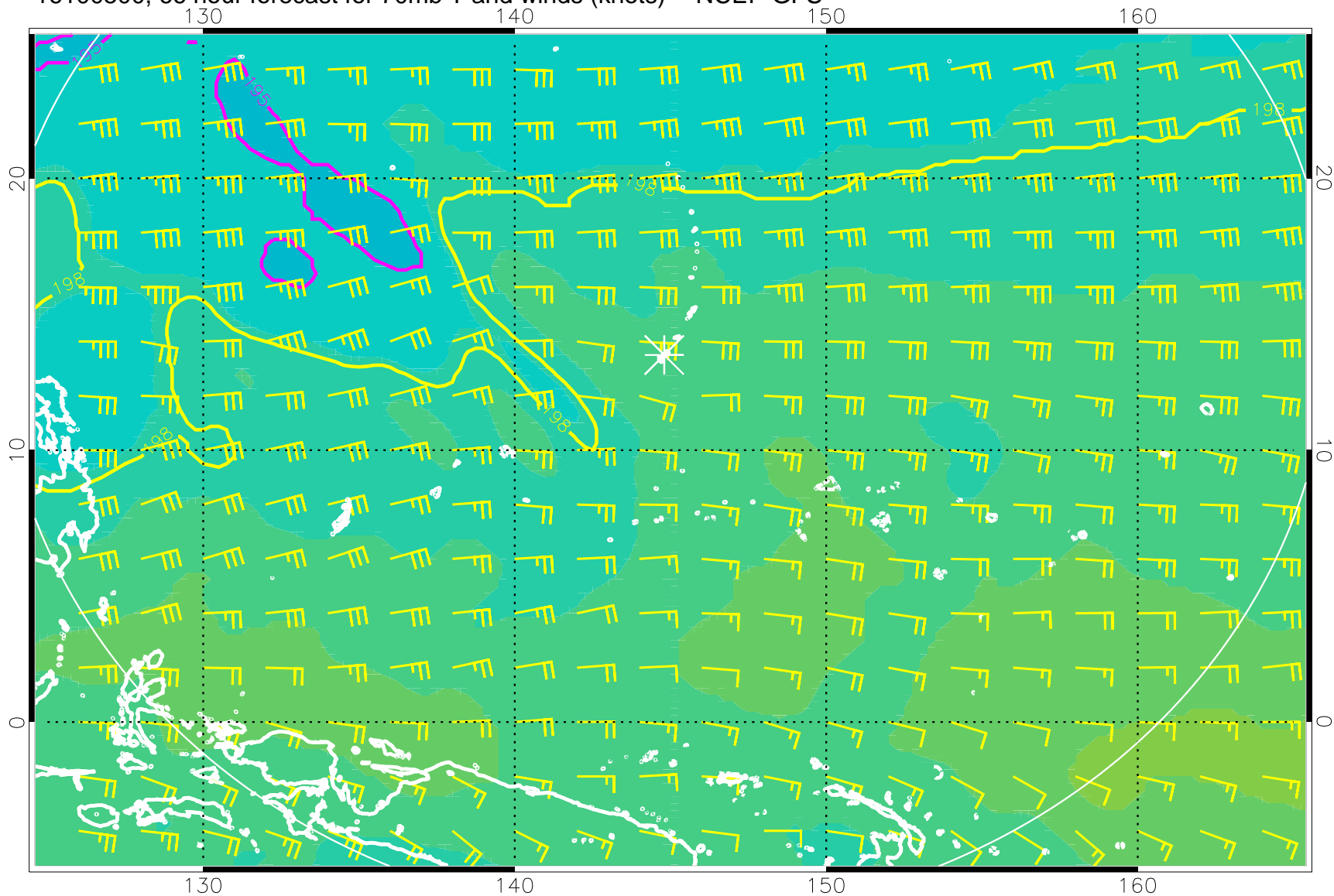
16100500, 66 hour forecast for 70mb T and winds (knots) -- NCEP GFS
