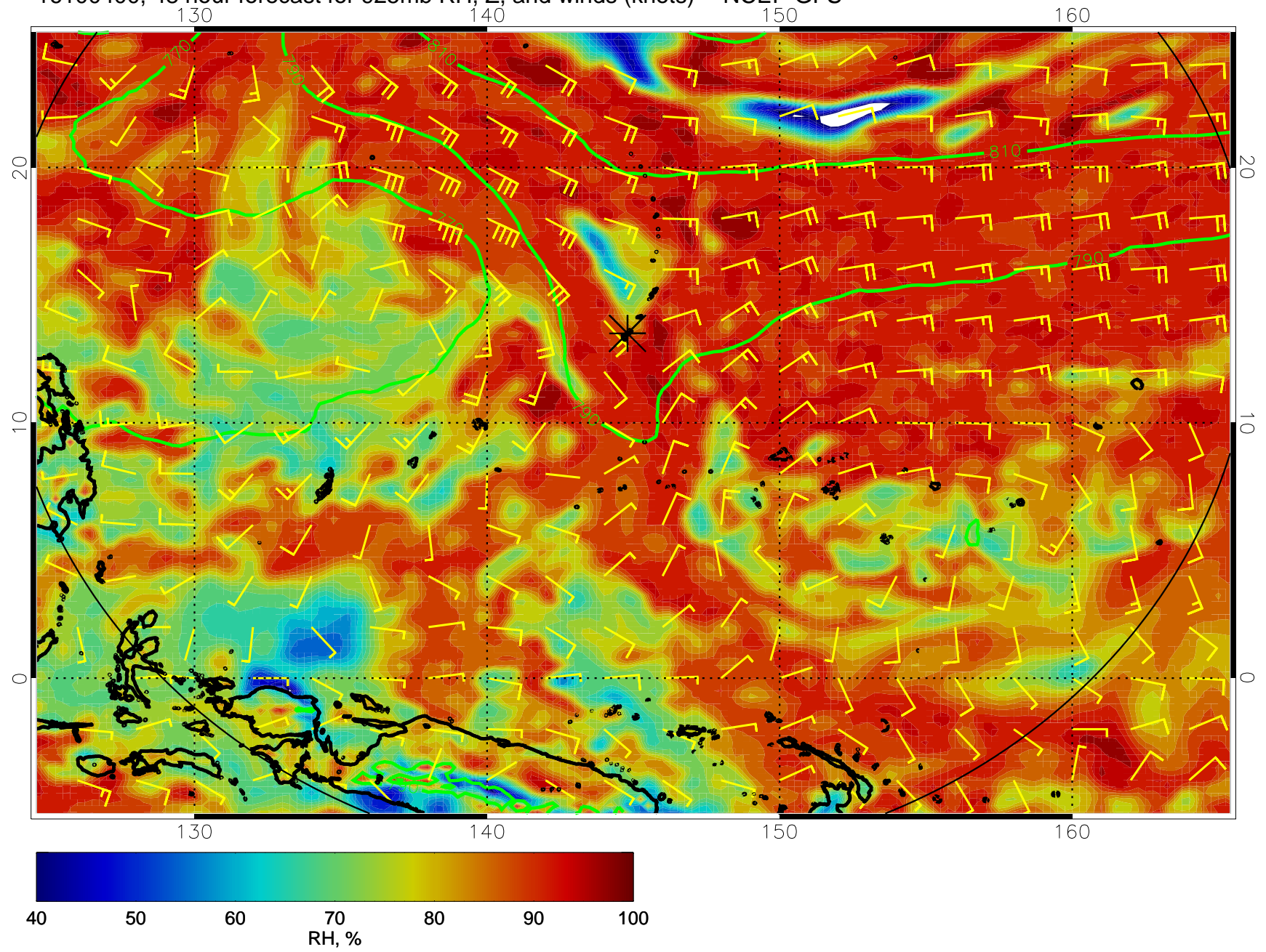
16100400, 48 hour forecast for 925mb RH, Z, and winds (knots) -- NCEP GFS
