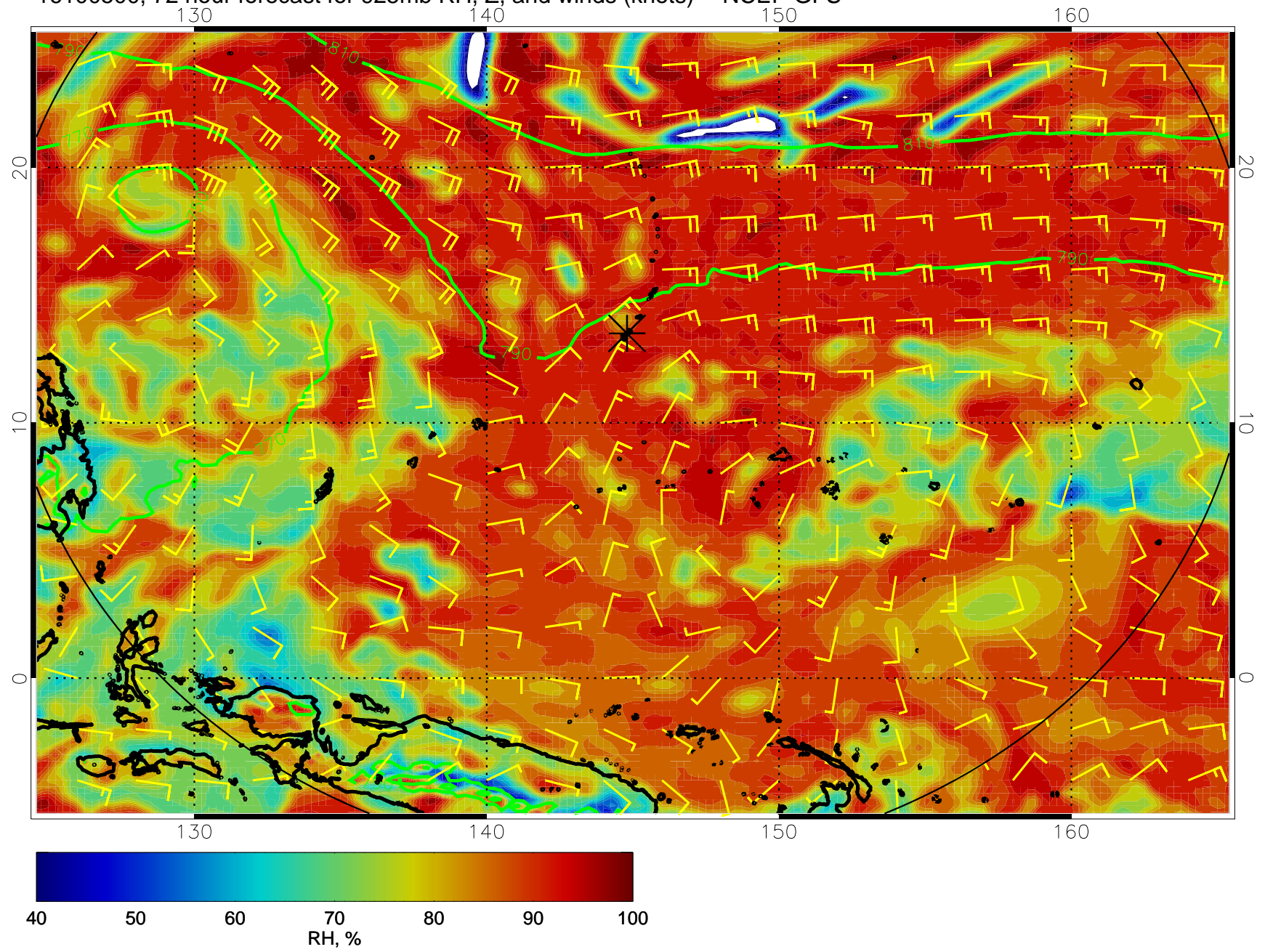
16100500, 72 hour forecast for 925mb RH, Z, and winds (knots) -- NCEP GFS
