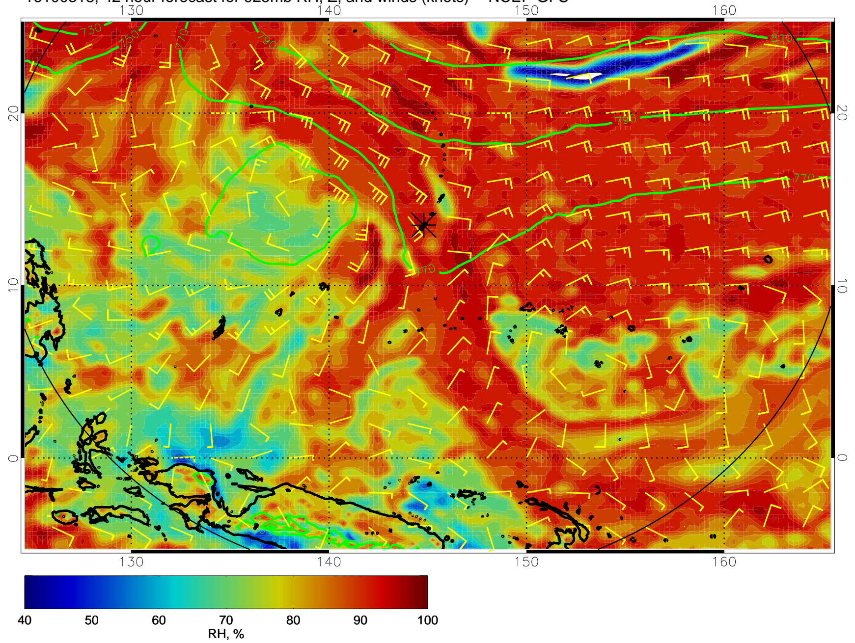
16100318, 42 hour forecast for 925mb RH, Z, and winds (knots) -- NCEP GFS
