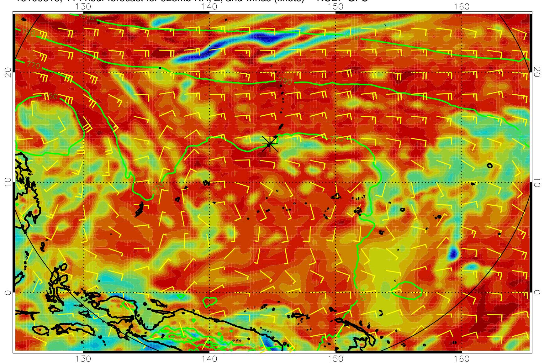
16100618, 114 hour forecast for 925mb RH, Z, and winds (knots) -- NCEP GFS
