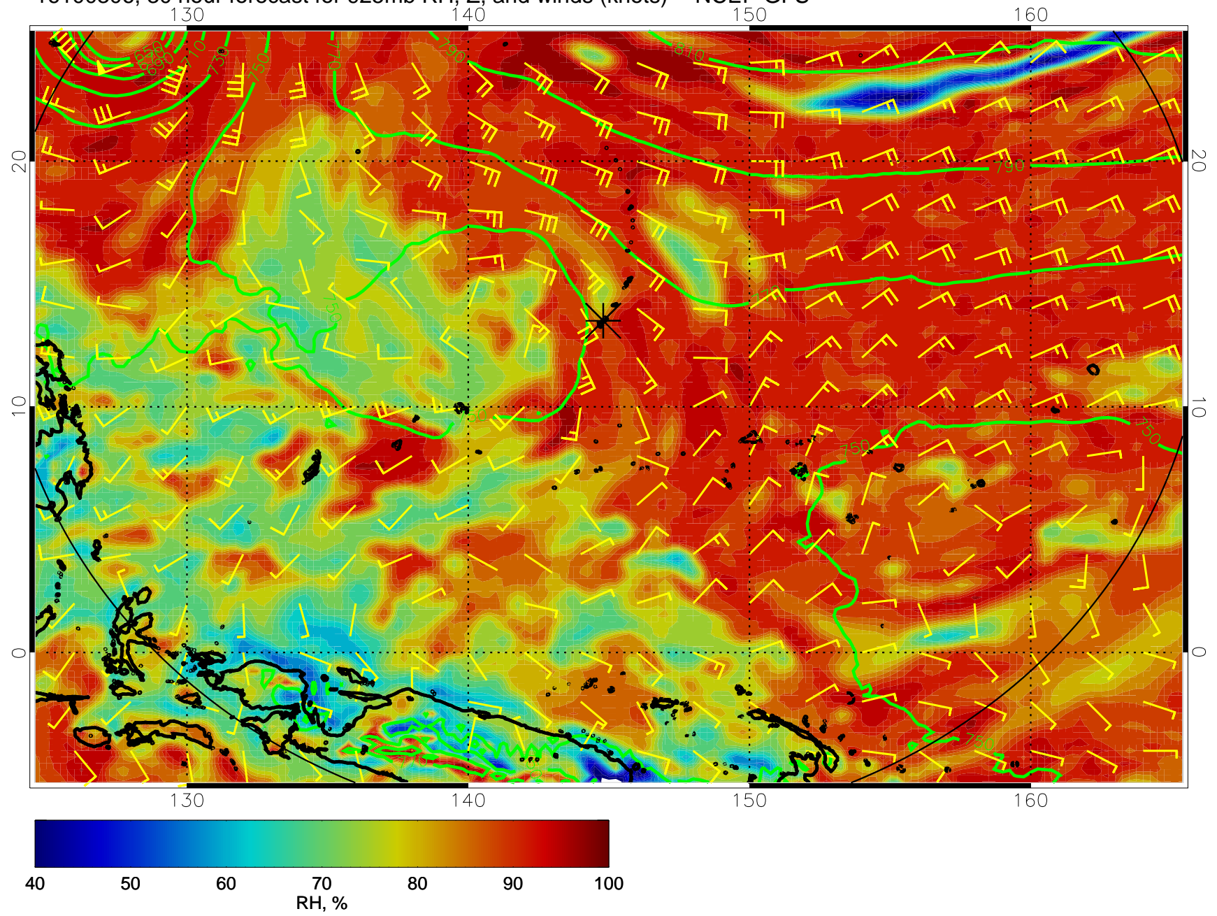
16100306, 30 hour forecast for 925mb RH, Z, and winds (knots) -- NCEP GFS
