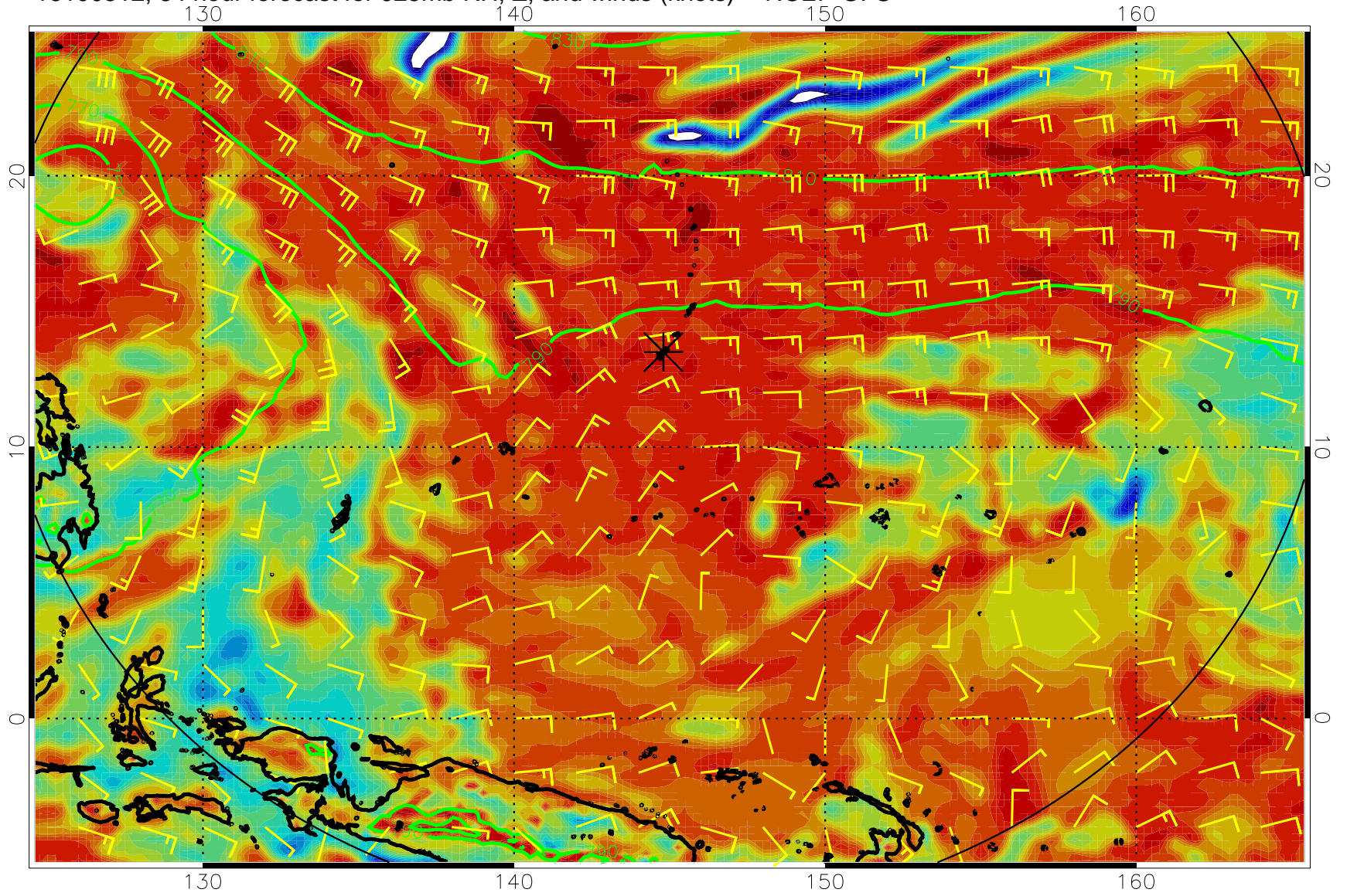
16100512, 84 hour forecast for 925mb RH, Z, and winds (knots) -- NCEP GFS
