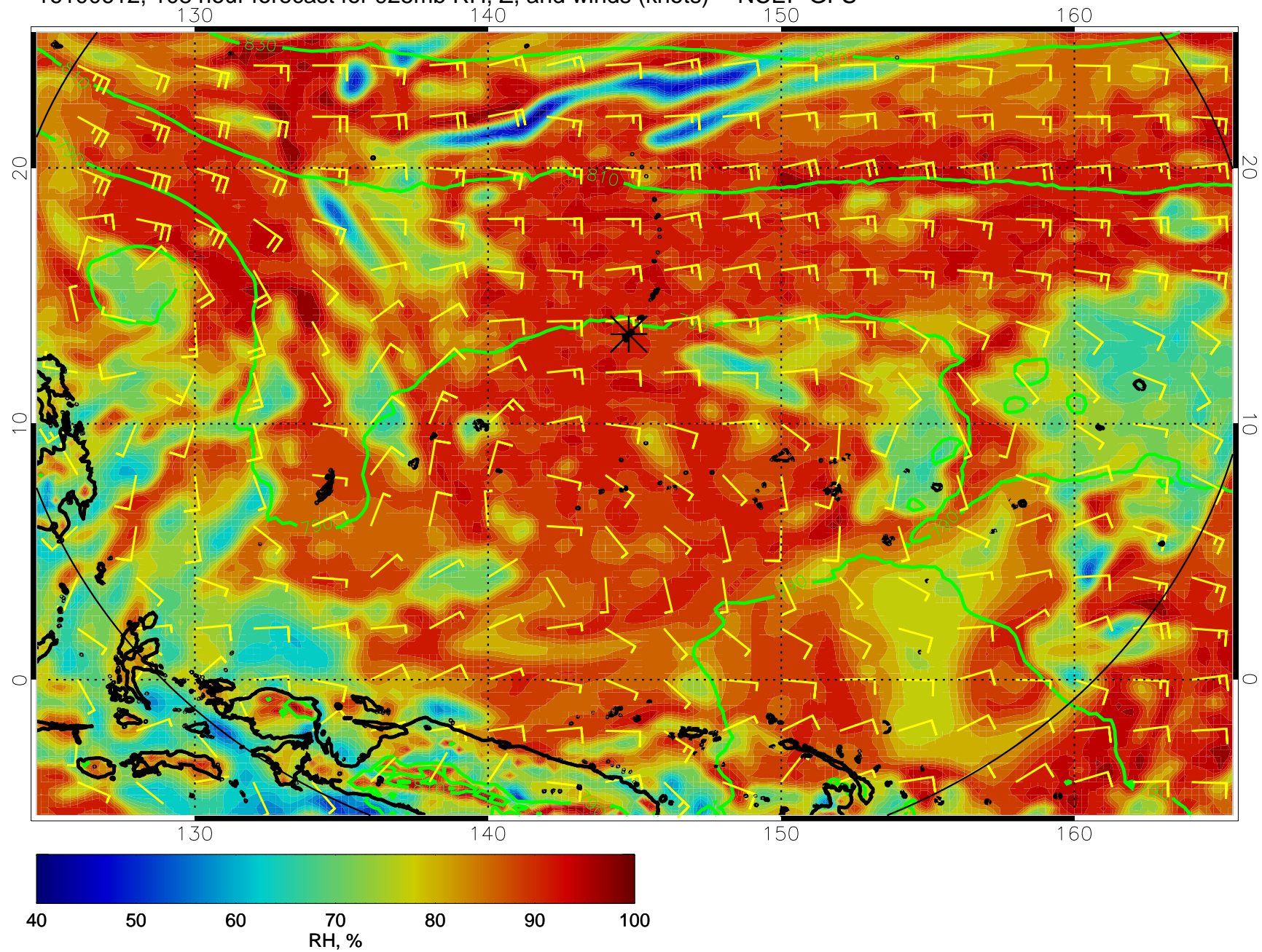
16100612, 108 hour forecast for 925mb RH, Z, and winds (knots) -- NCEP GFS
