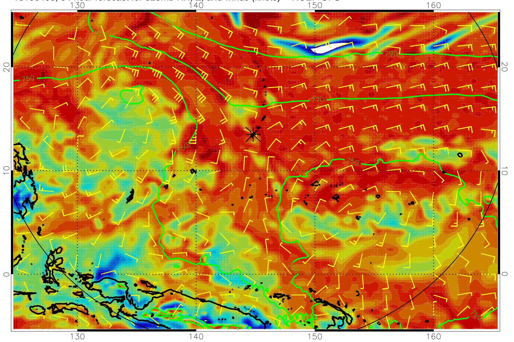
16100406, 54 hour forecast for 925mb RH, Z, and winds (knots) -- NCEP GFS
