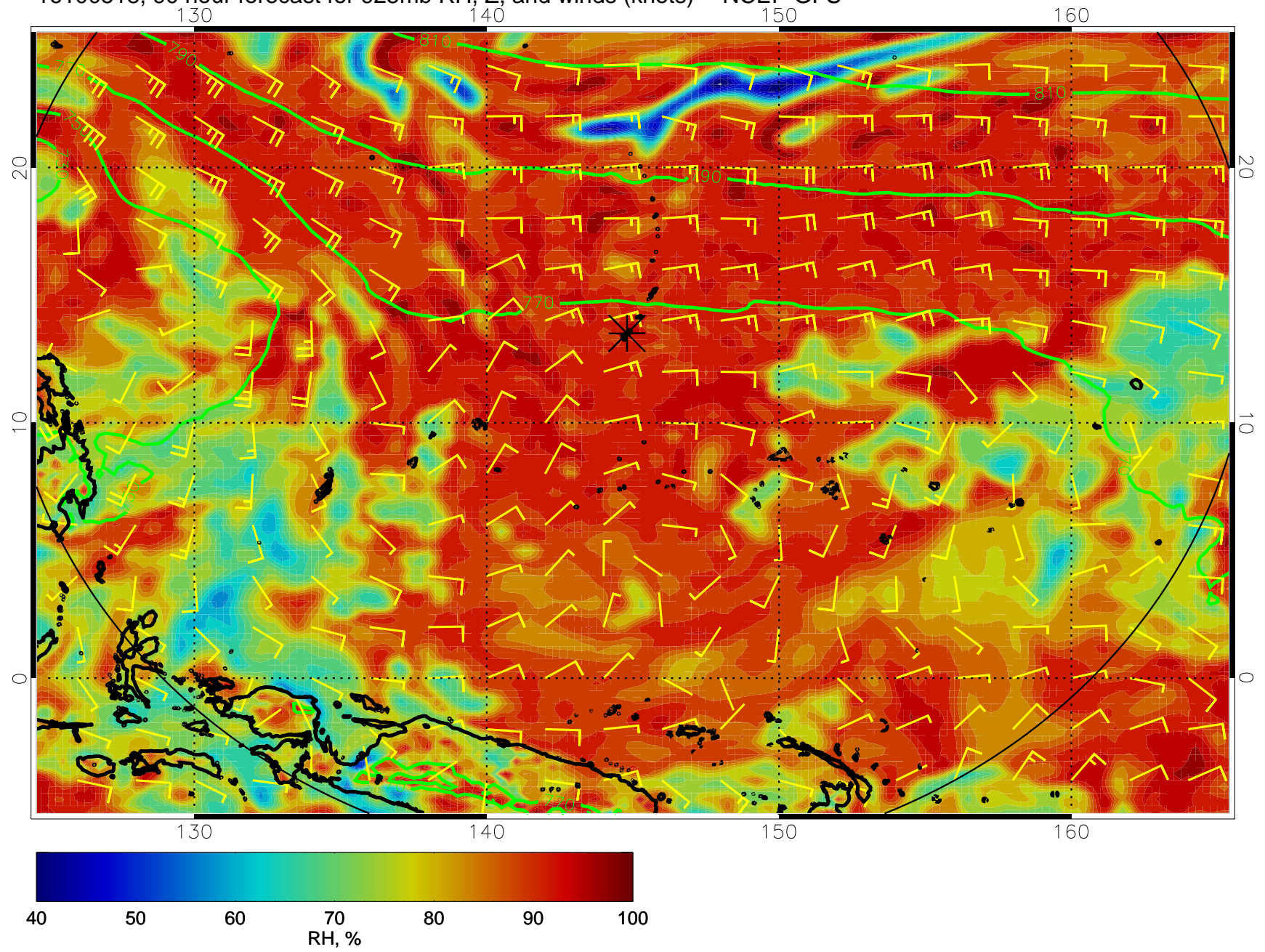
16100518, 90 hour forecast for 925mb RH, Z, and winds (knots) -- NCEP GFS
