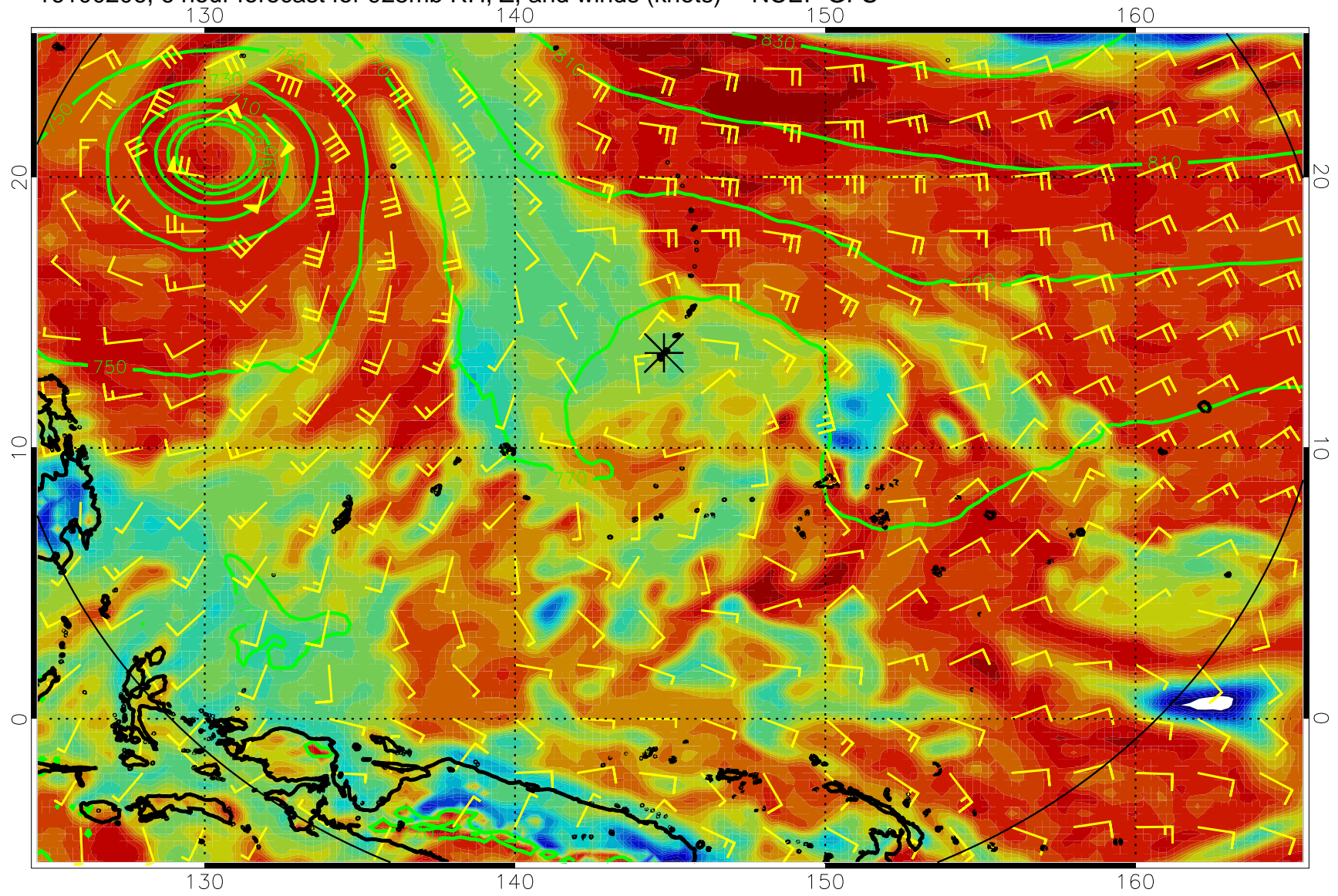
16100206, 6 hour forecast for 925mb RH, Z, and winds (knots) -- NCEP GFS
