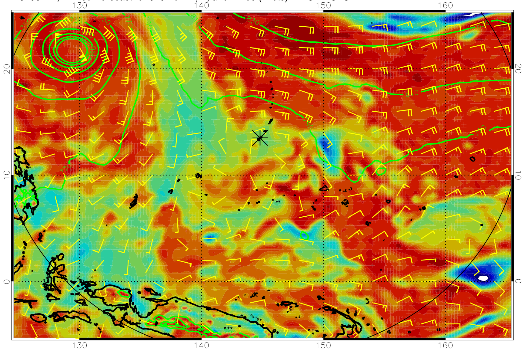
16100212, 12 hour forecast for 925mb RH, Z, and winds (knots) -- NCEP GFS
