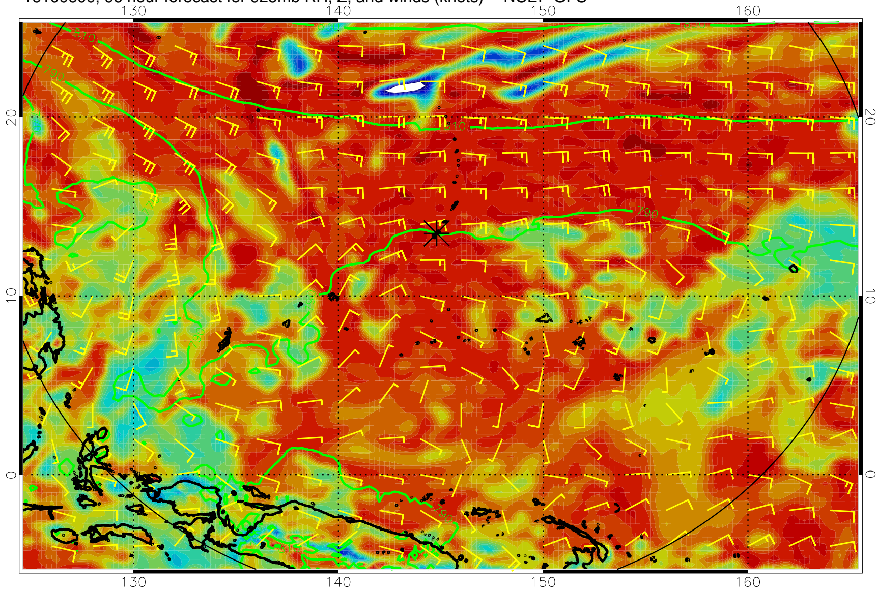
16100600, 96 hour forecast for 925mb RH, Z, and winds (knots) -- NCEP GFS
