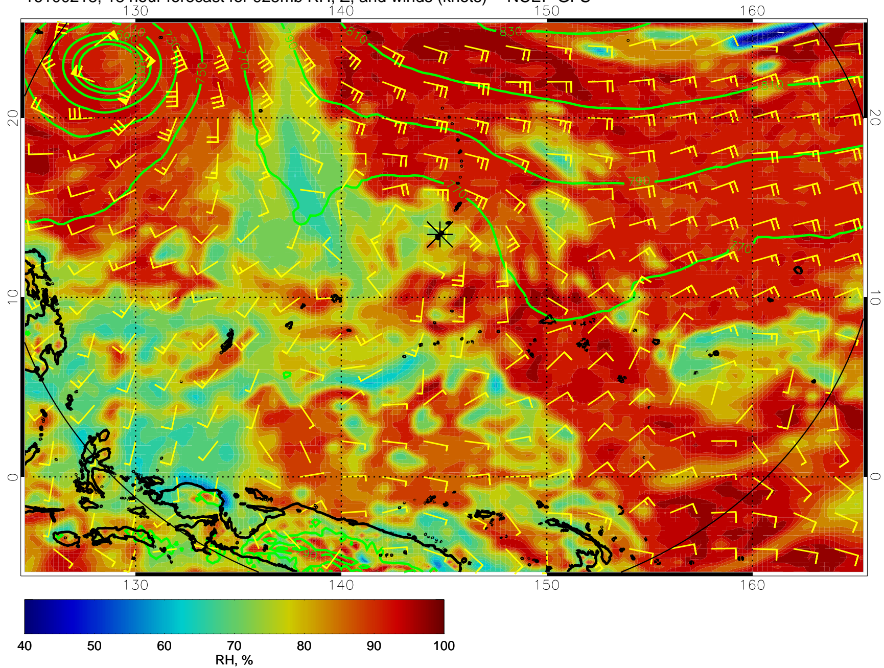
16100218, 18 hour forecast for 925mb RH, Z, and winds (knots) -- NCEP GFS
