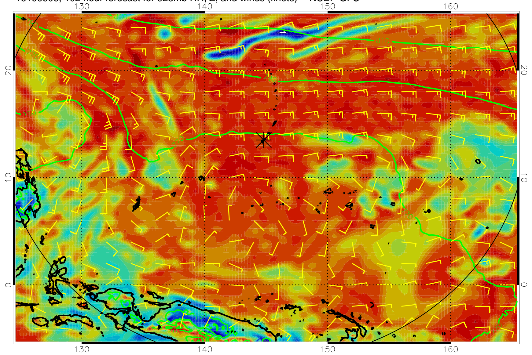
16100606, 102 hour forecast for 925mb RH, Z, and winds (knots) -- NCEP GFS
