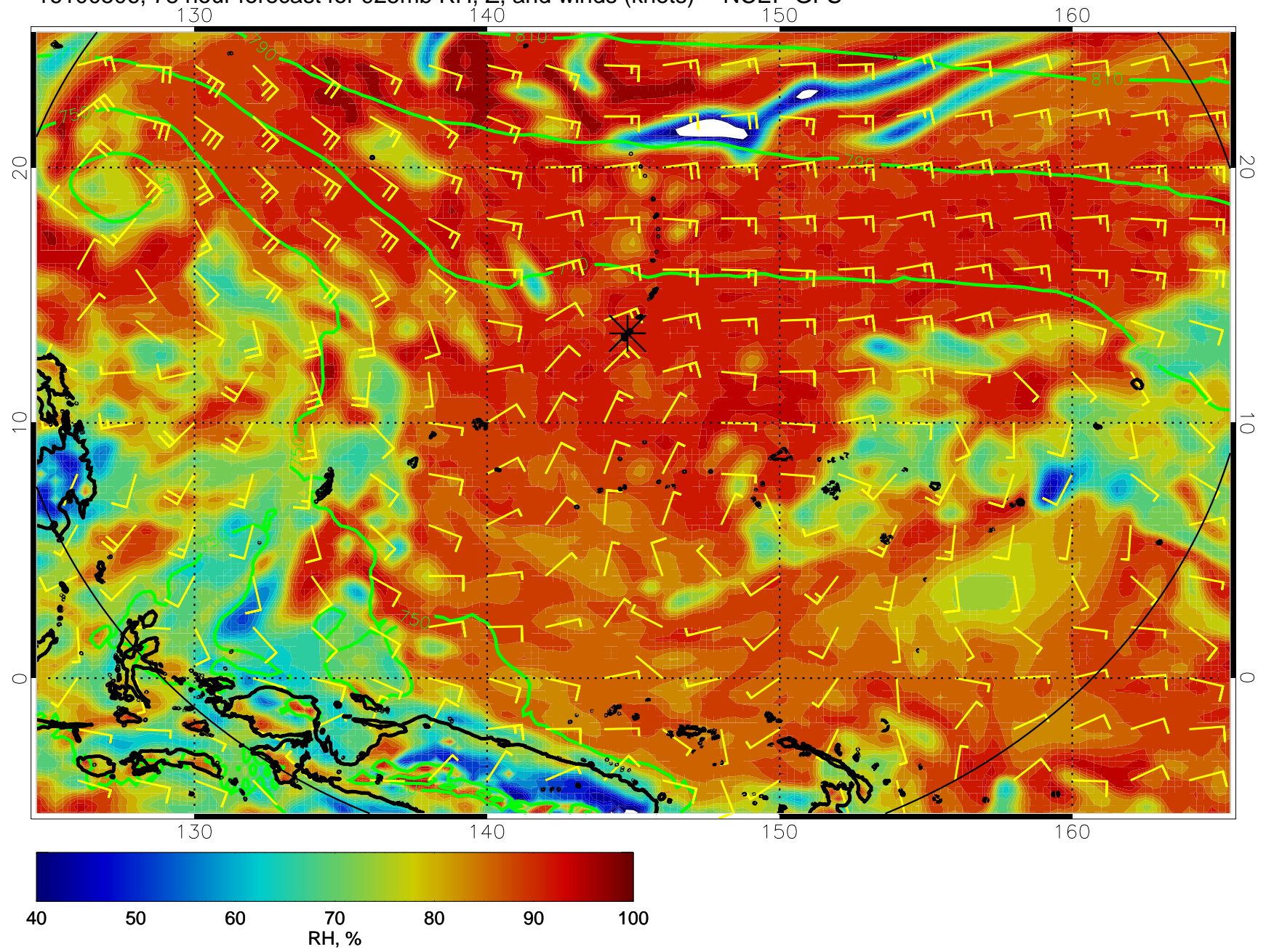
16100506, 78 hour forecast for 925mb RH, Z, and winds (knots) -- NCEP GFS
