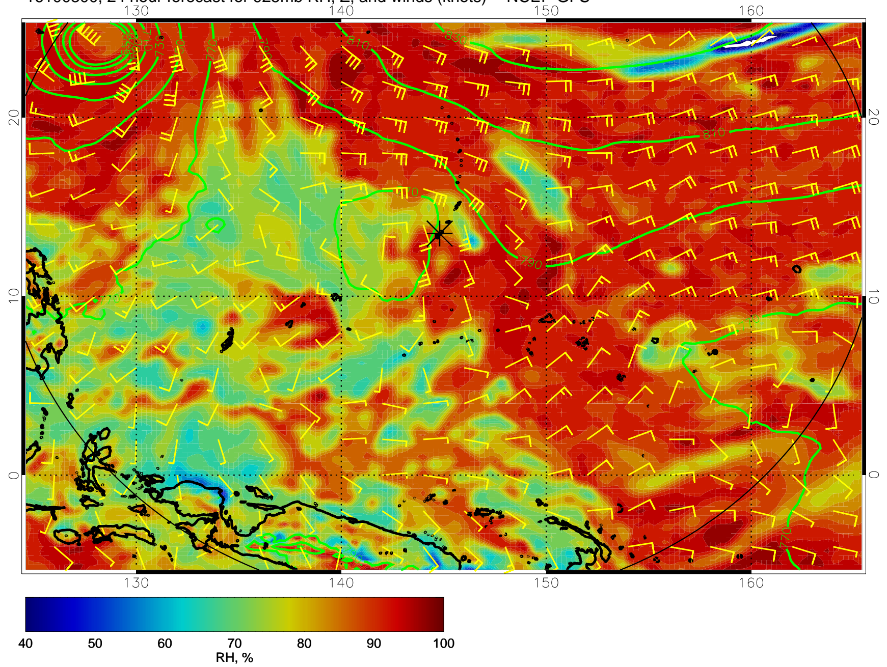
16100300, 24 hour forecast for 925mb RH, Z, and winds (knots) -- NCEP GFS
