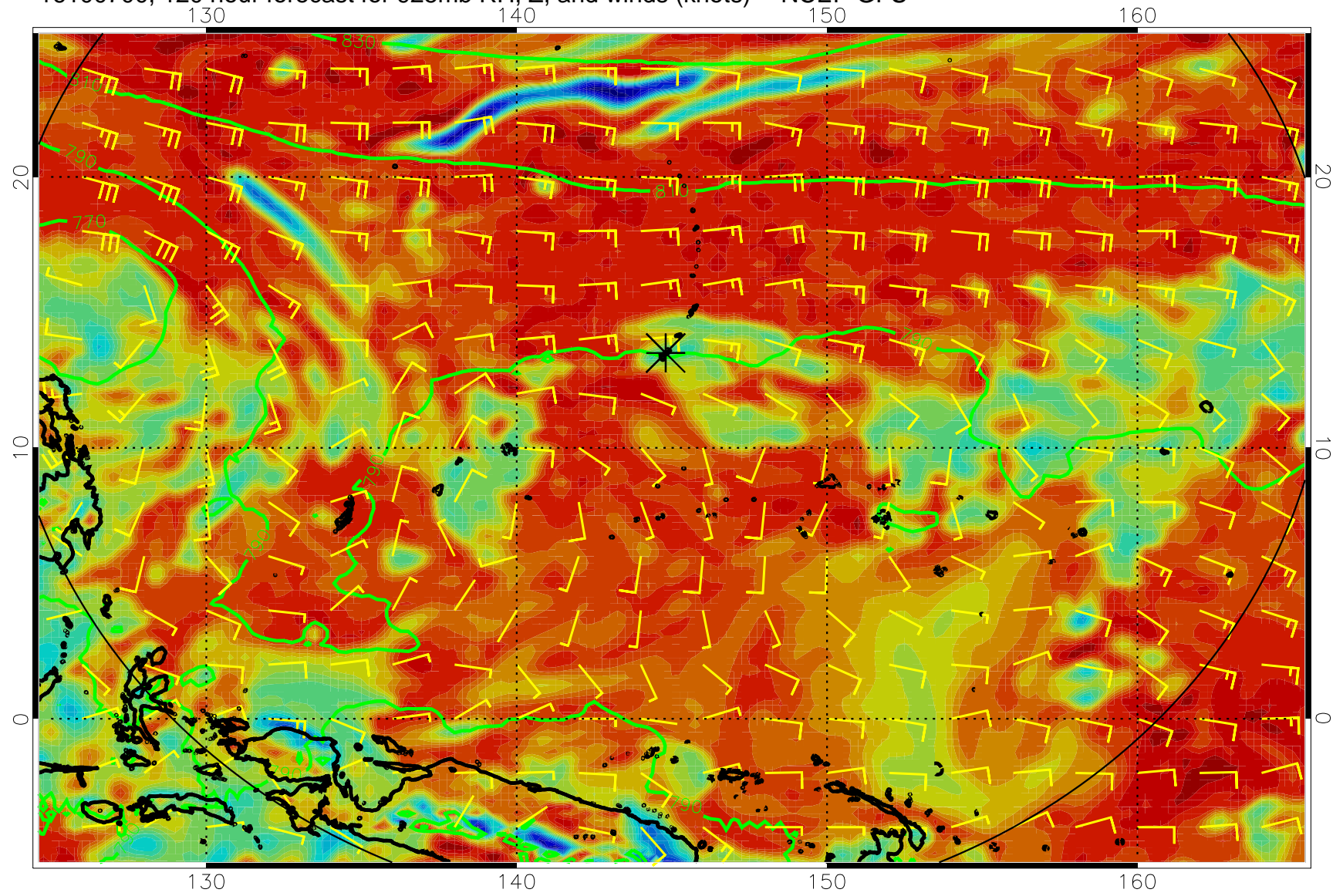
16100700, 120 hour forecast for 925mb RH, Z, and winds (knots) -- NCEP GFS
