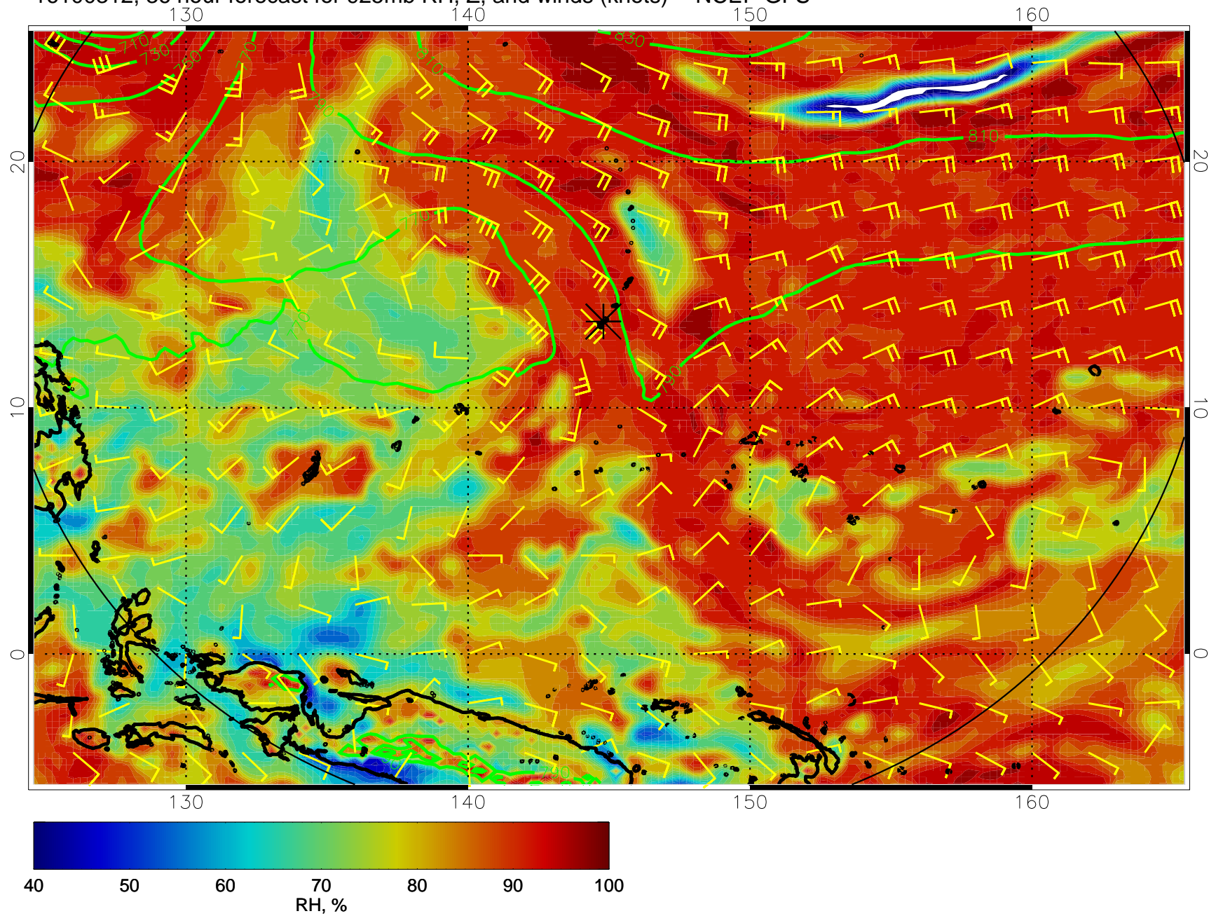
16100312, 36 hour forecast for 925mb RH, Z, and winds (knots) -- NCEP GFS
