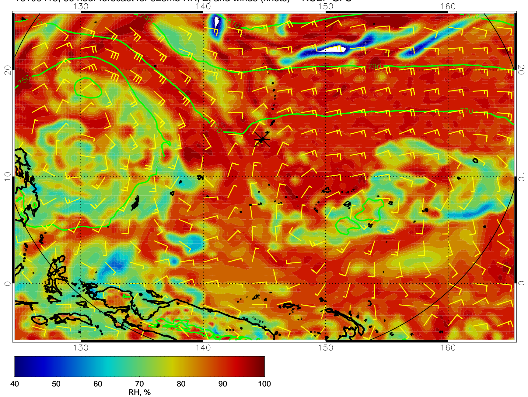
16100418, 66 hour forecast for 925mb RH, Z, and winds (knots) -- NCEP GFS
