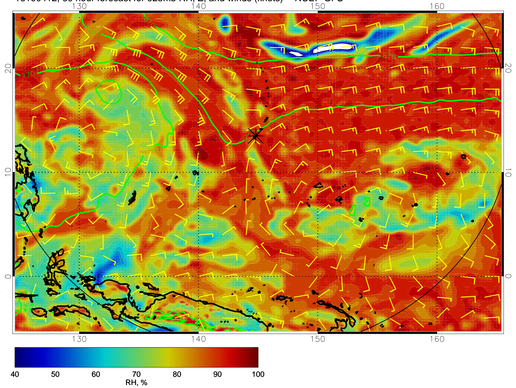
16100412, 60 hour forecast for 925mb RH, Z, and winds (knots) -- NCEP GFS
