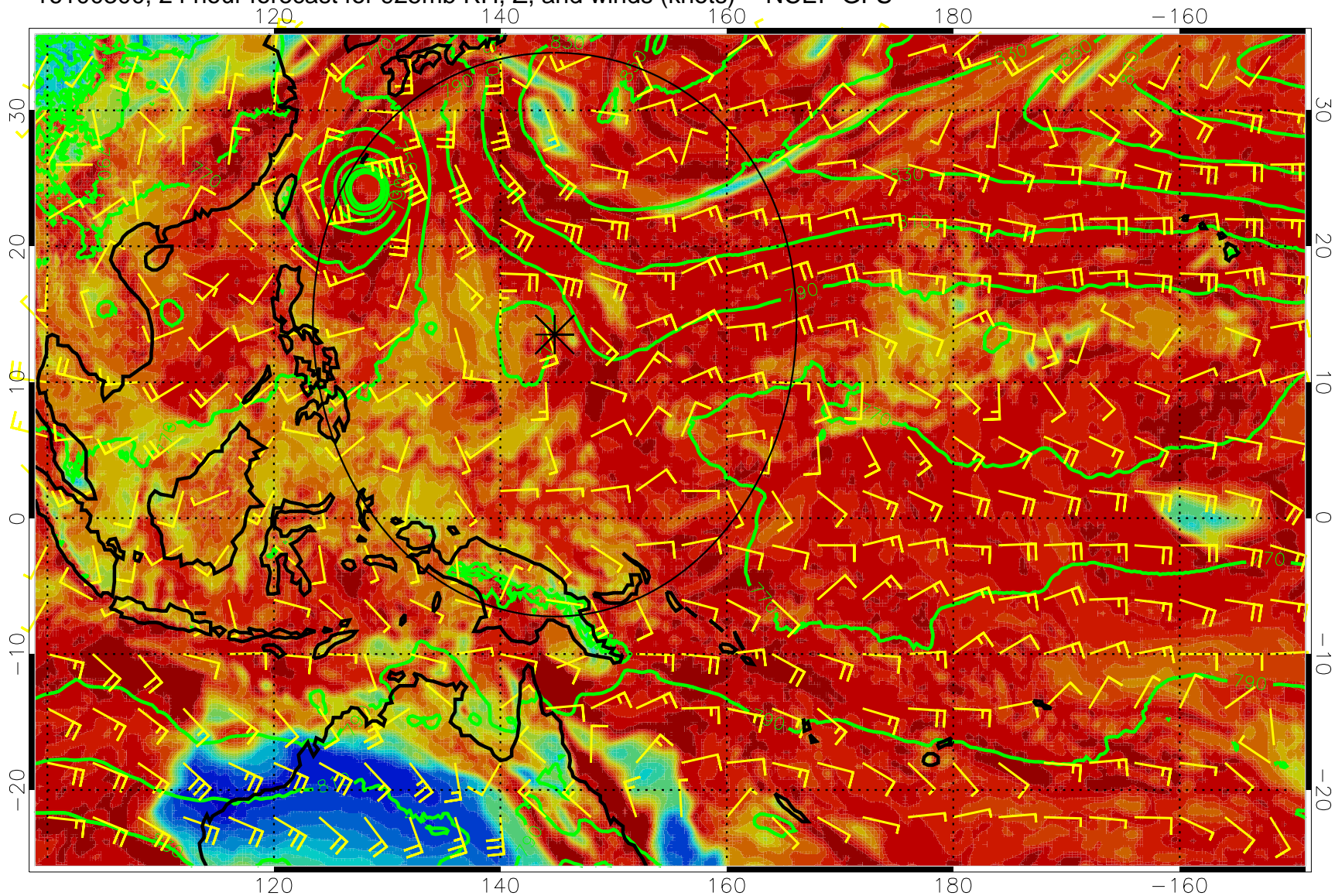
16100300, 24 hour forecast for 925mb RH, Z, and winds (knots) -- NCEP GFS
