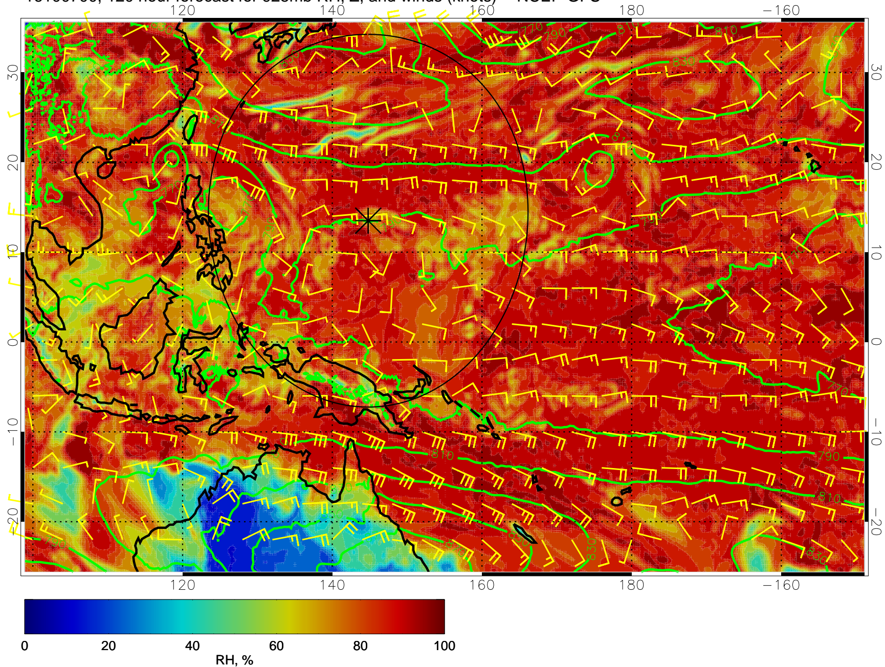
16100700, 120 hour forecast for 925mb RH, Z, and winds (knots) -- NCEP GFS
