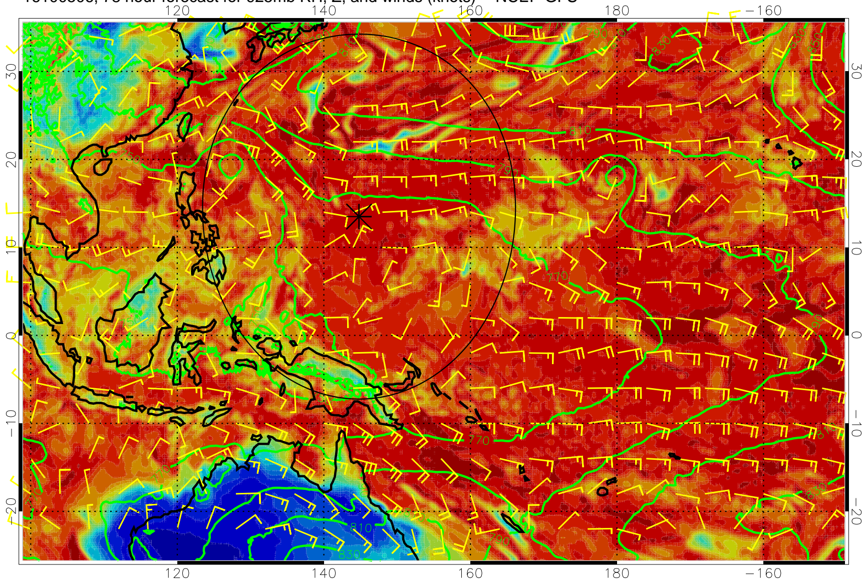
16100506, 78 hour forecast for 925mb RH, Z, and winds (knots) -- NCEP GFS
