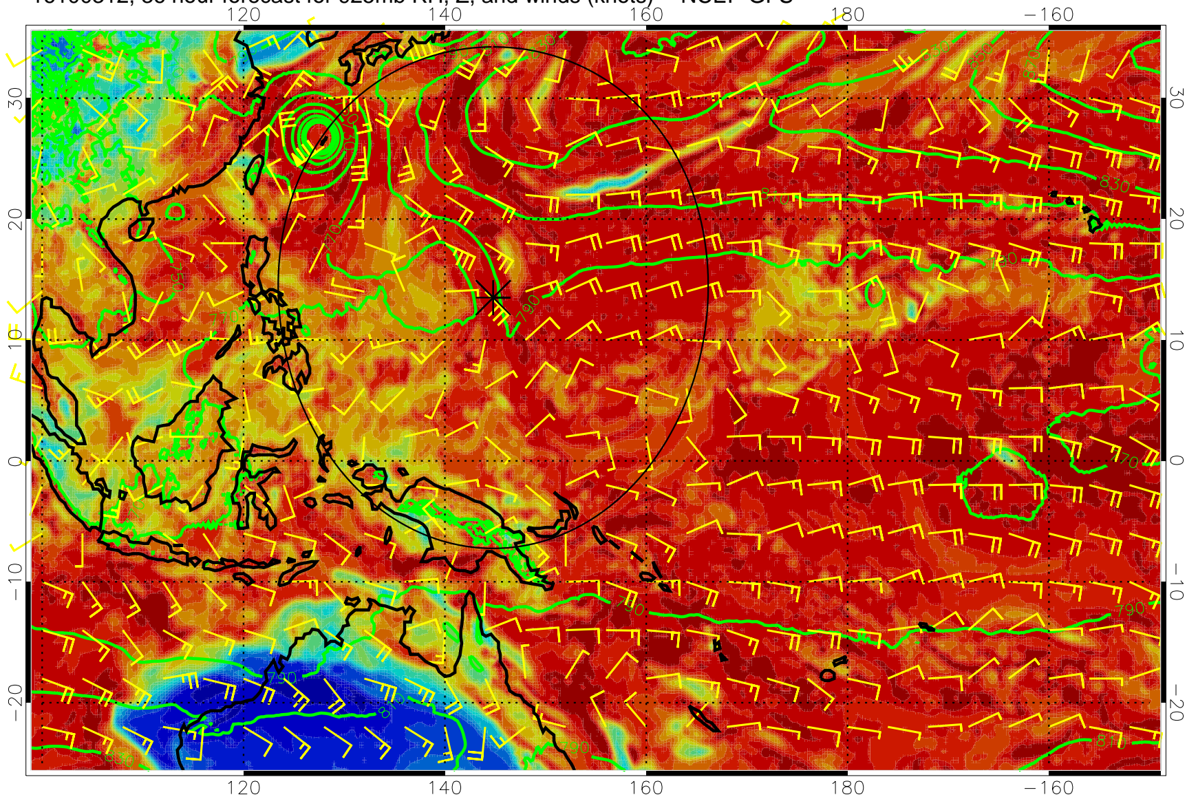
16100312, 36 hour forecast for 925mb RH, Z, and winds (knots) -- NCEP GFS
