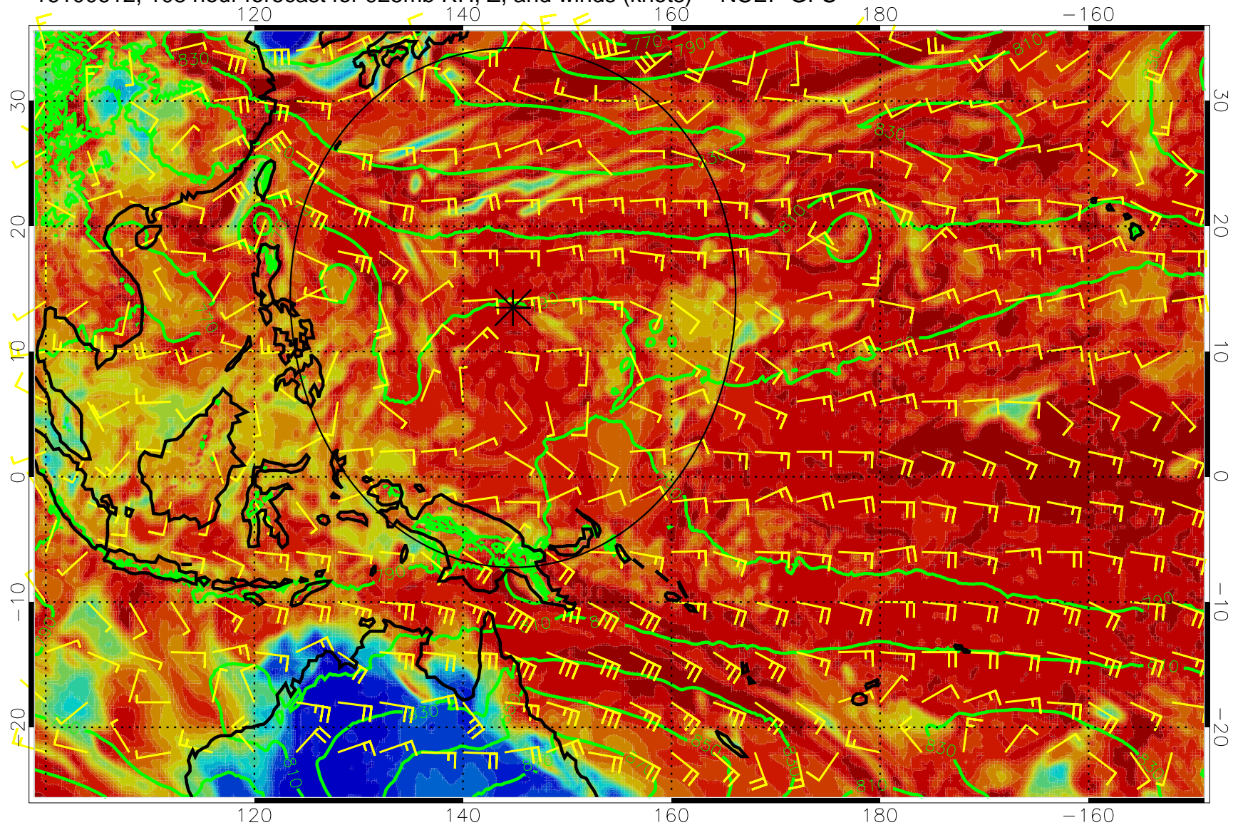
16100612, 108 hour forecast for 925mb RH, Z, and winds (knots) -- NCEP GFS
