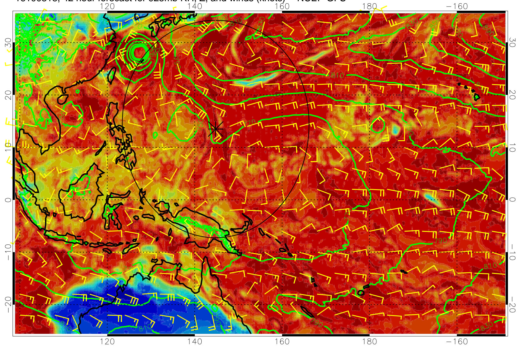
16100318, 42 hour forecast for 925mb RH, Z, and winds (knots) -- NCEP GFS
