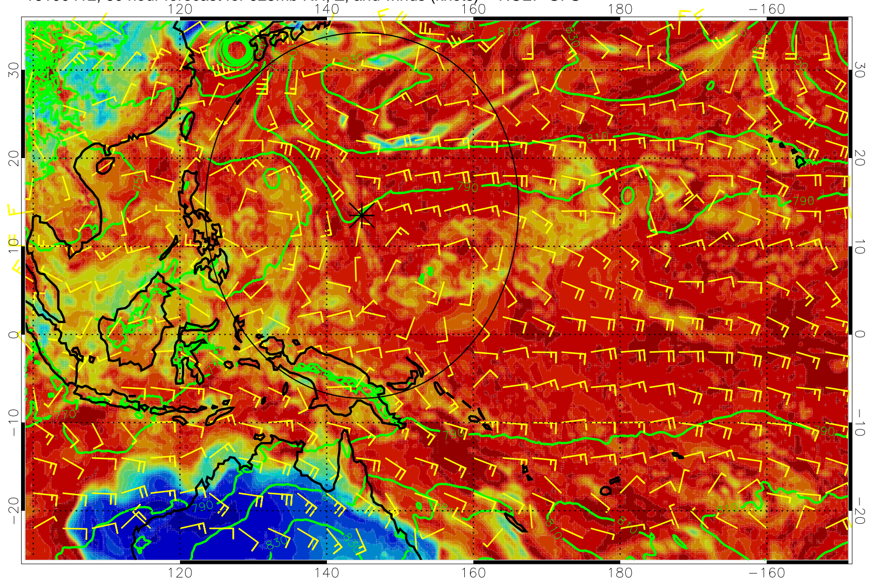
16100412, 60 hour forecast for 925mb RH, Z, and winds (knots) -- NCEP GFS
