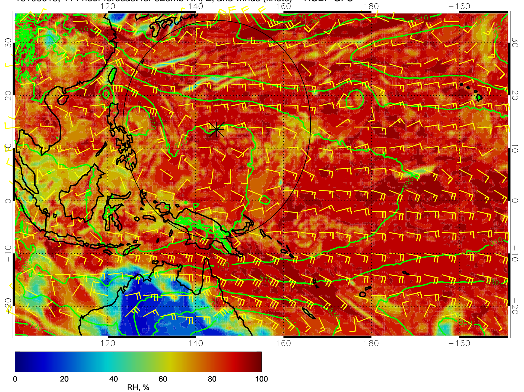
16100618, 114 hour forecast for 925mb RH, Z, and winds (knots) -- NCEP GFS
