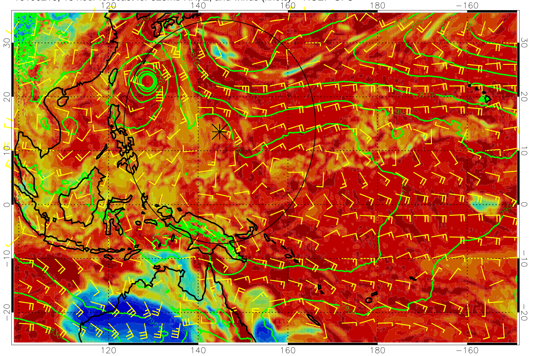
16100218, 18 hour forecast for 925mb RH, Z, and winds (knots) -- NCEP GFS
