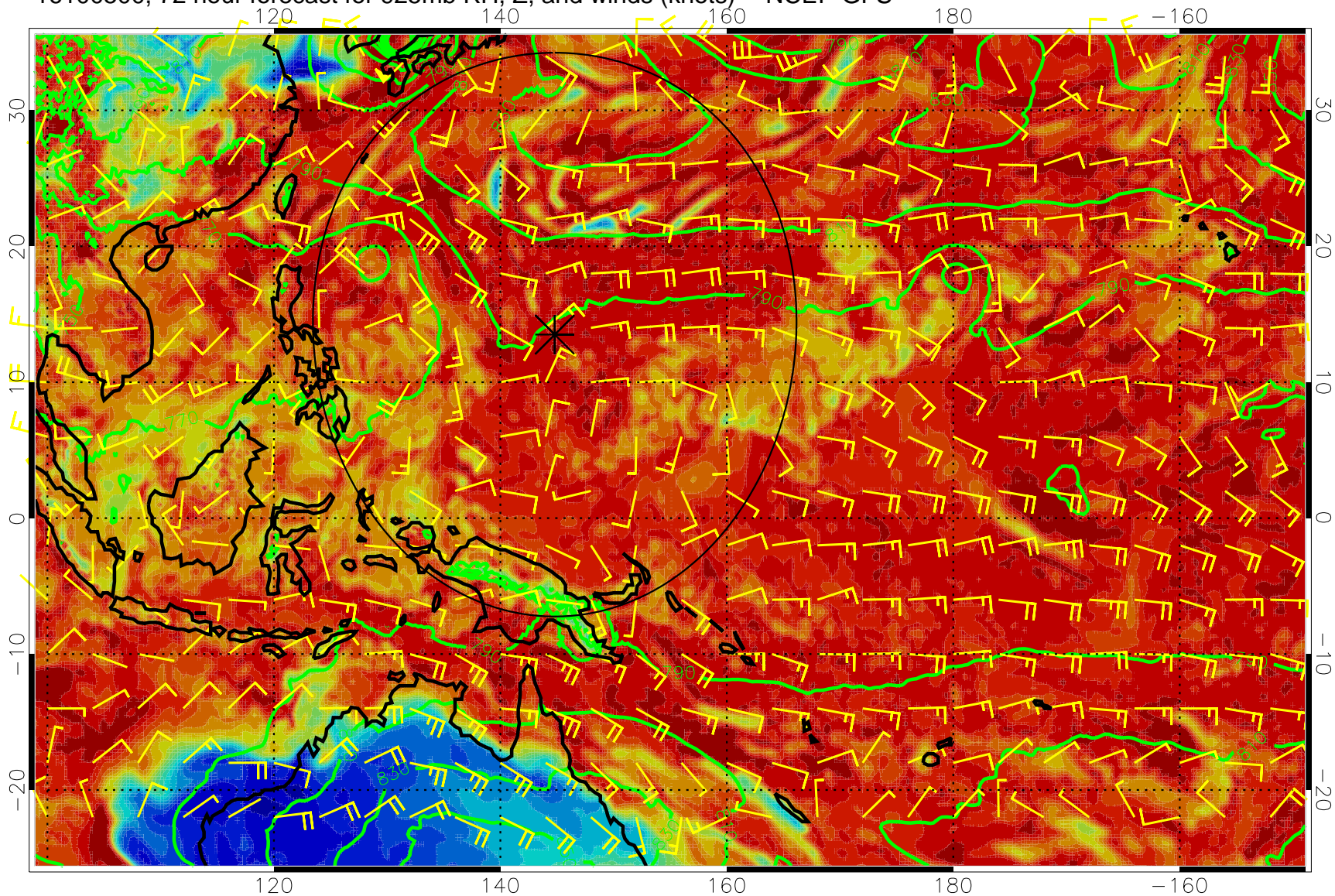
16100500, 72 hour forecast for 925mb RH, Z, and winds (knots) -- NCEP GFS
