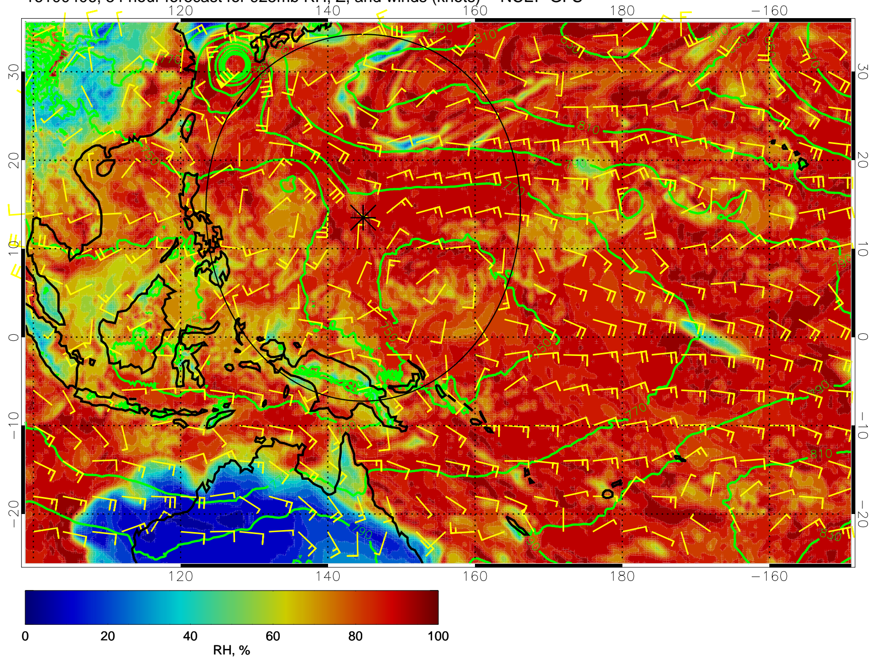
16100406, 54 hour forecast for 925mb RH, Z, and winds (knots) -- NCEP GFS
