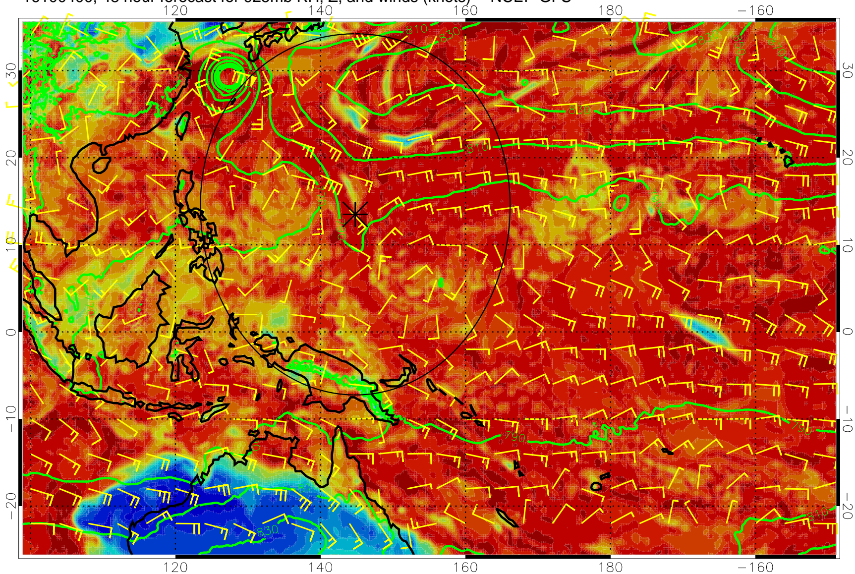
16100400, 48 hour forecast for 925mb RH, Z, and winds (knots) -- NCEP GFS
