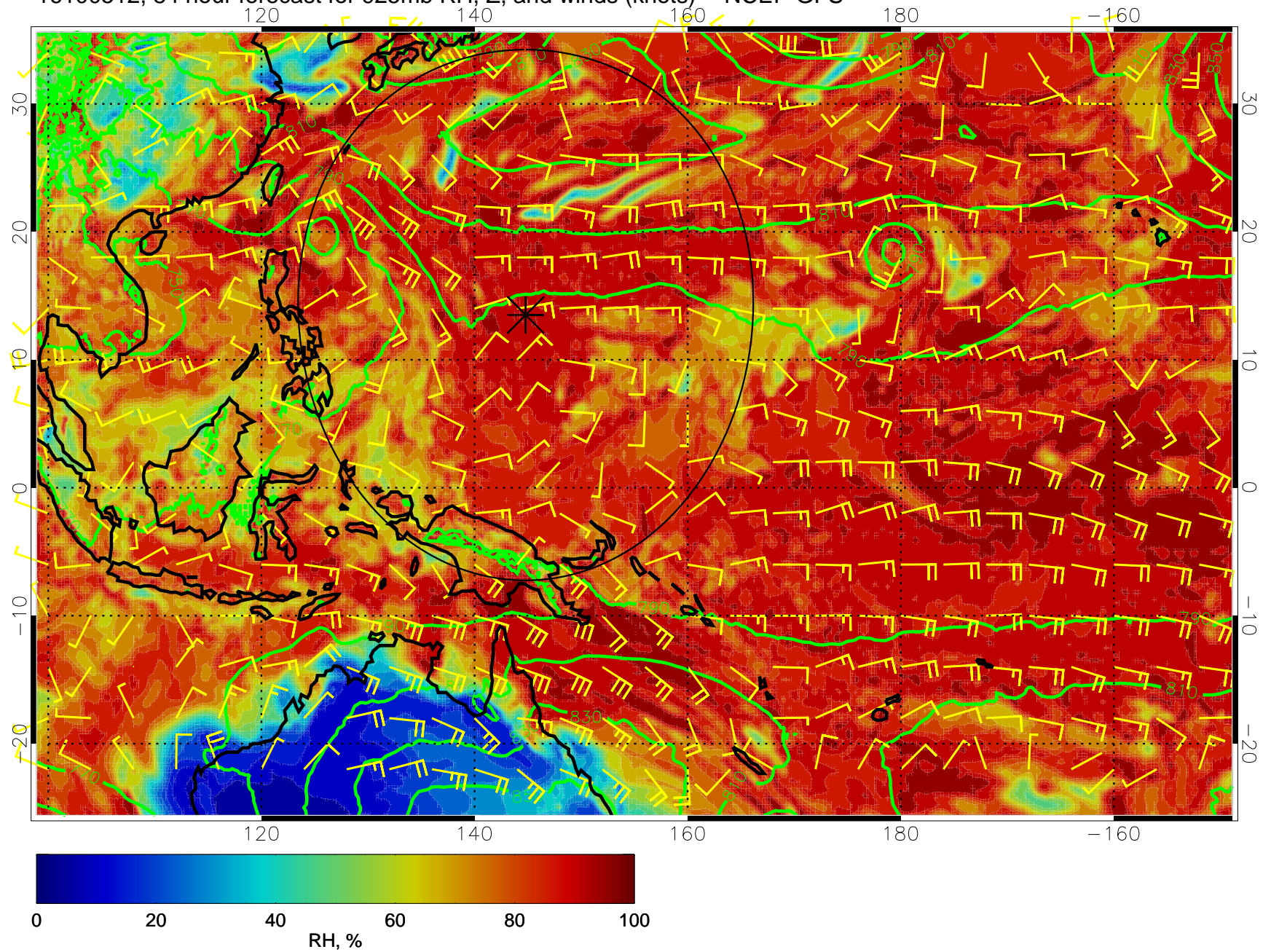
16100512, 84 hour forecast for 925mb RH, Z, and winds (knots) -- NCEP GFS
