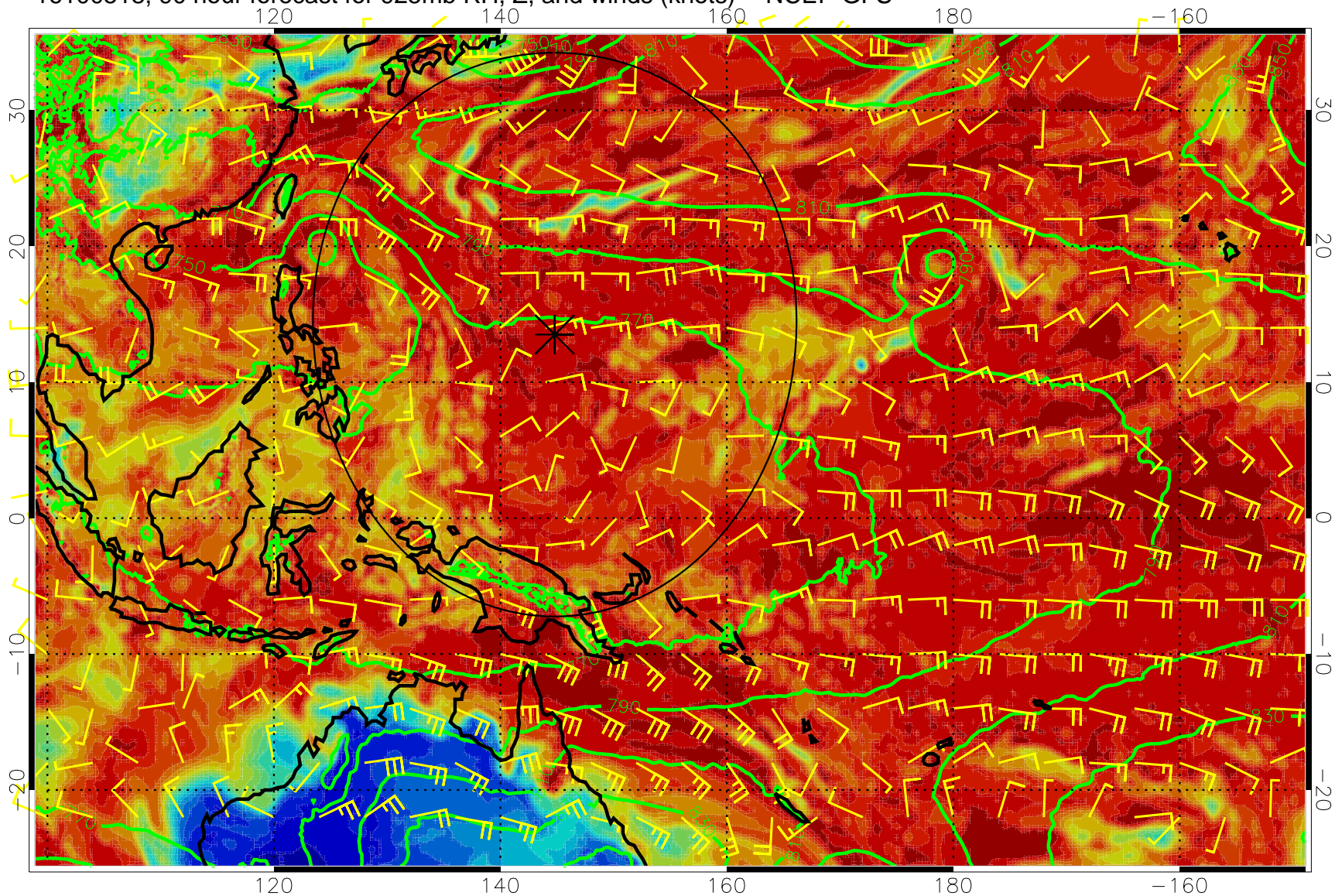
16100518, 90 hour forecast for 925mb RH, Z, and winds (knots) -- NCEP GFS
