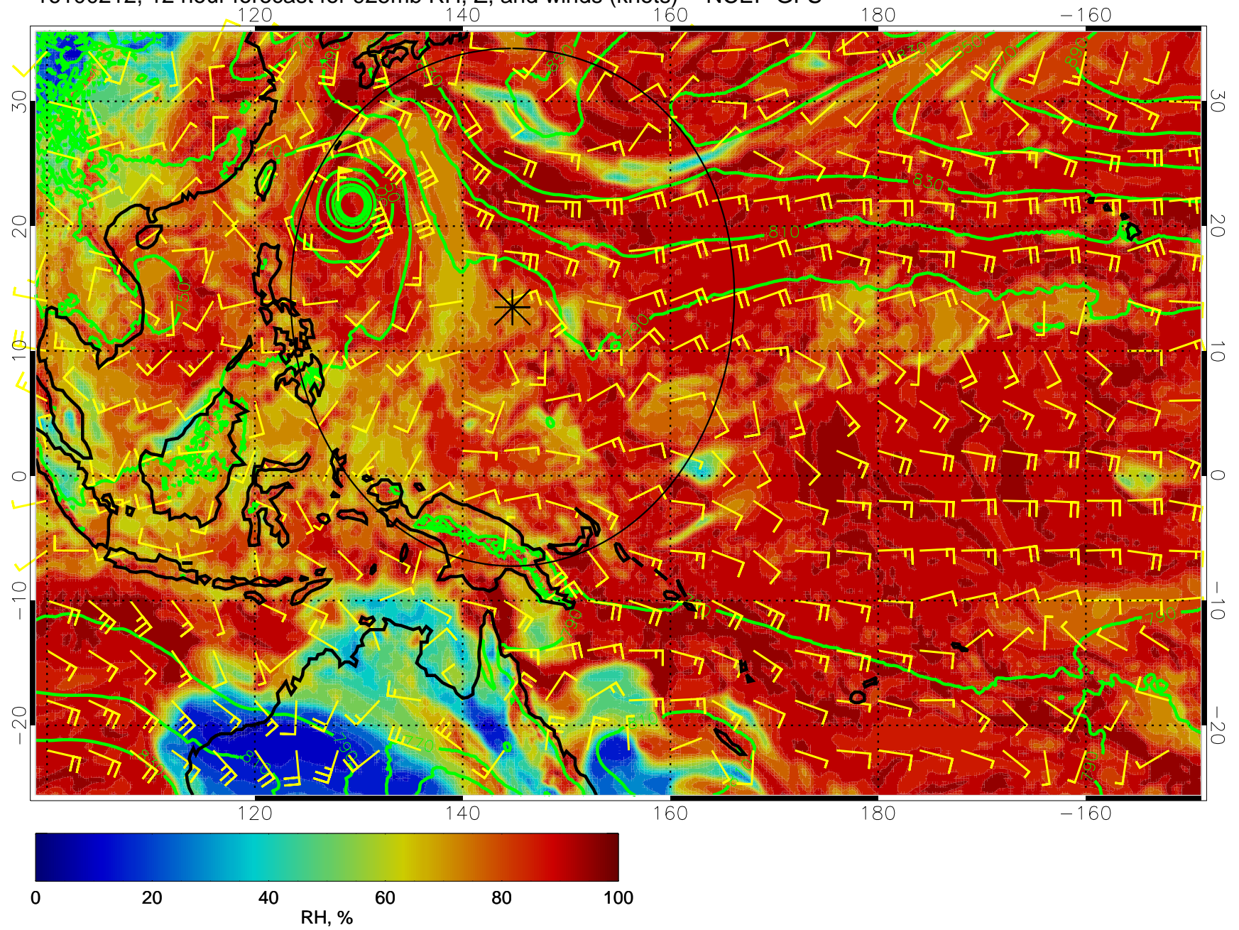
16100212, 12 hour forecast for 925mb RH, Z, and winds (knots) -- NCEP GFS
