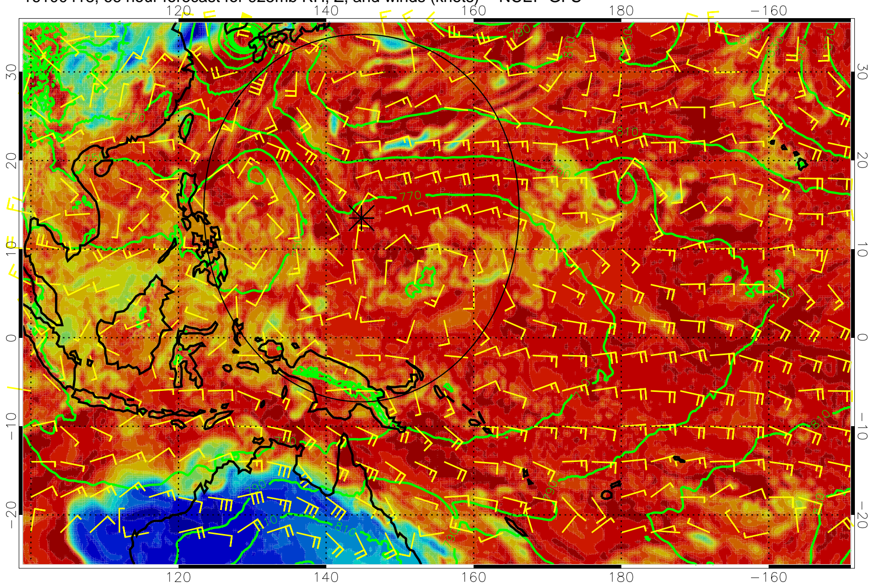
16100418, 66 hour forecast for 925mb RH, Z, and winds (knots) -- NCEP GFS
