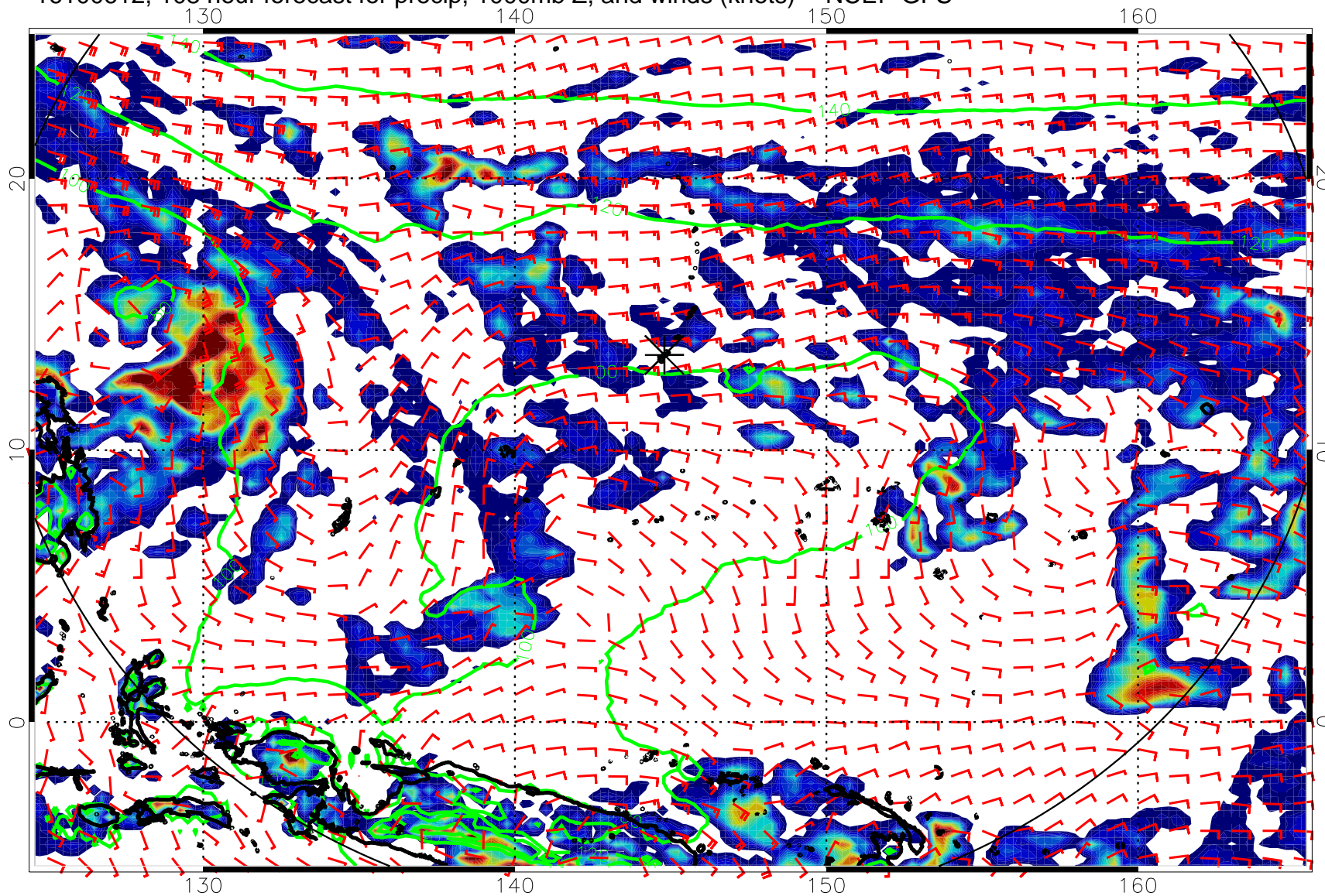
16100612, 108 hour forecast for precip, 1000mb Z, and winds (knots) -- NCEP GFS
