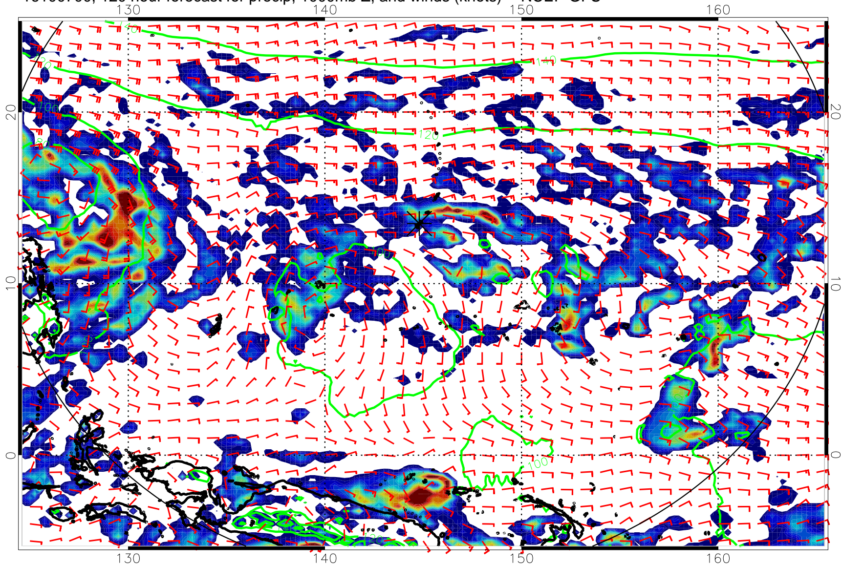
16100700, 120 hour forecast for precip, 1000mb Z, and winds (knots) -- NCEP GFS
