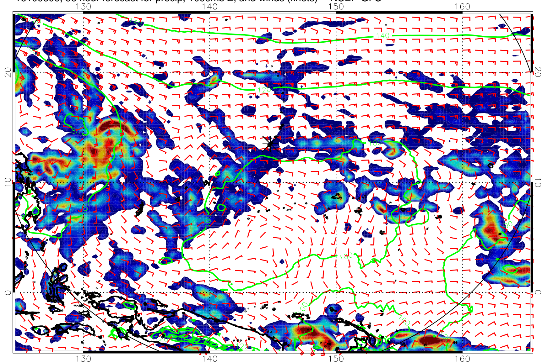
16100600, 96 hour forecast for precip, 1000mb Z, and winds (knots) -- NCEP GFS
