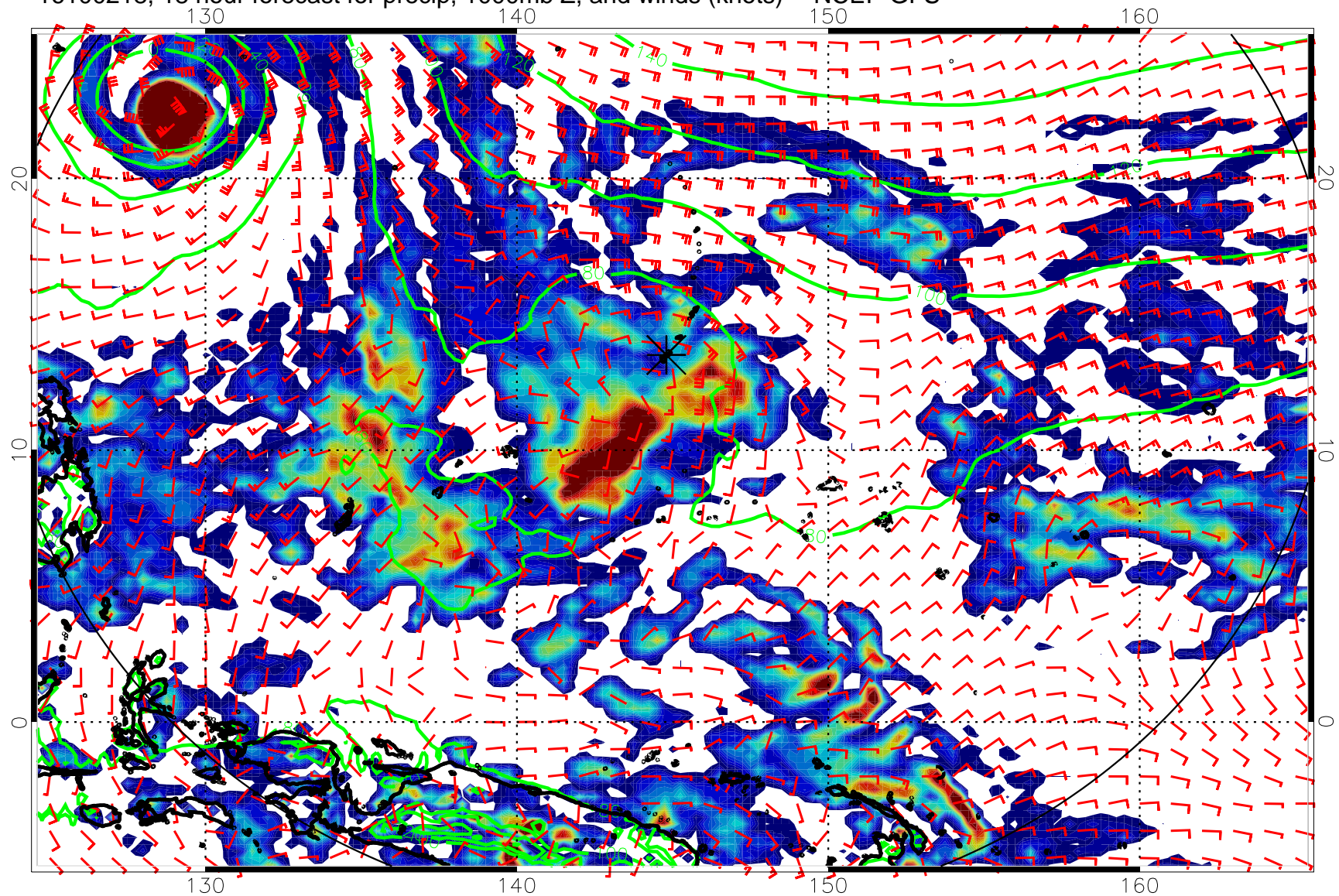
16100218, 18 hour forecast for precip, 1000mb Z, and winds (knots) -- NCEP GFS
