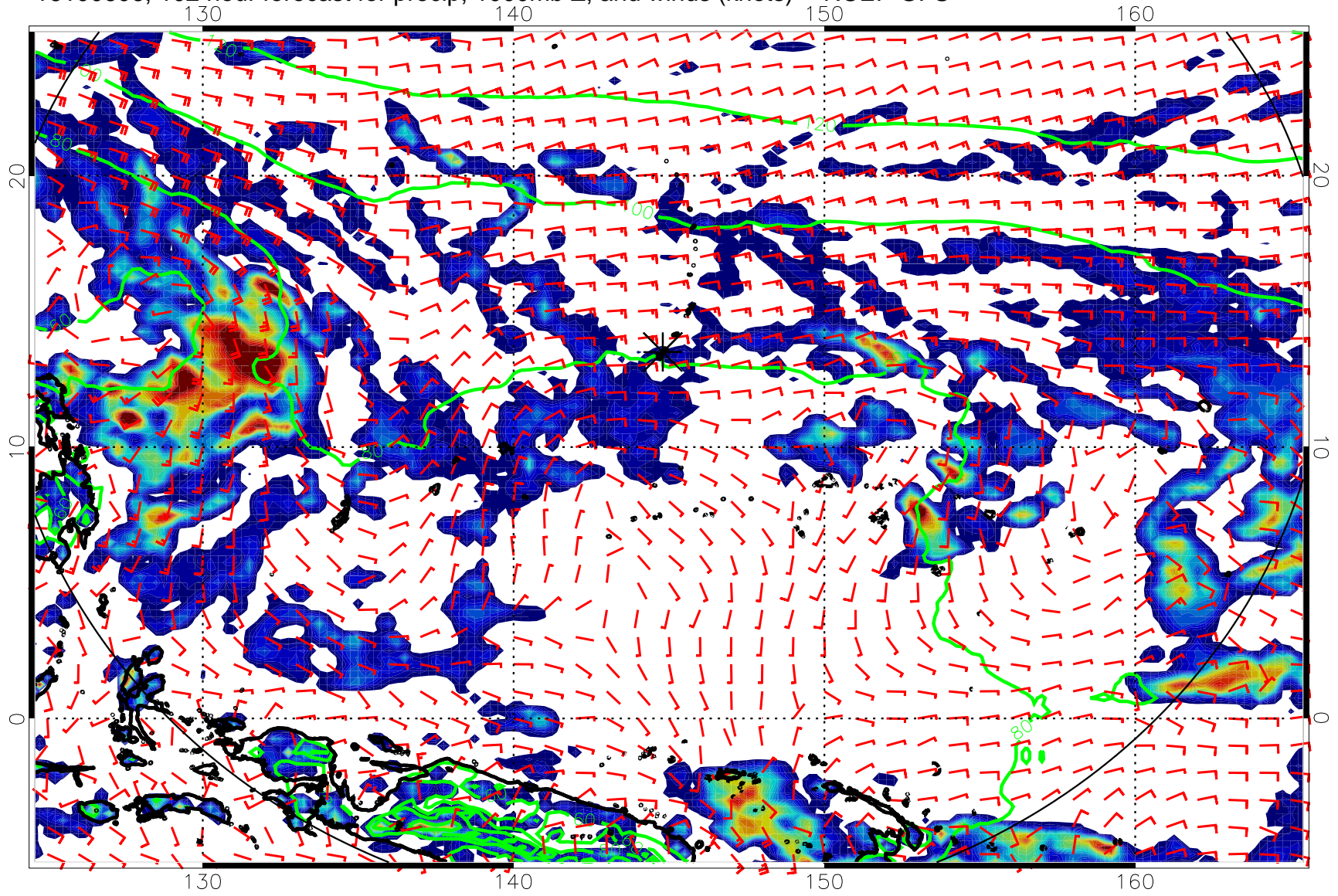
16100606, 102 hour forecast for precip, 1000mb Z, and winds (knots) -- NCEP GFS
