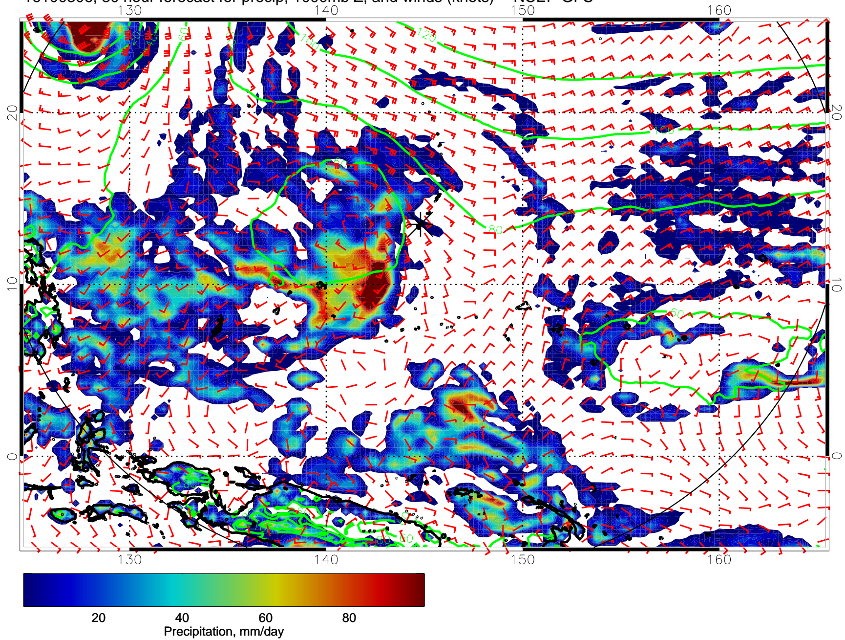
16100306, 30 hour forecast for precip, 1000mb Z, and winds (knots) -- NCEP GFS
