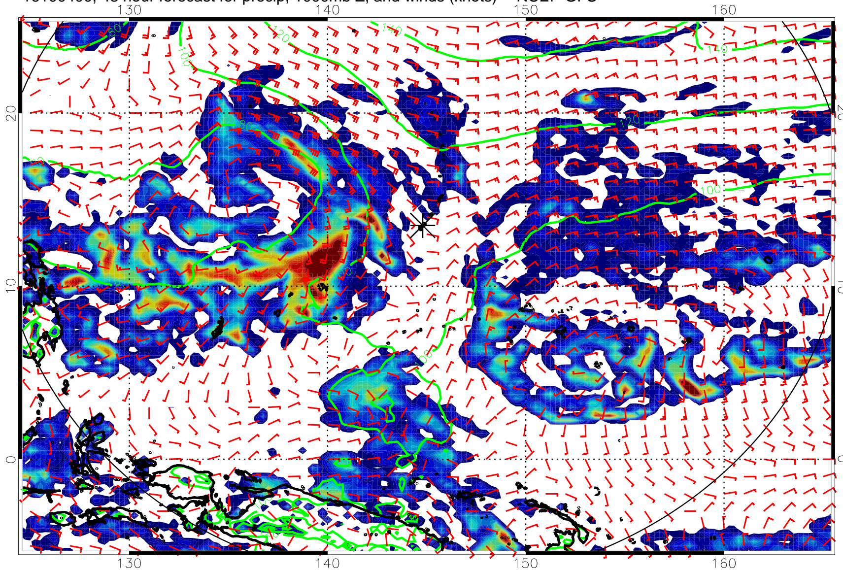
16100400, 48 hour forecast for precip, 1000mb Z, and winds (knots) -- NCEP GFS
