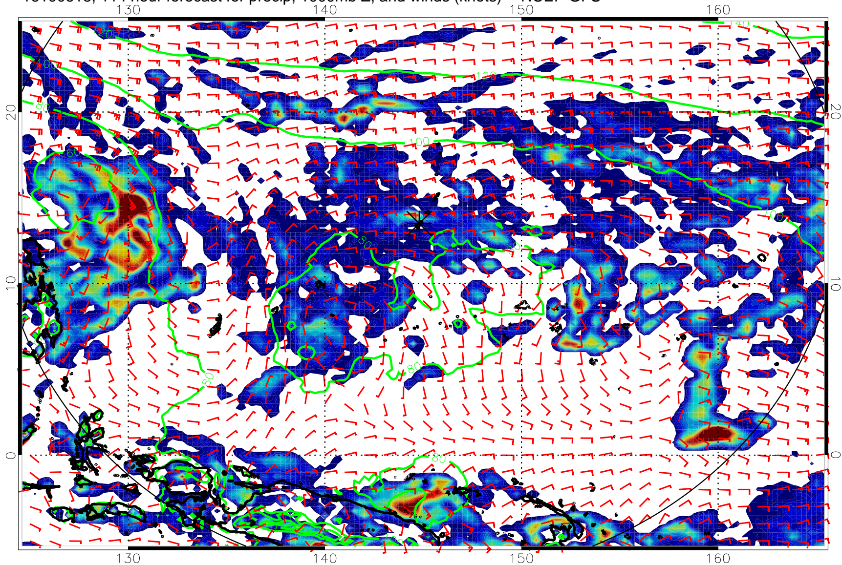
16100618, 114 hour forecast for precip, 1000mb Z, and winds (knots) -- NCEP GFS
