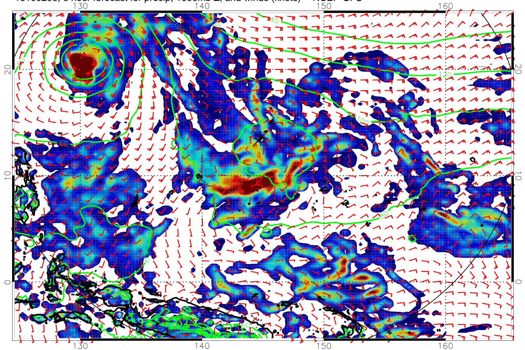
16100206, 6 hour forecast for precip, 1000mb Z, and winds (knots) -- NCEP GFS
