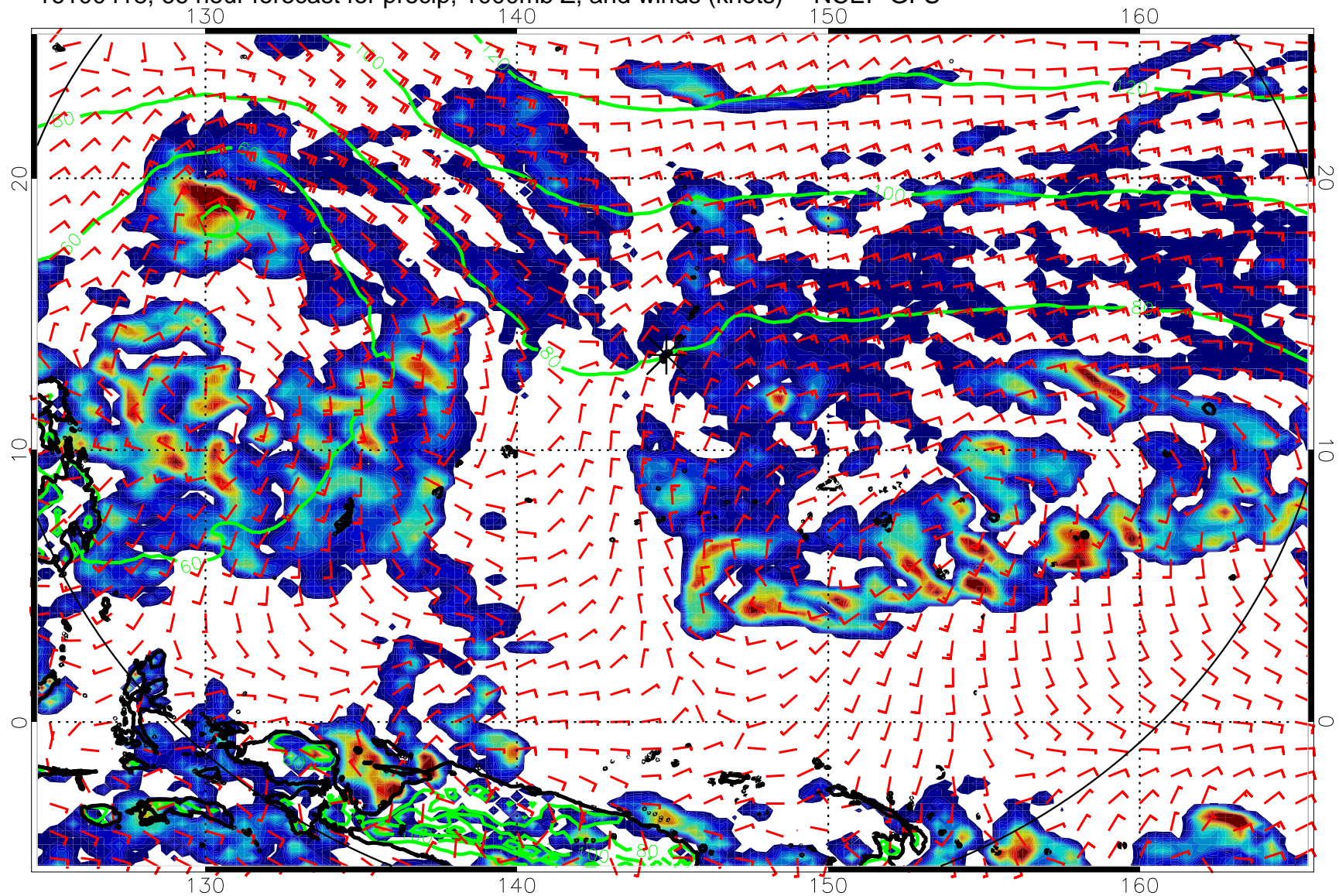
16100418, 66 hour forecast for precip, 1000mb Z, and winds (knots) -- NCEP GFS
