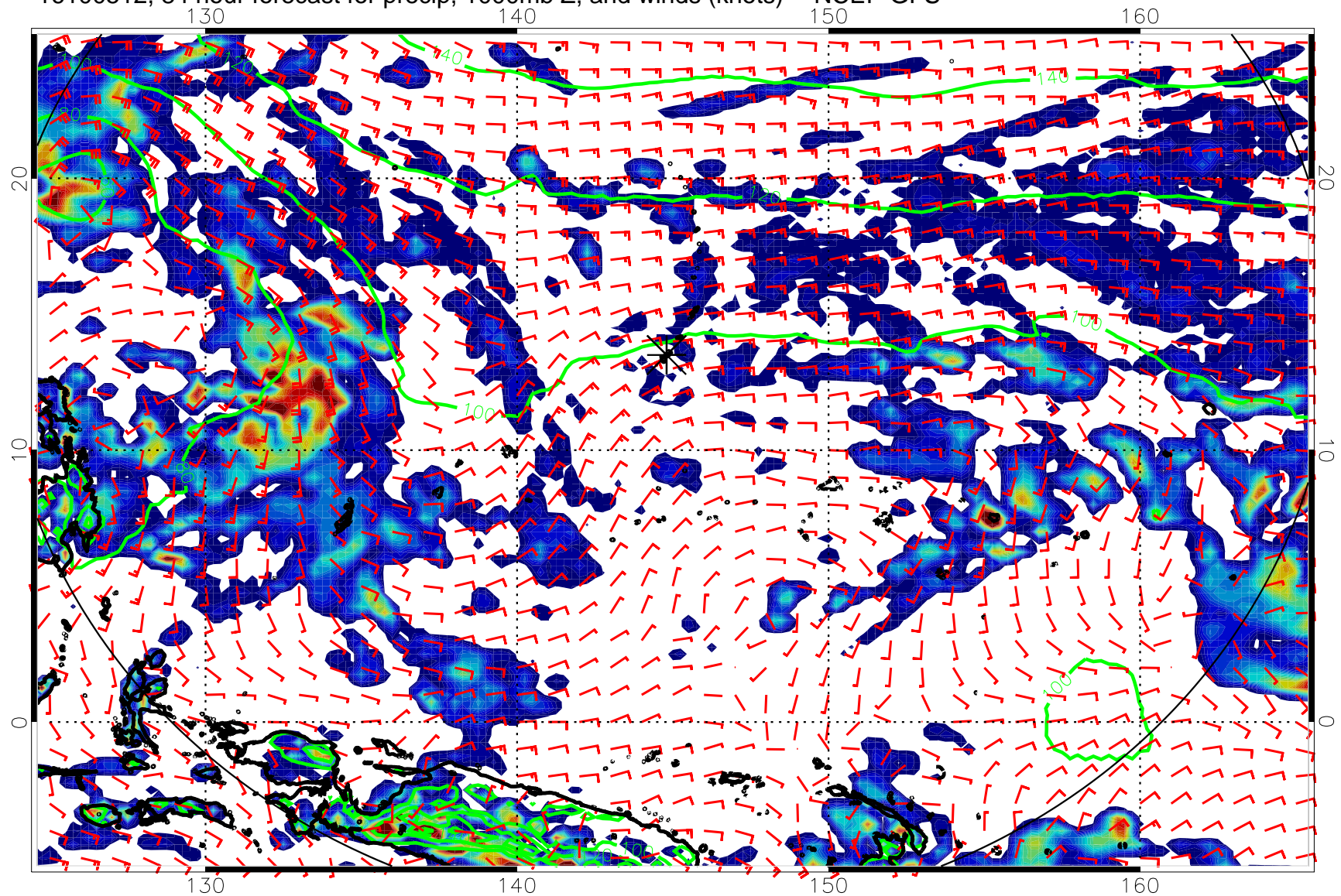
16100512, 84 hour forecast for precip, 1000mb Z, and winds (knots) -- NCEP GFS
