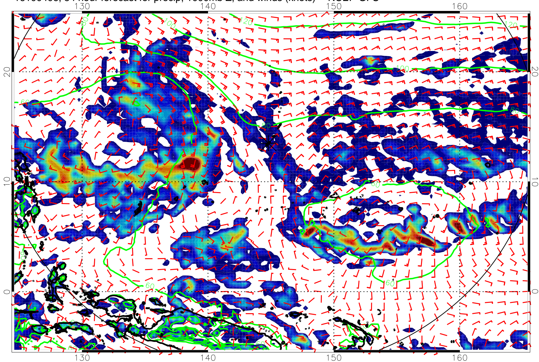
16100406, 54 hour forecast for precip, 1000mb Z, and winds (knots) -- NCEP GFS
