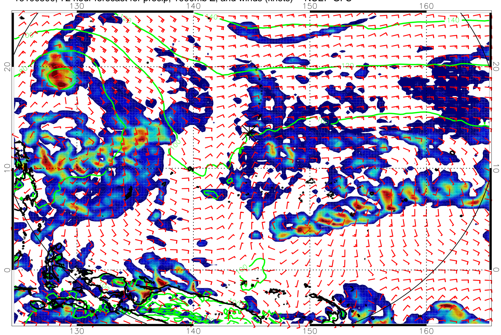
16100500, 72 hour forecast for precip, 1000mb Z, and winds (knots) -- NCEP GFS
