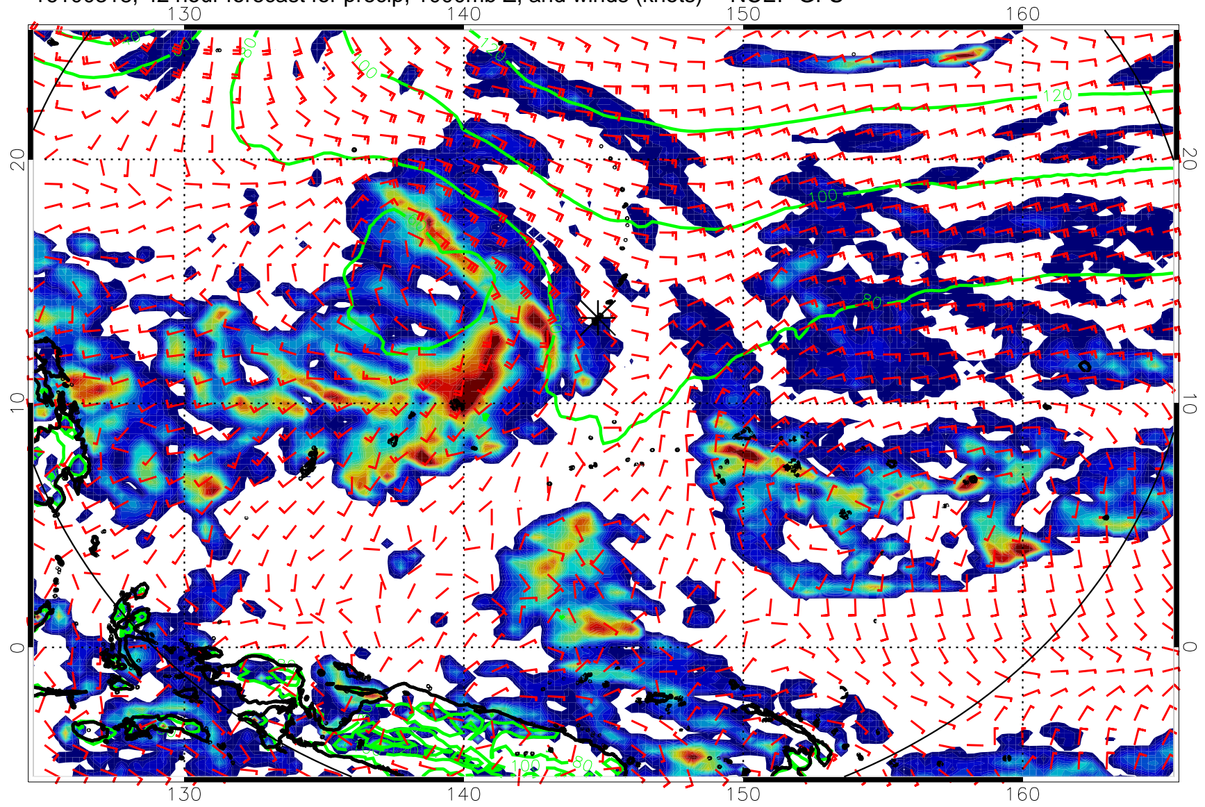
16100318, 42 hour forecast for precip, 1000mb Z, and winds (knots) -- NCEP GFS
