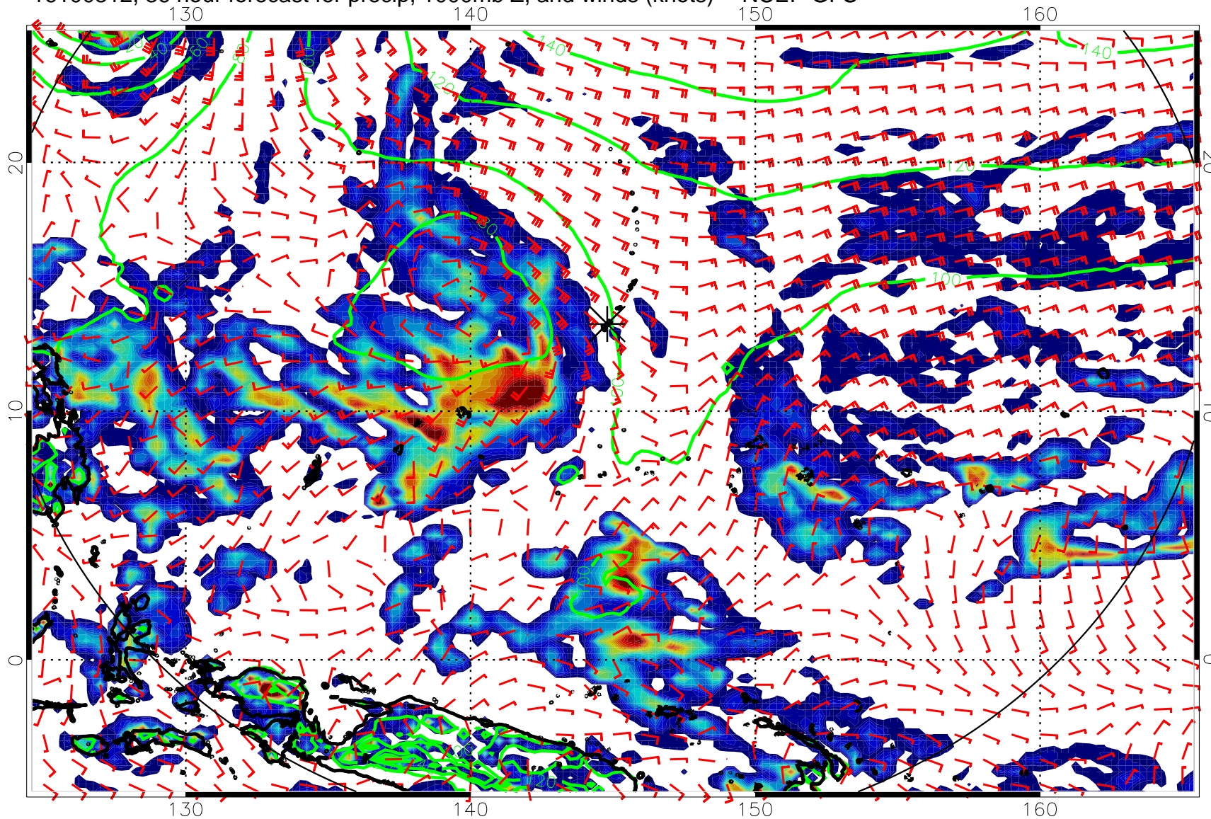
16100312, 36 hour forecast for precip, 1000mb Z, and winds (knots) -- NCEP GFS
