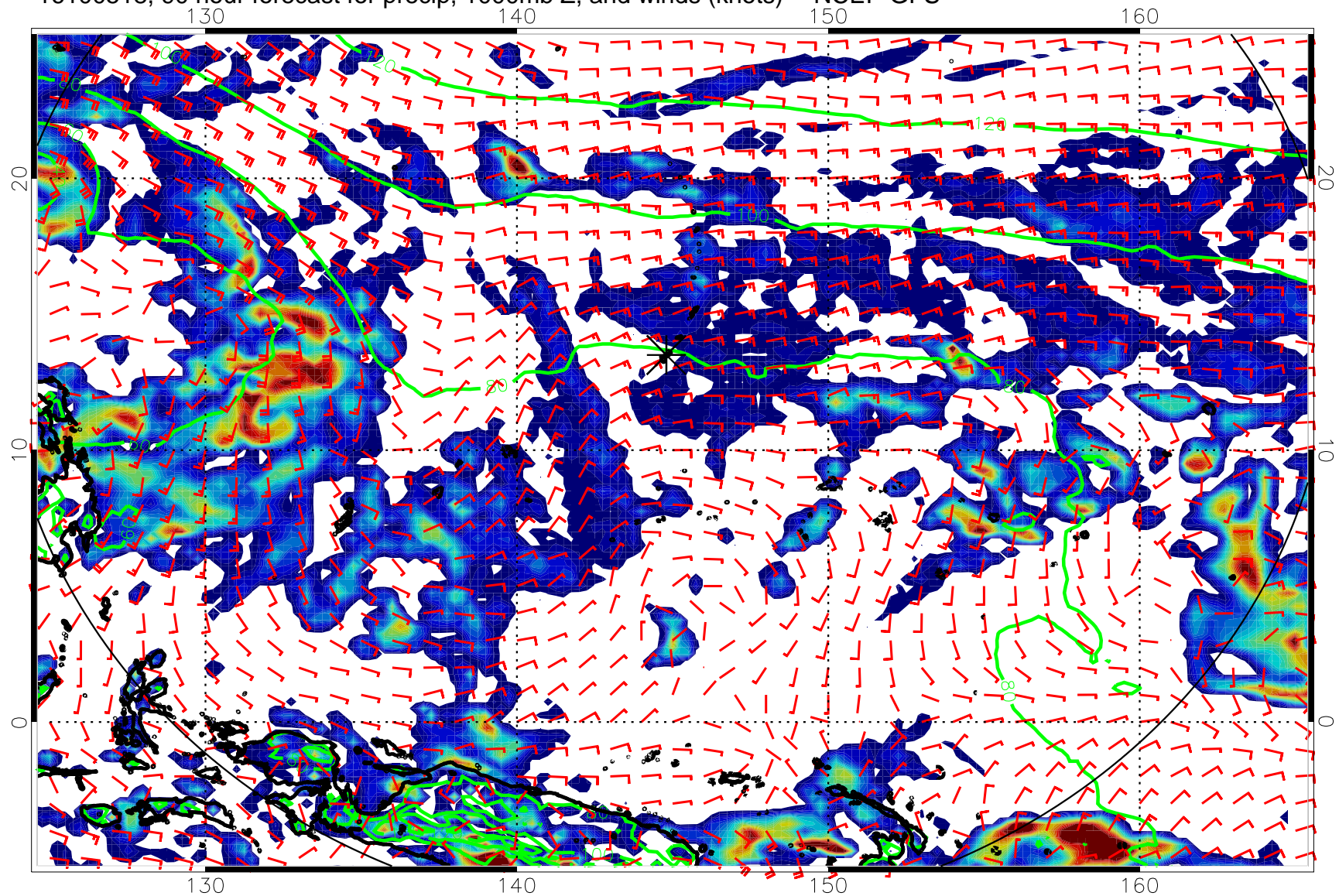
16100518, 90 hour forecast for precip, 1000mb Z, and winds (knots) -- NCEP GFS
