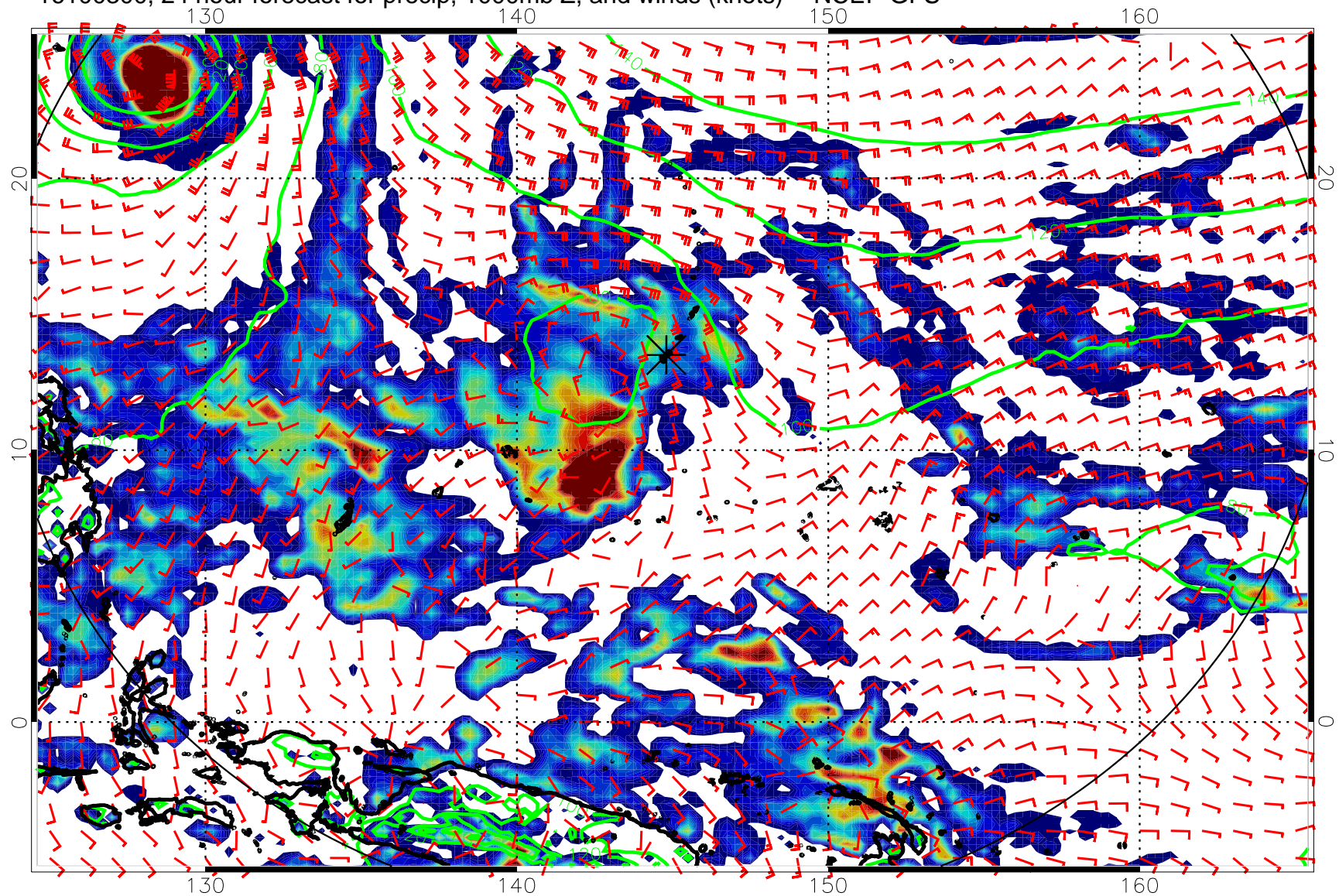
16100300, 24 hour forecast for precip, 1000mb Z, and winds (knots) -- NCEP GFS
