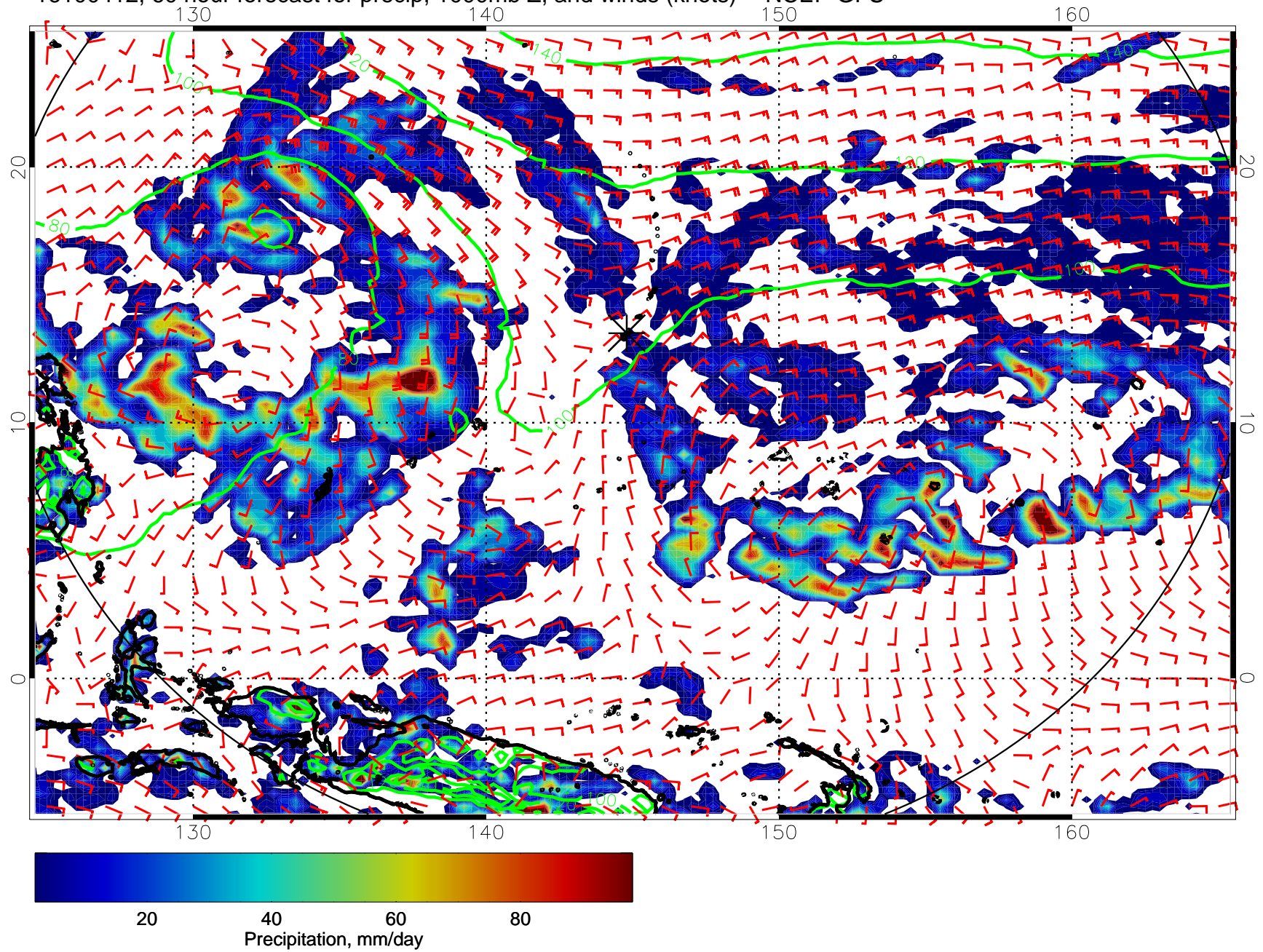
16100412, 60 hour forecast for precip, 1000mb Z, and winds (knots) -- NCEP GFS
