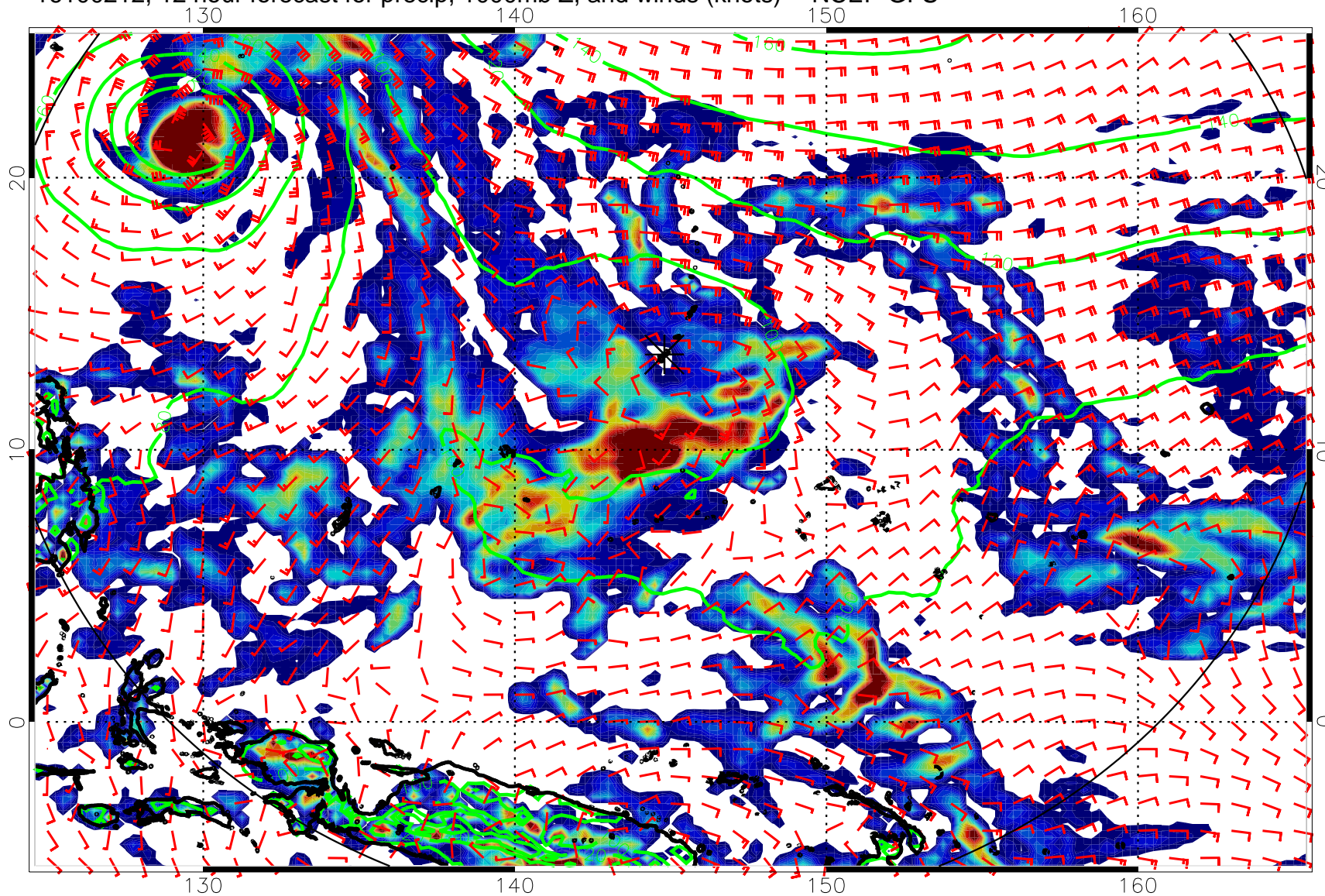
16100212, 12 hour forecast for precip, 1000mb Z, and winds (knots) -- NCEP GFS
