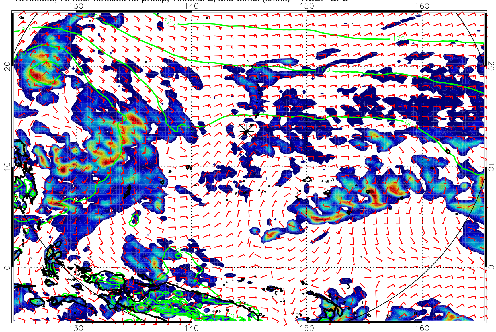
16100506, 78 hour forecast for precip, 1000mb Z, and winds (knots) -- NCEP GFS
