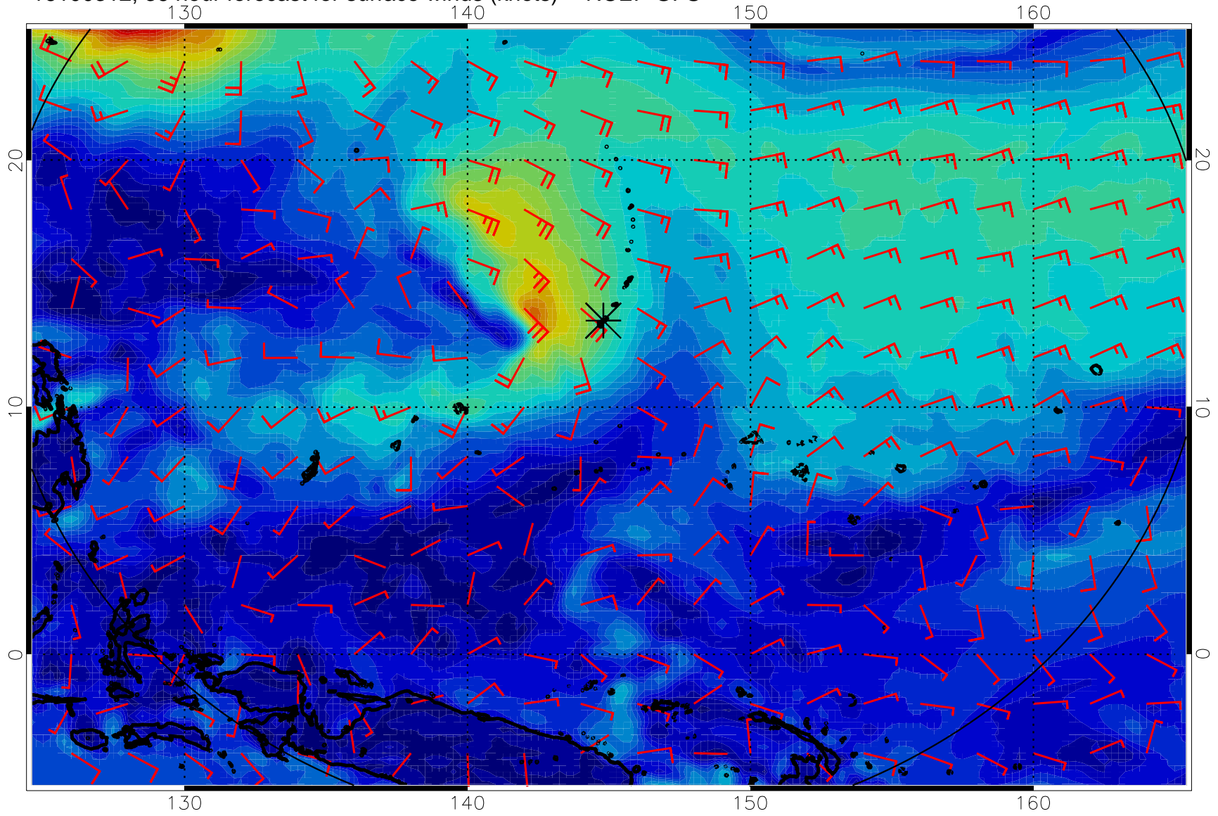
16100312, 36 hour forecast for surface winds (knots) -- NCEP GFS
