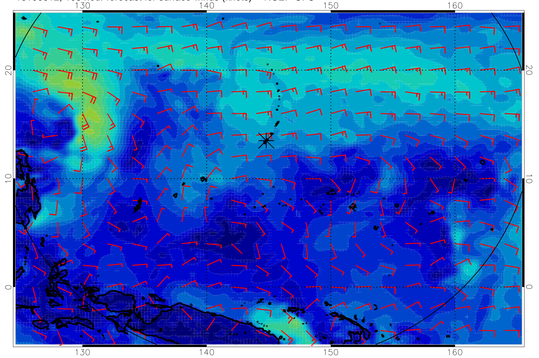
16100612, 108 hour forecast for surface winds (knots) -- NCEP GFS
