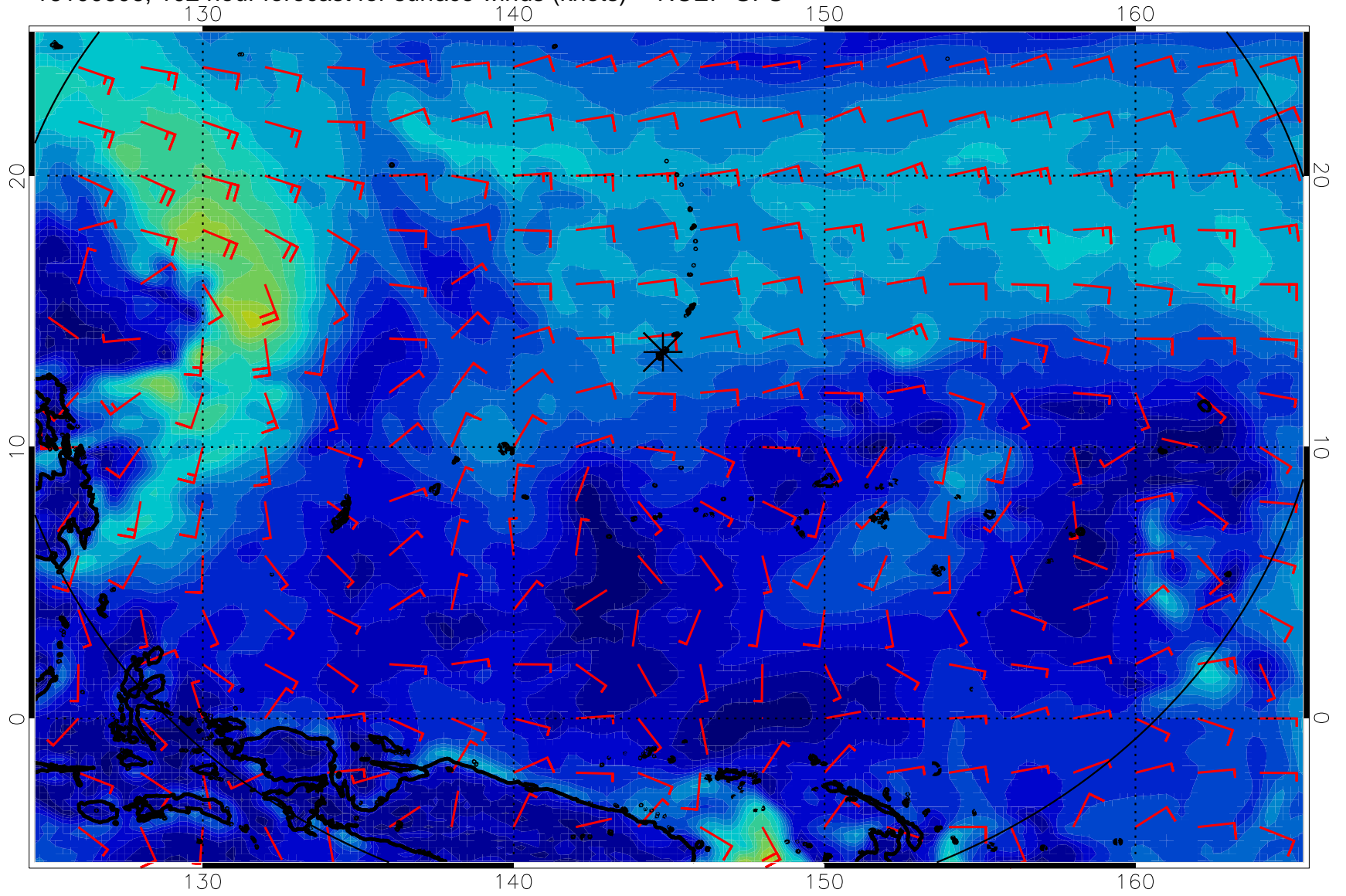
16100606, 102 hour forecast for surface winds (knots) -- NCEP GFS
