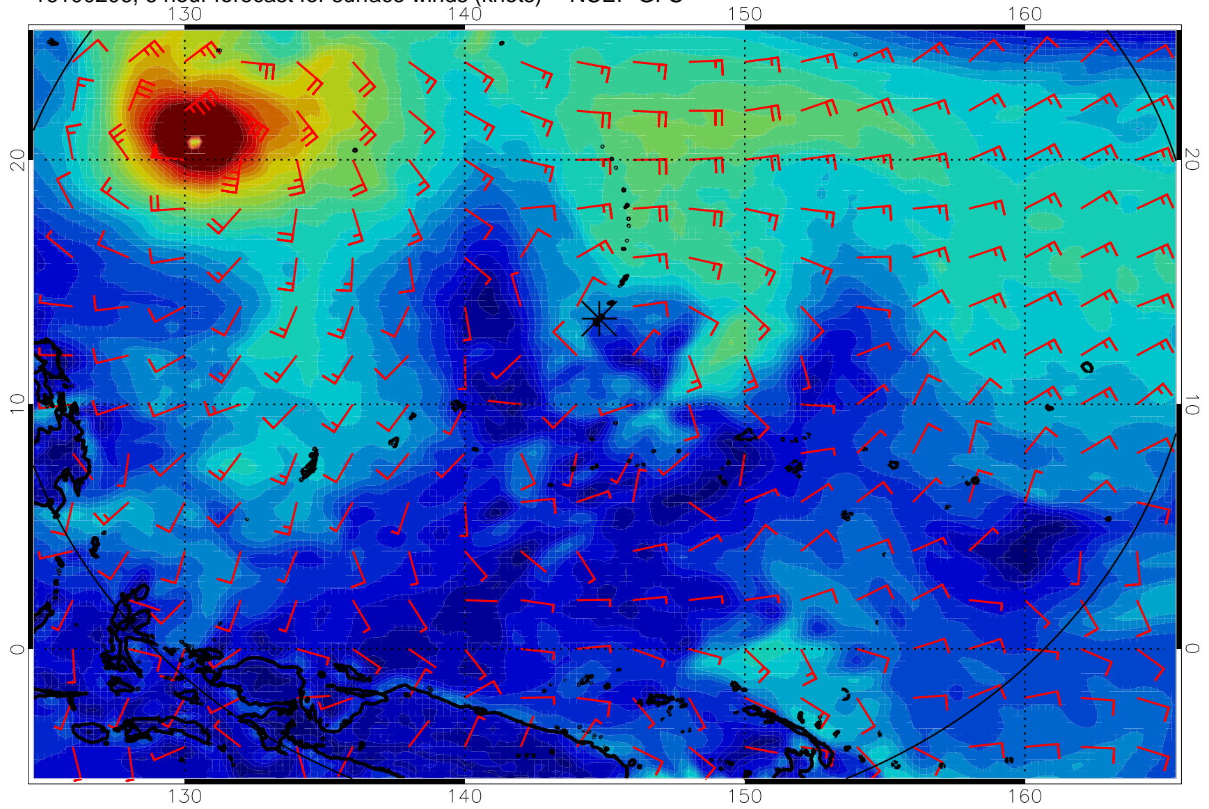
16100206, 6 hour forecast for surface winds (knots) -- NCEP GFS
