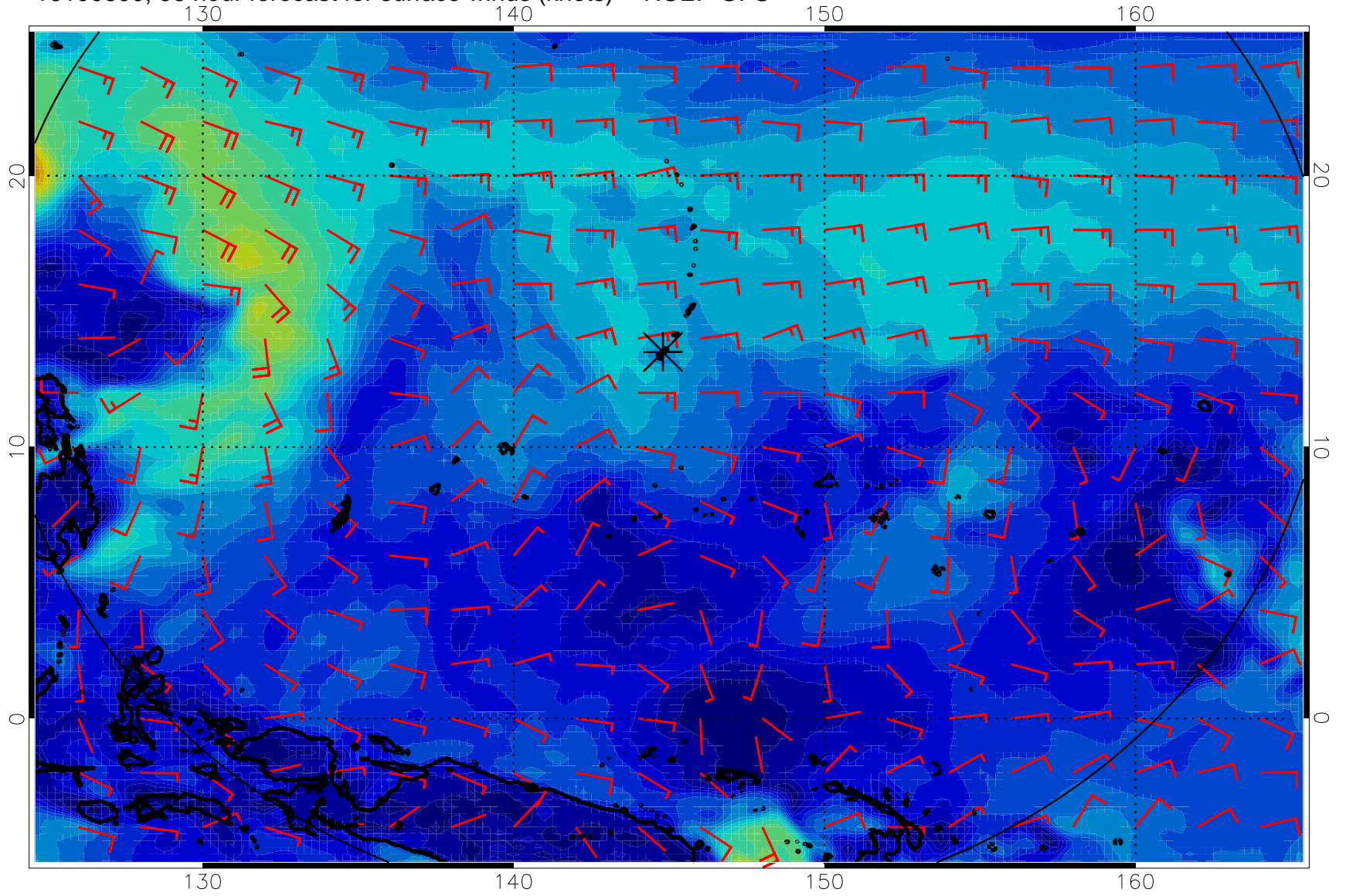
16100600, 96 hour forecast for surface winds (knots) -- NCEP GFS
