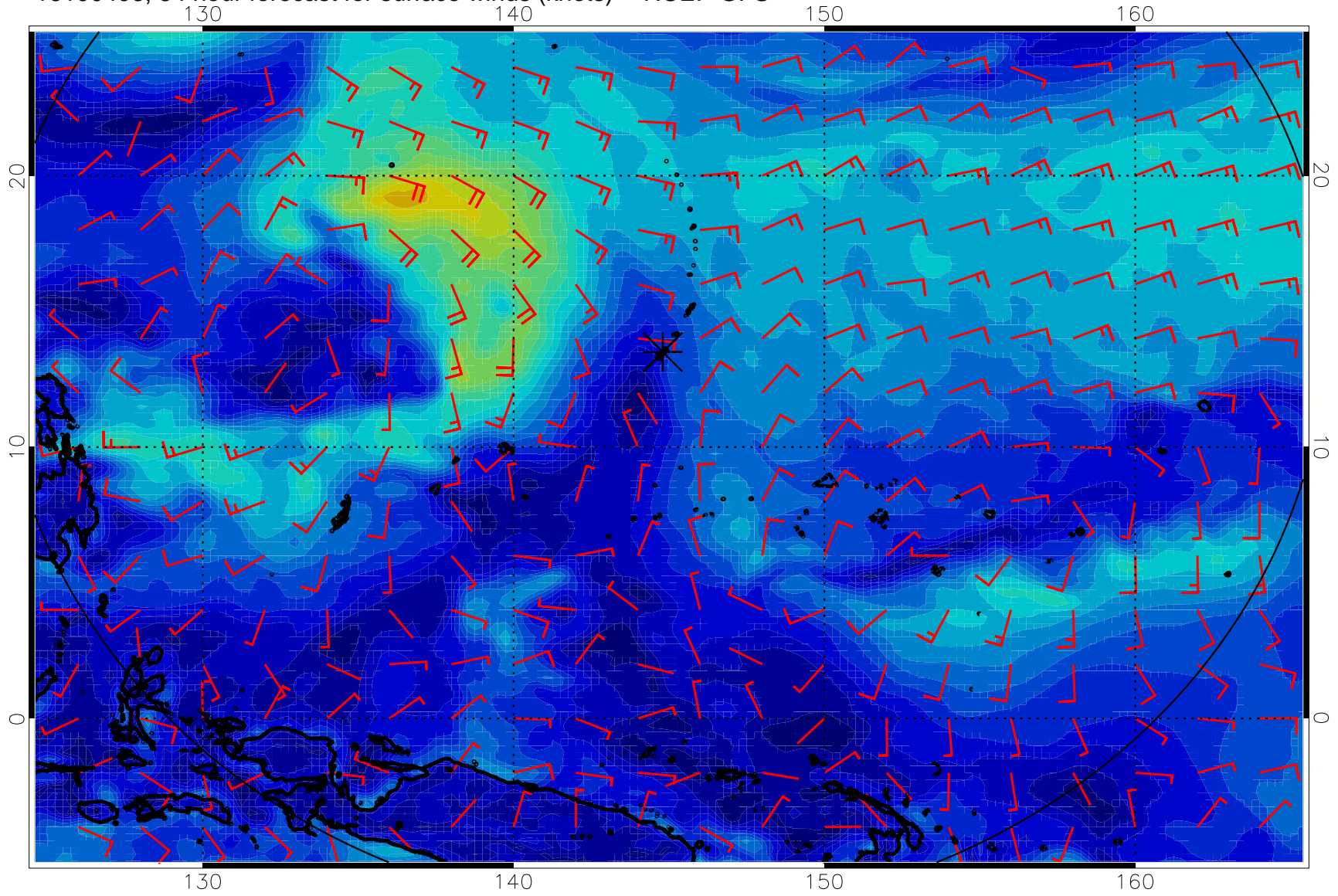
16100406, 54 hour forecast for surface winds (knots) -- NCEP GFS
