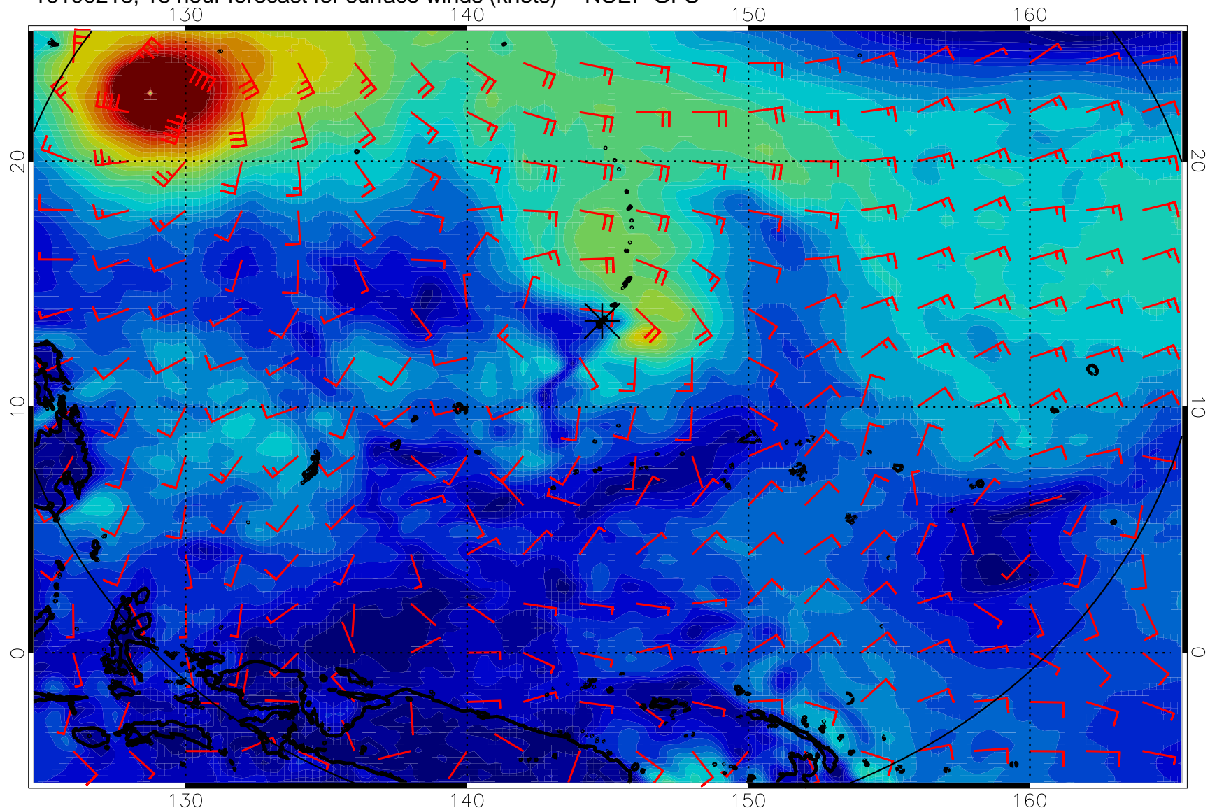
16100218, 18 hour forecast for surface winds (knots) -- NCEP GFS
