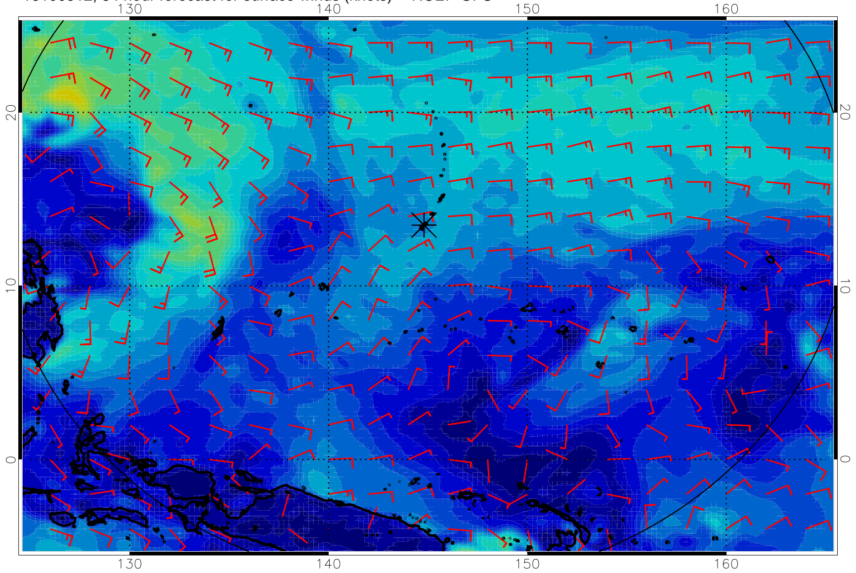
16100512, 84 hour forecast for surface winds (knots) -- NCEP GFS
