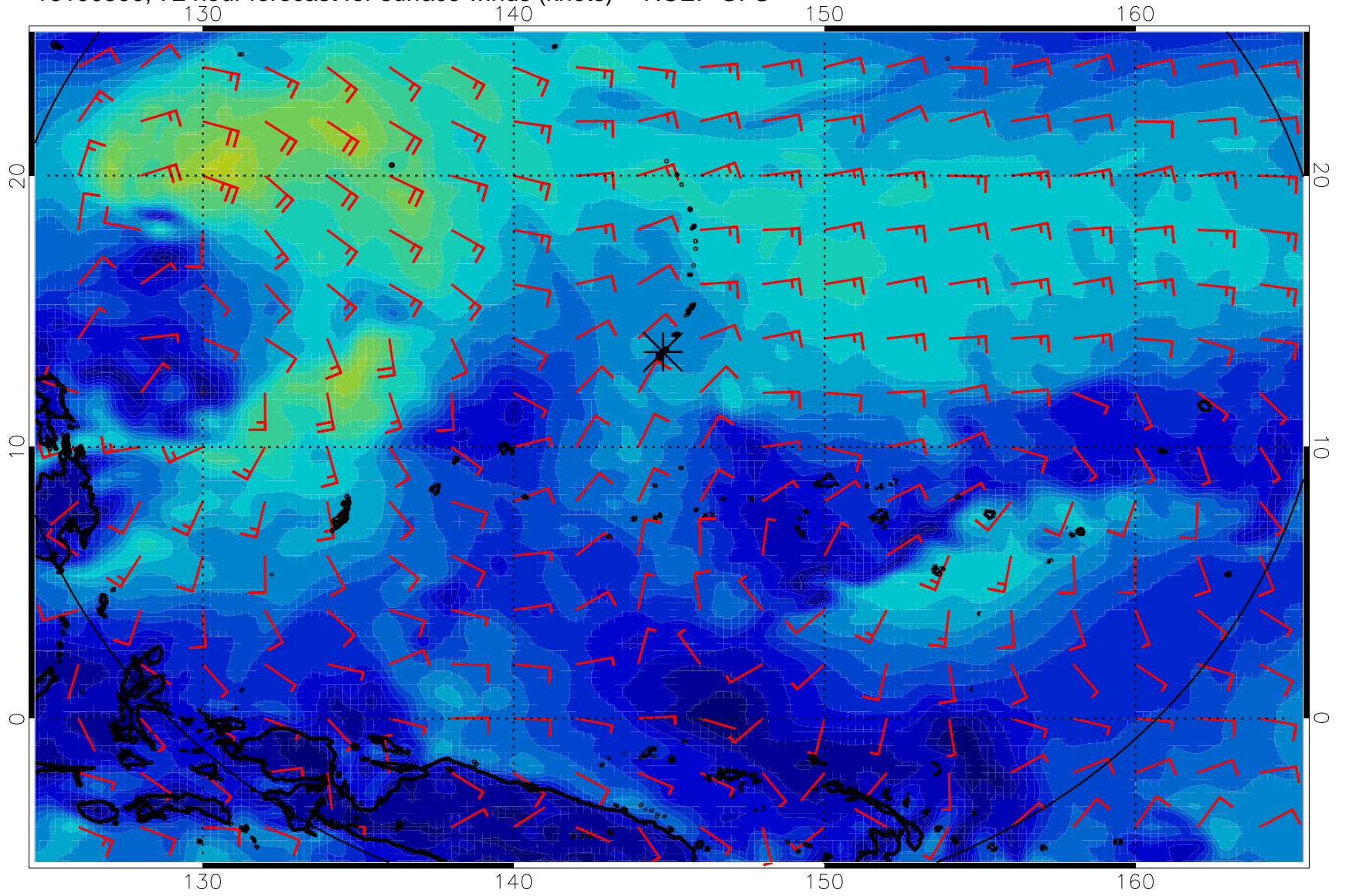
16100500, 72 hour forecast for surface winds (knots) -- NCEP GFS
