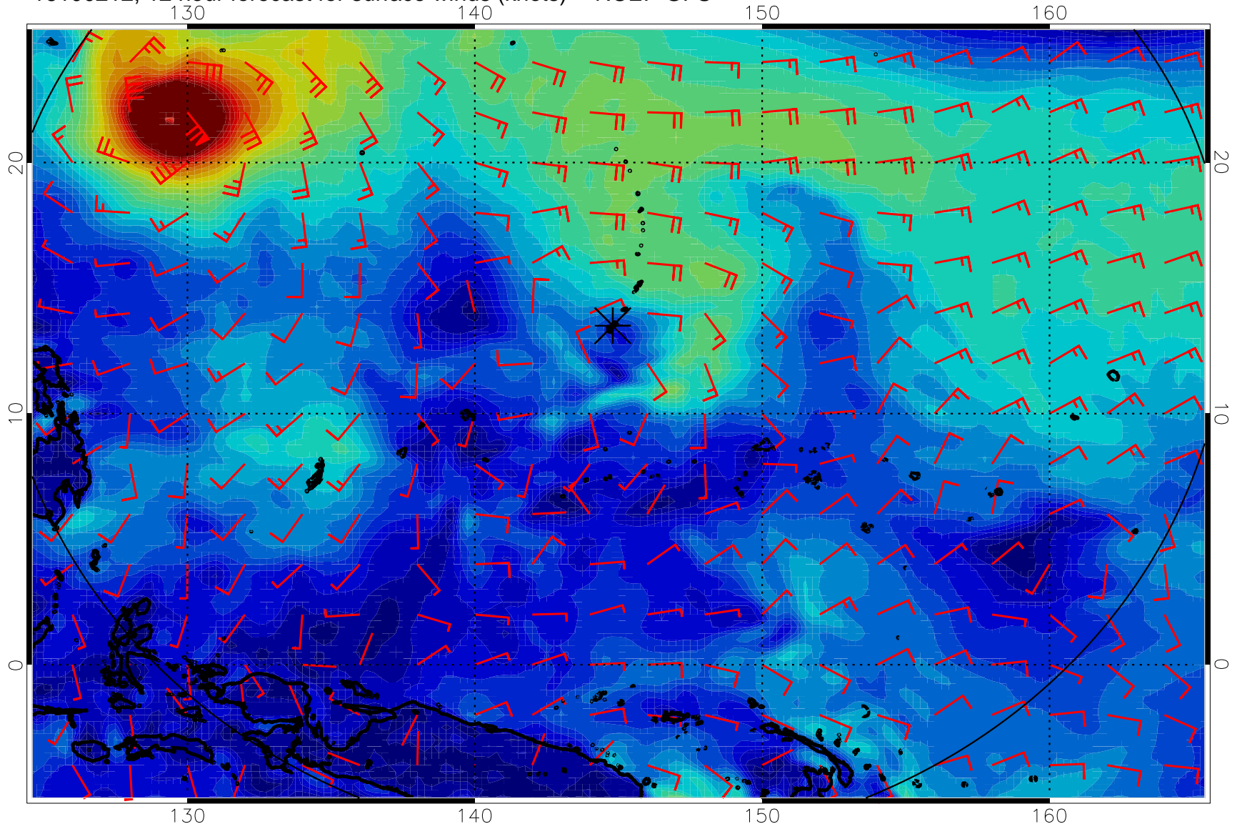
16100212, 12 hour forecast for surface winds (knots) -- NCEP GFS
