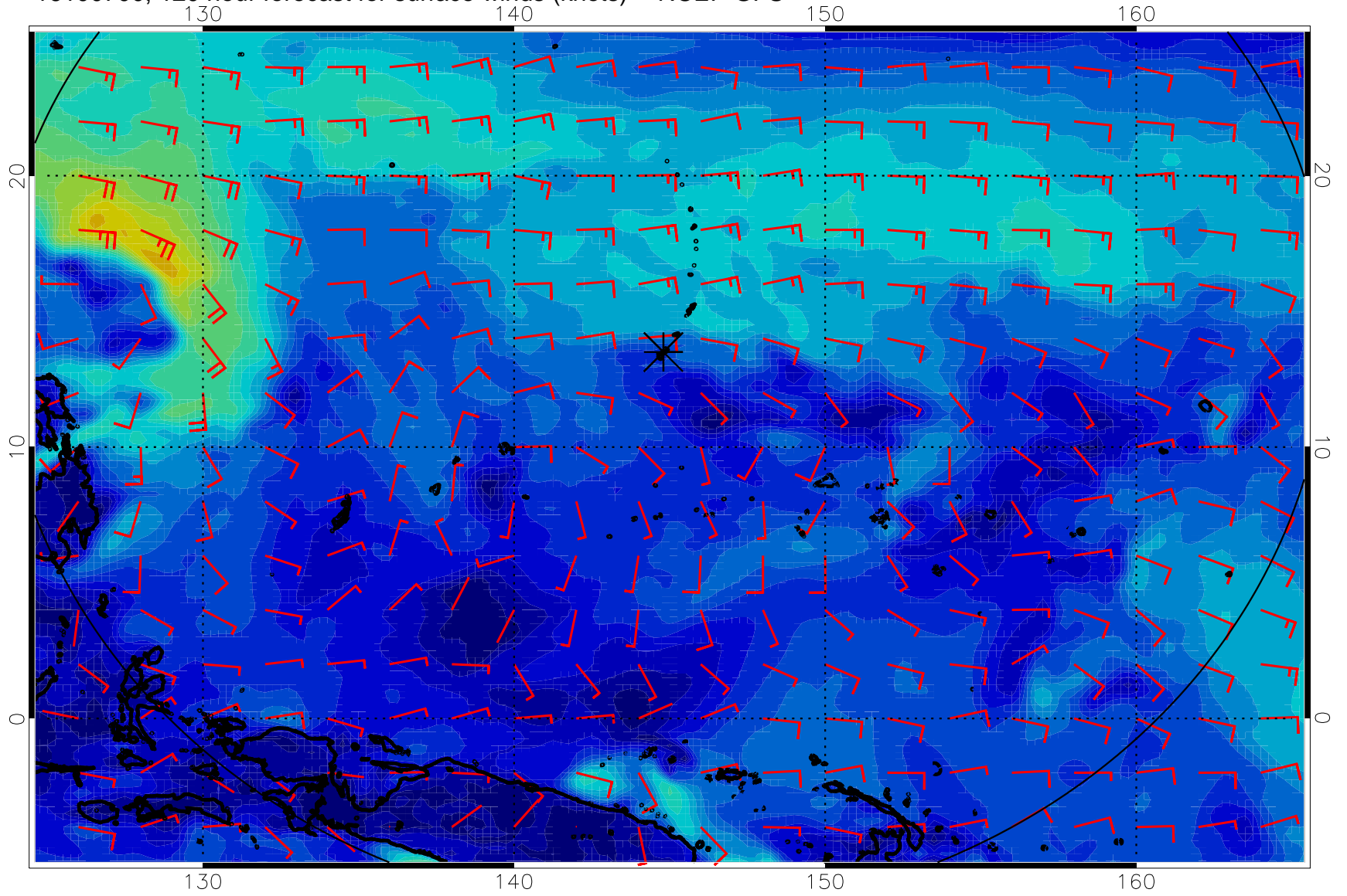
16100700, 120 hour forecast for surface winds (knots) -- NCEP GFS
