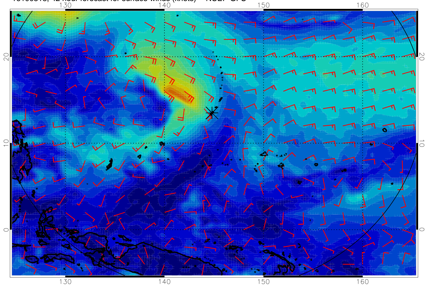
16100318, 42 hour forecast for surface winds (knots) -- NCEP GFS
