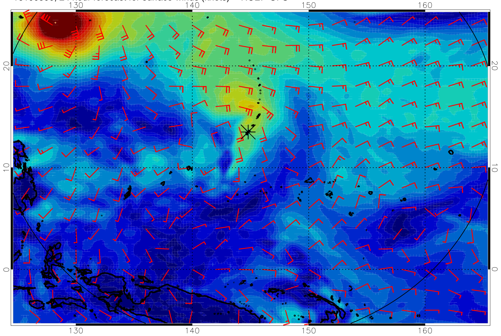
16100300, 24 hour forecast for surface winds (knots) -- NCEP GFS
