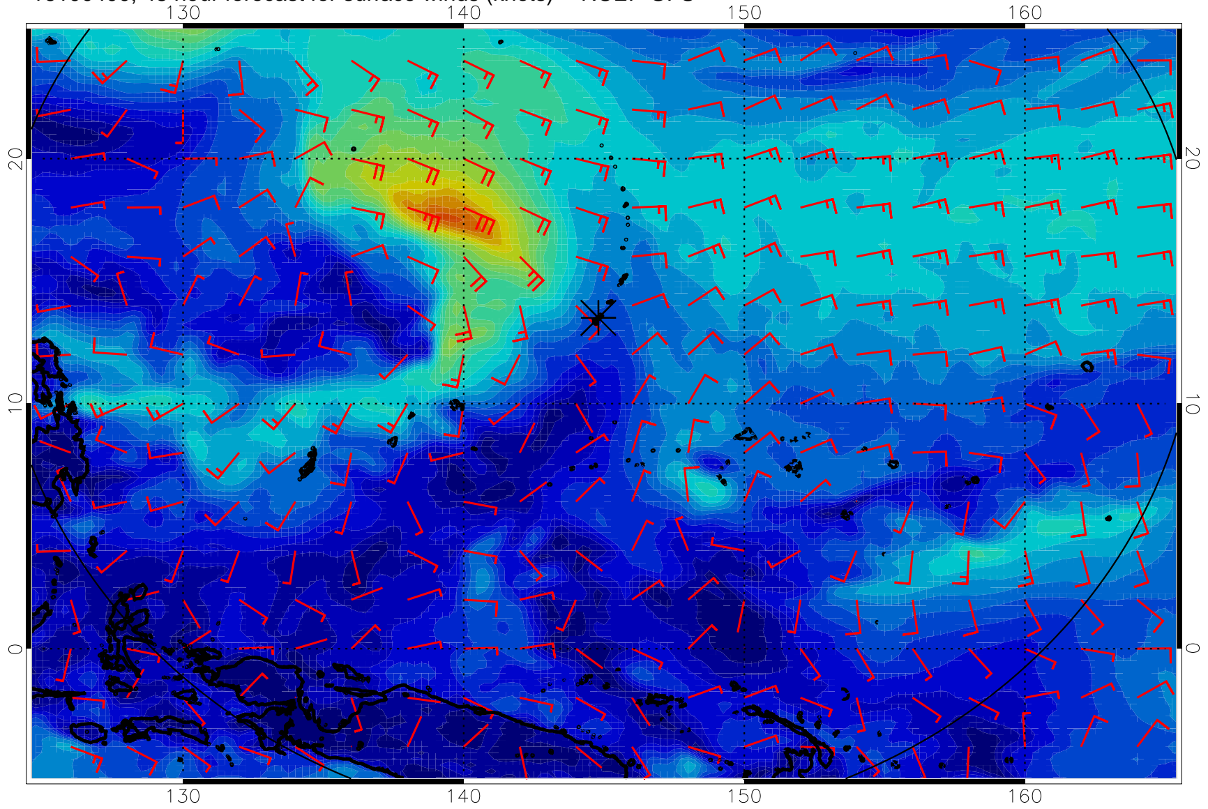
16100400, 48 hour forecast for surface winds (knots) -- NCEP GFS
