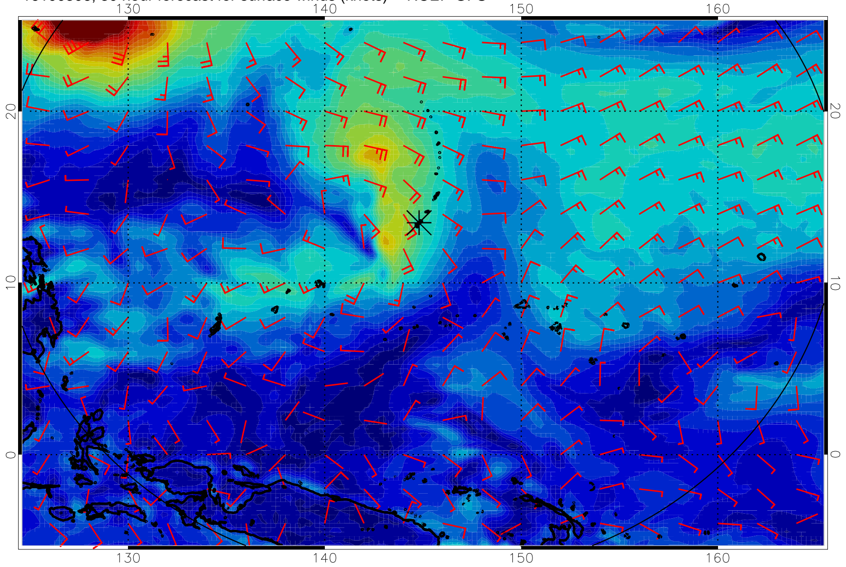
16100306, 30 hour forecast for surface winds (knots) -- NCEP GFS
