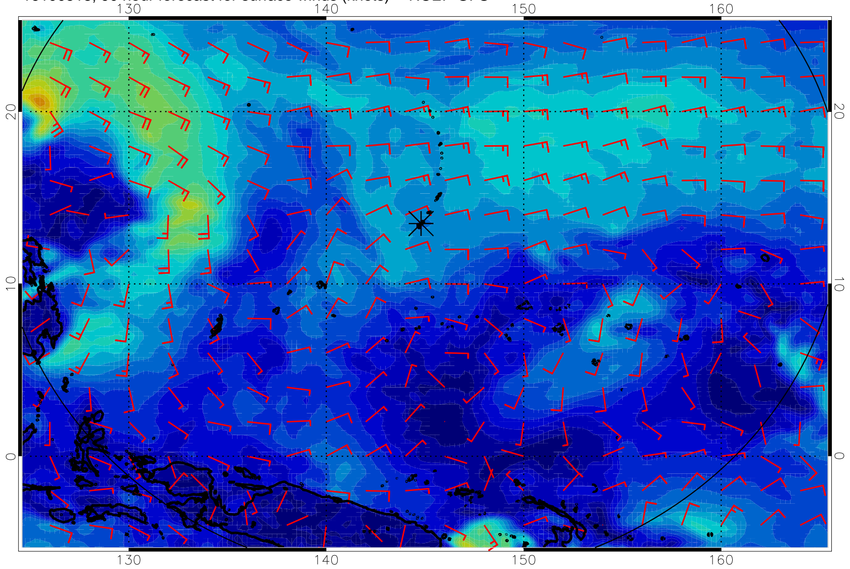
16100518, 90 hour forecast for surface winds (knots) -- NCEP GFS
