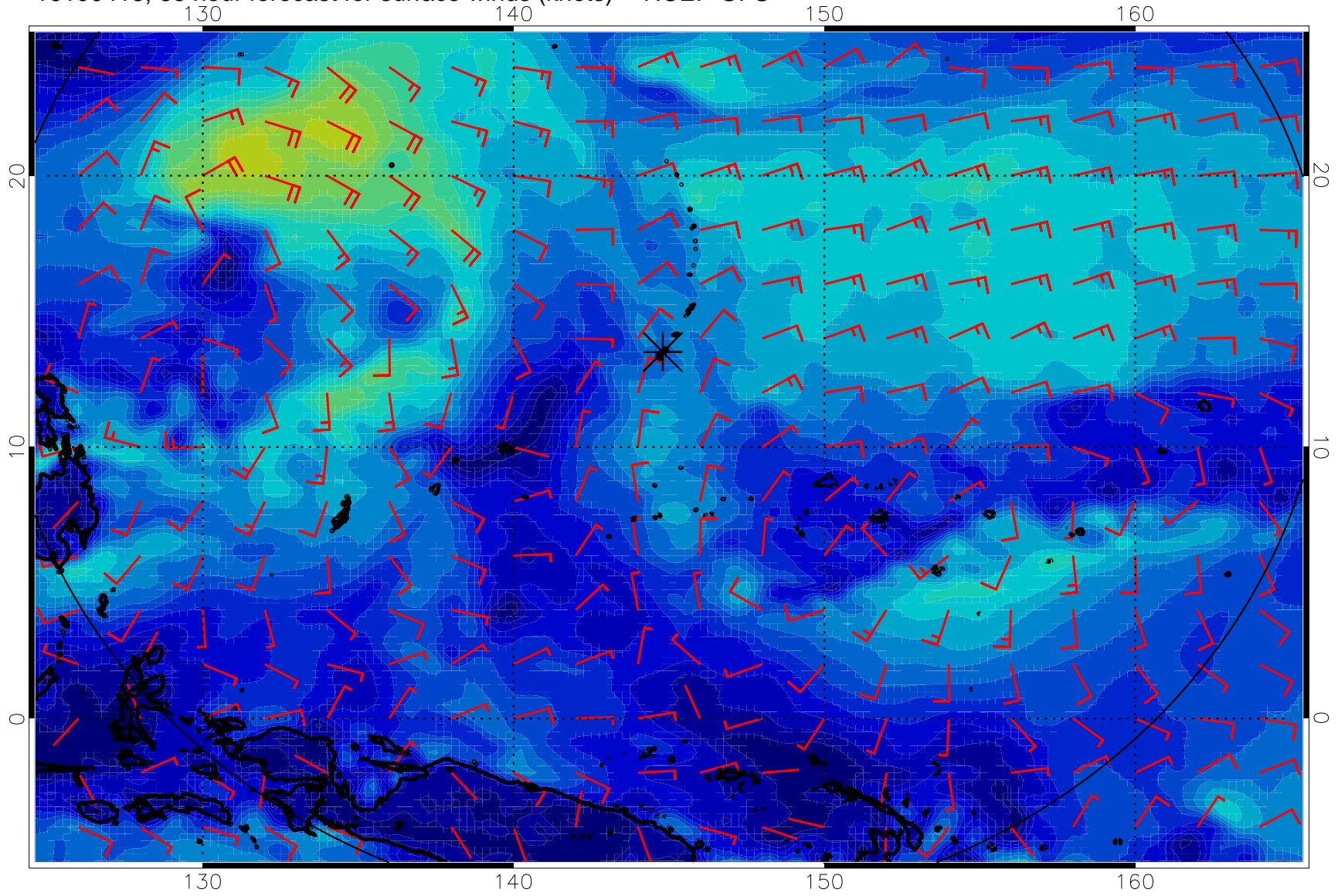
16100418, 66 hour forecast for surface winds (knots) -- NCEP GFS
