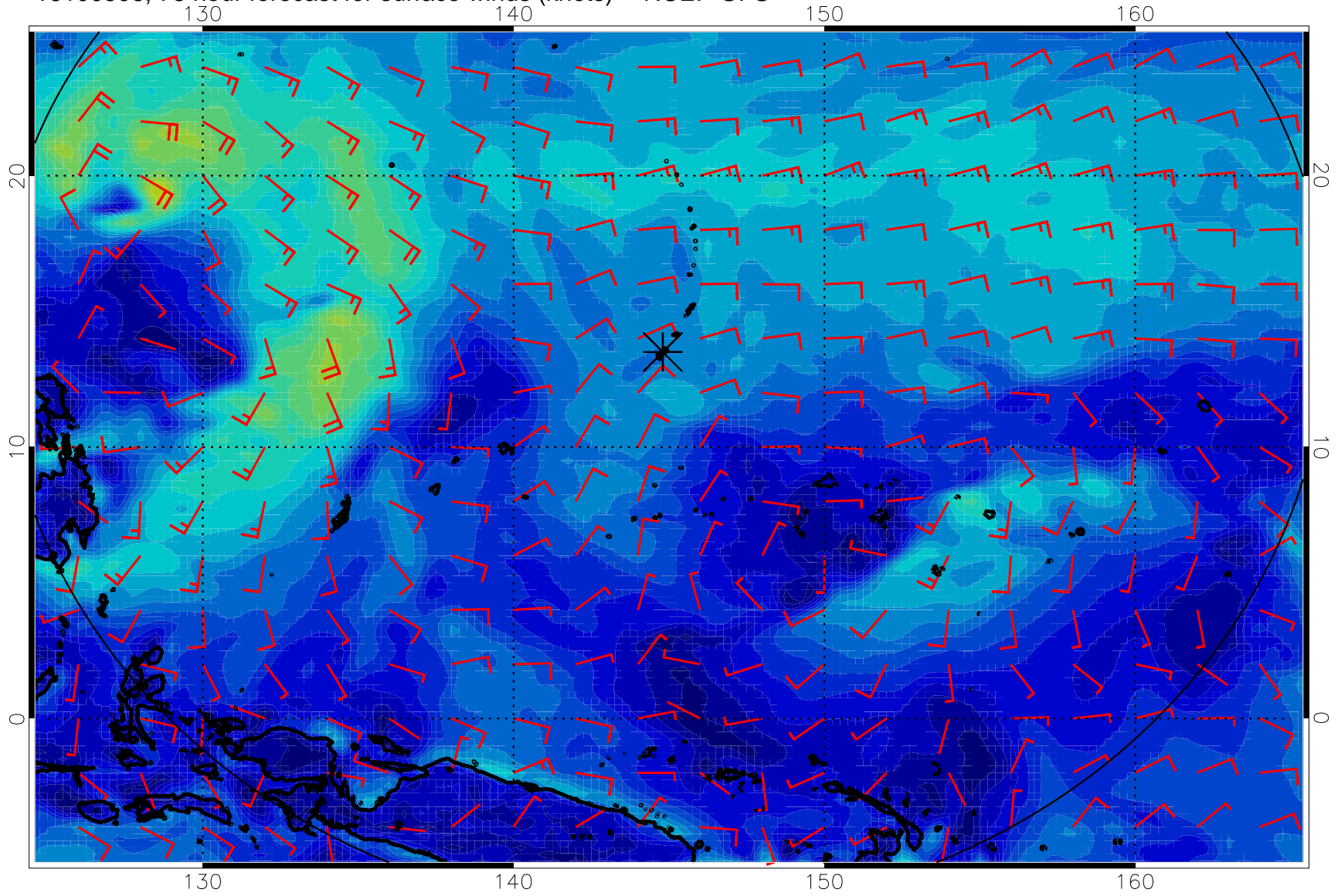
16100506, 78 hour forecast for surface winds (knots) -- NCEP GFS
