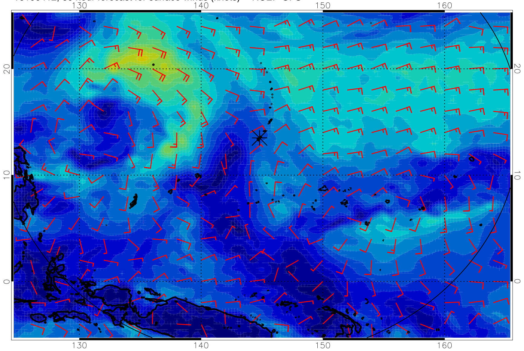
16100412, 60 hour forecast for surface winds (knots) -- NCEP GFS
