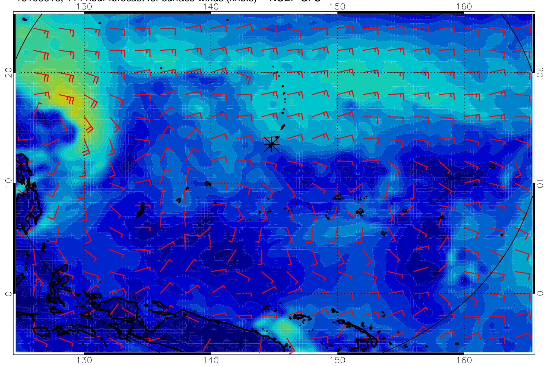
16100618, 114 hour forecast for surface winds (knots) -- NCEP GFS
