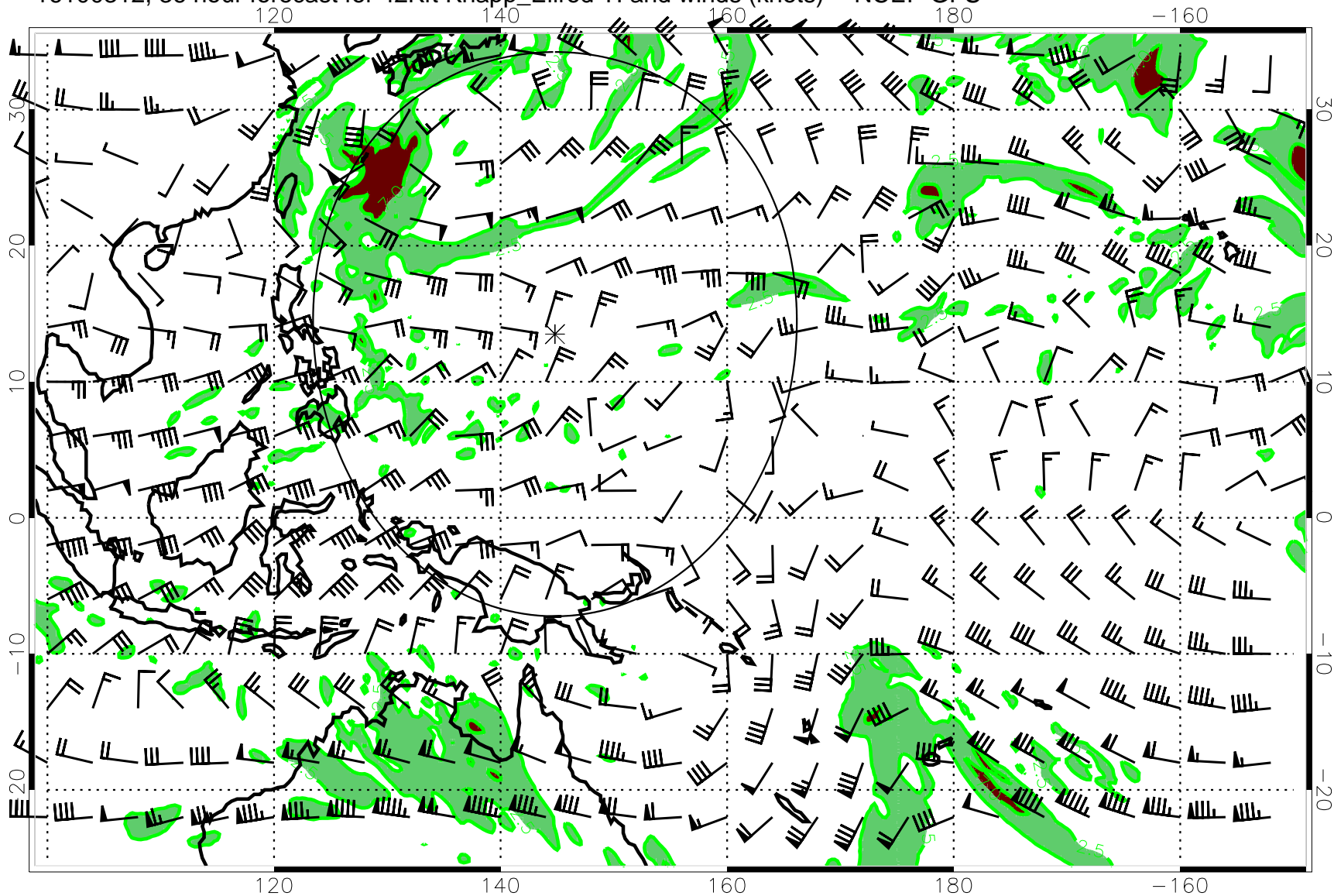
16100312, 36 hour forecast for 42Kft Knapp_Ellrod TI and winds (knots) -- NCEP GFS
