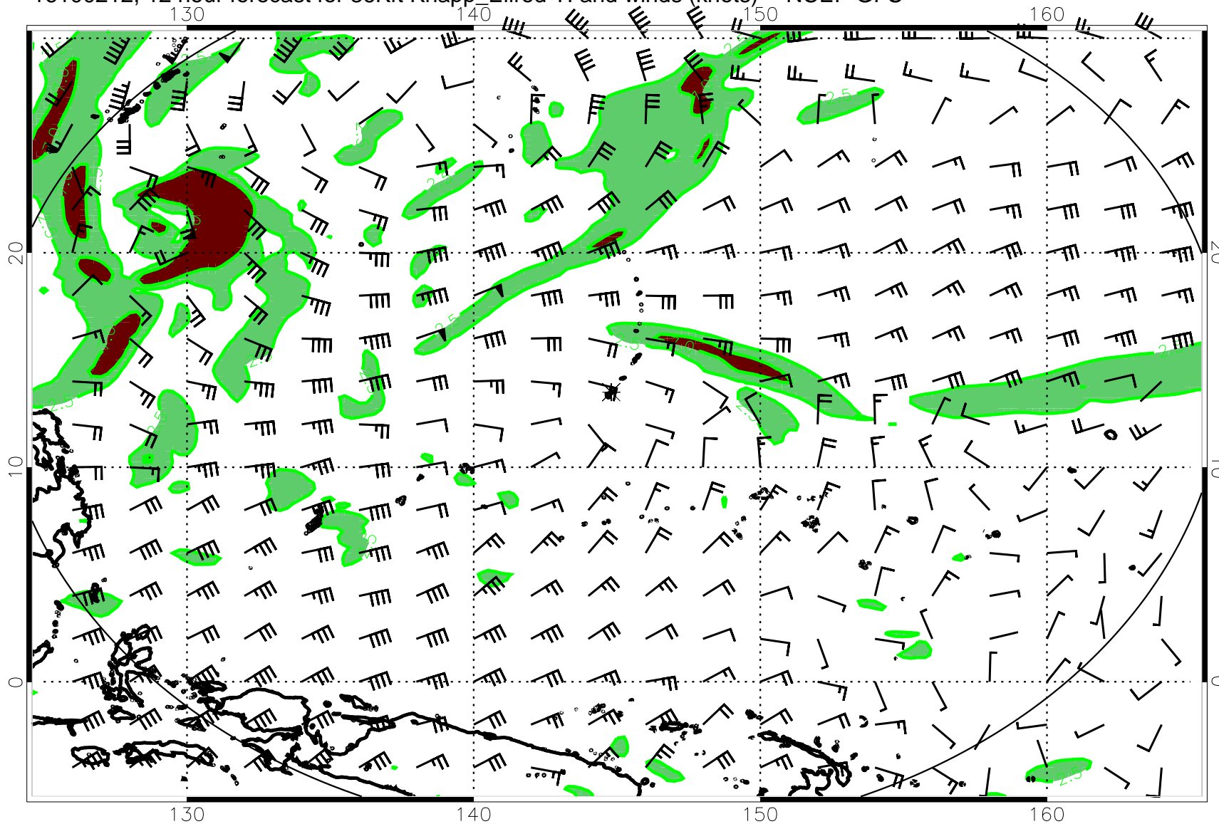
16100212, 12 hour forecast for 36Kft Knapp_Ellrod TI and winds (knots) -- NCEP GFS
