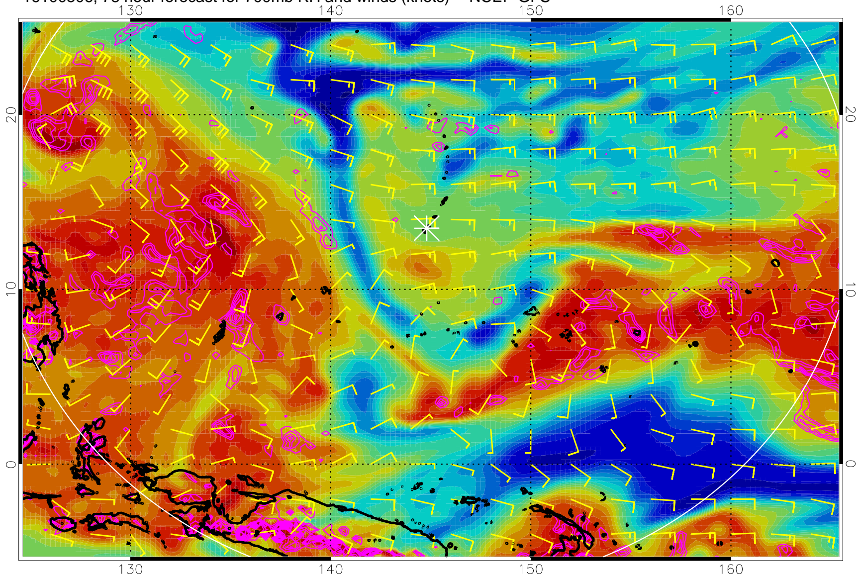
16100506, 78 hour forecast for 700mb RH and winds (knots) -- NCEP GFS
