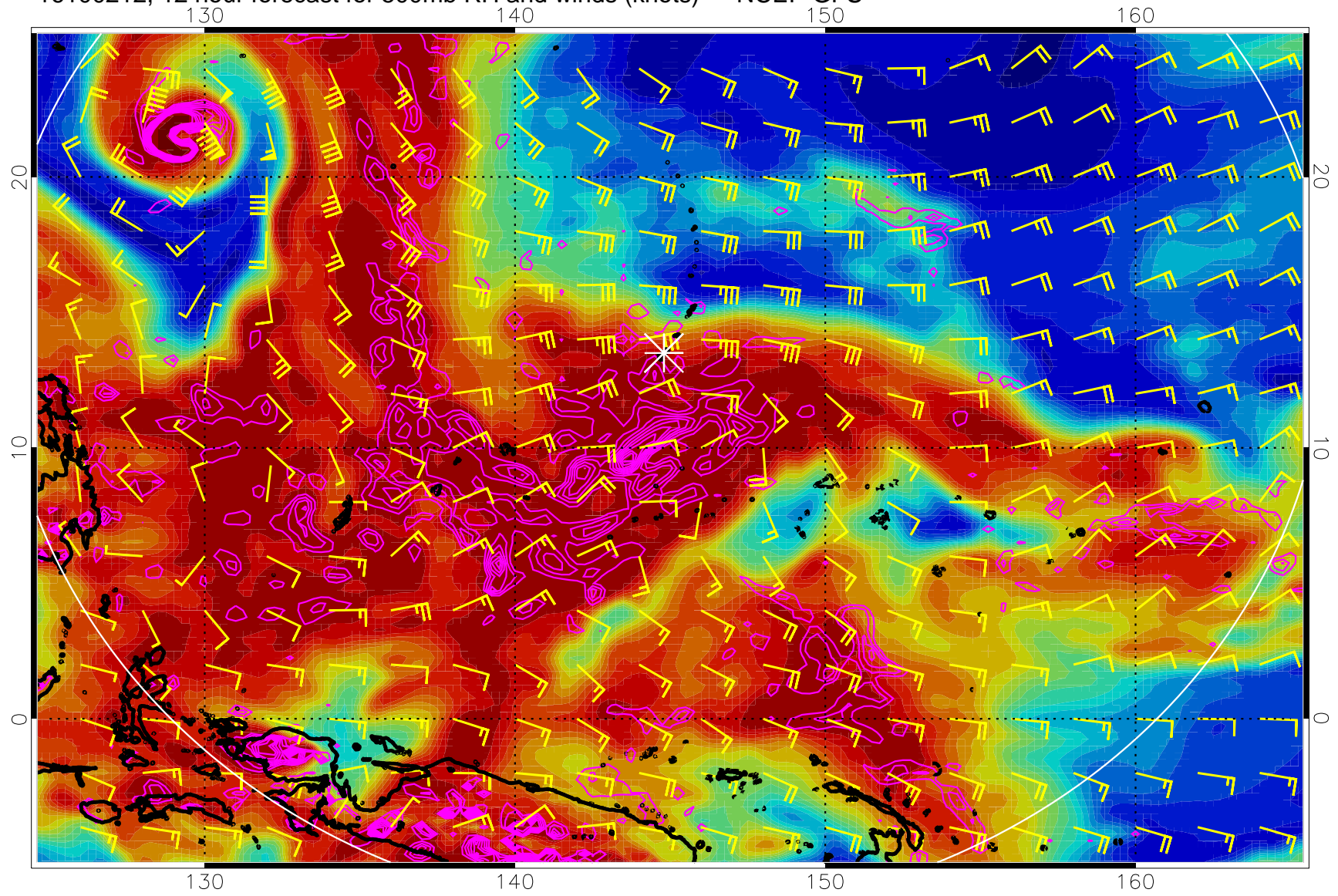
16100212, 12 hour forecast for 500mb RH and winds (knots) -- NCEP GFS
