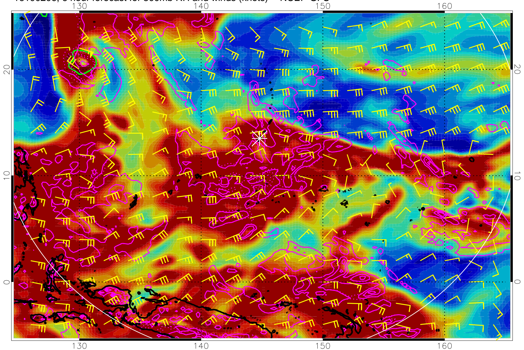
16100206, 6 hour forecast for 300mb RH and winds (knots) -- NCEP GFS
