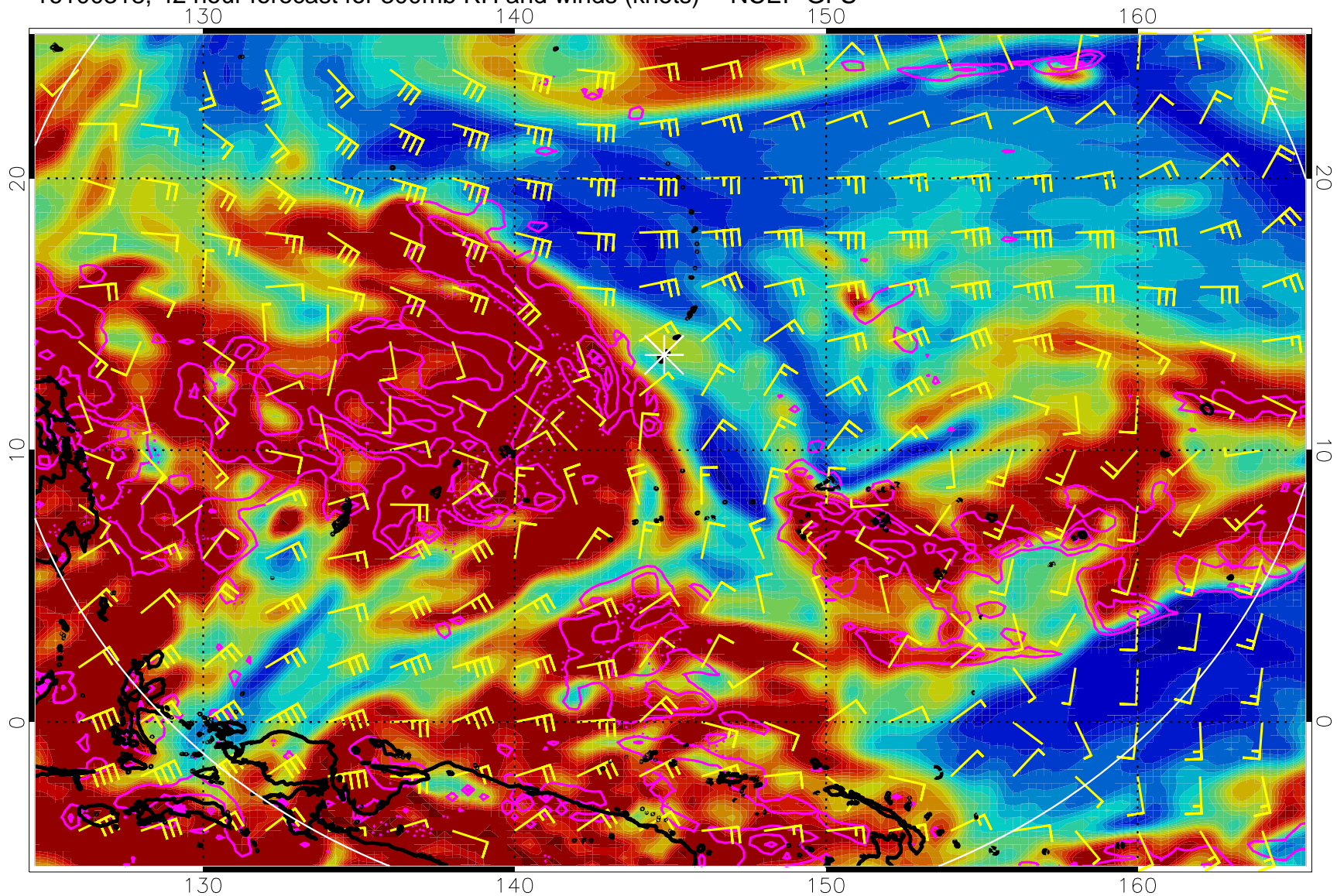
16100318, 42 hour forecast for 300mb RH and winds (knots) -- NCEP GFS
