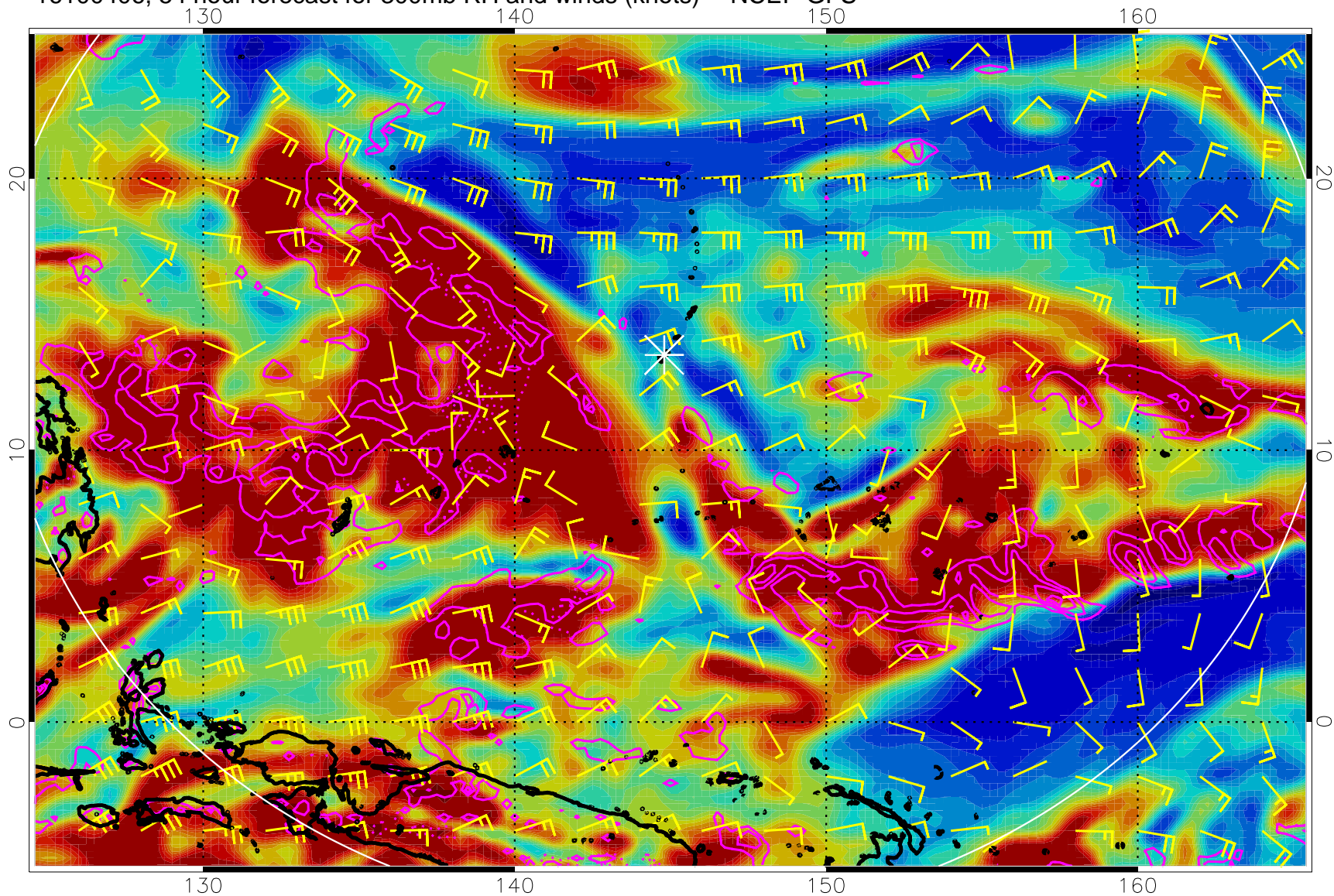
16100406, 54 hour forecast for 300mb RH and winds (knots) -- NCEP GFS
