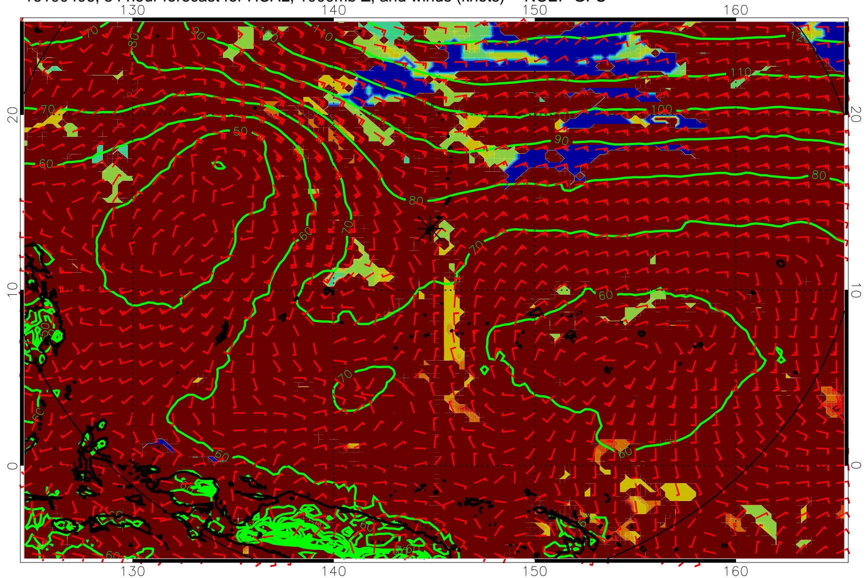
16100406, 54 hour forecast for HCAL, 1000mb Z, and winds (knots) -- NCEP GFS
