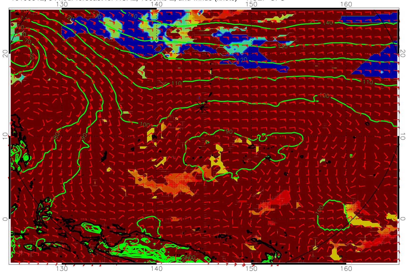
16100512, 84 hour forecast for HCAL, 1000mb Z, and winds (knots) -- NCEP GFS
