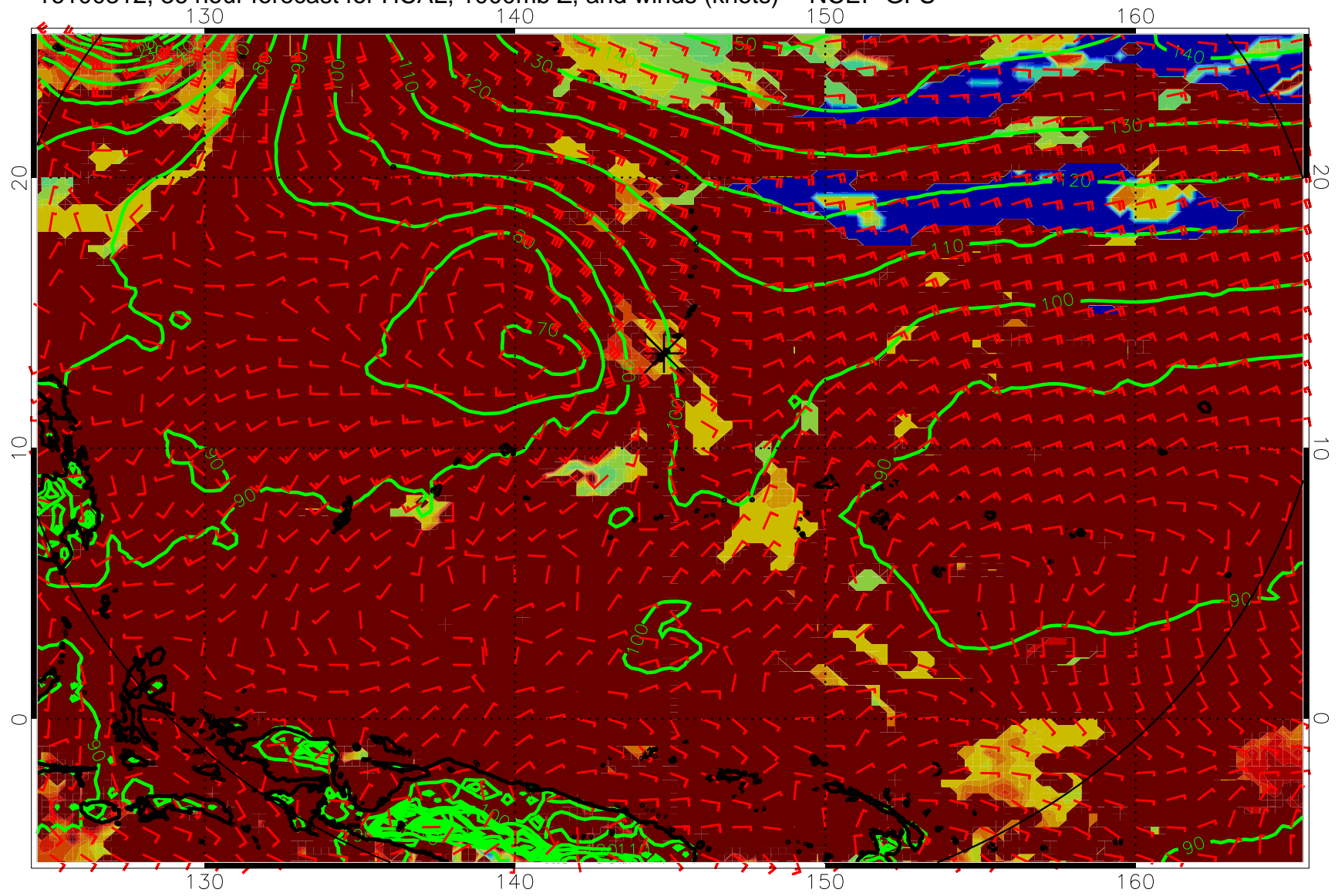
16100312, 36 hour forecast for HCAL, 1000mb Z, and winds (knots) -- NCEP GFS
