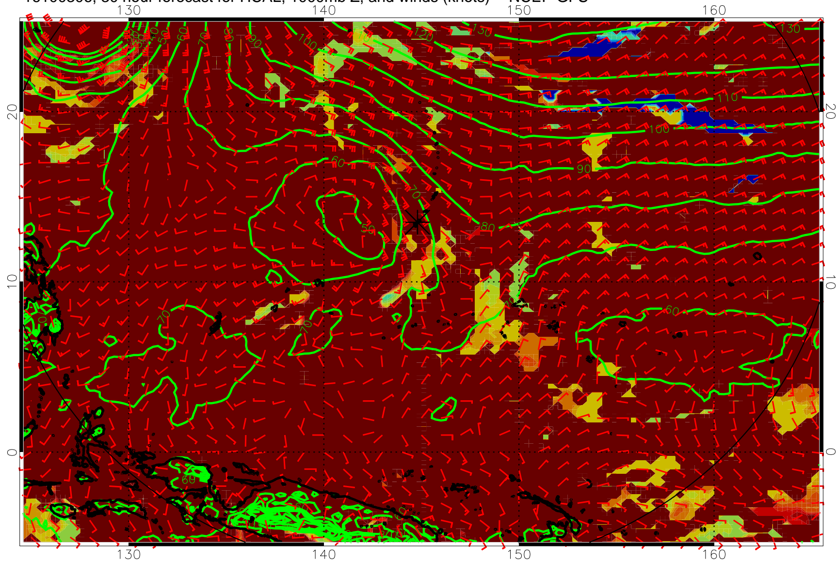
16100306, 30 hour forecast for HCAL, 1000mb Z, and winds (knots) -- NCEP GFS
