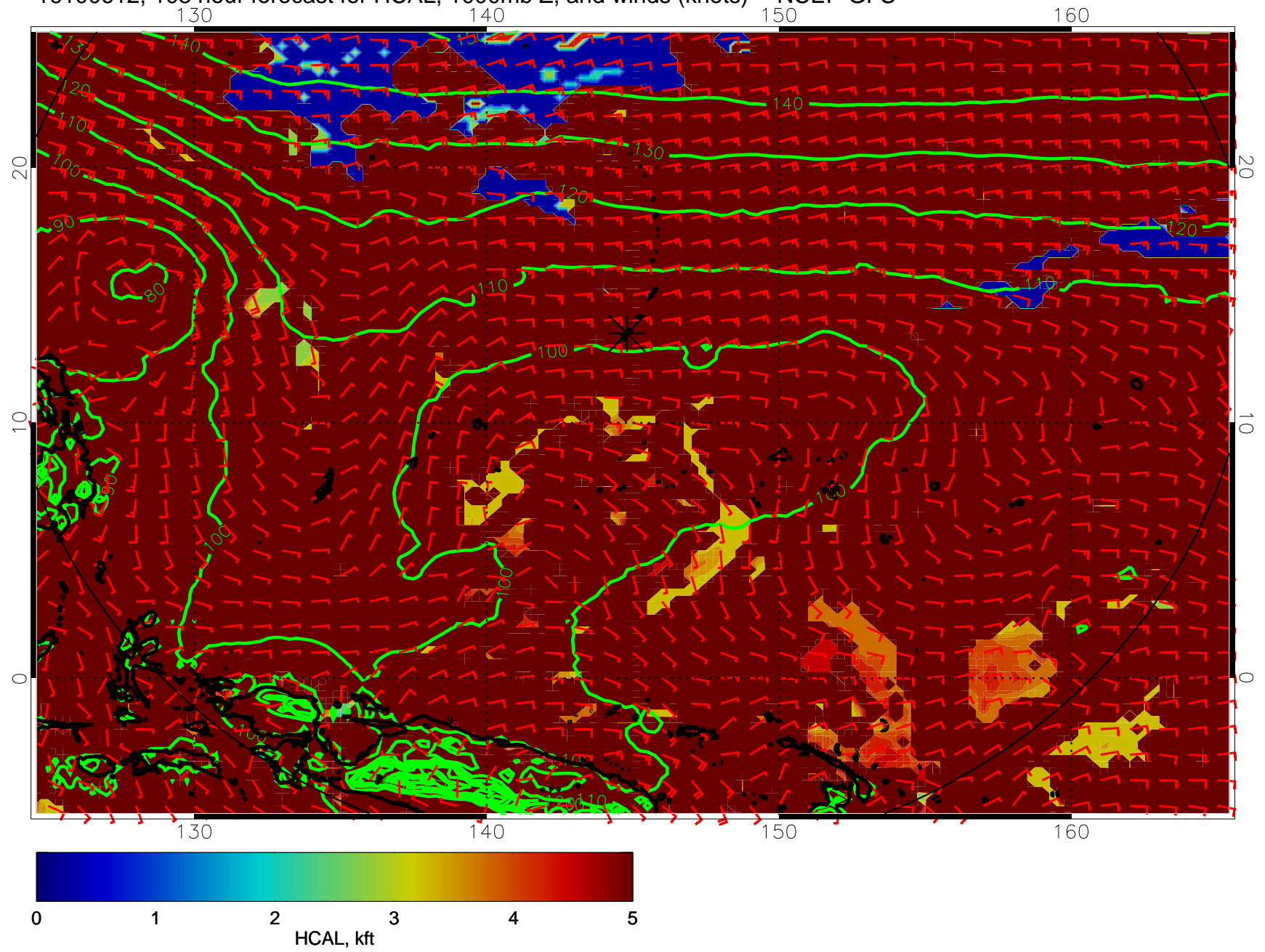
16100612, 108 hour forecast for HCAL, 1000mb Z, and winds (knots) -- NCEP GFS
