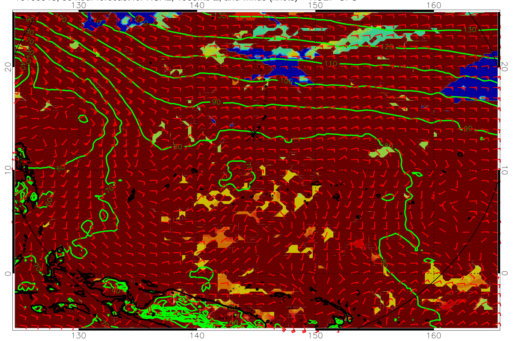
16100518, 90 hour forecast for HCAL, 1000mb Z, and winds (knots) -- NCEP GFS
