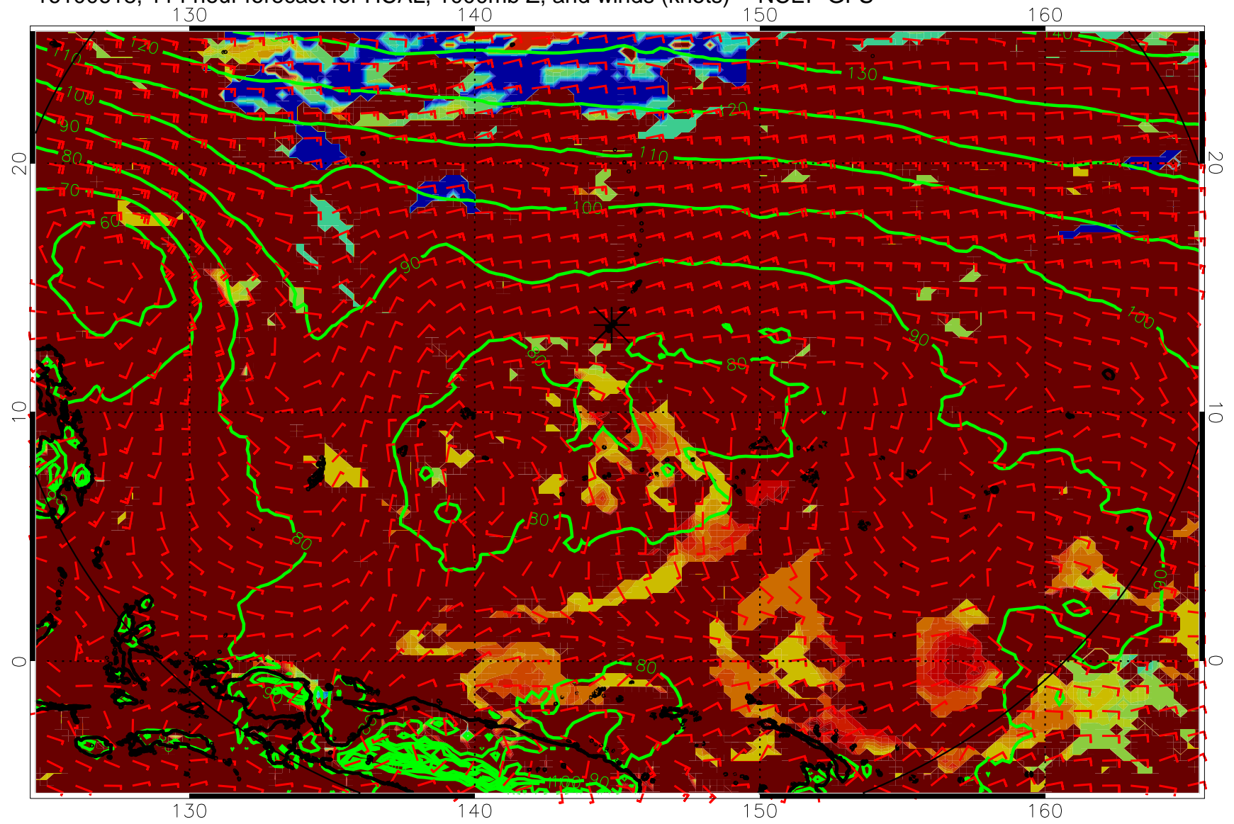
16100618, 114 hour forecast for HCAL, 1000mb Z, and winds (knots) -- NCEP GFS
