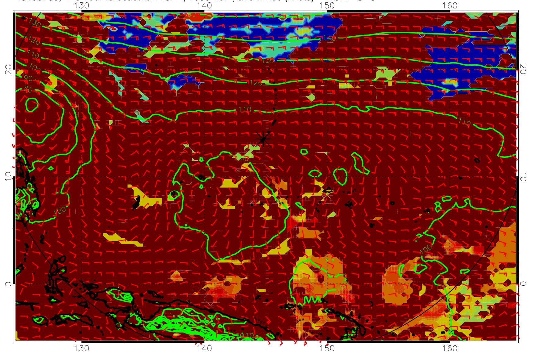
16100700, 120 hour forecast for HCAL, 1000mb Z, and winds (knots) -- NCEP GFS
