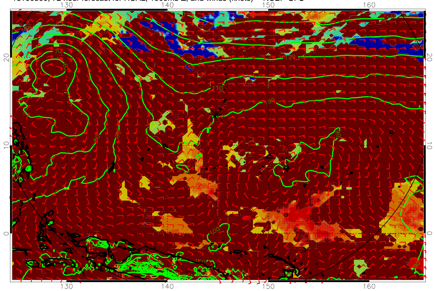
16100500, 72 hour forecast for HCAL, 1000mb Z, and winds (knots) -- NCEP GFS
