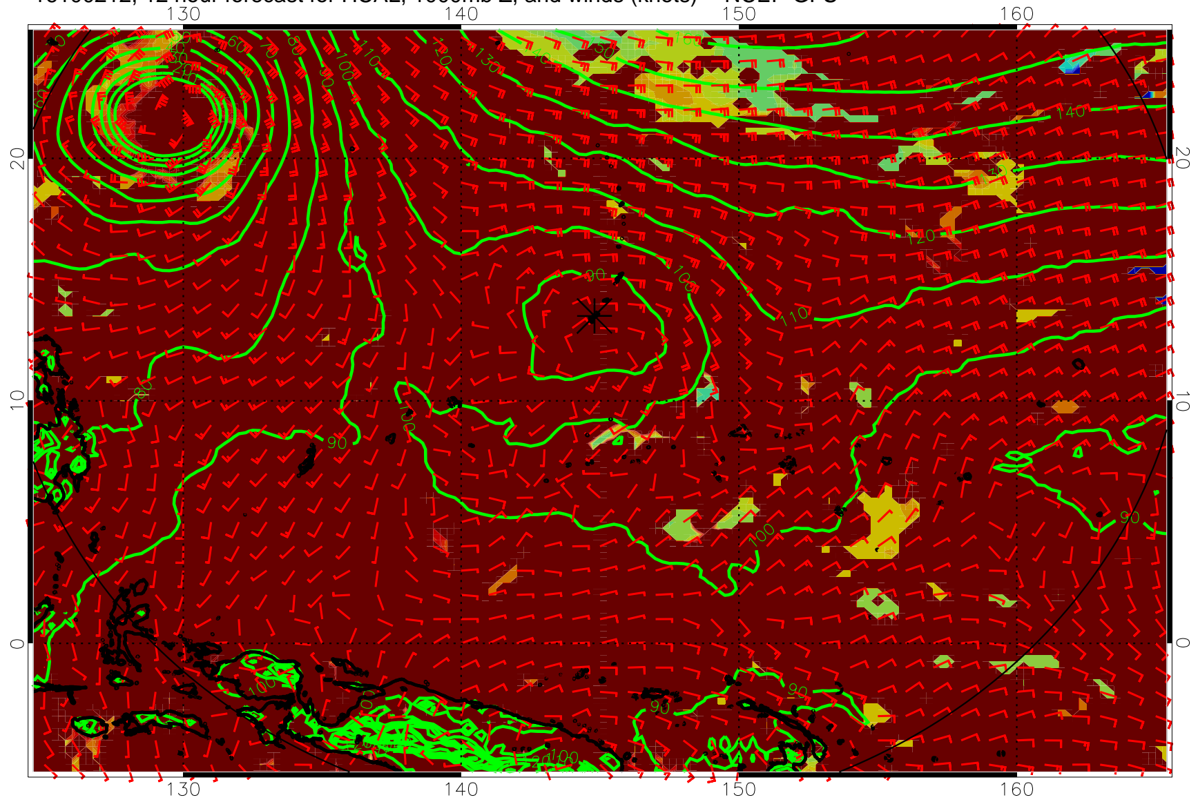
16100212, 12 hour forecast for HCAL, 1000mb Z, and winds (knots) -- NCEP GFS
