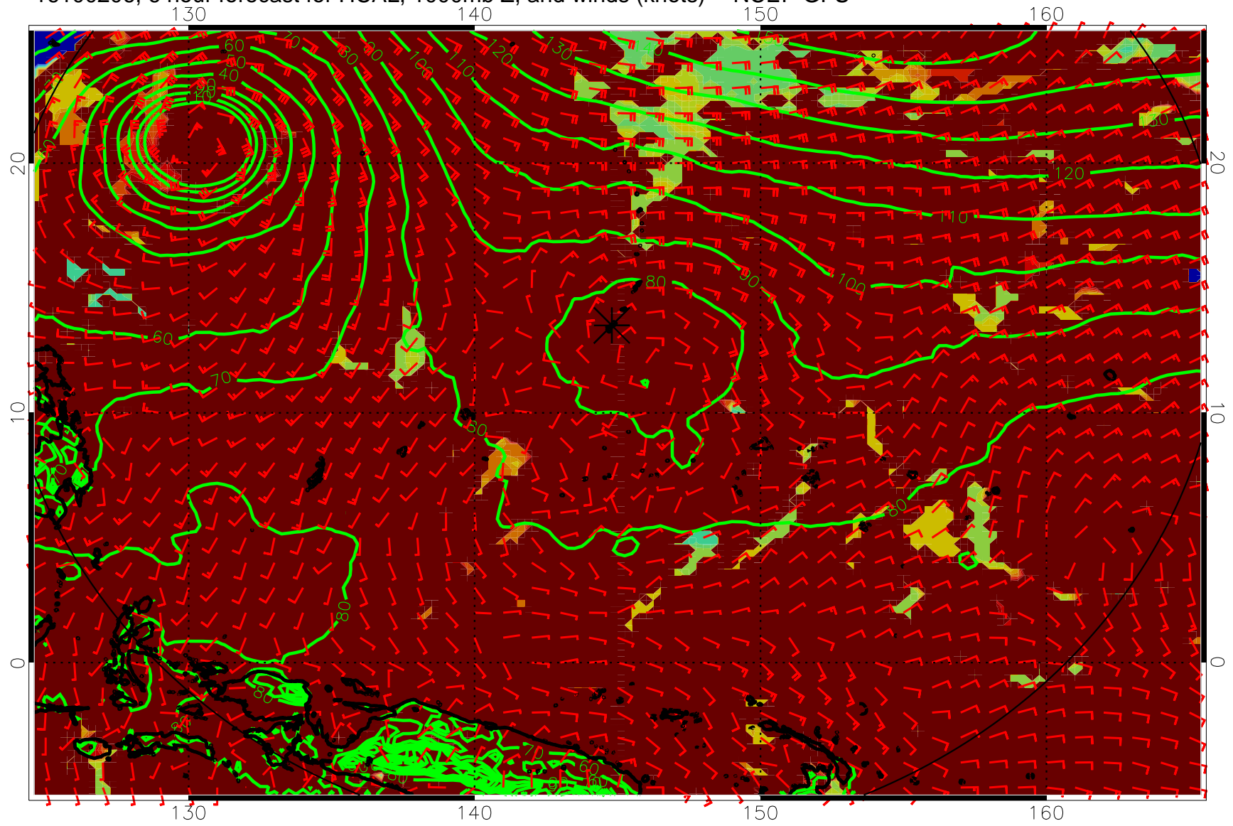
16100206, 6 hour forecast for HCAL, 1000mb Z, and winds (knots) -- NCEP GFS
