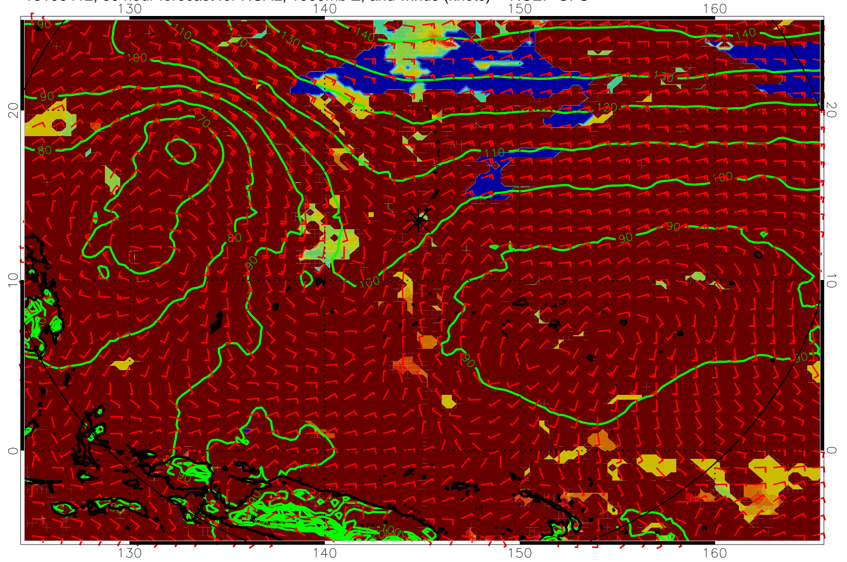
16100412, 60 hour forecast for HCAL, 1000mb Z, and winds (knots) -- NCEP GFS
