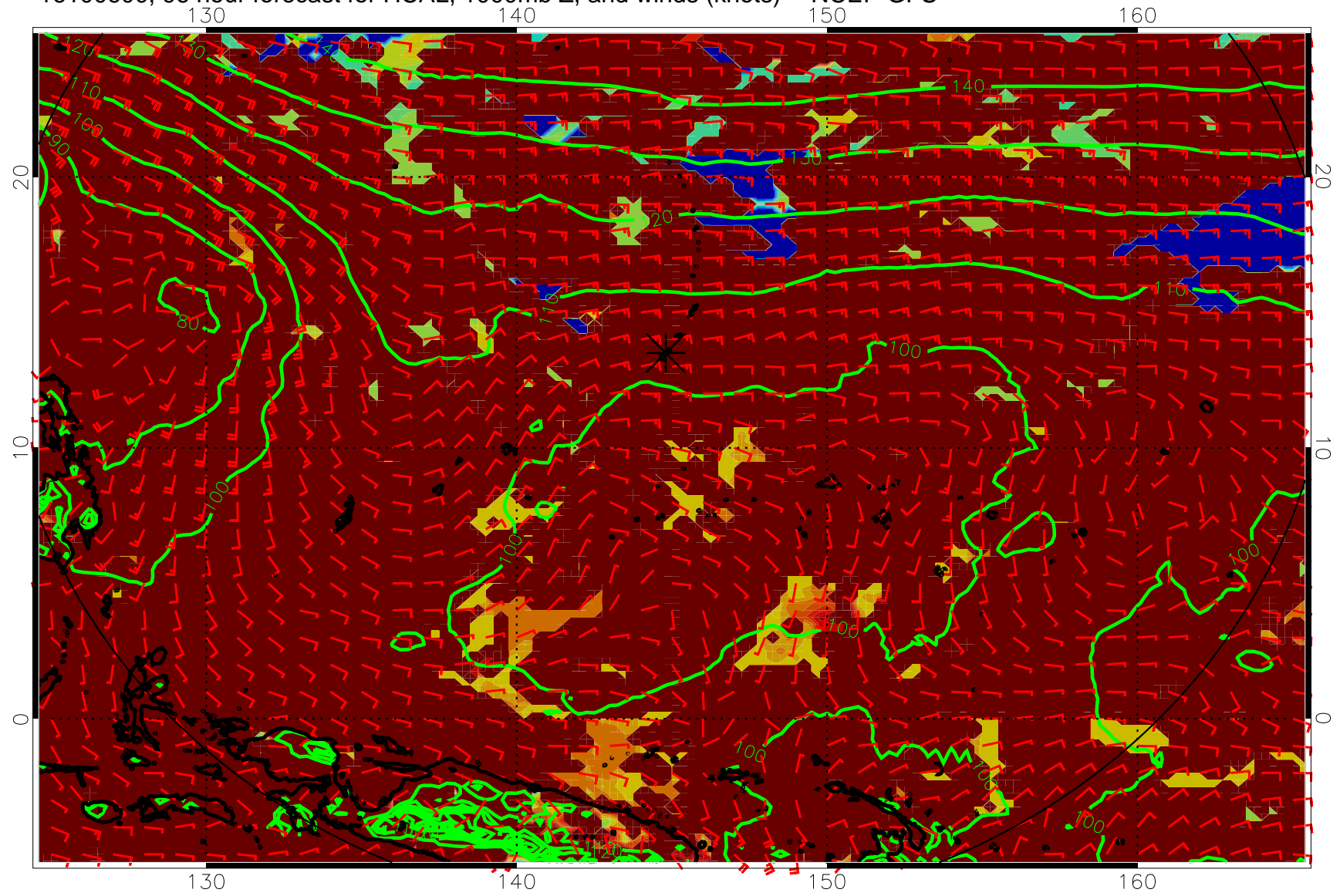
16100600, 96 hour forecast for HCAL, 1000mb Z, and winds (knots) -- NCEP GFS
