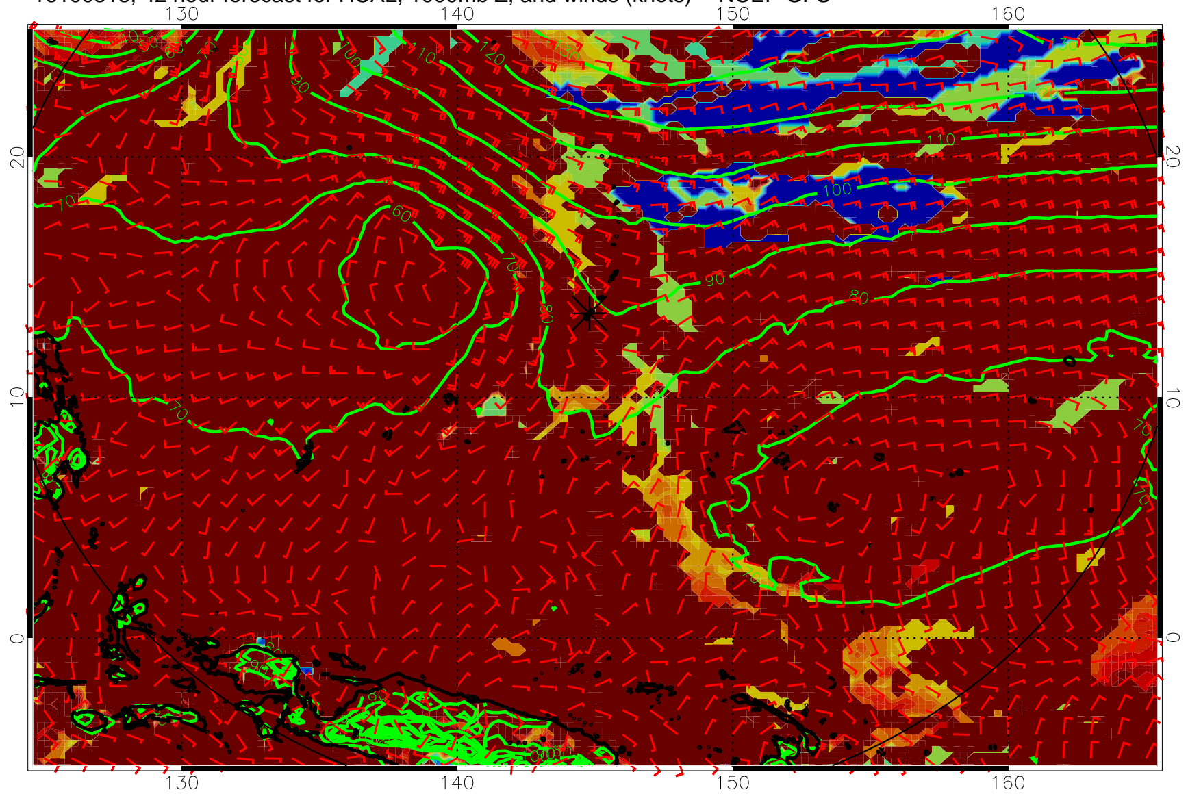
16100318, 42 hour forecast for HCAL, 1000mb Z, and winds (knots) -- NCEP GFS
