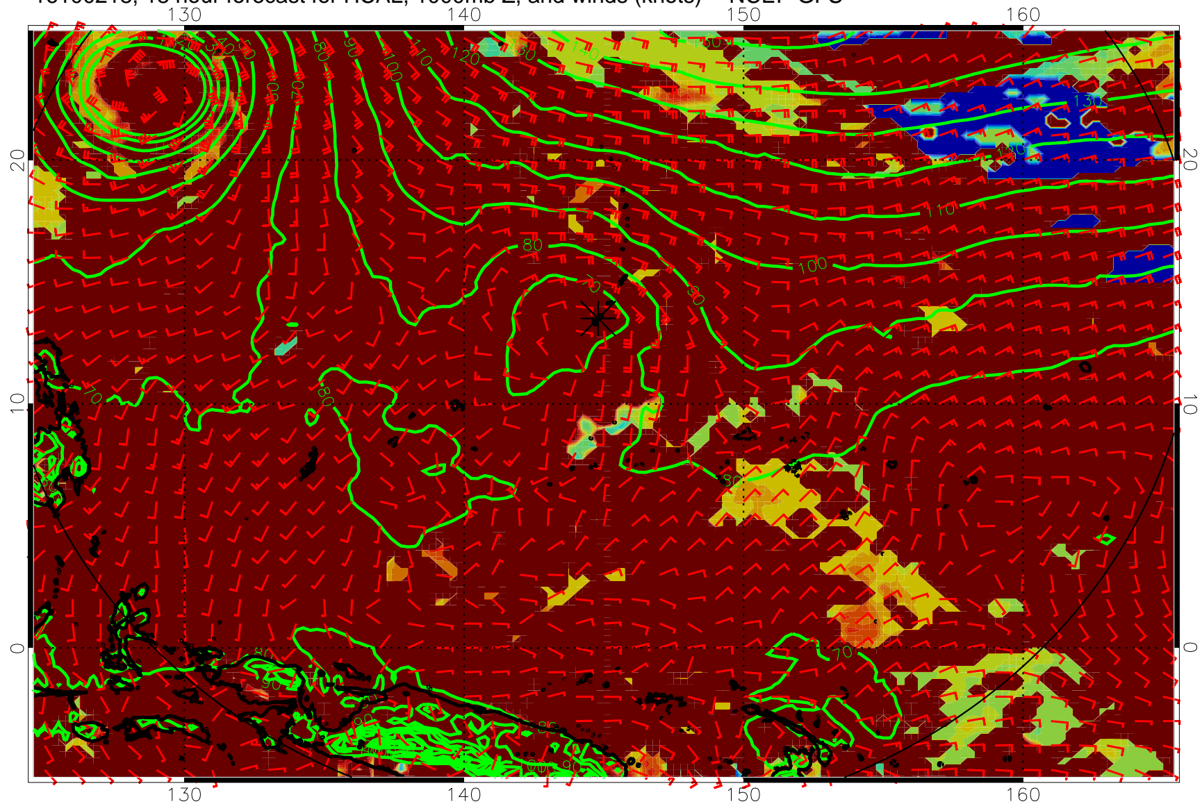
16100218, 18 hour forecast for HCAL, 1000mb Z, and winds (knots) -- NCEP GFS
