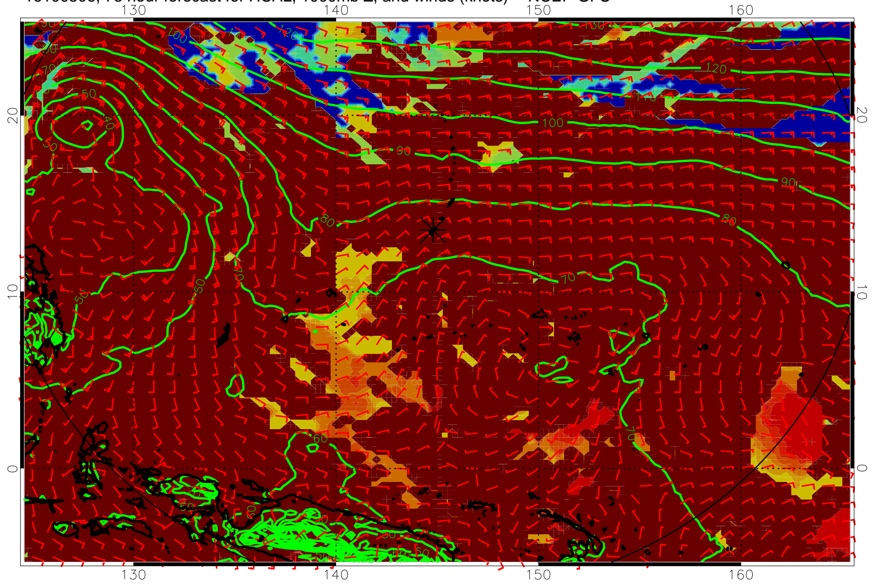
16100506, 78 hour forecast for HCAL, 1000mb Z, and winds (knots) -- NCEP GFS
