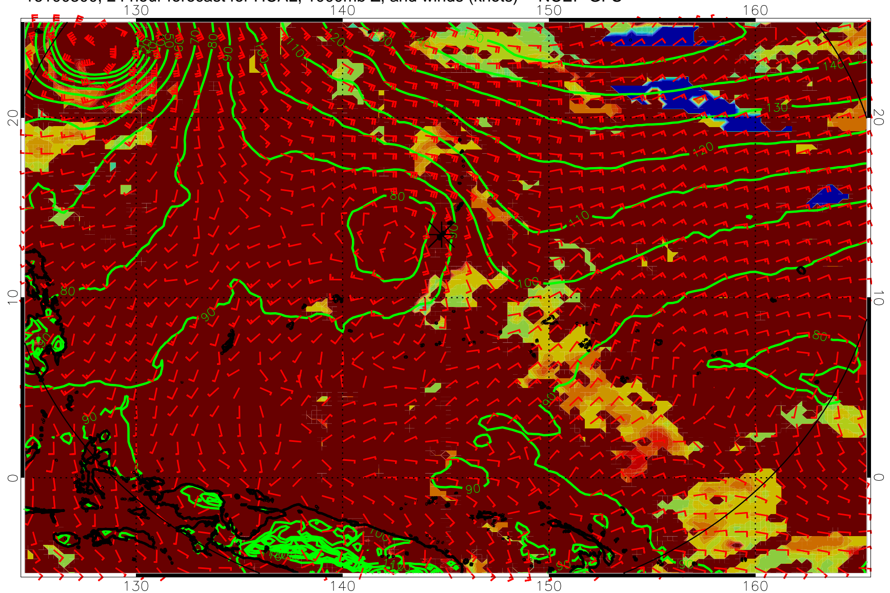
16100300, 24 hour forecast for HCAL, 1000mb Z, and winds (knots) -- NCEP GFS
