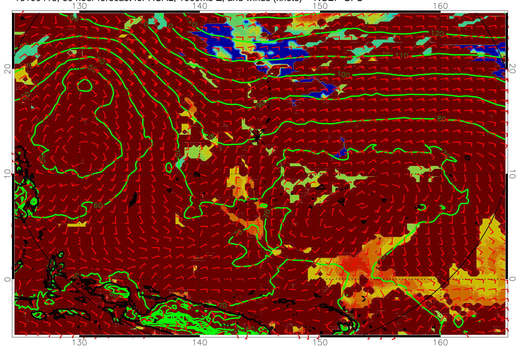
16100418, 66 hour forecast for HCAL, 1000mb Z, and winds (knots) -- NCEP GFS
