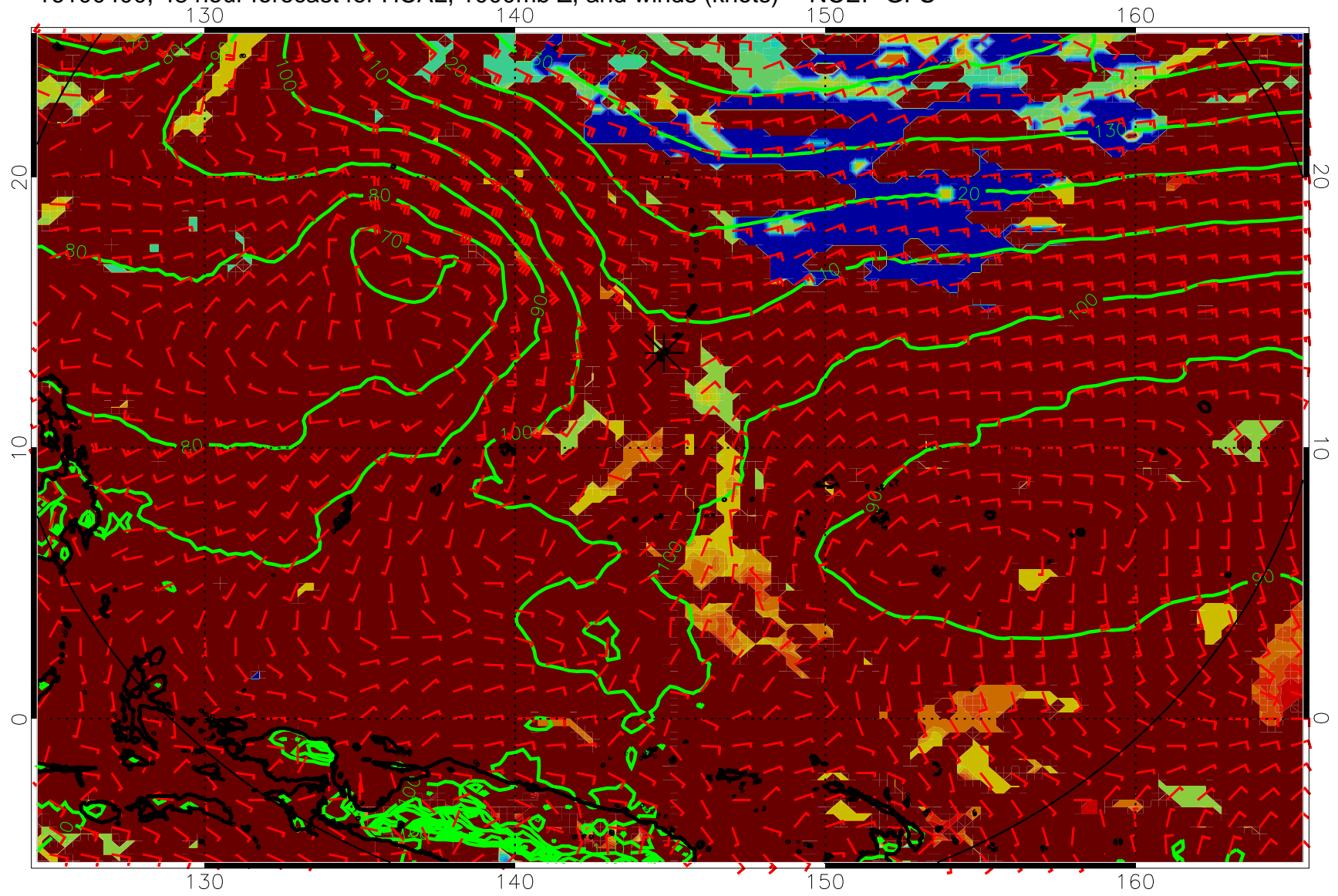
16100400, 48 hour forecast for HCAL, 1000mb Z, and winds (knots) -- NCEP GFS
