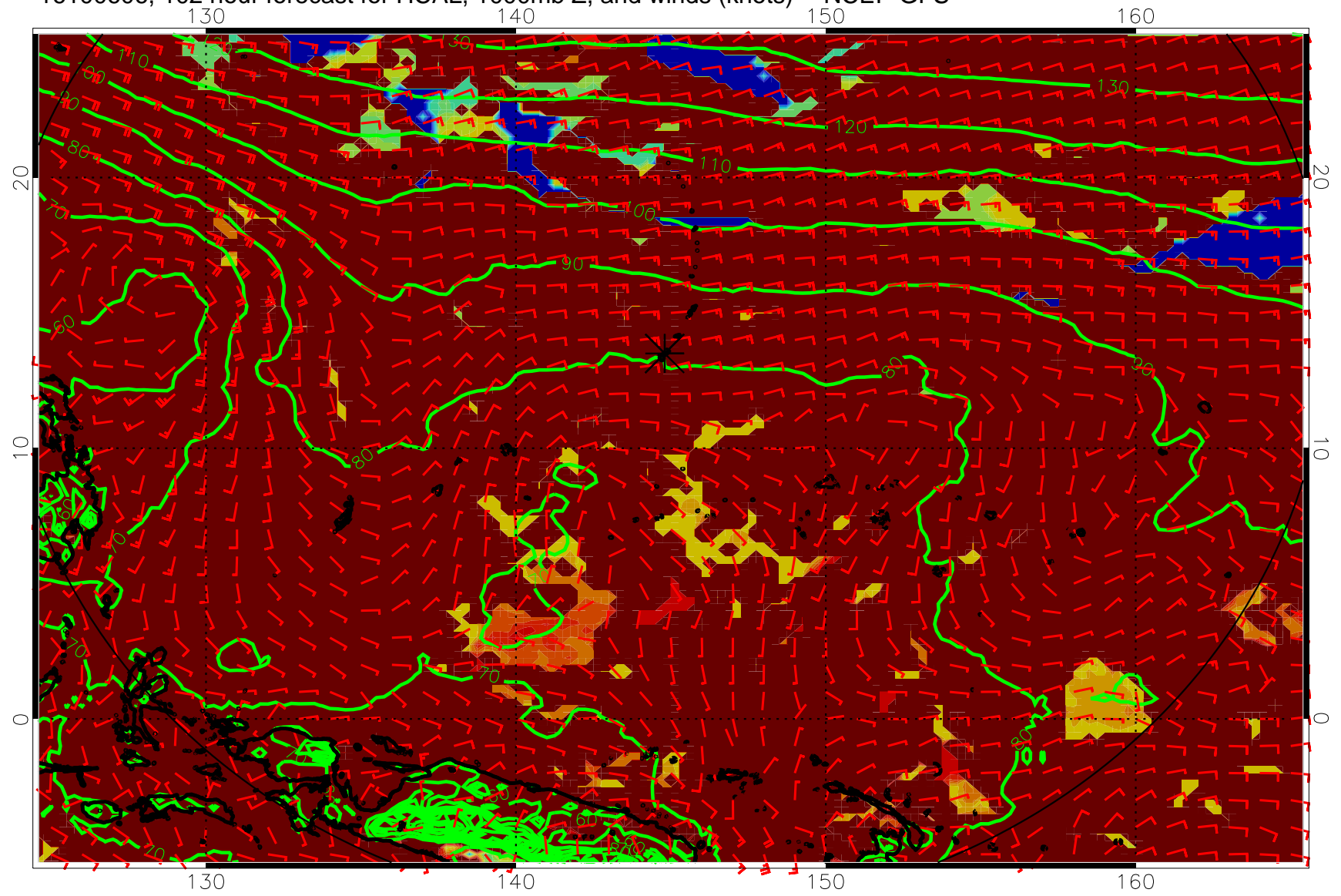
16100606, 102 hour forecast for HCAL, 1000mb Z, and winds (knots) -- NCEP GFS
