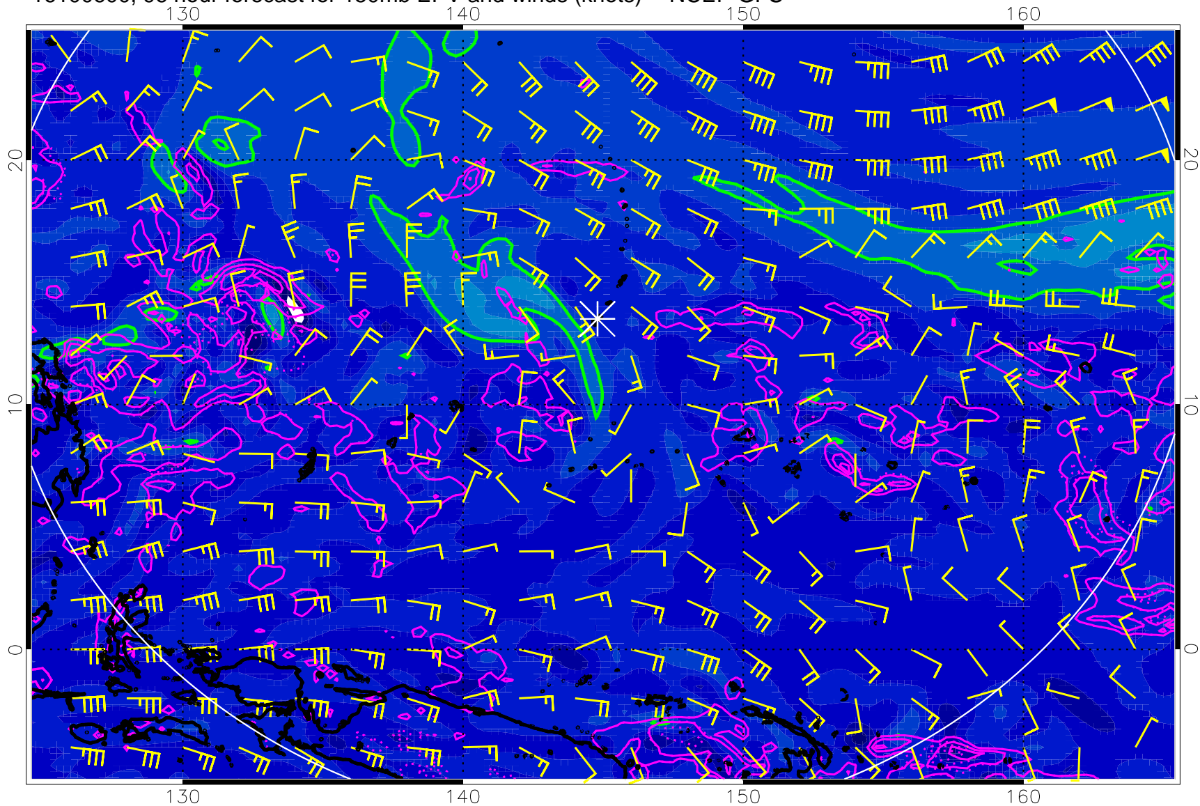
16100600, 96 hour forecast for 150mb EPV and winds (knots) -- NCEP GFS
