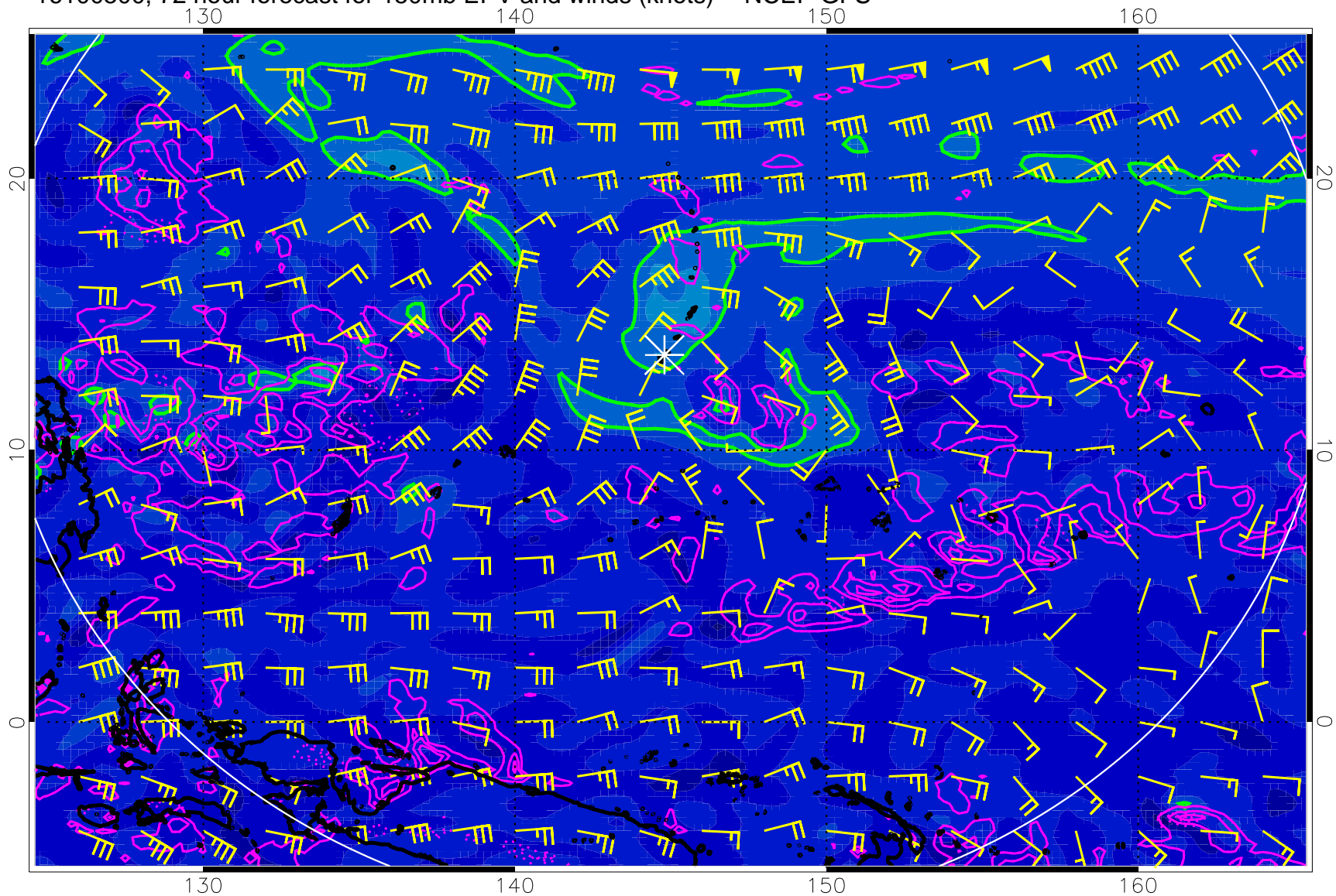
16100500, 72 hour forecast for 150mb EPV and winds (knots) -- NCEP GFS
