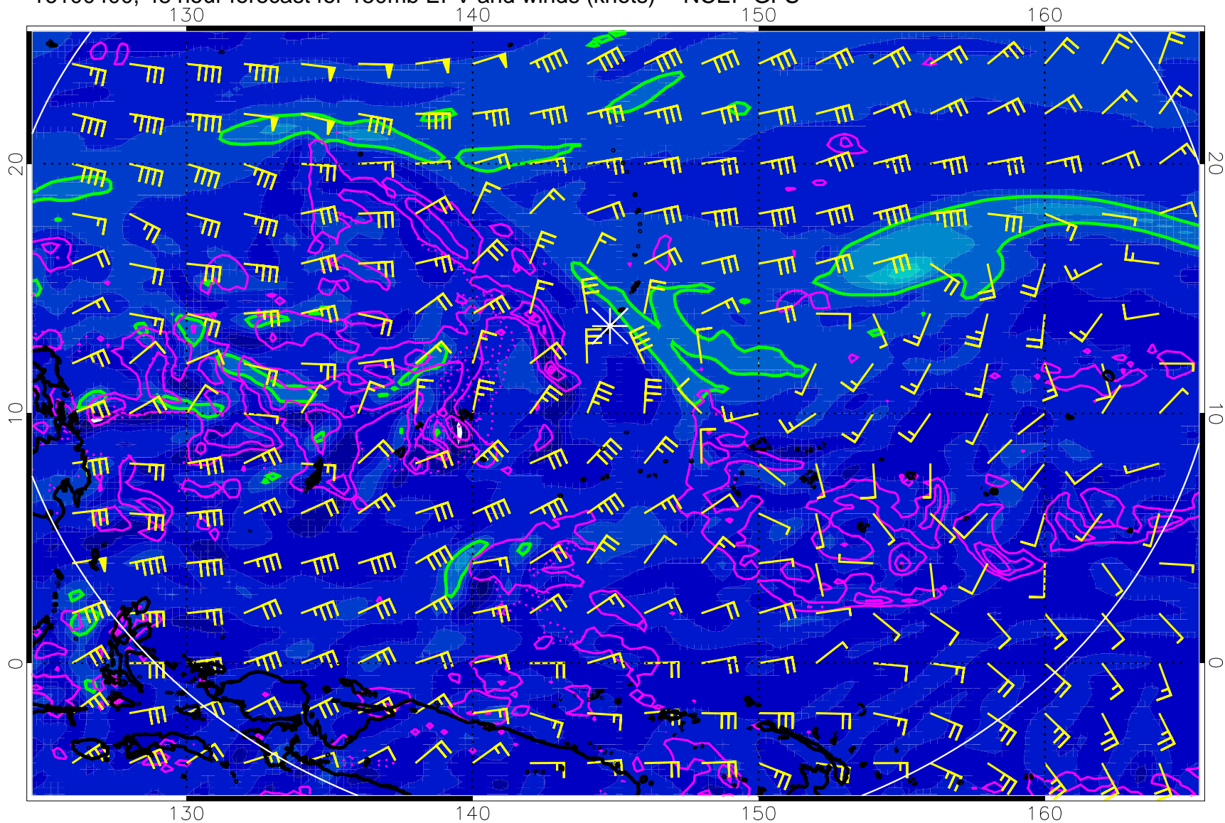
16100400, 48 hour forecast for 150mb EPV and winds (knots) -- NCEP GFS
