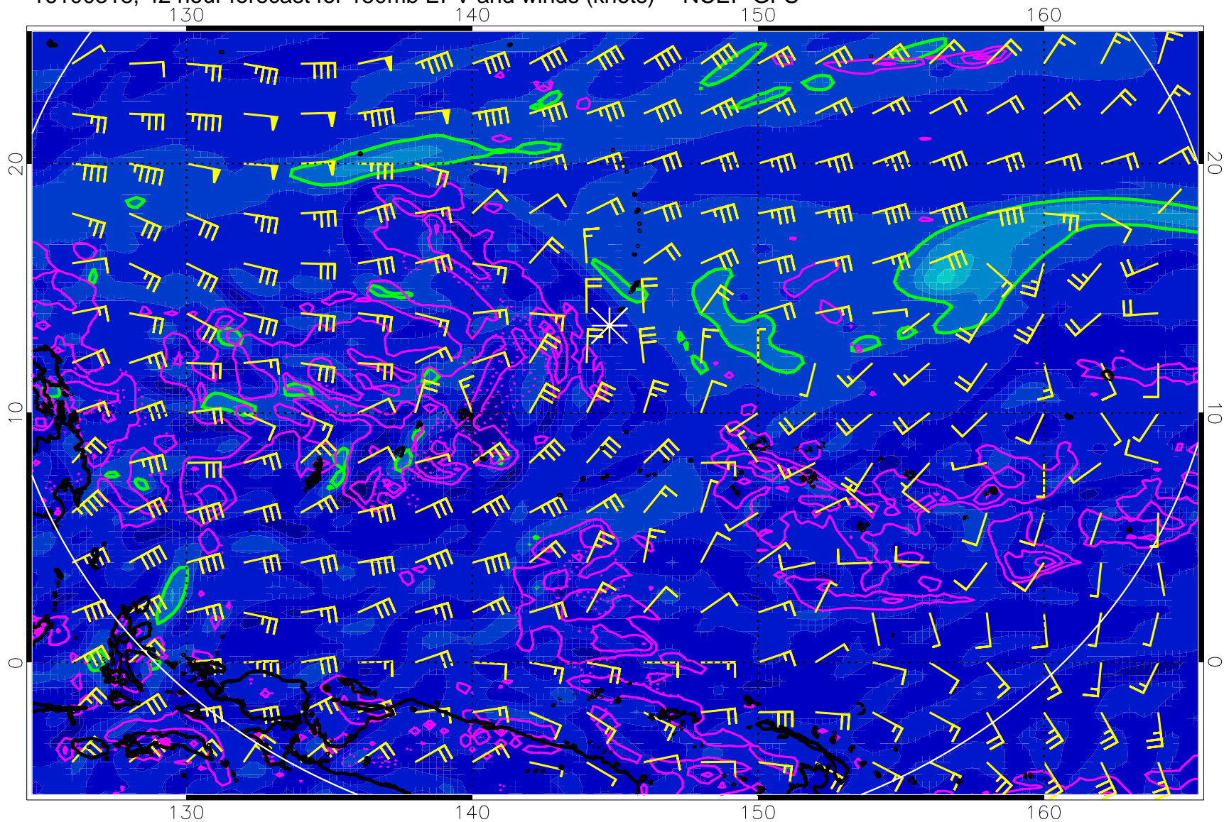
16100318, 42 hour forecast for 150mb EPV and winds (knots) -- NCEP GFS
