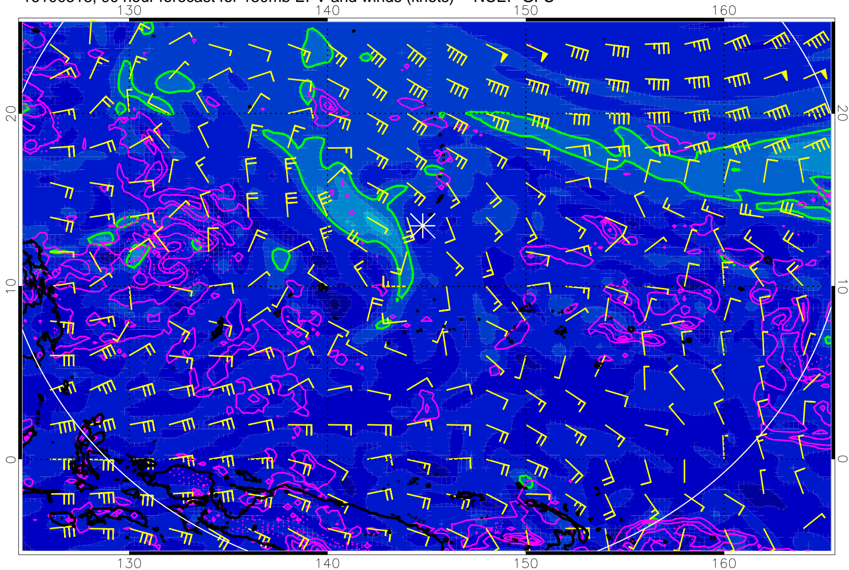
16100518, 90 hour forecast for 150mb EPV and winds (knots) -- NCEP GFS
