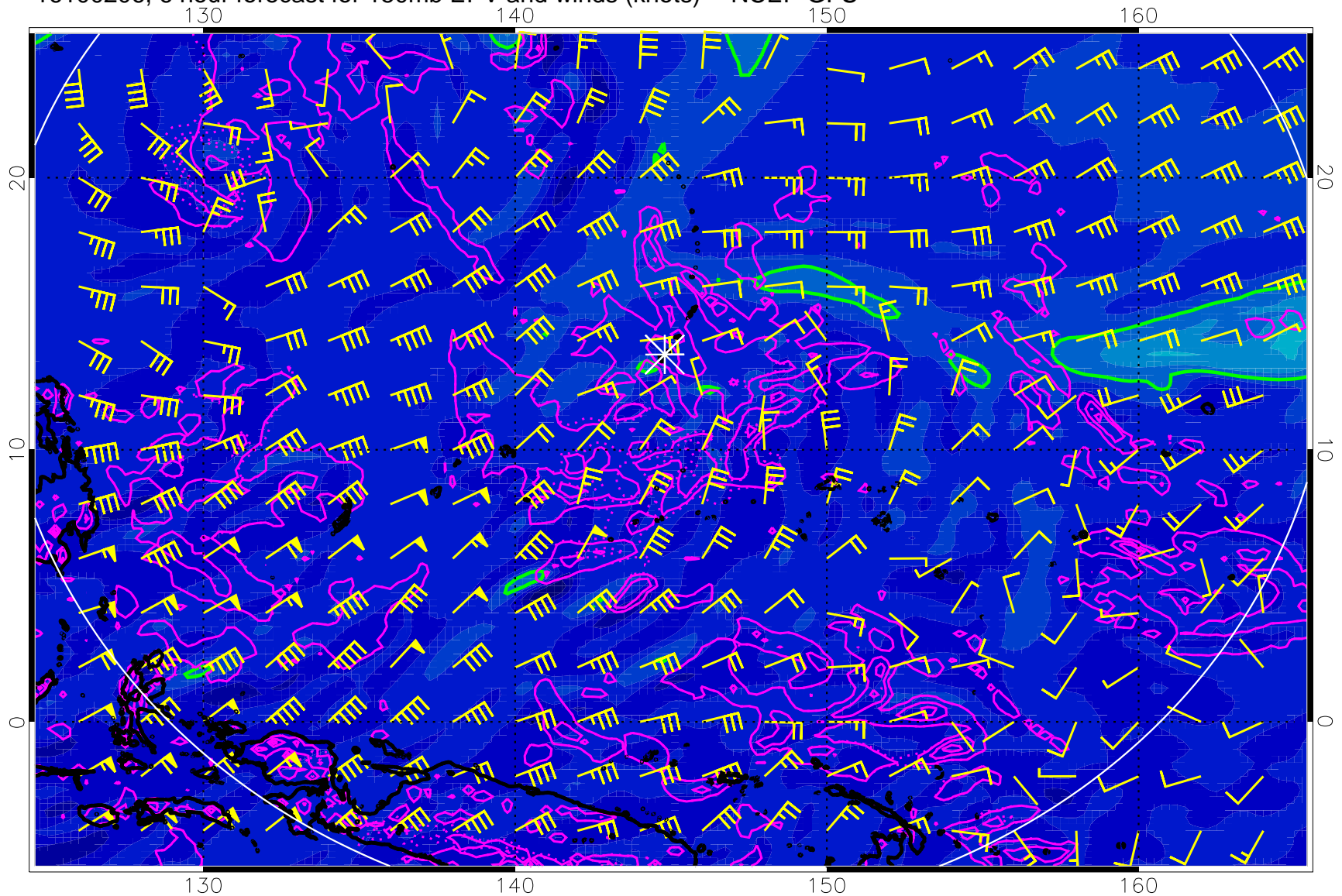
16100206, 6 hour forecast for 150mb EPV and winds (knots) -- NCEP GFS
