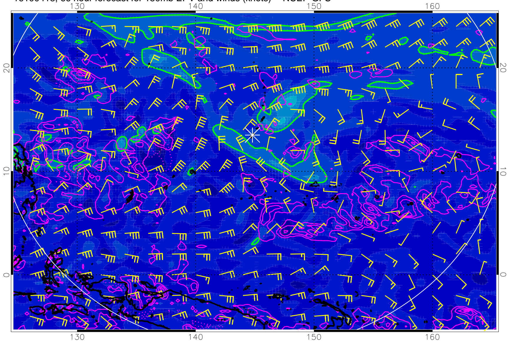
16100418, 66 hour forecast for 150mb EPV and winds (knots) -- NCEP GFS
