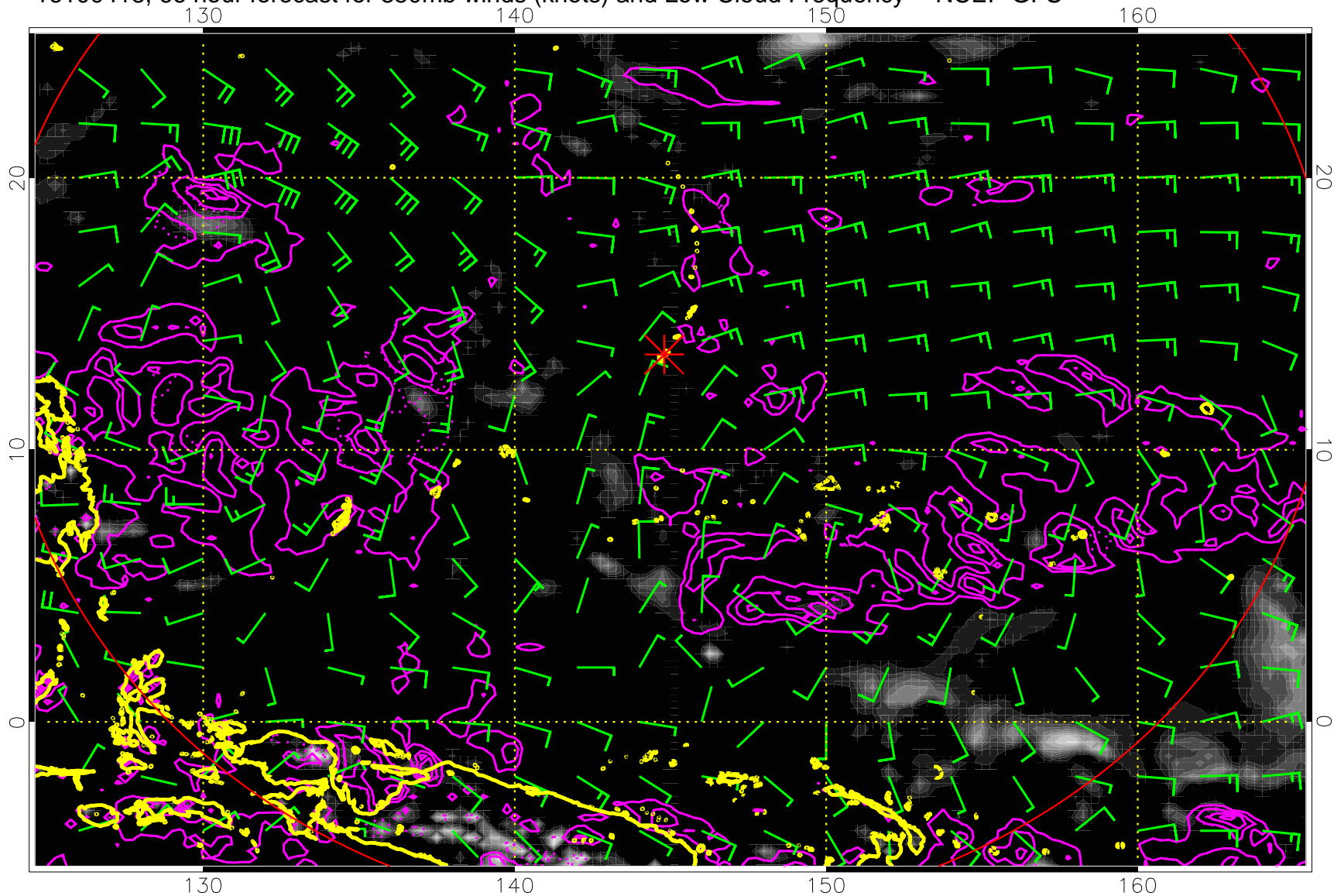
16100418, 66 hour forecast for 850mb winds (knots) and Low Cloud Frequency -- NCEP GFS
