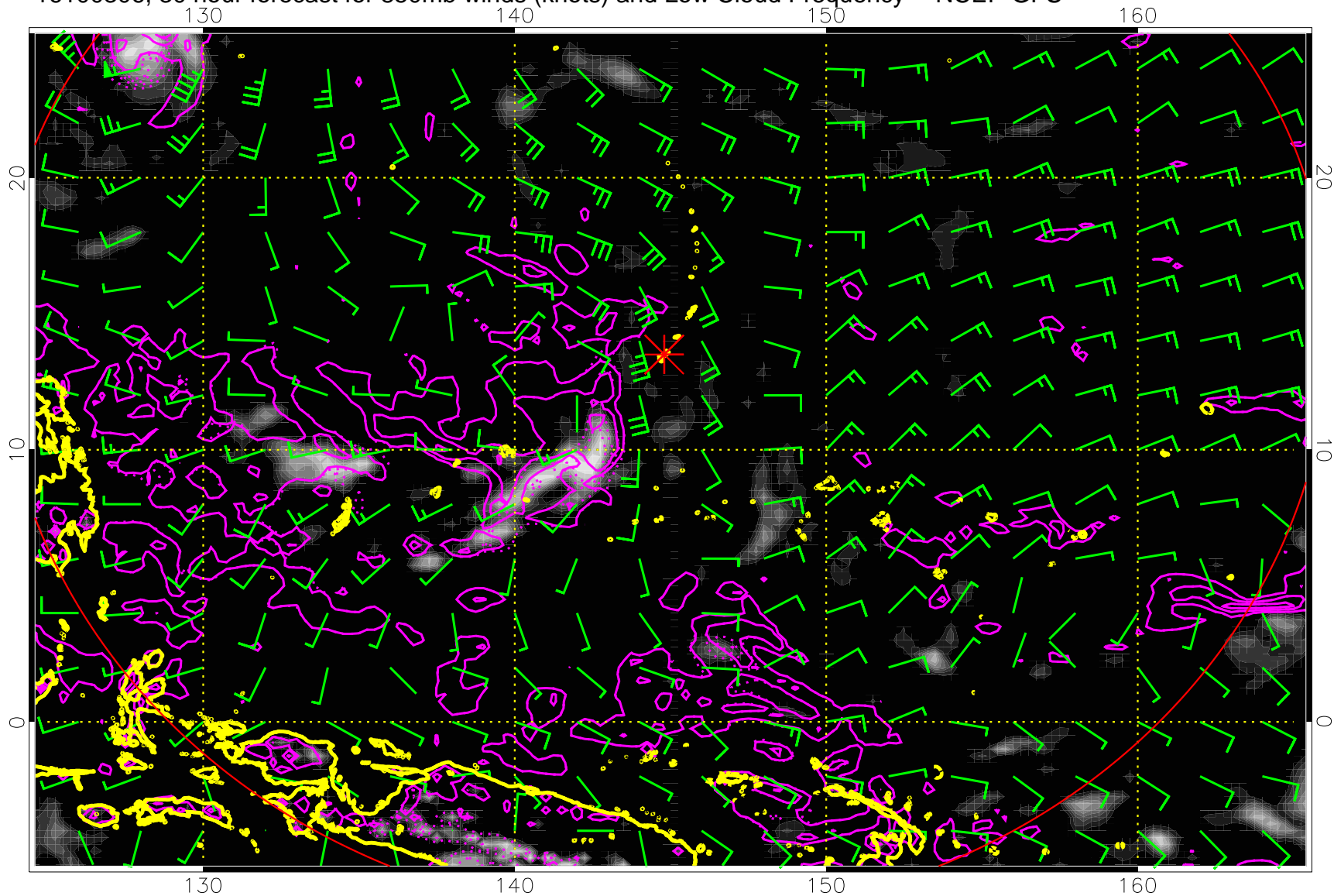
16100306, 30 hour forecast for 850mb winds (knots) and Low Cloud Frequency -- NCEP GFS
