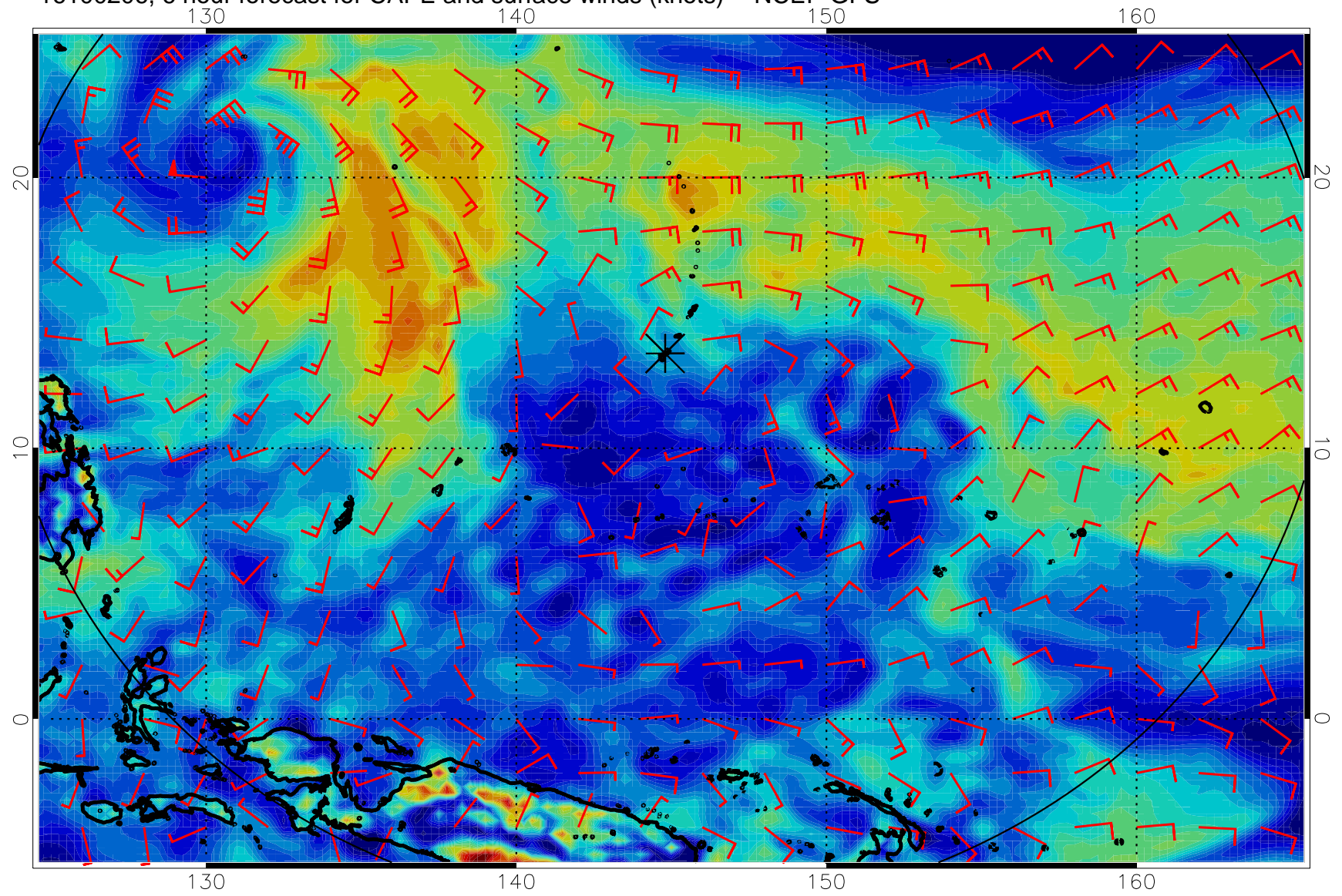
16100206, 6 hour forecast for CAPE and surface winds (knots) -- NCEP GFS
