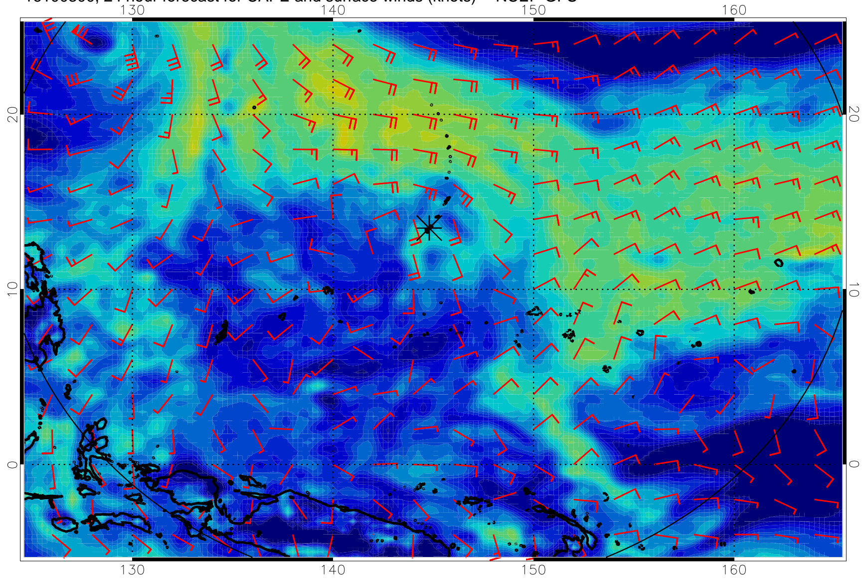
16100300, 24 hour forecast for CAPE and surface winds (knots) -- NCEP GFS
