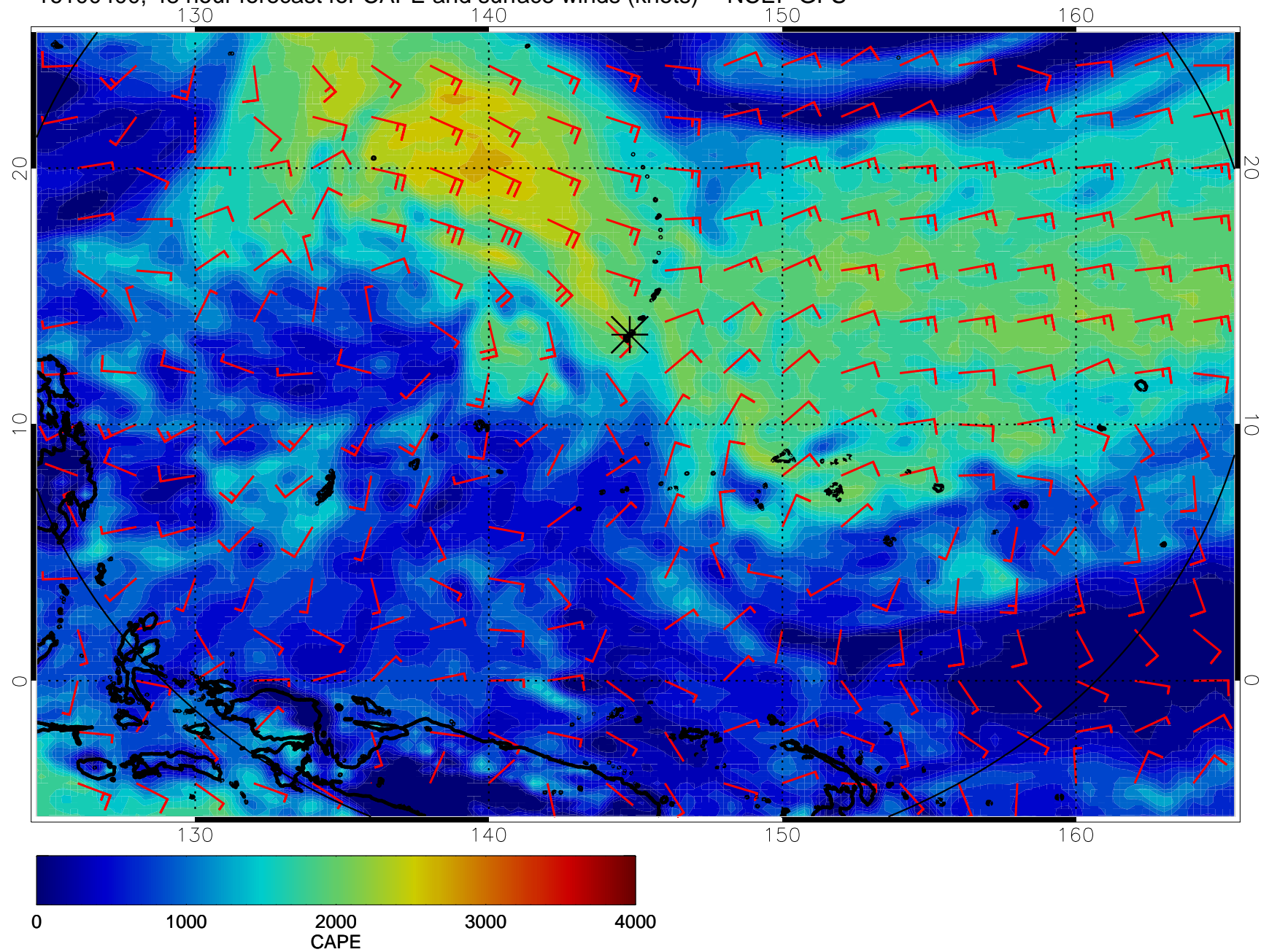
16100400, 48 hour forecast for CAPE and surface winds (knots) -- NCEP GFS
