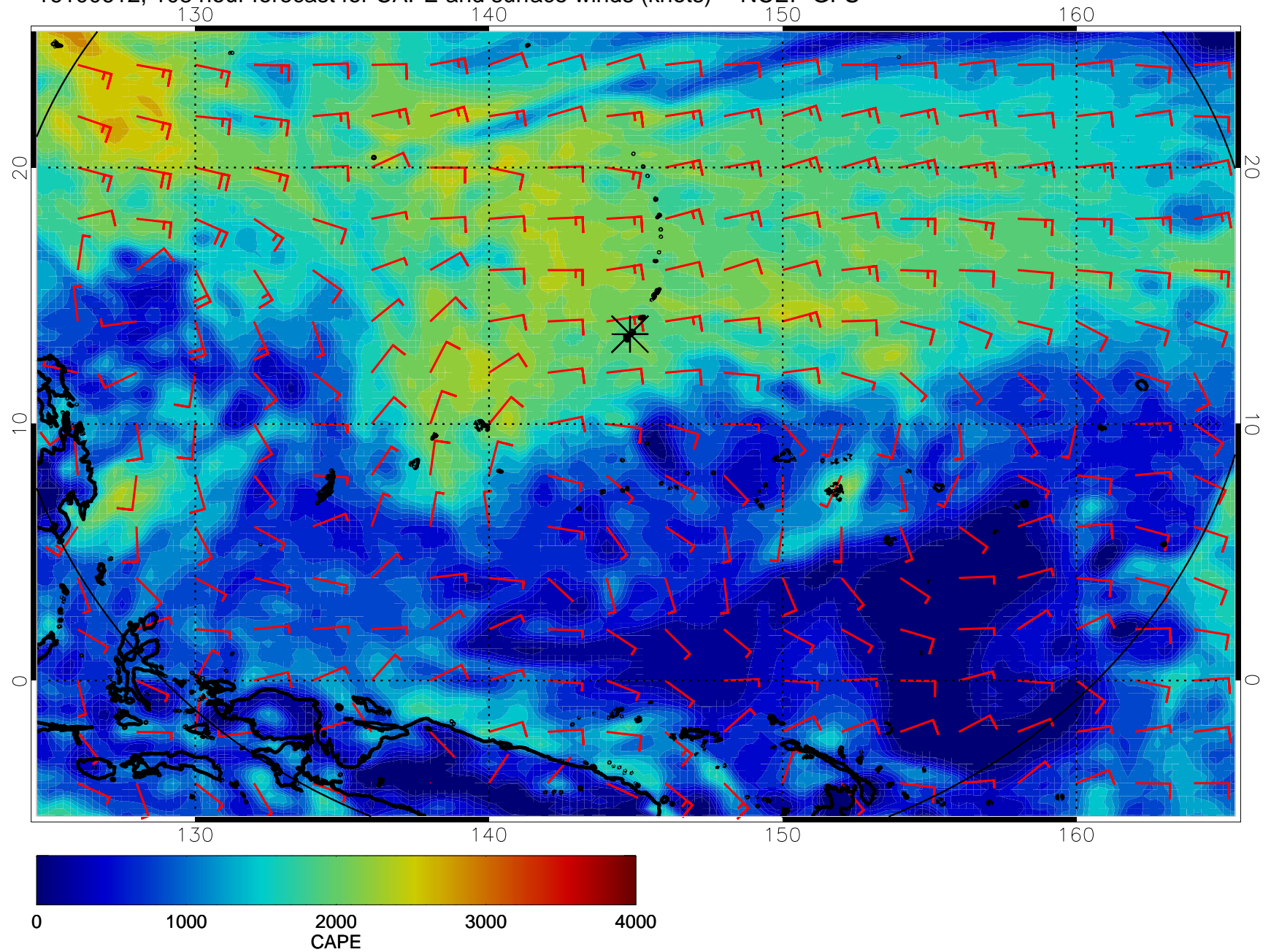
16100612, 108 hour forecast for CAPE and surface winds (knots) -- NCEP GFS
