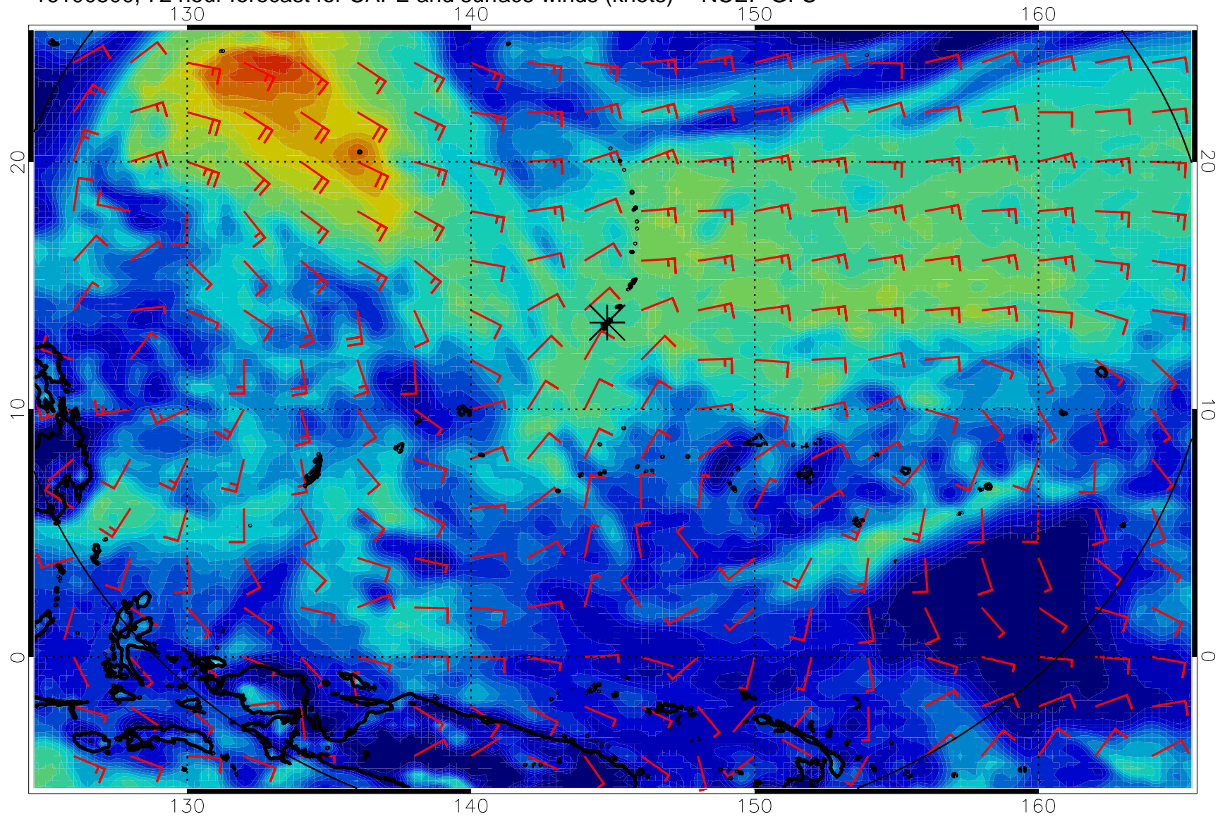
16100500, 72 hour forecast for CAPE and surface winds (knots) -- NCEP GFS
