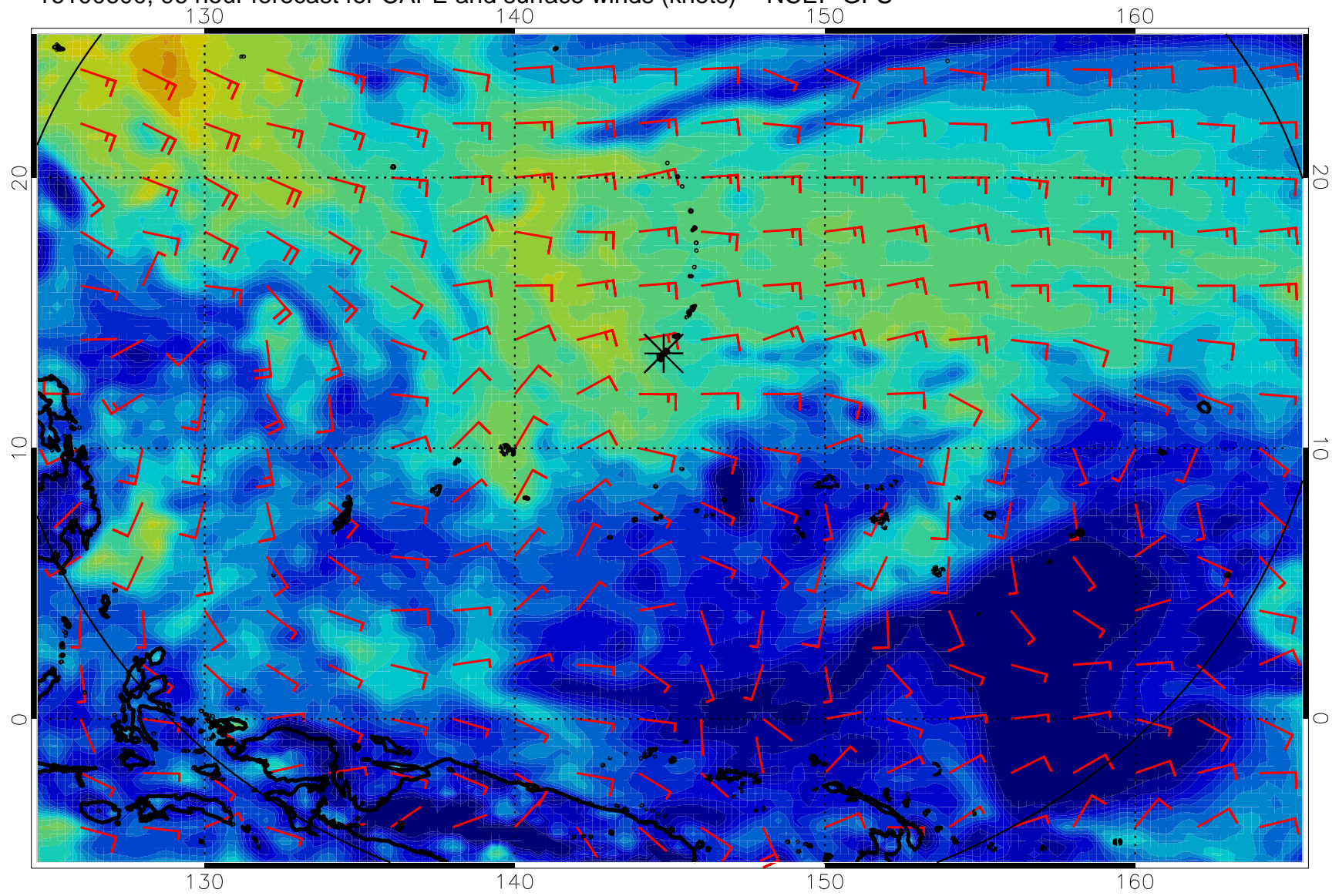
16100600, 96 hour forecast for CAPE and surface winds (knots) -- NCEP GFS
