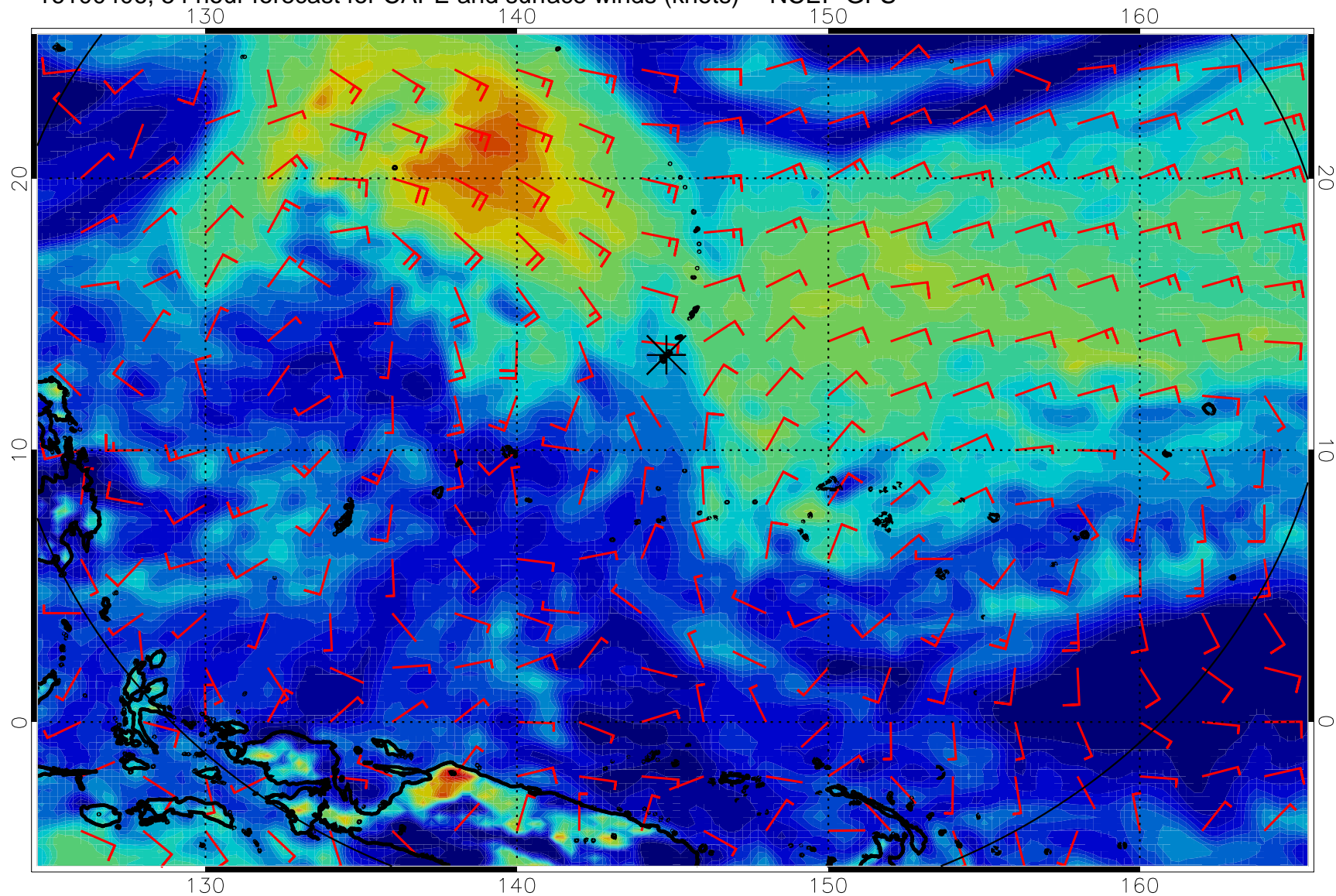
16100406, 54 hour forecast for CAPE and surface winds (knots) -- NCEP GFS
