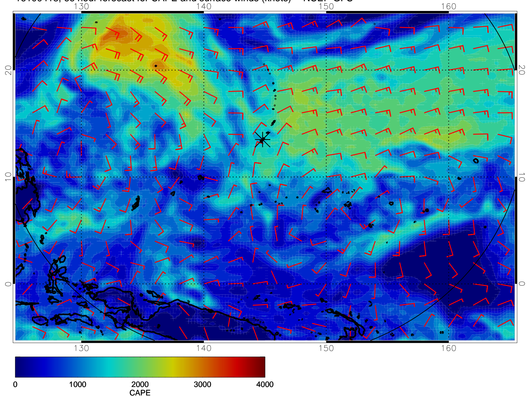
16100418, 66 hour forecast for CAPE and surface winds (knots) -- NCEP GFS
