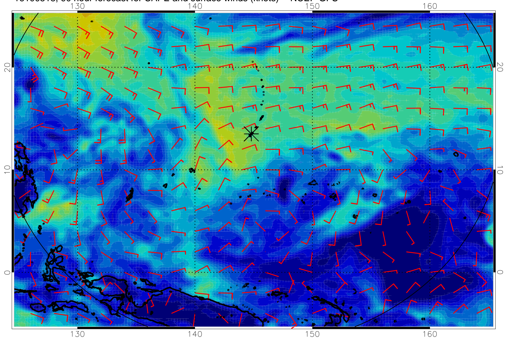
16100518, 90 hour forecast for CAPE and surface winds (knots) -- NCEP GFS
