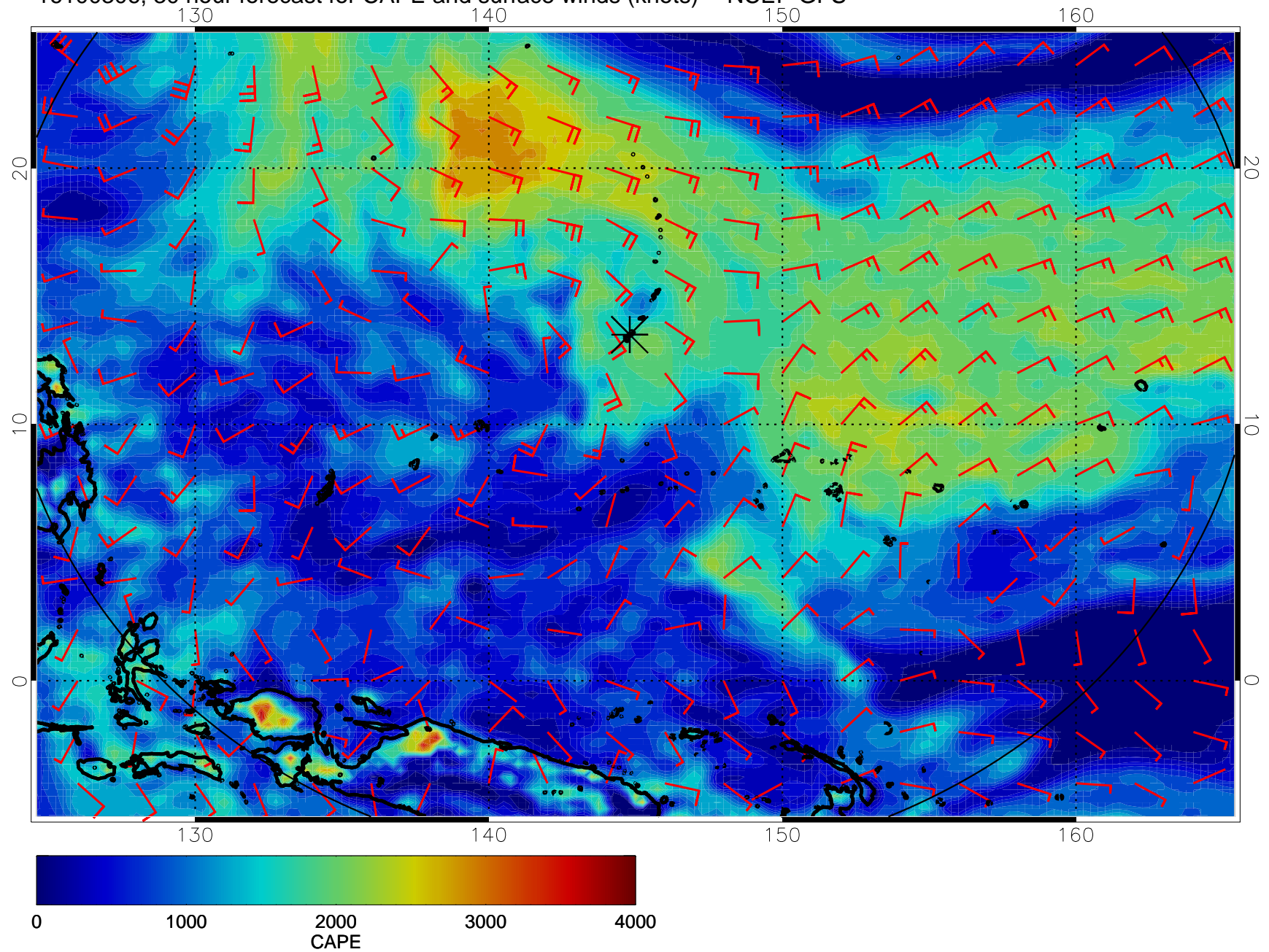
16100306, 30 hour forecast for CAPE and surface winds (knots) -- NCEP GFS
