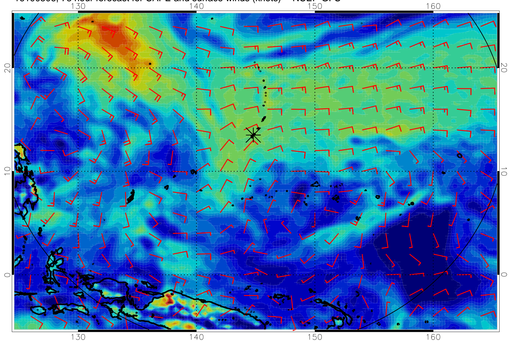
16100506, 78 hour forecast for CAPE and surface winds (knots) -- NCEP GFS
