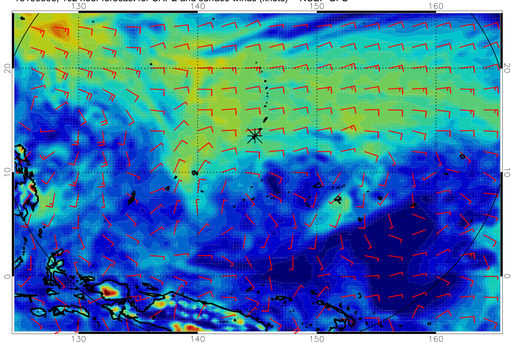
16100606, 102 hour forecast for CAPE and surface winds (knots) -- NCEP GFS
