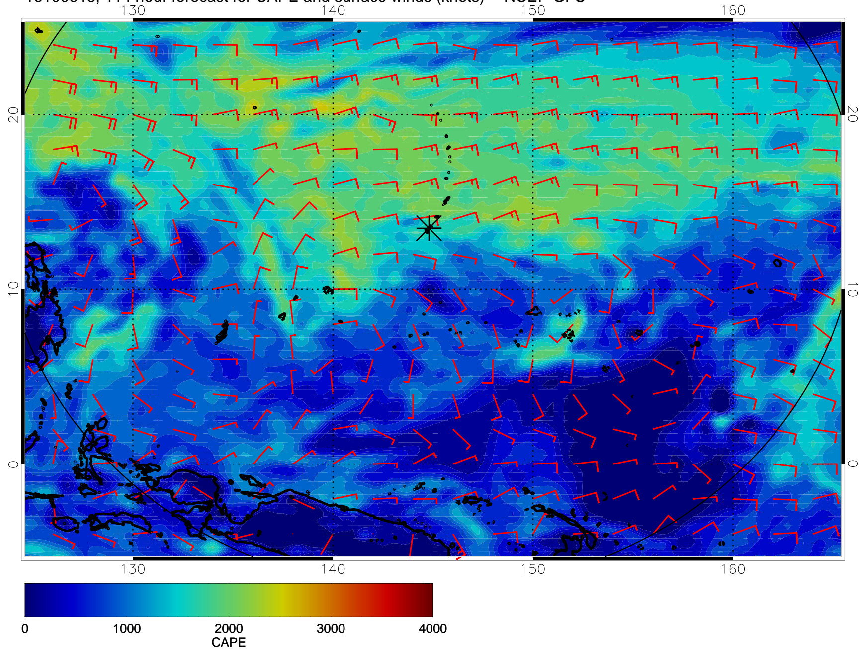
16100618, 114 hour forecast for CAPE and surface winds (knots) -- NCEP GFS
