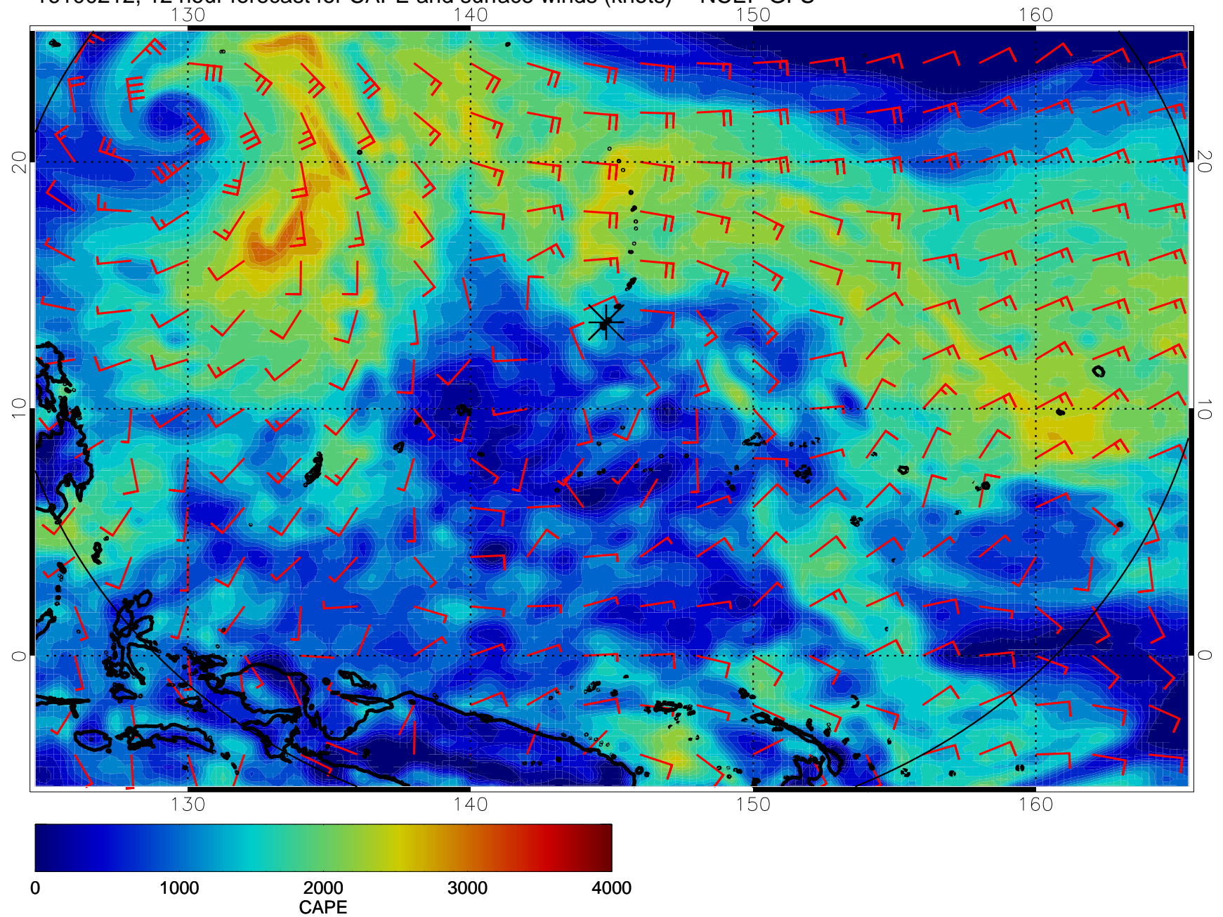
16100212, 12 hour forecast for CAPE and surface winds (knots) -- NCEP GFS
