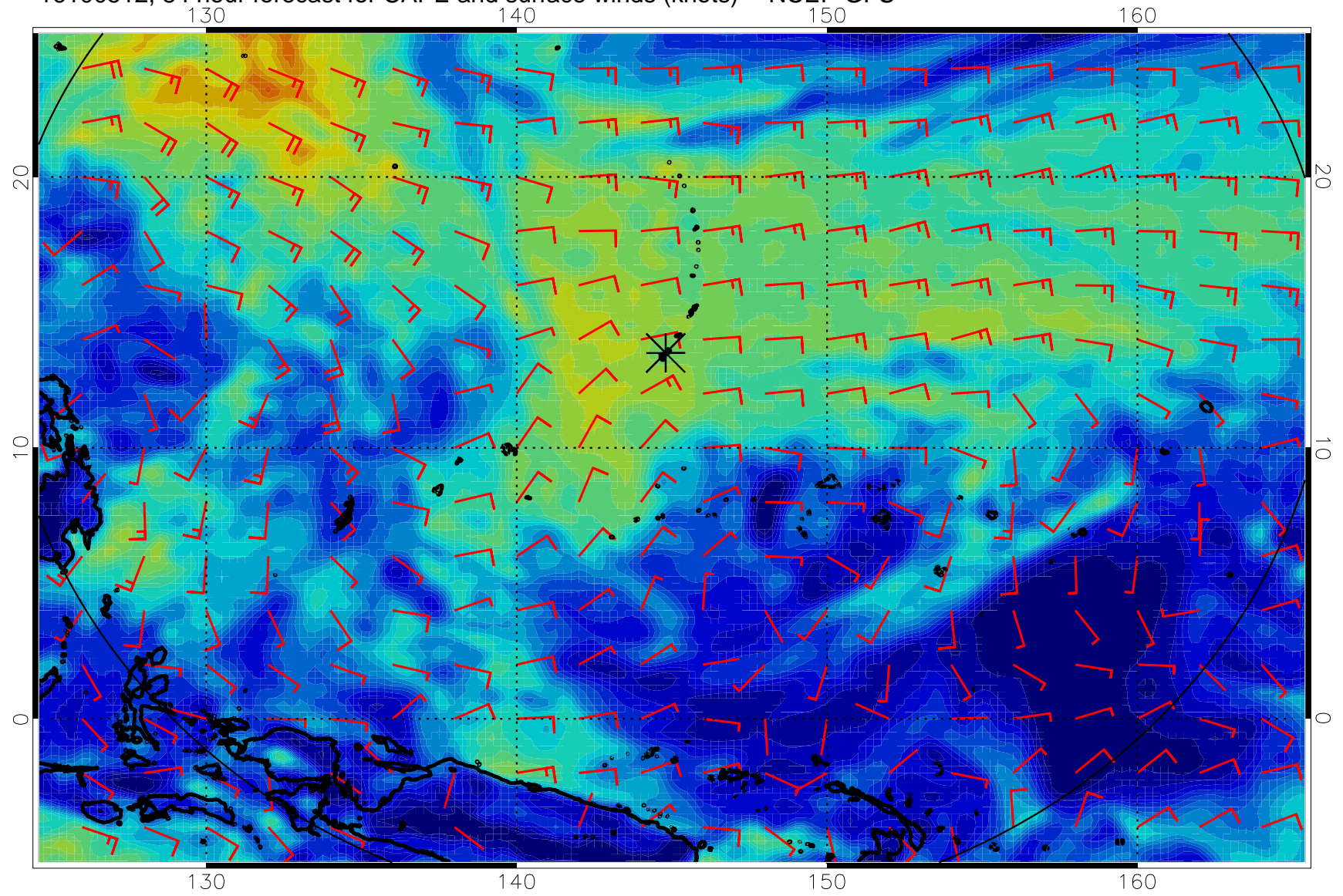
16100512, 84 hour forecast for CAPE and surface winds (knots) -- NCEP GFS
