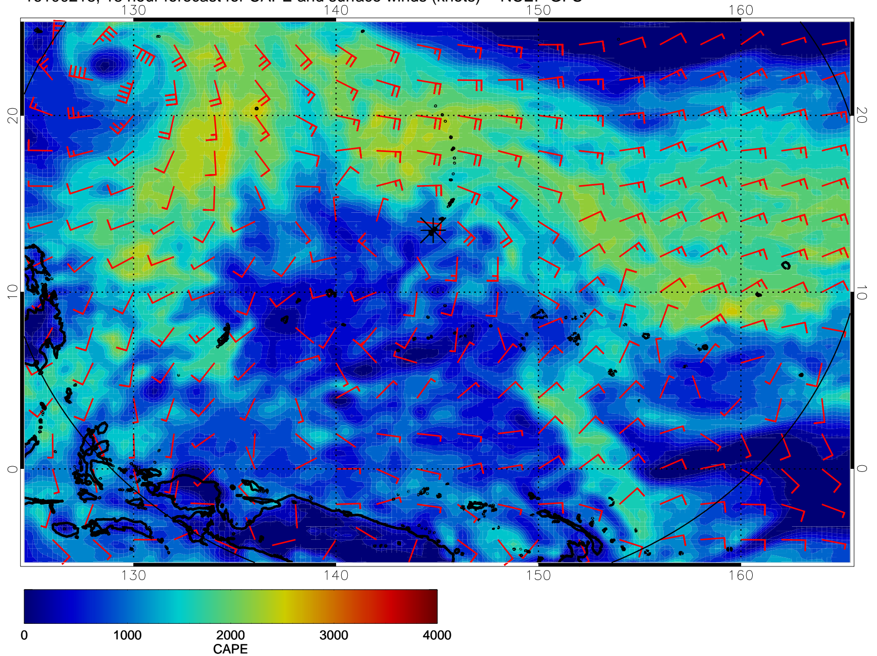
16100218, 18 hour forecast for CAPE and surface winds (knots) -- NCEP GFS
