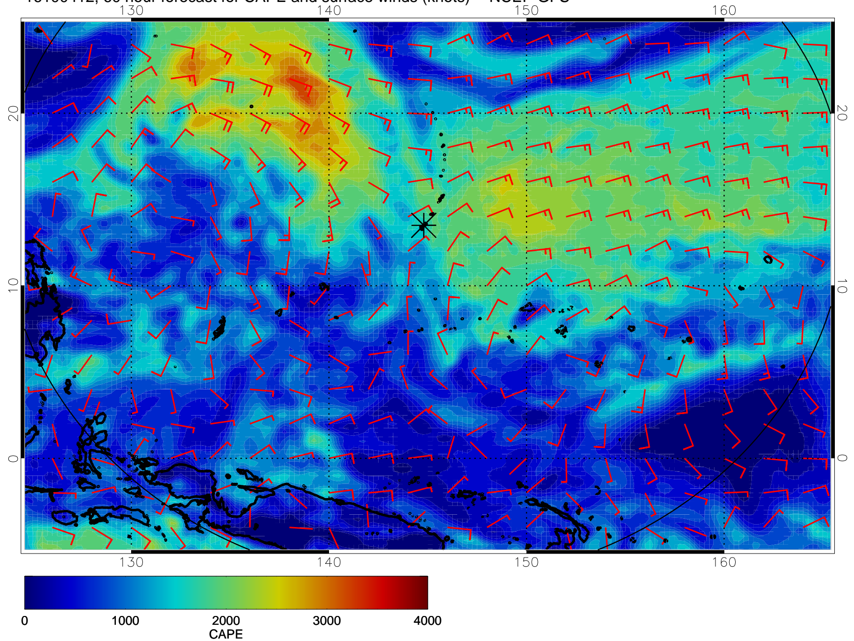
16100412, 60 hour forecast for CAPE and surface winds (knots) -- NCEP GFS
