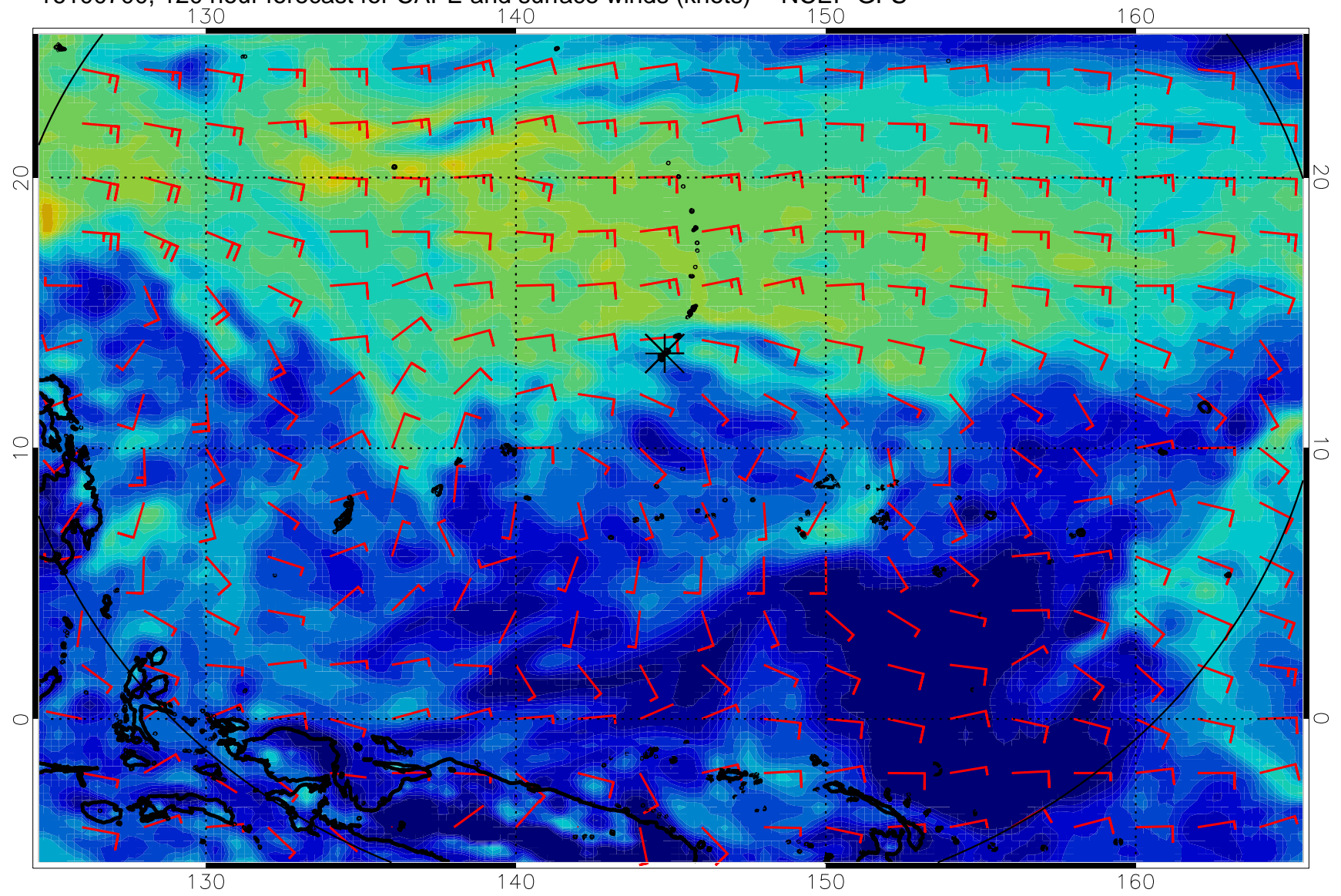
16100700, 120 hour forecast for CAPE and surface winds (knots) -- NCEP GFS
