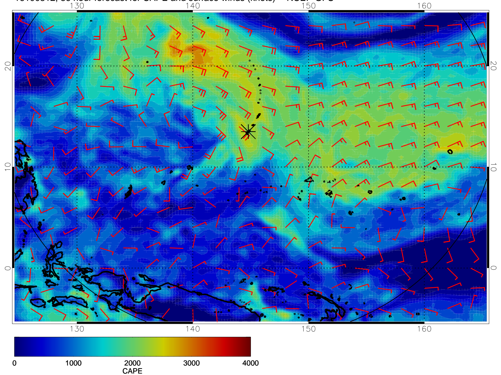
16100312, 36 hour forecast for CAPE and surface winds (knots) -- NCEP GFS
