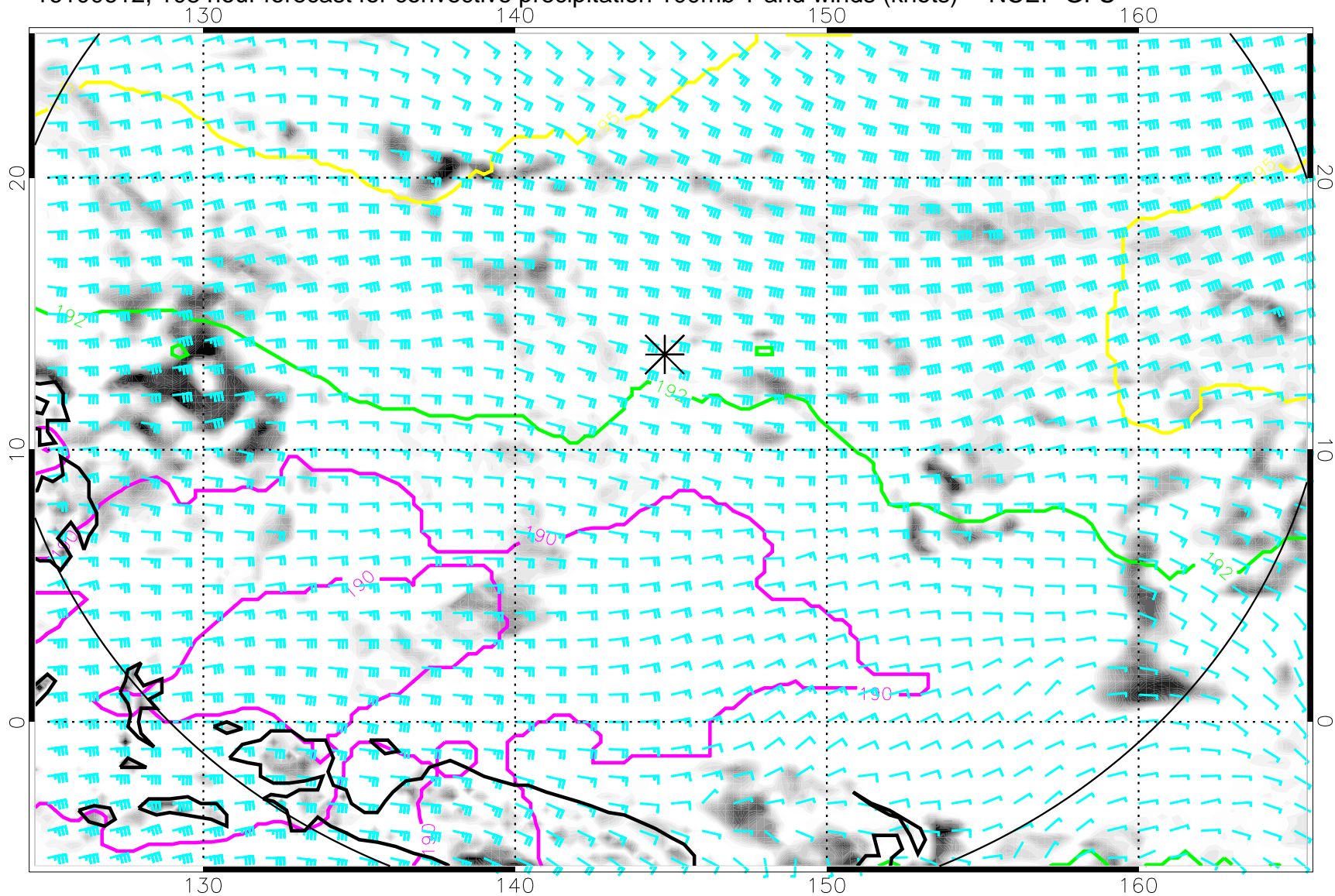
16100612, 108 hour forecast for convective precipitation 100mb T and winds (knots) -- NCEP GFS
