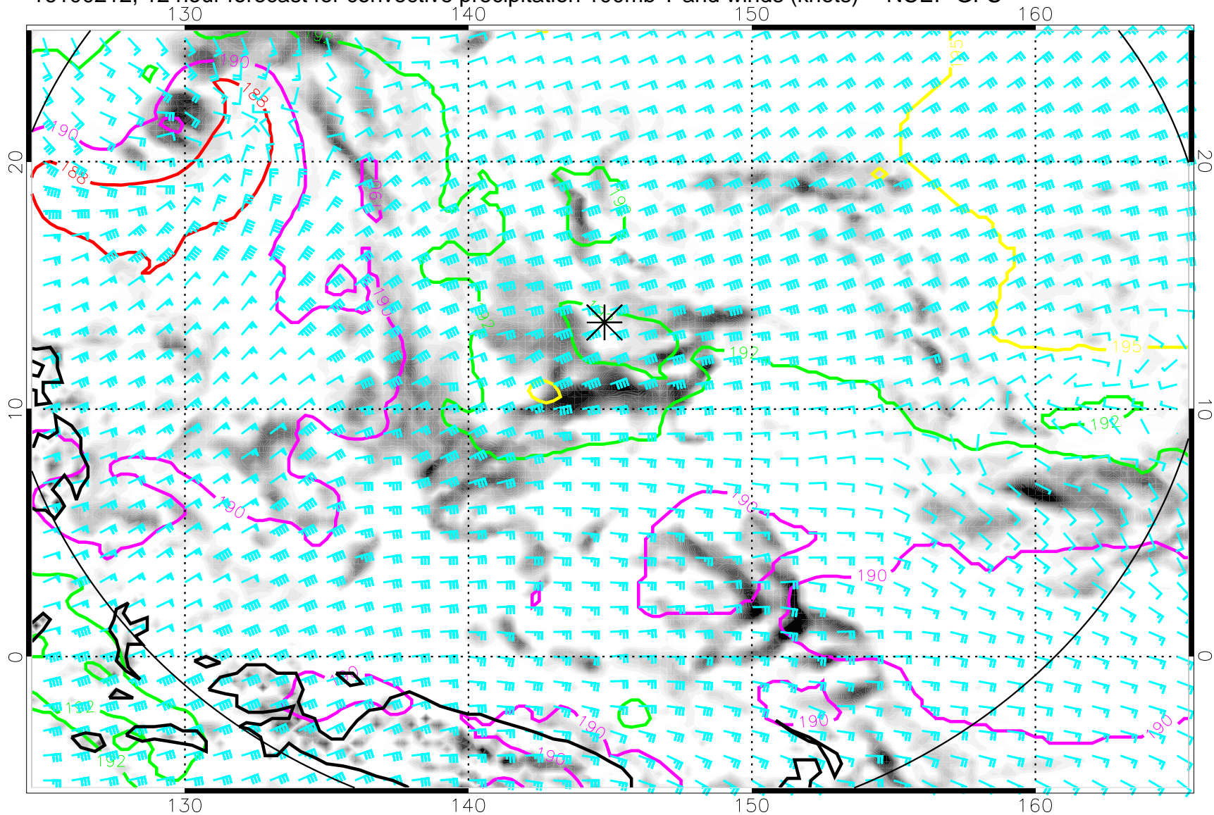
16100212, 12 hour forecast for convective precipitation 100mb T and winds (knots) -- NCEP GFS
