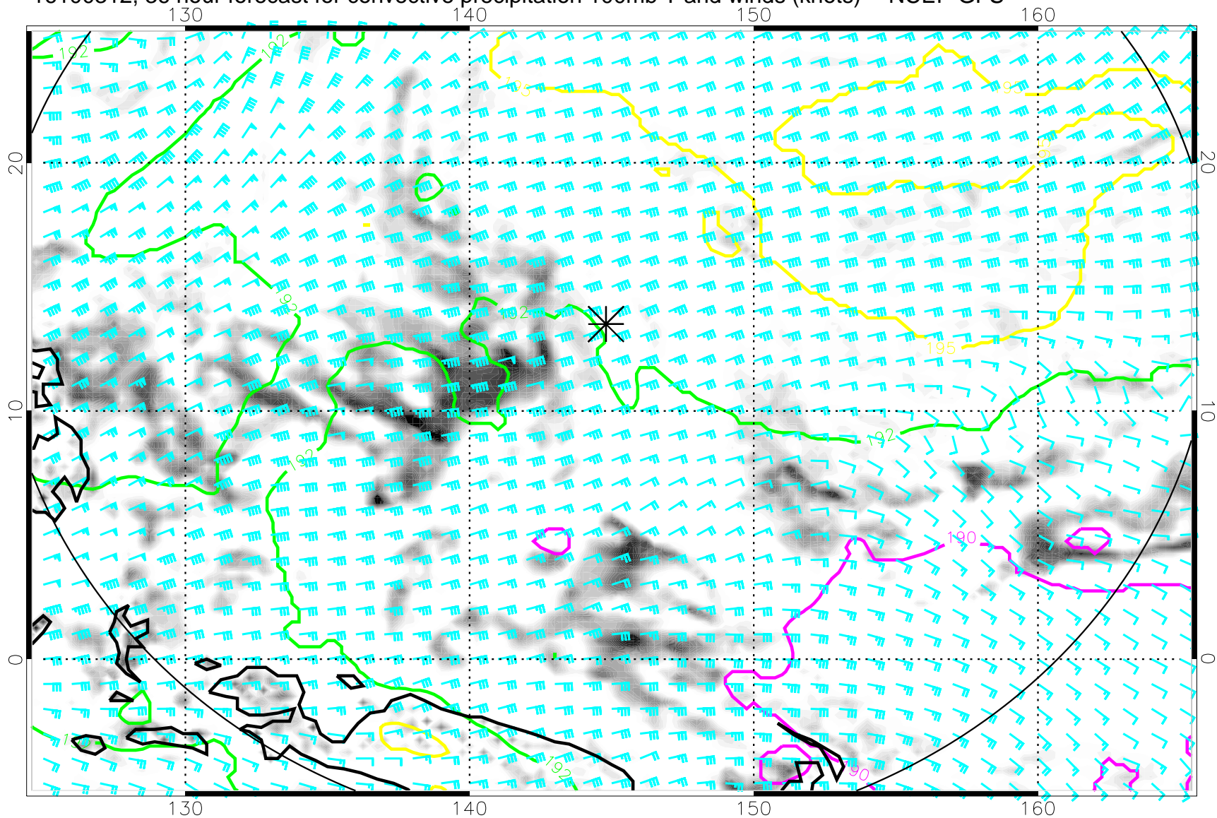
16100312, 36 hour forecast for convective precipitation 100mb T and winds (knots) -- NCEP GFS
