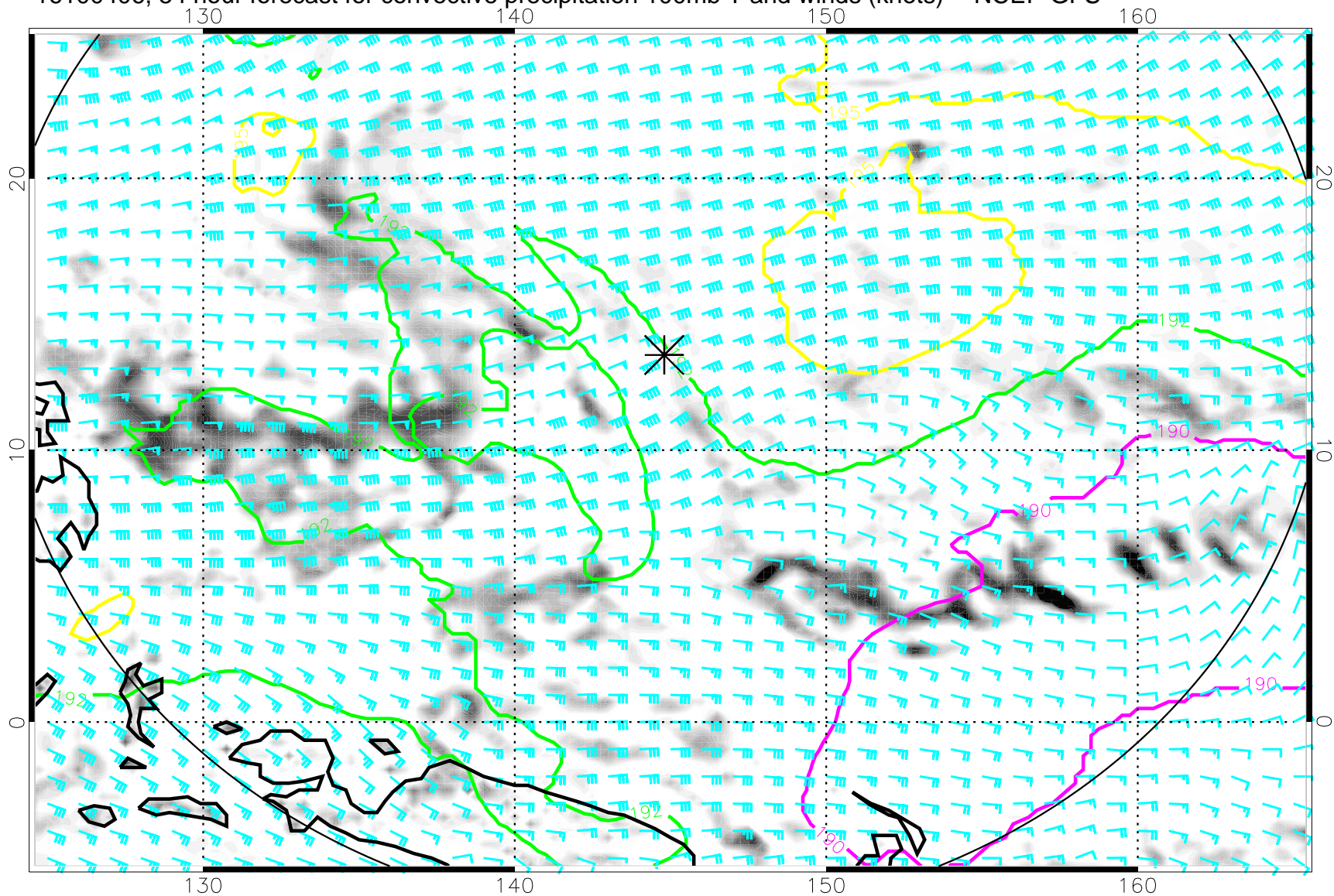
16100406, 54 hour forecast for convective precipitation 100mb T and winds (knots) -- NCEP GFS
