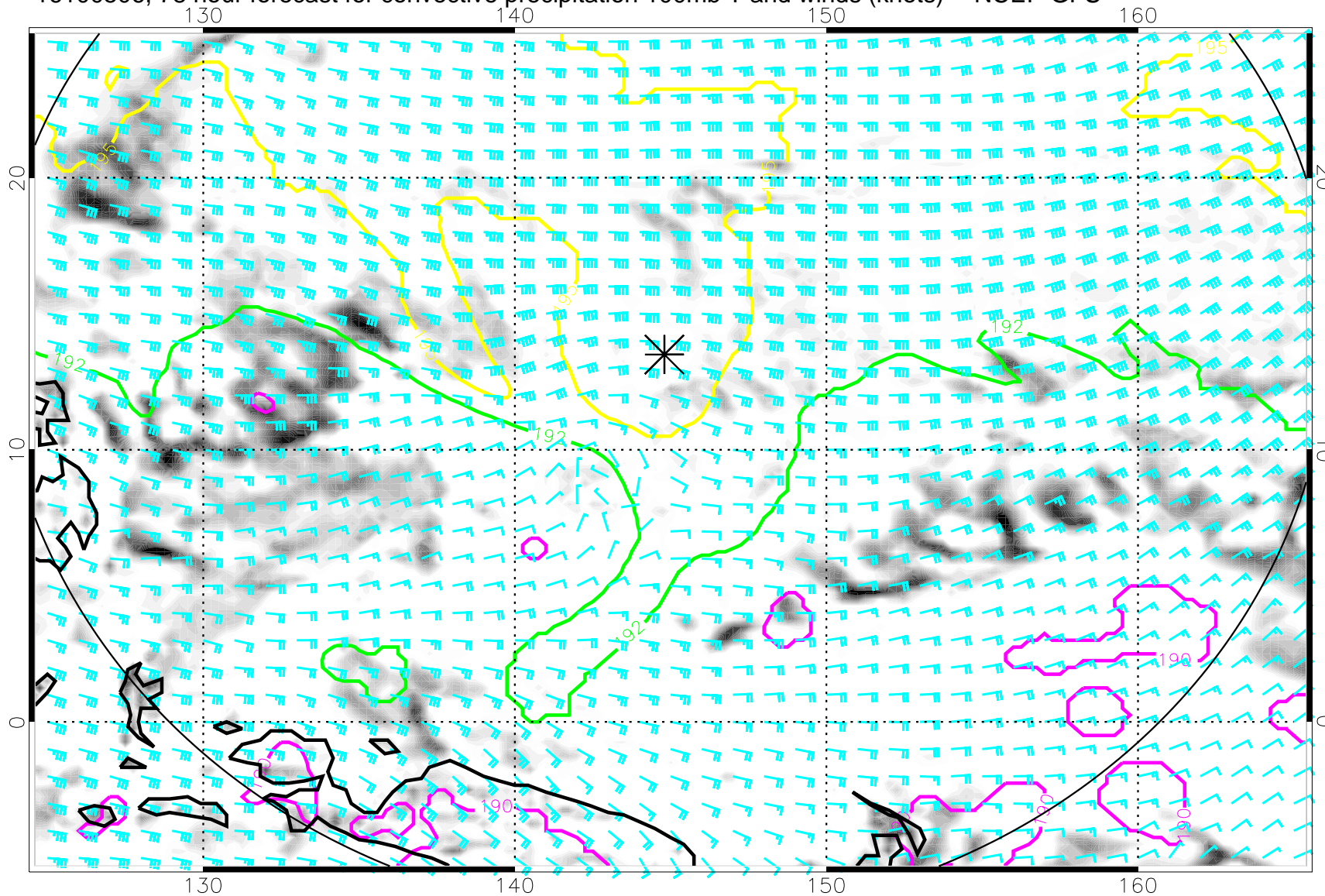
16100506, 78 hour forecast for convective precipitation 100mb T and winds (knots) -- NCEP GFS
