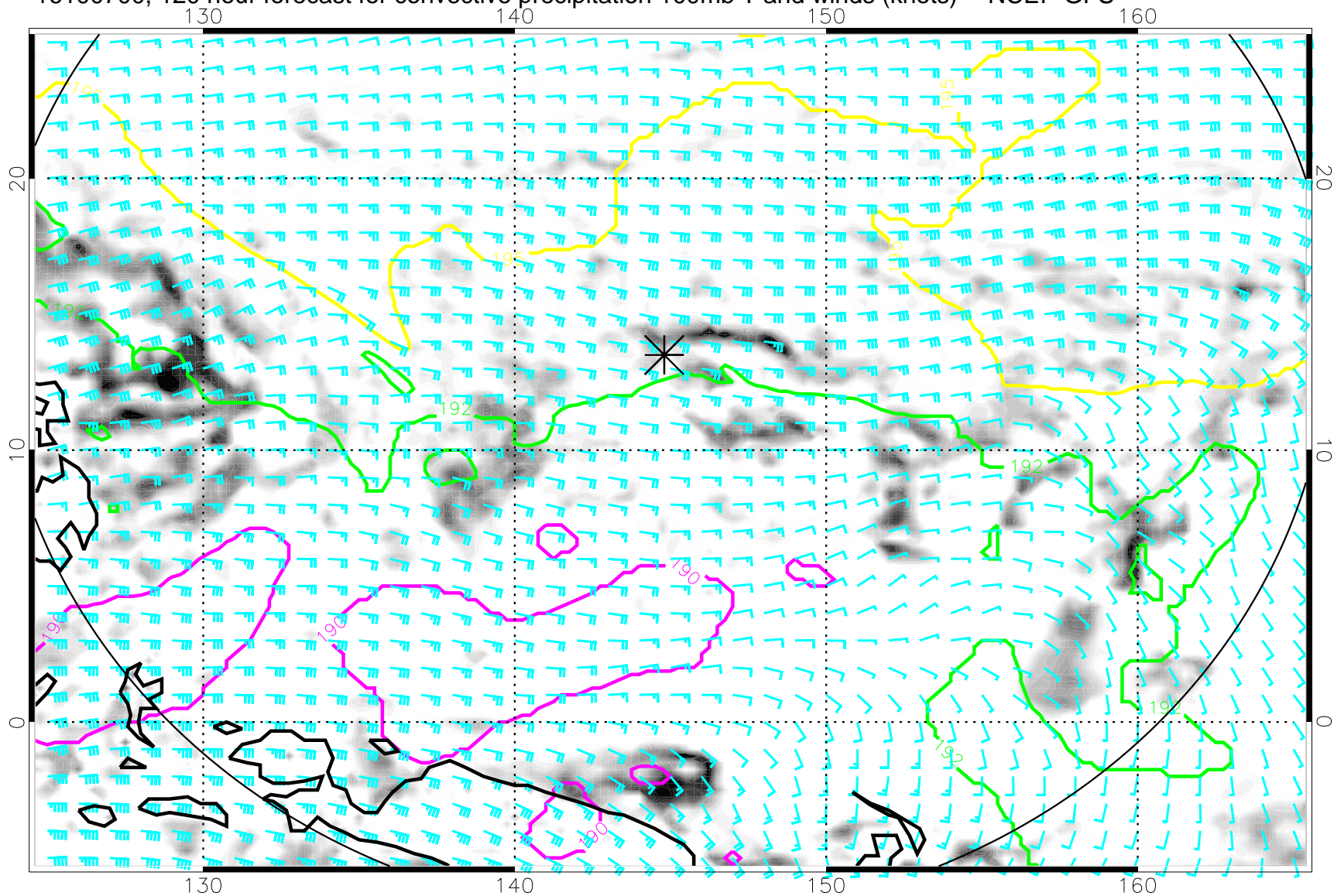
16100700, 120 hour forecast for convective precipitation 100mb T and winds (knots) -- NCEP GFS
