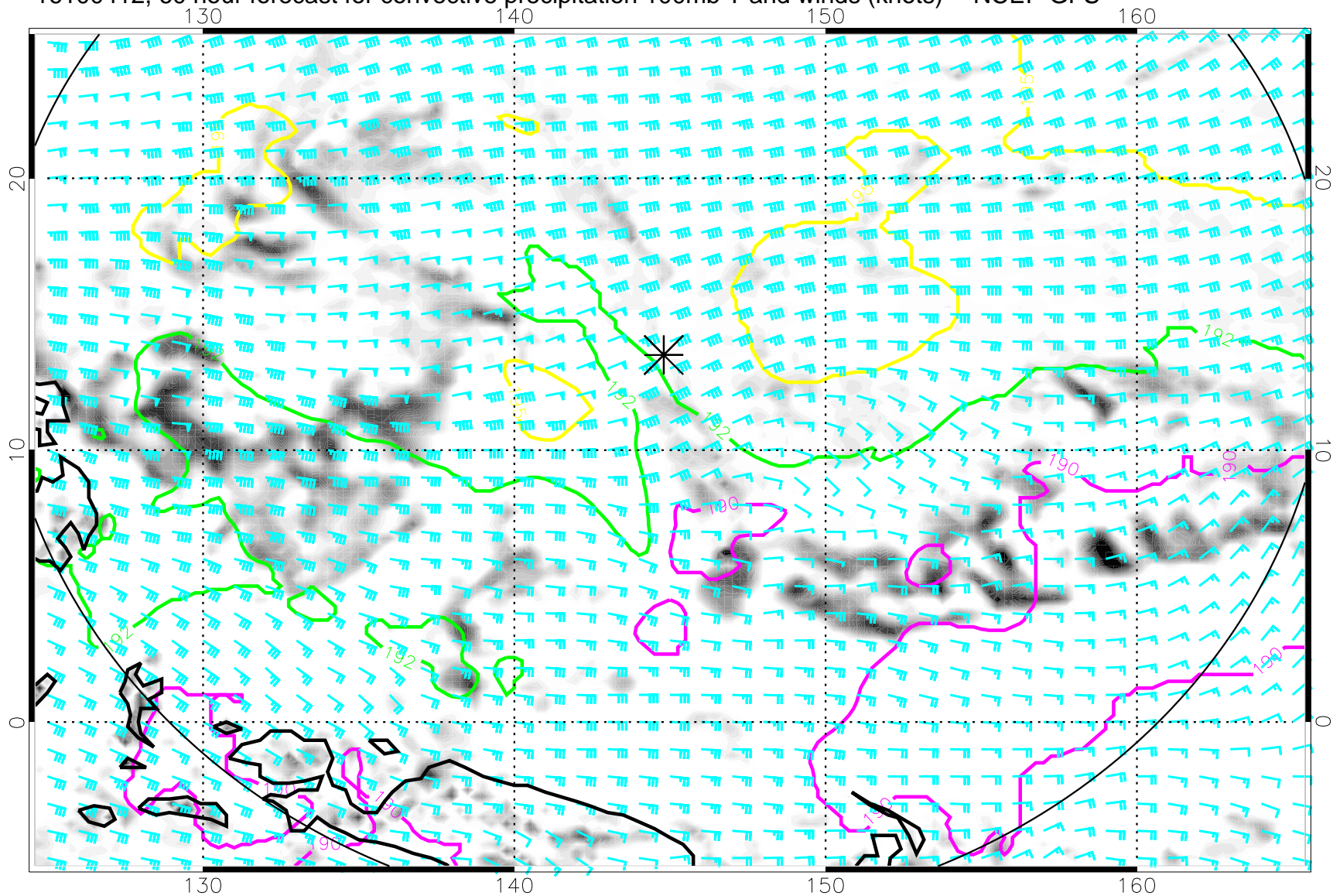
16100412, 60 hour forecast for convective precipitation 100mb T and winds (knots) -- NCEP GFS
