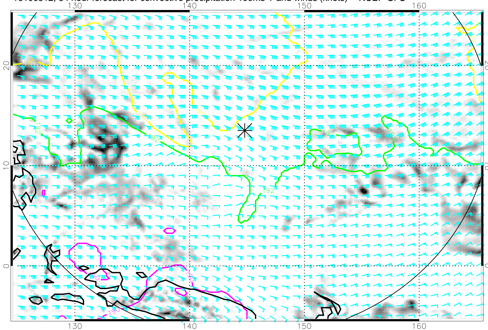
16100512, 84 hour forecast for convective precipitation 100mb T and winds (knots) -- NCEP GFS
