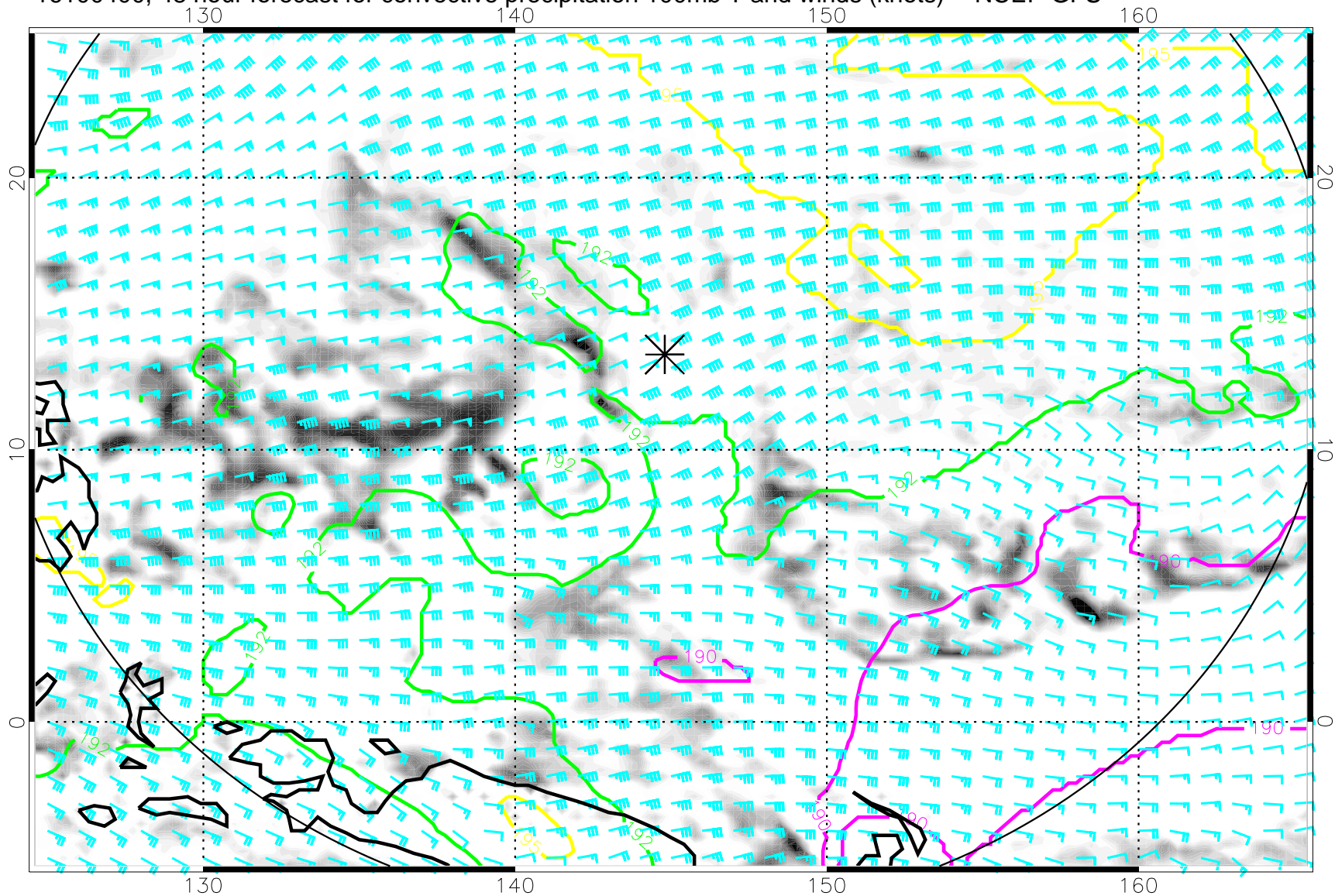
16100400, 48 hour forecast for convective precipitation 100mb T and winds (knots) -- NCEP GFS
