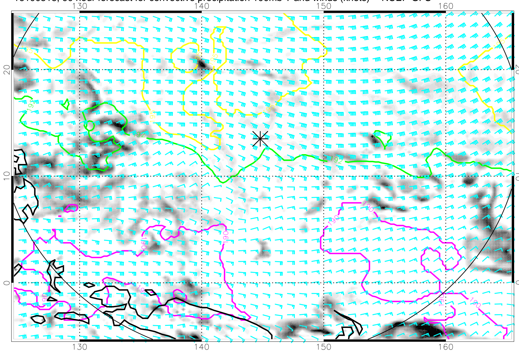
16100518, 90 hour forecast for convective precipitation 100mb T and winds (knots) -- NCEP GFS
