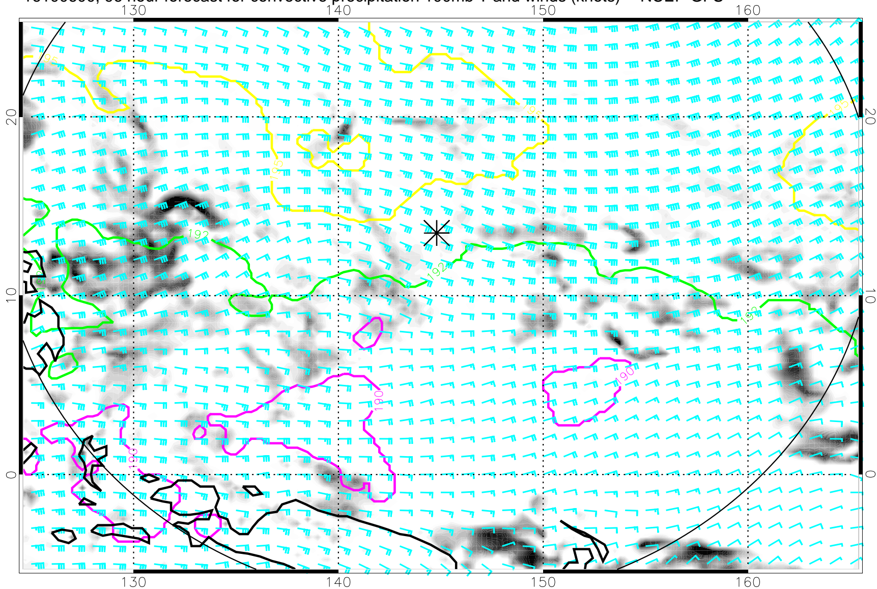
16100600, 96 hour forecast for convective precipitation 100mb T and winds (knots) -- NCEP GFS
