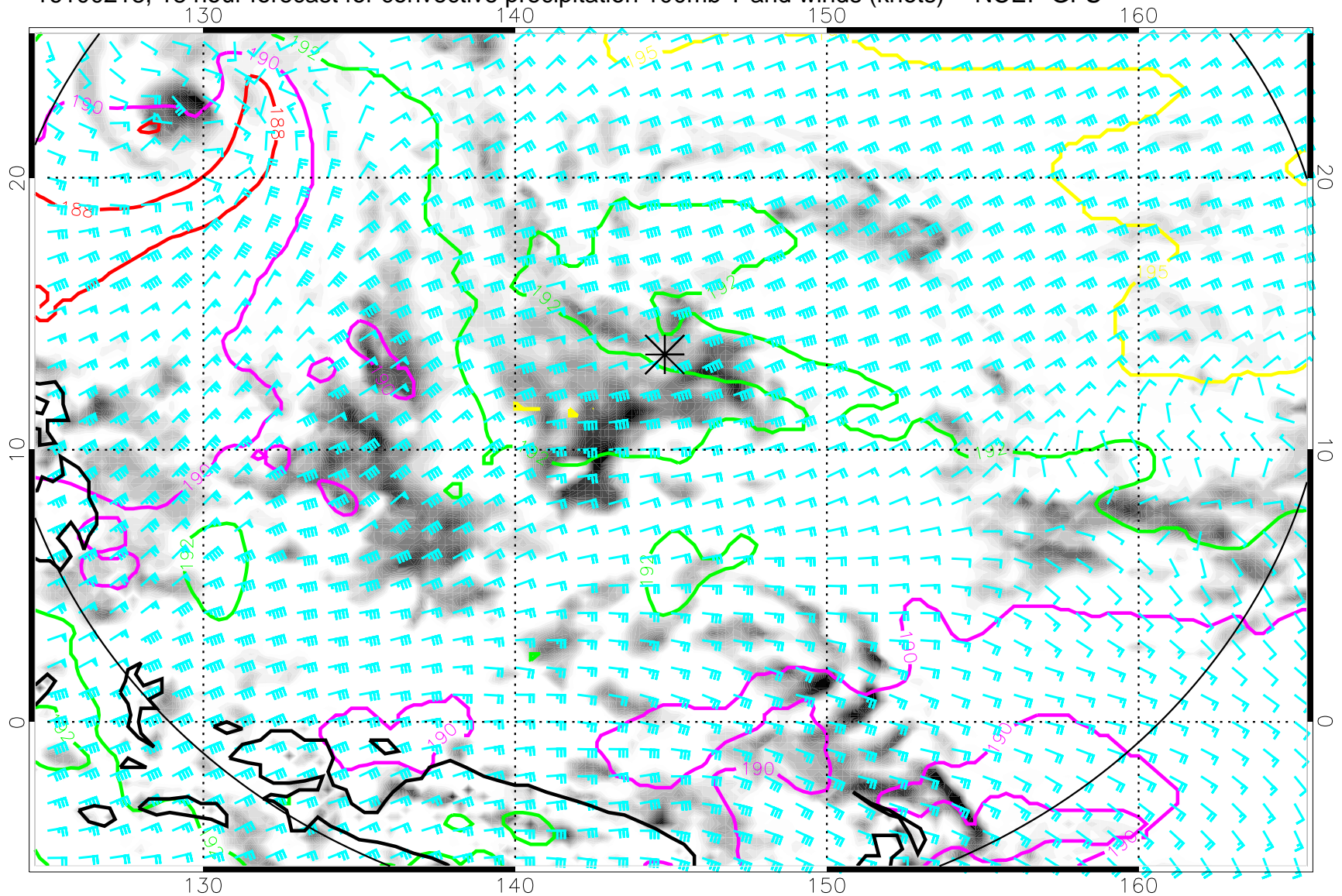
16100218, 18 hour forecast for convective precipitation 100mb T and winds (knots) -- NCEP GFS
