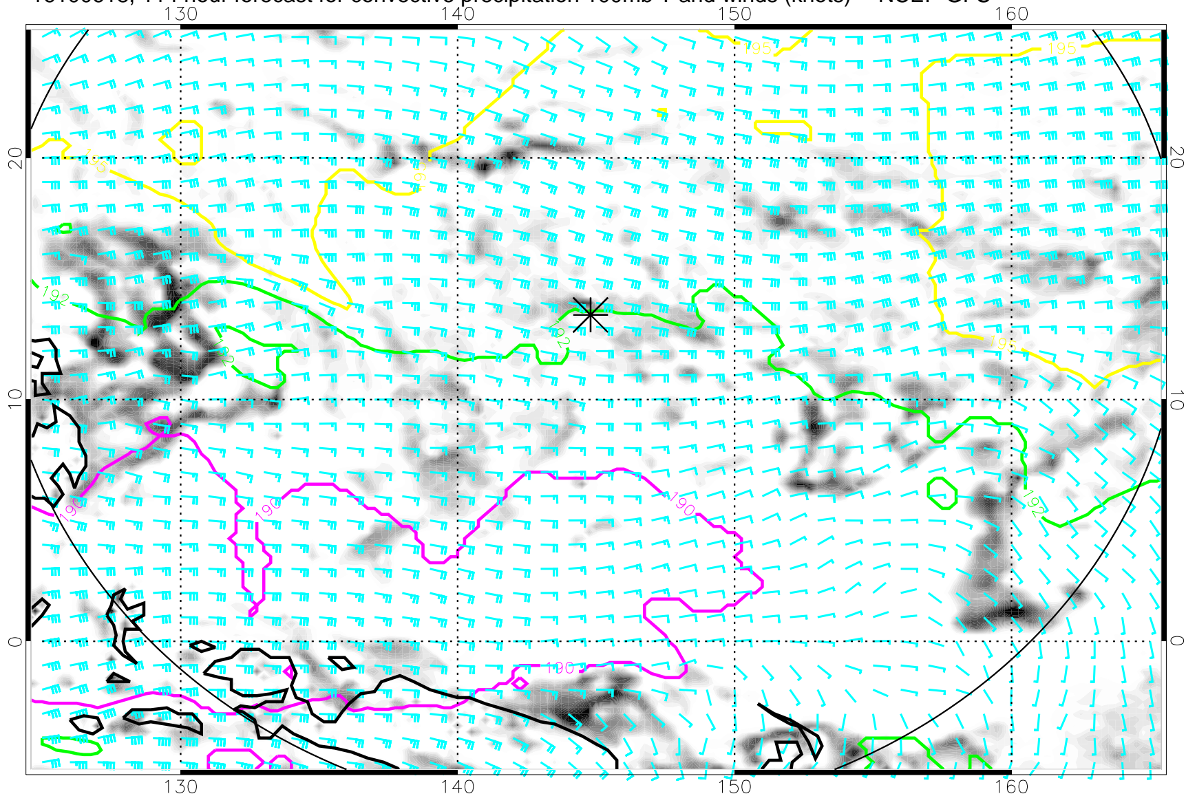
16100618, 114 hour forecast for convective precipitation 100mb T and winds (knots) -- NCEP GFS
