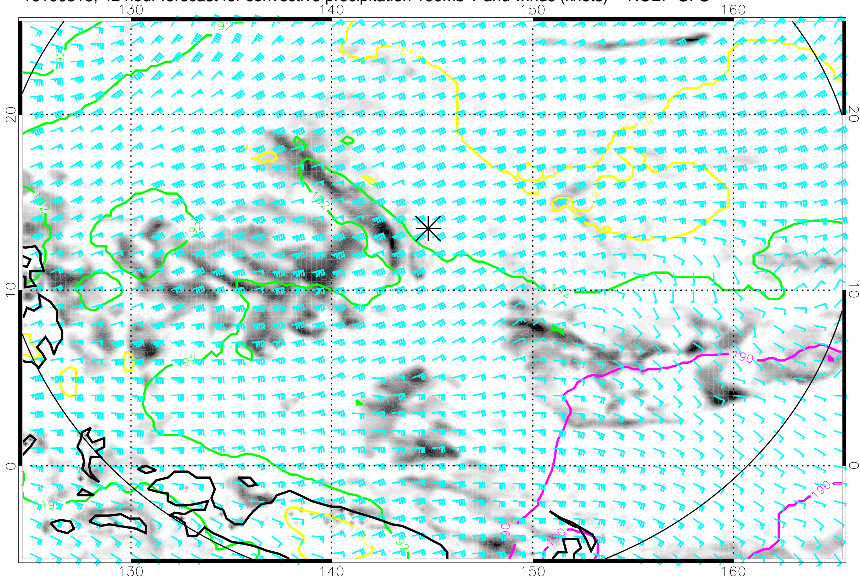
16100318, 42 hour forecast for convective precipitation 100mb T and winds (knots) -- NCEP GFS
