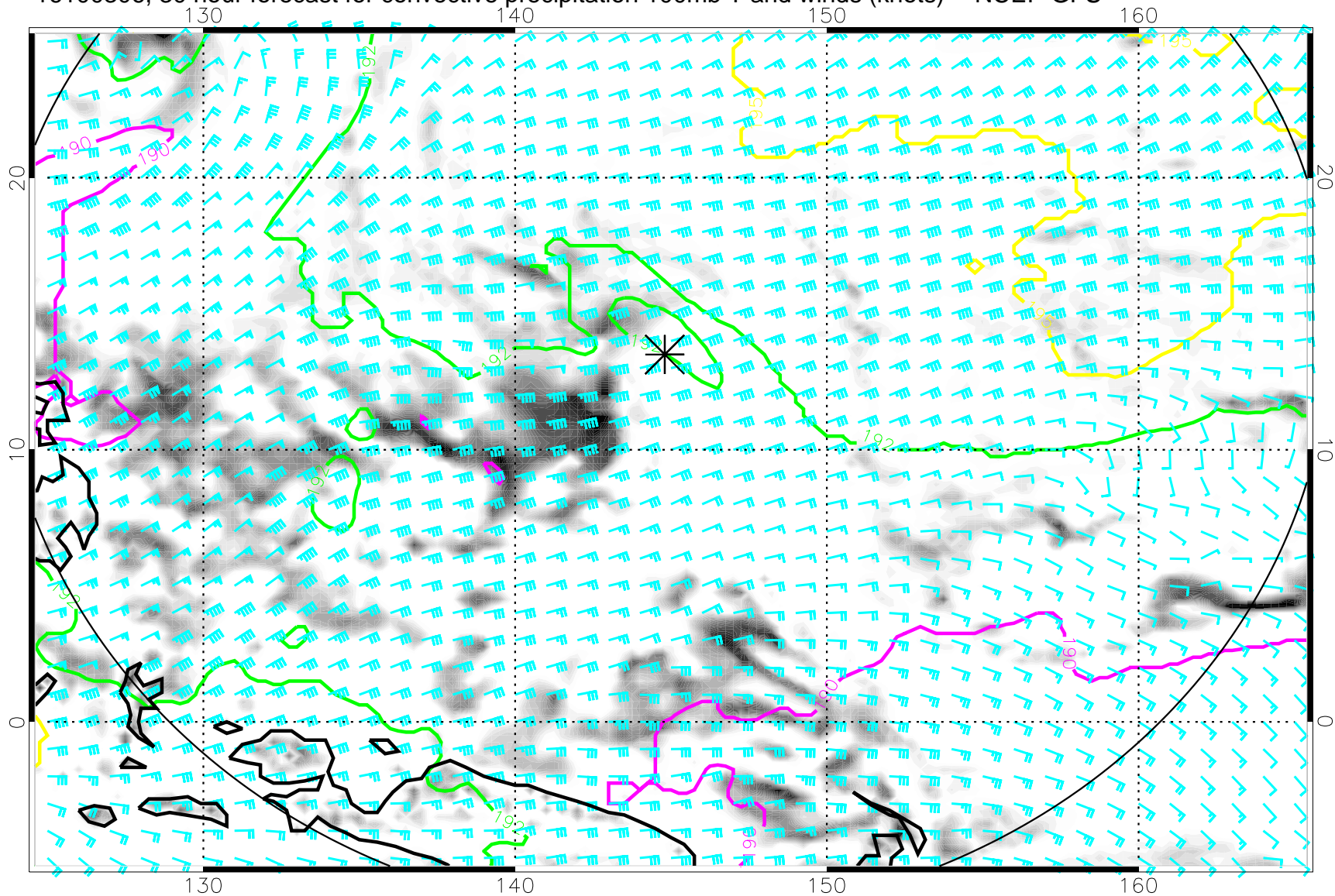
16100306, 30 hour forecast for convective precipitation 100mb T and winds (knots) -- NCEP GFS
