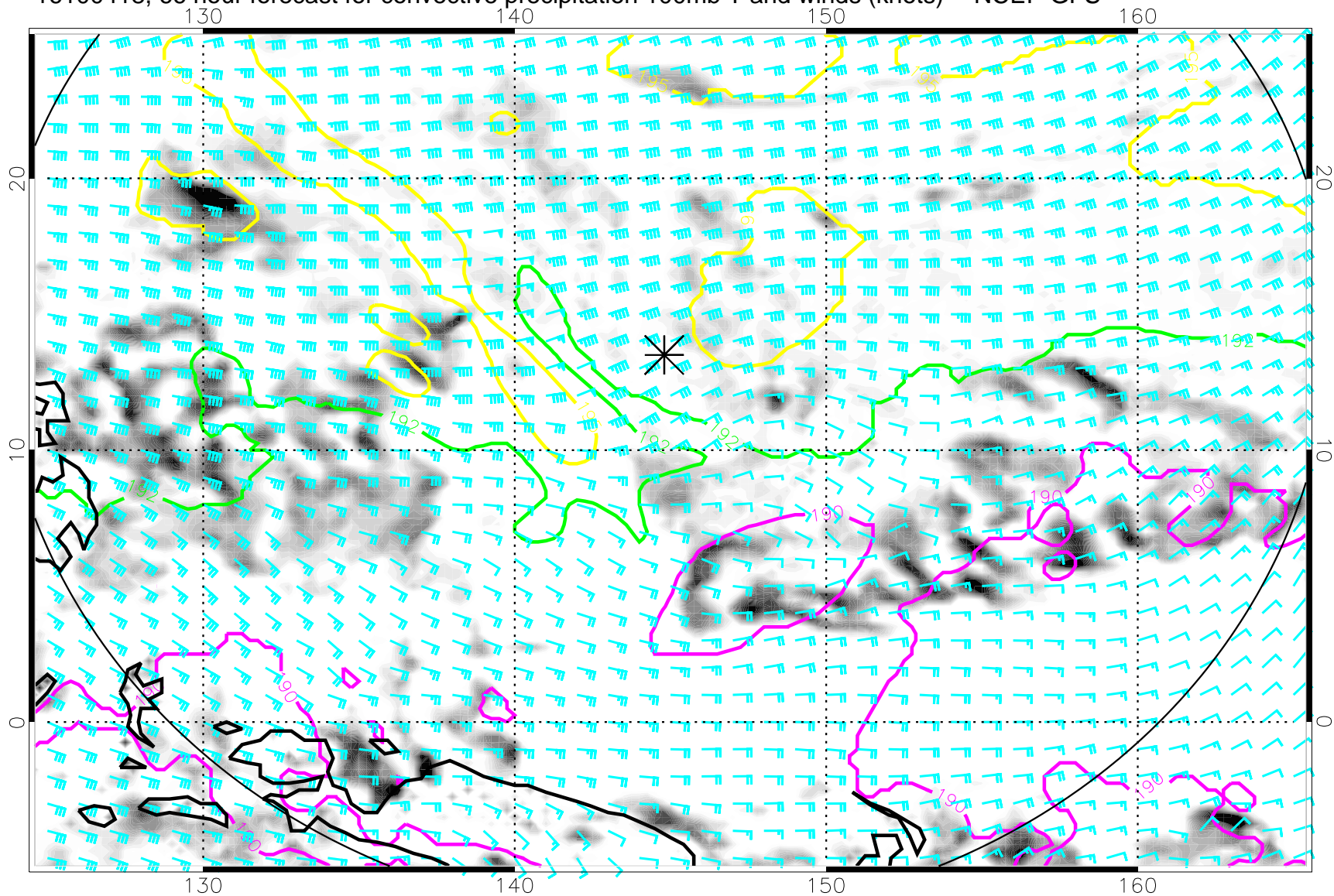
16100418, 66 hour forecast for convective precipitation 100mb T and winds (knots) -- NCEP GFS
