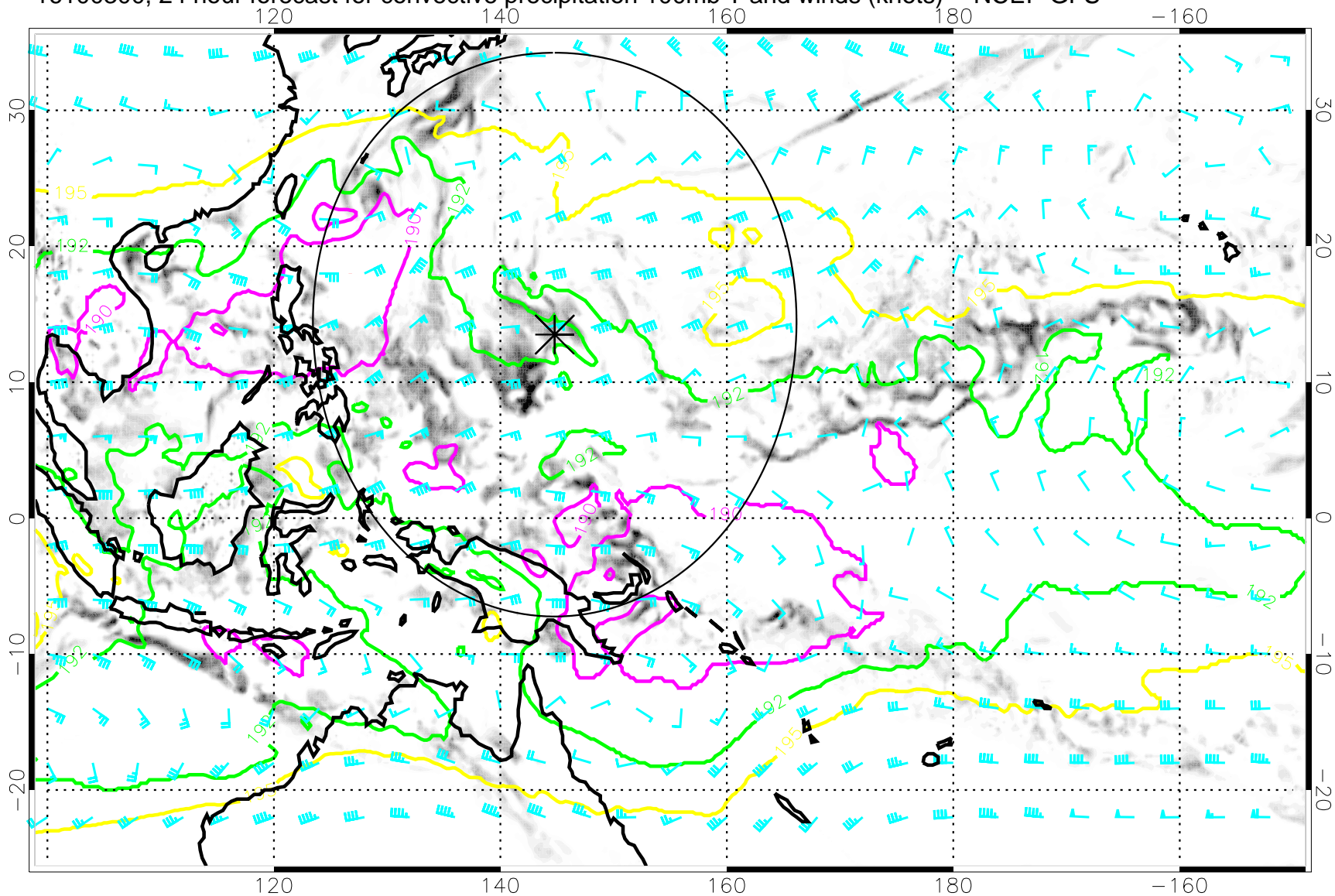
16100300, 24 hour forecast for convective precipitation 100mb T and winds (knots) -- NCEP GFS
