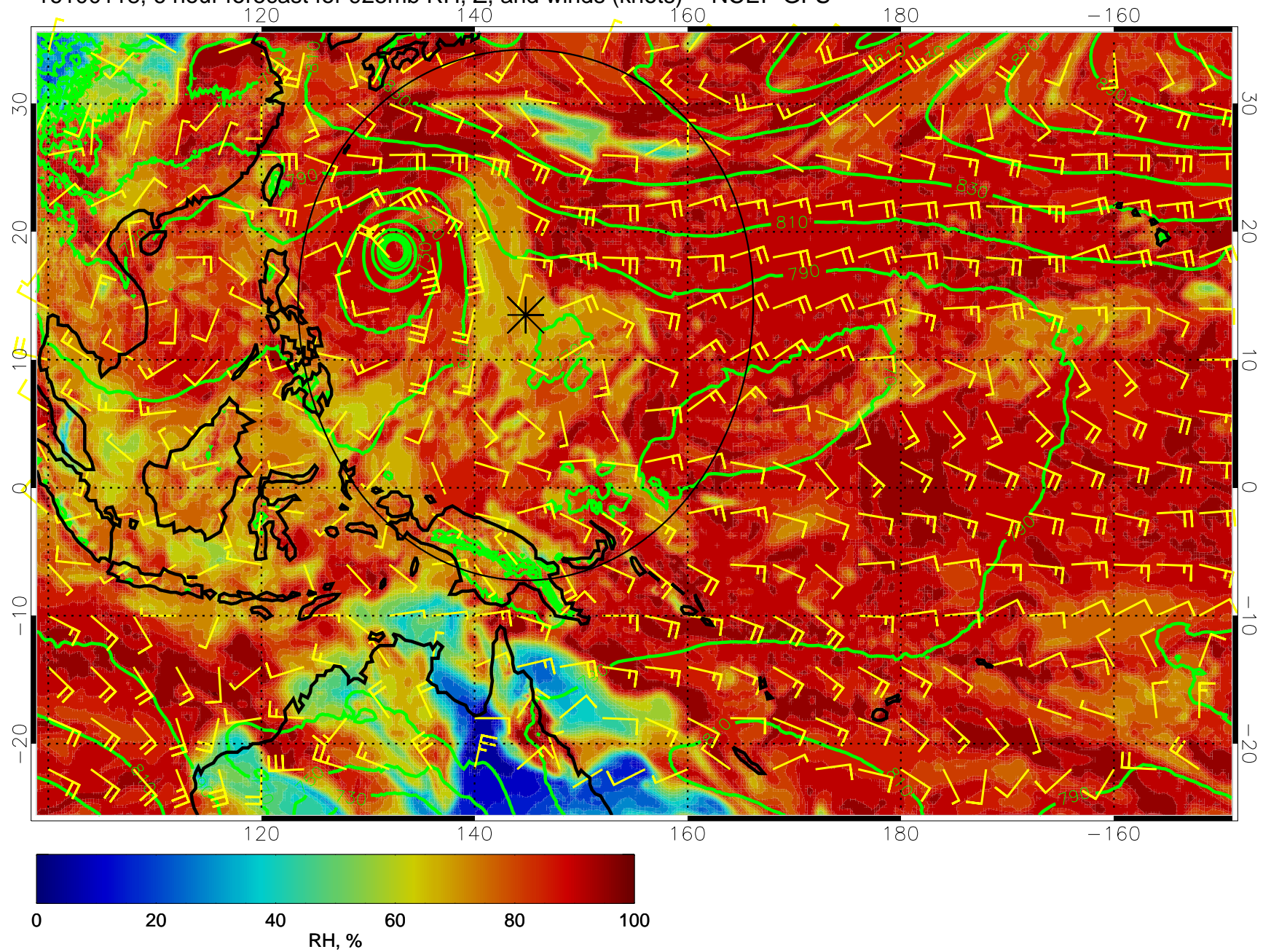
16100118, 6 hour forecast for 925mb RH, Z, and winds (knots) -- NCEP GFS
