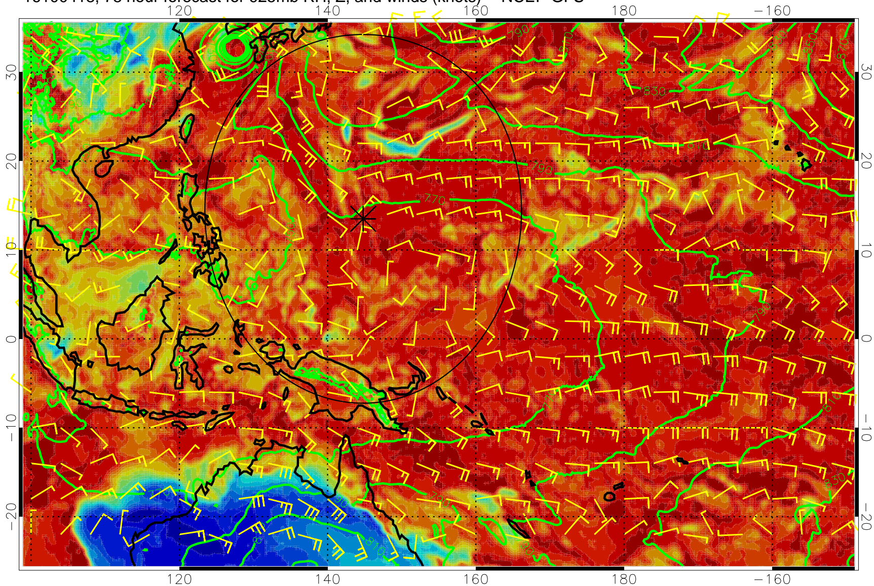
16100418, 78 hour forecast for 925mb RH, Z, and winds (knots) -- NCEP GFS
