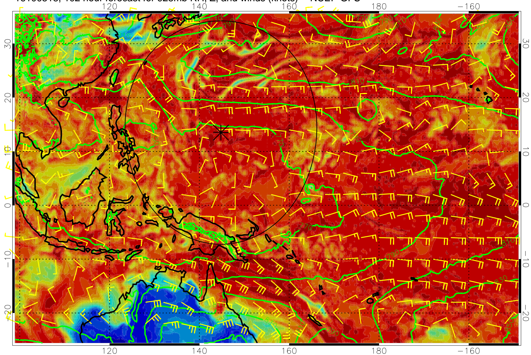
16100518, 102 hour forecast for 925mb RH, Z, and winds (knots) -- NCEP GFS
