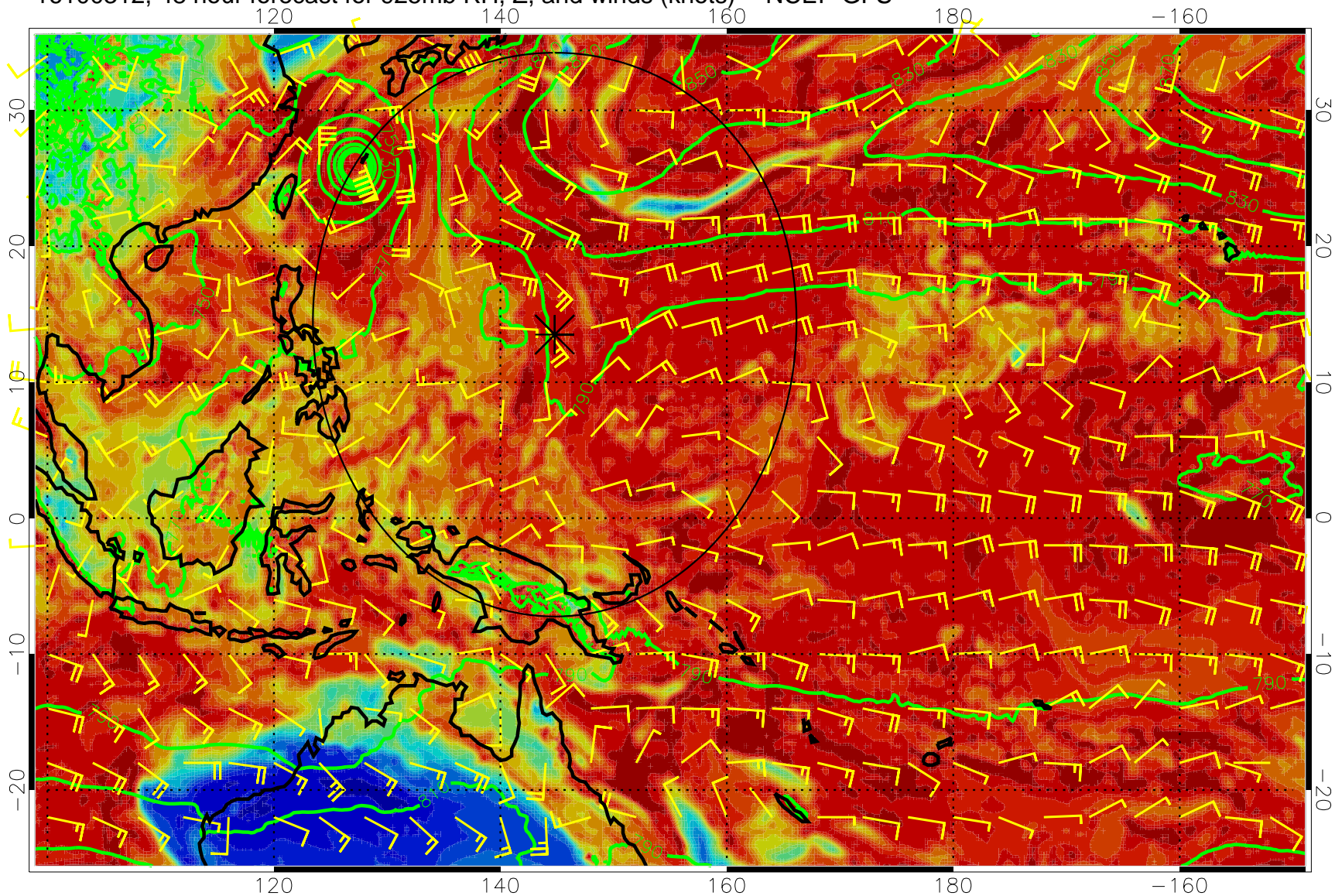
16100312, 48 hour forecast for 925mb RH, Z, and winds (knots) -- NCEP GFS
