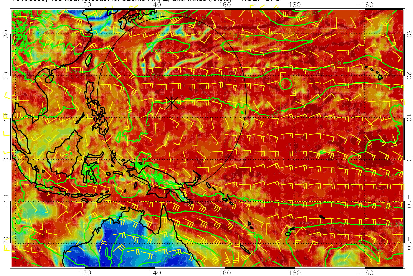
16100600, 108 hour forecast for 925mb RH, Z, and winds (knots) -- NCEP GFS
