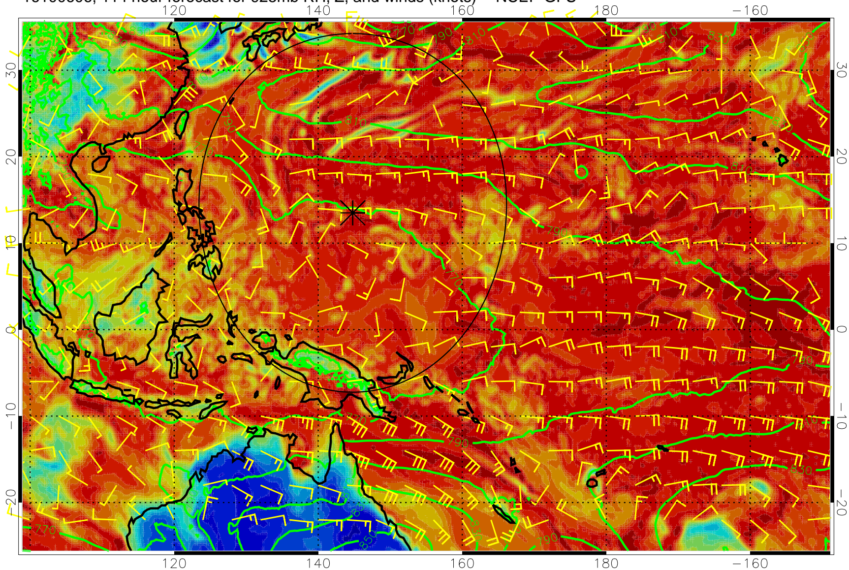
16100606, 114 hour forecast for 925mb RH, Z, and winds (knots) -- NCEP GFS
