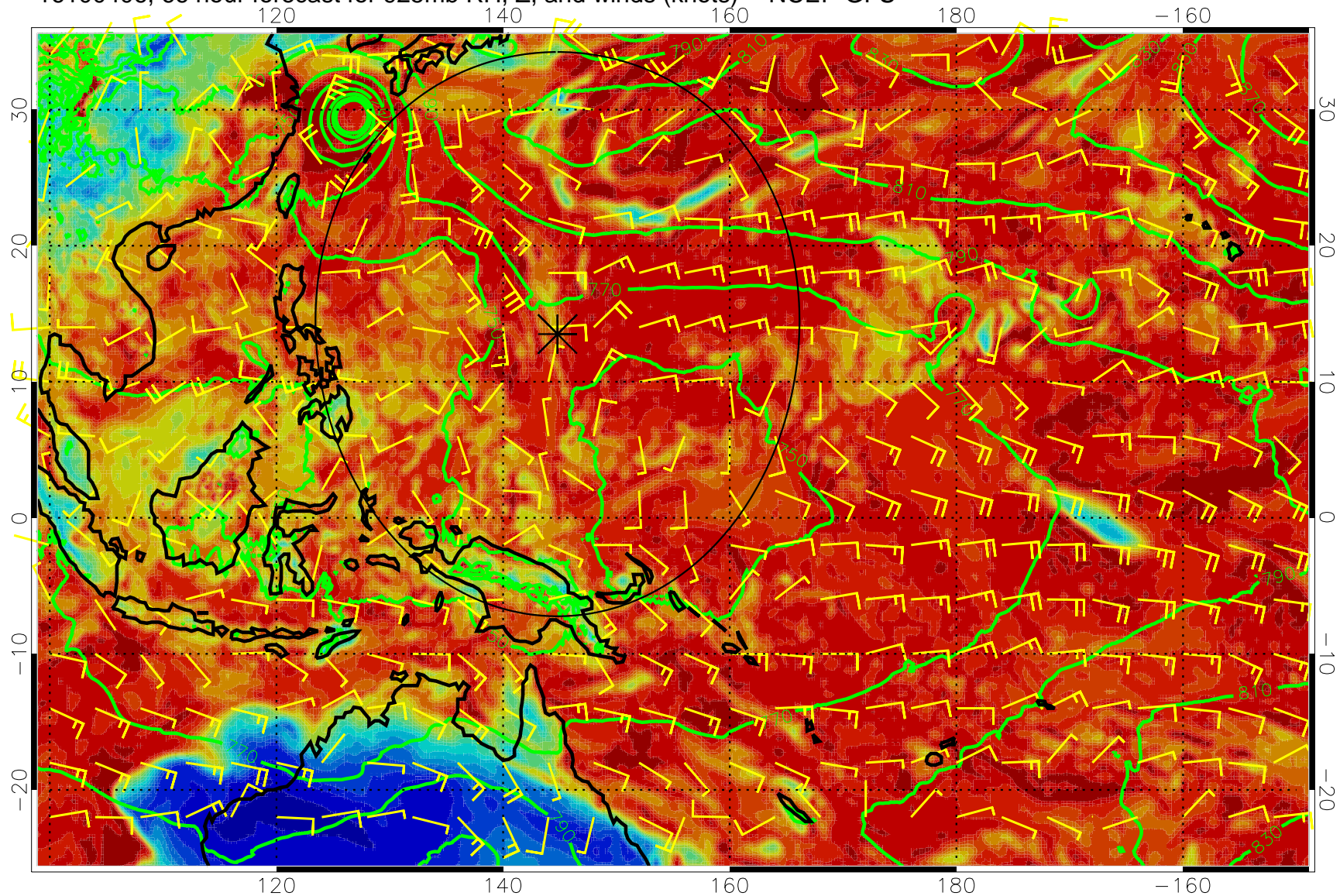
16100406, 66 hour forecast for 925mb RH, Z, and winds (knots) -- NCEP GFS
