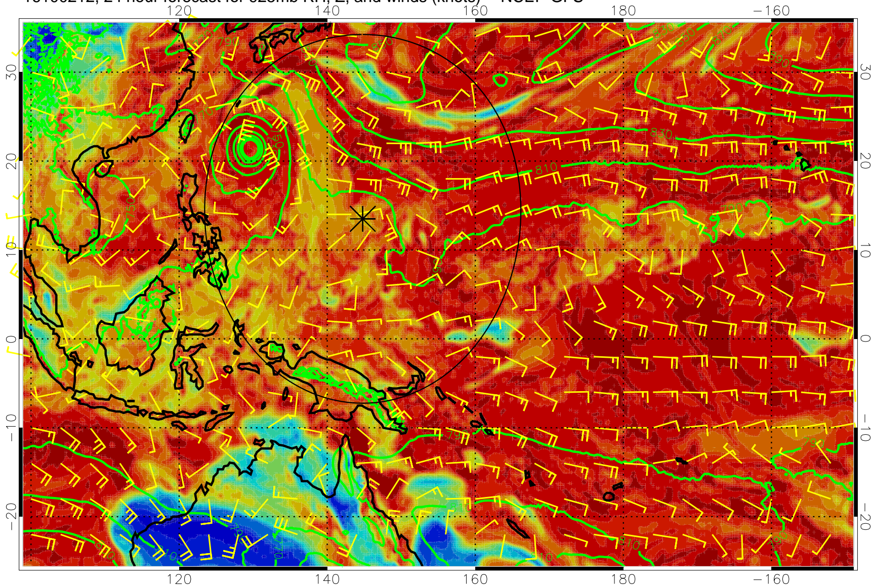
16100212, 24 hour forecast for 925mb RH, Z, and winds (knots) -- NCEP GFS
