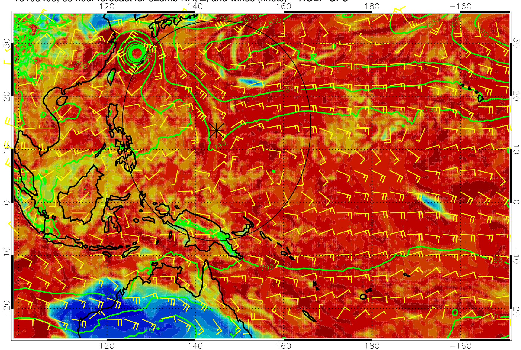
16100400, 60 hour forecast for 925mb RH, Z, and winds (knots) -- NCEP GFS
