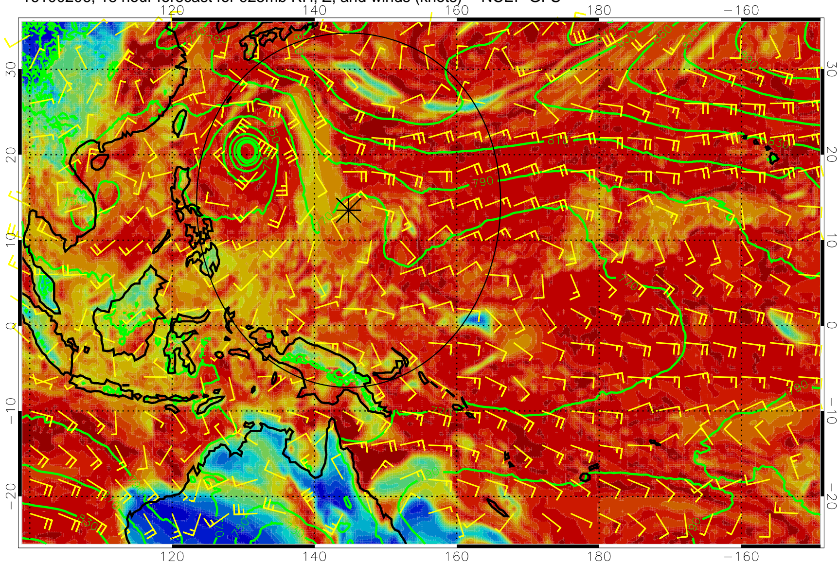
16100206, 18 hour forecast for 925mb RH, Z, and winds (knots) -- NCEP GFS
