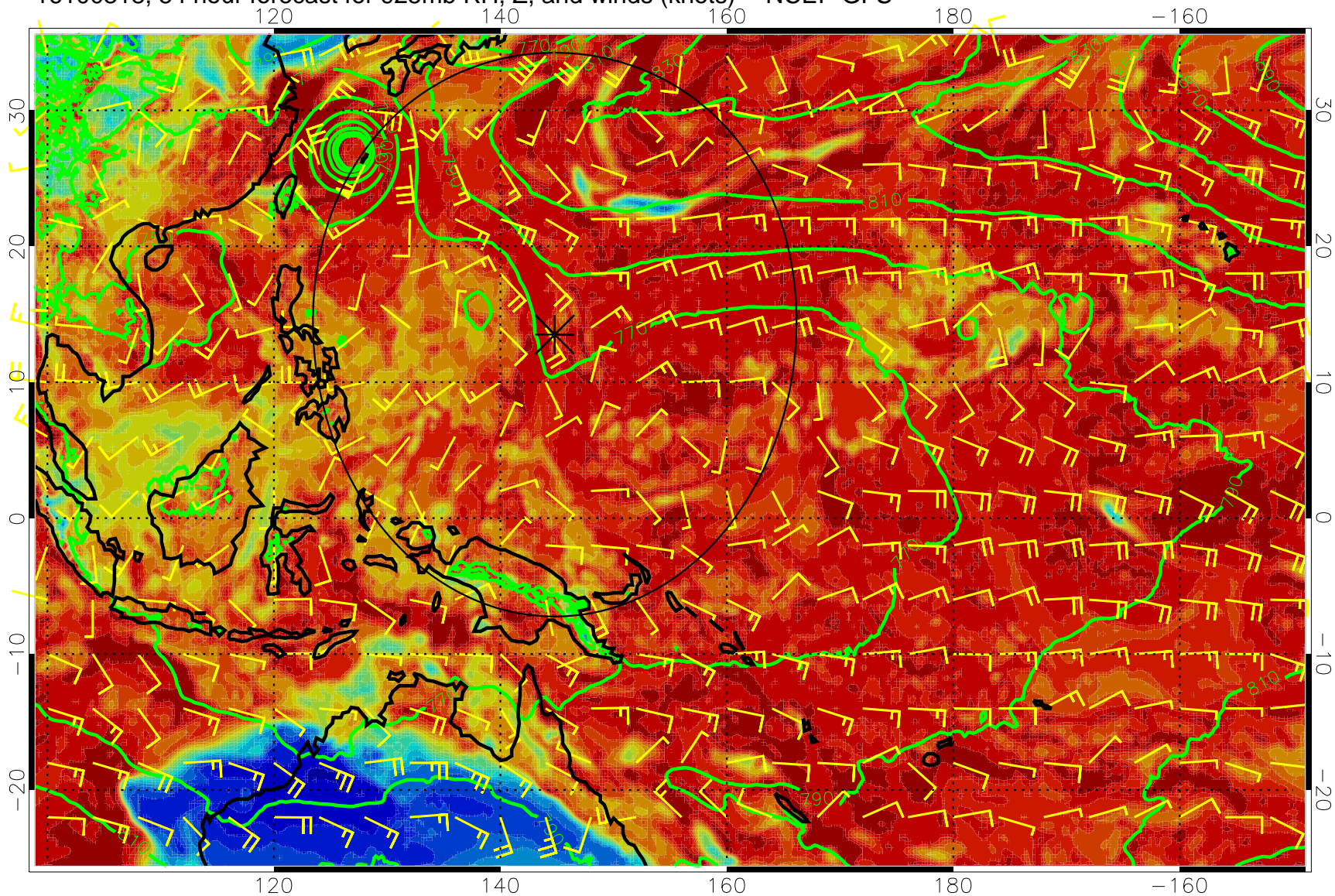
16100318, 54 hour forecast for 925mb RH, Z, and winds (knots) -- NCEP GFS
