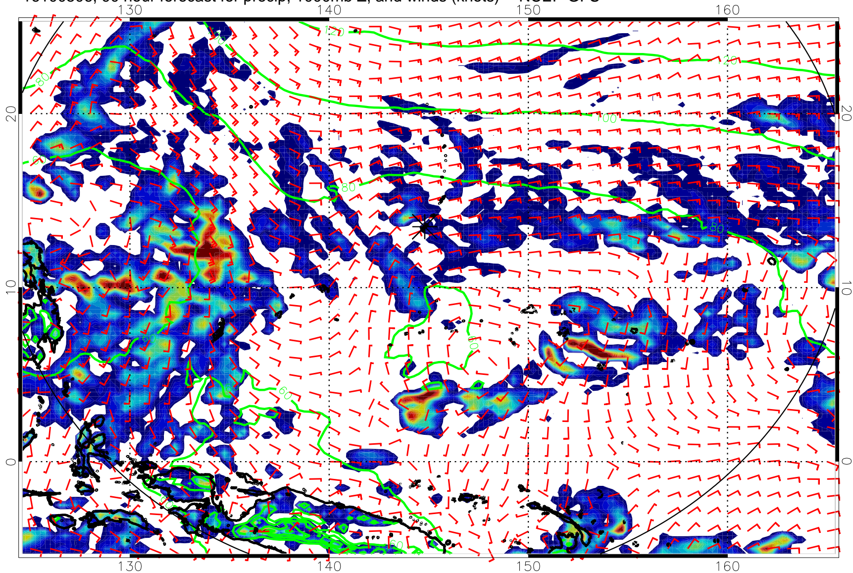
16100506, 90 hour forecast for precip, 1000mb Z, and winds (knots) -- NCEP GFS
