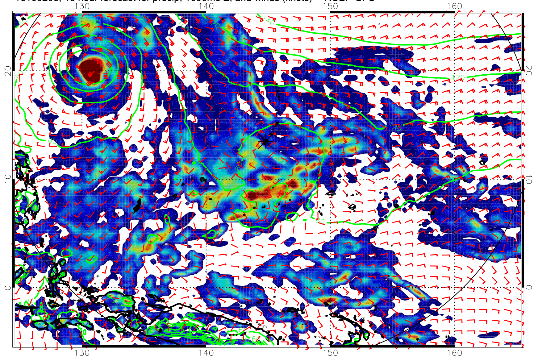
16100206, 18 hour forecast for precip, 1000mb Z, and winds (knots) -- NCEP GFS
