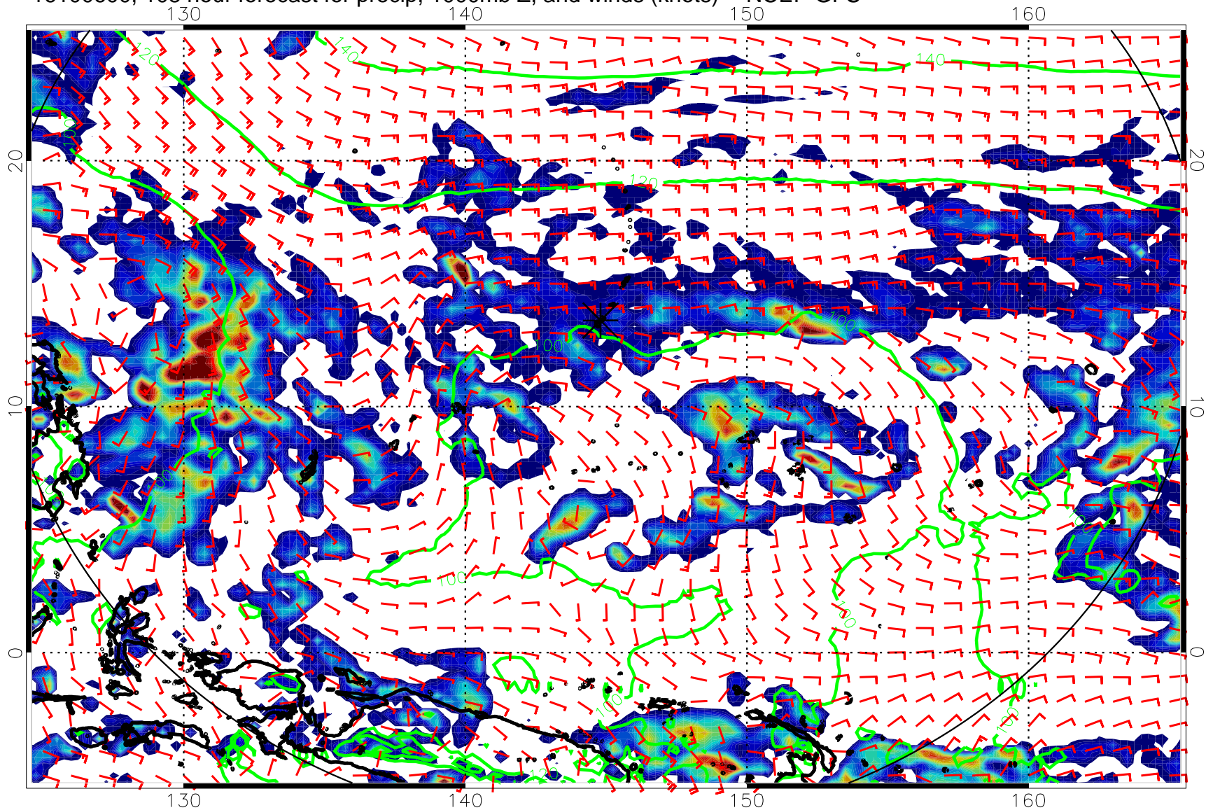
16100600, 108 hour forecast for precip, 1000mb Z, and winds (knots) -- NCEP GFS
