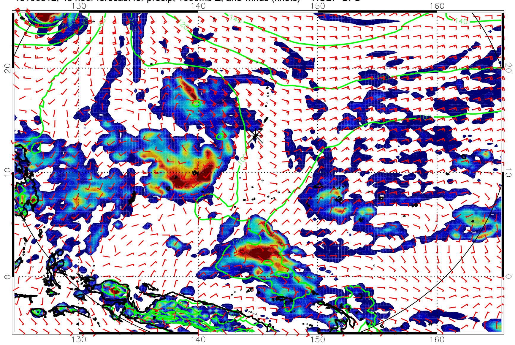
16100312, 48 hour forecast for precip, 1000mb Z, and winds (knots) -- NCEP GFS
