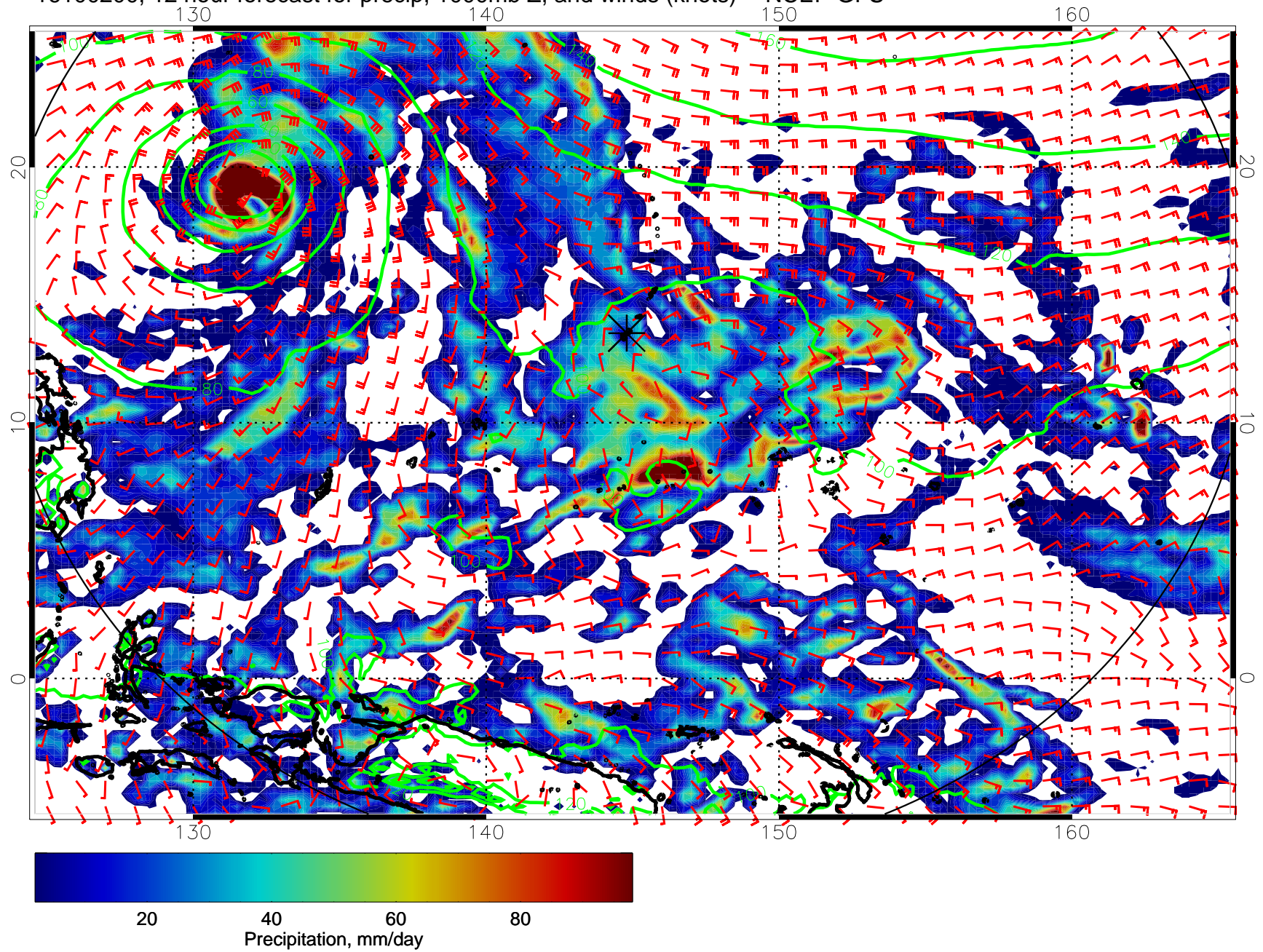
16100200, 12 hour forecast for precip, 1000mb Z, and winds (knots) -- NCEP GFS
