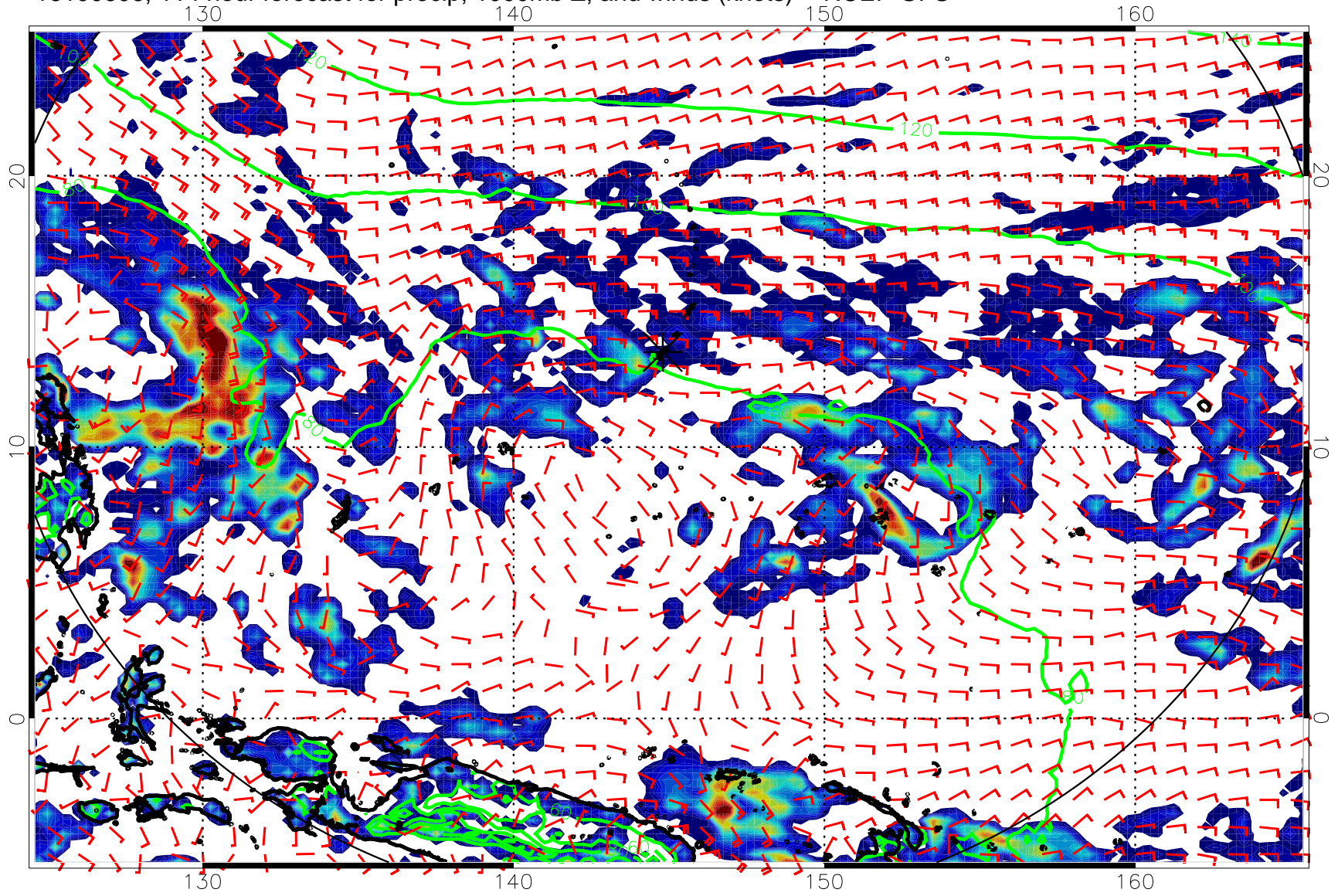
16100606, 114 hour forecast for precip, 1000mb Z, and winds (knots) -- NCEP GFS
