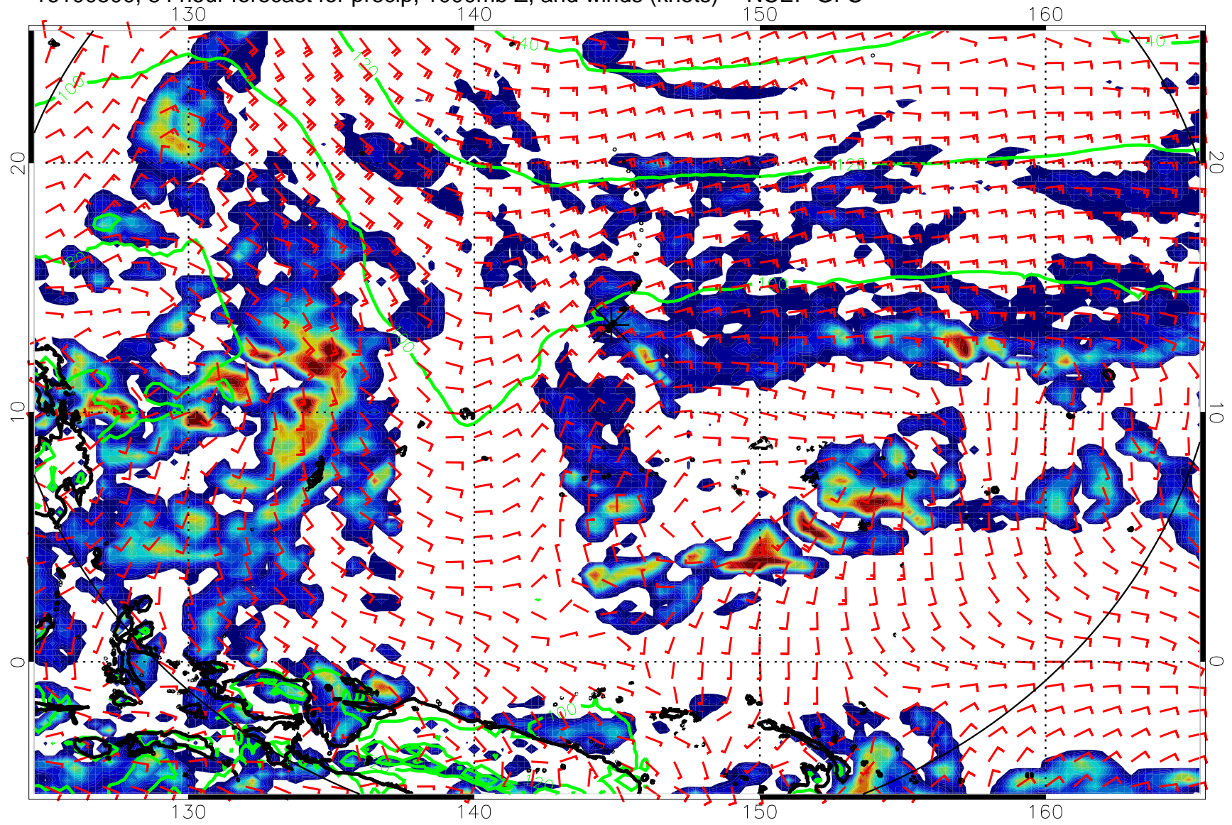
16100500, 84 hour forecast for precip, 1000mb Z, and winds (knots) -- NCEP GFS
