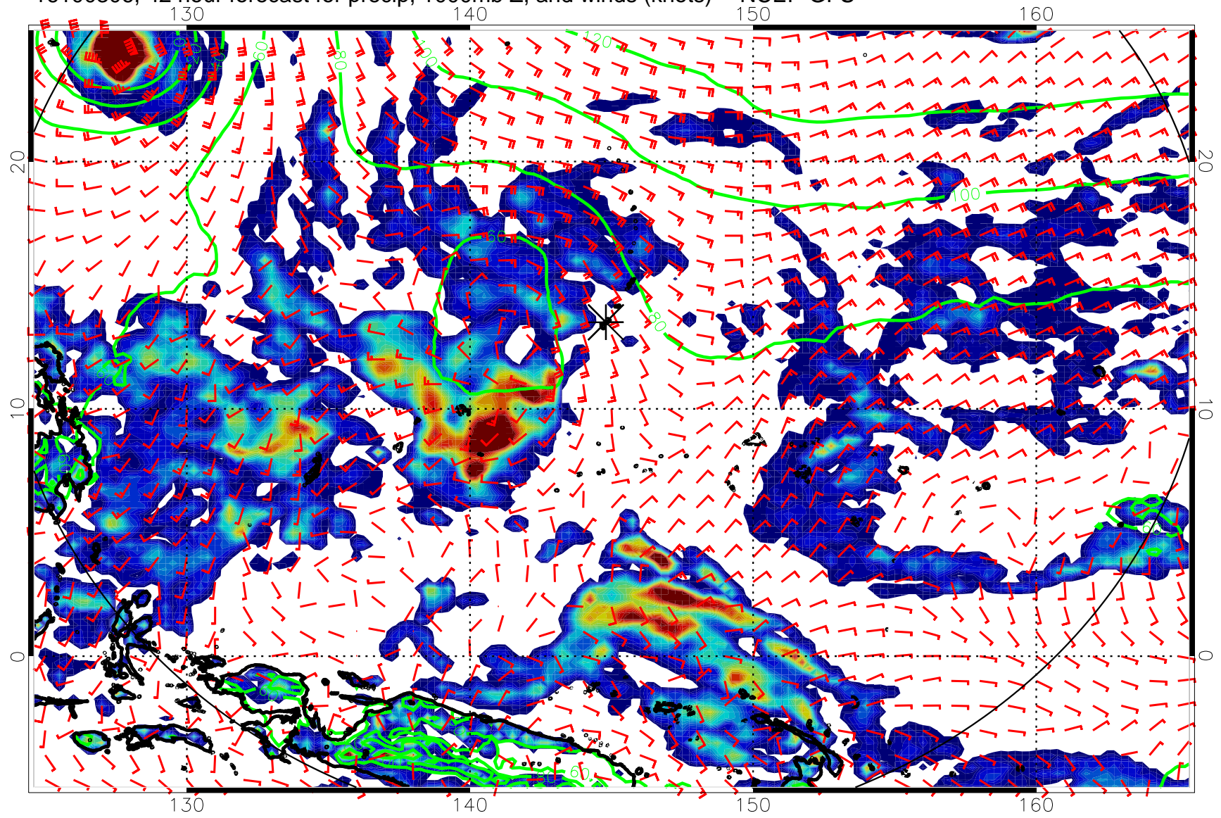
16100306, 42 hour forecast for precip, 1000mb Z, and winds (knots) -- NCEP GFS
