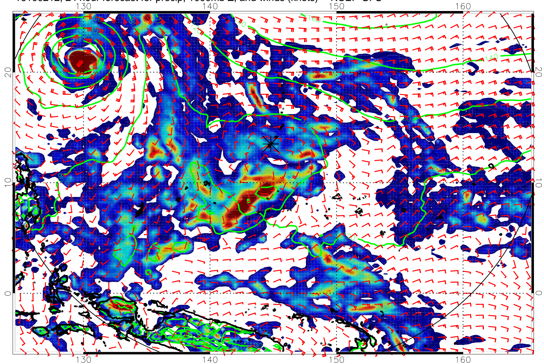
16100212, 24 hour forecast for precip, 1000mb Z, and winds (knots) -- NCEP GFS
