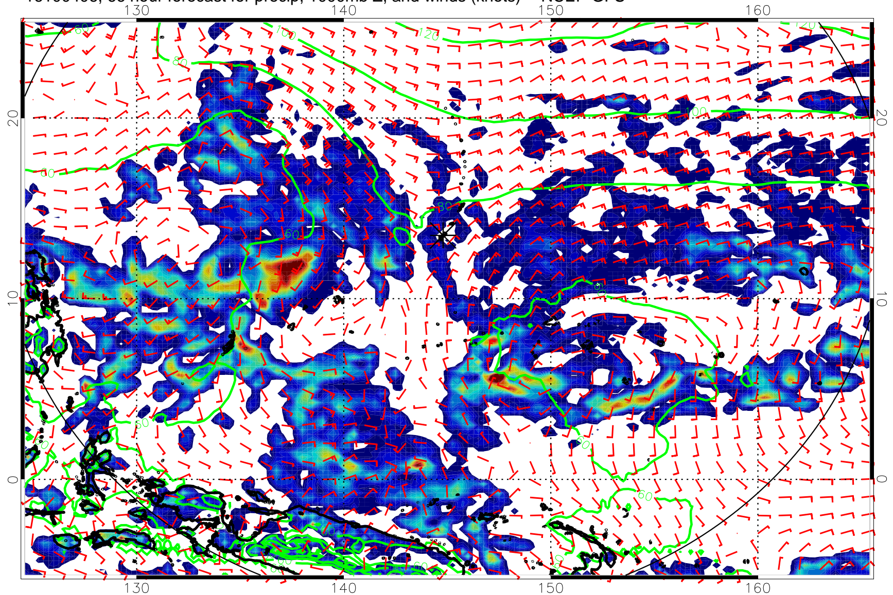
16100406, 66 hour forecast for precip, 1000mb Z, and winds (knots) -- NCEP GFS
