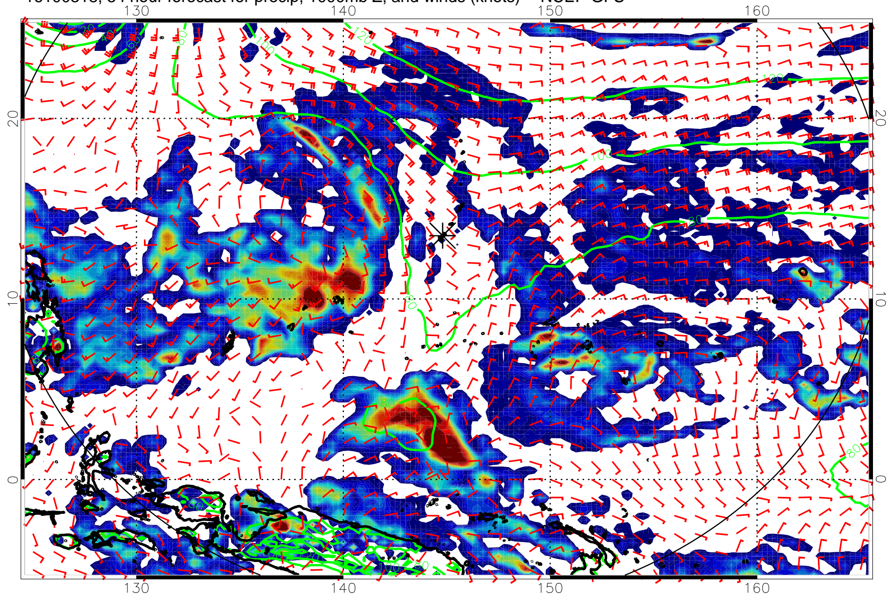
16100318, 54 hour forecast for precip, 1000mb Z, and winds (knots) -- NCEP GFS
