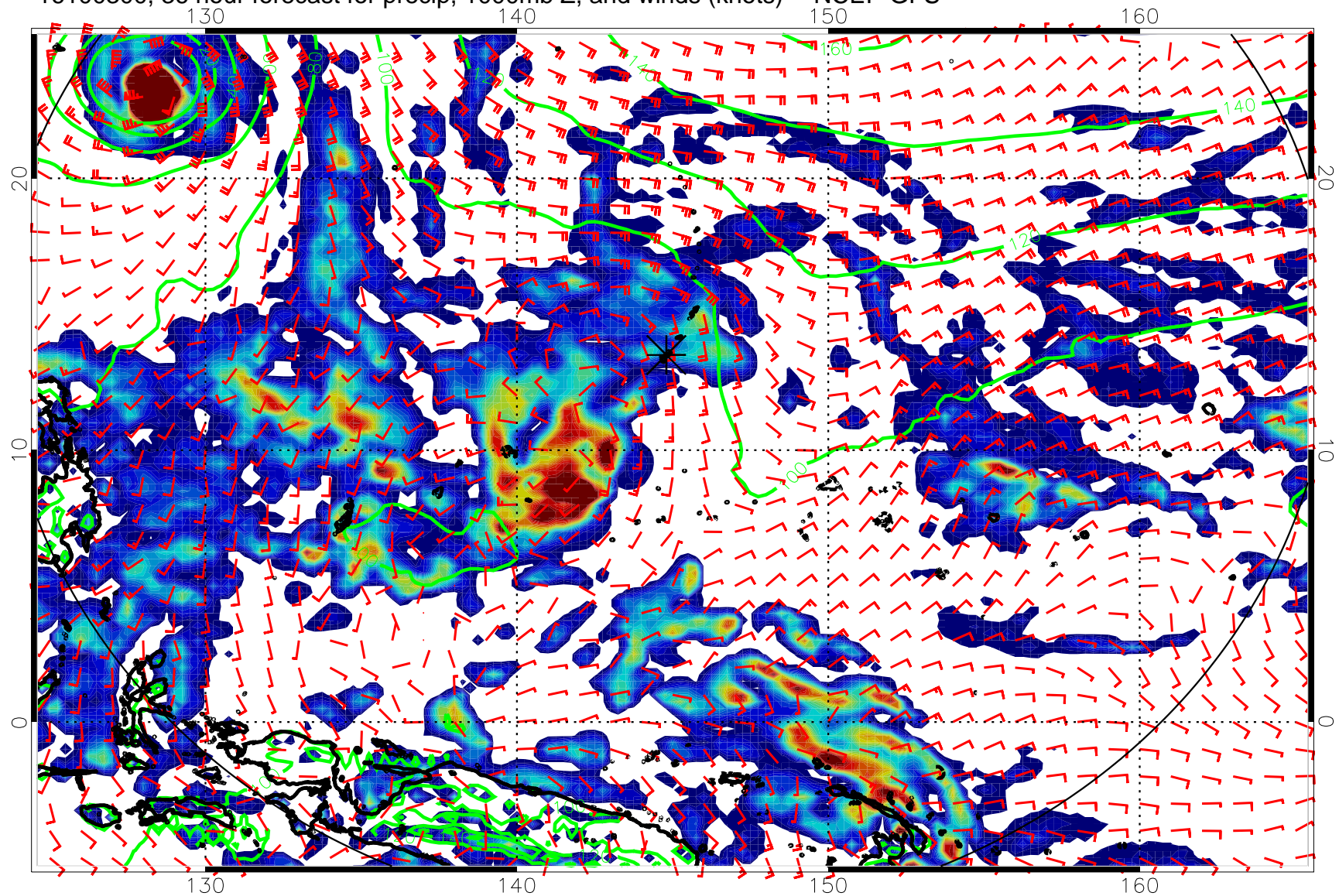
16100300, 36 hour forecast for precip, 1000mb Z, and winds (knots) -- NCEP GFS
