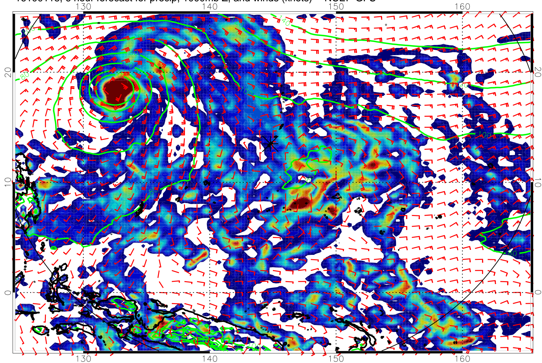
16100118, 6 hour forecast for precip, 1000mb Z, and winds (knots) -- NCEP GFS
