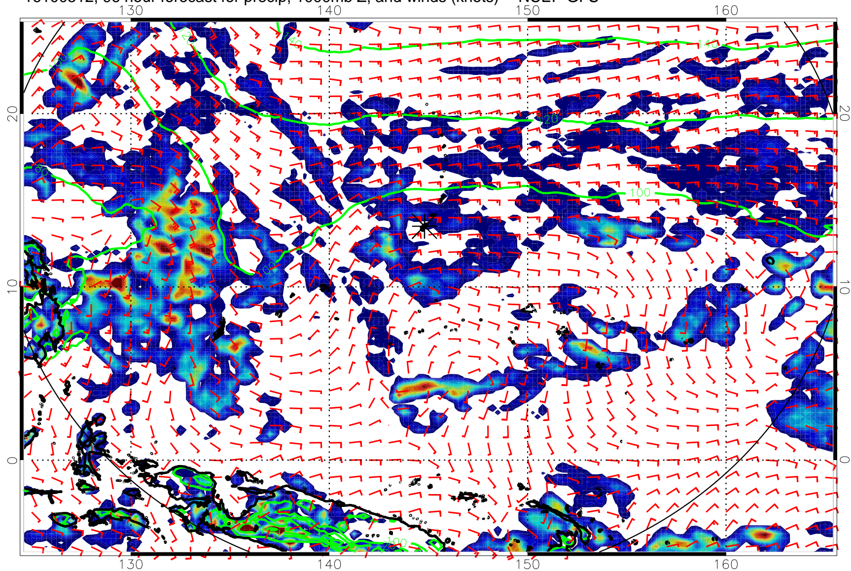
16100512, 96 hour forecast for precip, 1000mb Z, and winds (knots) -- NCEP GFS
