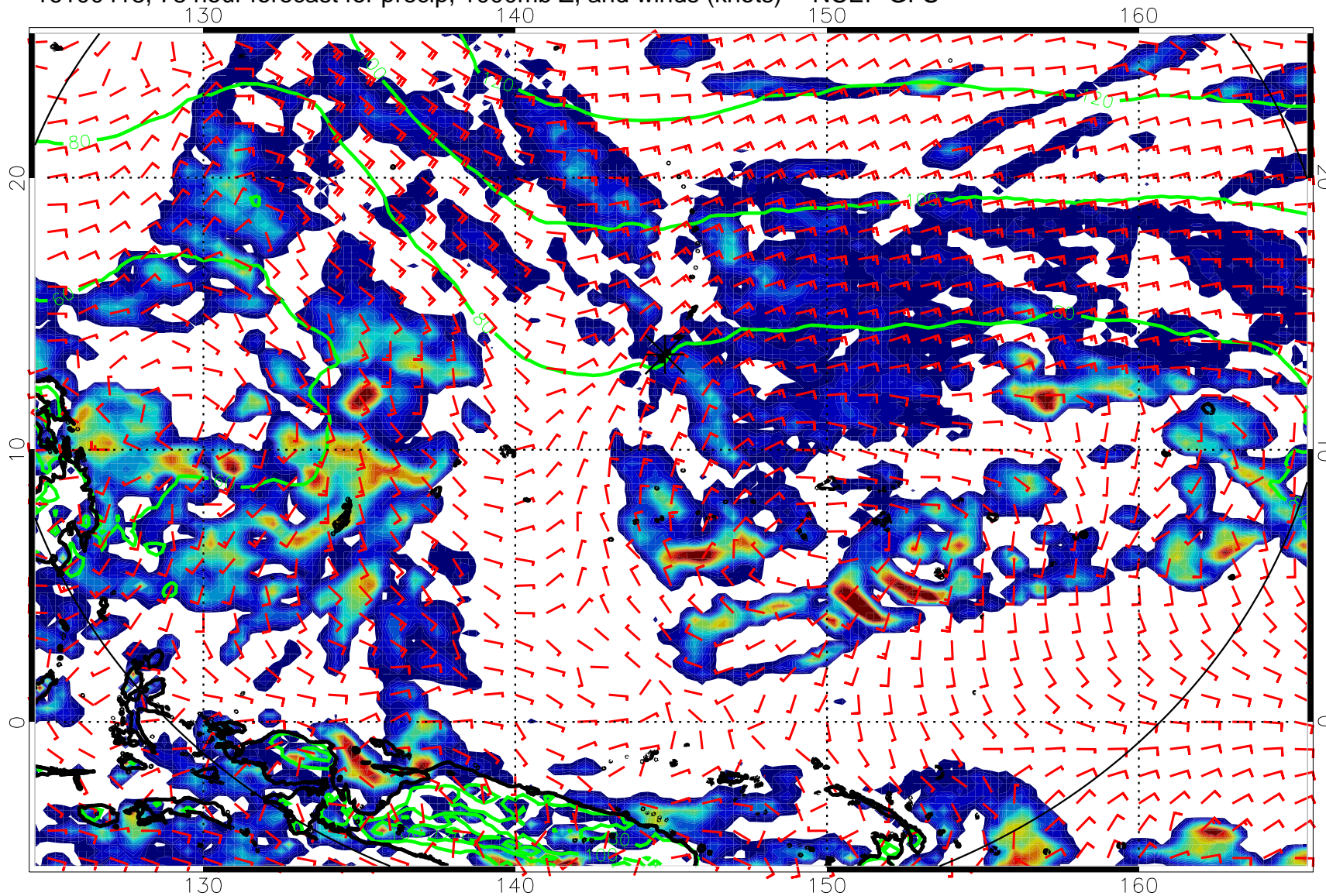
16100418, 78 hour forecast for precip, 1000mb Z, and winds (knots) -- NCEP GFS
