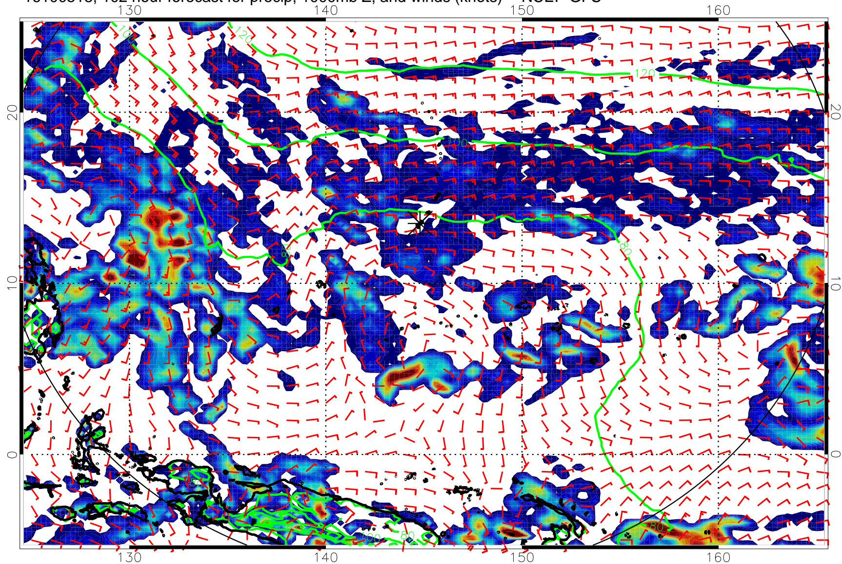
16100518, 102 hour forecast for precip, 1000mb Z, and winds (knots) -- NCEP GFS
