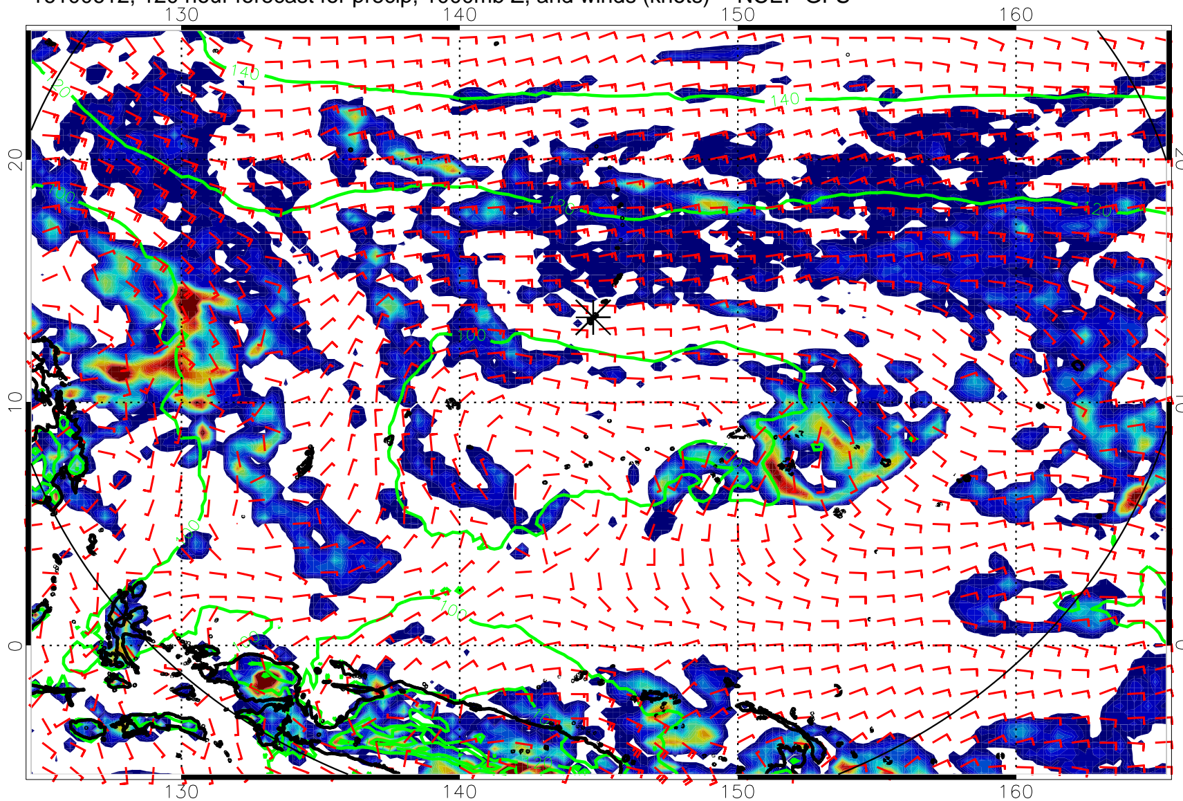
16100612, 120 hour forecast for precip, 1000mb Z, and winds (knots) -- NCEP GFS
