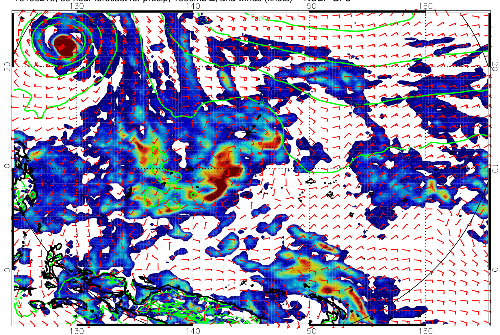
16100218, 30 hour forecast for precip, 1000mb Z, and winds (knots) -- NCEP GFS
