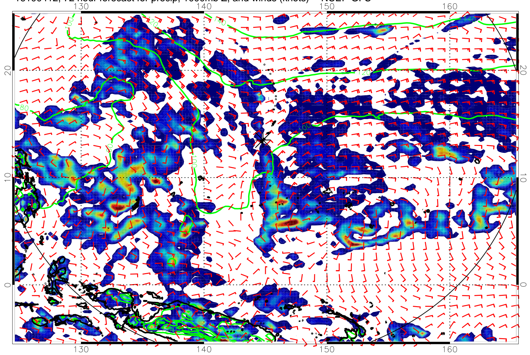
16100412, 72 hour forecast for precip, 1000mb Z, and winds (knots) -- NCEP GFS
