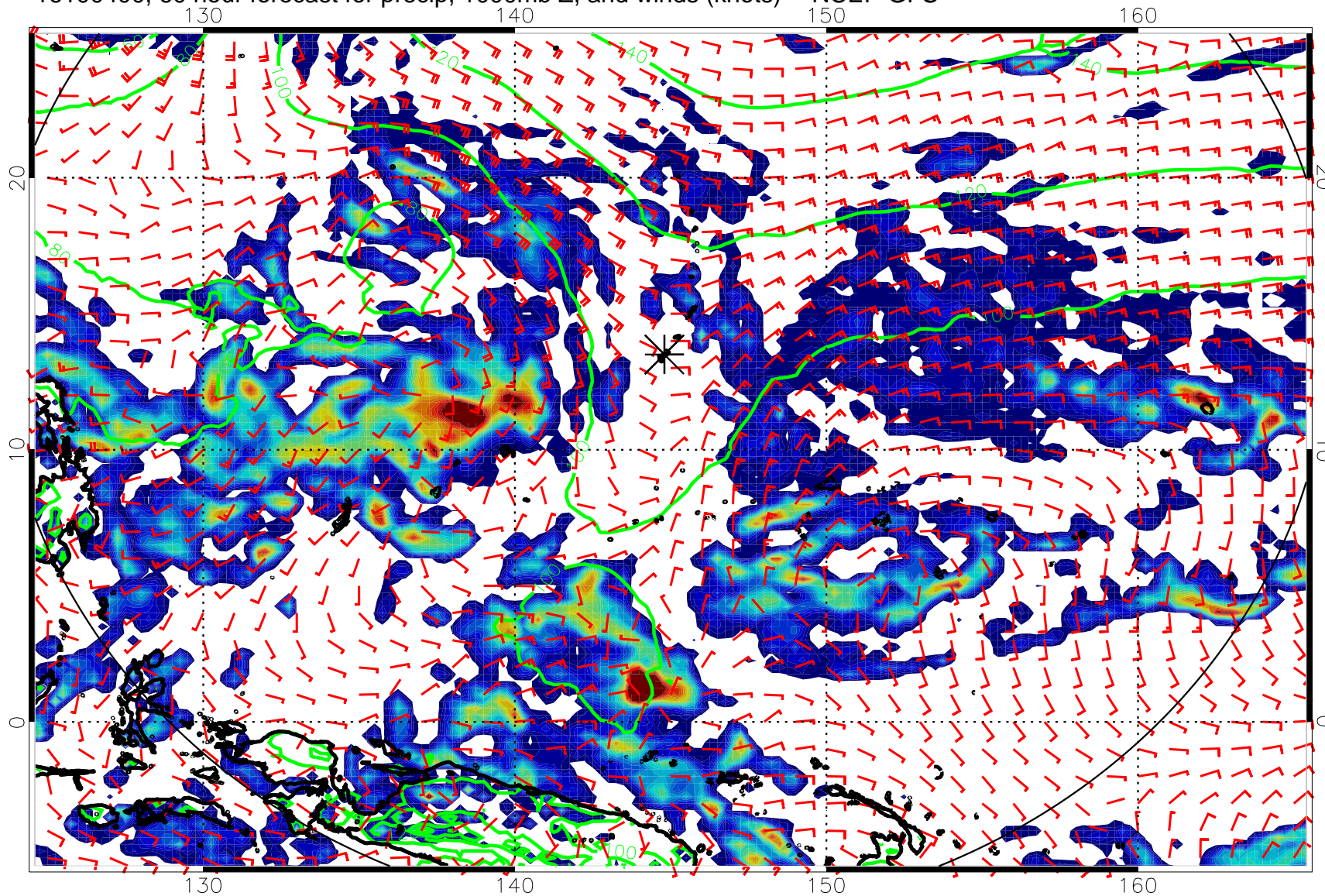
16100400, 60 hour forecast for precip, 1000mb Z, and winds (knots) -- NCEP GFS
