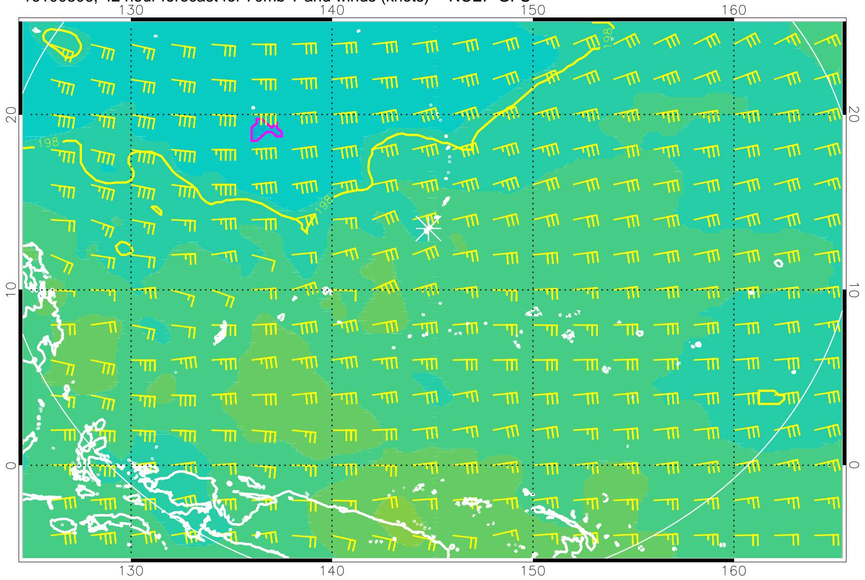
16100306, 42 hour forecast for 70mb T and winds (knots) -- NCEP GFS
