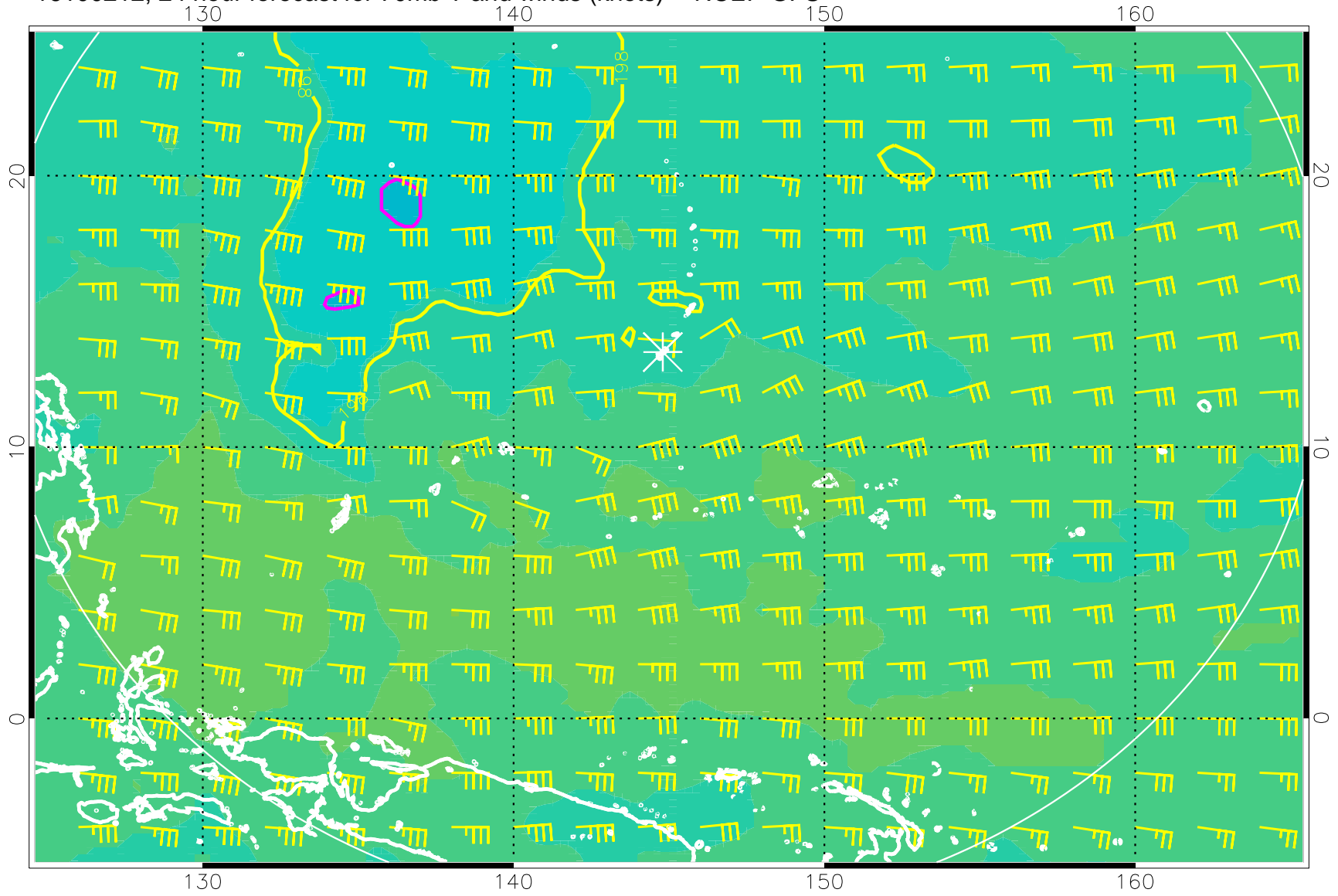
16100212, 24 hour forecast for 70mb T and winds (knots) -- NCEP GFS
