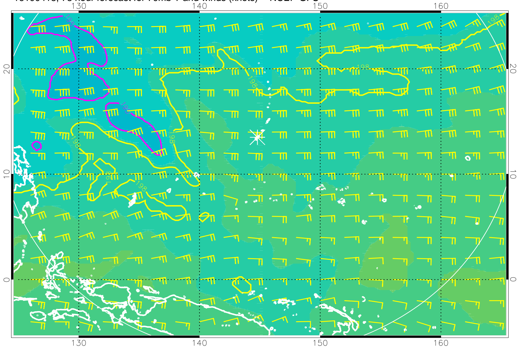
16100418, 78 hour forecast for 70mb T and winds (knots) -- NCEP GFS
