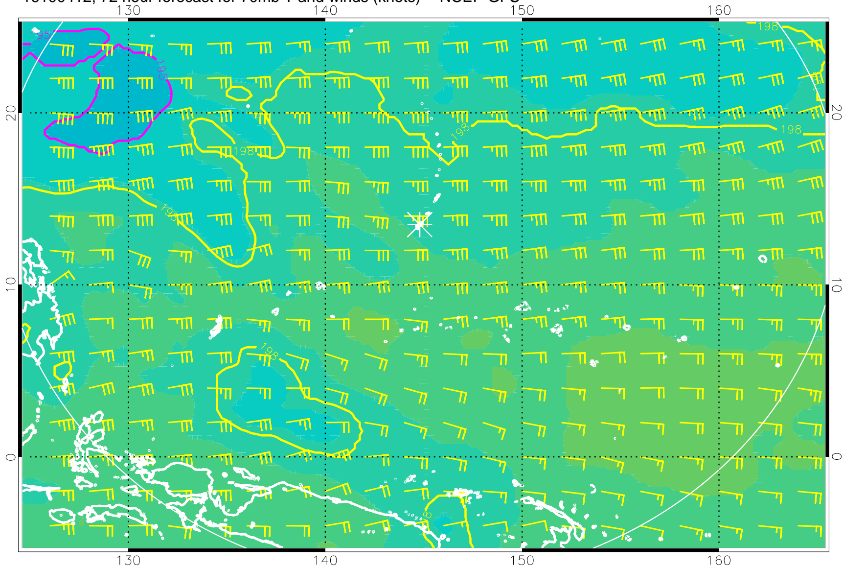
16100412, 72 hour forecast for 70mb T and winds (knots) -- NCEP GFS
