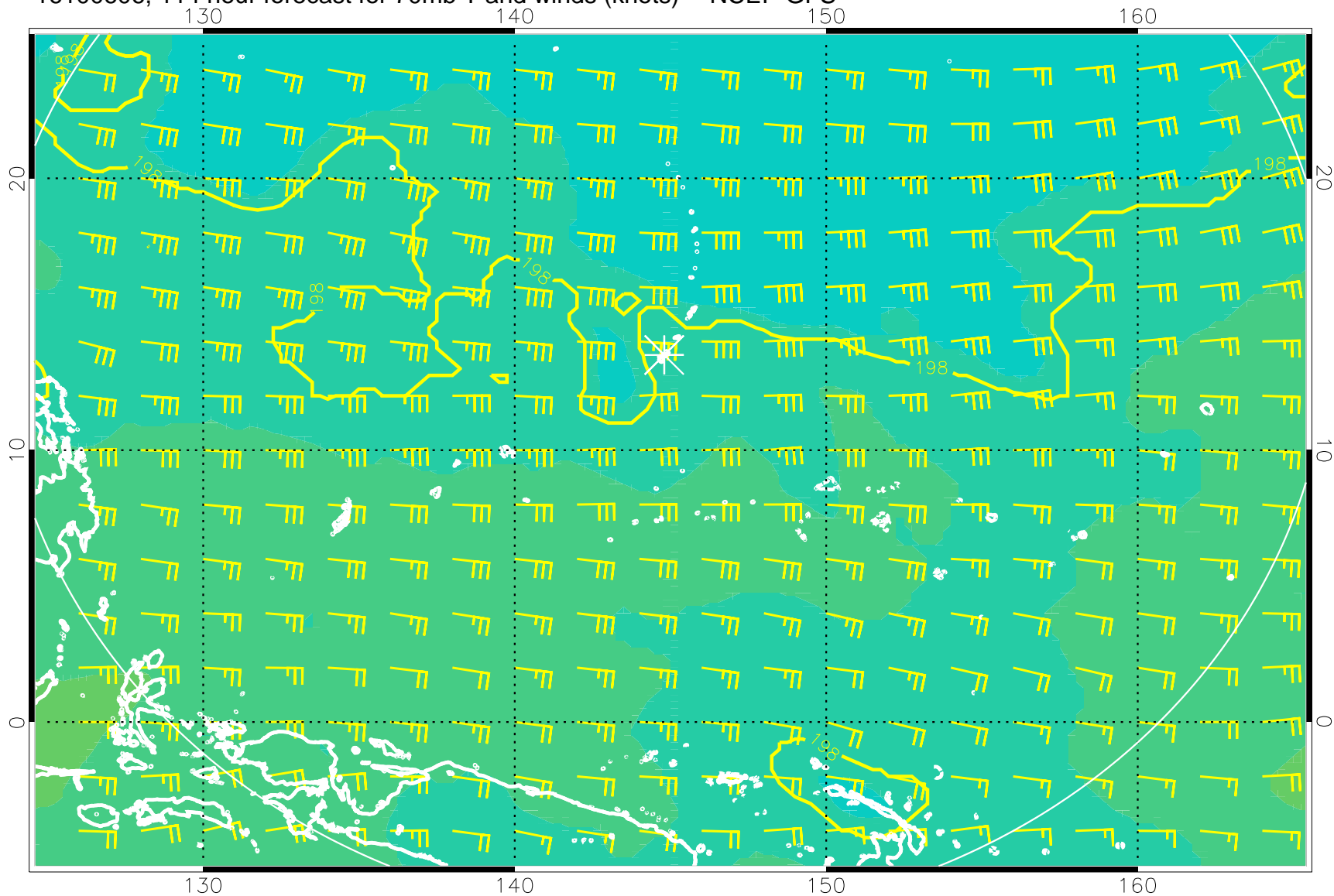
16100606, 114 hour forecast for 70mb T and winds (knots) -- NCEP GFS
