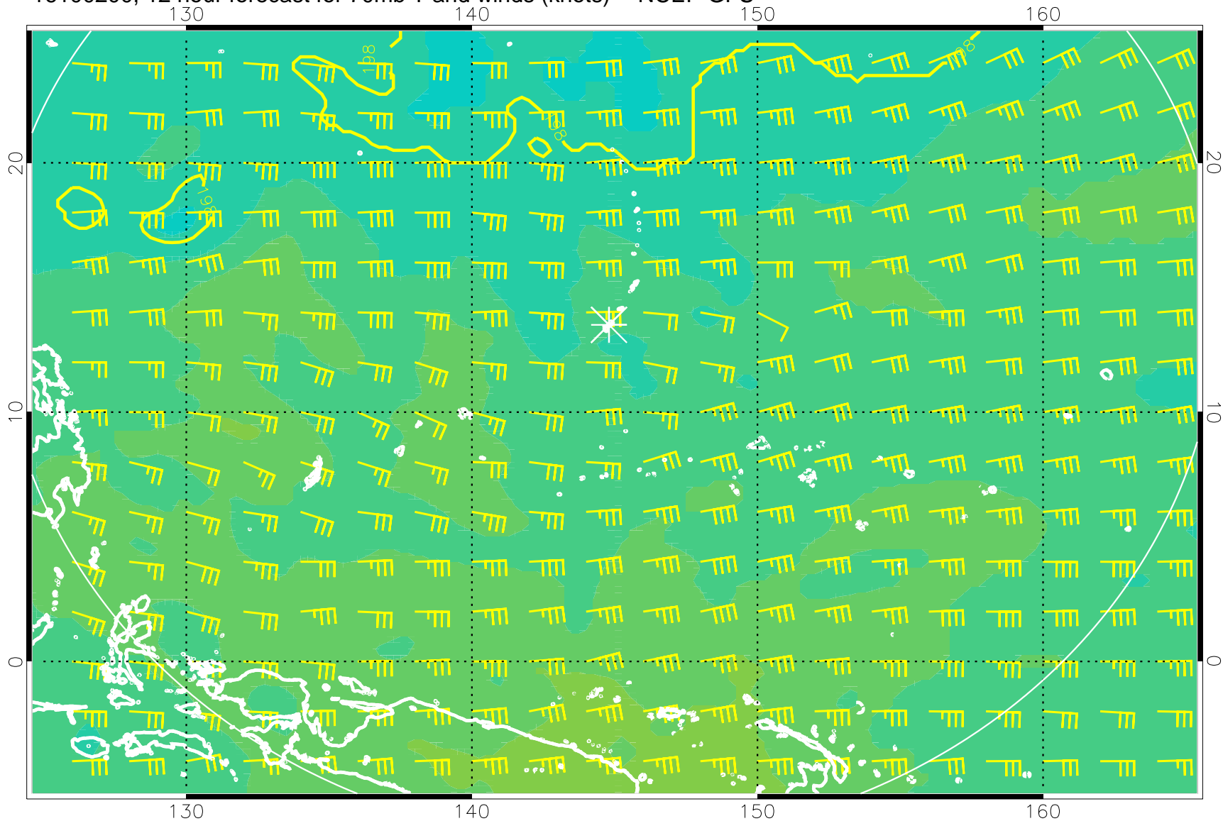
16100200, 12 hour forecast for 70mb T and winds (knots) -- NCEP GFS
