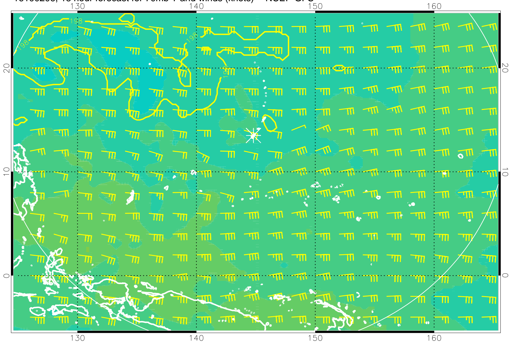
16100206, 18 hour forecast for 70mb T and winds (knots) -- NCEP GFS
