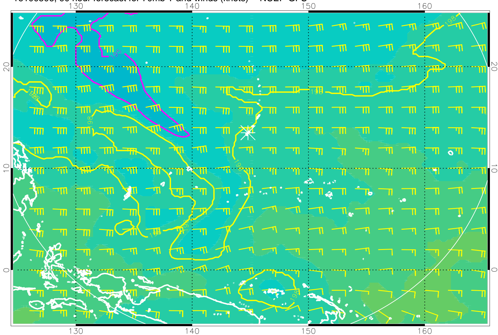
16100506, 90 hour forecast for 70mb T and winds (knots) -- NCEP GFS
