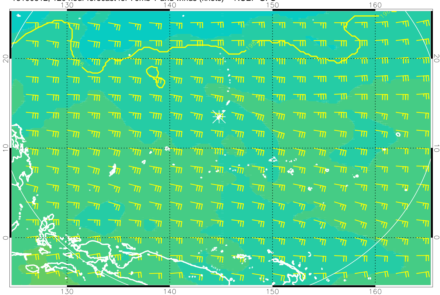
16100612, 120 hour forecast for 70mb T and winds (knots) -- NCEP GFS
