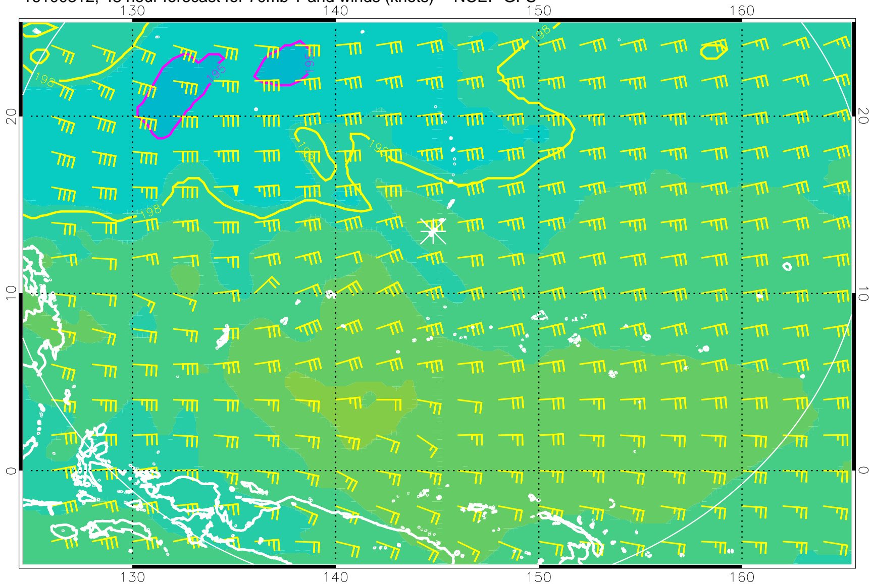
16100312, 48 hour forecast for 70mb T and winds (knots) -- NCEP GFS
