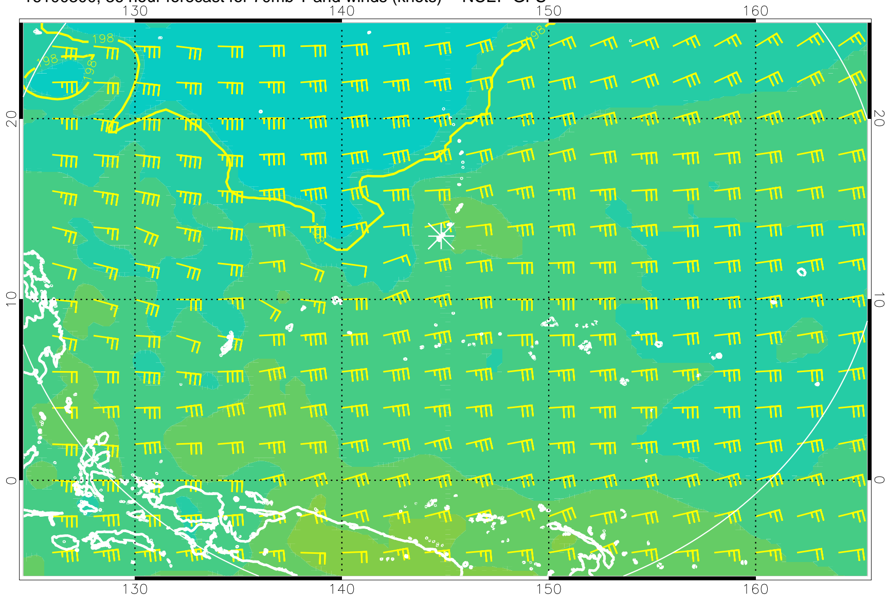
16100300, 36 hour forecast for 70mb T and winds (knots) -- NCEP GFS
