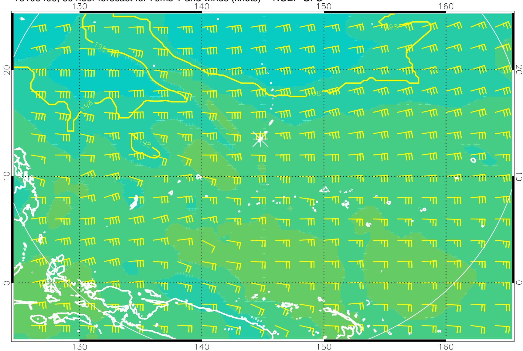
16100400, 60 hour forecast for 70mb T and winds (knots) -- NCEP GFS
