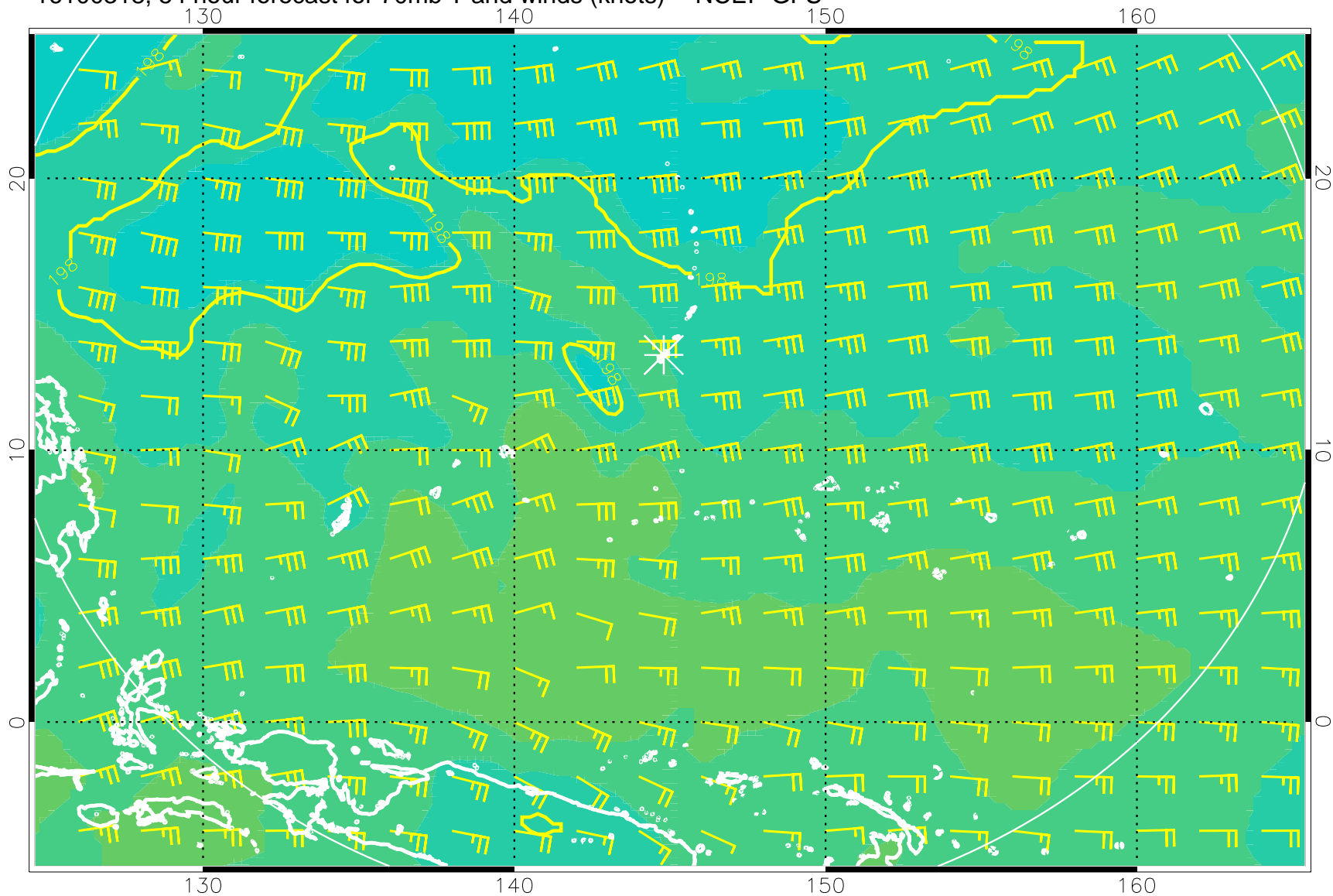
16100318, 54 hour forecast for 70mb T and winds (knots) -- NCEP GFS
