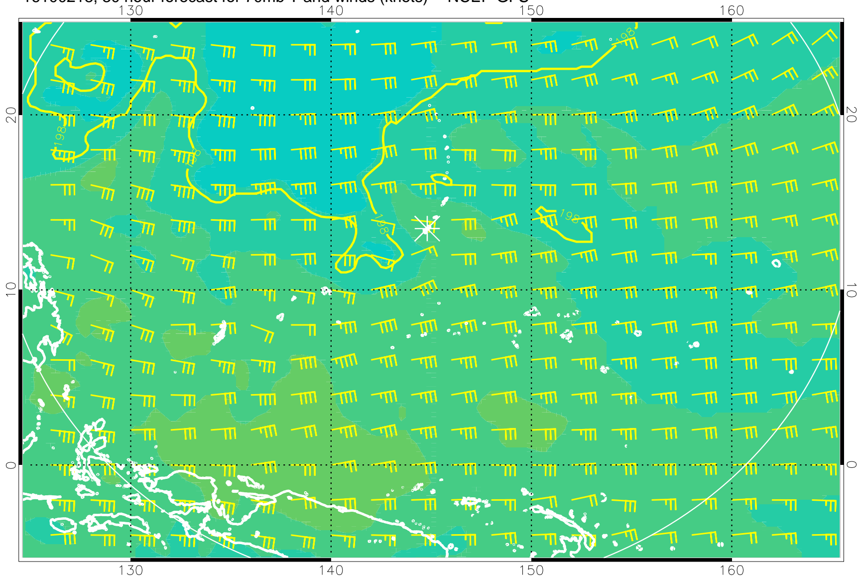
16100218, 30 hour forecast for 70mb T and winds (knots) -- NCEP GFS
