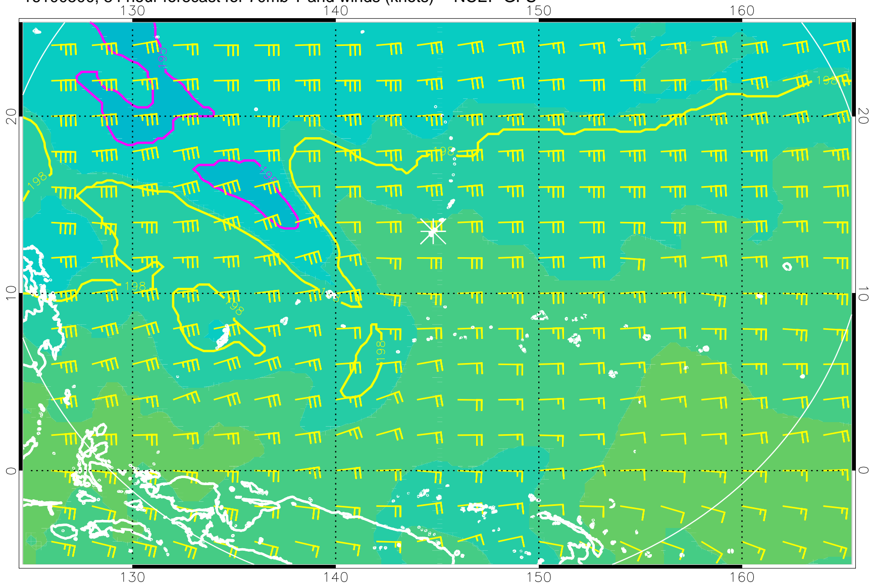
16100500, 84 hour forecast for 70mb T and winds (knots) -- NCEP GFS
