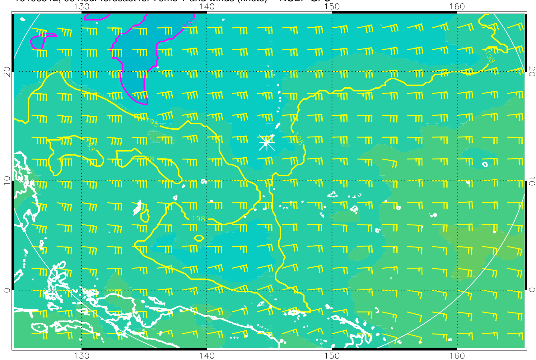
16100512, 96 hour forecast for 70mb T and winds (knots) -- NCEP GFS
