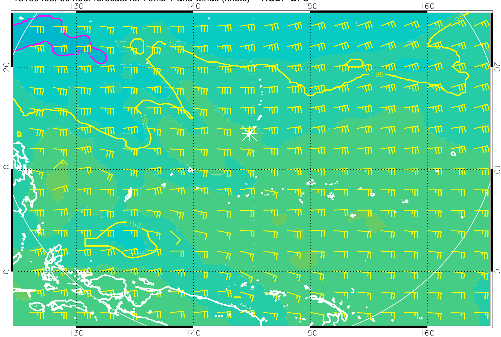
16100406, 66 hour forecast for 70mb T and winds (knots) -- NCEP GFS
