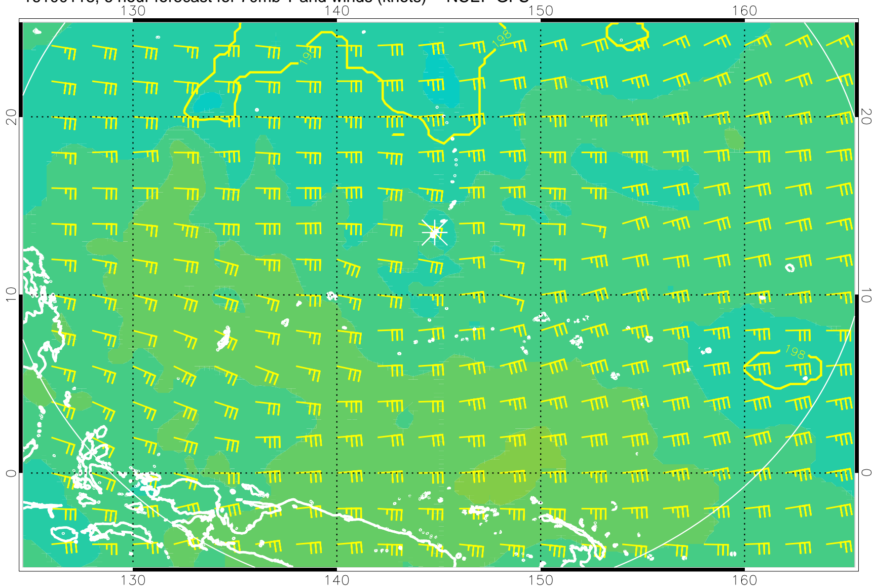
16100118, 6 hour forecast for 70mb T and winds (knots) -- NCEP GFS
