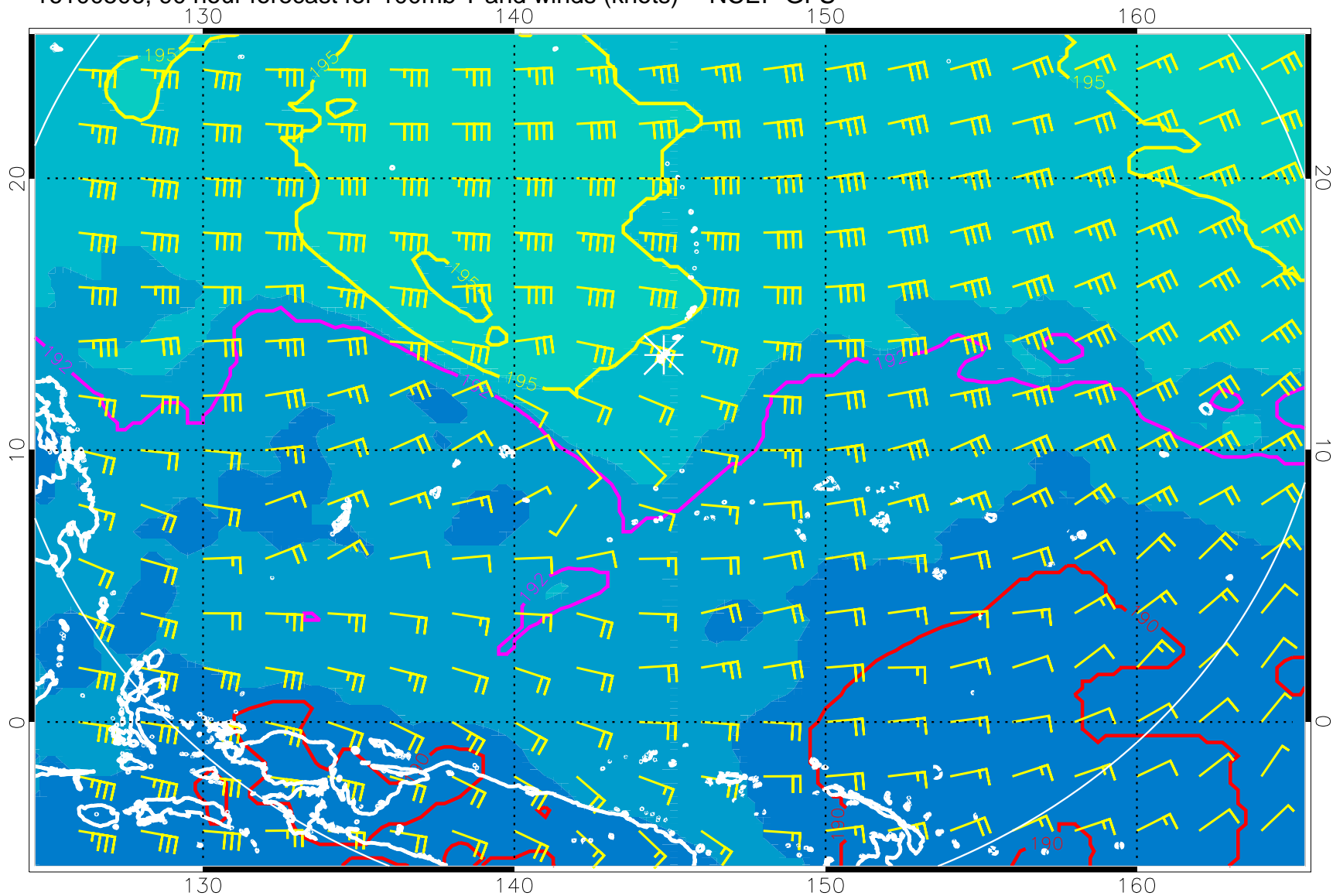
16100506, 90 hour forecast for 100mb T and winds (knots) -- NCEP GFS
