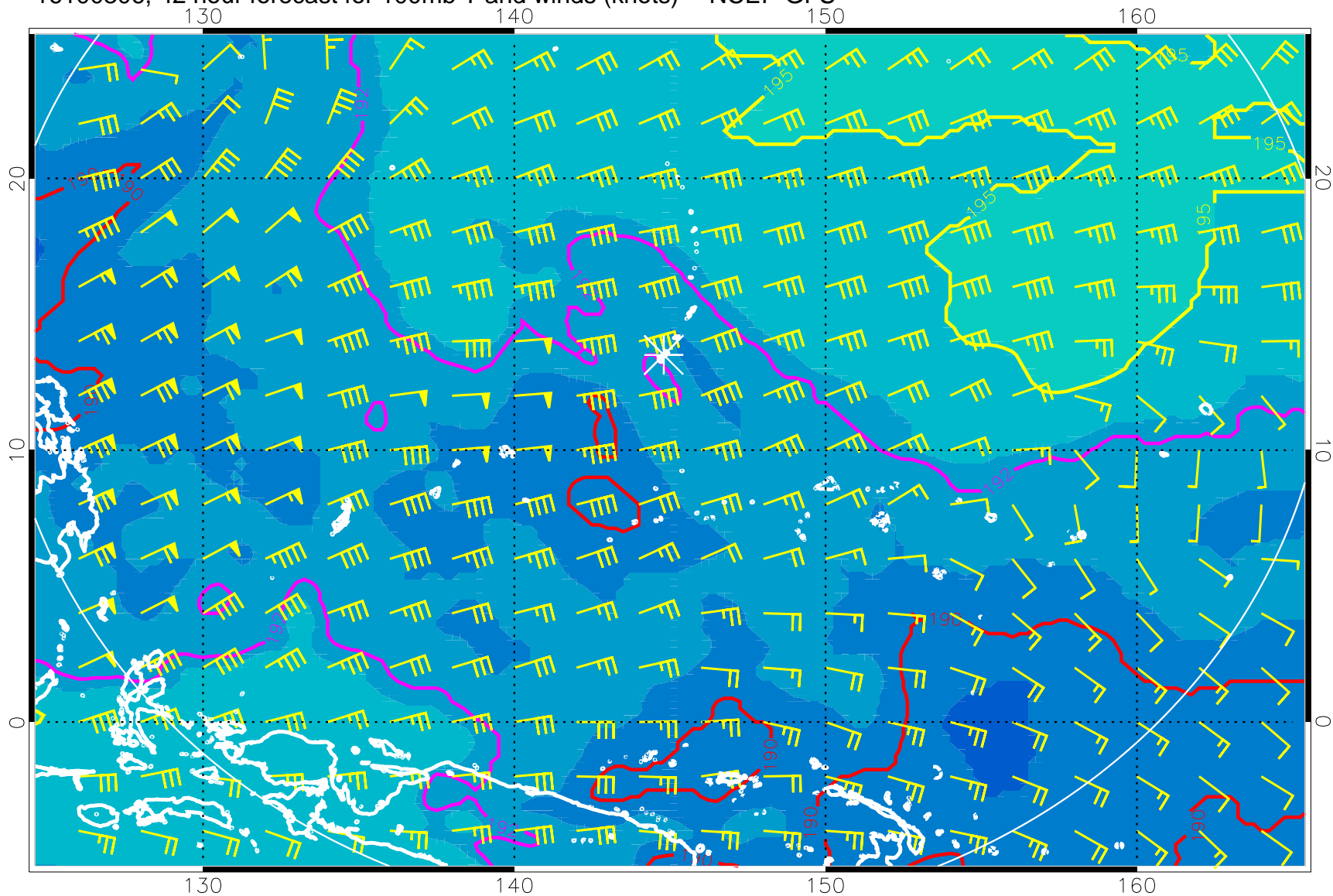
16100306, 42 hour forecast for 100mb T and winds (knots) -- NCEP GFS
