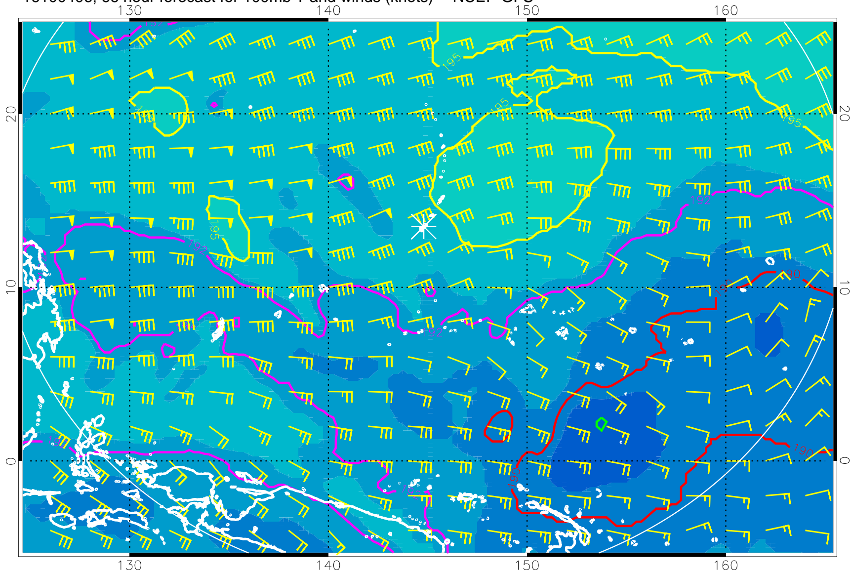
16100406, 66 hour forecast for 100mb T and winds (knots) -- NCEP GFS
