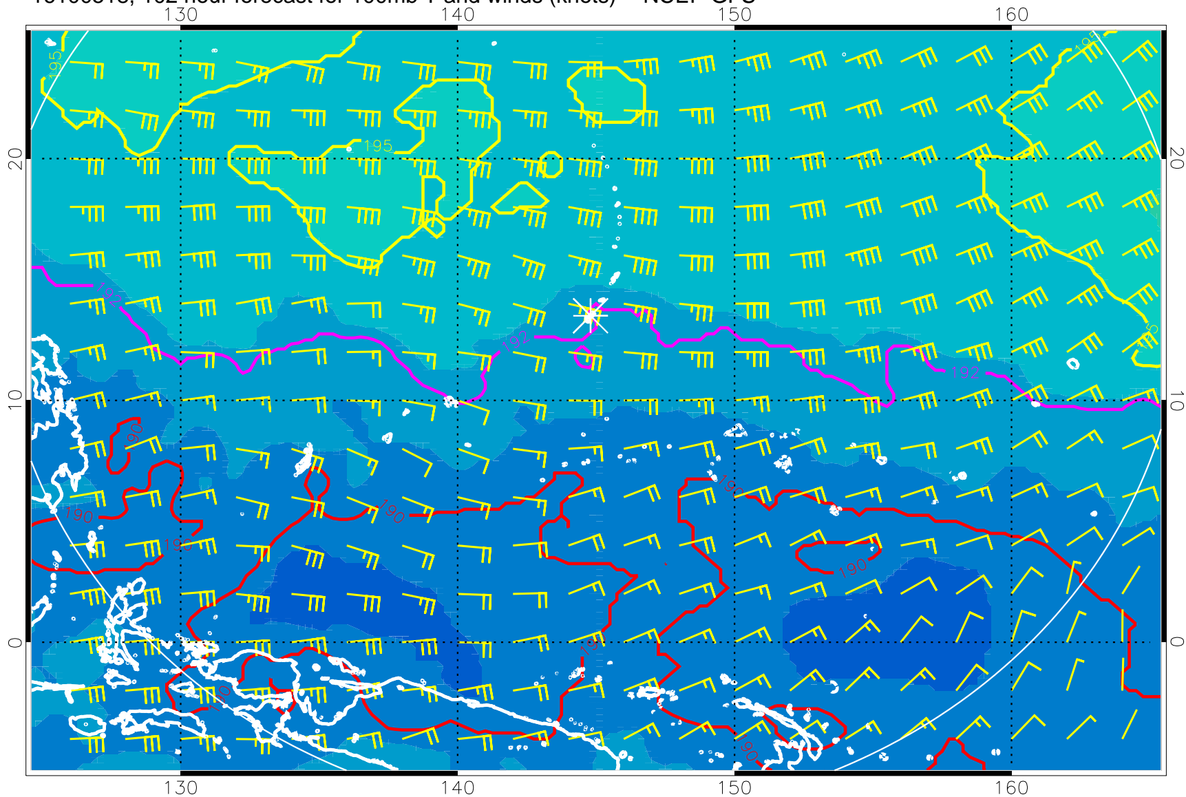
16100518, 102 hour forecast for 100mb T and winds (knots) -- NCEP GFS
