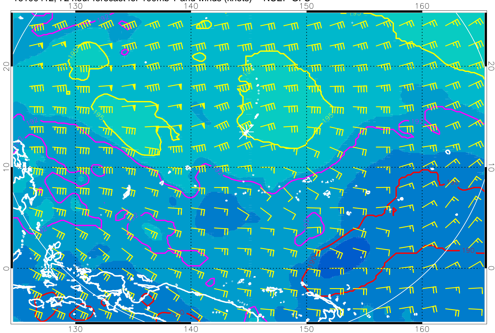
16100412, 72 hour forecast for 100mb T and winds (knots) -- NCEP GFS
