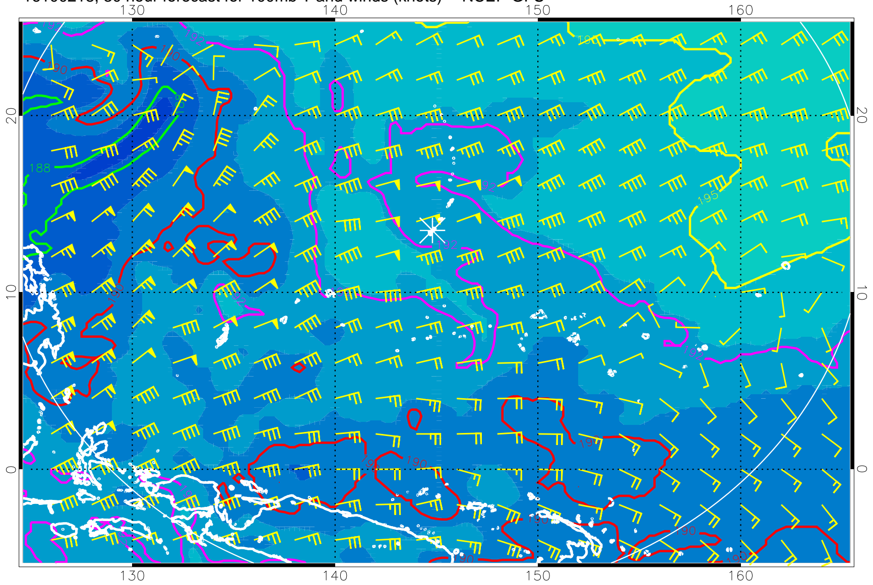
16100218, 30 hour forecast for 100mb T and winds (knots) -- NCEP GFS
