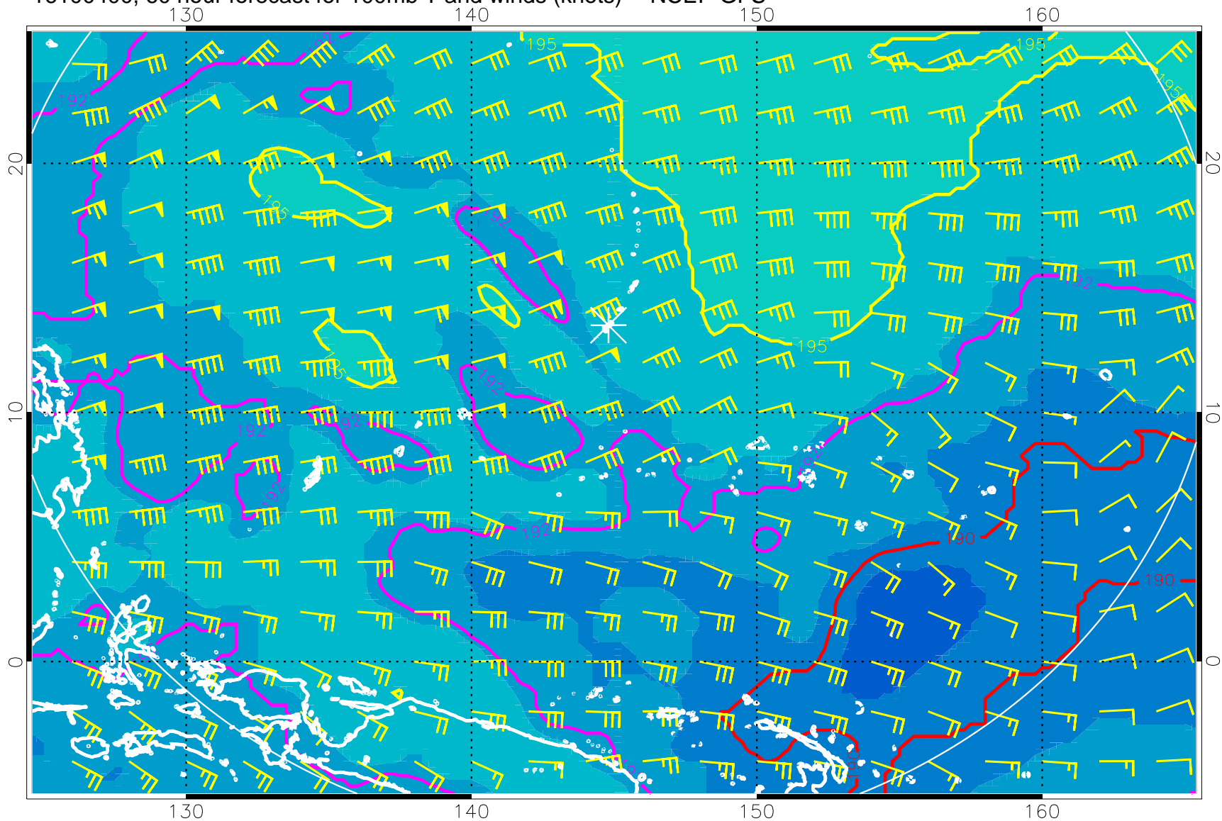
16100400, 60 hour forecast for 100mb T and winds (knots) -- NCEP GFS
