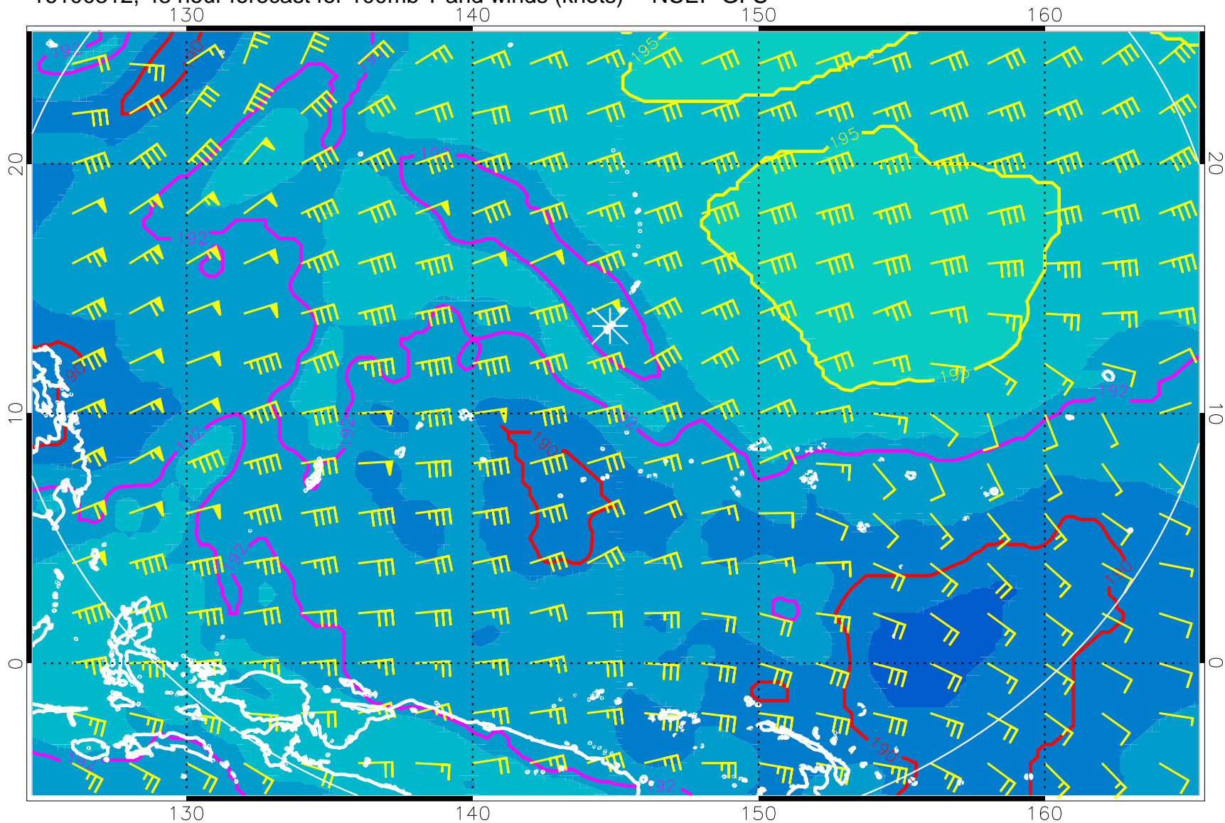
16100312, 48 hour forecast for 100mb T and winds (knots) -- NCEP GFS
