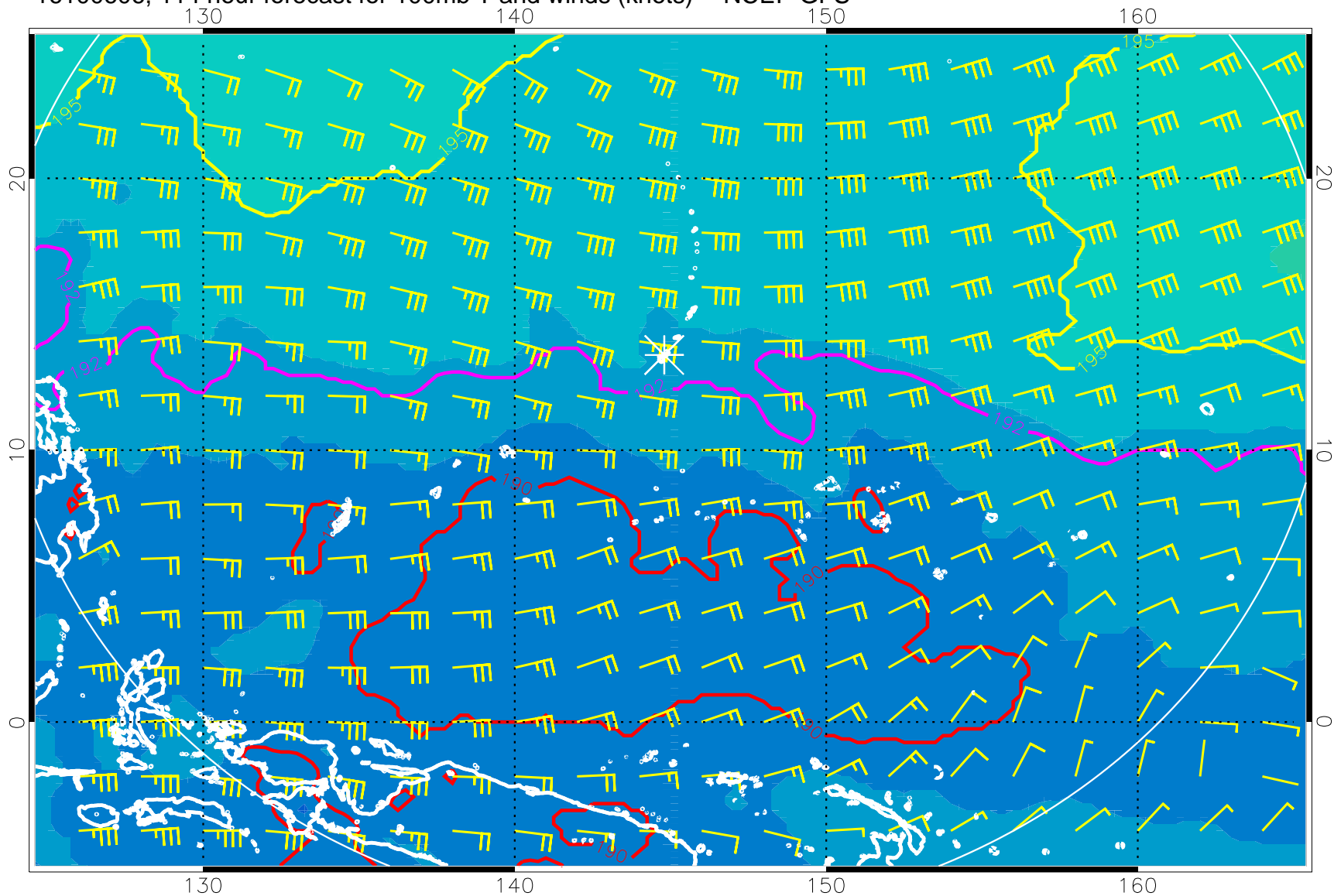
16100606, 114 hour forecast for 100mb T and winds (knots) -- NCEP GFS
