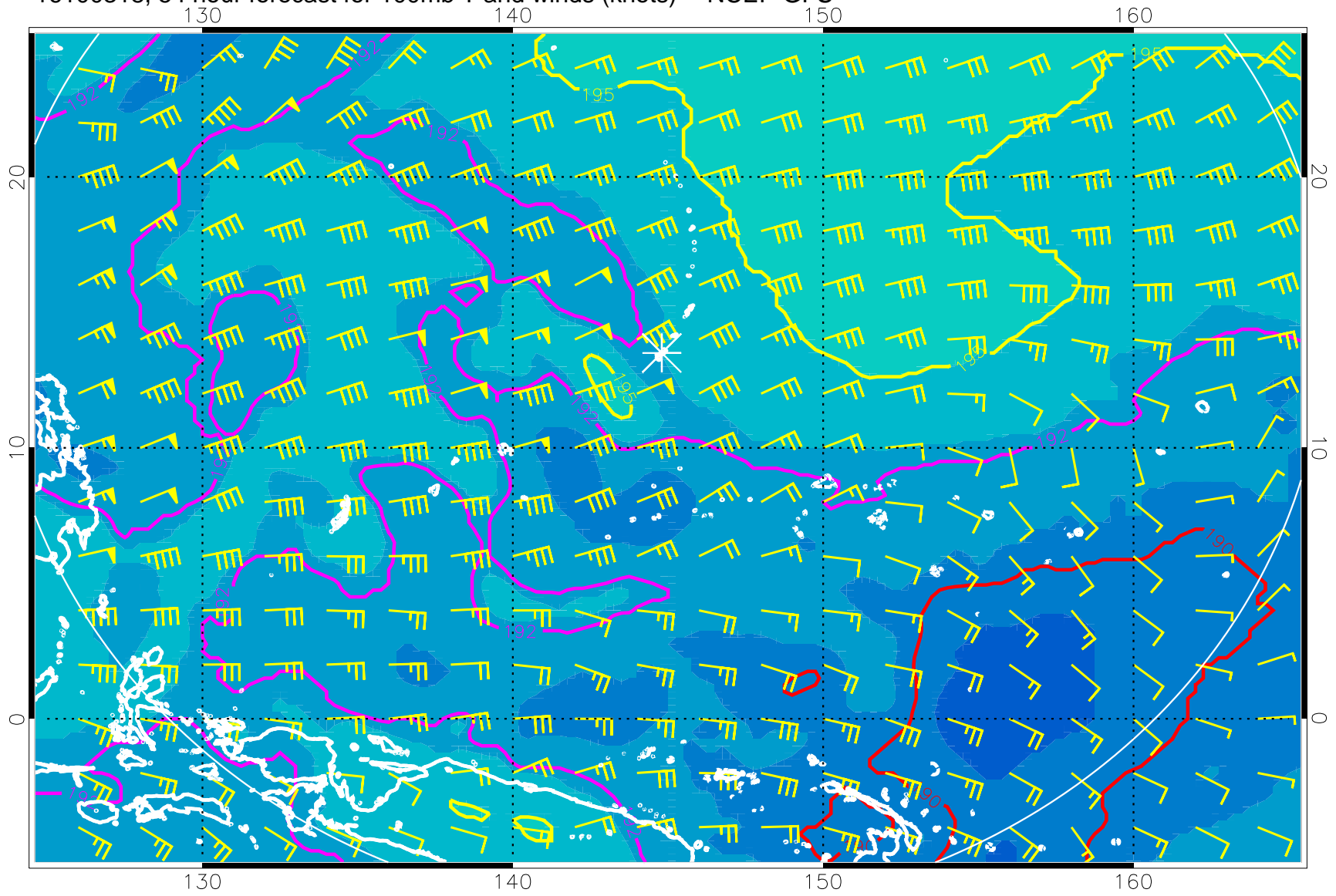
16100318, 54 hour forecast for 100mb T and winds (knots) -- NCEP GFS
