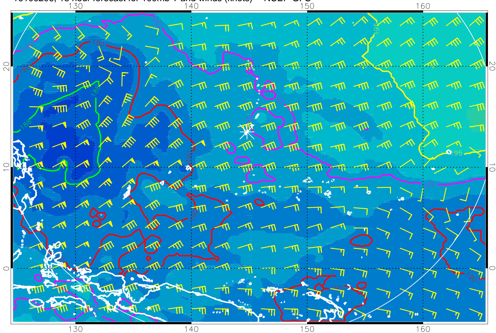
16100206, 18 hour forecast for 100mb T and winds (knots) -- NCEP GFS
