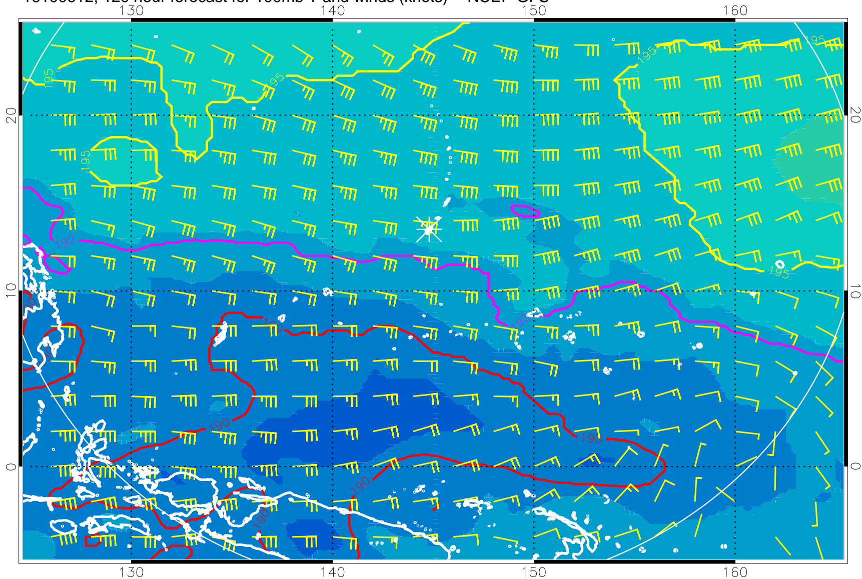
16100612, 120 hour forecast for 100mb T and winds (knots) -- NCEP GFS
