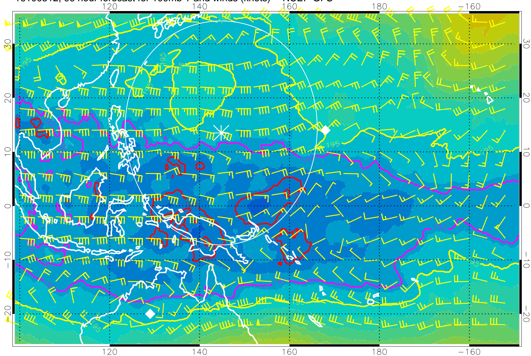
16100512, 96 hour forecast for 100mb T and winds (knots) -- NCEP GFS
