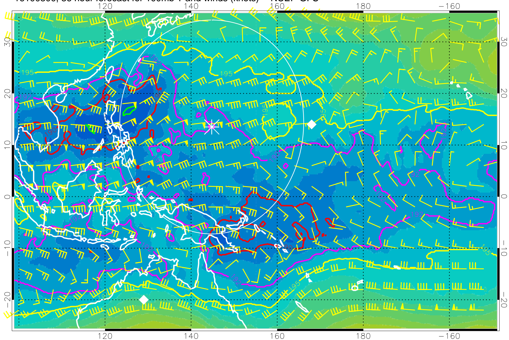
16100300, 36 hour forecast for 100mb T and winds (knots) -- NCEP GFS
