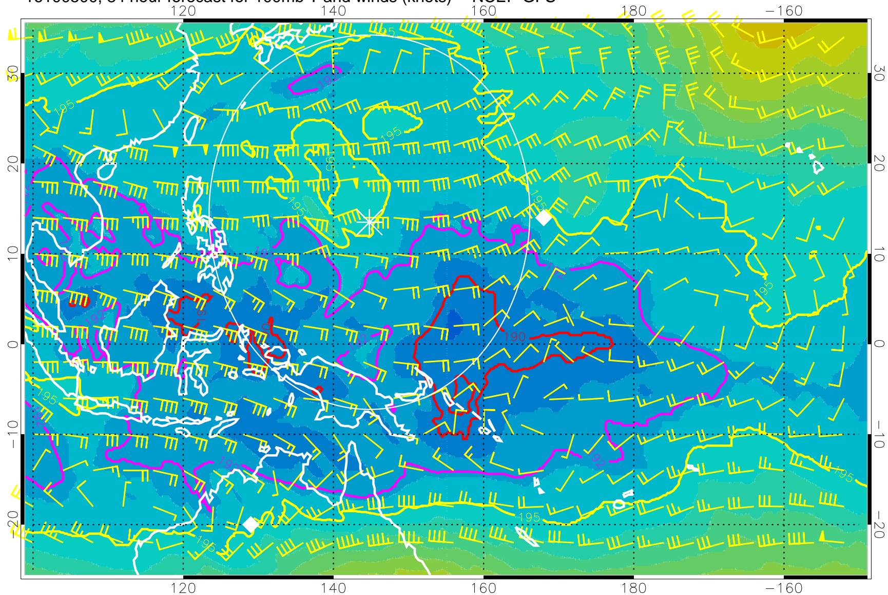
16100500, 84 hour forecast for 100mb T and winds (knots) -- NCEP GFS
