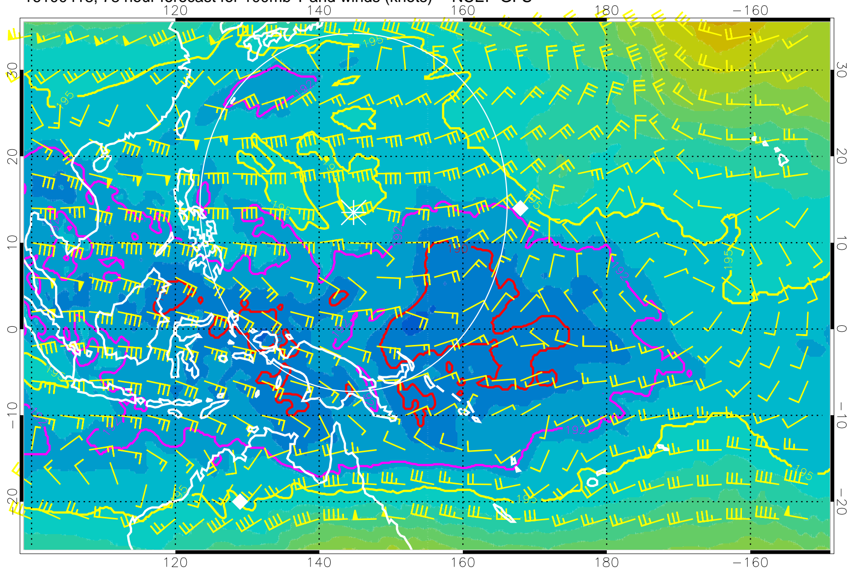
16100418, 78 hour forecast for 100mb T and winds (knots) -- NCEP GFS
