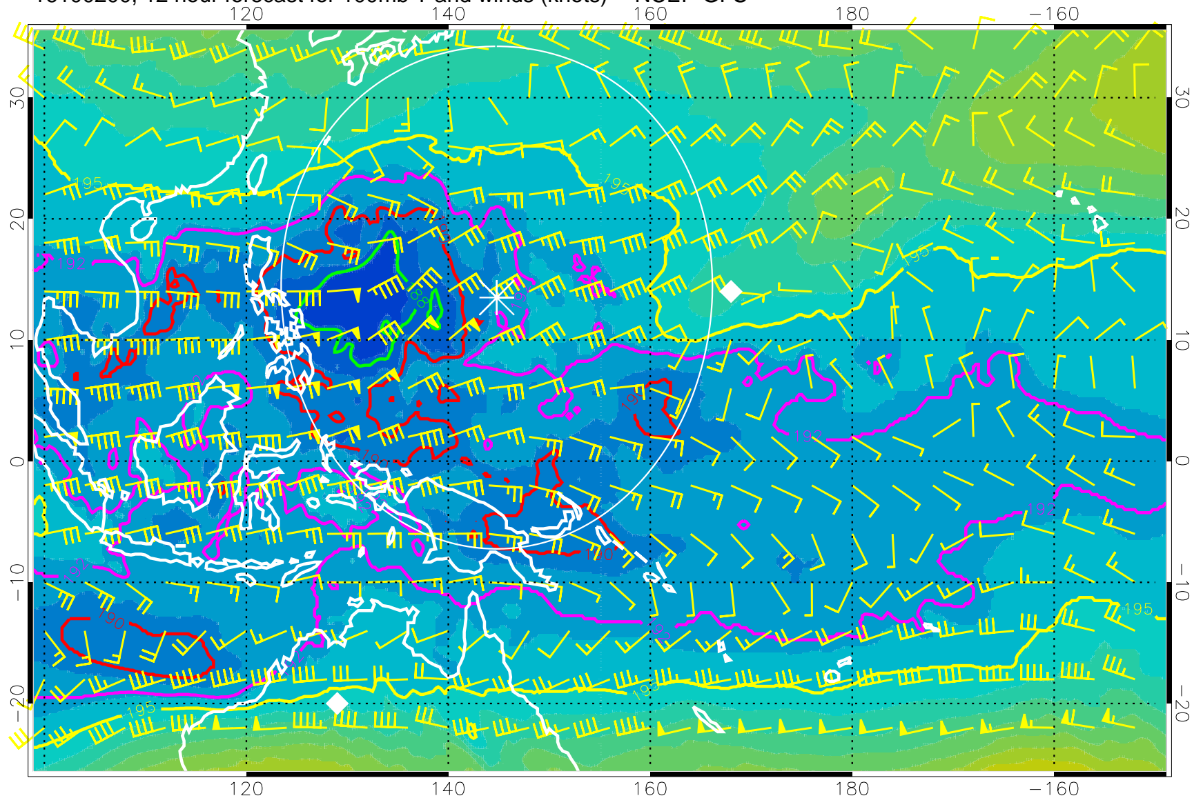
16100200, 12 hour forecast for 100mb T and winds (knots) -- NCEP GFS
