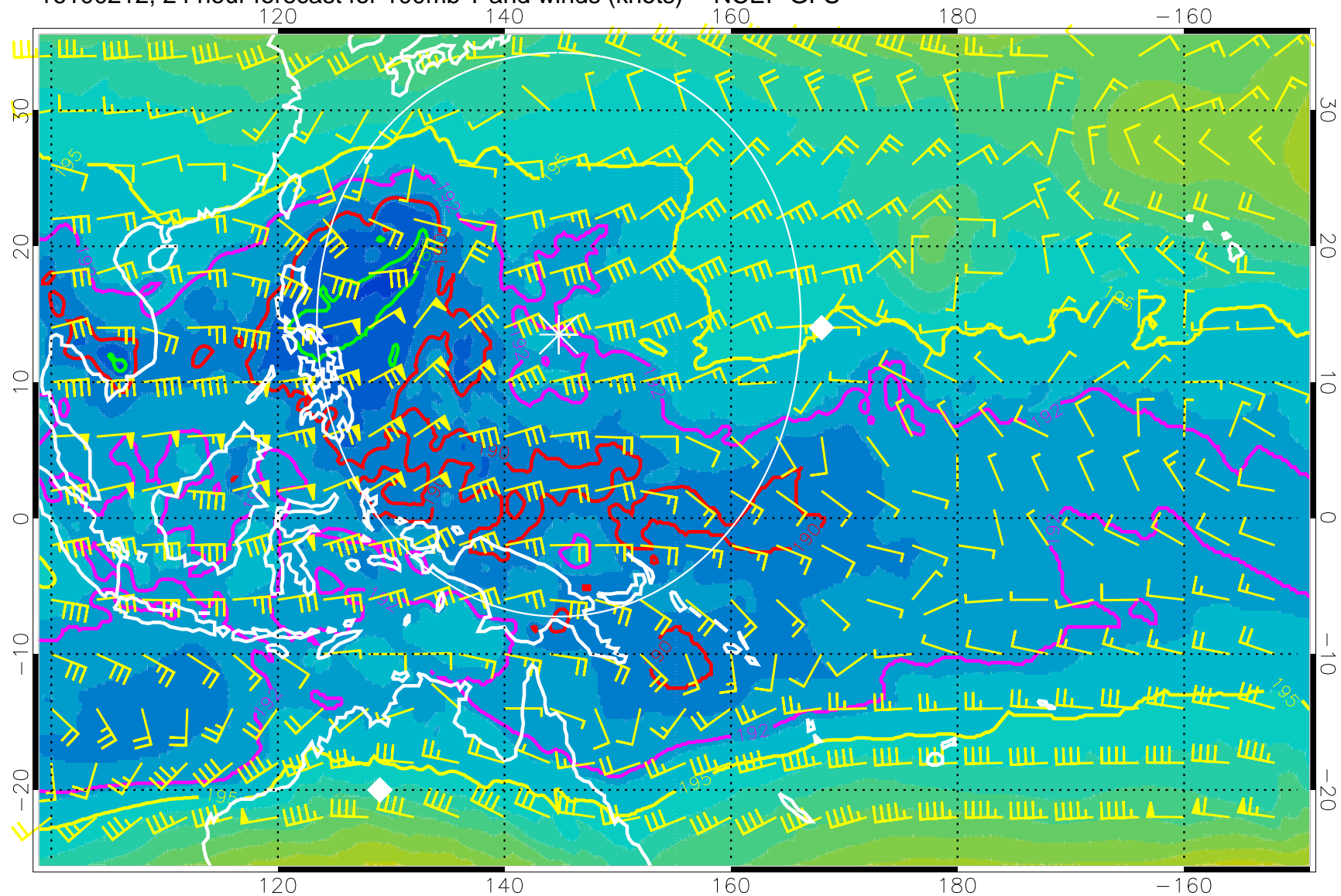
16100212, 24 hour forecast for 100mb T and winds (knots) -- NCEP GFS
