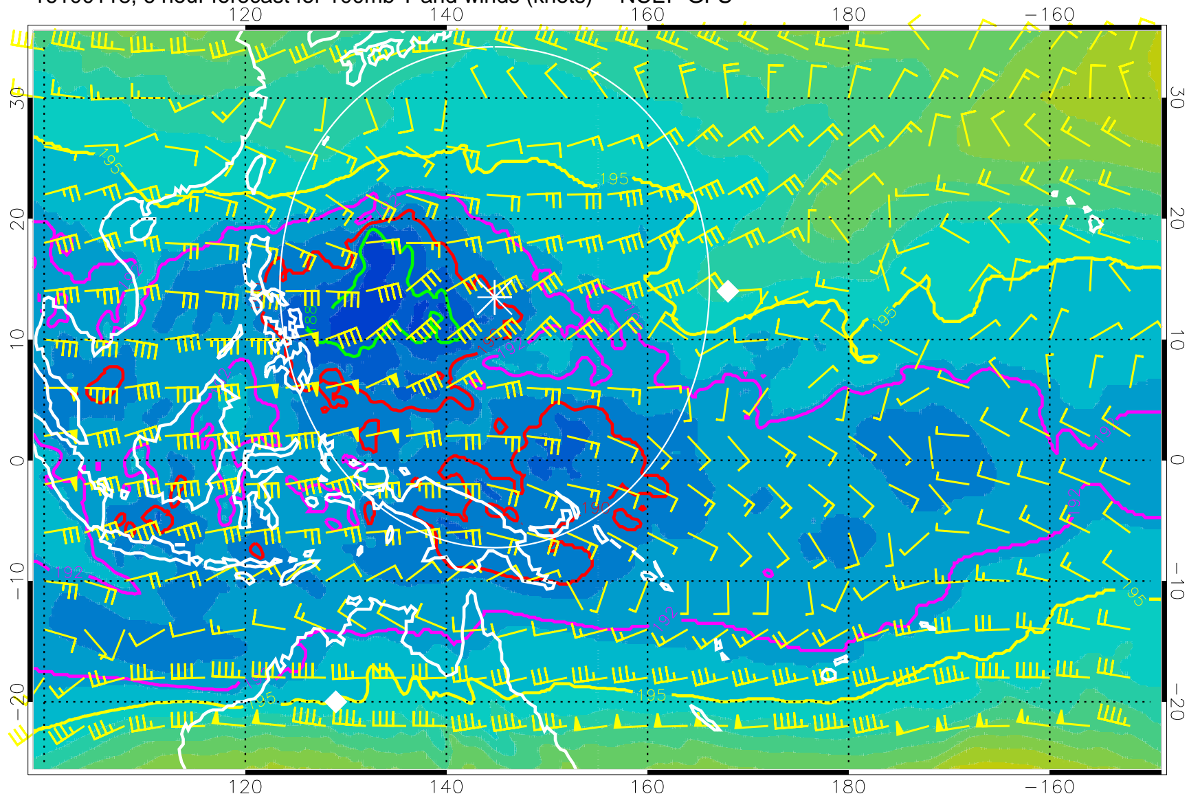
16100118, 6 hour forecast for 100mb T and winds (knots) -- NCEP GFS
