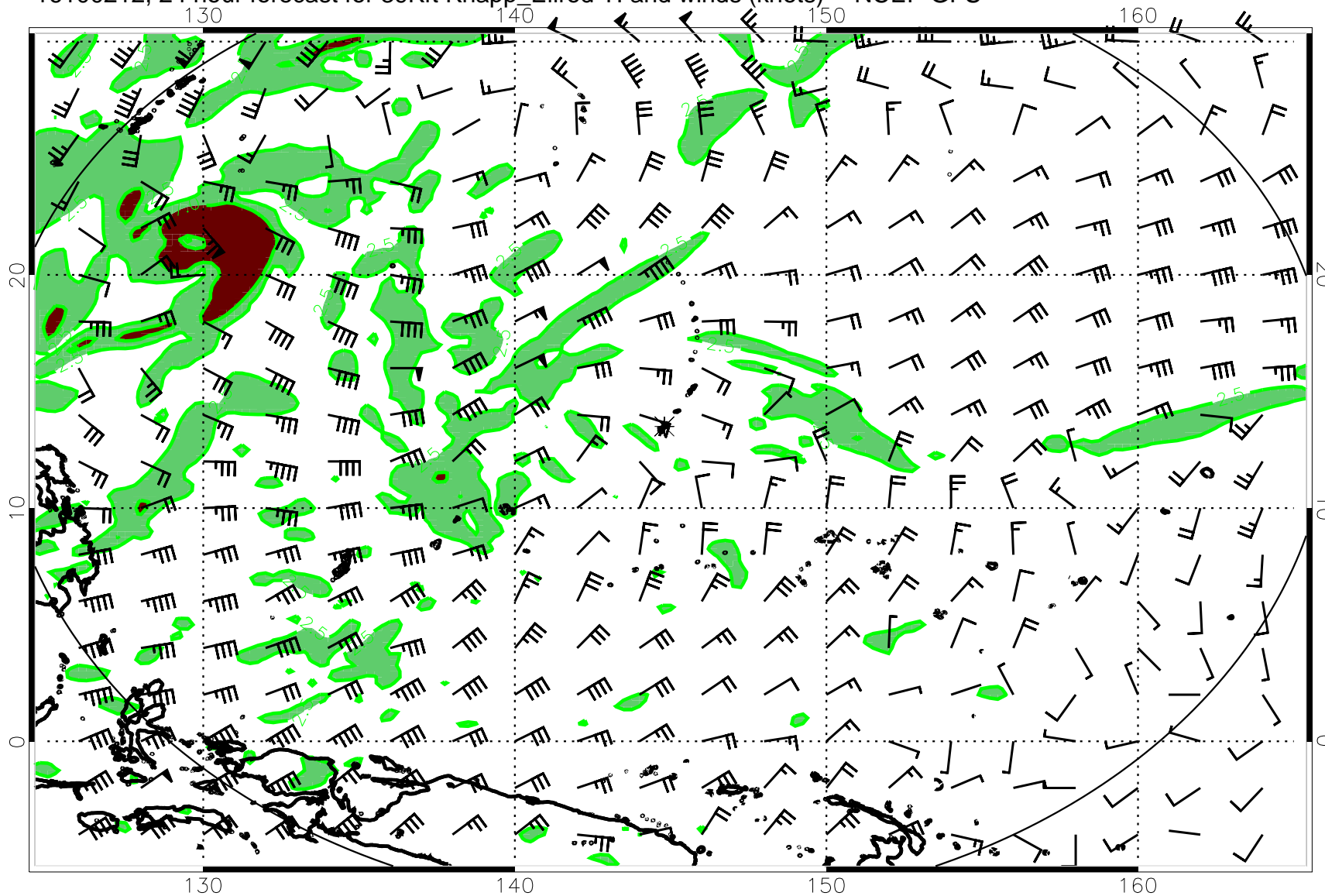
16100212, 24 hour forecast for 39Kft Knapp_Ellrod TI and winds (knots) -- NCEP GFS
