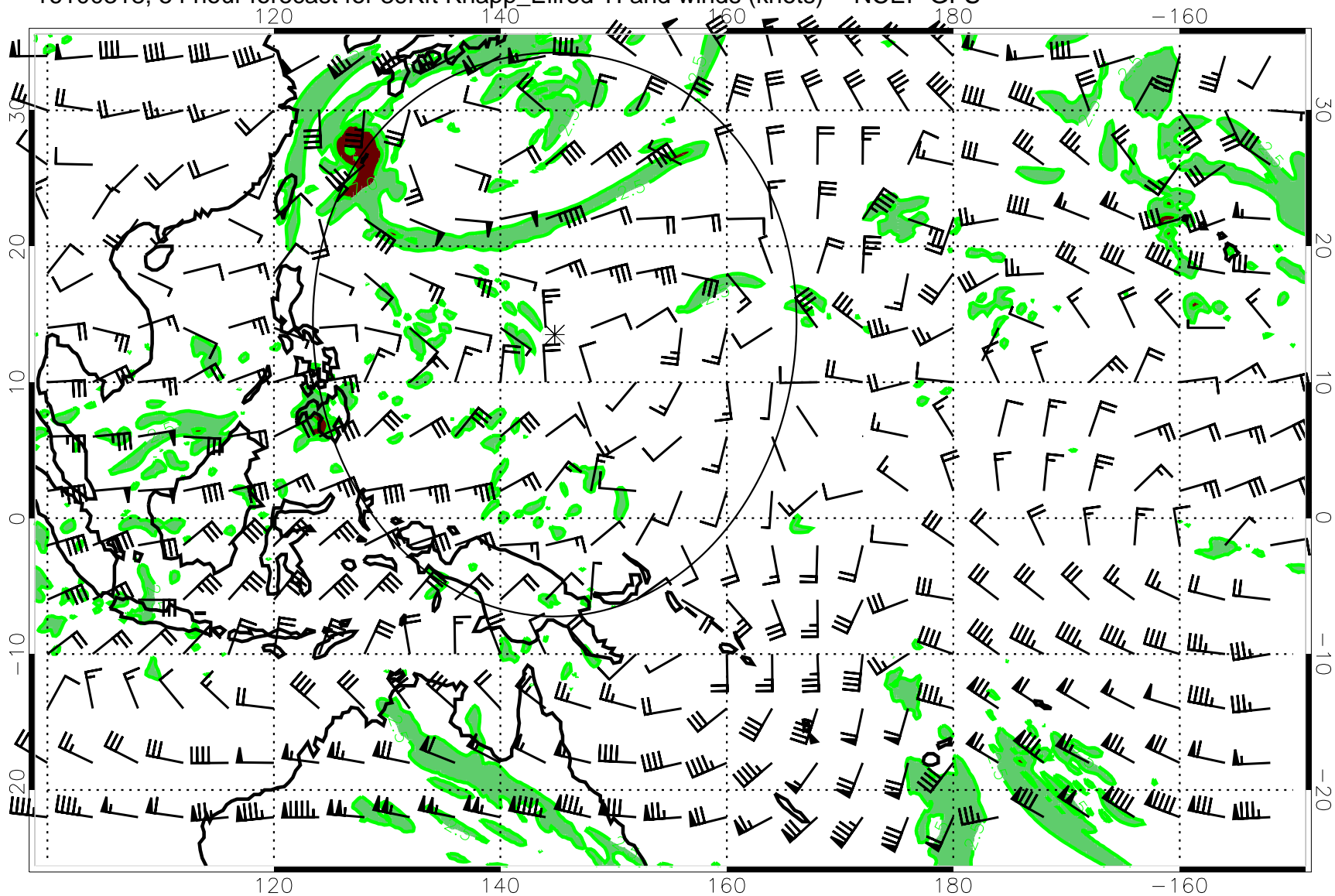
16100318, 54 hour forecast for 39Kft Knapp_Ellrod TI and winds (knots) -- NCEP GFS
