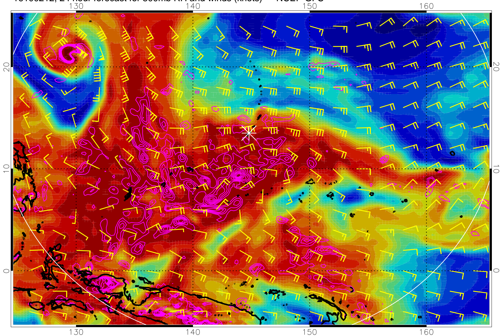
16100212, 24 hour forecast for 500mb RH and winds (knots) -- NCEP GFS
