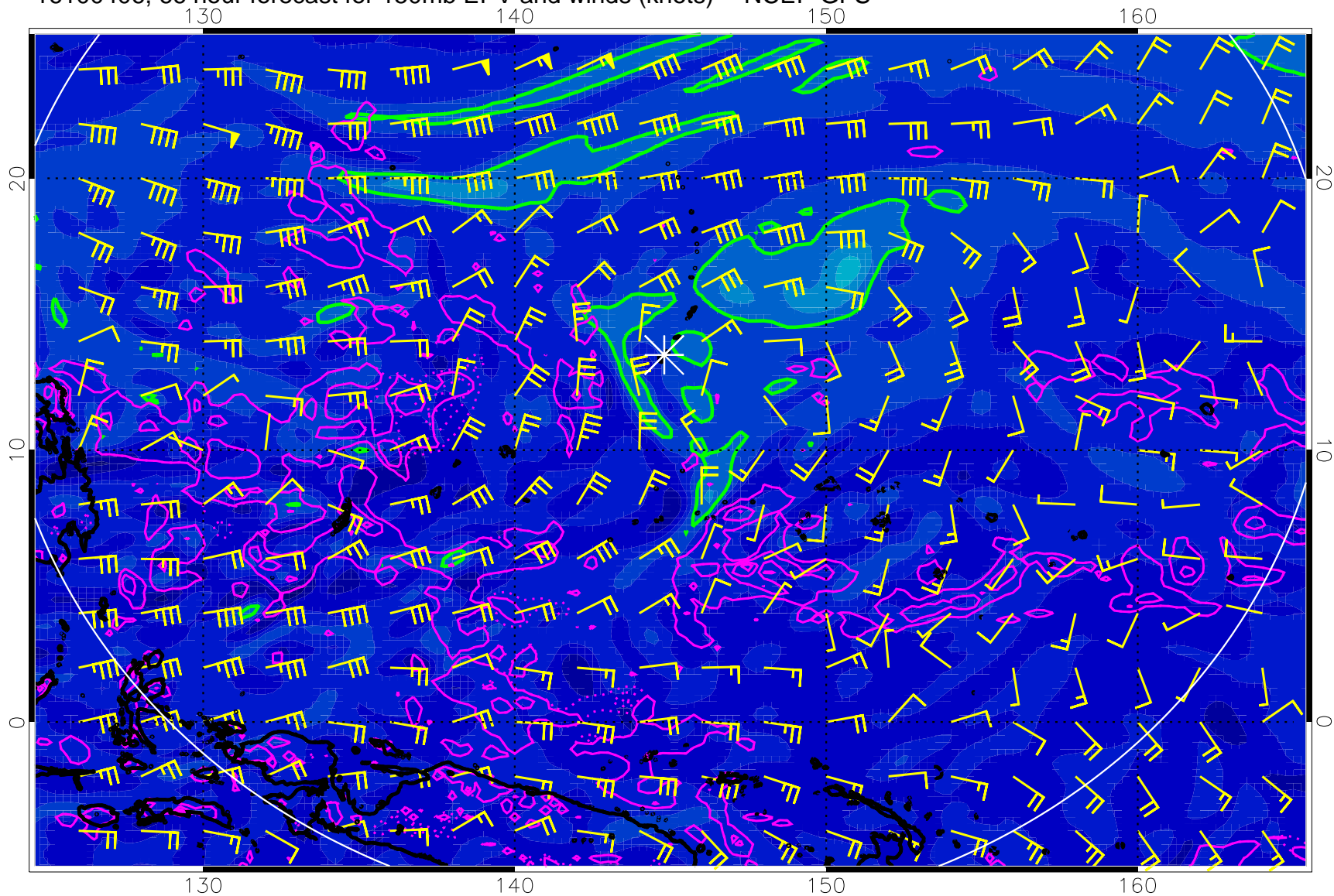
16100406, 66 hour forecast for 150mb EPV and winds (knots) -- NCEP GFS
