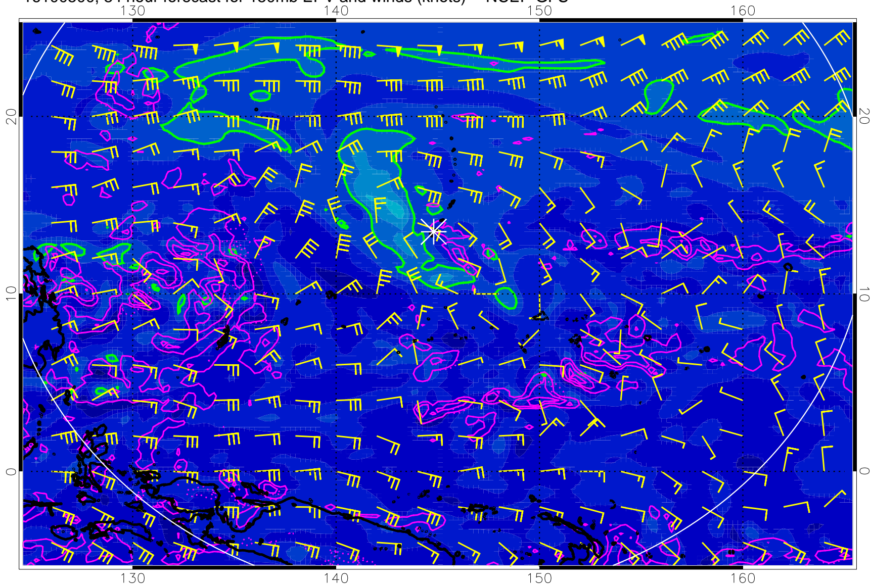
16100500, 84 hour forecast for 150mb EPV and winds (knots) -- NCEP GFS
