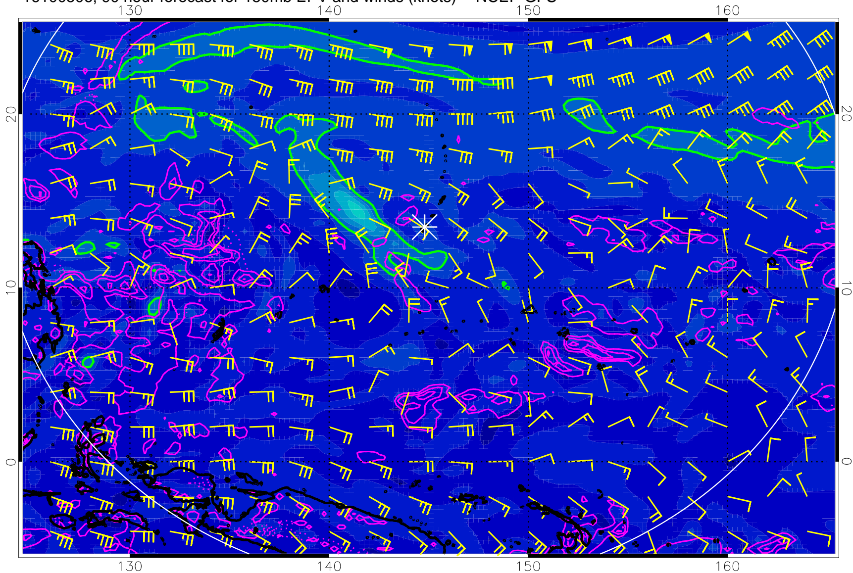
16100506, 90 hour forecast for 150mb EPV and winds (knots) -- NCEP GFS
