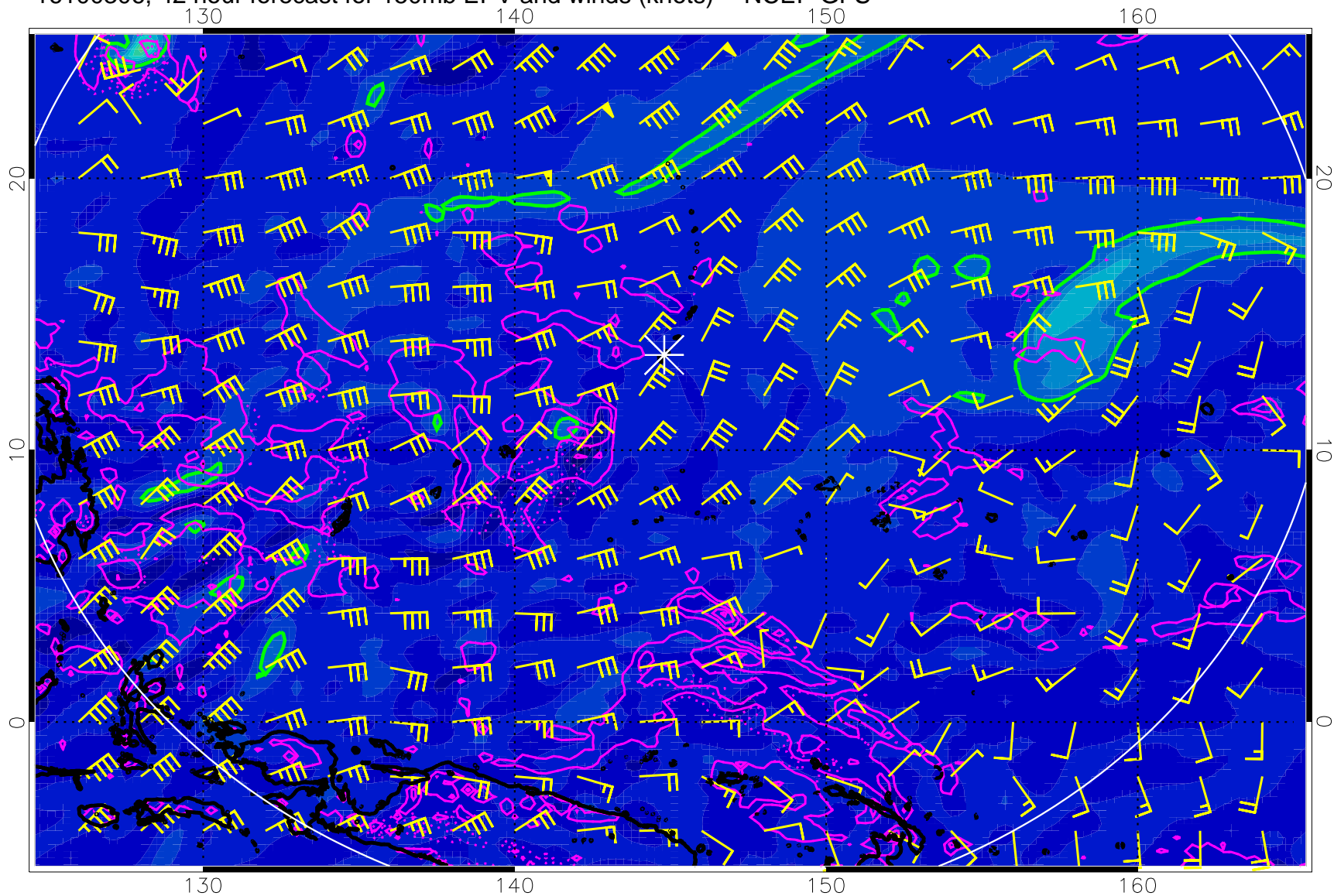
16100306, 42 hour forecast for 150mb EPV and winds (knots) -- NCEP GFS
