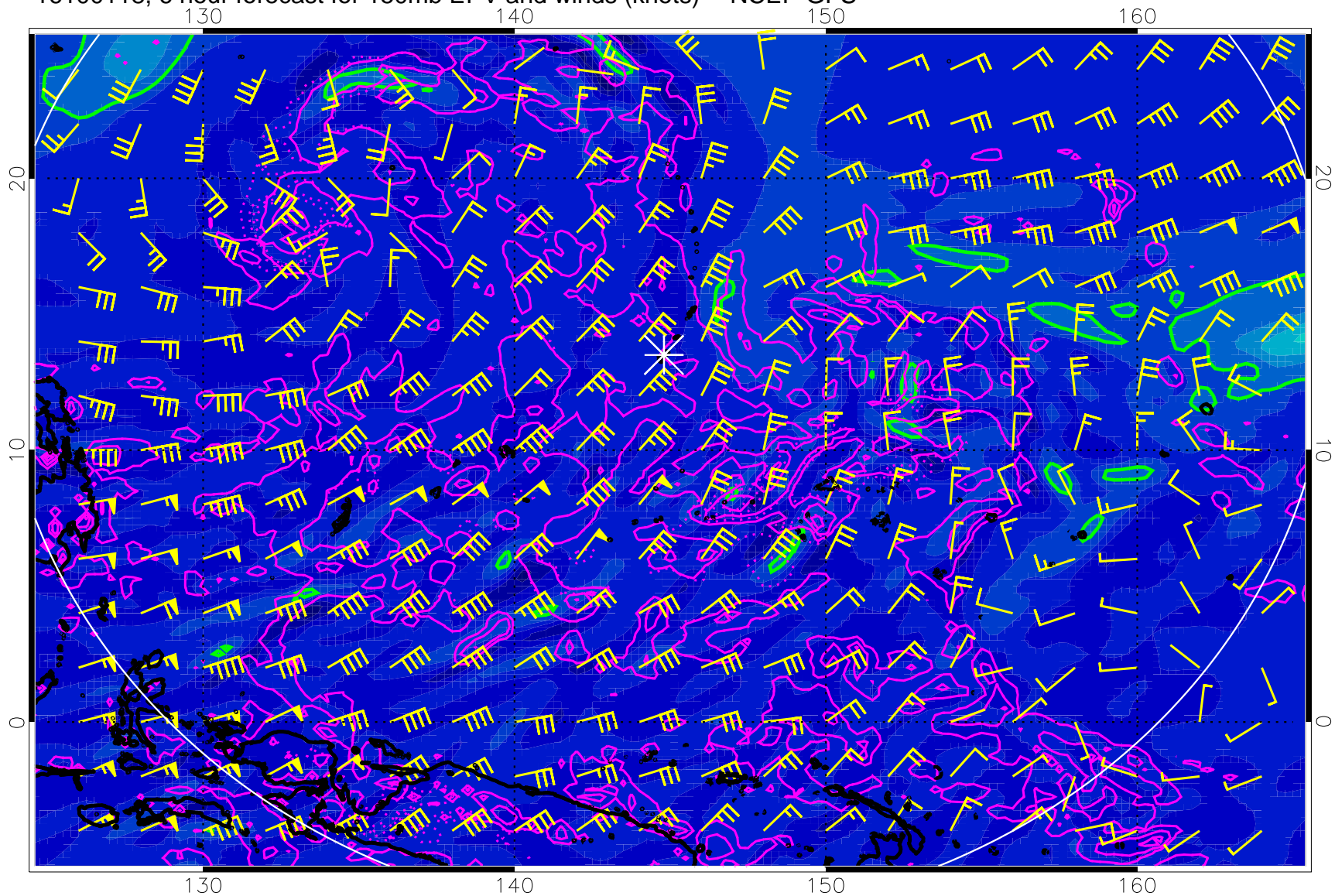
16100118, 6 hour forecast for 150mb EPV and winds (knots) -- NCEP GFS
