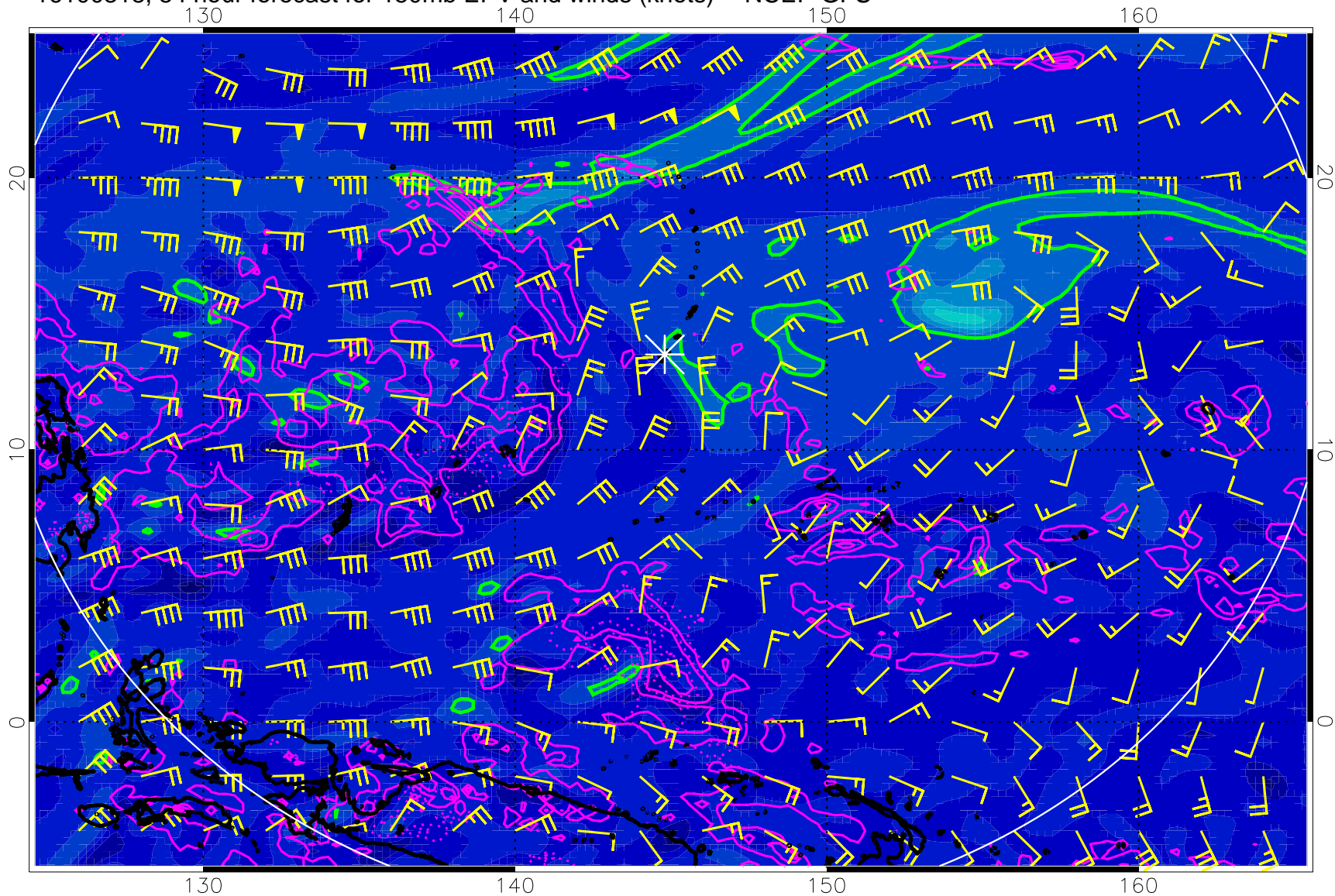
16100318, 54 hour forecast for 150mb EPV and winds (knots) -- NCEP GFS
