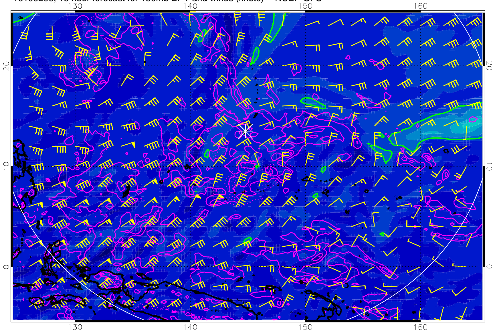
16100206, 18 hour forecast for 150mb EPV and winds (knots) -- NCEP GFS
