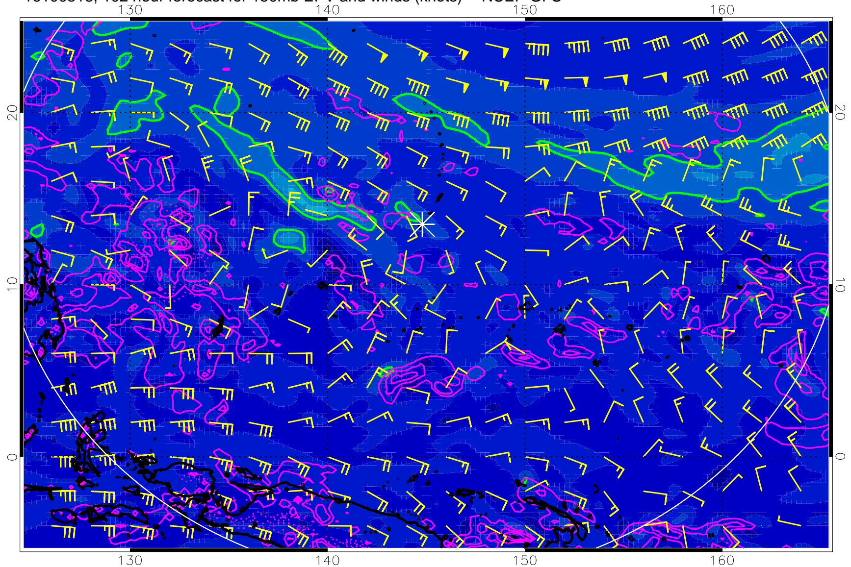
16100518, 102 hour forecast for 150mb EPV and winds (knots) -- NCEP GFS
