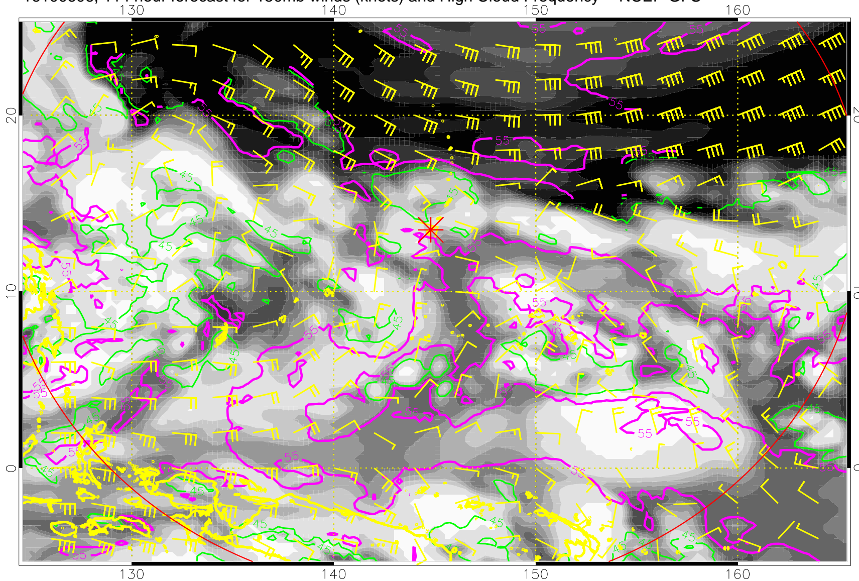
16100606, 114 hour forecast for 150mb winds (knots) and High Cloud Frequency -- NCEP GFS
