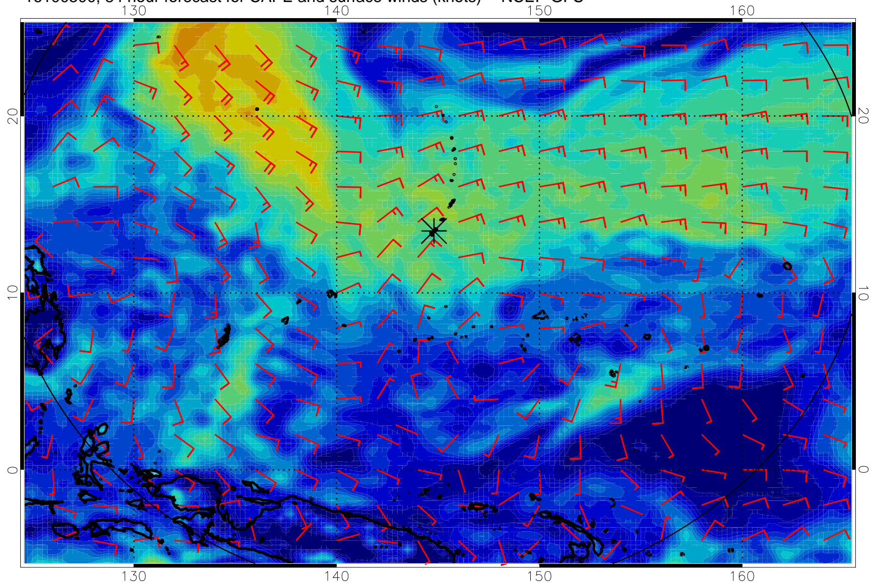
16100500, 84 hour forecast for CAPE and surface winds (knots) -- NCEP GFS
