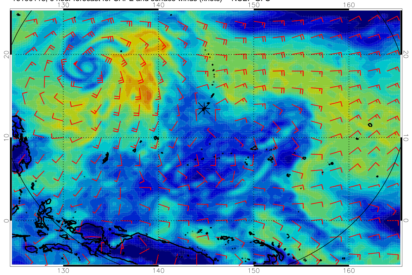
16100118, 6 hour forecast for CAPE and surface winds (knots) -- NCEP GFS
