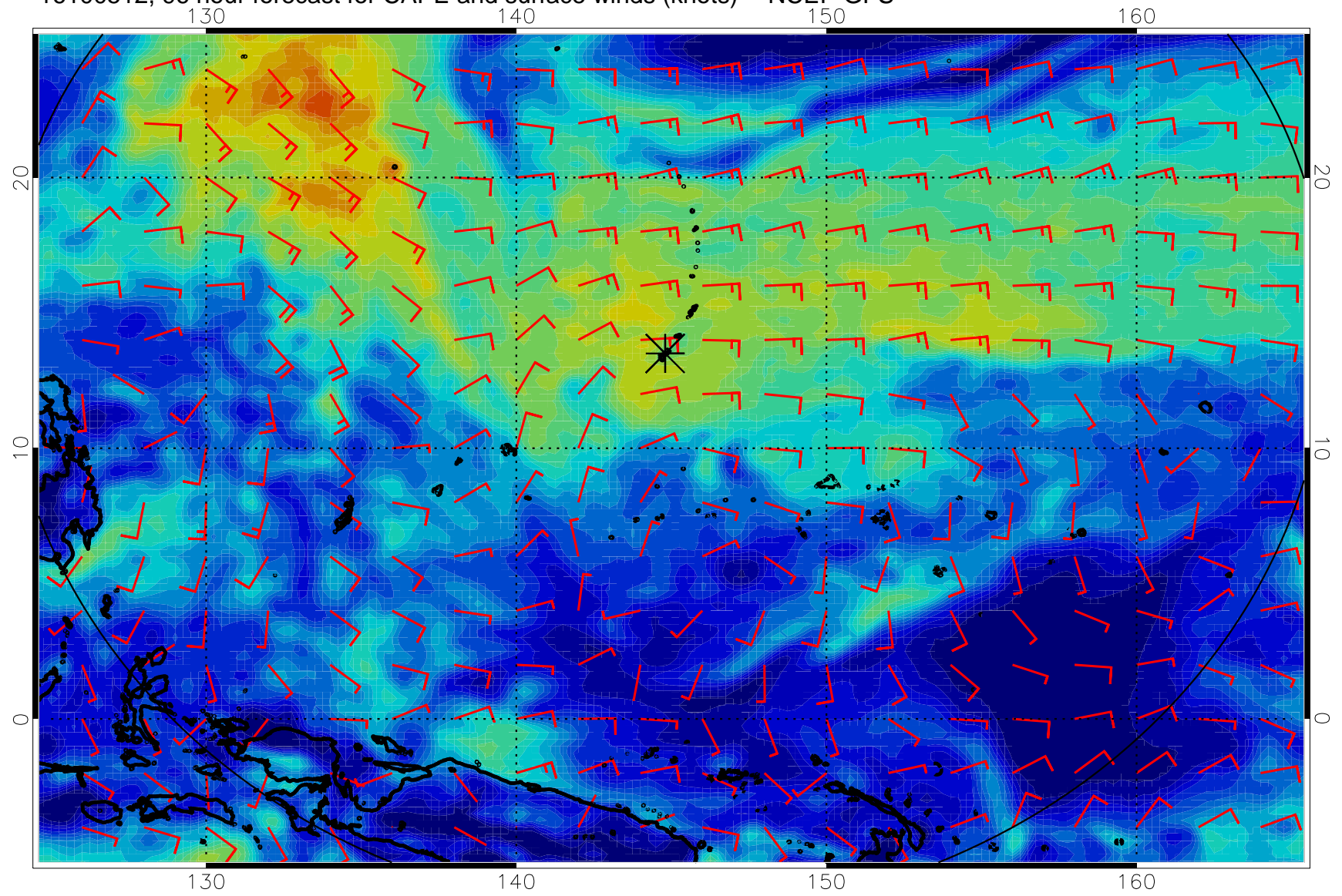
16100512, 96 hour forecast for CAPE and surface winds (knots) -- NCEP GFS
