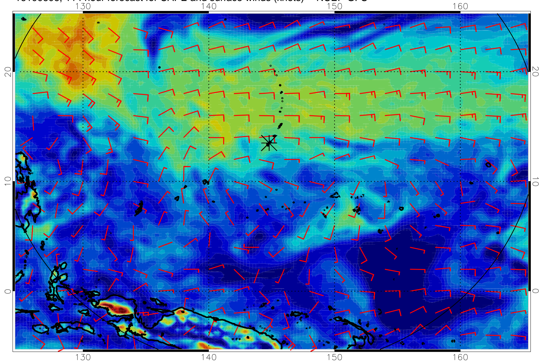
16100606, 114 hour forecast for CAPE and surface winds (knots) -- NCEP GFS
