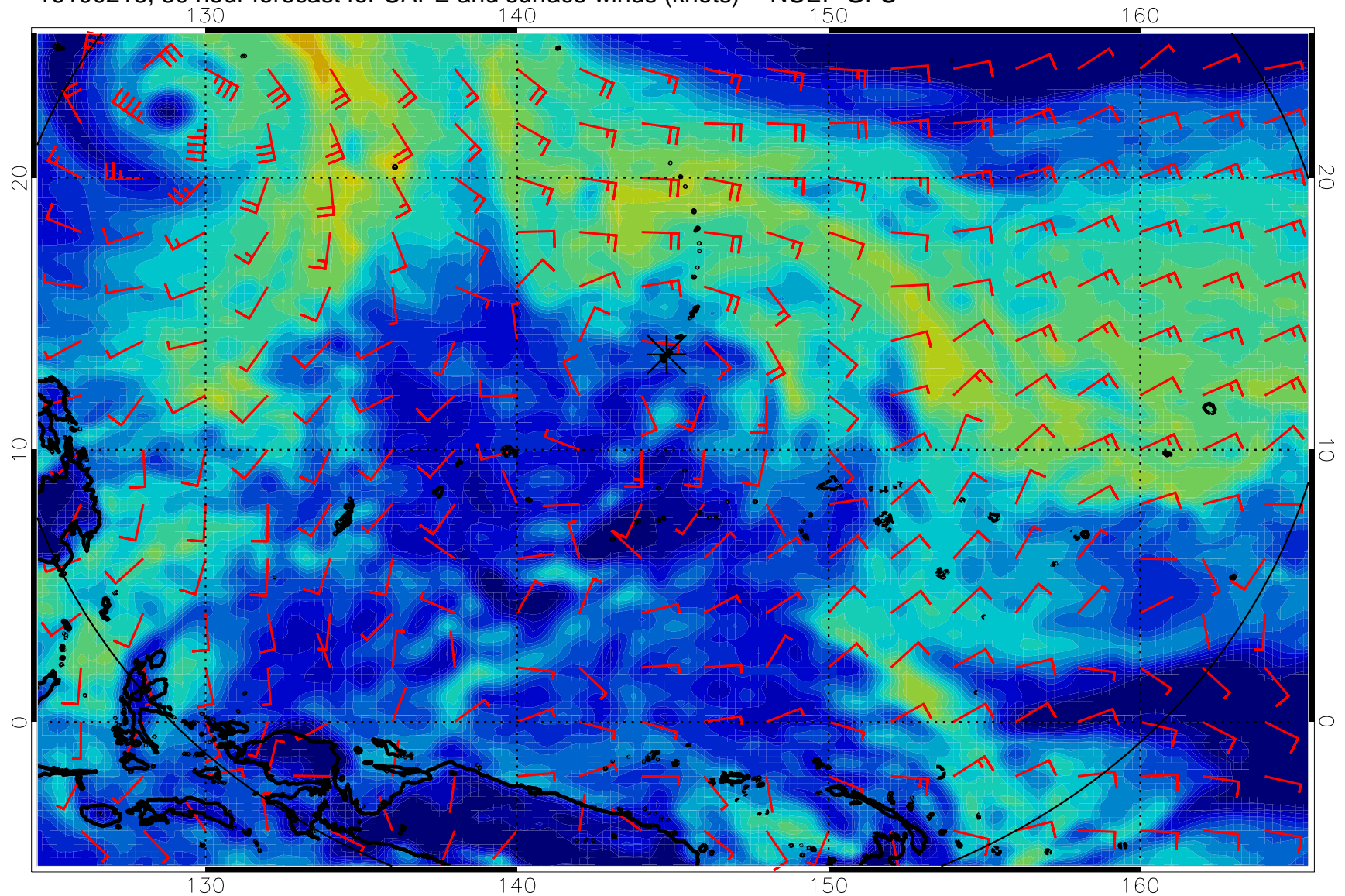
16100218, 30 hour forecast for CAPE and surface winds (knots) -- NCEP GFS
