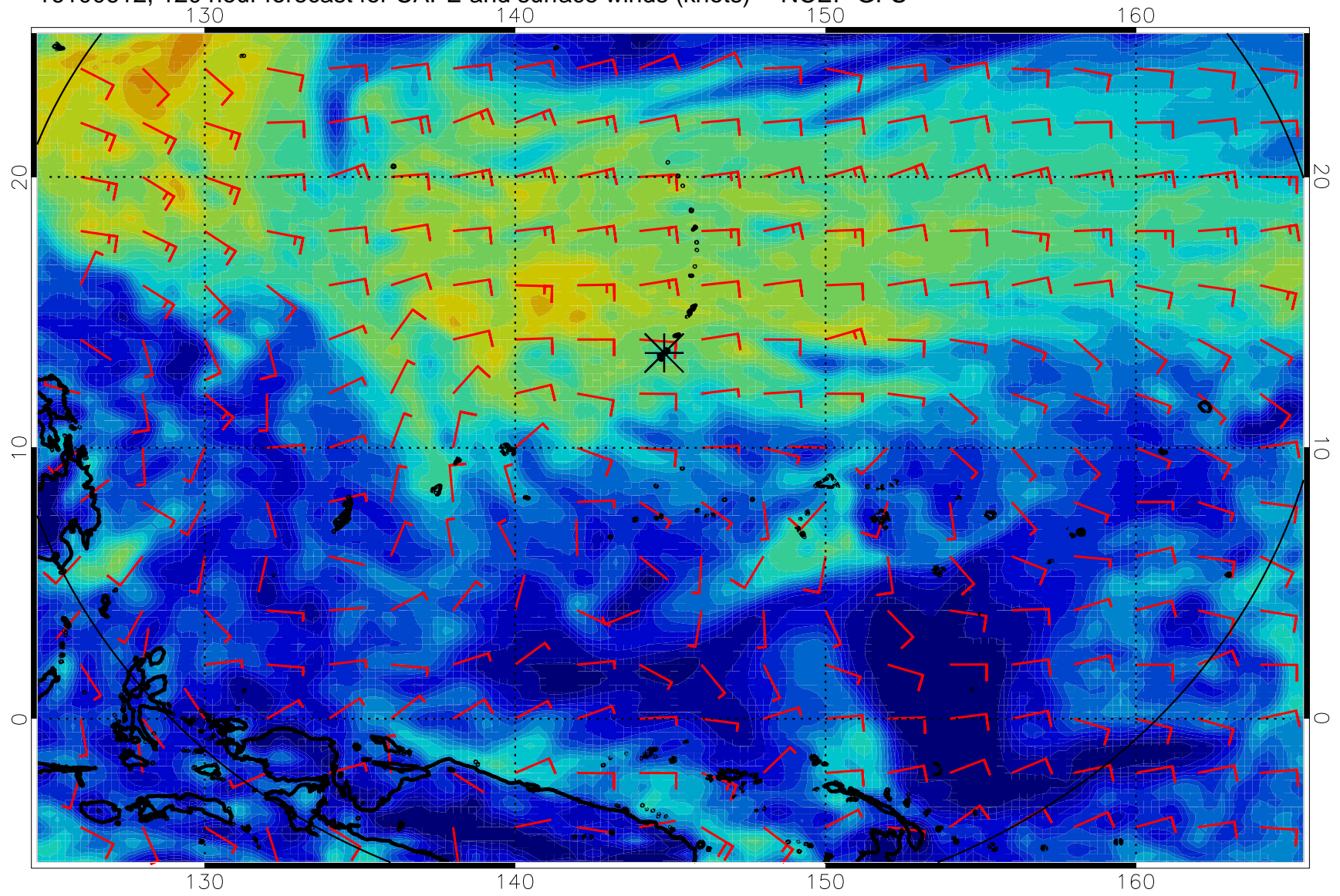
16100612, 120 hour forecast for CAPE and surface winds (knots) -- NCEP GFS
