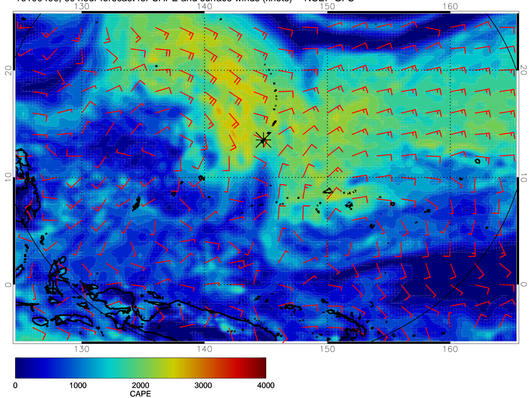
16100400, 60 hour forecast for CAPE and surface winds (knots) -- NCEP GFS
