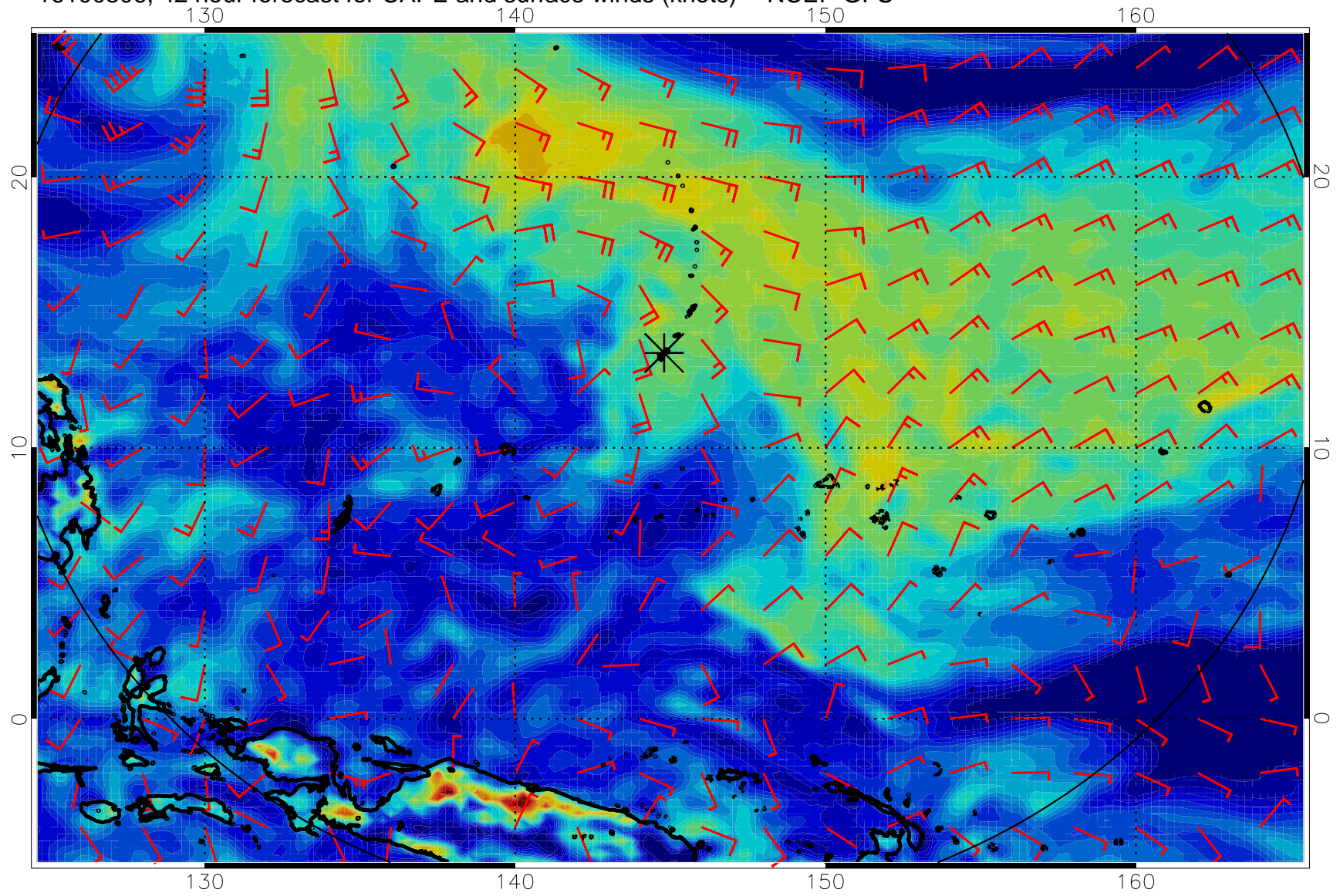
16100306, 42 hour forecast for CAPE and surface winds (knots) -- NCEP GFS
