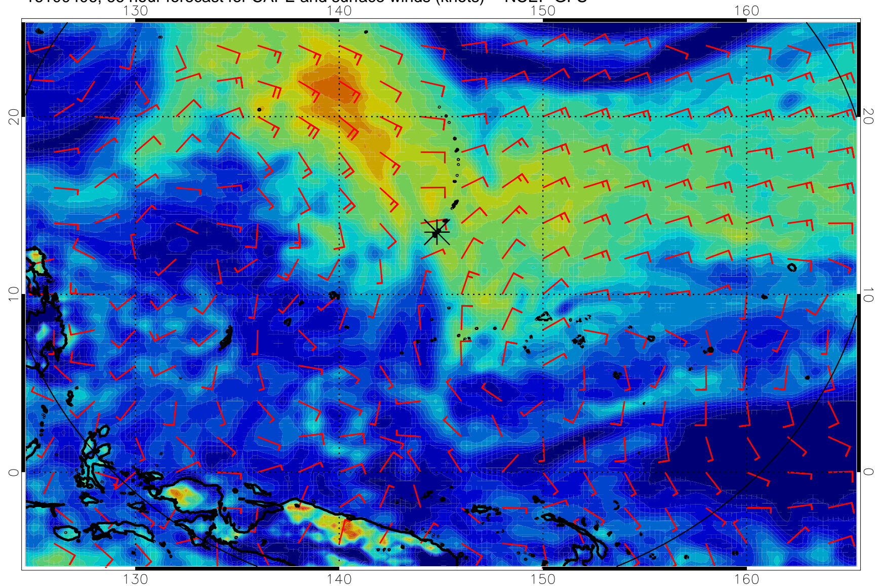
16100406, 66 hour forecast for CAPE and surface winds (knots) -- NCEP GFS
