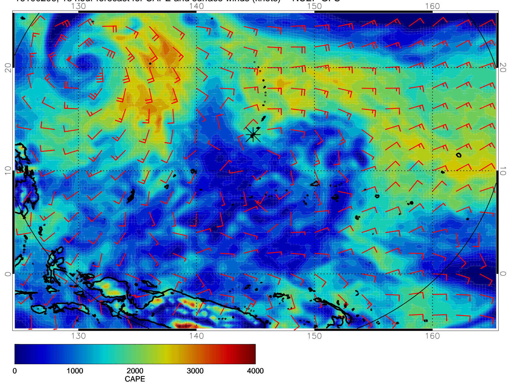
16100206, 18 hour forecast for CAPE and surface winds (knots) -- NCEP GFS
