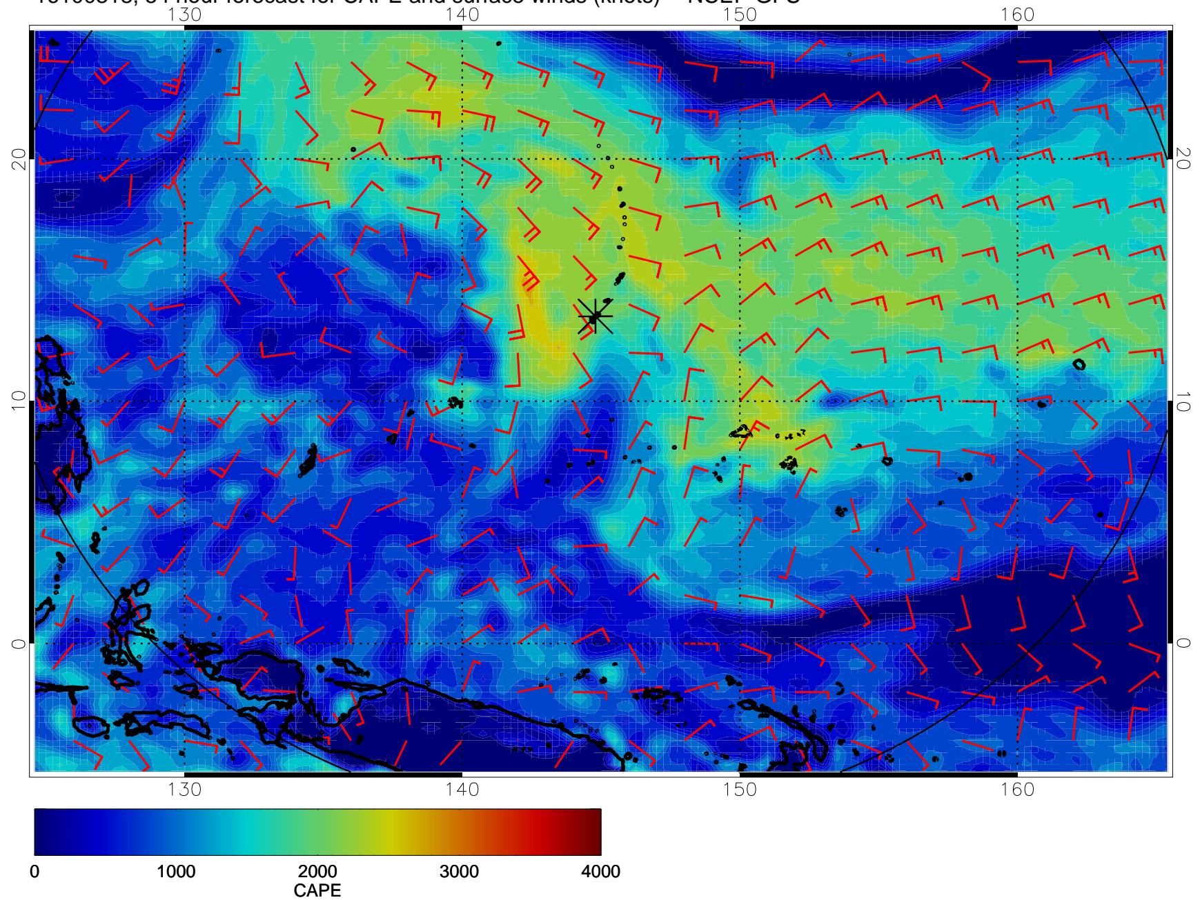
16100318, 54 hour forecast for CAPE and surface winds (knots) -- NCEP GFS
