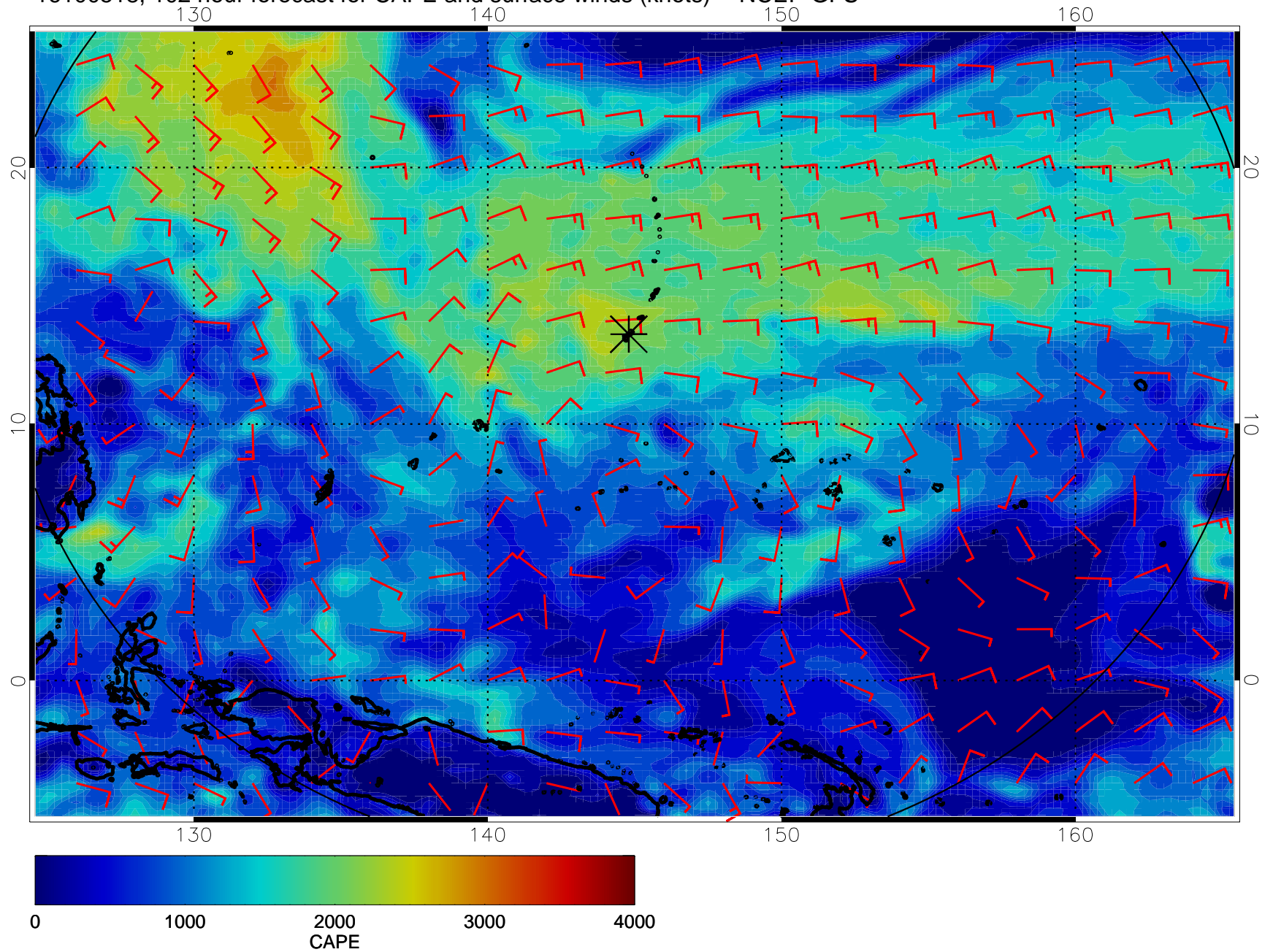
16100518, 102 hour forecast for CAPE and surface winds (knots) -- NCEP GFS
