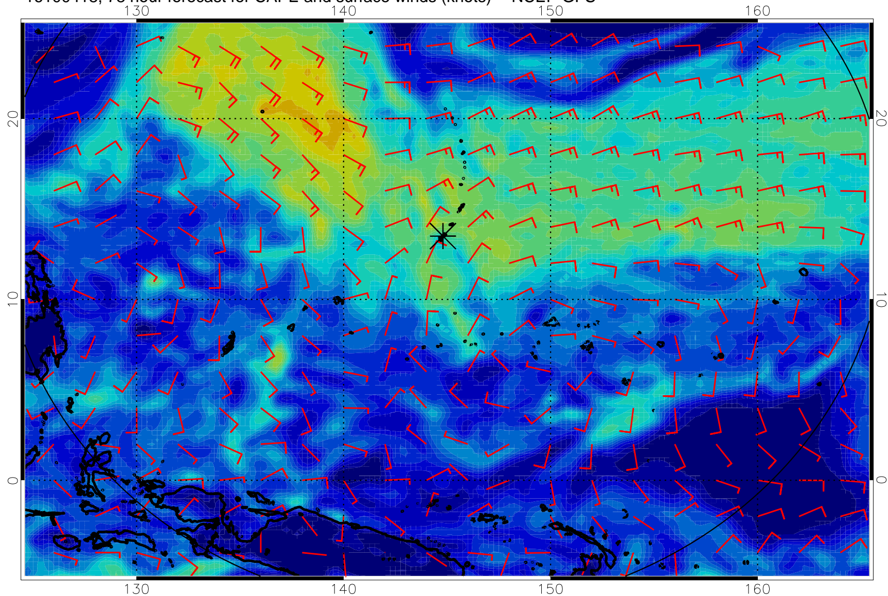
16100418, 78 hour forecast for CAPE and surface winds (knots) -- NCEP GFS
