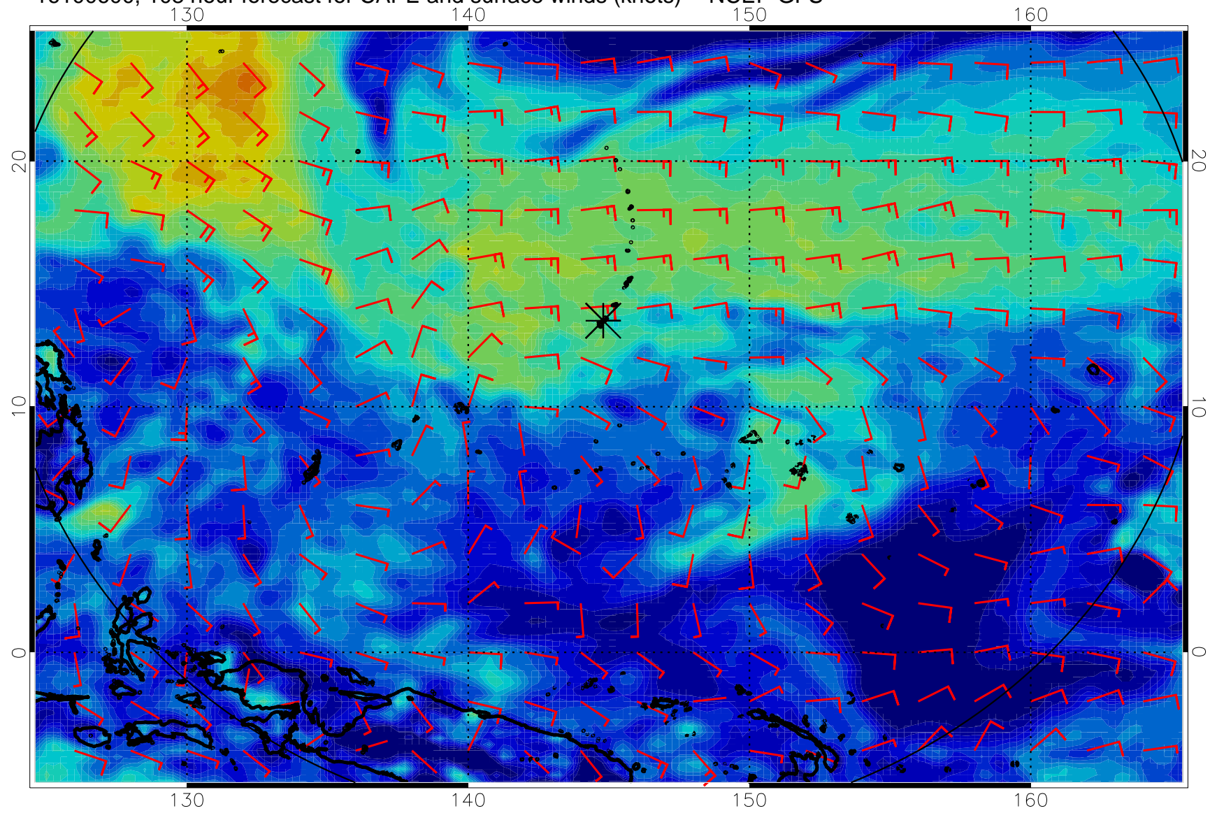
16100600, 108 hour forecast for CAPE and surface winds (knots) -- NCEP GFS
