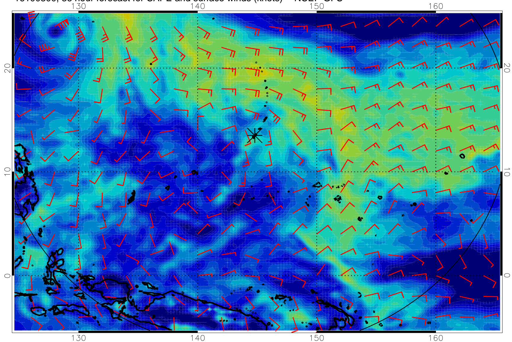
16100300, 36 hour forecast for CAPE and surface winds (knots) -- NCEP GFS
