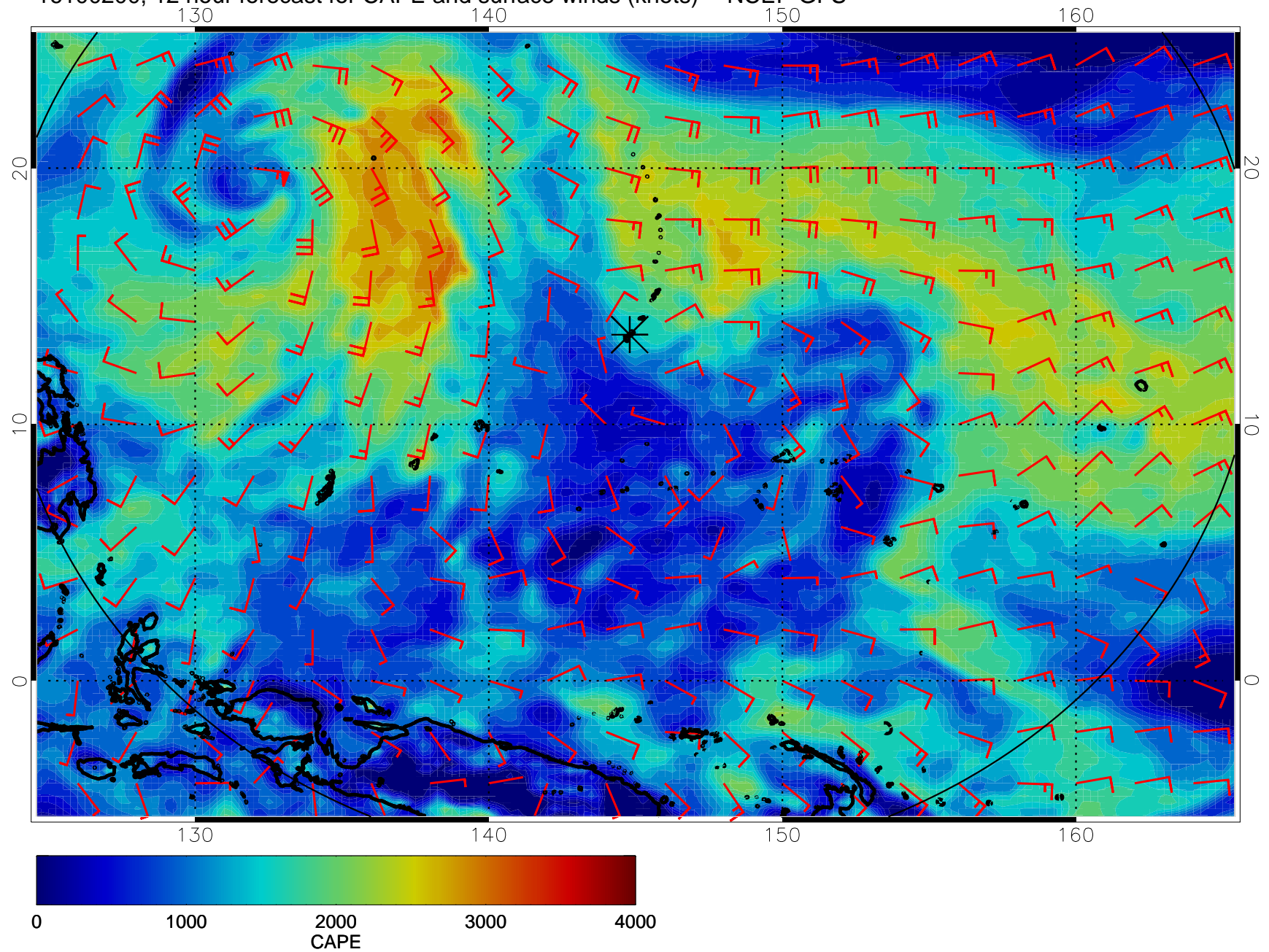
16100200, 12 hour forecast for CAPE and surface winds (knots) -- NCEP GFS
