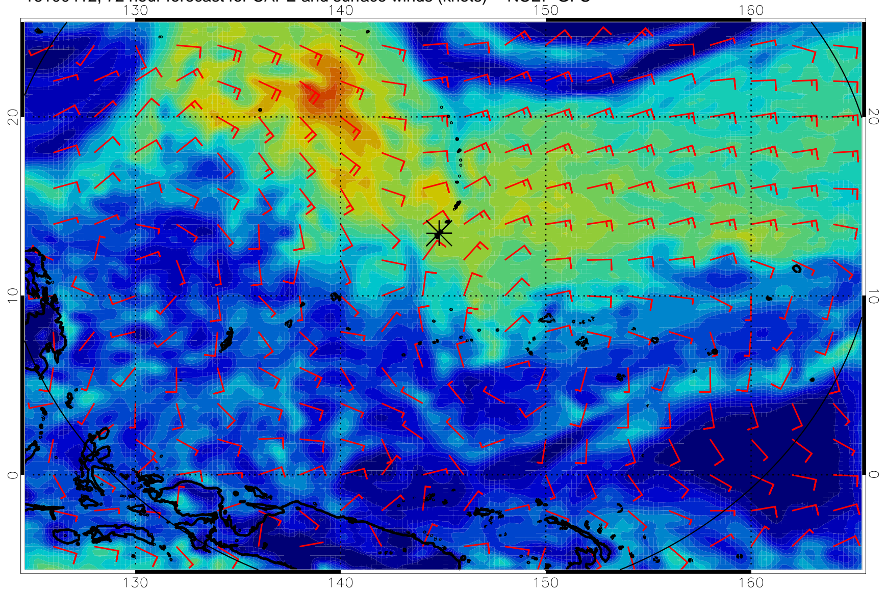
16100412, 72 hour forecast for CAPE and surface winds (knots) -- NCEP GFS
