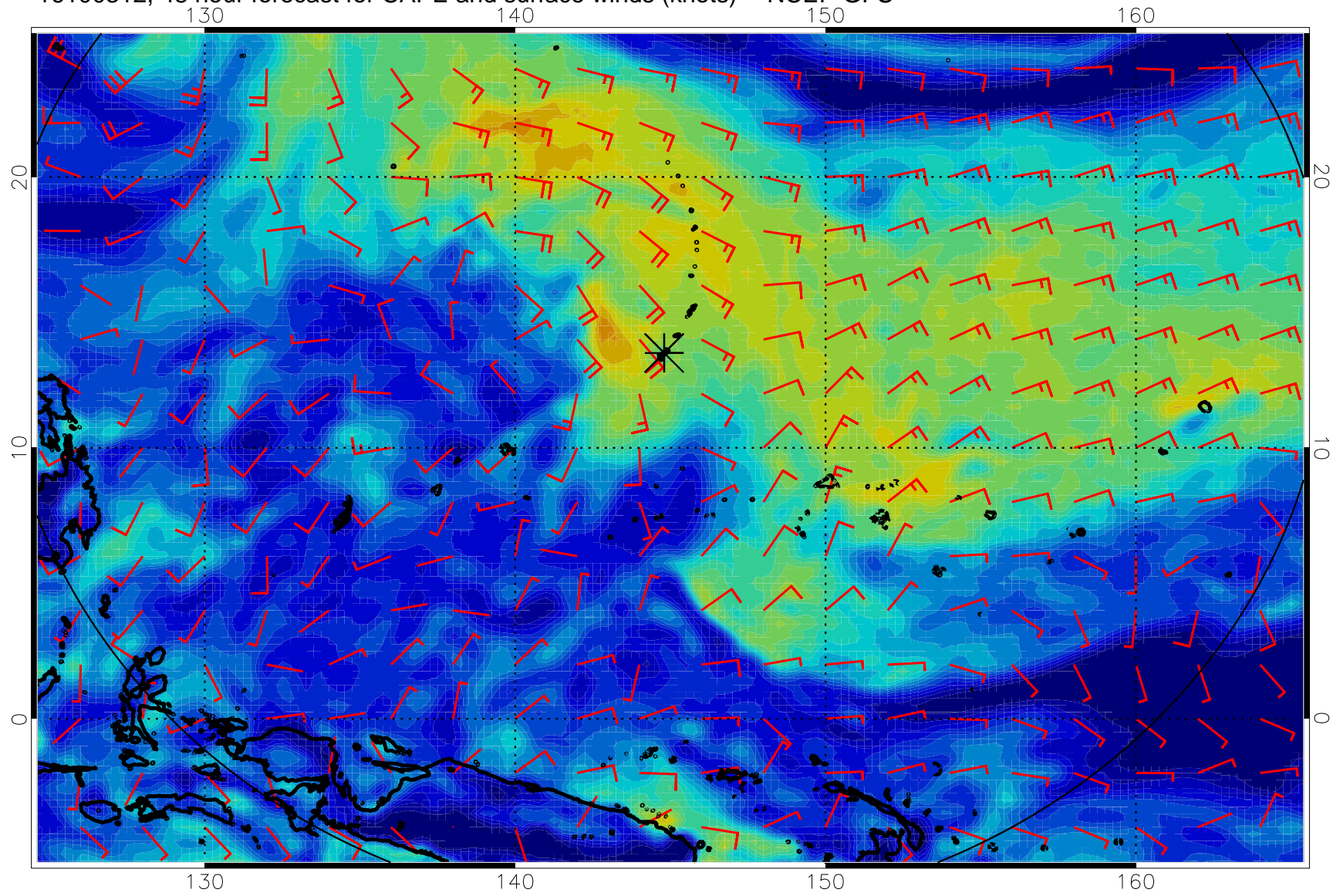
16100312, 48 hour forecast for CAPE and surface winds (knots) -- NCEP GFS
