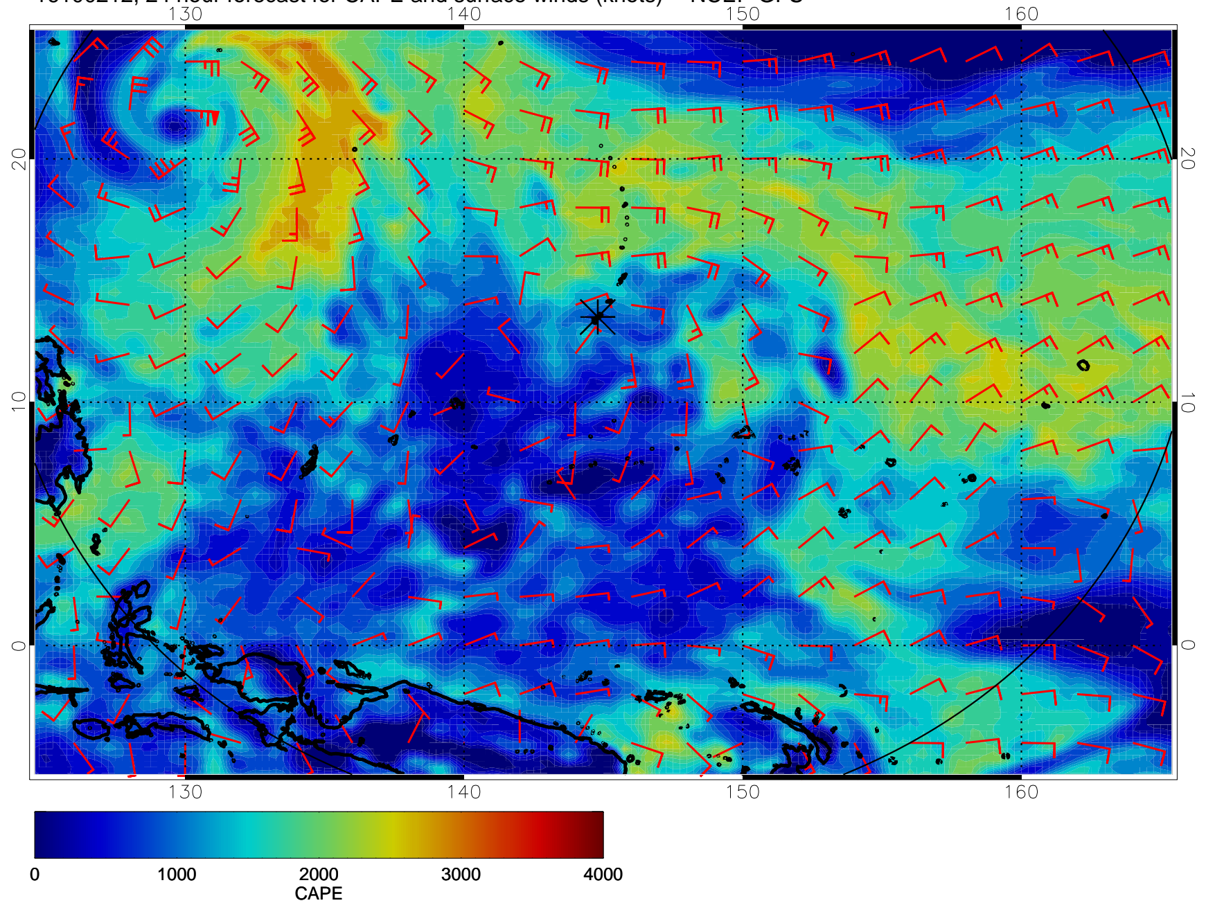
16100212, 24 hour forecast for CAPE and surface winds (knots) -- NCEP GFS
