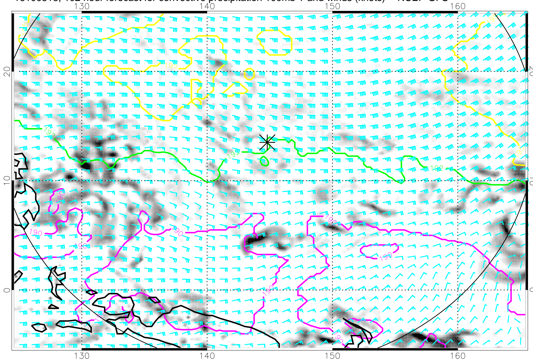
16100518, 102 hour forecast for convective precipitation 100mb T and winds (knots) -- NCEP GFS
