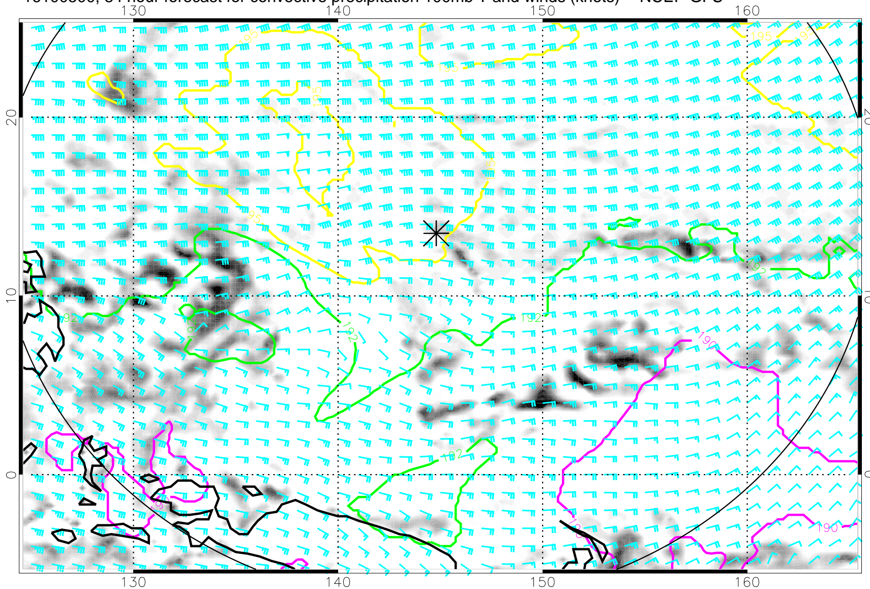
16100500, 84 hour forecast for convective precipitation 100mb T and winds (knots) -- NCEP GFS
