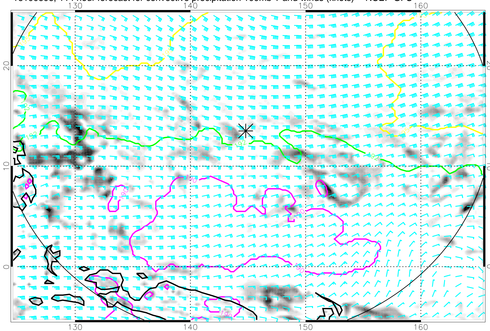
16100606, 114 hour forecast for convective precipitation 100mb T and winds (knots) -- NCEP GFS
