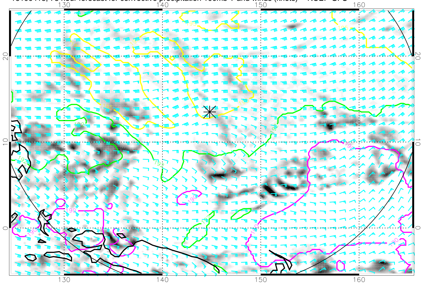
16100418, 78 hour forecast for convective precipitation 100mb T and winds (knots) -- NCEP GFS
