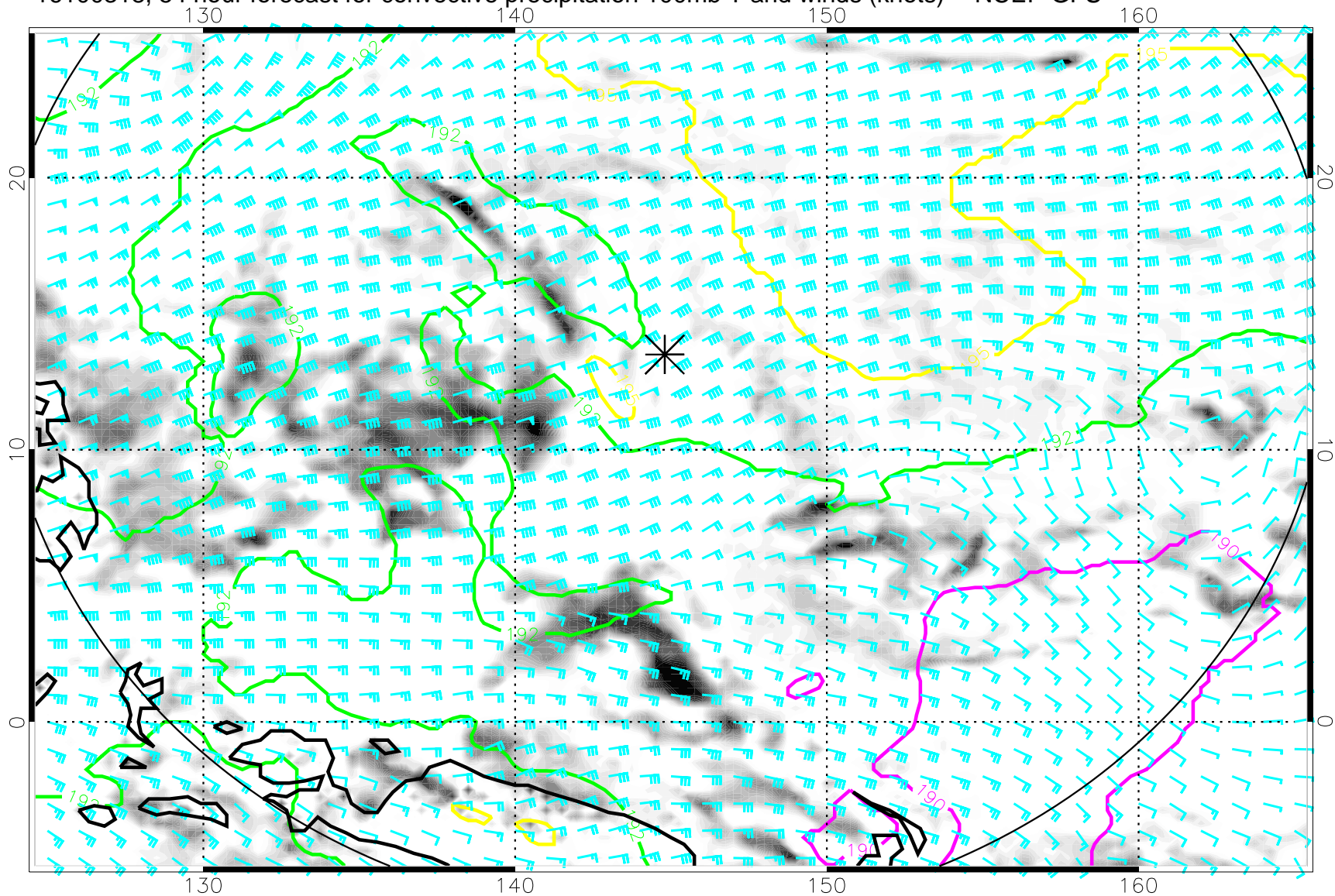
16100318, 54 hour forecast for convective precipitation 100mb T and winds (knots) -- NCEP GFS
