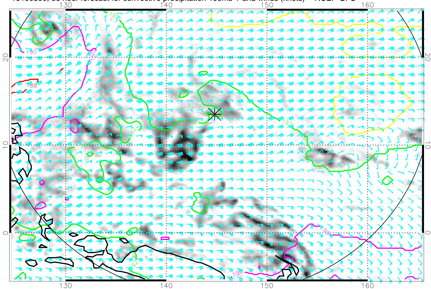
16100300, 36 hour forecast for convective precipitation 100mb T and winds (knots) -- NCEP GFS
