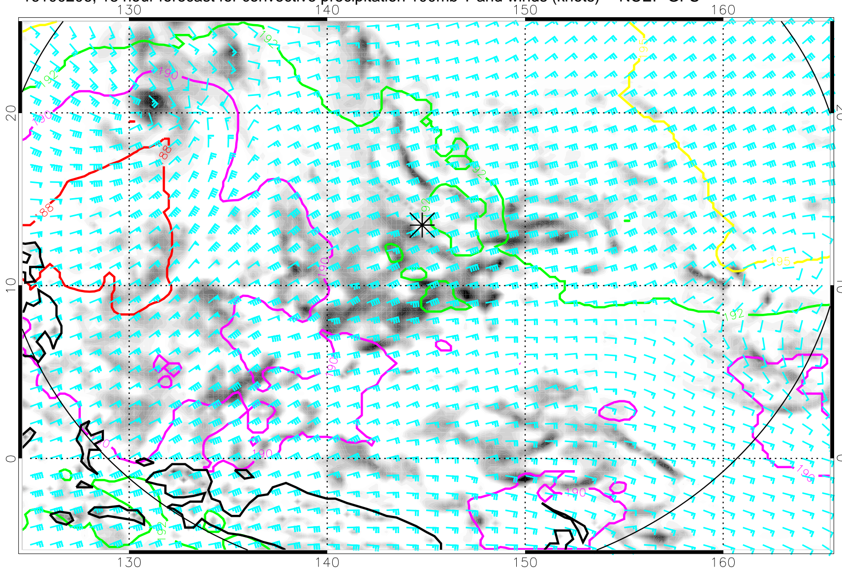
16100206, 18 hour forecast for convective precipitation 100mb T and winds (knots) -- NCEP GFS
