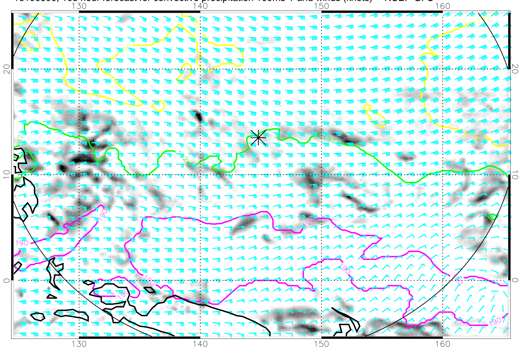
16100600, 108 hour forecast for convective precipitation 100mb T and winds (knots) -- NCEP GFS
