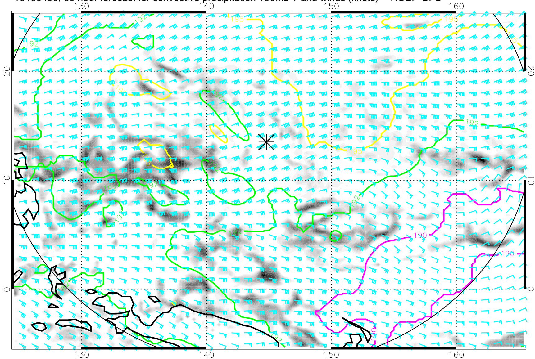
16100400, 60 hour forecast for convective precipitation 100mb T and winds (knots) -- NCEP GFS
