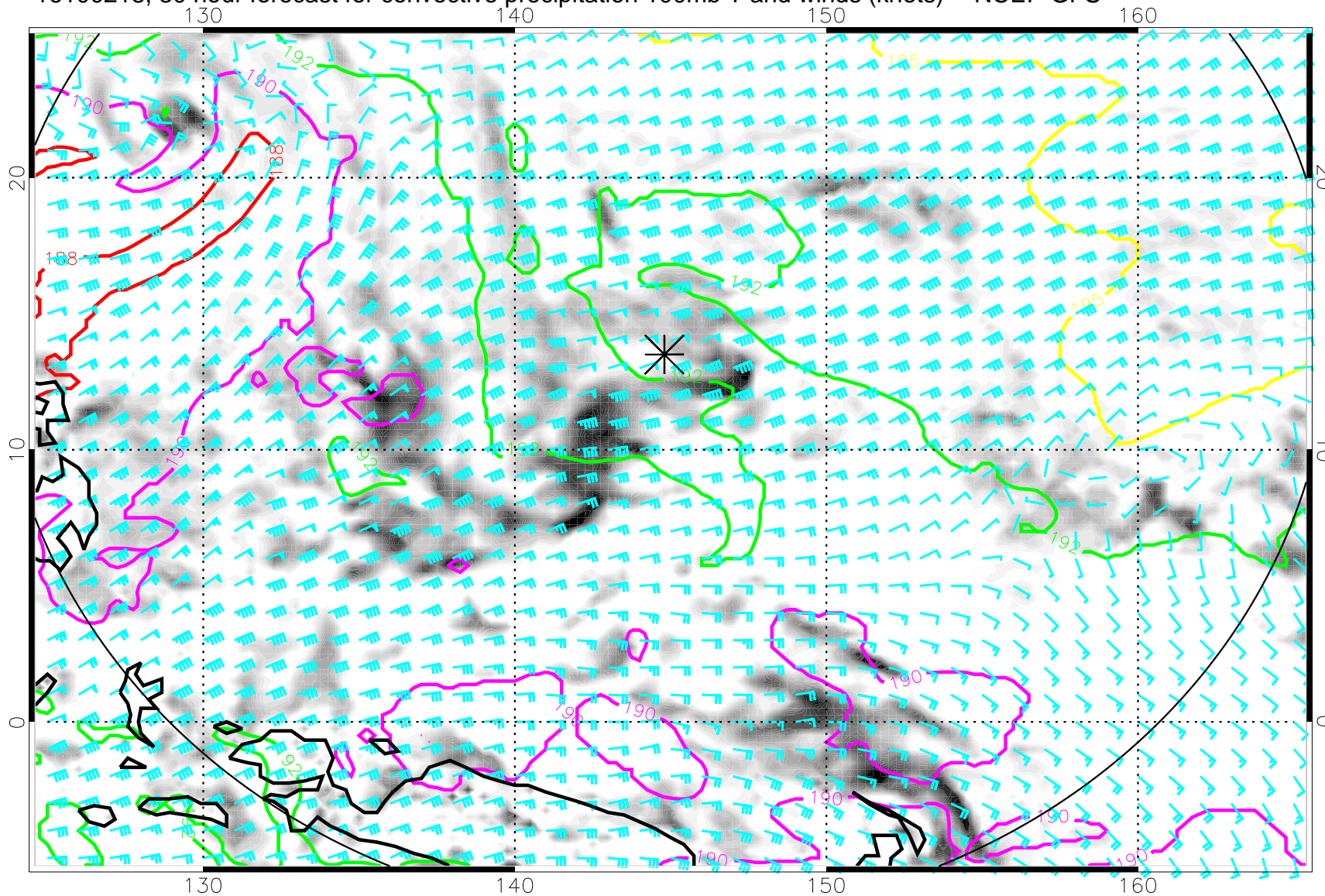
16100218, 30 hour forecast for convective precipitation 100mb T and winds (knots) -- NCEP GFS
