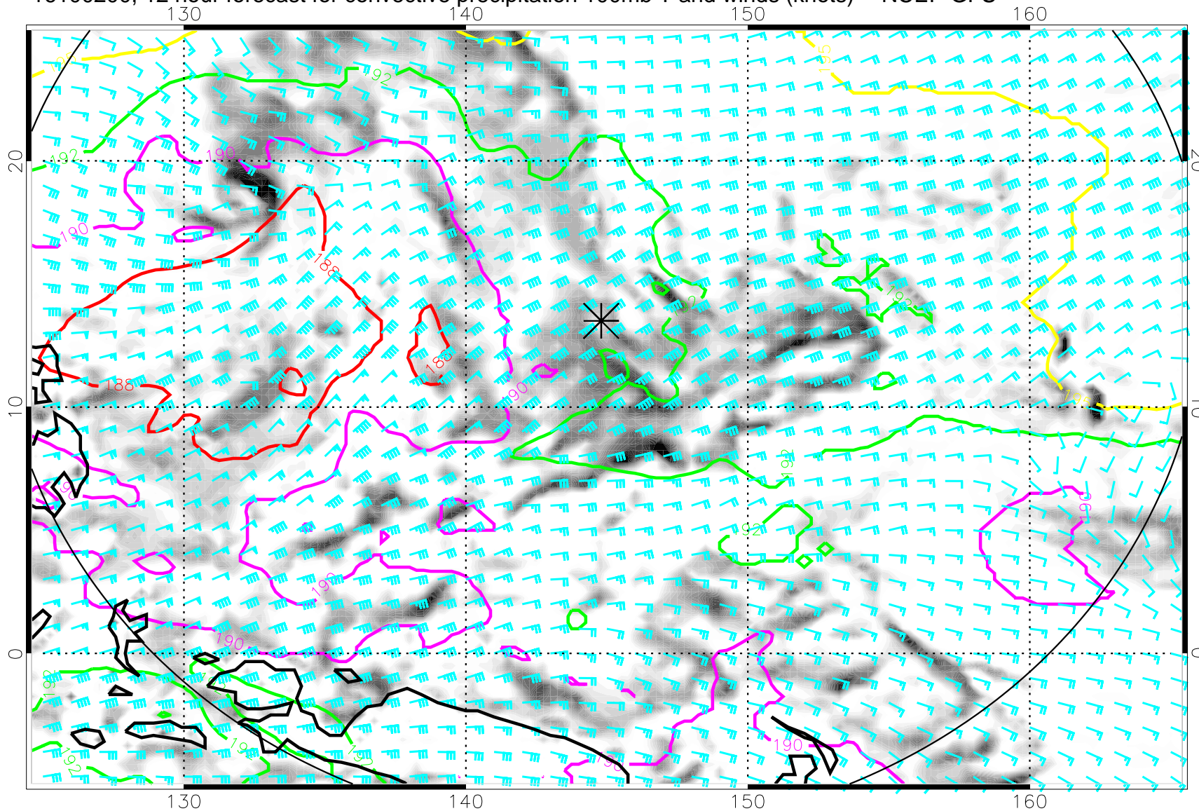
16100200, 12 hour forecast for convective precipitation 100mb T and winds (knots) -- NCEP GFS
