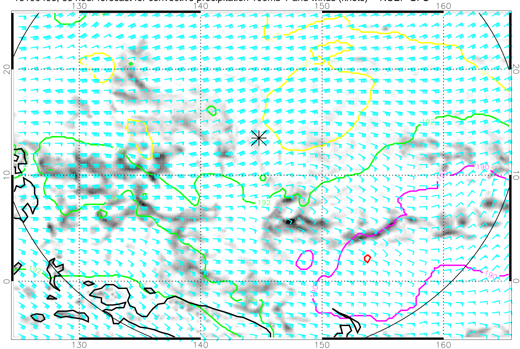
16100406, 66 hour forecast for convective precipitation 100mb T and winds (knots) -- NCEP GFS
