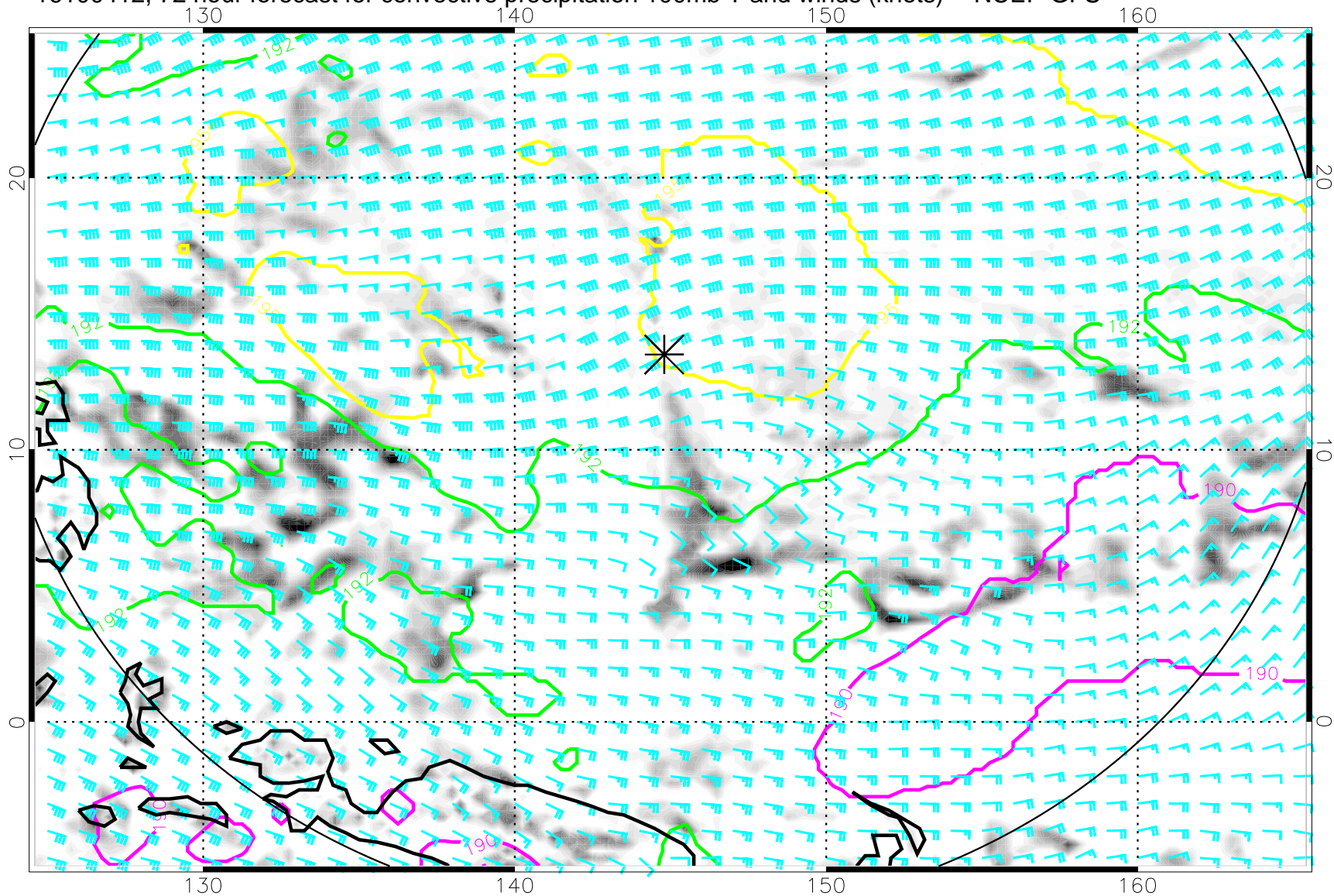
16100412, 72 hour forecast for convective precipitation 100mb T and winds (knots) -- NCEP GFS
