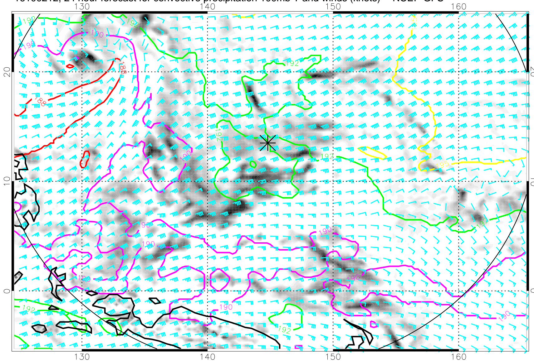
16100212, 24 hour forecast for convective precipitation 100mb T and winds (knots) -- NCEP GFS
