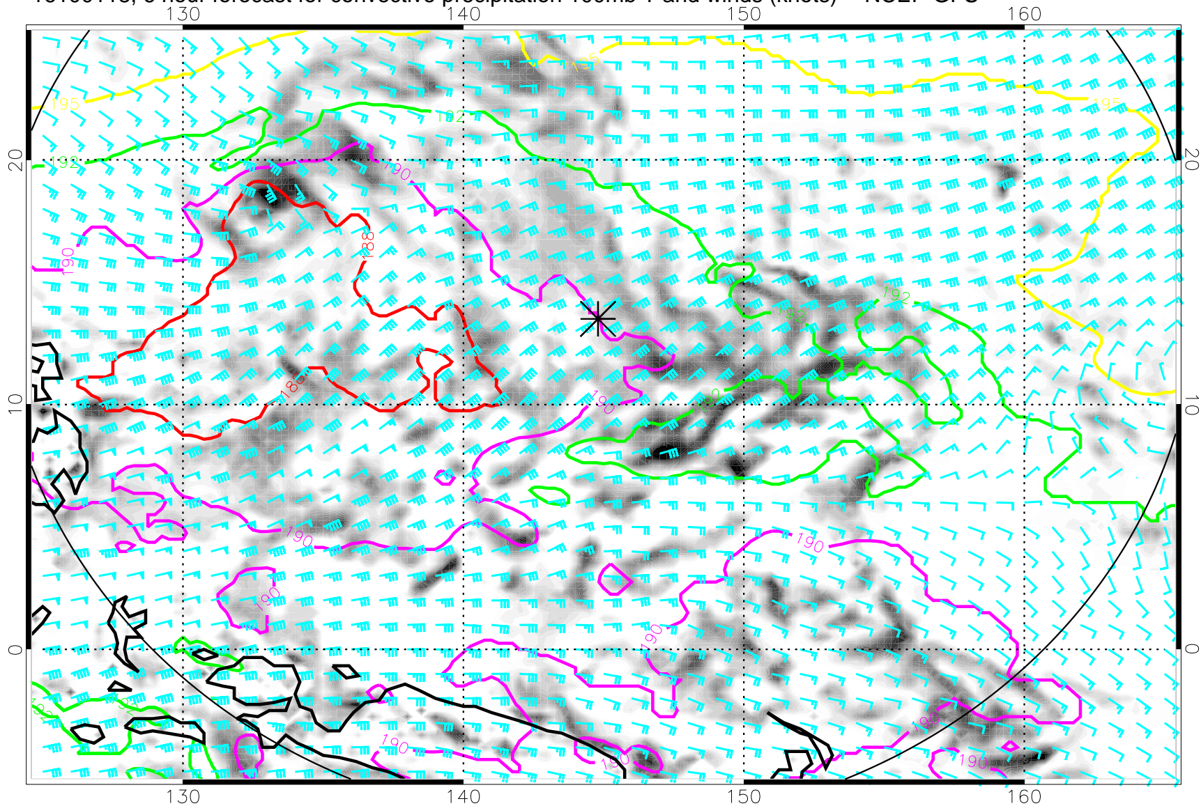
16100118, 6 hour forecast for convective precipitation 100mb T and winds (knots) -- NCEP GFS
