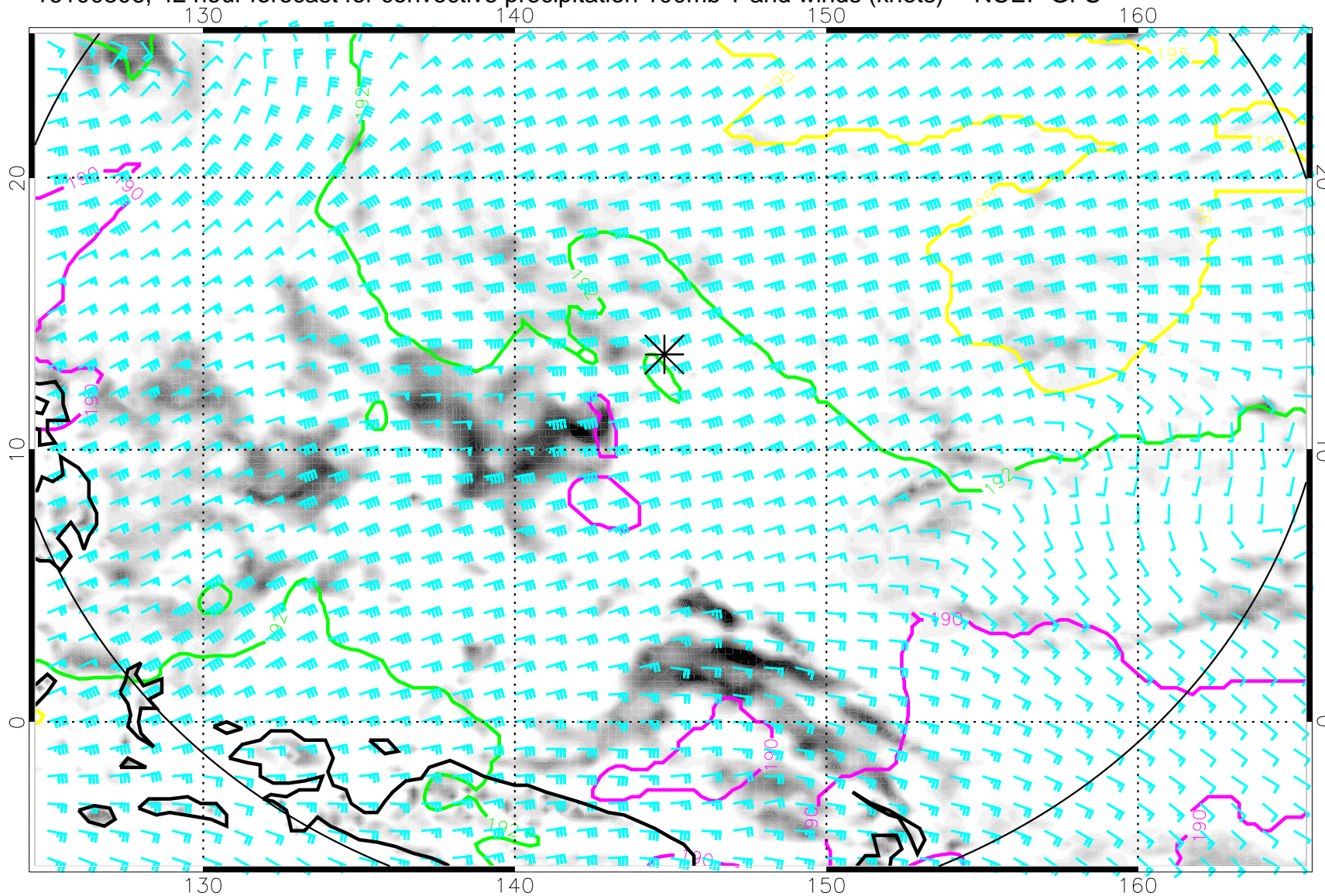
16100306, 42 hour forecast for convective precipitation 100mb T and winds (knots) -- NCEP GFS
