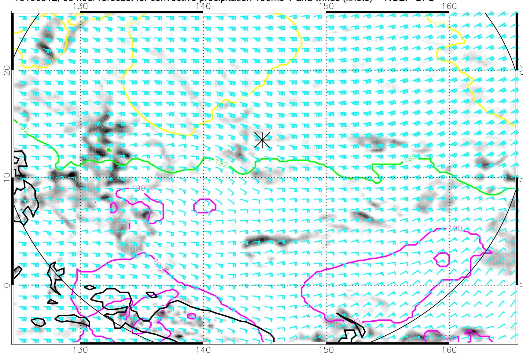
16100512, 96 hour forecast for convective precipitation 100mb T and winds (knots) -- NCEP GFS
