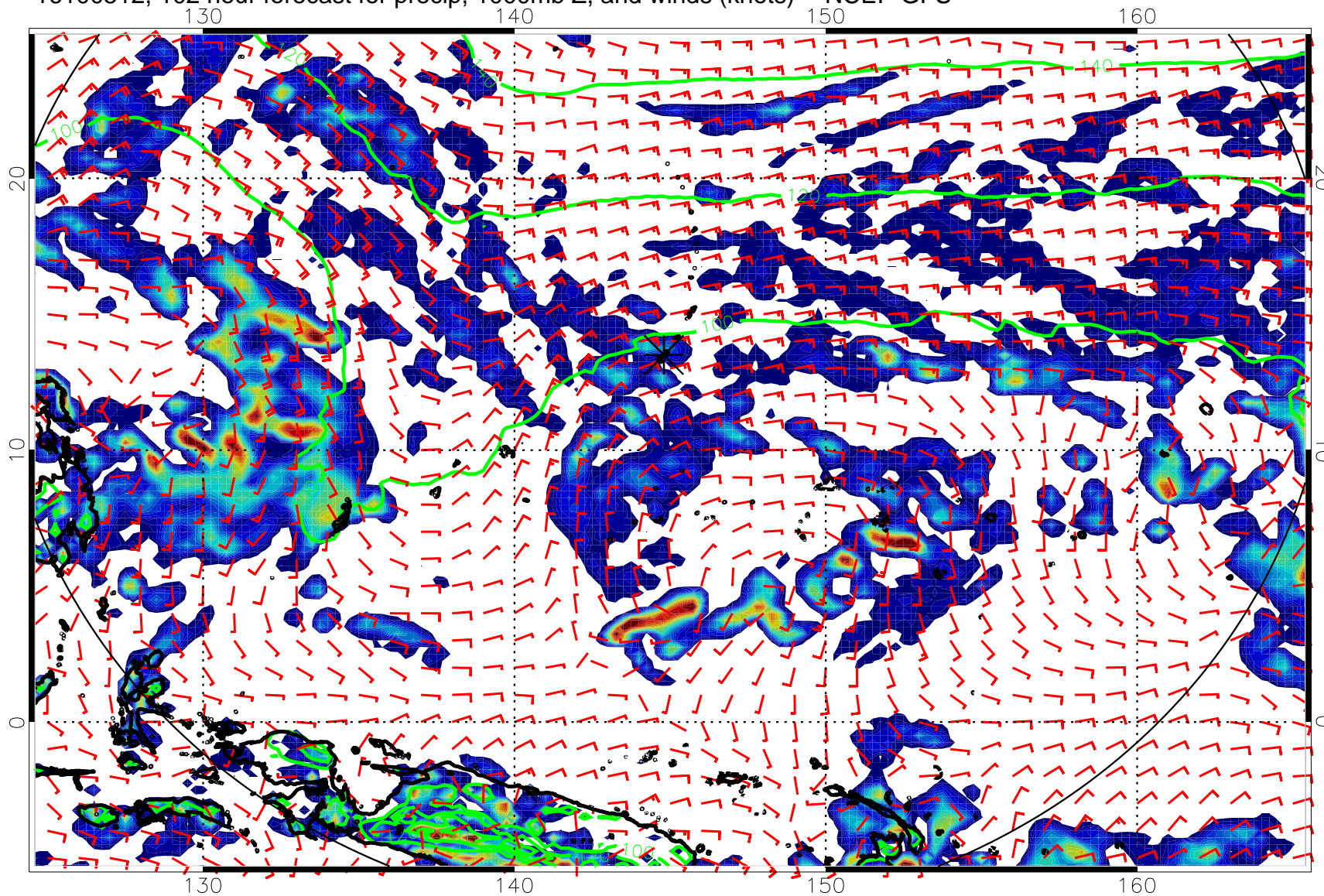
16100512, 102 hour forecast for precip, 1000mb Z, and winds (knots) -- NCEP GFS
