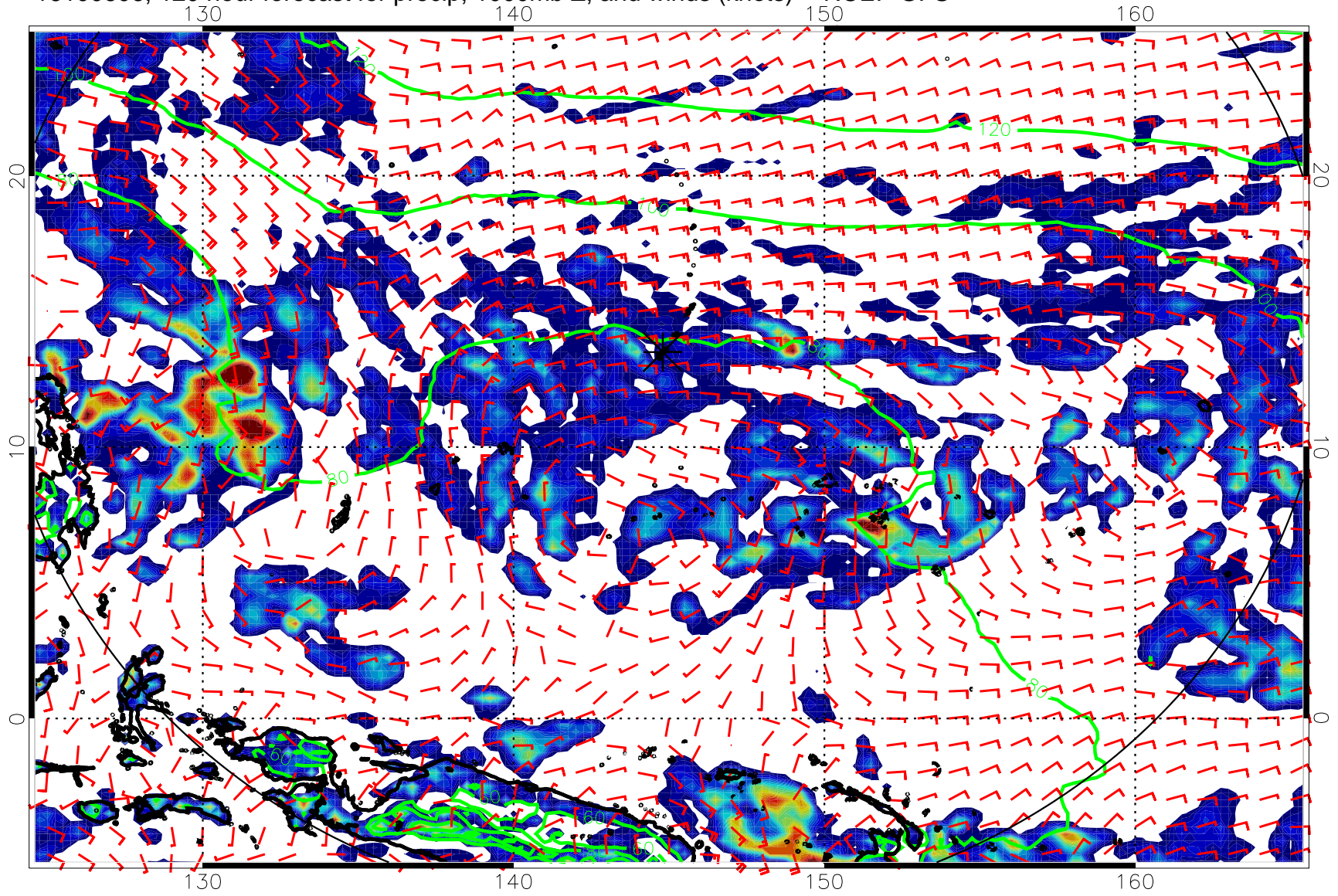
16100606, 120 hour forecast for precip, 1000mb Z, and winds (knots) -- NCEP GFS
