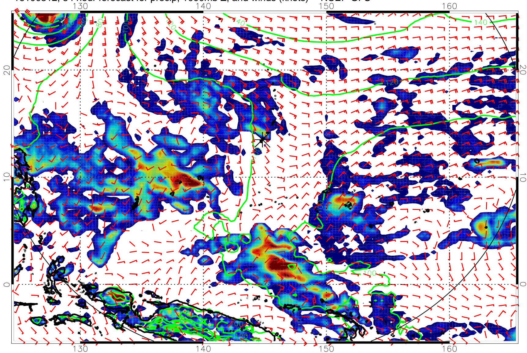
16100312, 54 hour forecast for precip, 1000mb Z, and winds (knots) -- NCEP GFS
