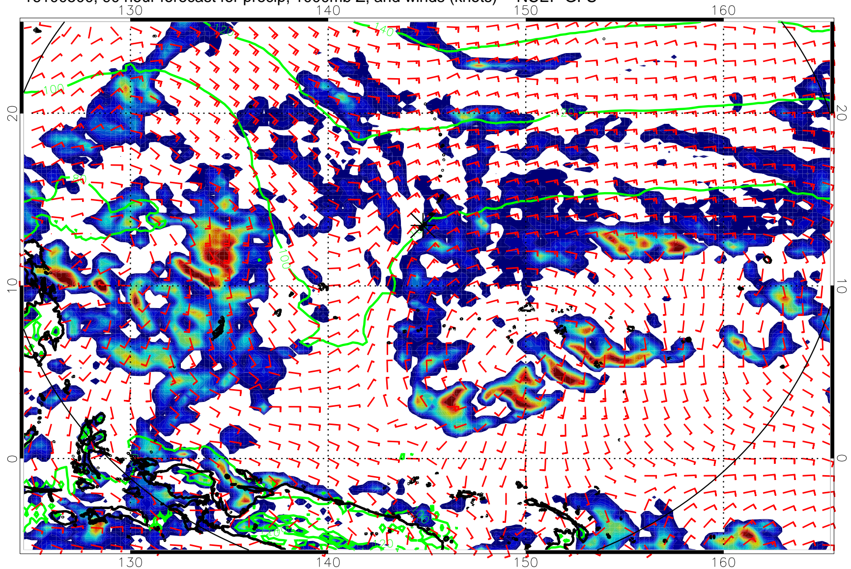
16100500, 90 hour forecast for precip, 1000mb Z, and winds (knots) -- NCEP GFS
