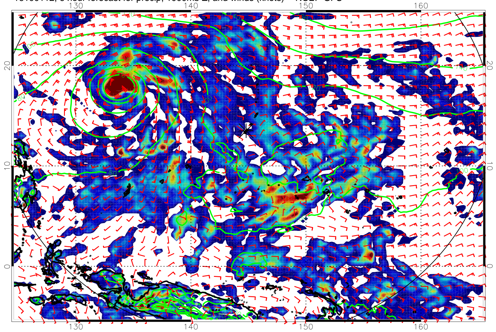
16100112, 6 hour forecast for precip, 1000mb Z, and winds (knots) -- NCEP GFS
