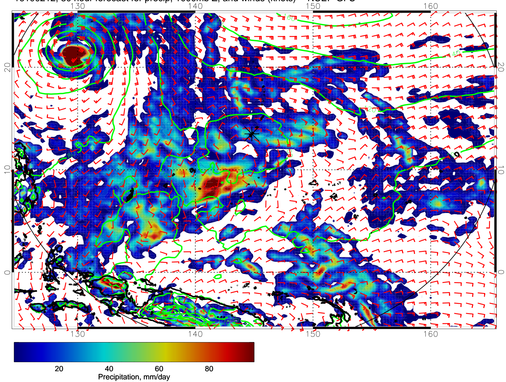
16100212, 30 hour forecast for precip, 1000mb Z, and winds (knots) -- NCEP GFS
