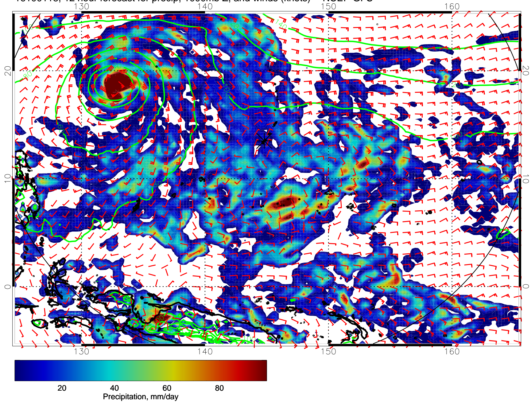
16100118, 12 hour forecast for precip, 1000mb Z, and winds (knots) -- NCEP GFS
