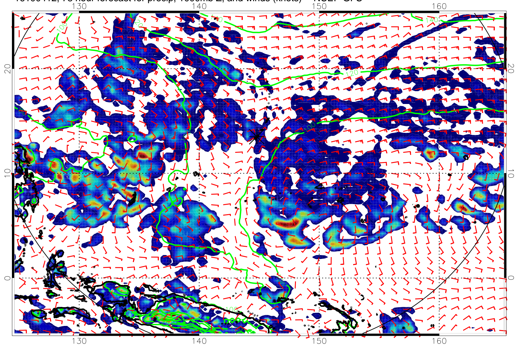
16100412, 78 hour forecast for precip, 1000mb Z, and winds (knots) -- NCEP GFS
