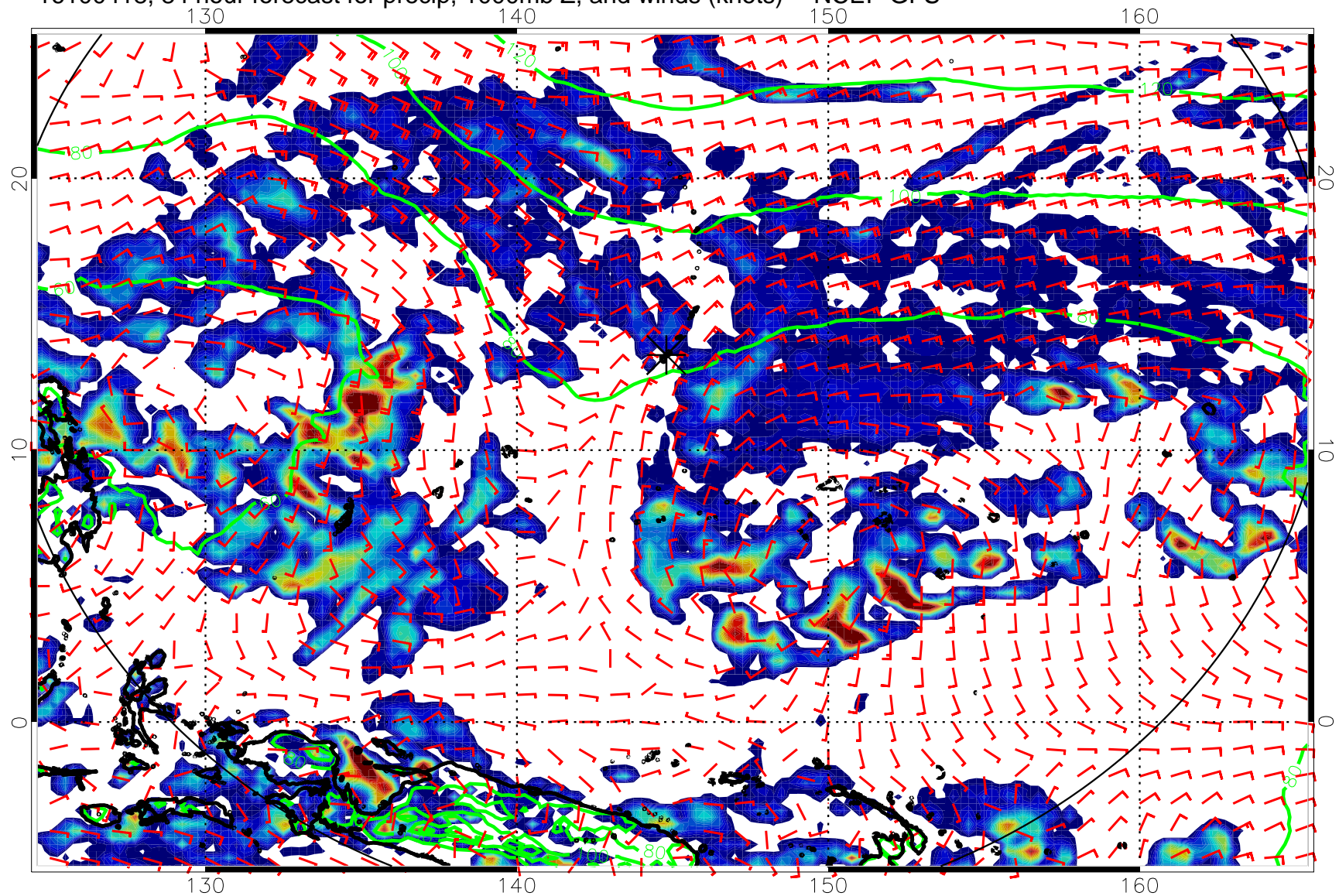
16100418, 84 hour forecast for precip, 1000mb Z, and winds (knots) -- NCEP GFS
