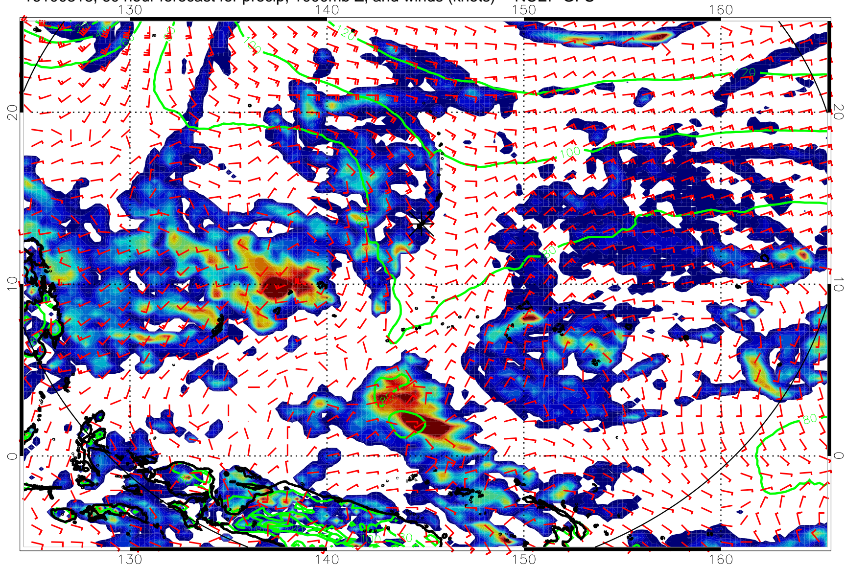
16100318, 60 hour forecast for precip, 1000mb Z, and winds (knots) -- NCEP GFS
