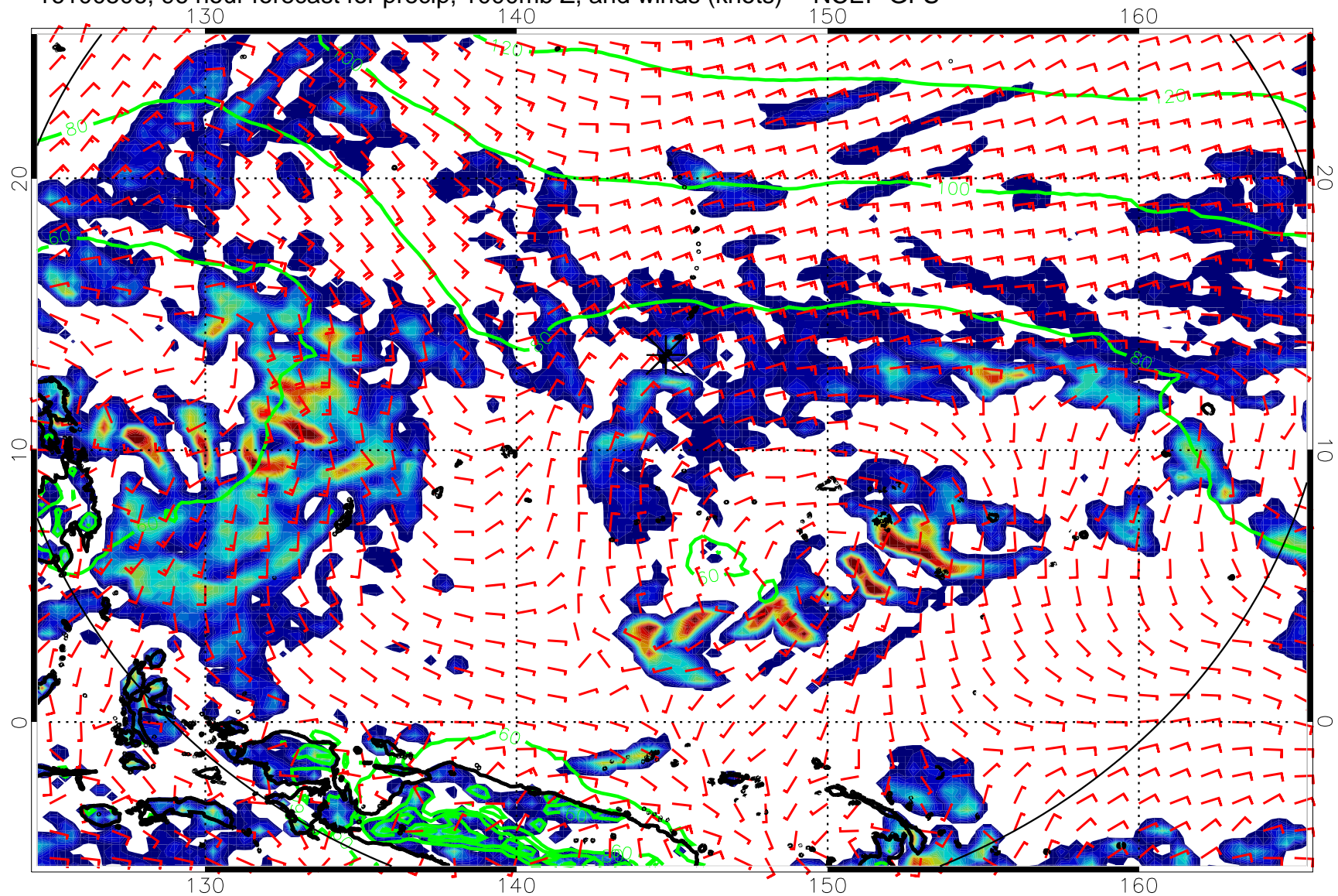
16100506, 96 hour forecast for precip, 1000mb Z, and winds (knots) -- NCEP GFS
