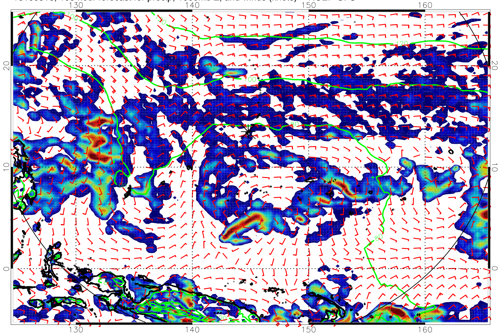
16100518, 108 hour forecast for precip, 1000mb Z, and winds (knots) -- NCEP GFS
