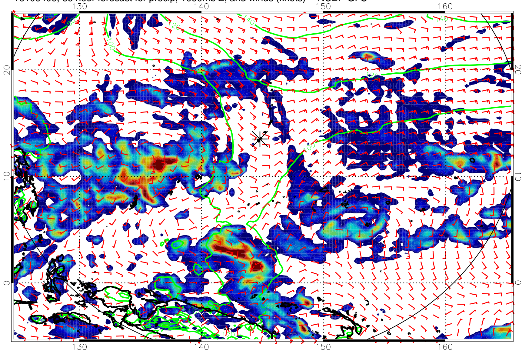
16100400, 66 hour forecast for precip, 1000mb Z, and winds (knots) -- NCEP GFS
