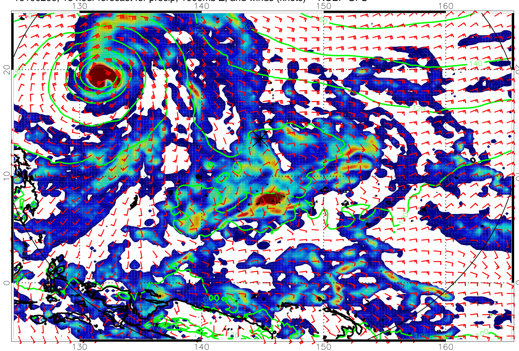
16100200, 18 hour forecast for precip, 1000mb Z, and winds (knots) -- NCEP GFS
