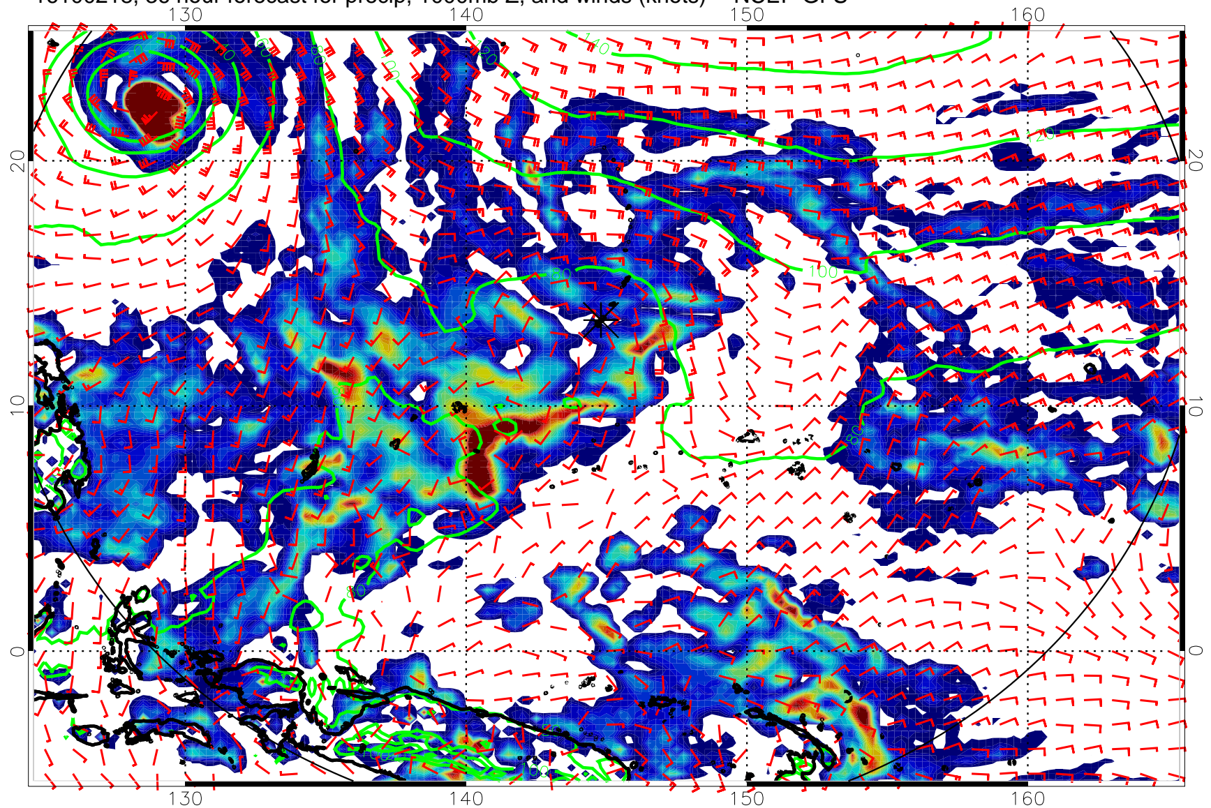
16100218, 36 hour forecast for precip, 1000mb Z, and winds (knots) -- NCEP GFS
