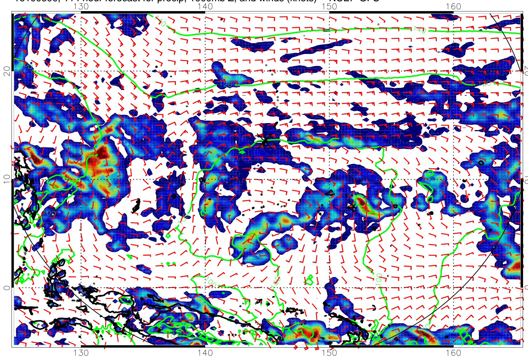
16100600, 114 hour forecast for precip, 1000mb Z, and winds (knots) -- NCEP GFS
