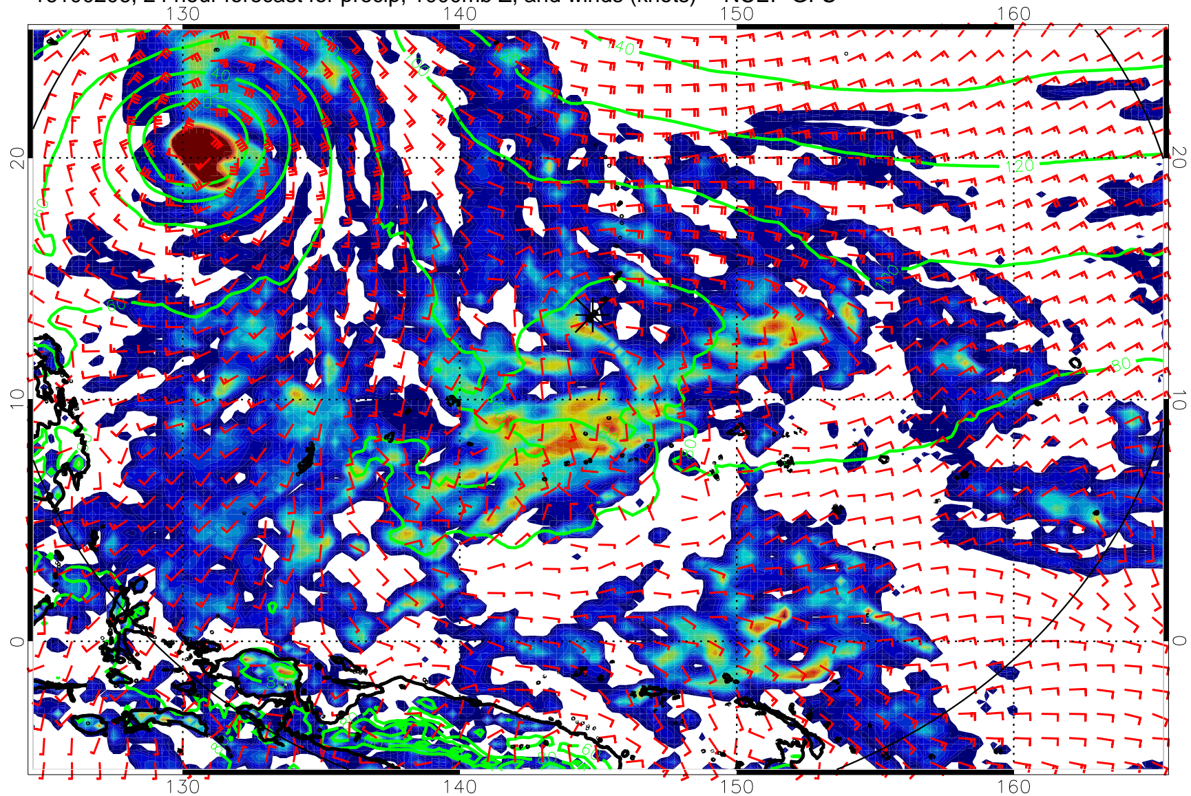
16100206, 24 hour forecast for precip, 1000mb Z, and winds (knots) -- NCEP GFS
