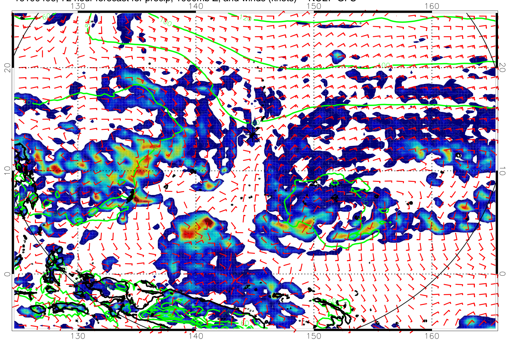
16100406, 72 hour forecast for precip, 1000mb Z, and winds (knots) -- NCEP GFS
