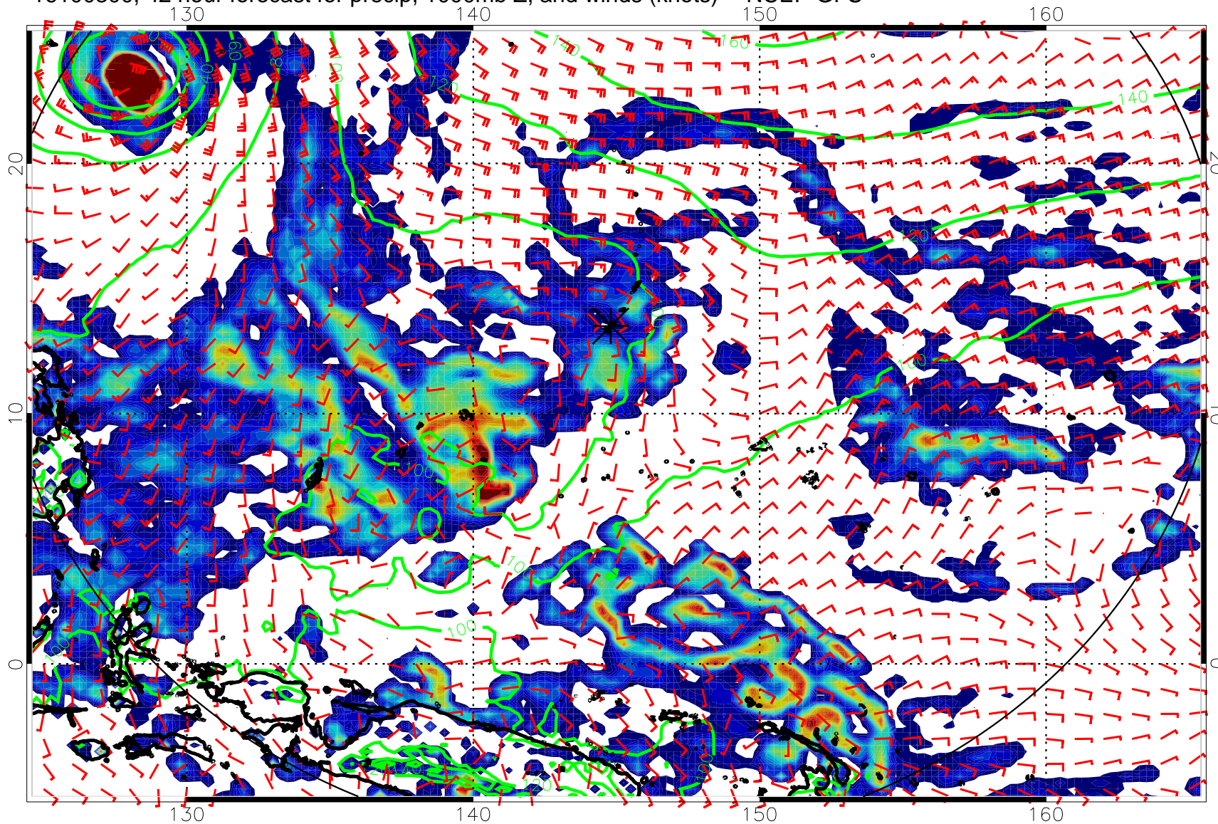
16100300, 42 hour forecast for precip, 1000mb Z, and winds (knots) -- NCEP GFS
