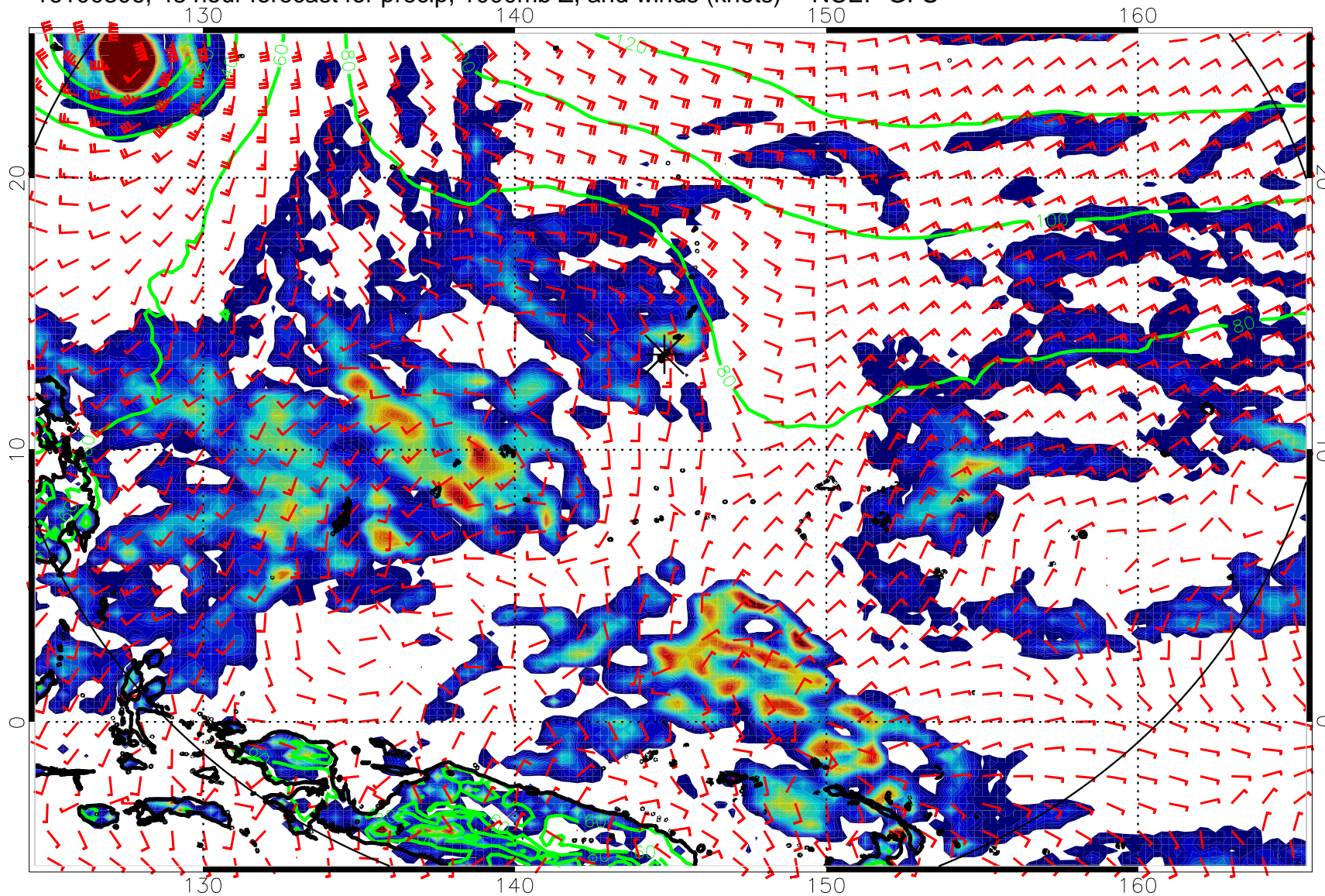
16100306, 48 hour forecast for precip, 1000mb Z, and winds (knots) -- NCEP GFS
