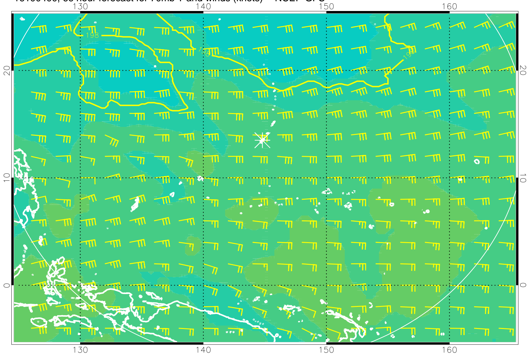
16100400, 66 hour forecast for 70mb T and winds (knots) -- NCEP GFS
