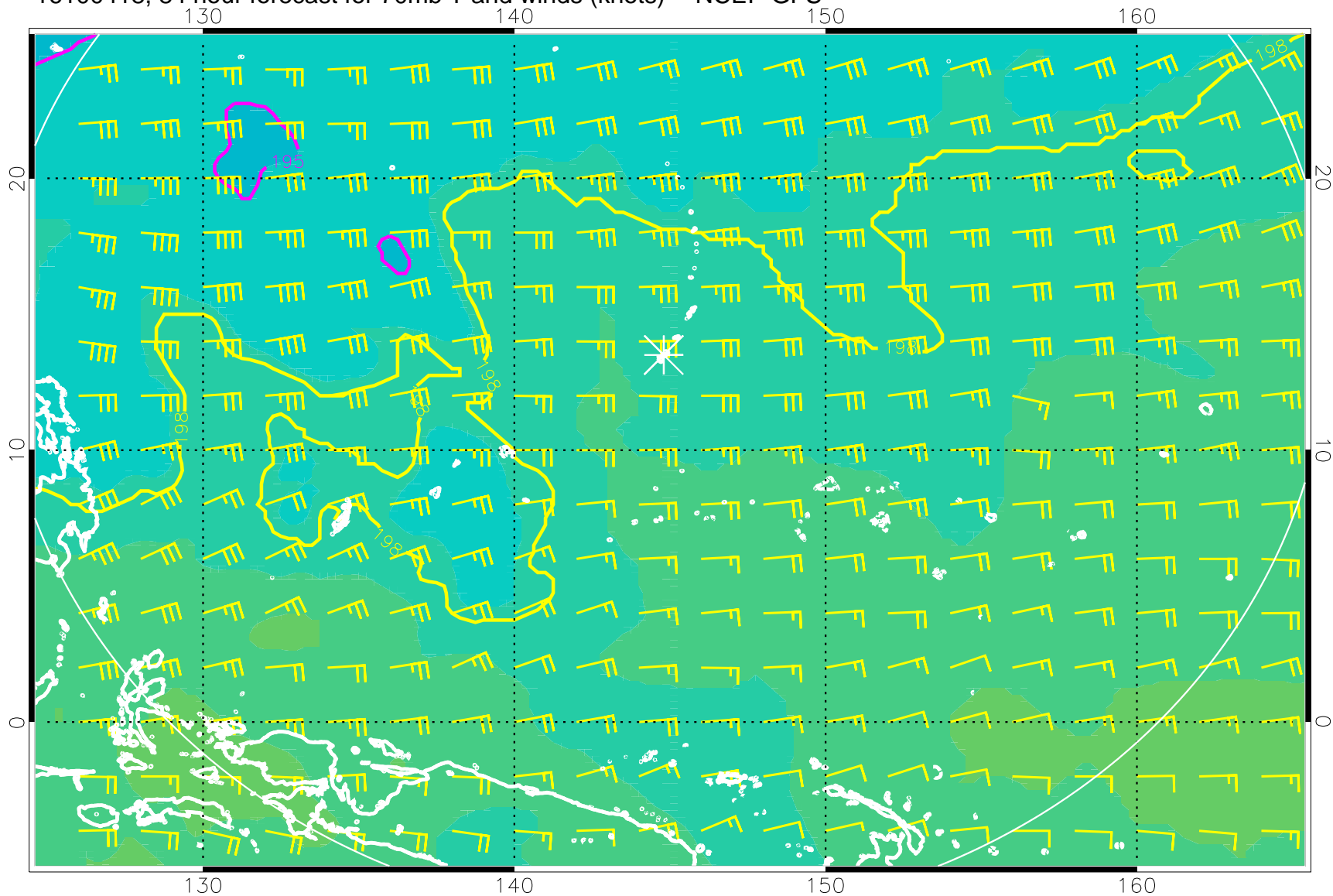
16100418, 84 hour forecast for 70mb T and winds (knots) -- NCEP GFS
