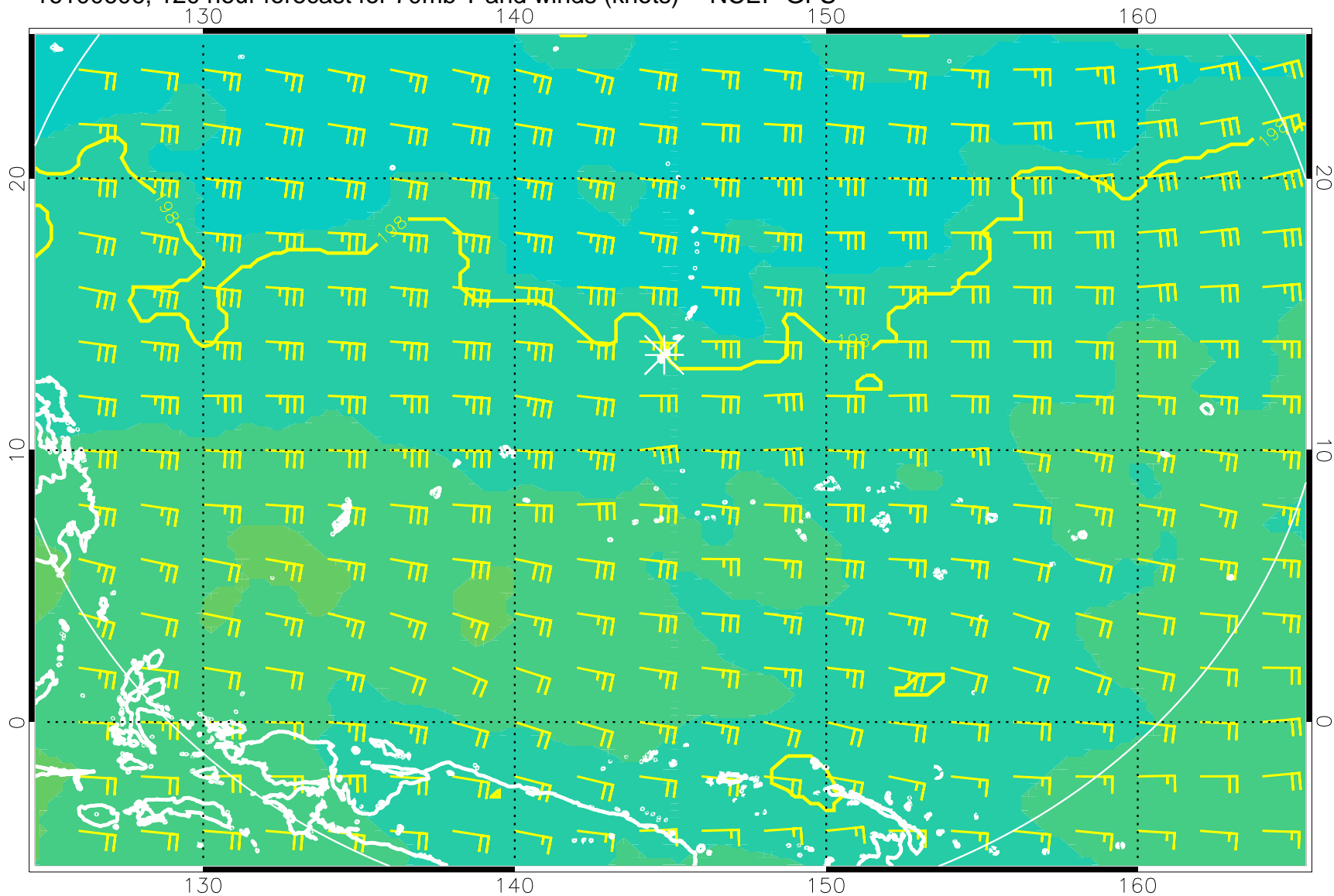
16100606, 120 hour forecast for 70mb T and winds (knots) -- NCEP GFS
