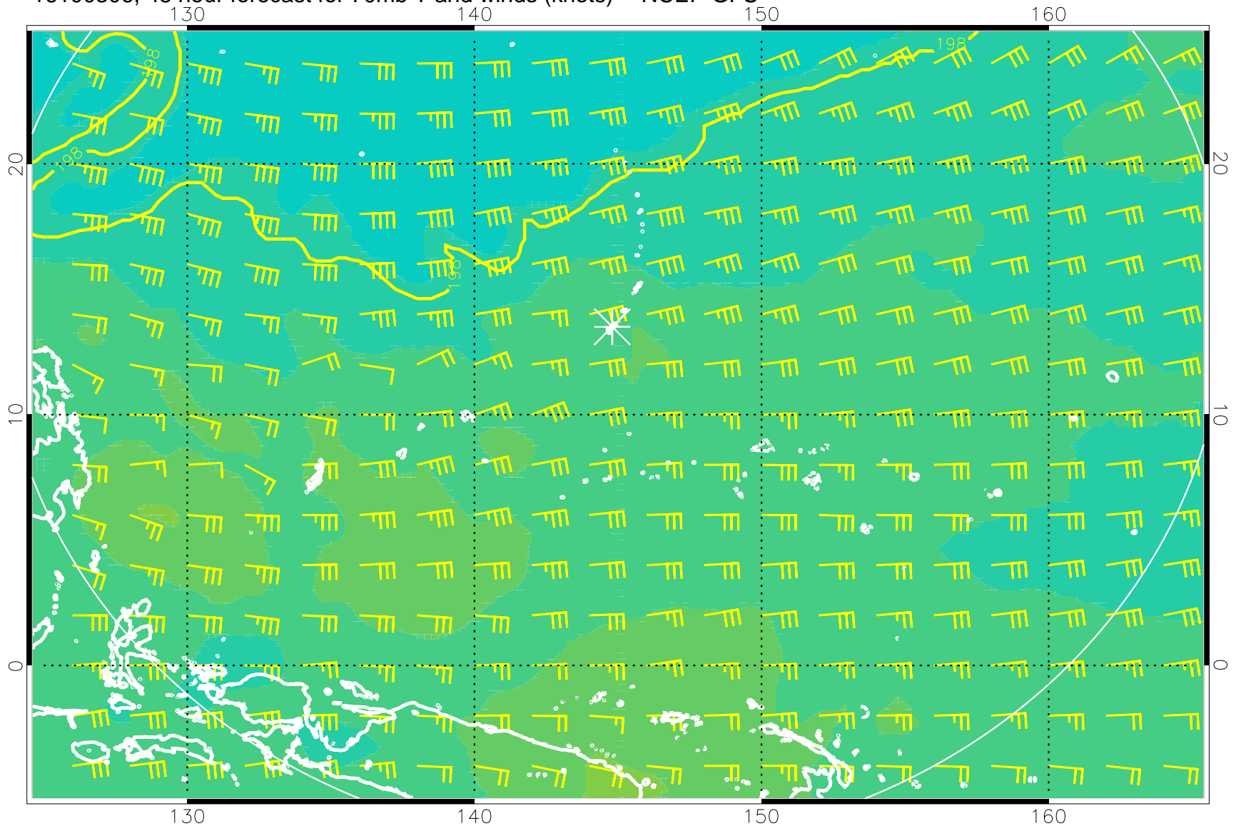
16100306, 48 hour forecast for 70mb T and winds (knots) -- NCEP GFS
