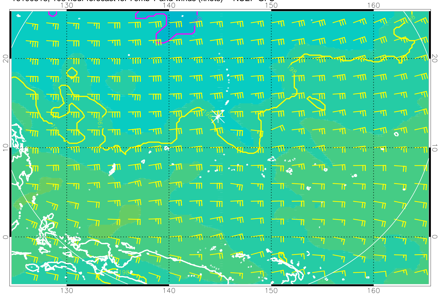
16100518, 108 hour forecast for 70mb T and winds (knots) -- NCEP GFS
