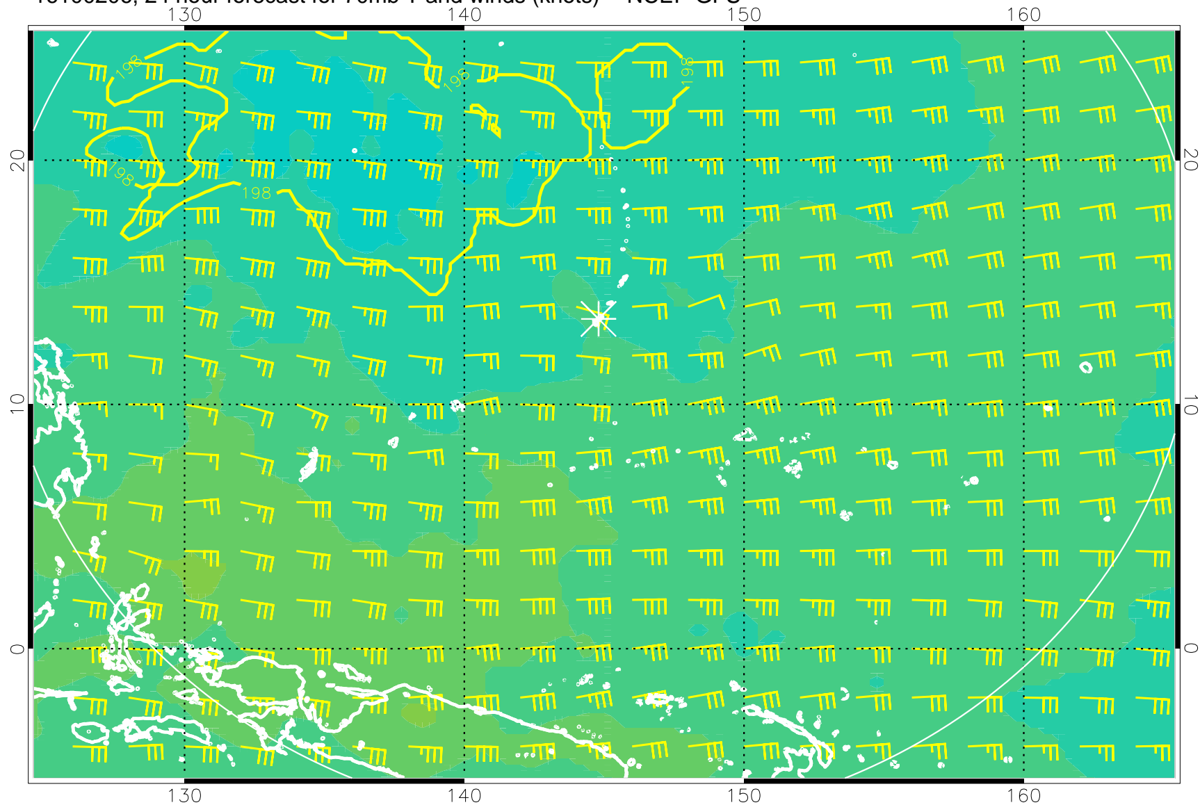
16100206, 24 hour forecast for 70mb T and winds (knots) -- NCEP GFS
