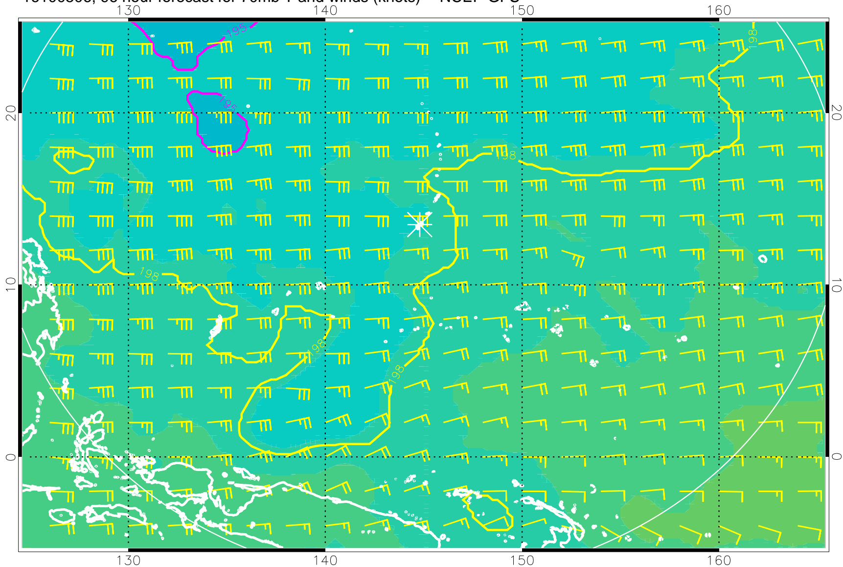
16100506, 96 hour forecast for 70mb T and winds (knots) -- NCEP GFS
