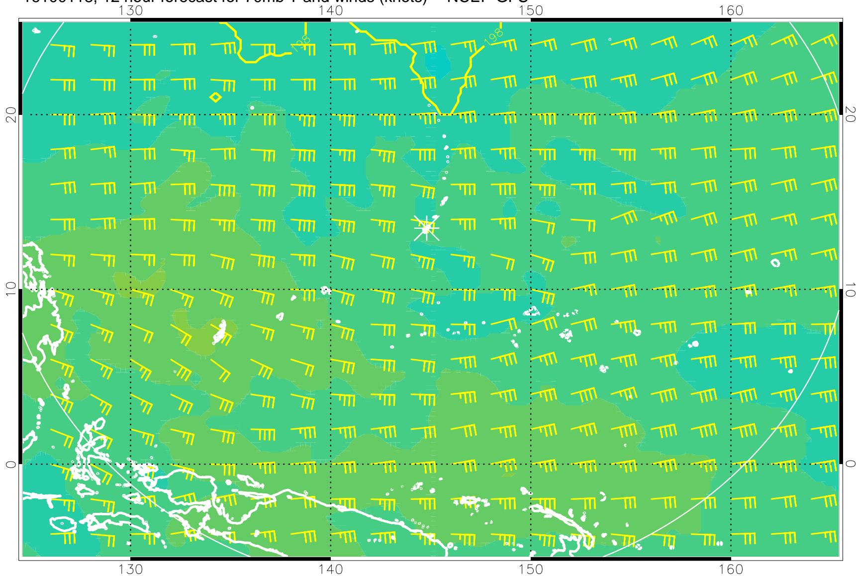
16100118, 12 hour forecast for 70mb T and winds (knots) -- NCEP GFS
