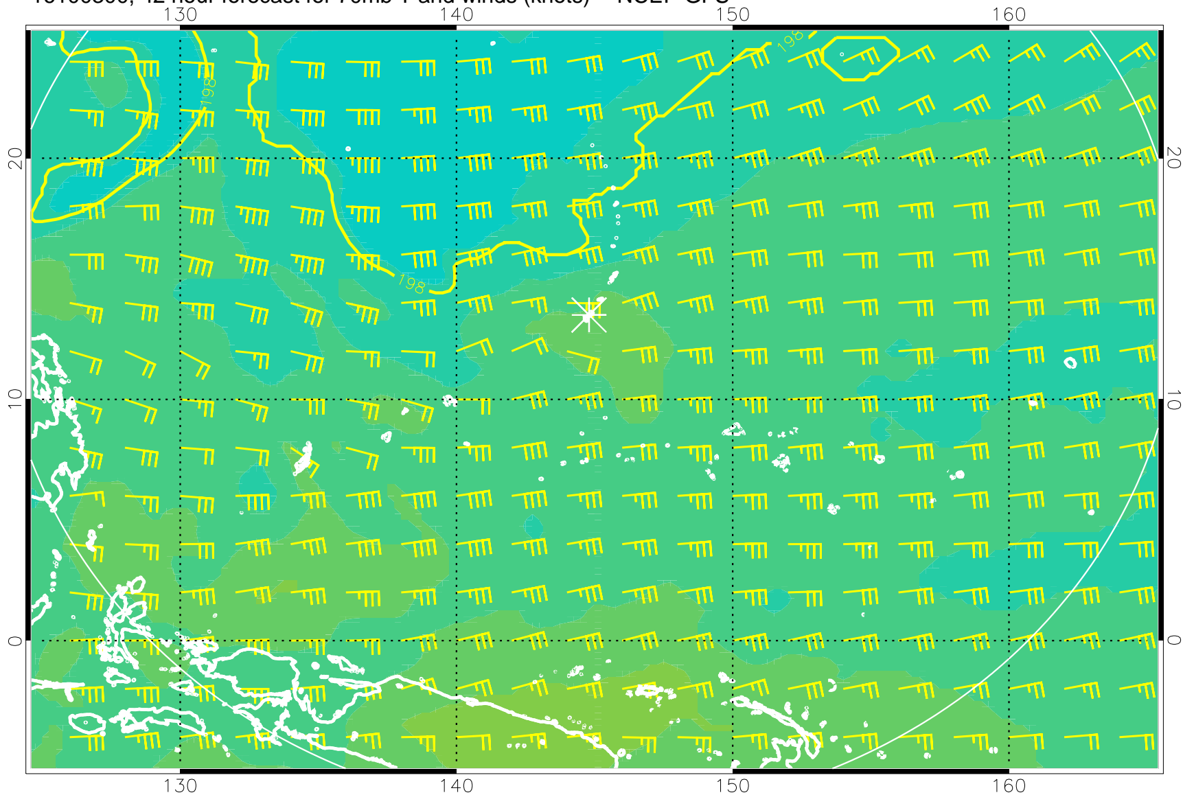
16100300, 42 hour forecast for 70mb T and winds (knots) -- NCEP GFS
