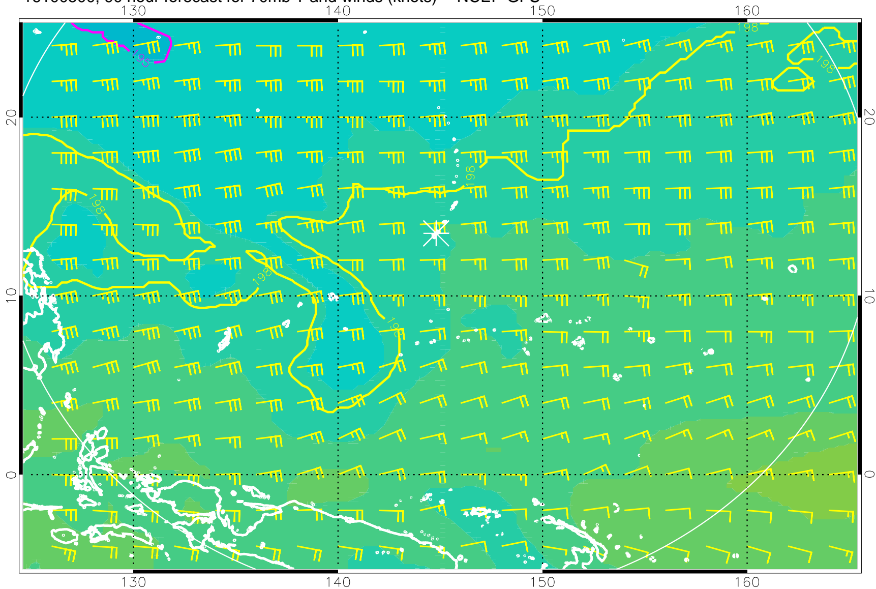
16100500, 90 hour forecast for 70mb T and winds (knots) -- NCEP GFS
