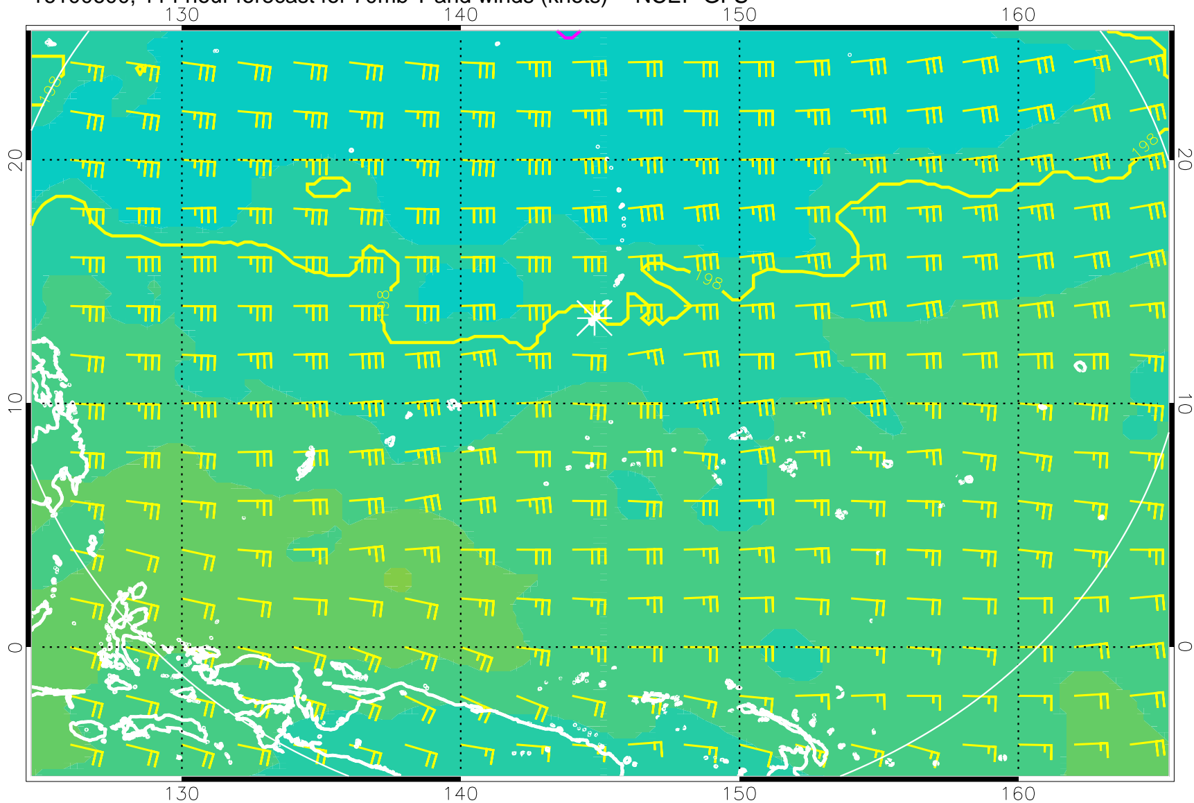
16100600, 114 hour forecast for 70mb T and winds (knots) -- NCEP GFS
