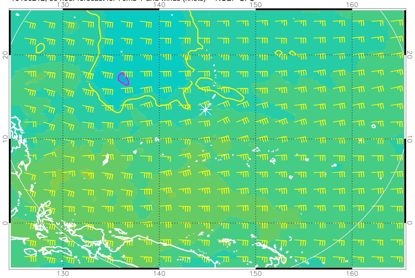
16100212, 30 hour forecast for 70mb T and winds (knots) -- NCEP GFS
