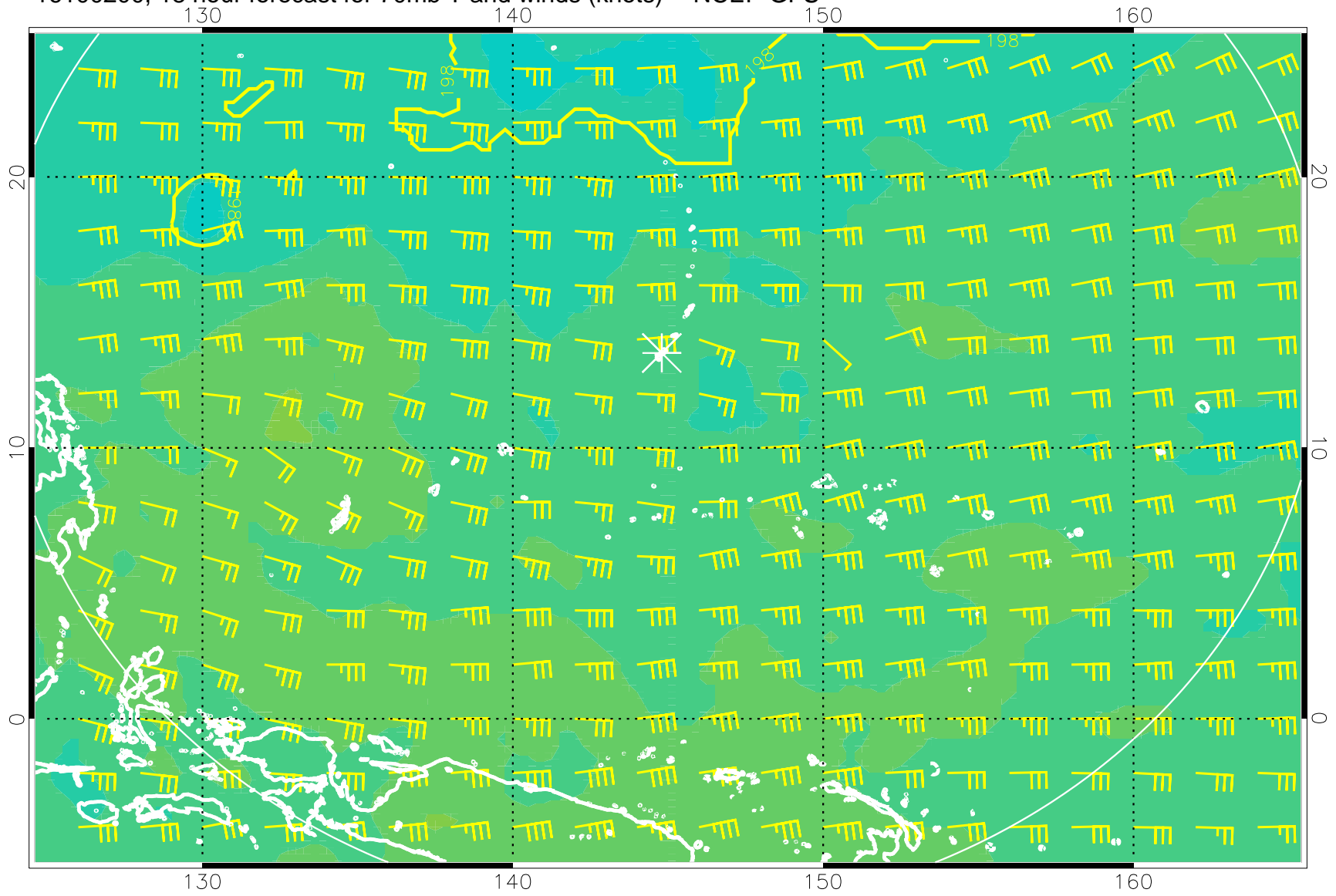
16100200, 18 hour forecast for 70mb T and winds (knots) -- NCEP GFS
