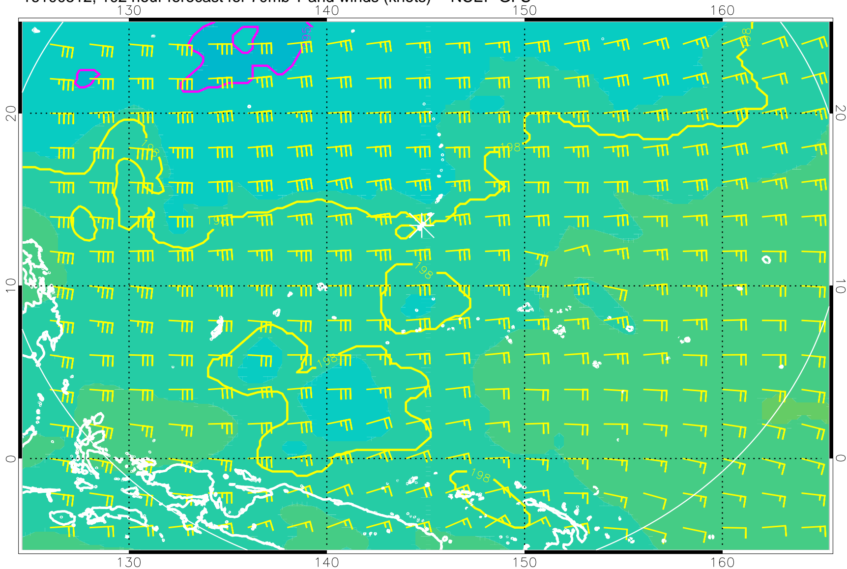
16100512, 102 hour forecast for 70mb T and winds (knots) -- NCEP GFS
