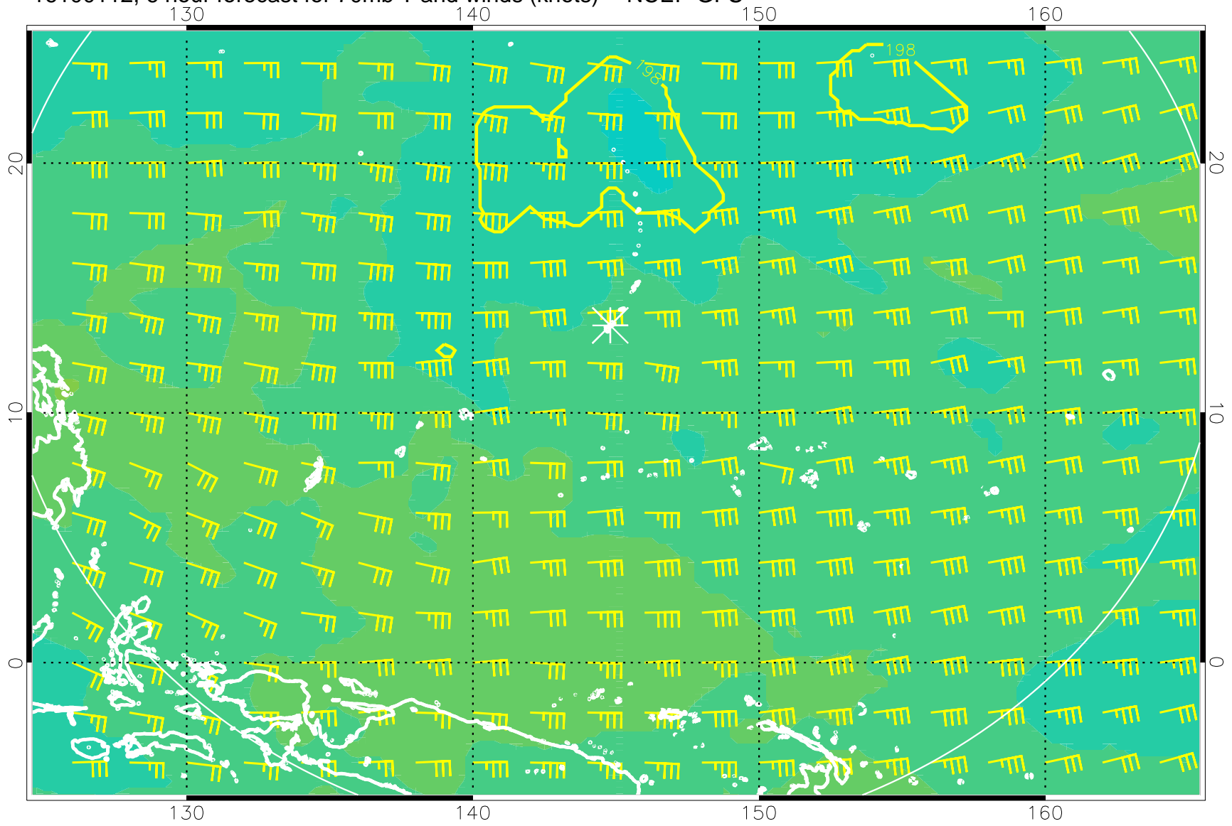
16100112, 6 hour forecast for 70mb T and winds (knots) -- NCEP GFS
