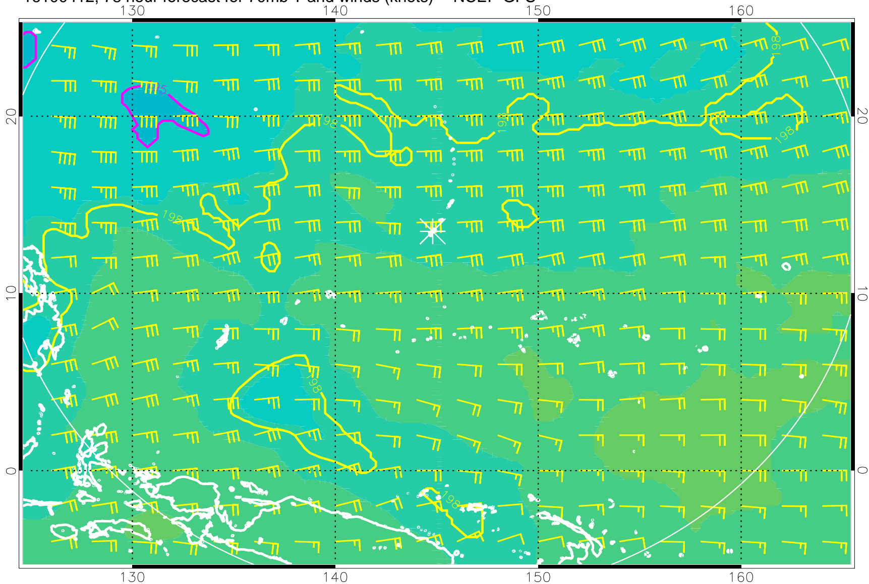
16100412, 78 hour forecast for 70mb T and winds (knots) -- NCEP GFS
