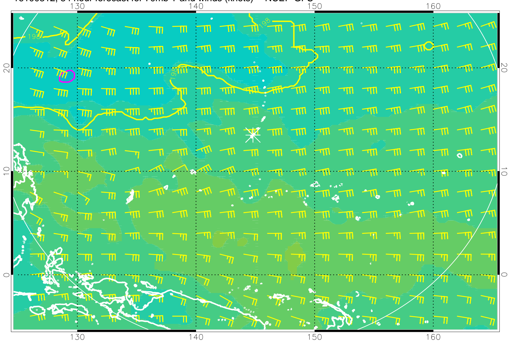
16100312, 54 hour forecast for 70mb T and winds (knots) -- NCEP GFS
