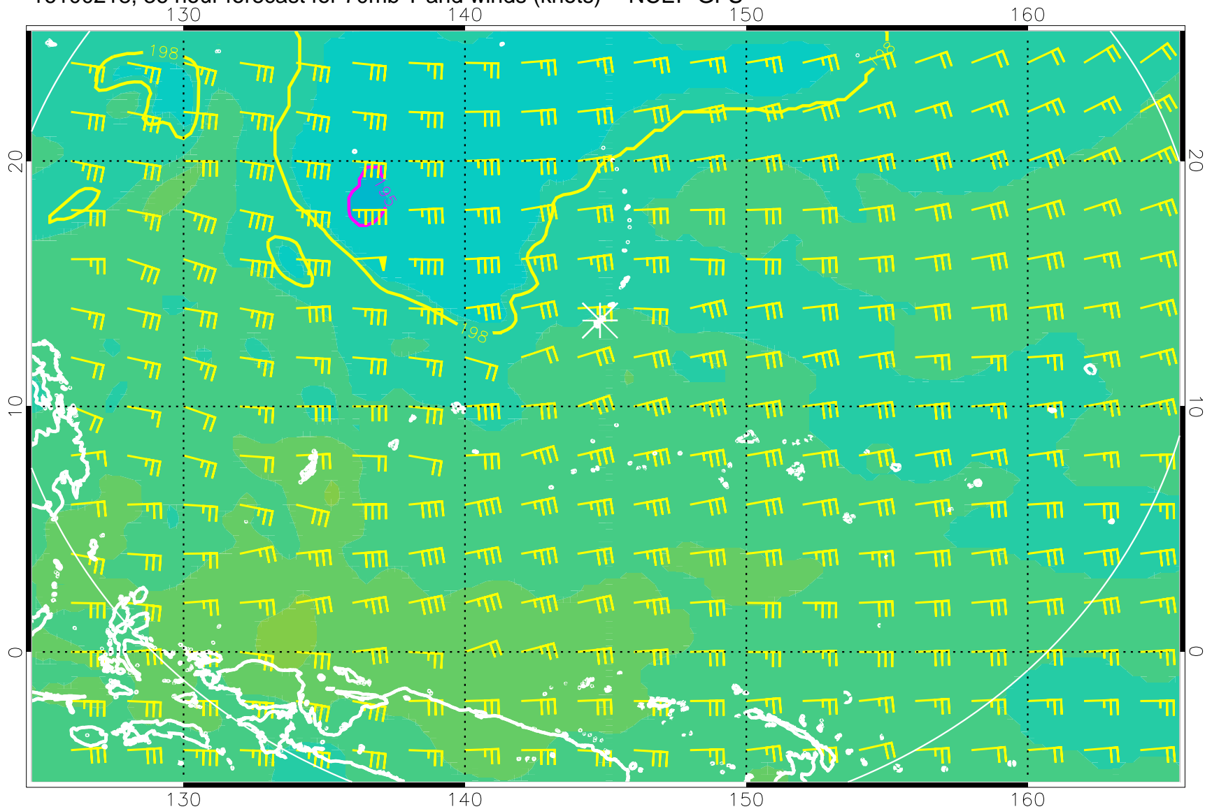
16100218, 36 hour forecast for 70mb T and winds (knots) -- NCEP GFS
