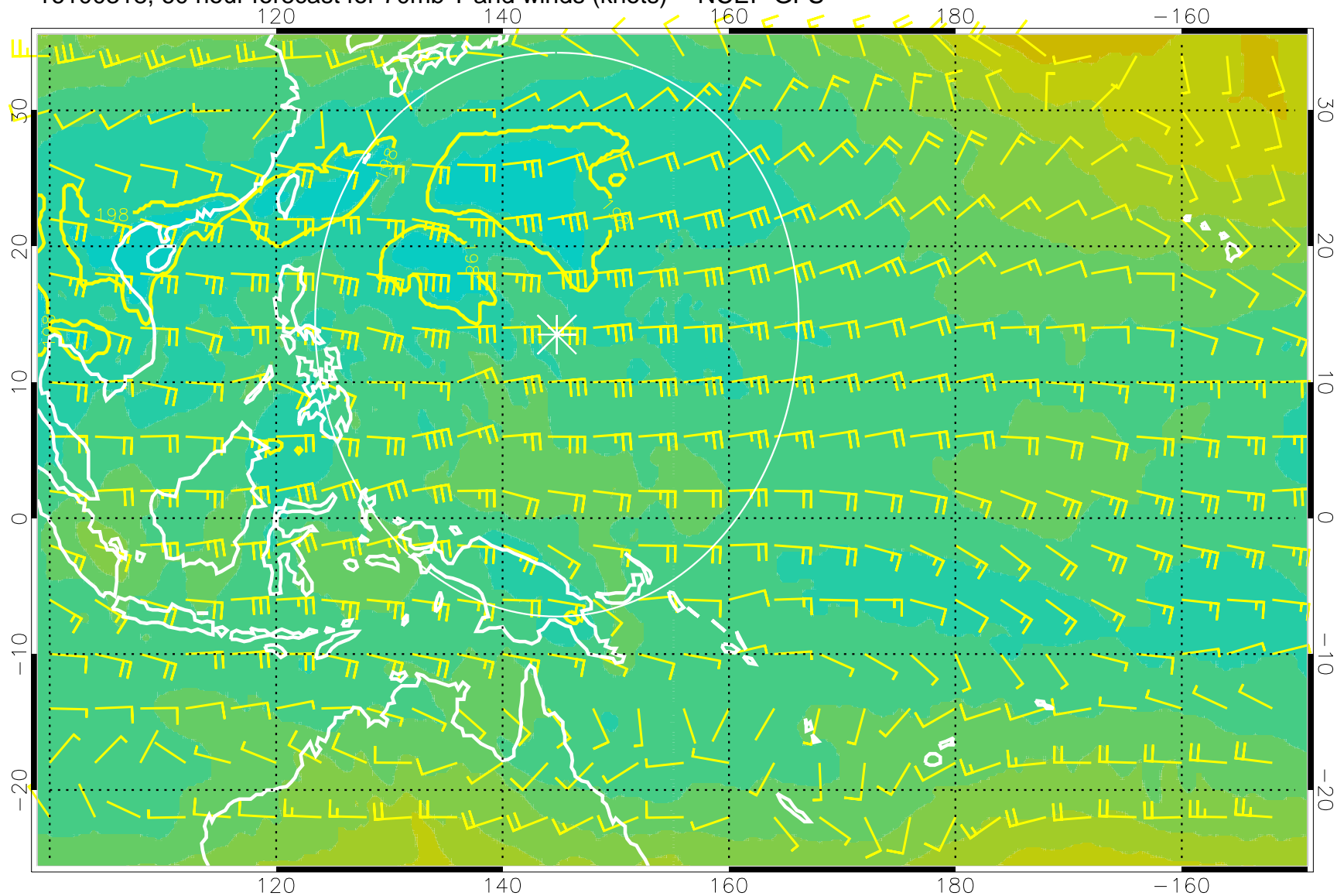
16100318, 60 hour forecast for 70mb T and winds (knots) -- NCEP GFS
