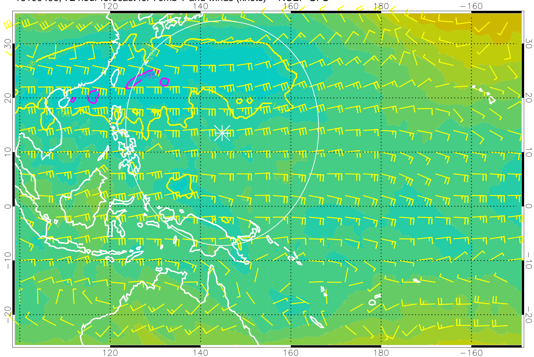
16100406, 72 hour forecast for 70mb T and winds (knots) -- NCEP GFS
