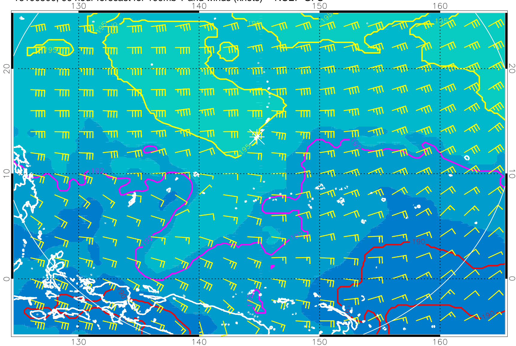
16100500, 90 hour forecast for 100mb T and winds (knots) -- NCEP GFS
