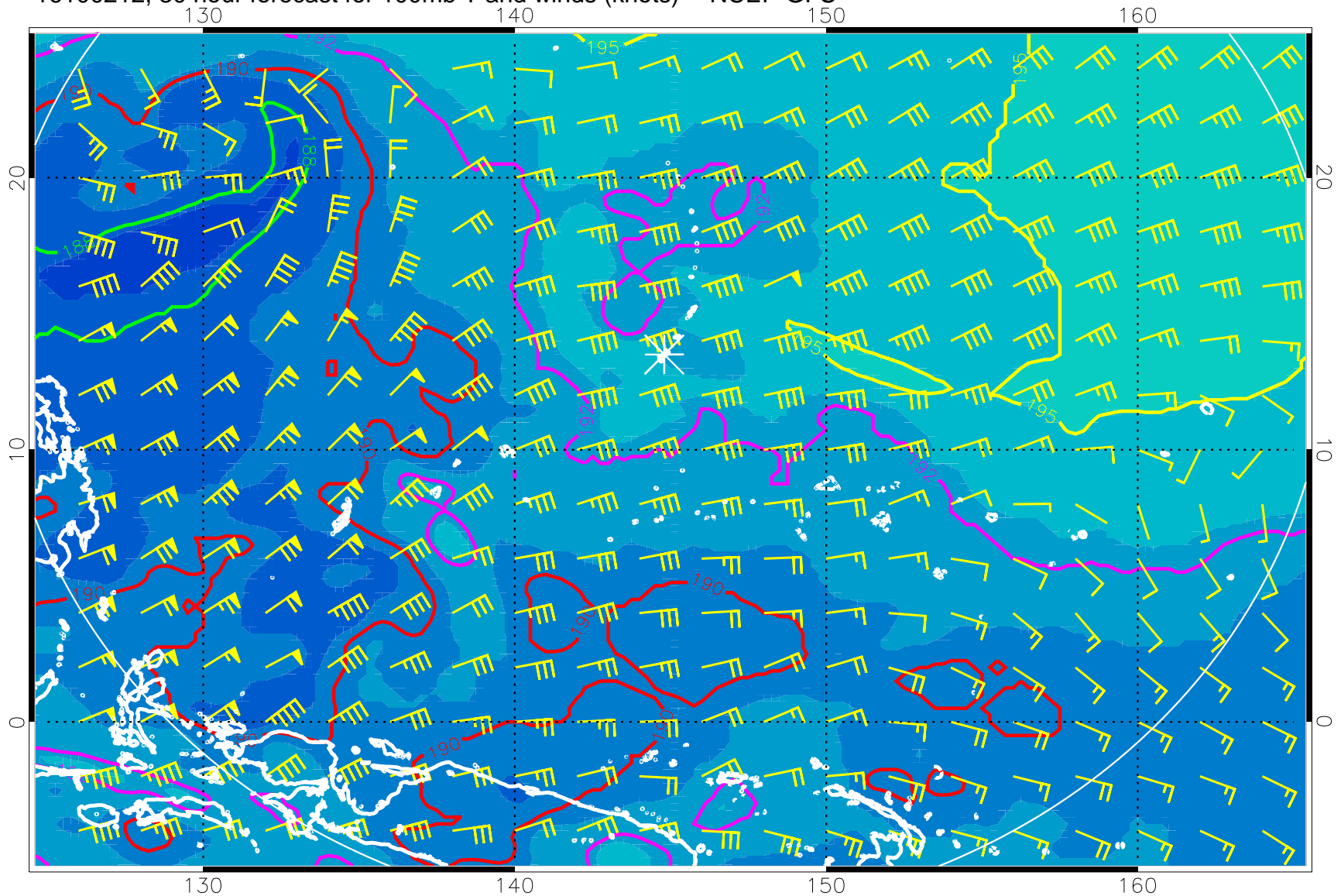
16100212, 30 hour forecast for 100mb T and winds (knots) -- NCEP GFS
