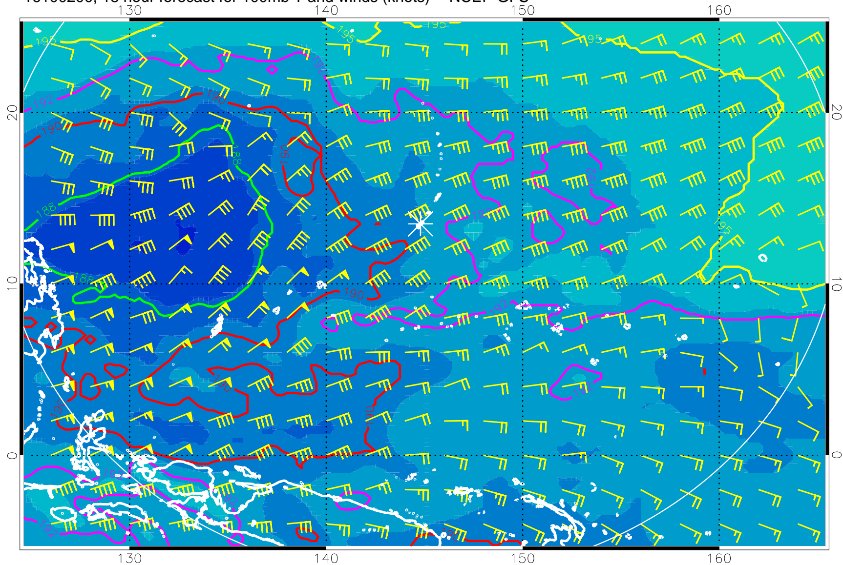
16100200, 18 hour forecast for 100mb T and winds (knots) -- NCEP GFS
