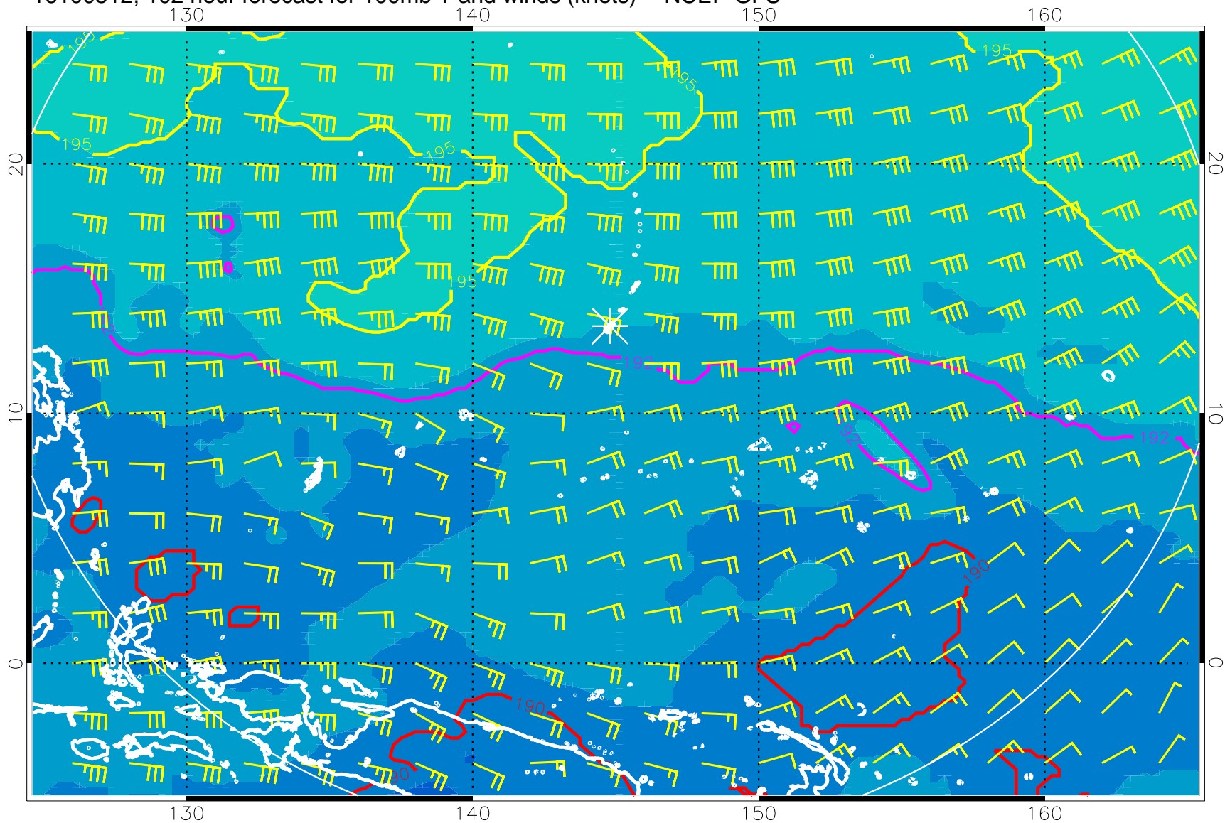
16100512, 102 hour forecast for 100mb T and winds (knots) -- NCEP GFS
