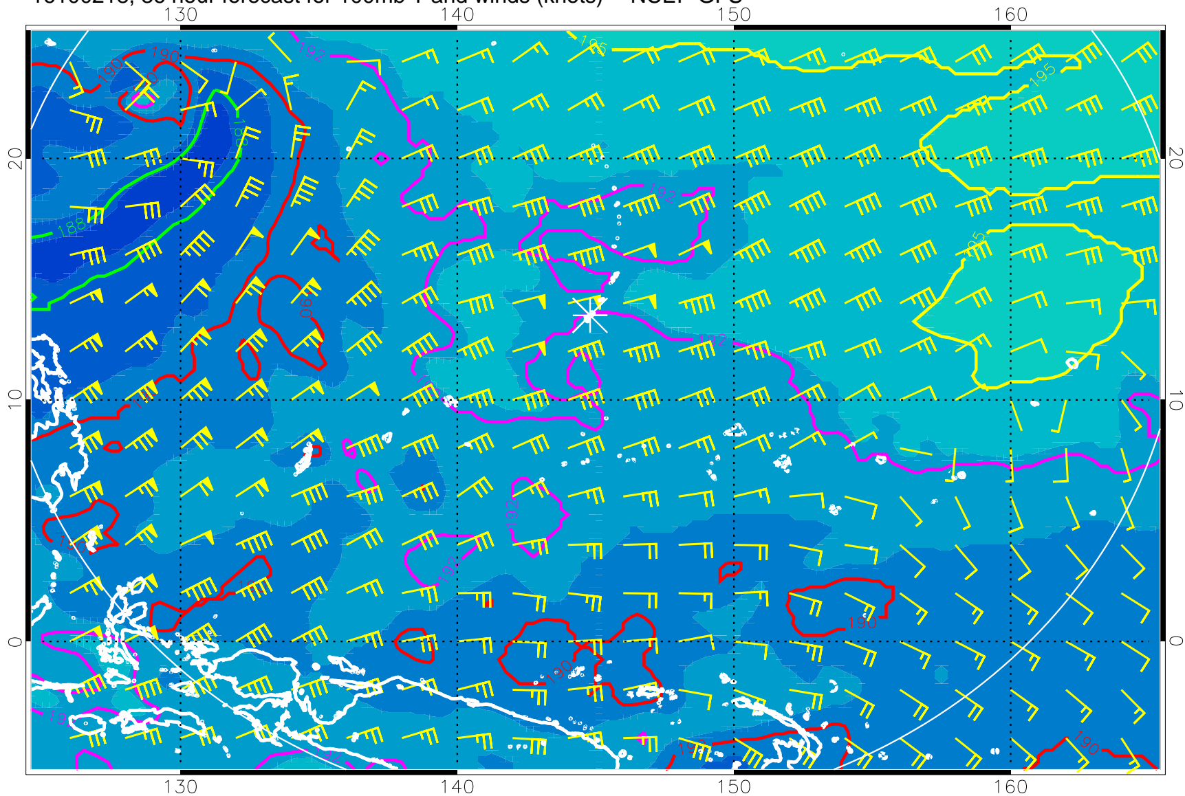
16100218, 36 hour forecast for 100mb T and winds (knots) -- NCEP GFS
