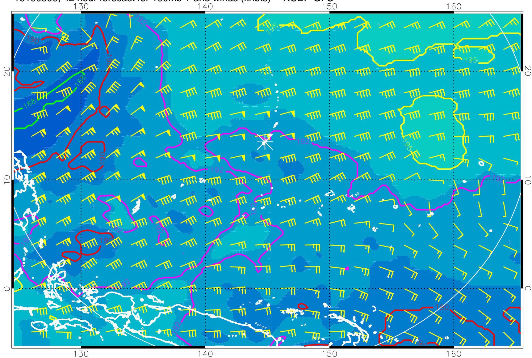
16100300, 42 hour forecast for 100mb T and winds (knots) -- NCEP GFS
