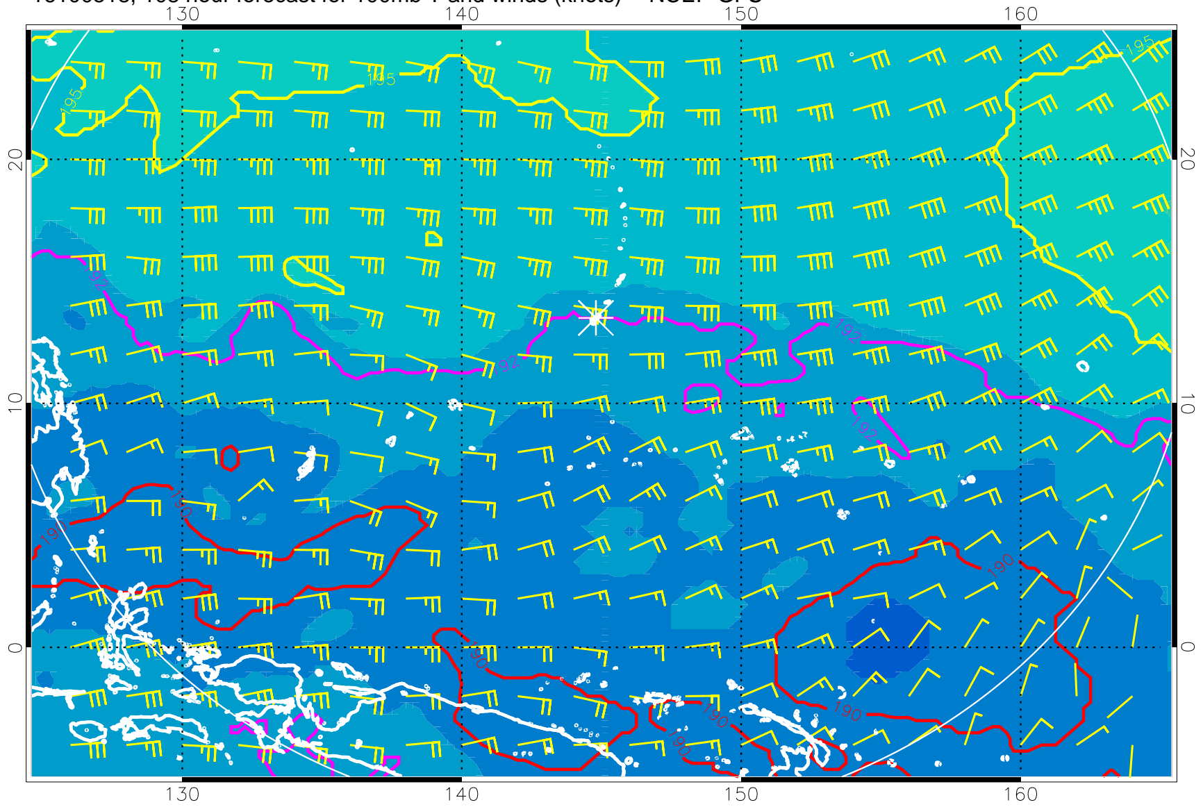
16100518, 108 hour forecast for 100mb T and winds (knots) -- NCEP GFS
