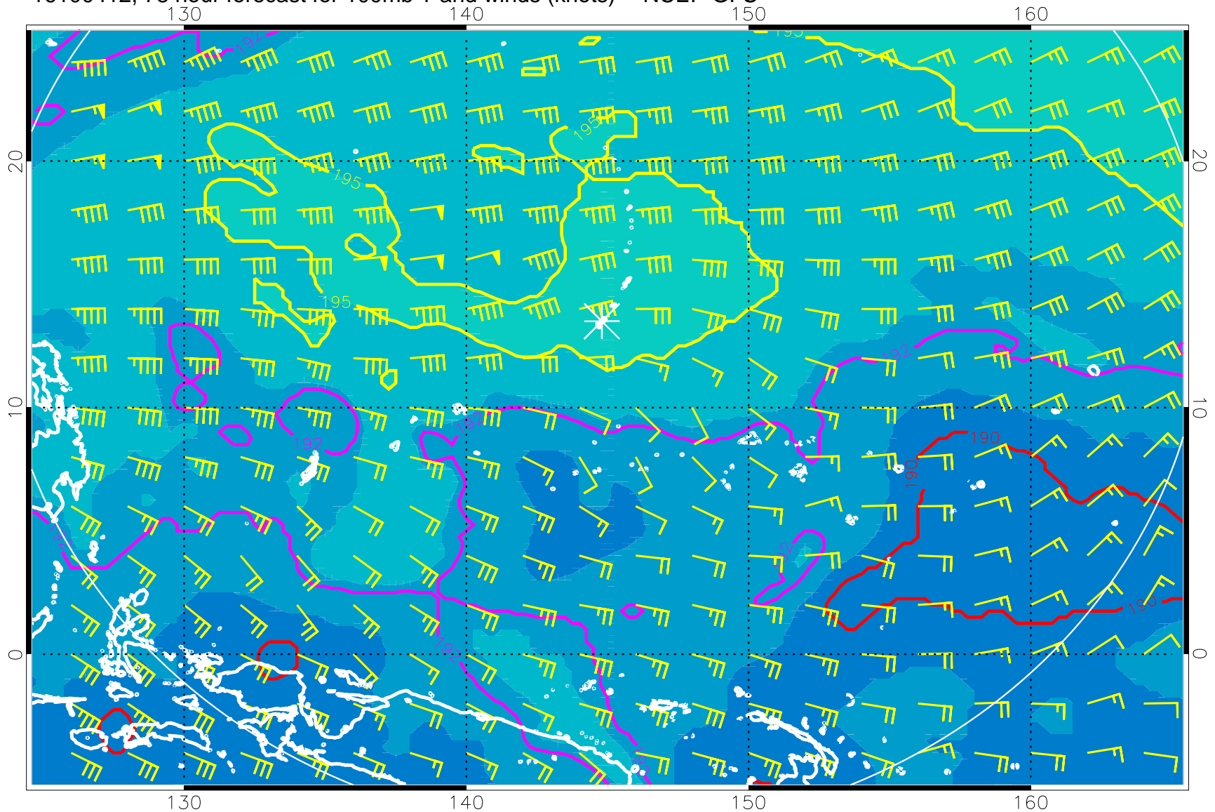
16100412, 78 hour forecast for 100mb T and winds (knots) -- NCEP GFS
