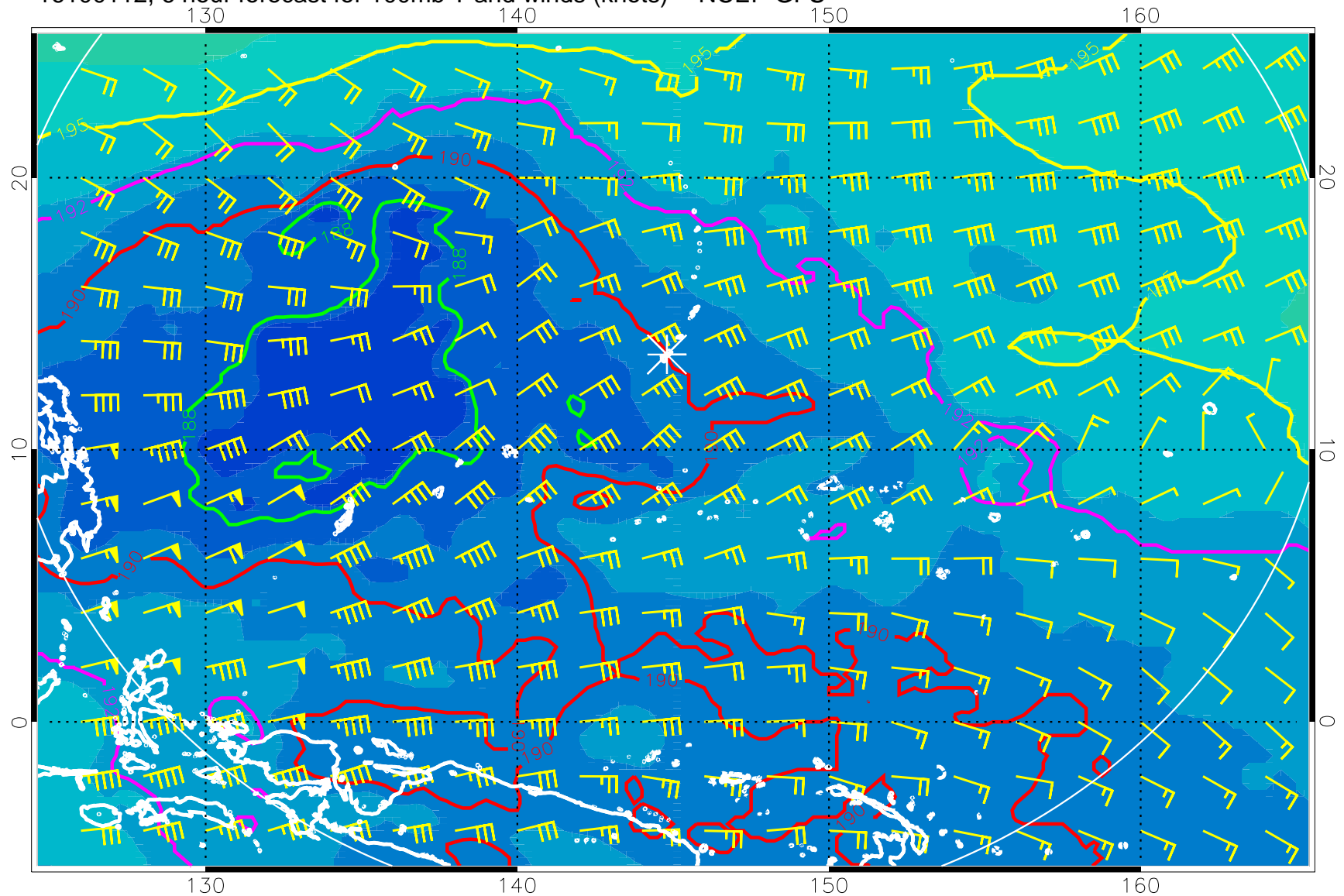
16100112, 6 hour forecast for 100mb T and winds (knots) -- NCEP GFS
