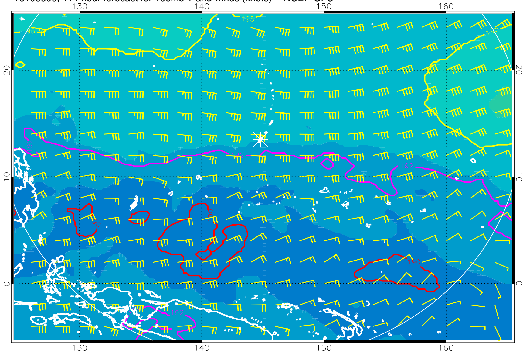
16100600, 114 hour forecast for 100mb T and winds (knots) -- NCEP GFS
