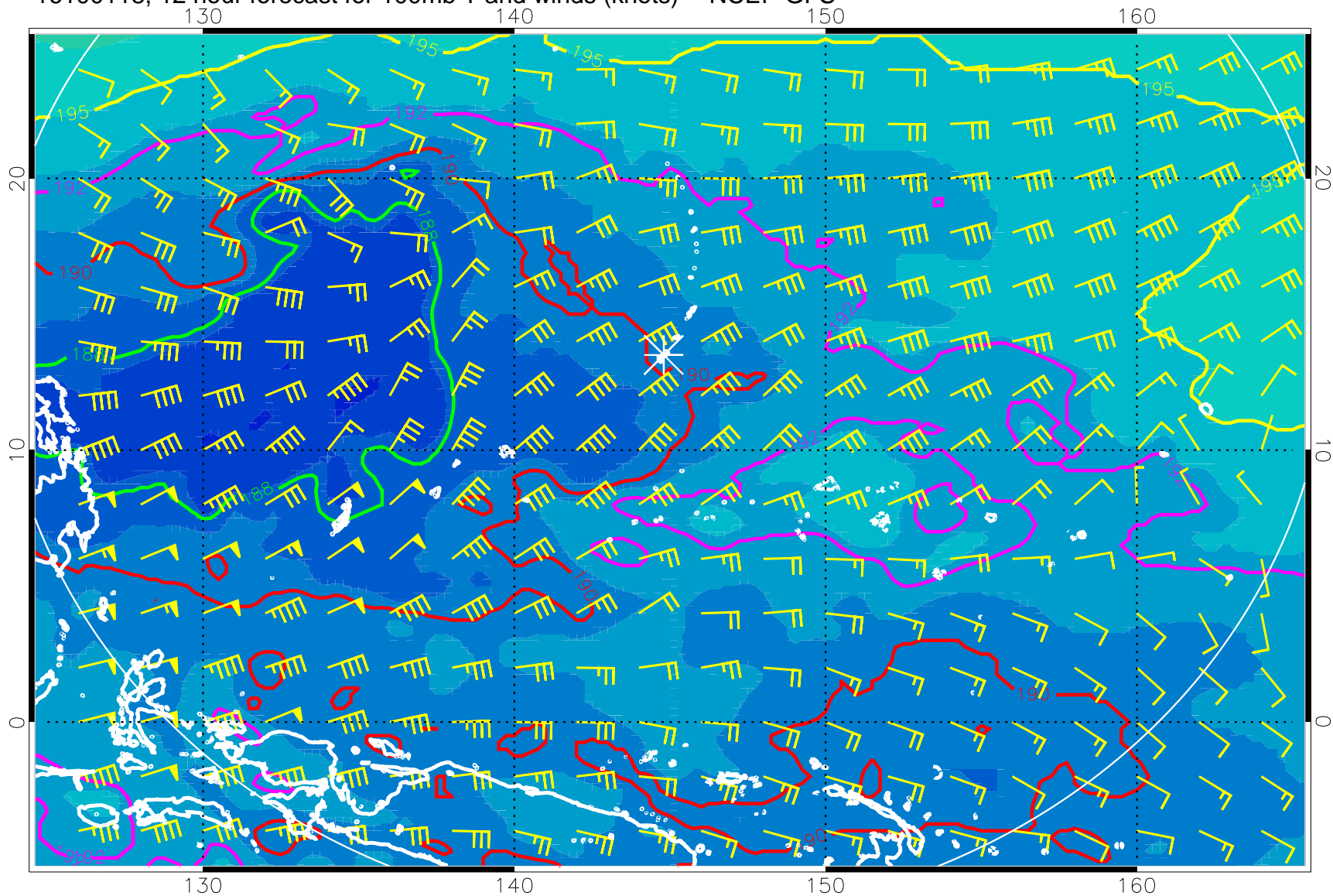
16100118, 12 hour forecast for 100mb T and winds (knots) -- NCEP GFS
