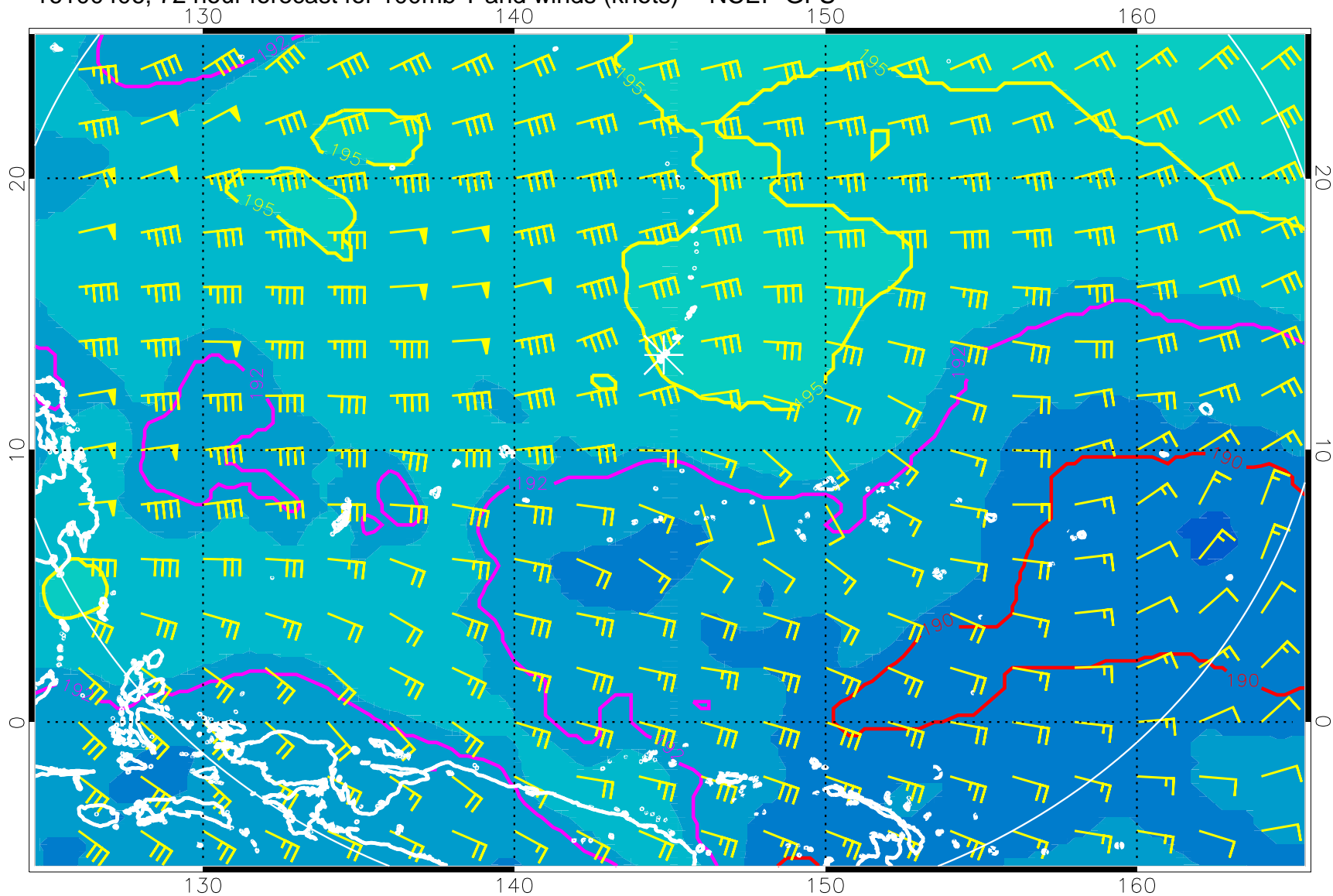
16100406, 72 hour forecast for 100mb T and winds (knots) -- NCEP GFS
