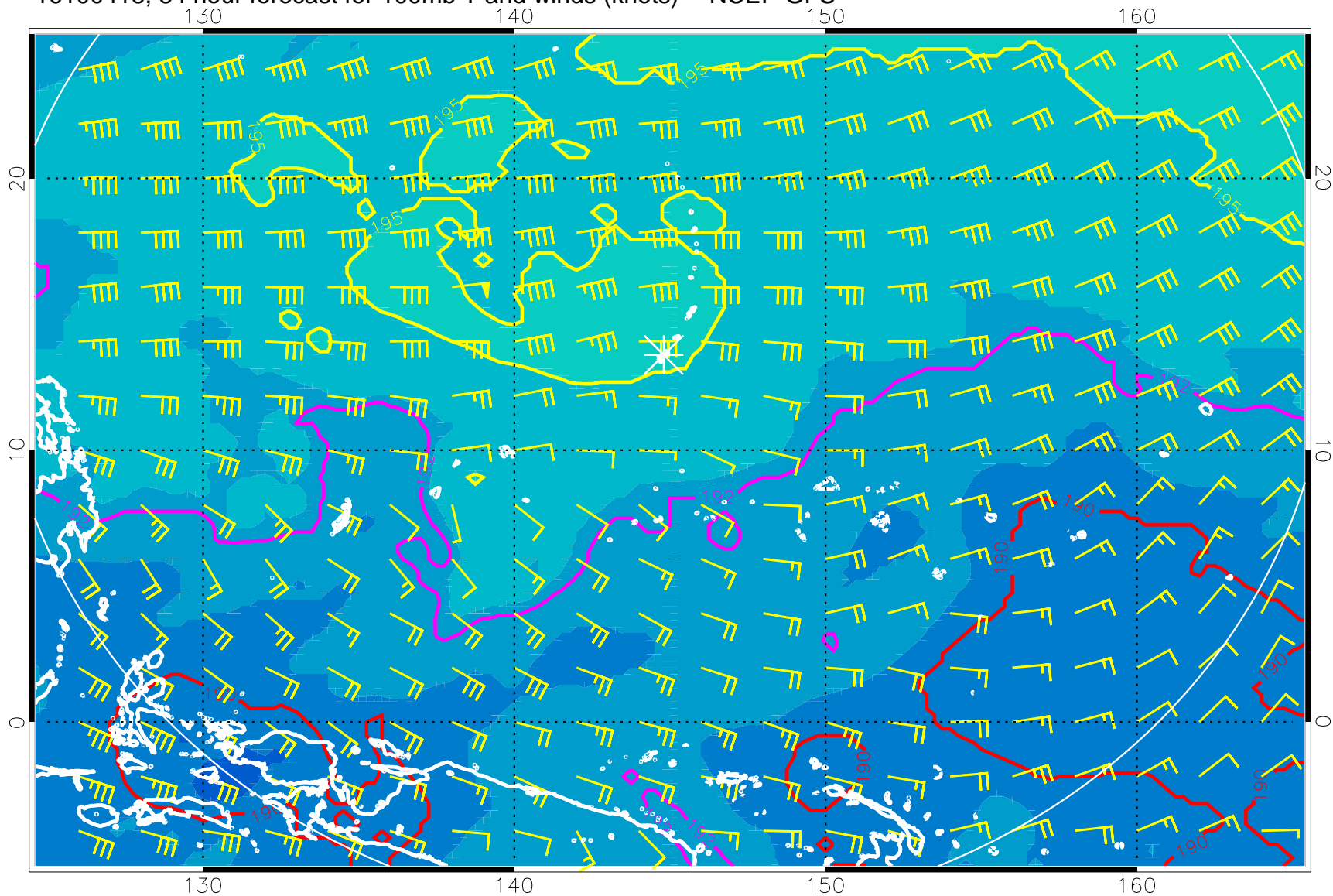
16100418, 84 hour forecast for 100mb T and winds (knots) -- NCEP GFS
