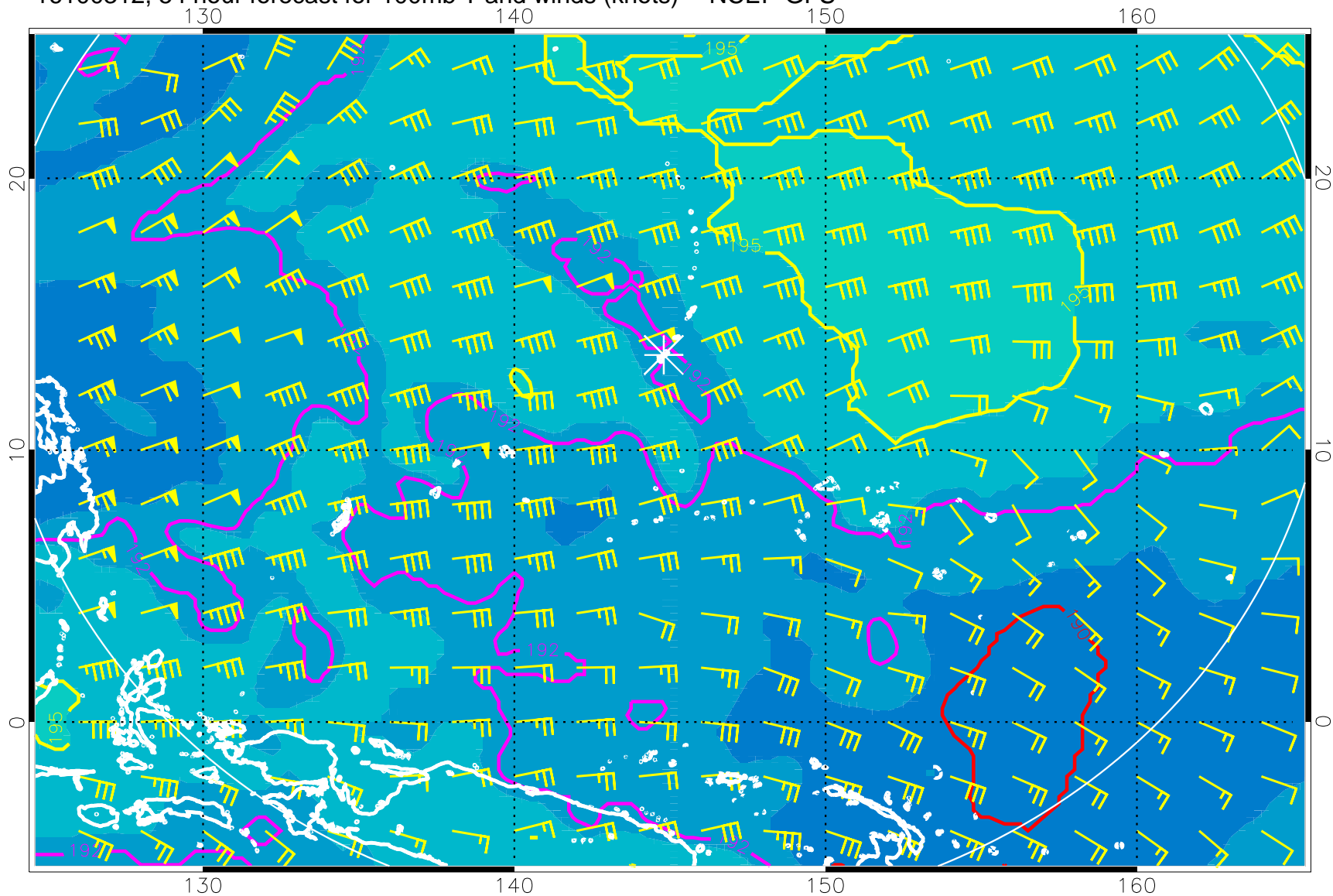
16100312, 54 hour forecast for 100mb T and winds (knots) -- NCEP GFS
