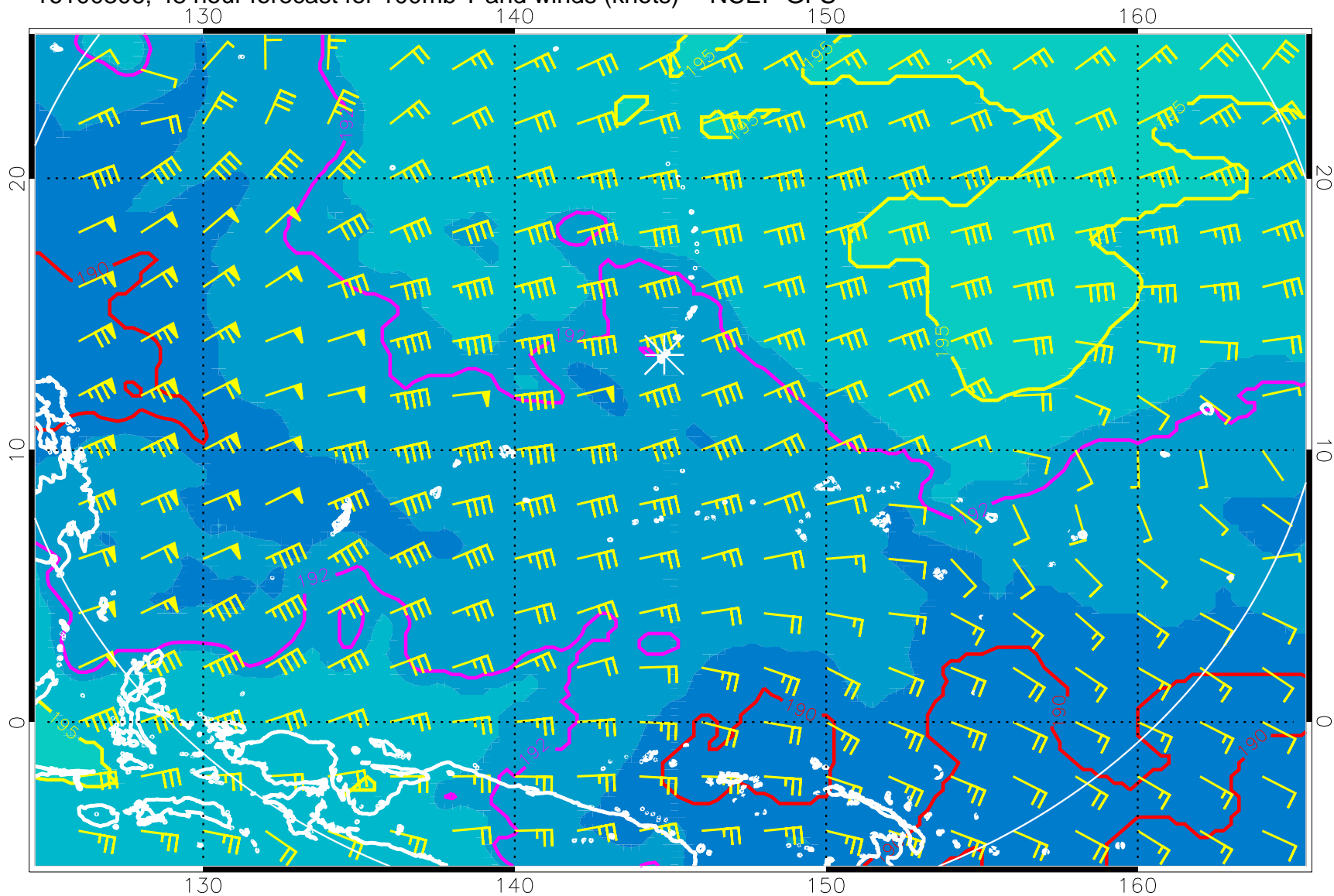
16100306, 48 hour forecast for 100mb T and winds (knots) -- NCEP GFS
