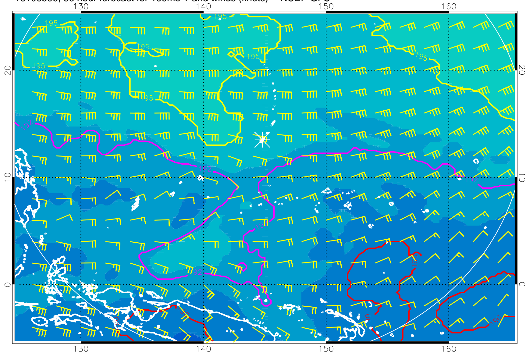
16100506, 96 hour forecast for 100mb T and winds (knots) -- NCEP GFS
