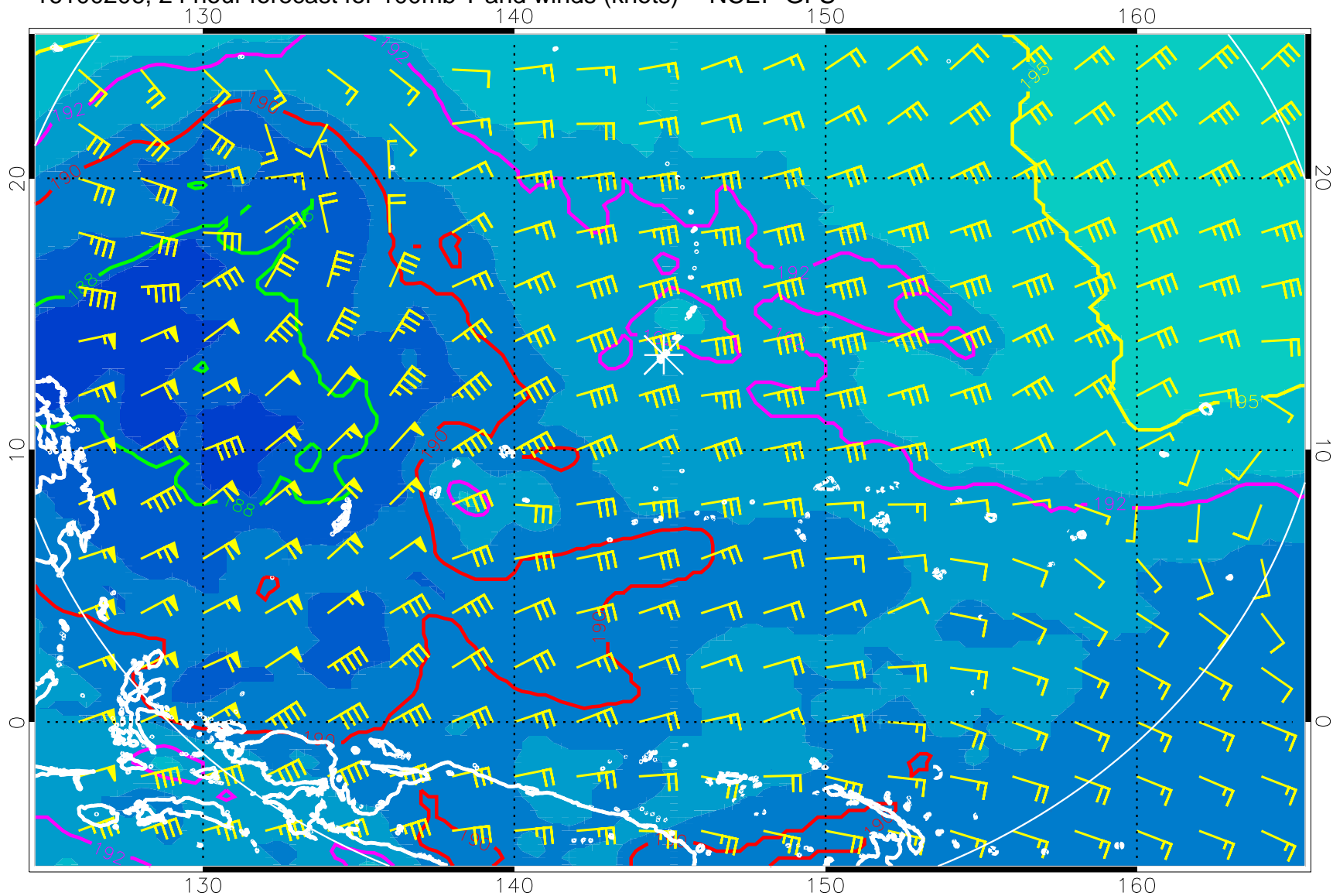
16100206, 24 hour forecast for 100mb T and winds (knots) -- NCEP GFS
