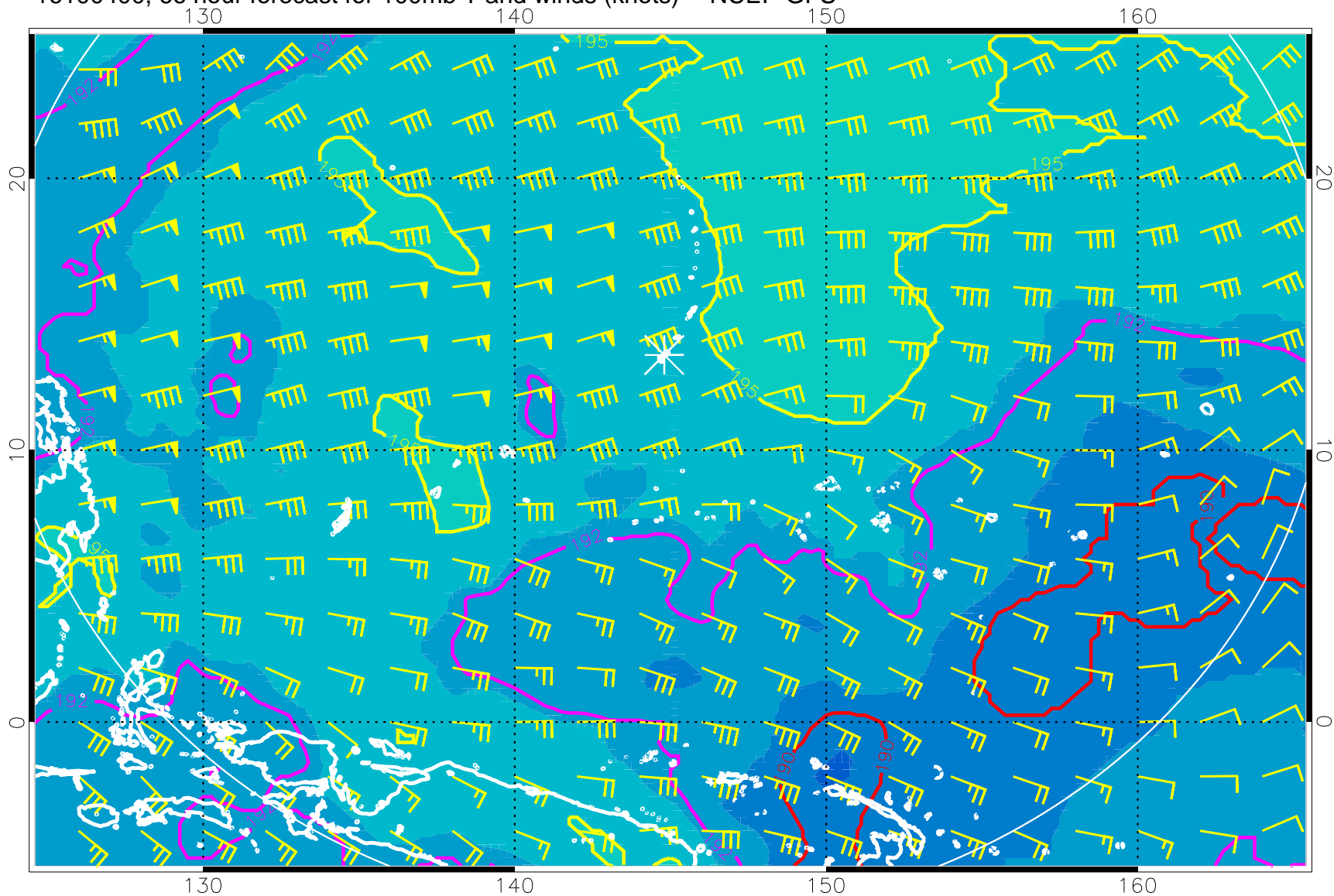
16100400, 66 hour forecast for 100mb T and winds (knots) -- NCEP GFS
