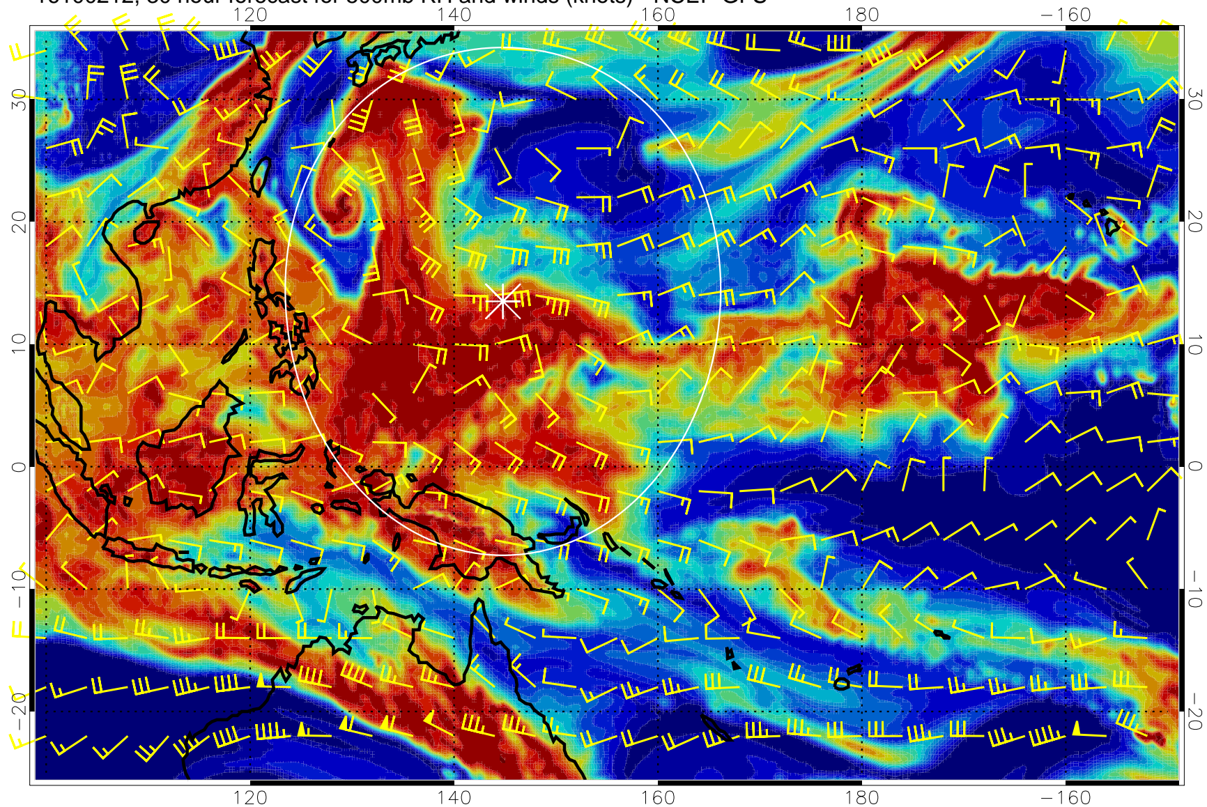
16100212, 30 hour forecast for 500mb RH and winds (knots) - NCEP GFS
