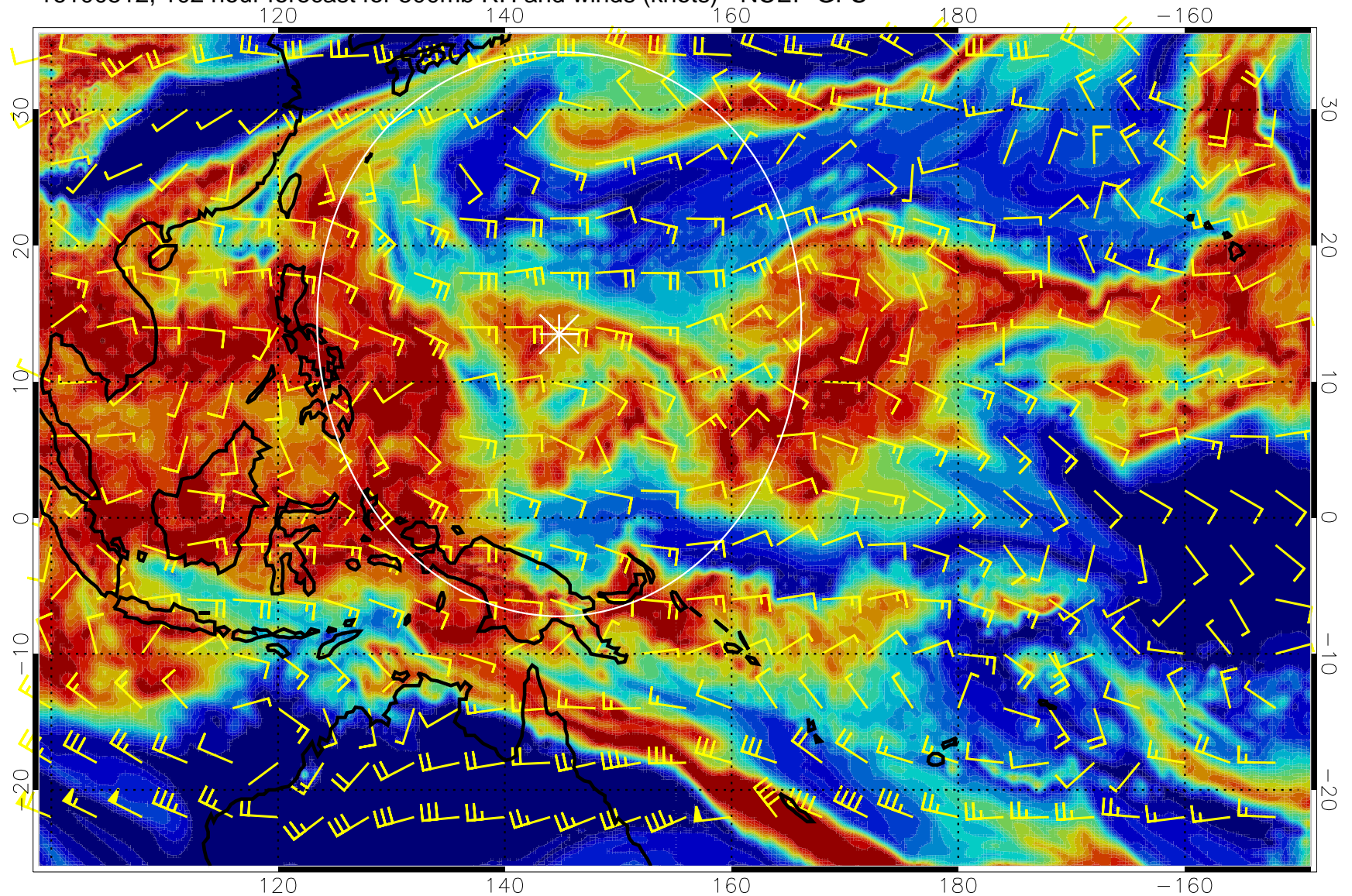
16100512, 102 hour forecast for 500mb RH and winds (knots) - NCEP GFS
