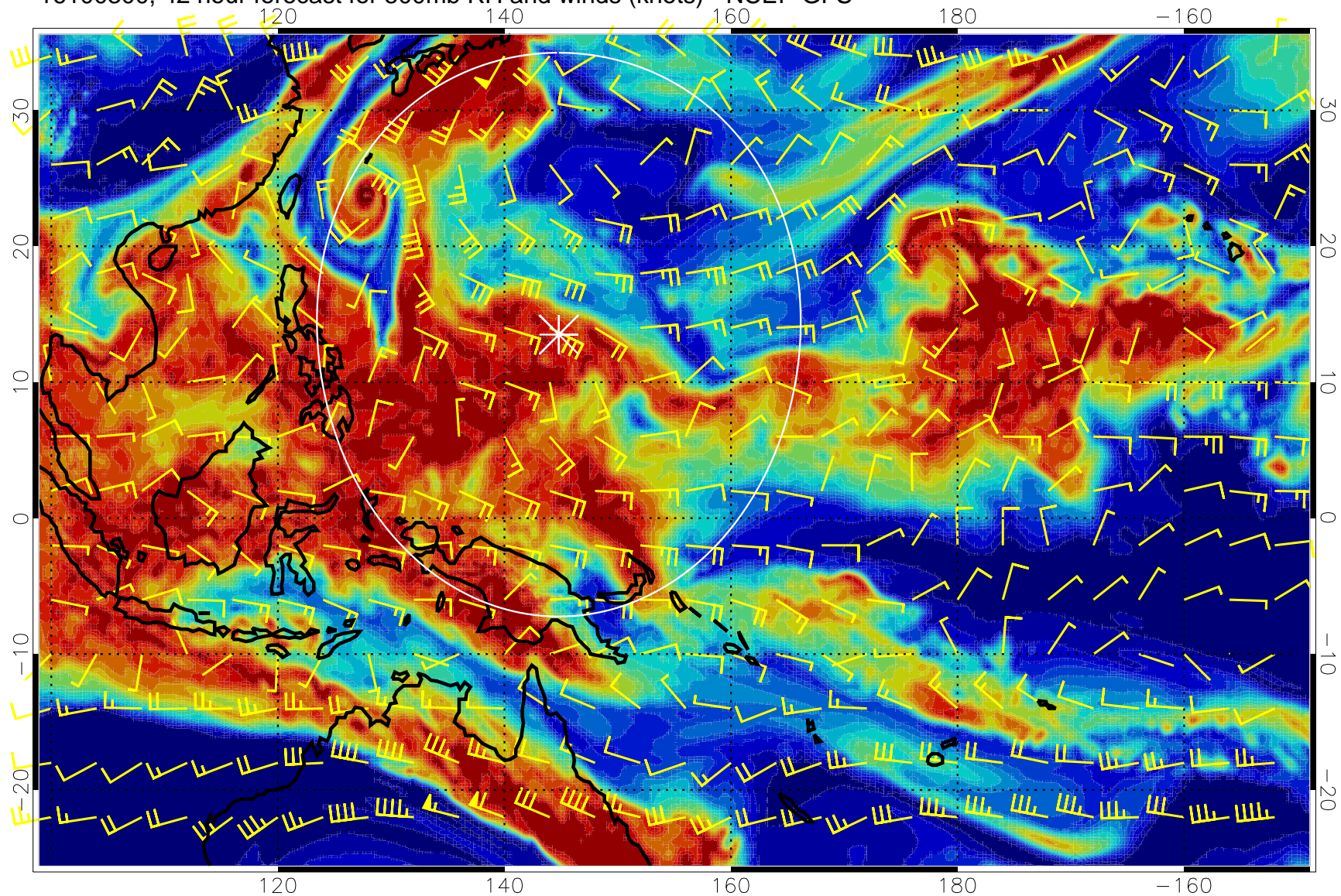
16100300, 42 hour forecast for 500mb RH and winds (knots) - NCEP GFS
