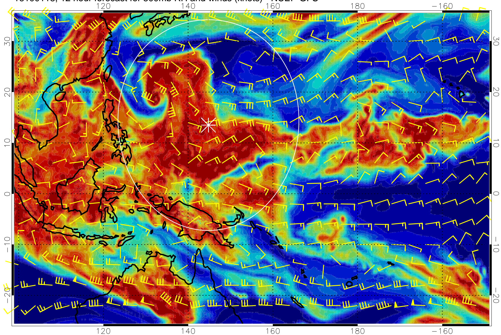
16100118, 12 hour forecast for 500mb RH and winds (knots) - NCEP GFS
