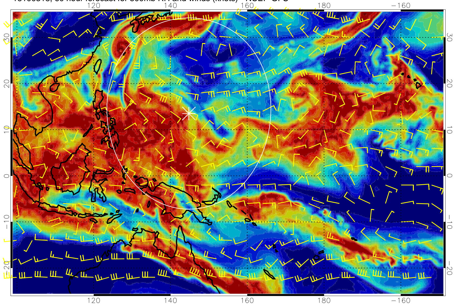
16100318, 60 hour forecast for 500mb RH and winds (knots) - NCEP GFS
