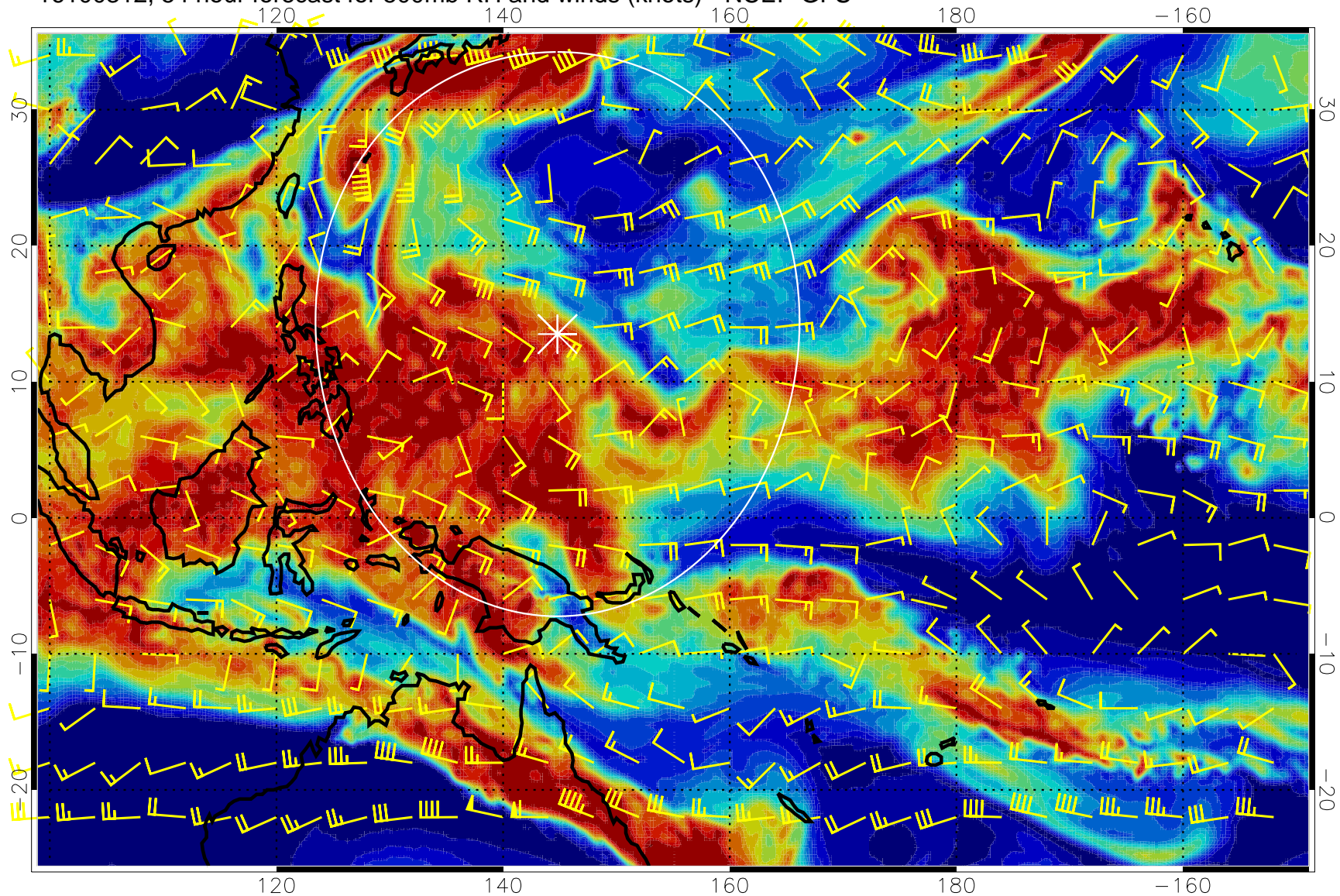
16100312, 54 hour forecast for 500mb RH and winds (knots) - NCEP GFS
