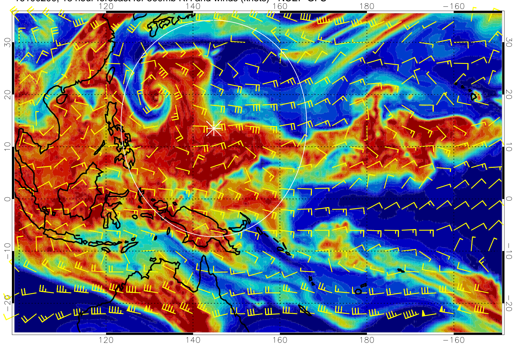
16100200, 18 hour forecast for 500mb RH and winds (knots) - NCEP GFS
