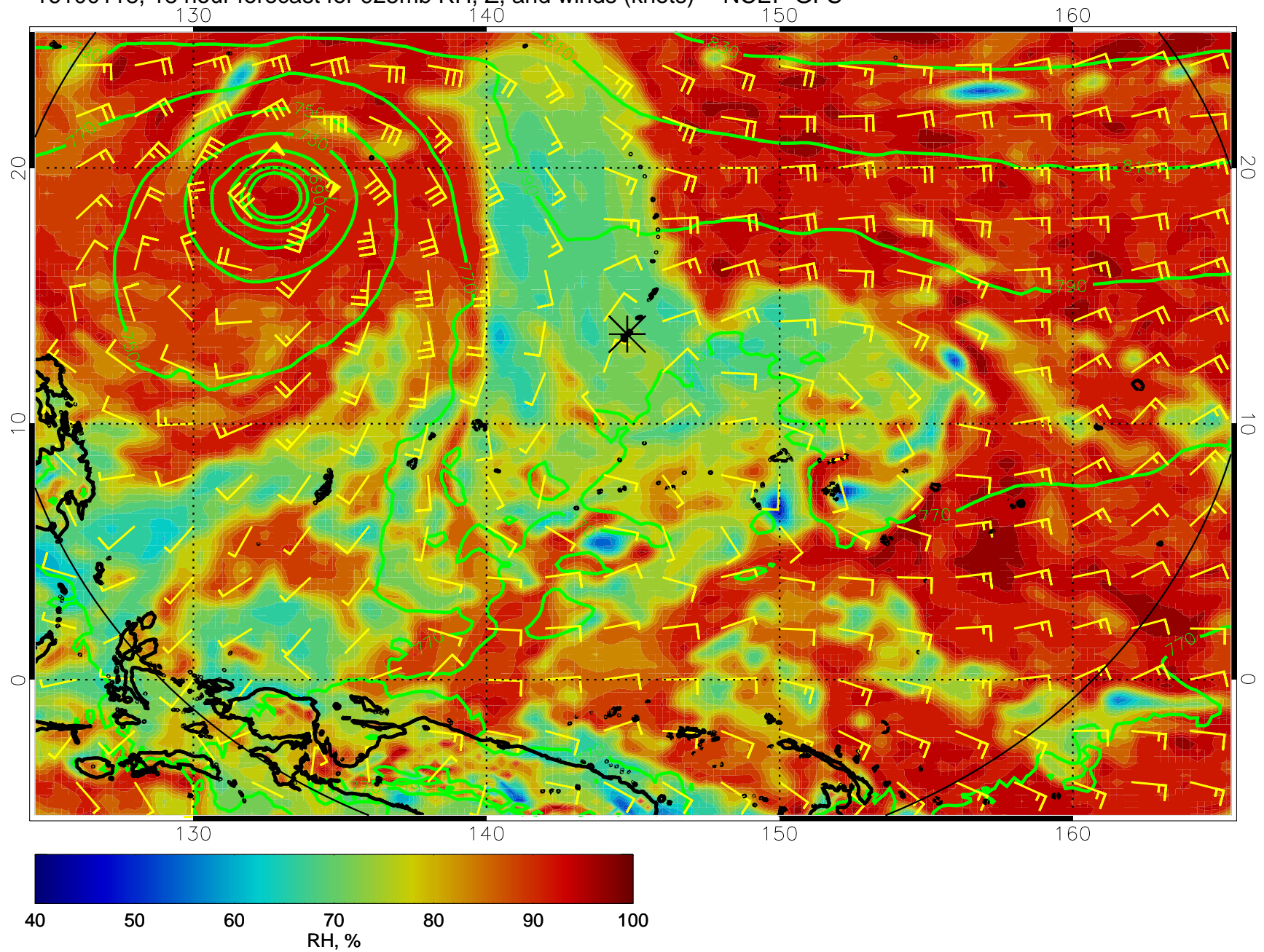
16100118, 18 hour forecast for 925mb RH, Z, and winds (knots) -- NCEP GFS
