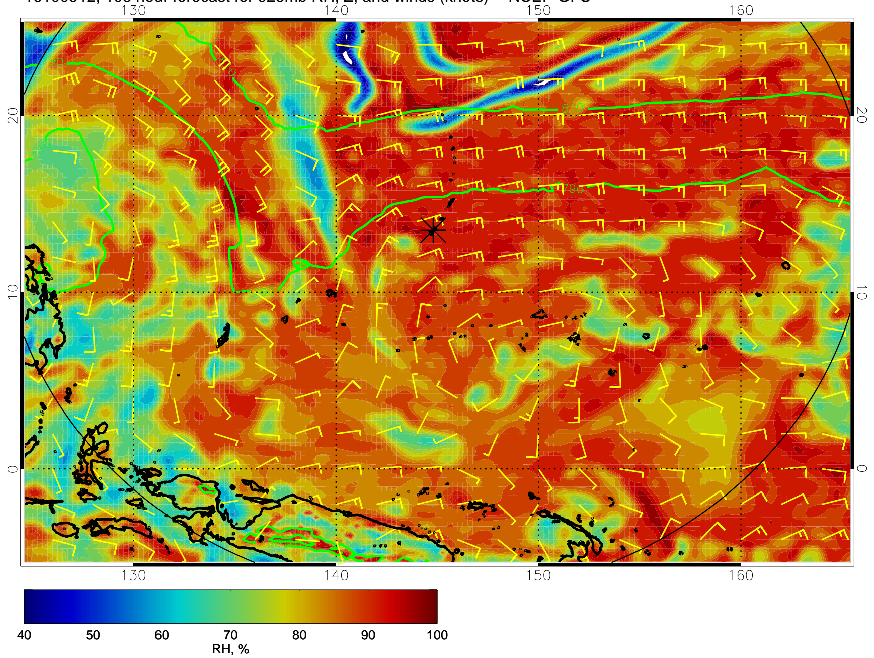
16100512, 108 hour forecast for 925mb RH, Z, and winds (knots) -- NCEP GFS
