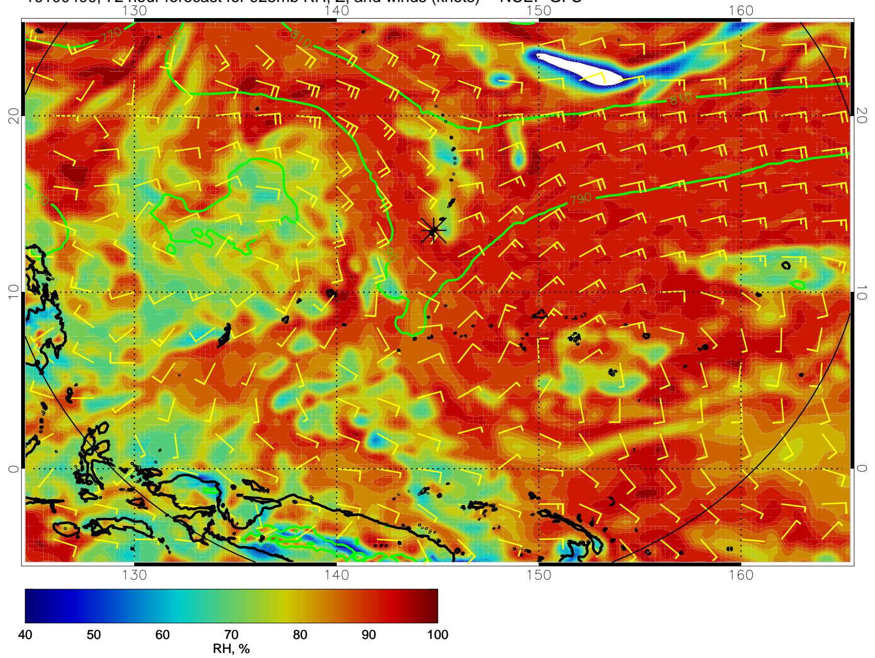
16100400, 72 hour forecast for 925mb RH, Z, and winds (knots) -- NCEP GFS
