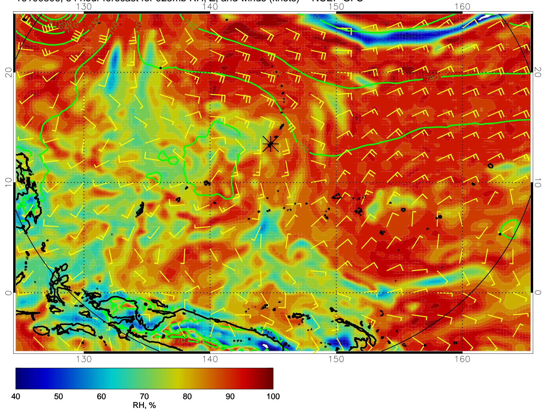
16100306, 54 hour forecast for 925mb RH, Z, and winds (knots) -- NCEP GFS
