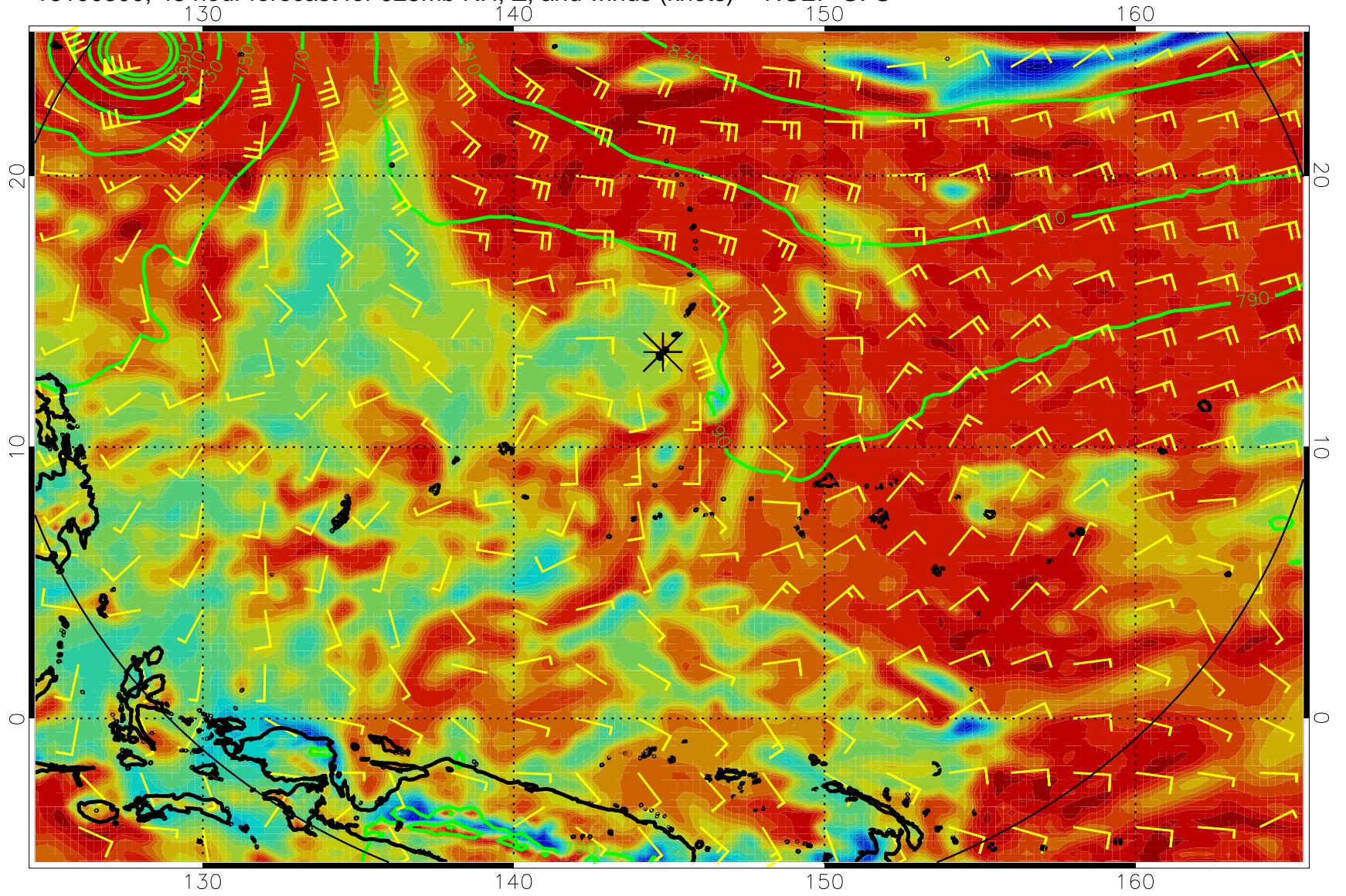
16100300, 48 hour forecast for 925mb RH, Z, and winds (knots) -- NCEP GFS
