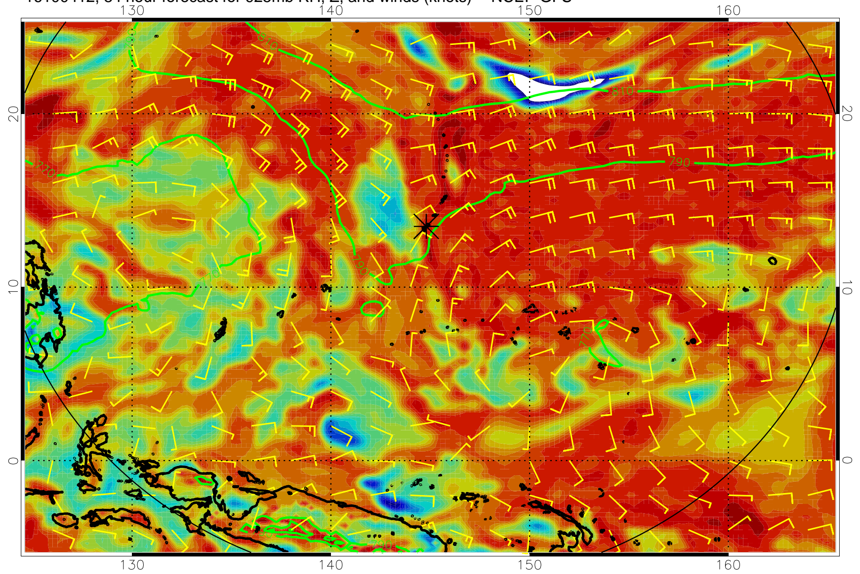
16100412, 84 hour forecast for 925mb RH, Z, and winds (knots) -- NCEP GFS
