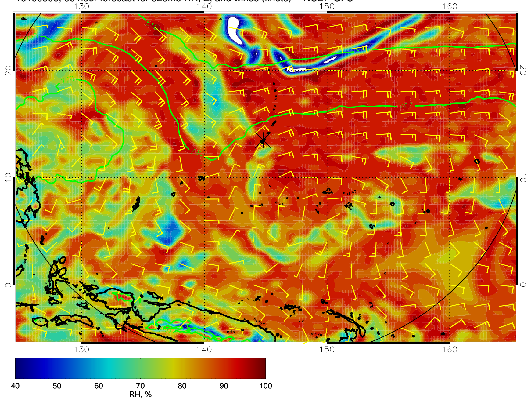
16100500, 96 hour forecast for 925mb RH, Z, and winds (knots) -- NCEP GFS
