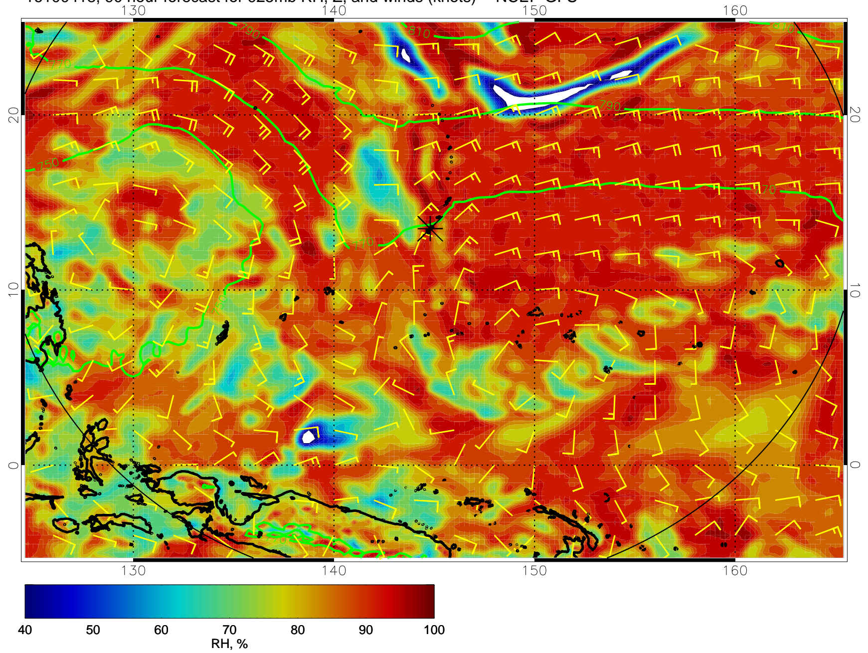
16100418, 90 hour forecast for 925mb RH, Z, and winds (knots) -- NCEP GFS
