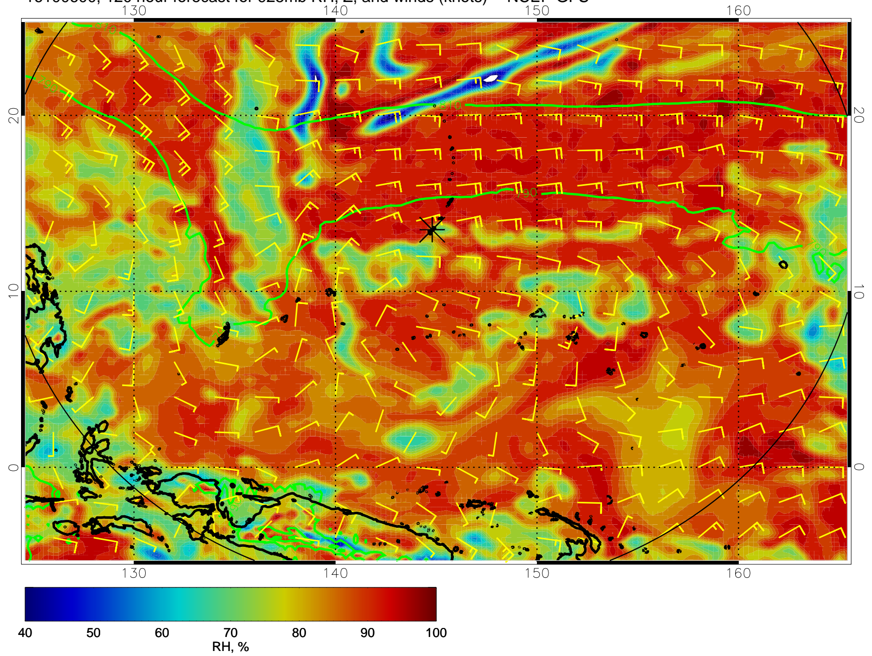
16100600, 120 hour forecast for 925mb RH, Z, and winds (knots) -- NCEP GFS
