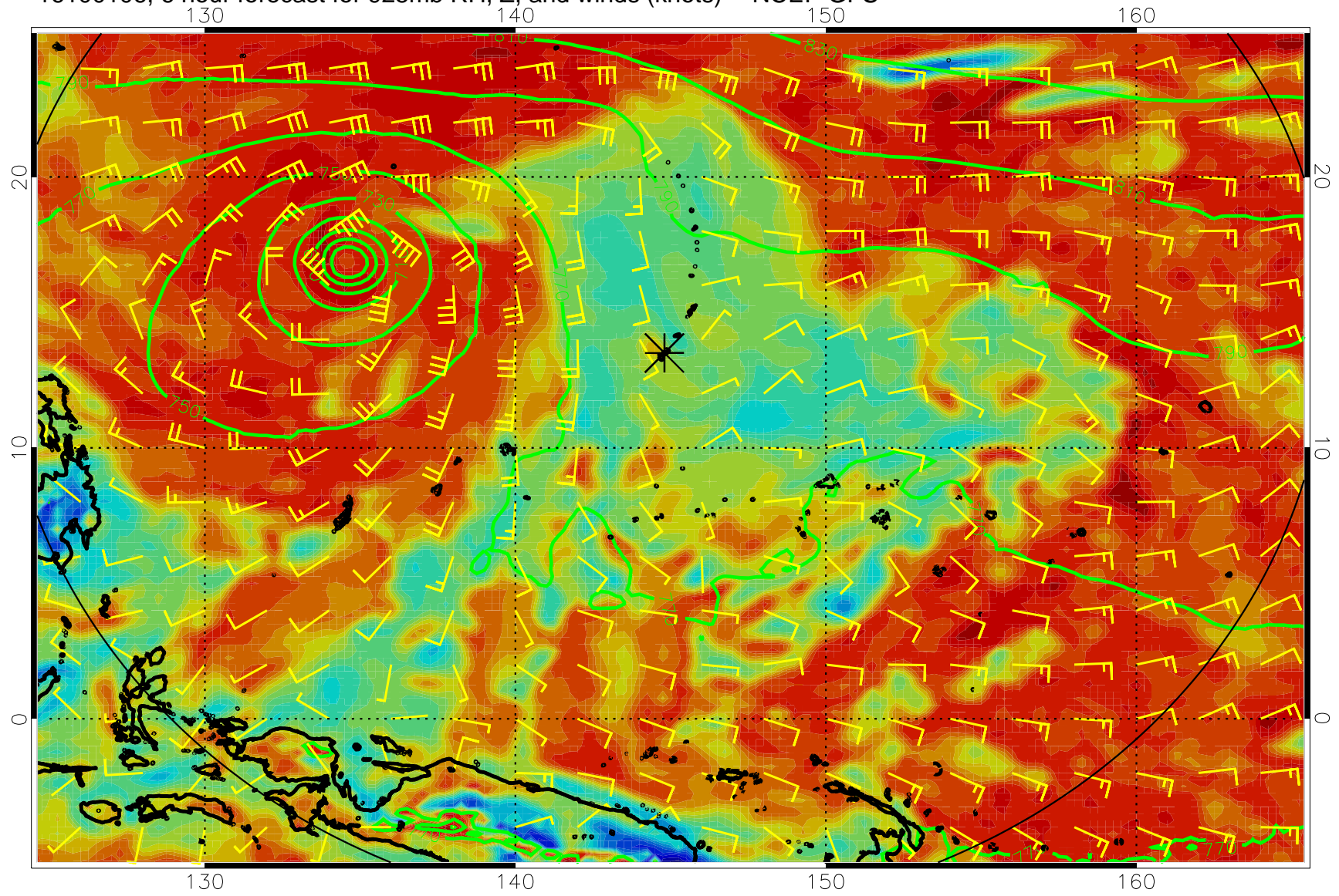
16100106, 6 hour forecast for 925mb RH, Z, and winds (knots) -- NCEP GFS
