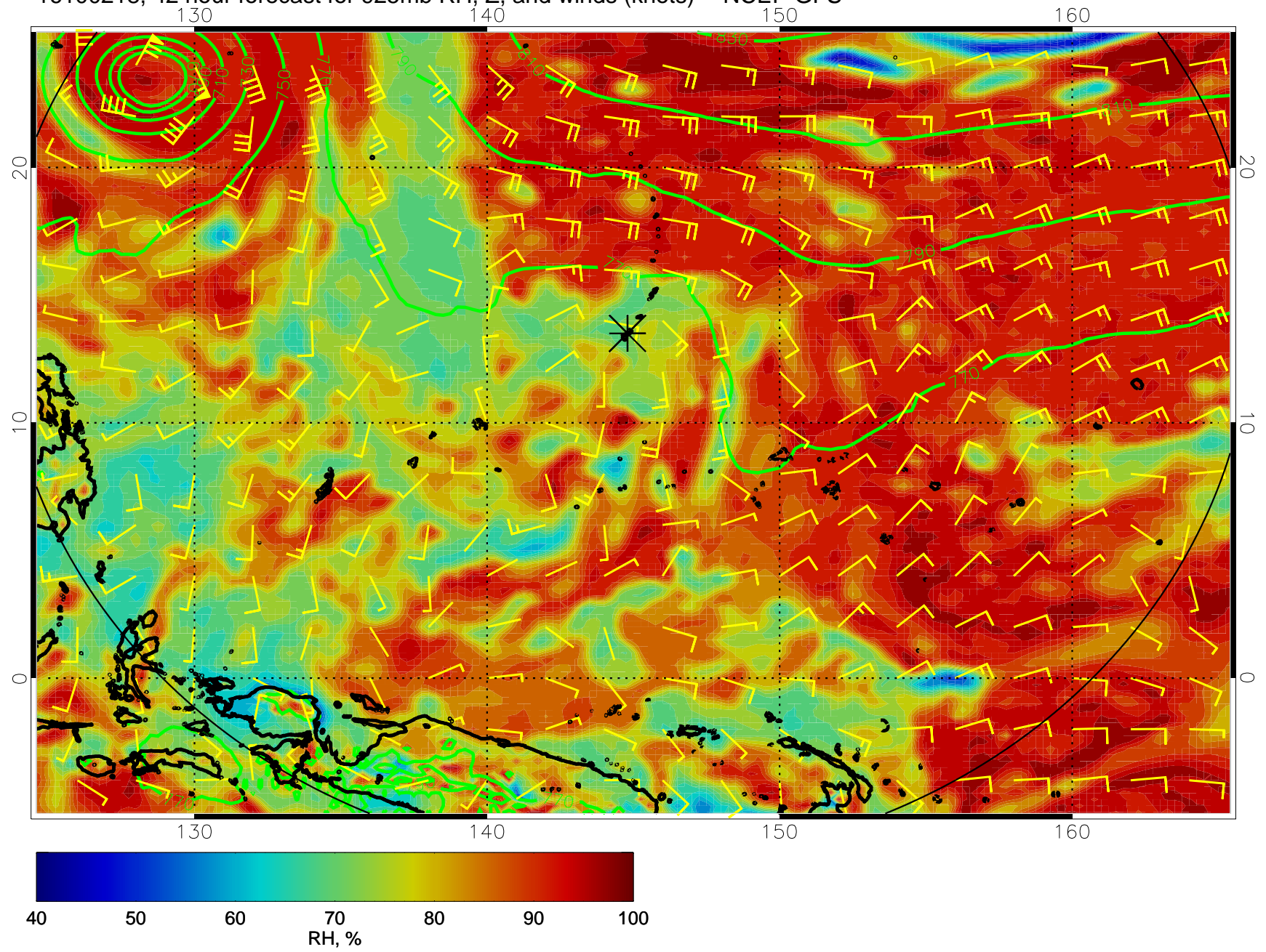
16100218, 42 hour forecast for 925mb RH, Z, and winds (knots) -- NCEP GFS
