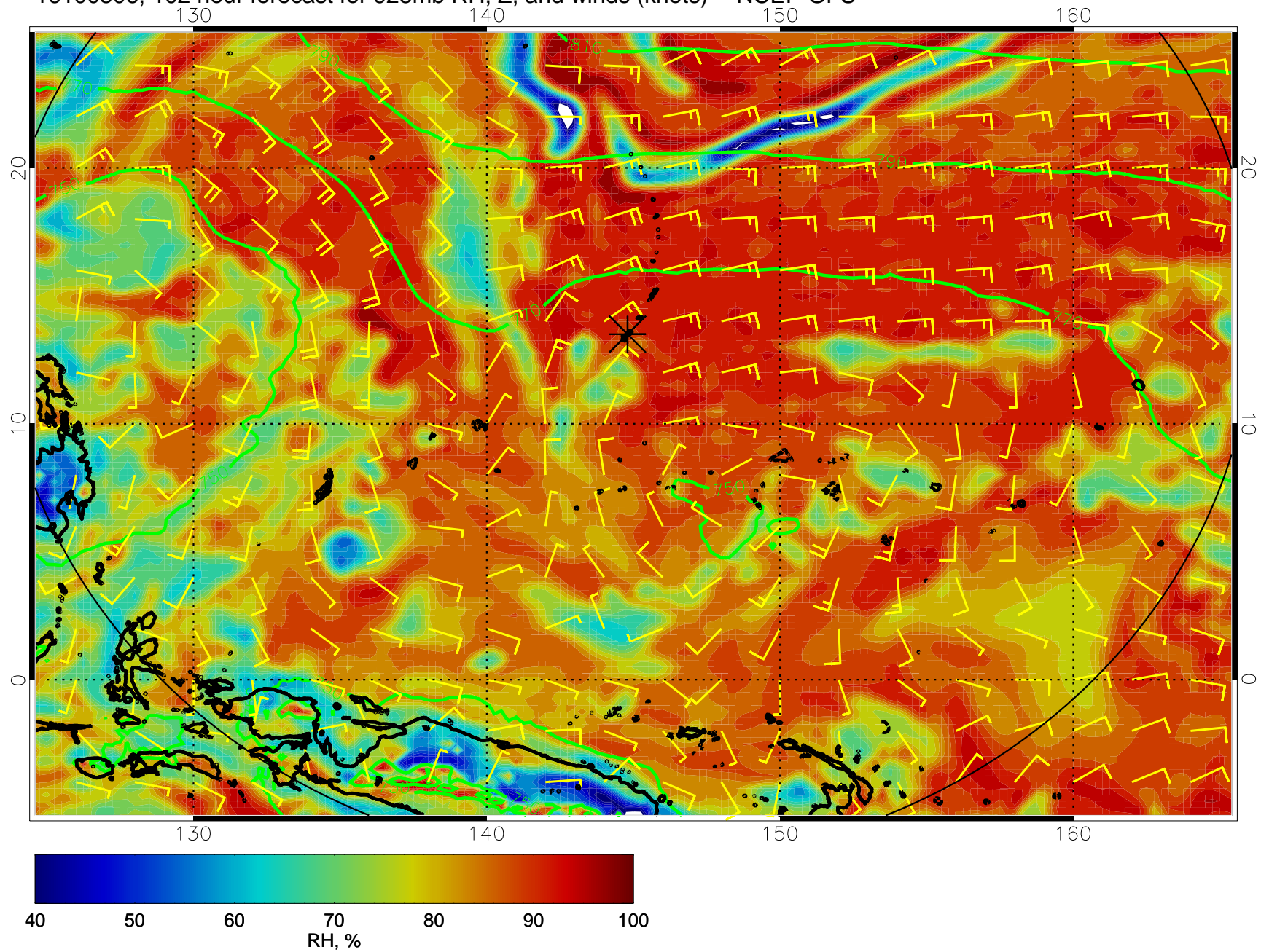
16100506, 102 hour forecast for 925mb RH, Z, and winds (knots) -- NCEP GFS
