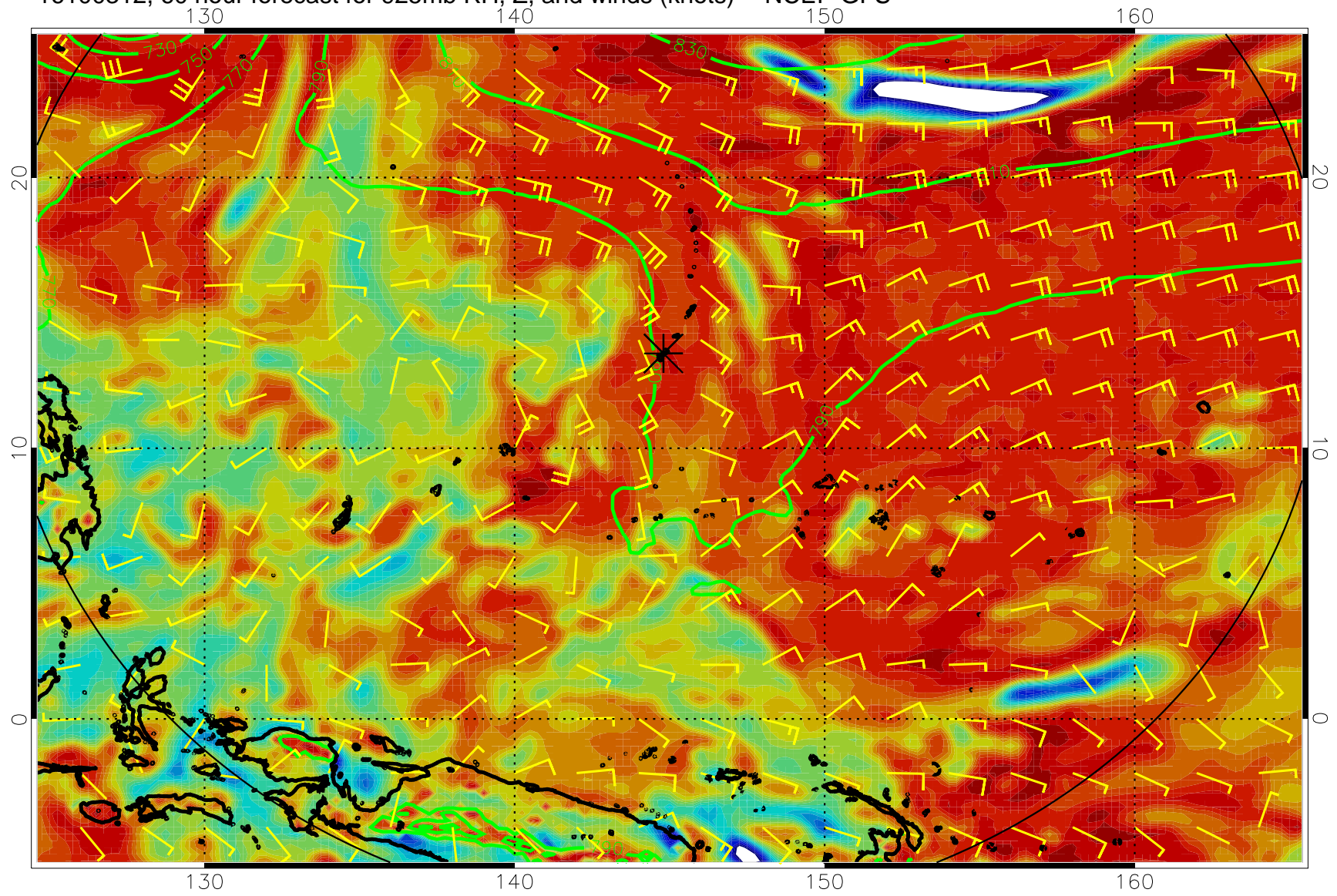
16100312, 60 hour forecast for 925mb RH, Z, and winds (knots) -- NCEP GFS
