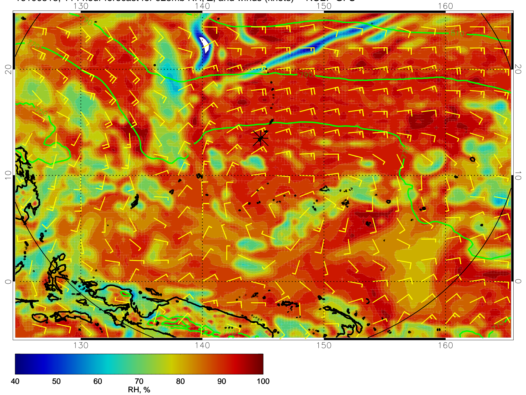
16100518, 114 hour forecast for 925mb RH, Z, and winds (knots) -- NCEP GFS
