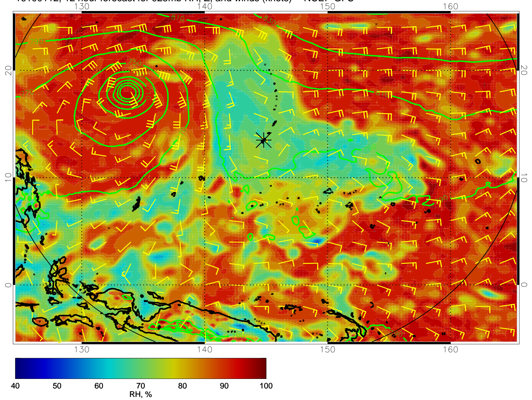
16100112, 12 hour forecast for 925mb RH, Z, and winds (knots) -- NCEP GFS
