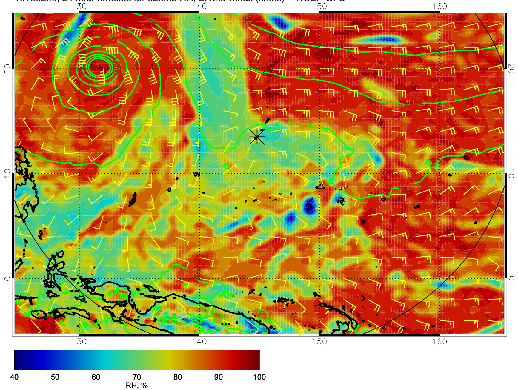
16100200, 24 hour forecast for 925mb RH, Z, and winds (knots) -- NCEP GFS
