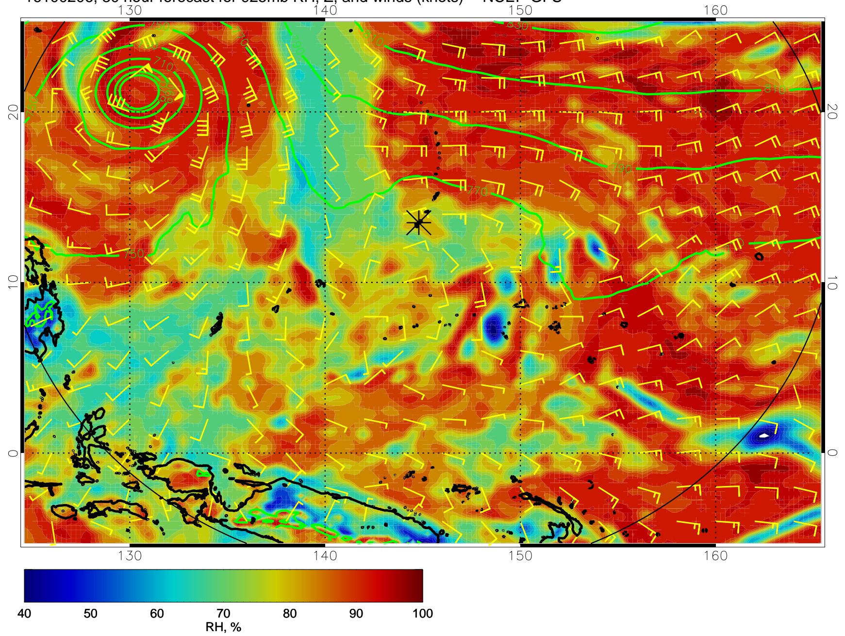
16100206, 30 hour forecast for 925mb RH, Z, and winds (knots) -- NCEP GFS
