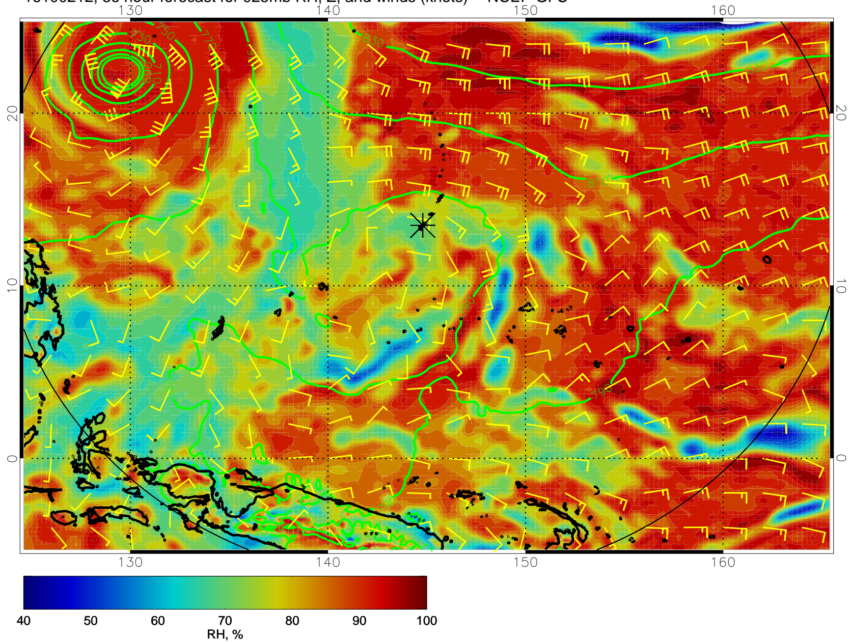
16100212, 36 hour forecast for 925mb RH, Z, and winds (knots) -- NCEP GFS
