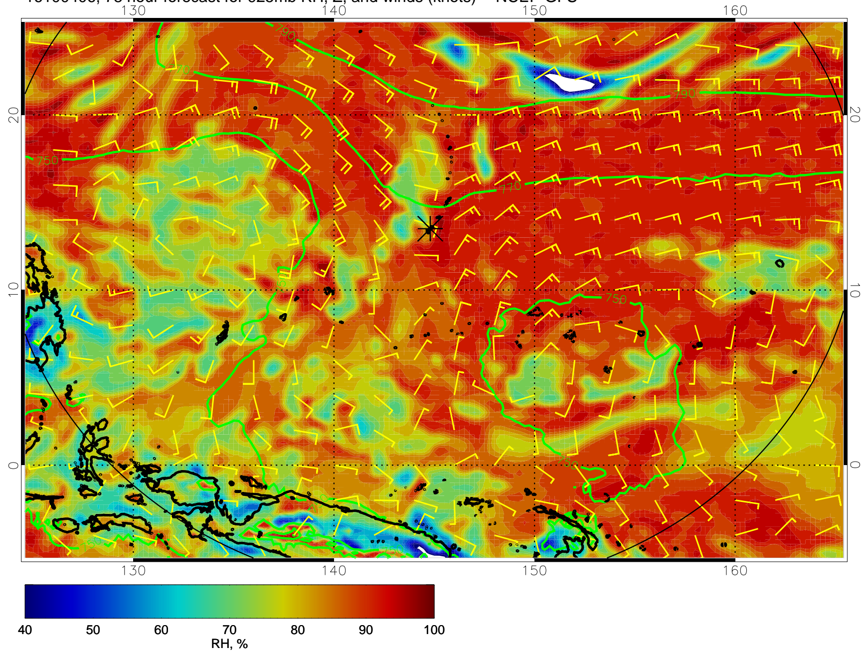
16100406, 78 hour forecast for 925mb RH, Z, and winds (knots) -- NCEP GFS
