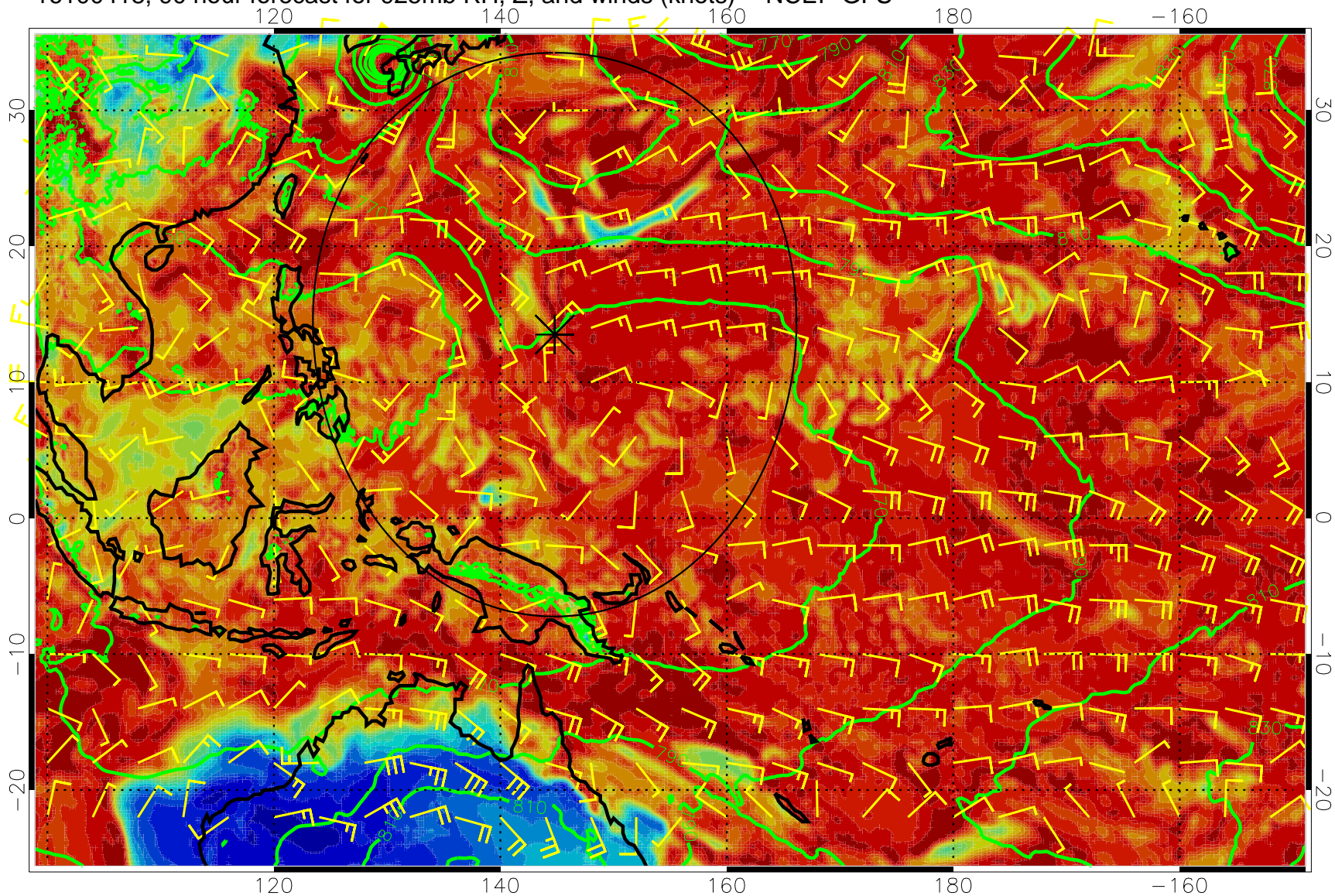
16100418, 90 hour forecast for 925mb RH, Z, and winds (knots) -- NCEP GFS
