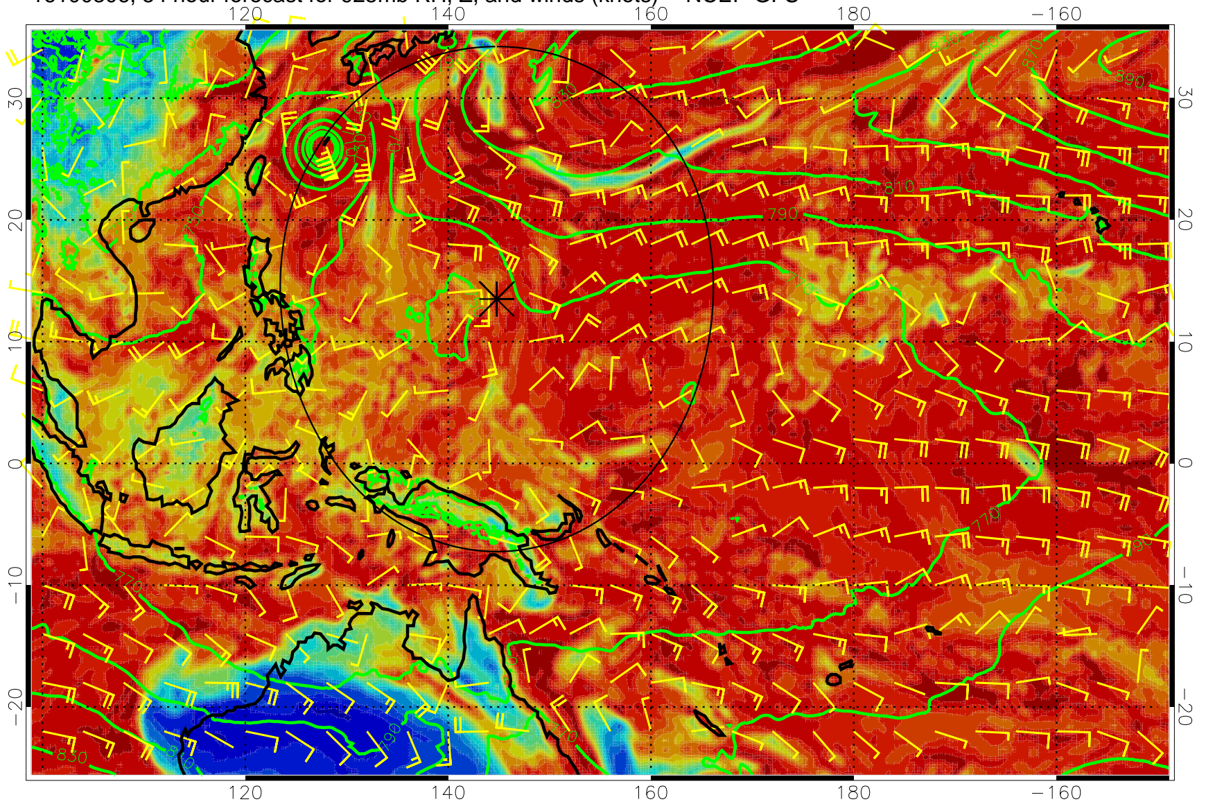
16100306, 54 hour forecast for 925mb RH, Z, and winds (knots) -- NCEP GFS
