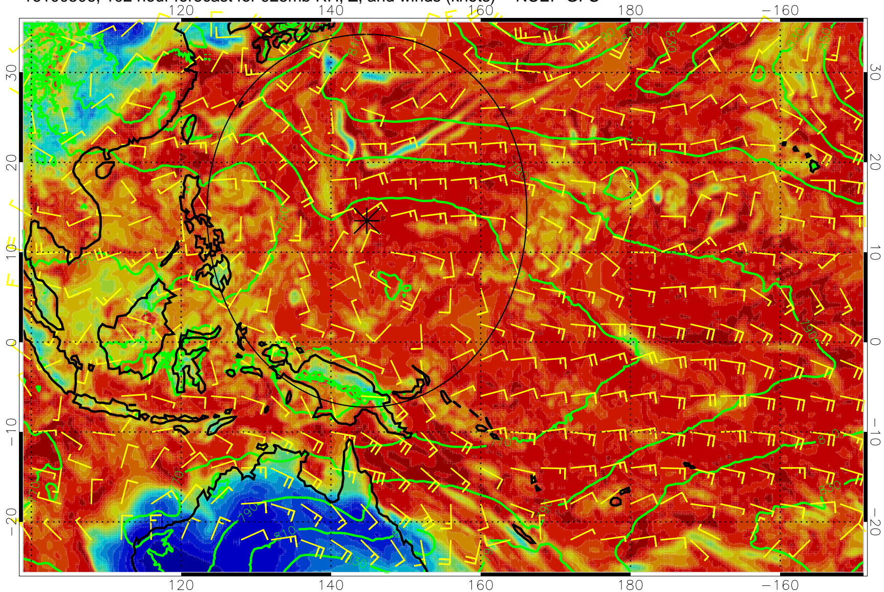
16100506, 102 hour forecast for 925mb RH, Z, and winds (knots) -- NCEP GFS
