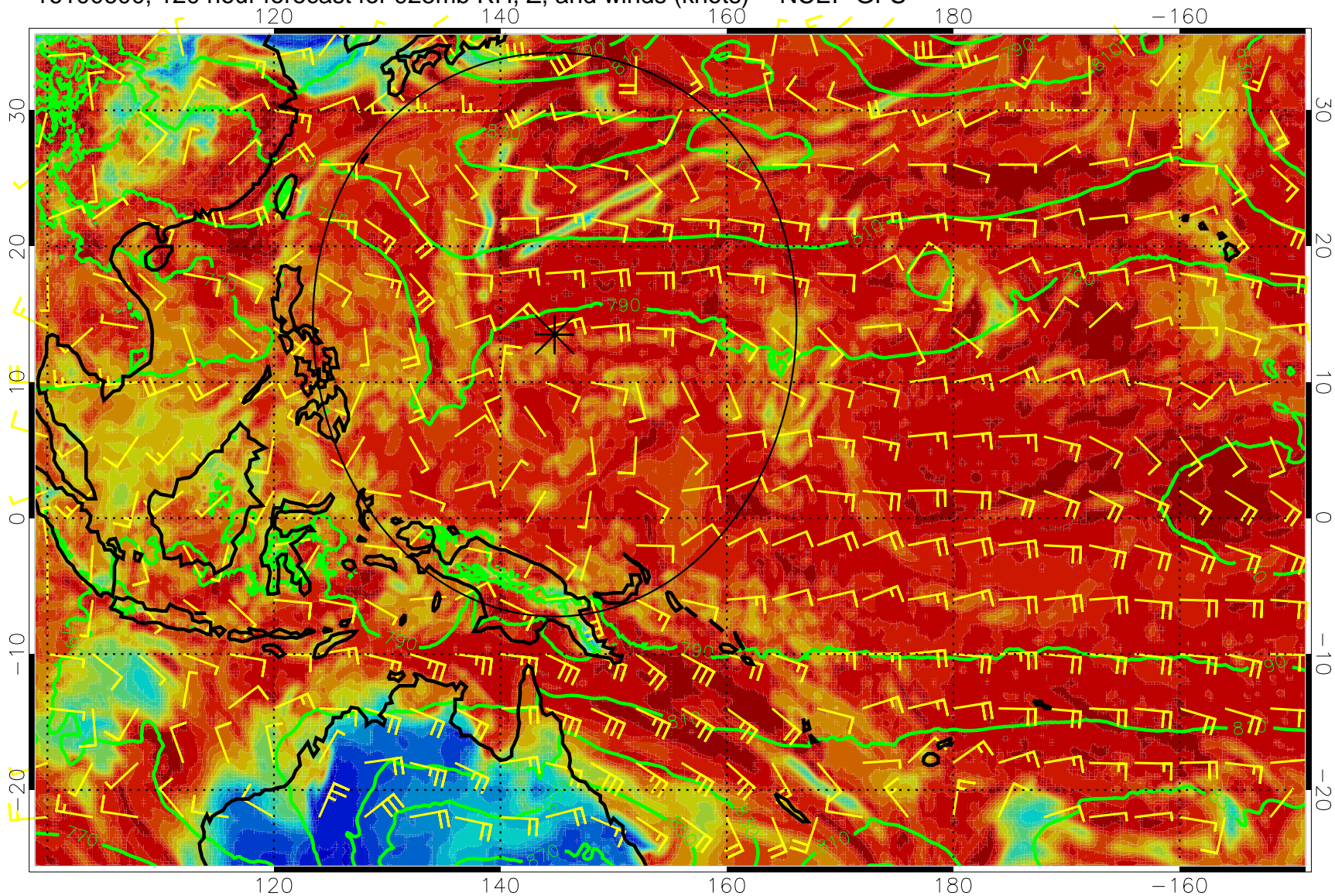
16100600, 120 hour forecast for 925mb RH, Z, and winds (knots) -- NCEP GFS
