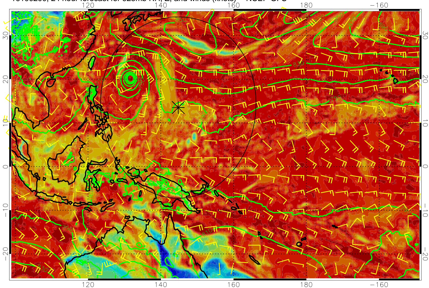
16100200, 24 hour forecast for 925mb RH, Z, and winds (knots) -- NCEP GFS
