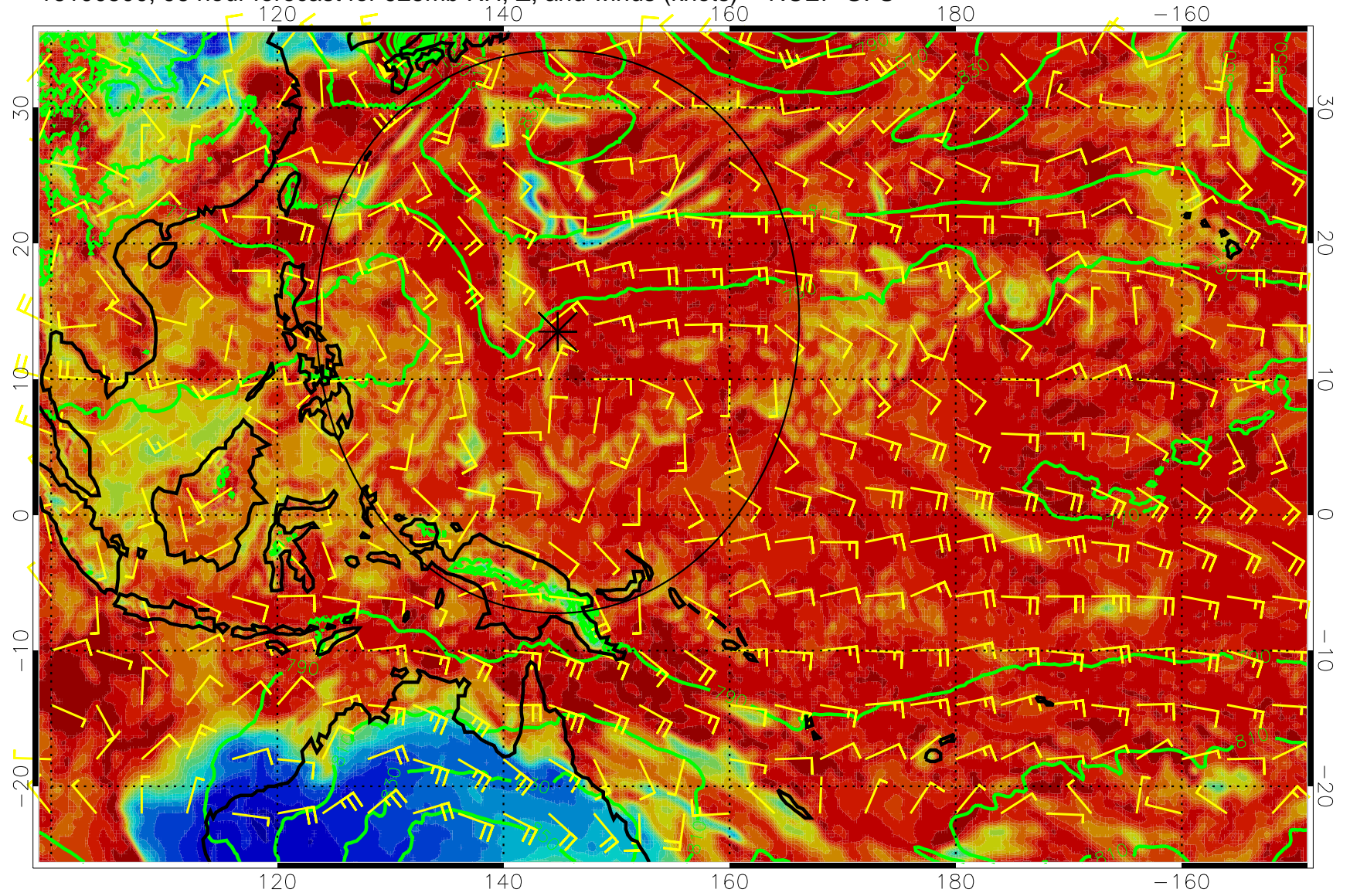
16100500, 96 hour forecast for 925mb RH, Z, and winds (knots) -- NCEP GFS
