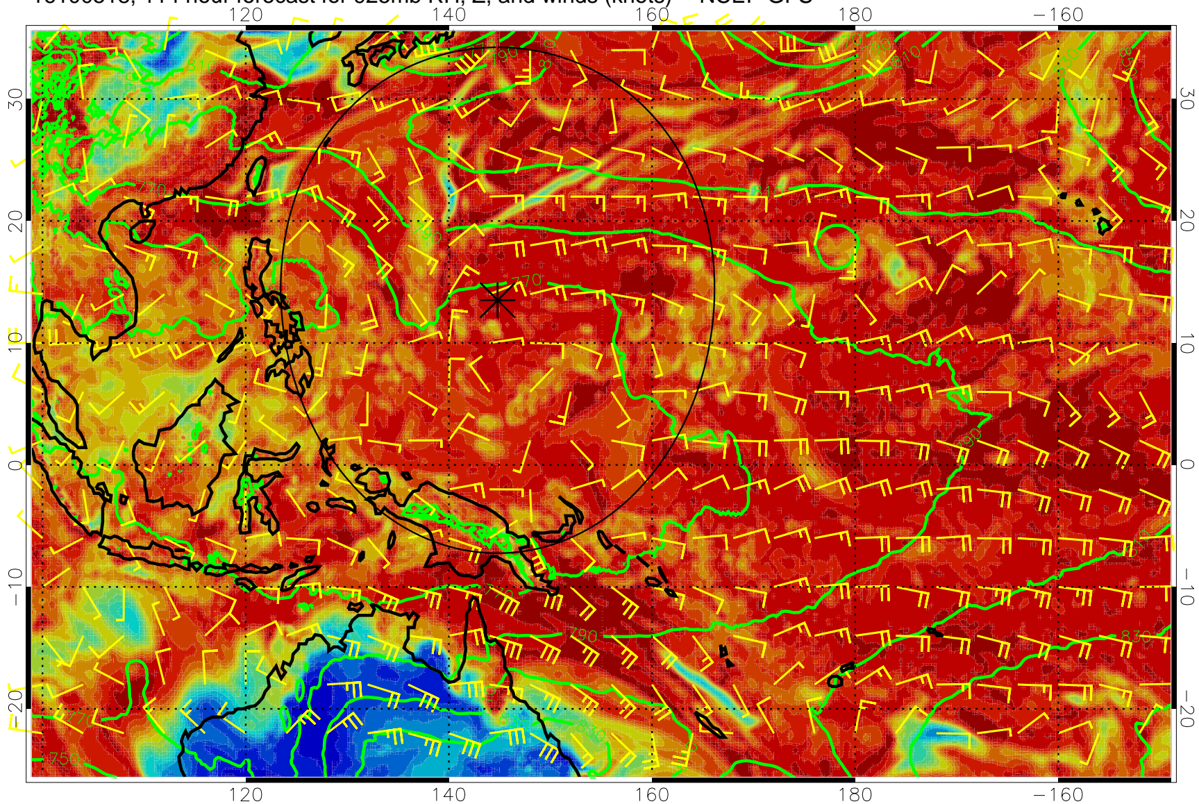
16100518, 114 hour forecast for 925mb RH, Z, and winds (knots) -- NCEP GFS
