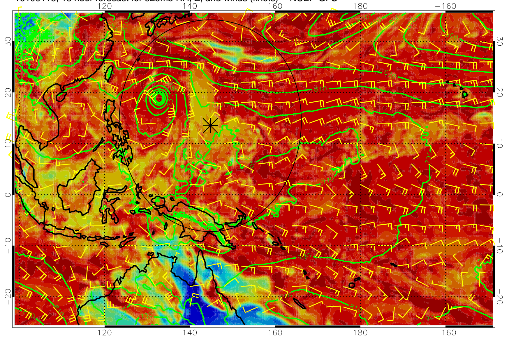
16100118, 18 hour forecast for 925mb RH, Z, and winds (knots) -- NCEP GFS
