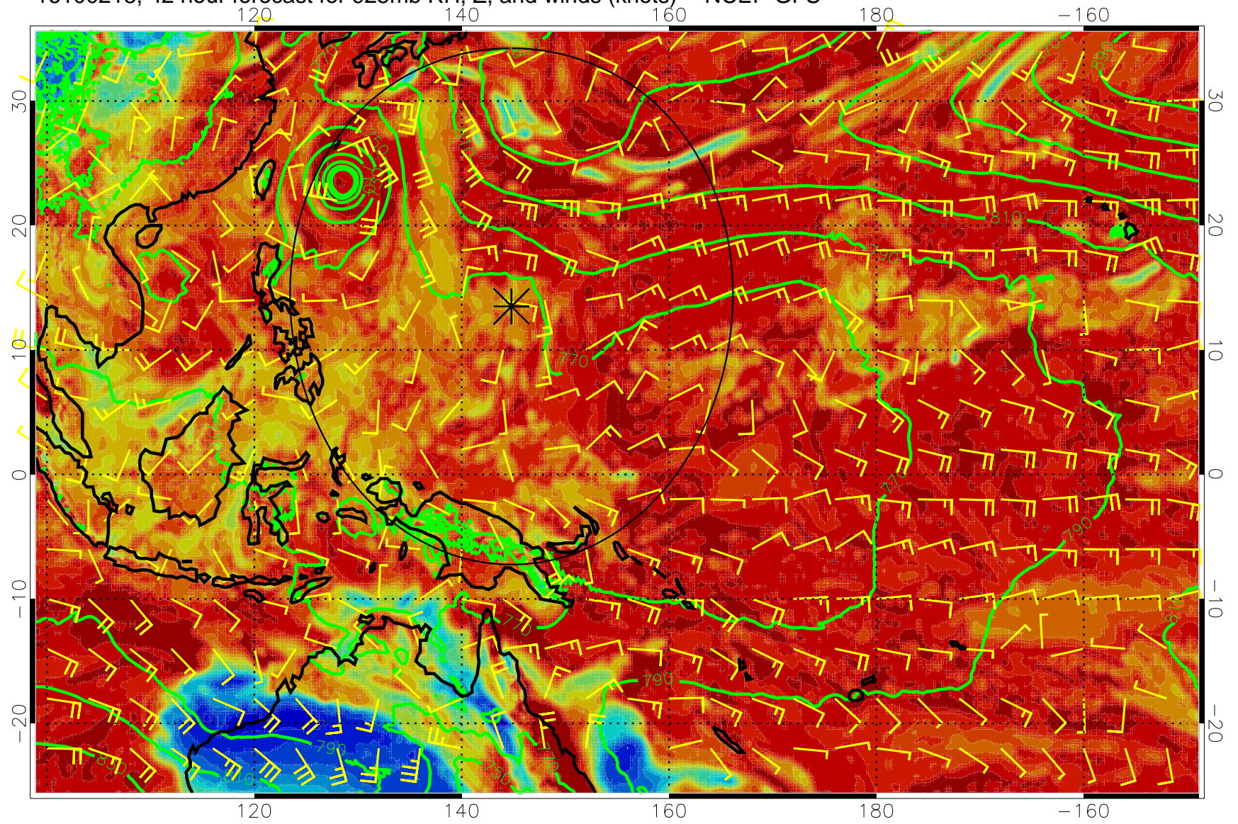
16100218, 42 hour forecast for 925mb RH, Z, and winds (knots) -- NCEP GFS
