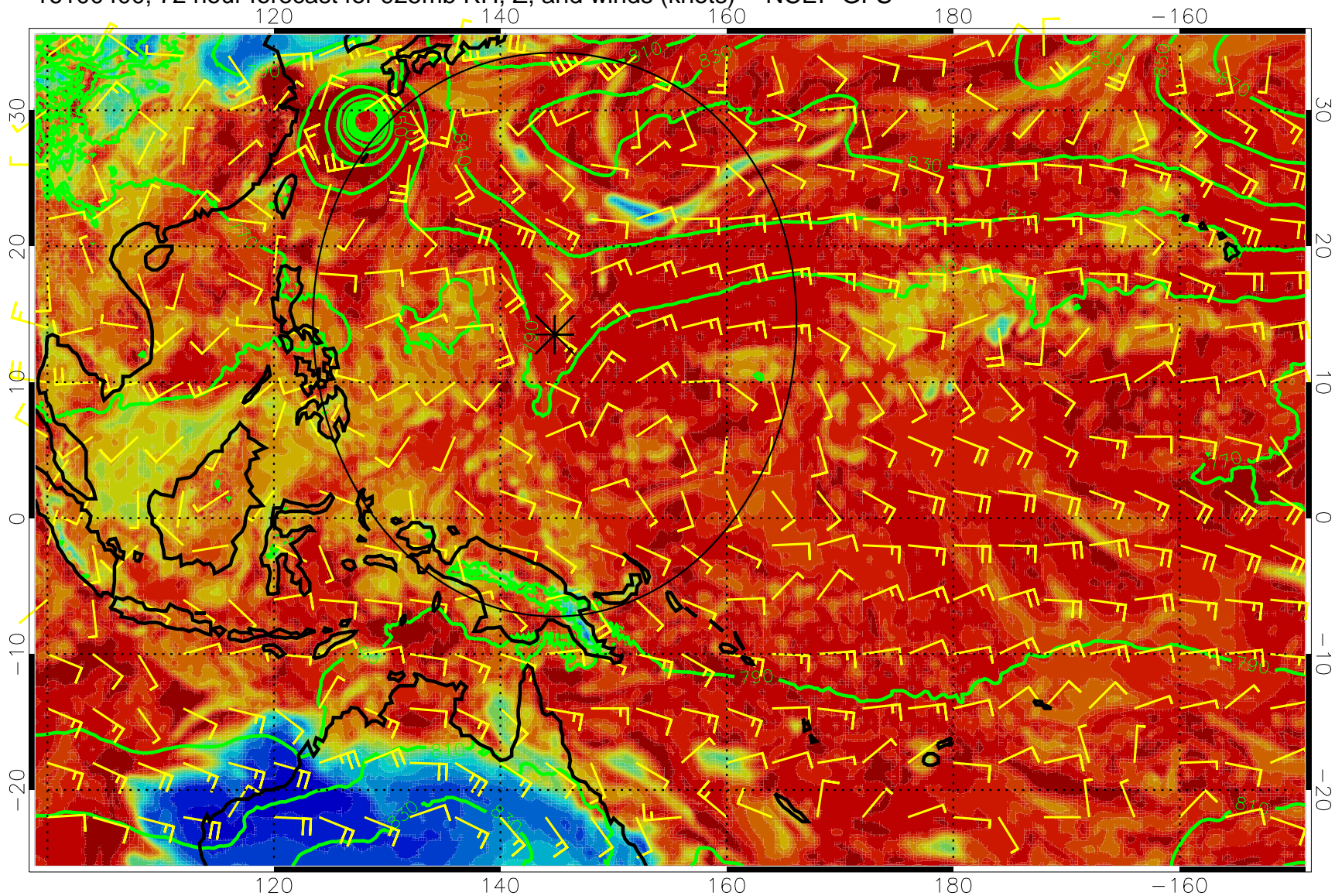
16100400, 72 hour forecast for 925mb RH, Z, and winds (knots) -- NCEP GFS
