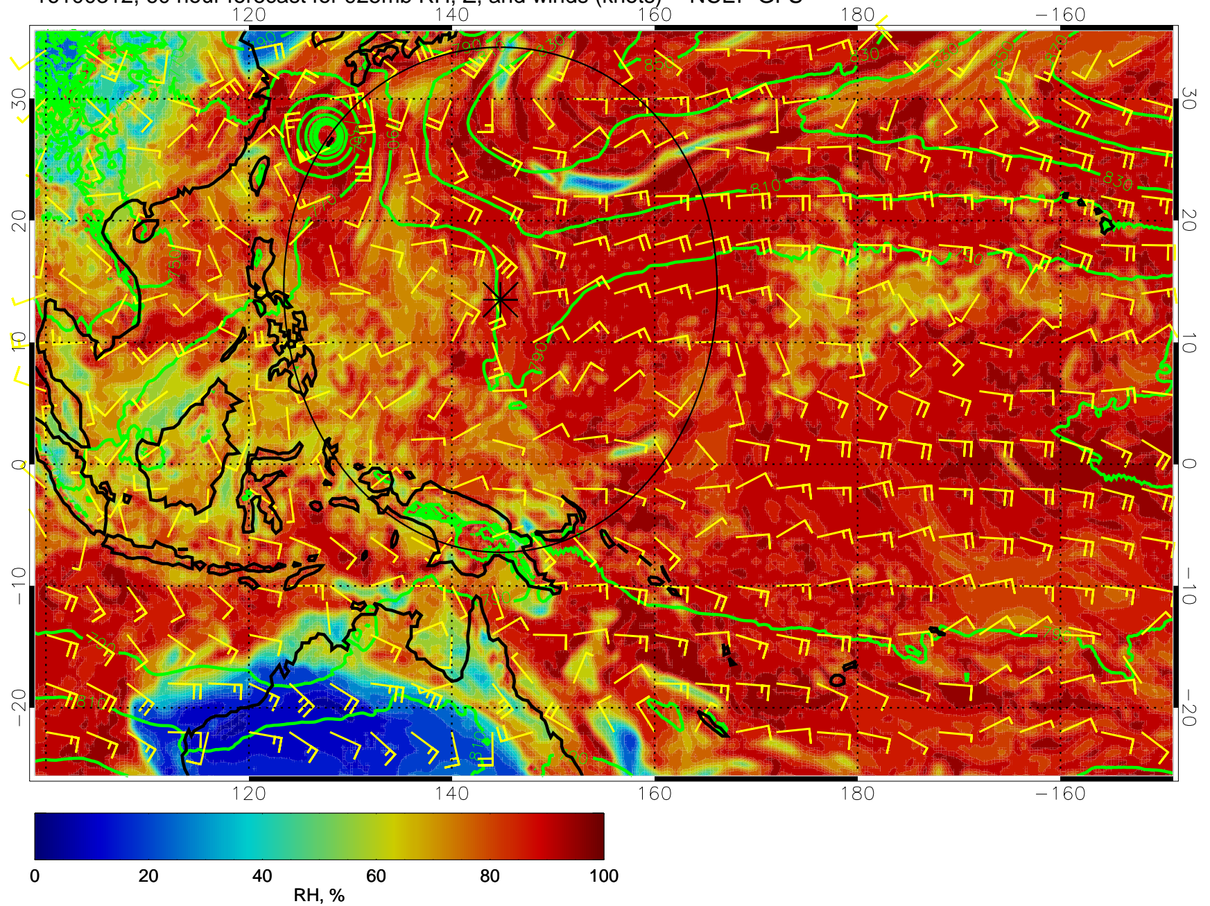
16100312, 60 hour forecast for 925mb RH, Z, and winds (knots) -- NCEP GFS
