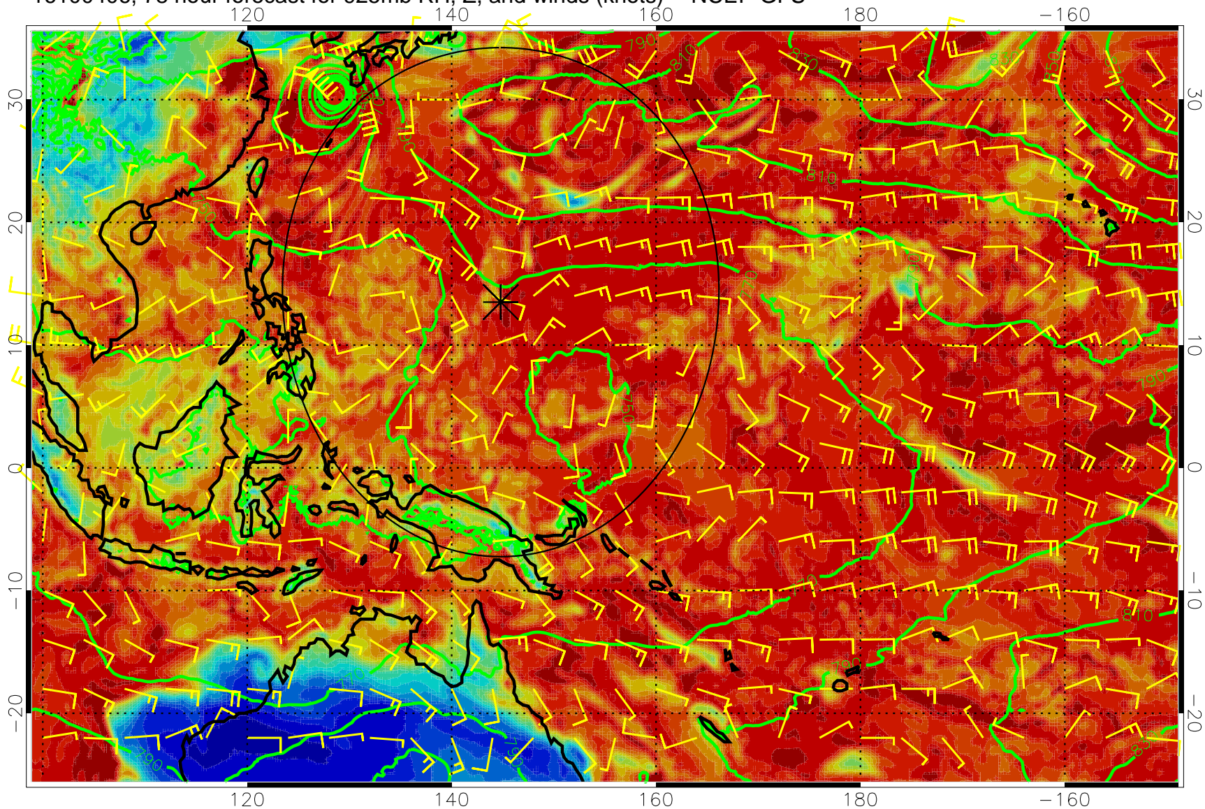
16100406, 78 hour forecast for 925mb RH, Z, and winds (knots) -- NCEP GFS
