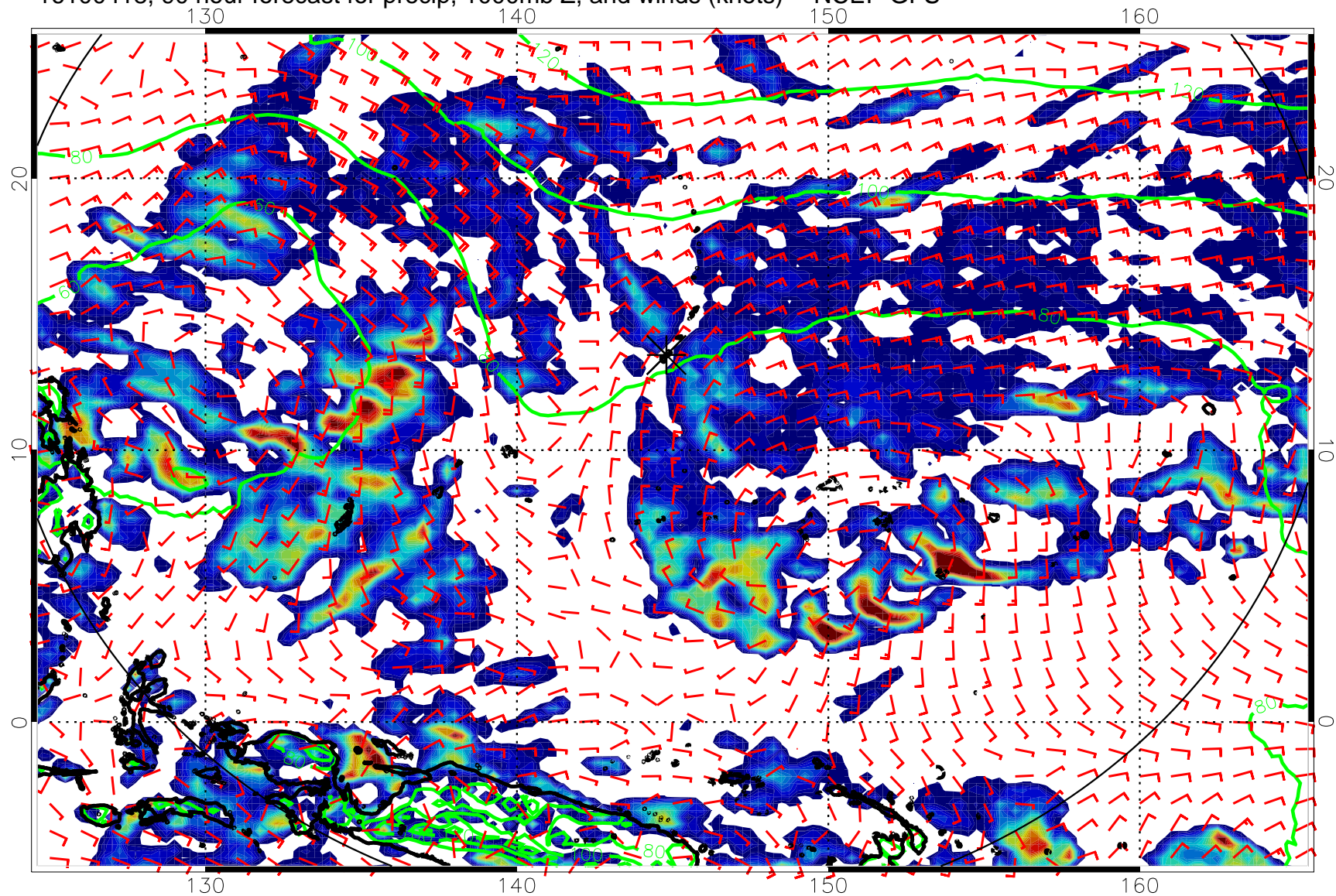
16100418, 90 hour forecast for precip, 1000mb Z, and winds (knots) -- NCEP GFS
