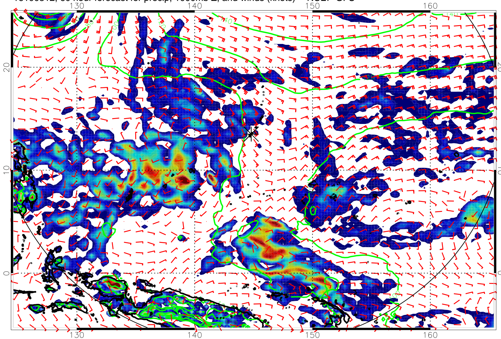
16100312, 60 hour forecast for precip, 1000mb Z, and winds (knots) -- NCEP GFS
