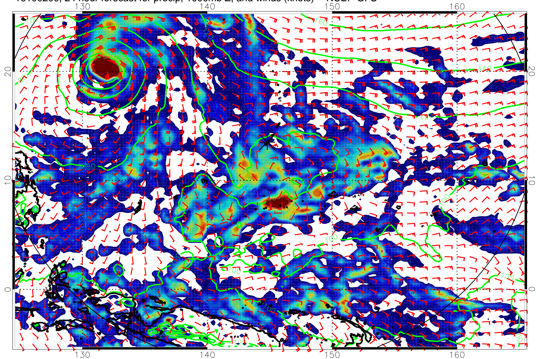
16100200, 24 hour forecast for precip, 1000mb Z, and winds (knots) -- NCEP GFS
