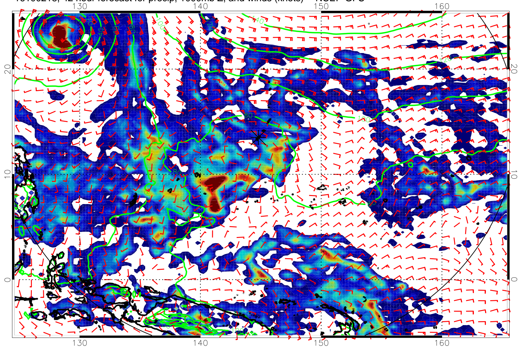
16100218, 42 hour forecast for precip, 1000mb Z, and winds (knots) -- NCEP GFS
