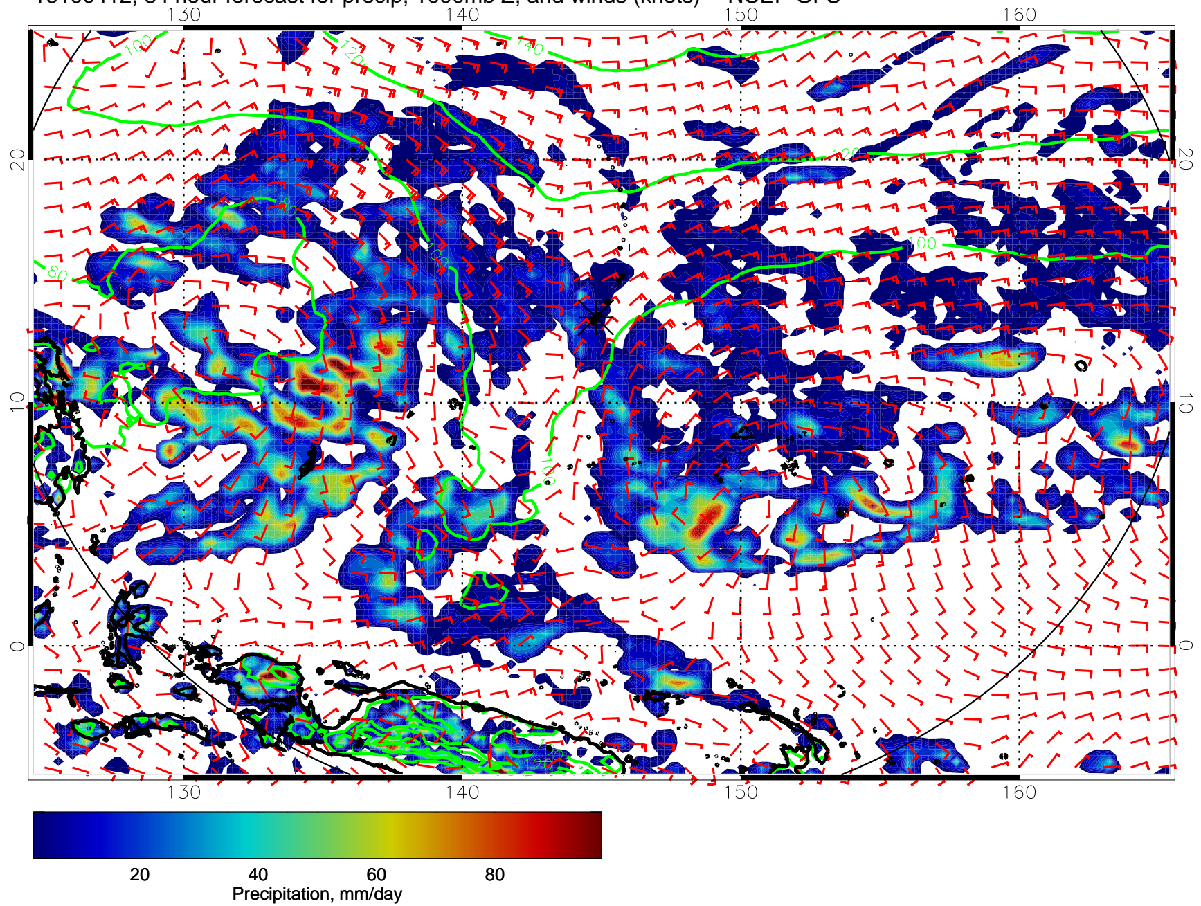
16100412, 84 hour forecast for precip, 1000mb Z, and winds (knots) -- NCEP GFS
