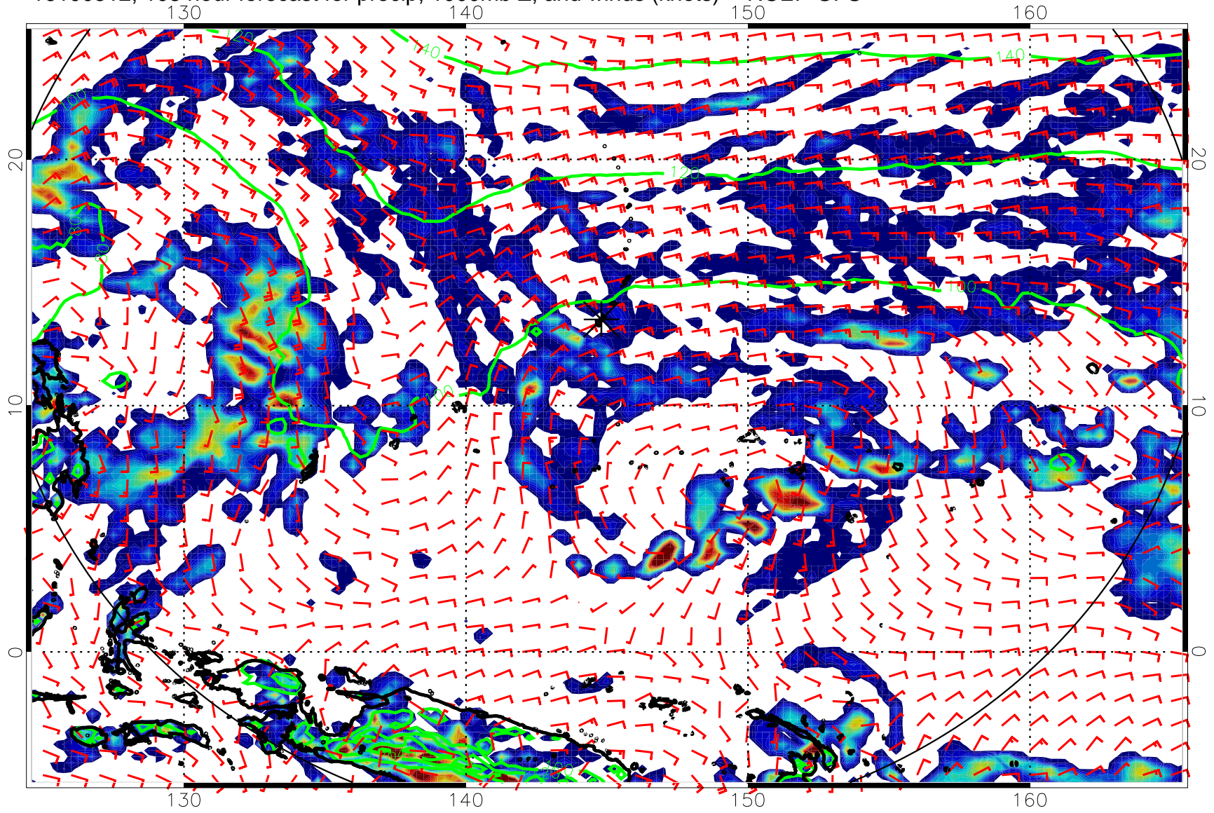
16100512, 108 hour forecast for precip, 1000mb Z, and winds (knots) -- NCEP GFS
