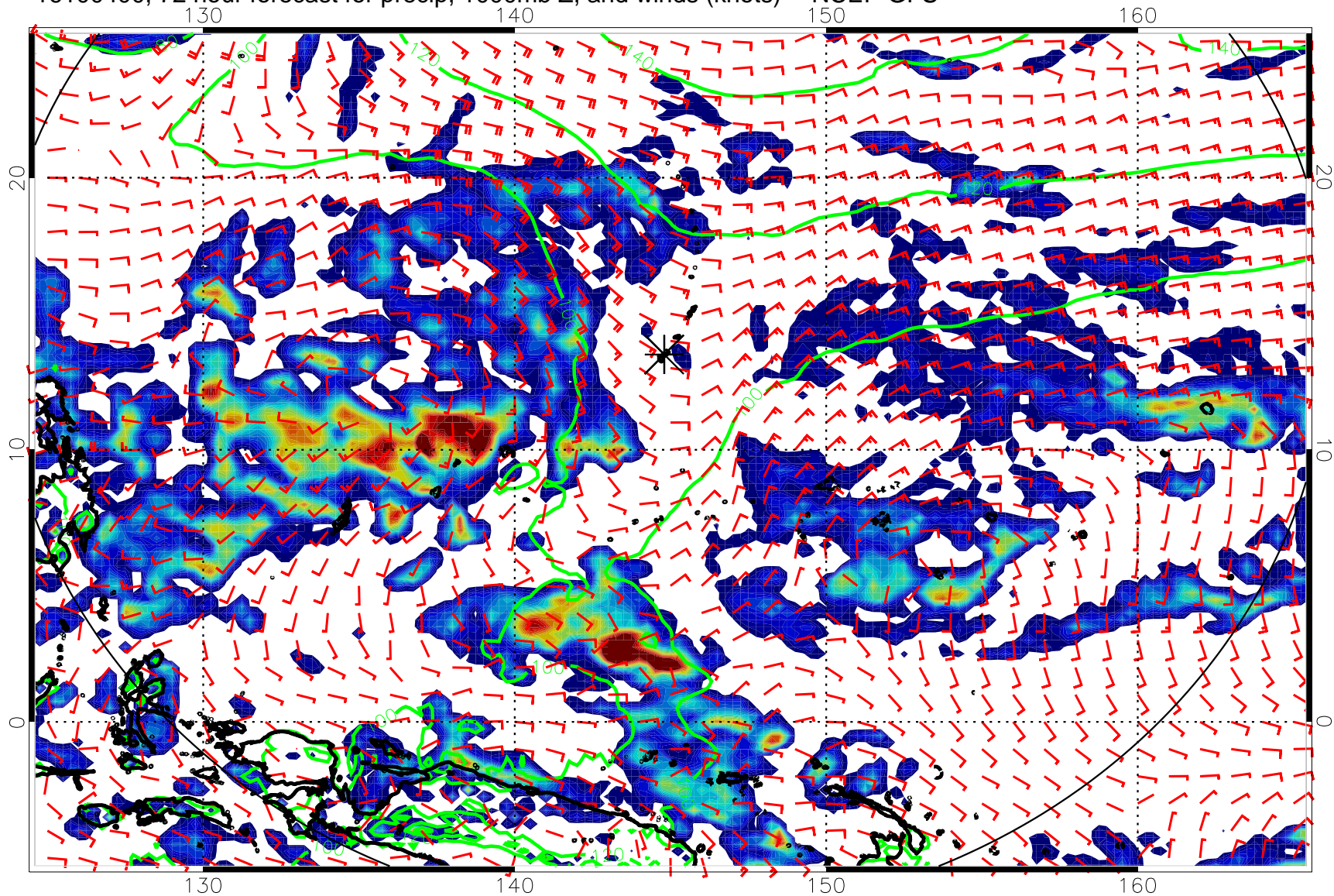
16100400, 72 hour forecast for precip, 1000mb Z, and winds (knots) -- NCEP GFS
