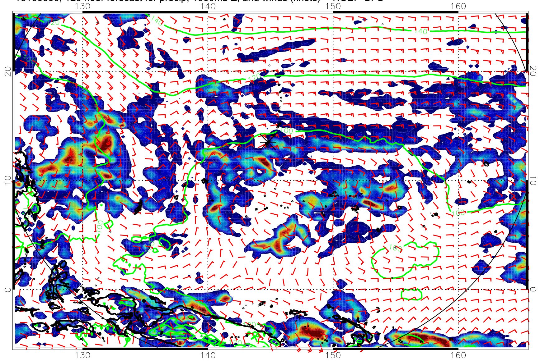
16100600, 120 hour forecast for precip, 1000mb Z, and winds (knots) -- NCEP GFS
