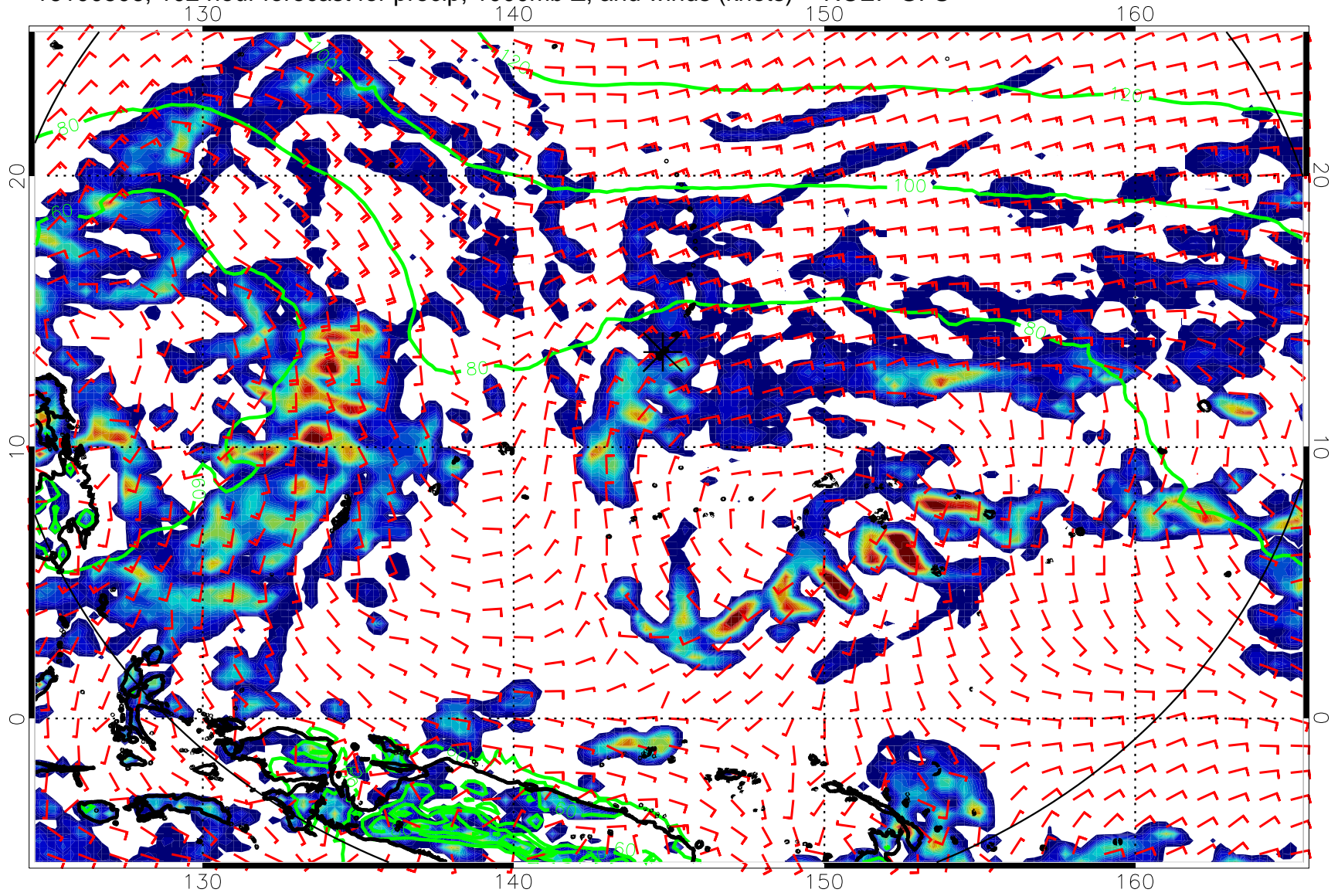
16100506, 102 hour forecast for precip, 1000mb Z, and winds (knots) -- NCEP GFS
