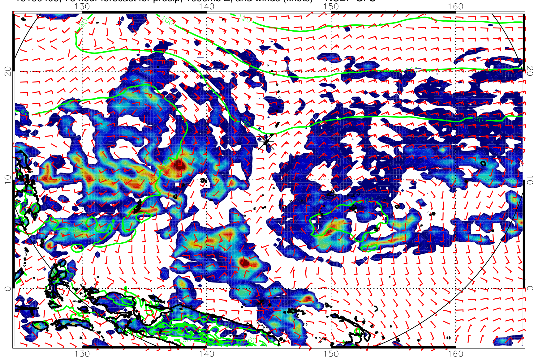
16100406, 78 hour forecast for precip, 1000mb Z, and winds (knots) -- NCEP GFS
