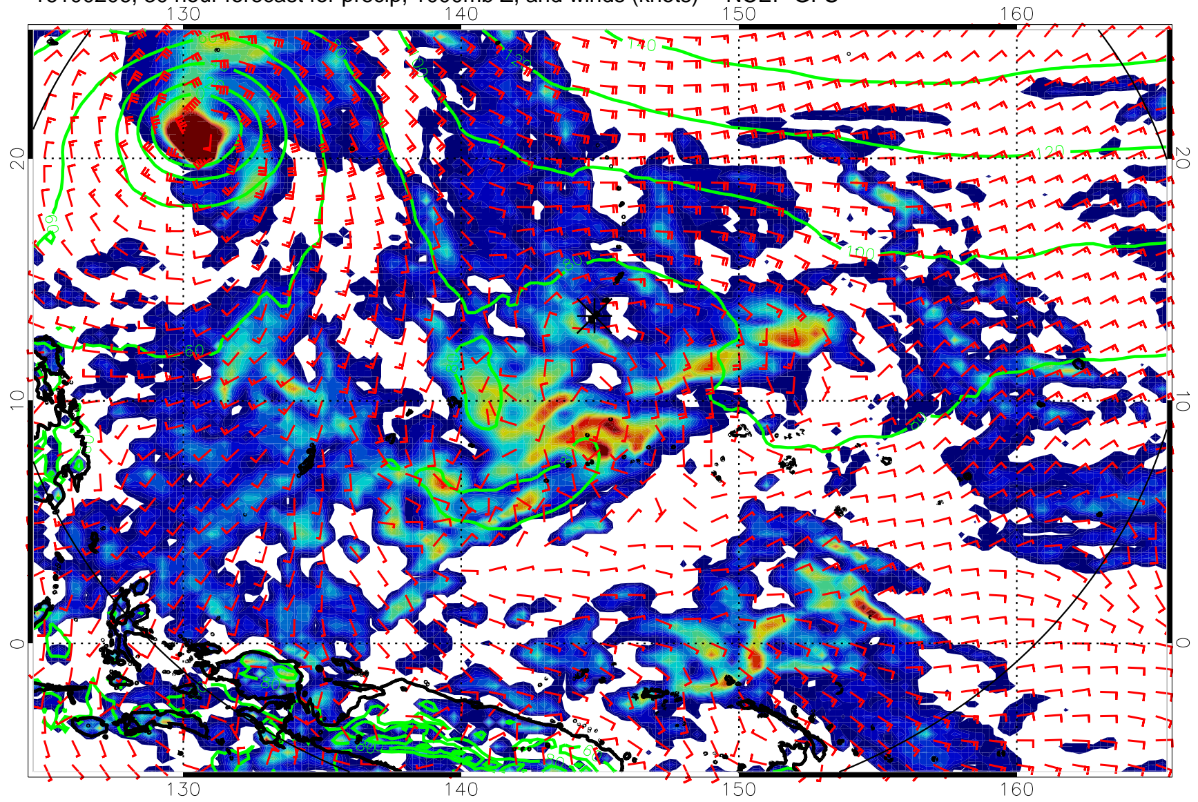
16100206, 30 hour forecast for precip, 1000mb Z, and winds (knots) -- NCEP GFS
