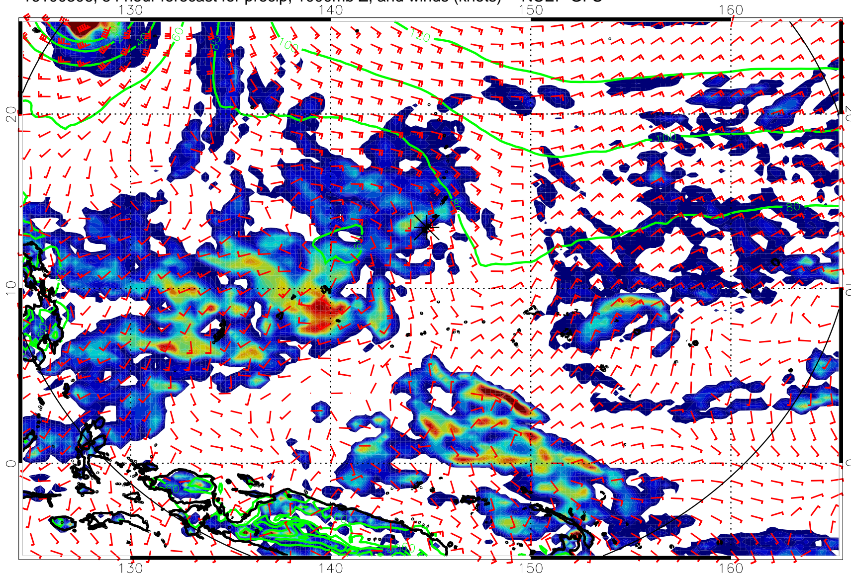
16100306, 54 hour forecast for precip, 1000mb Z, and winds (knots) -- NCEP GFS
