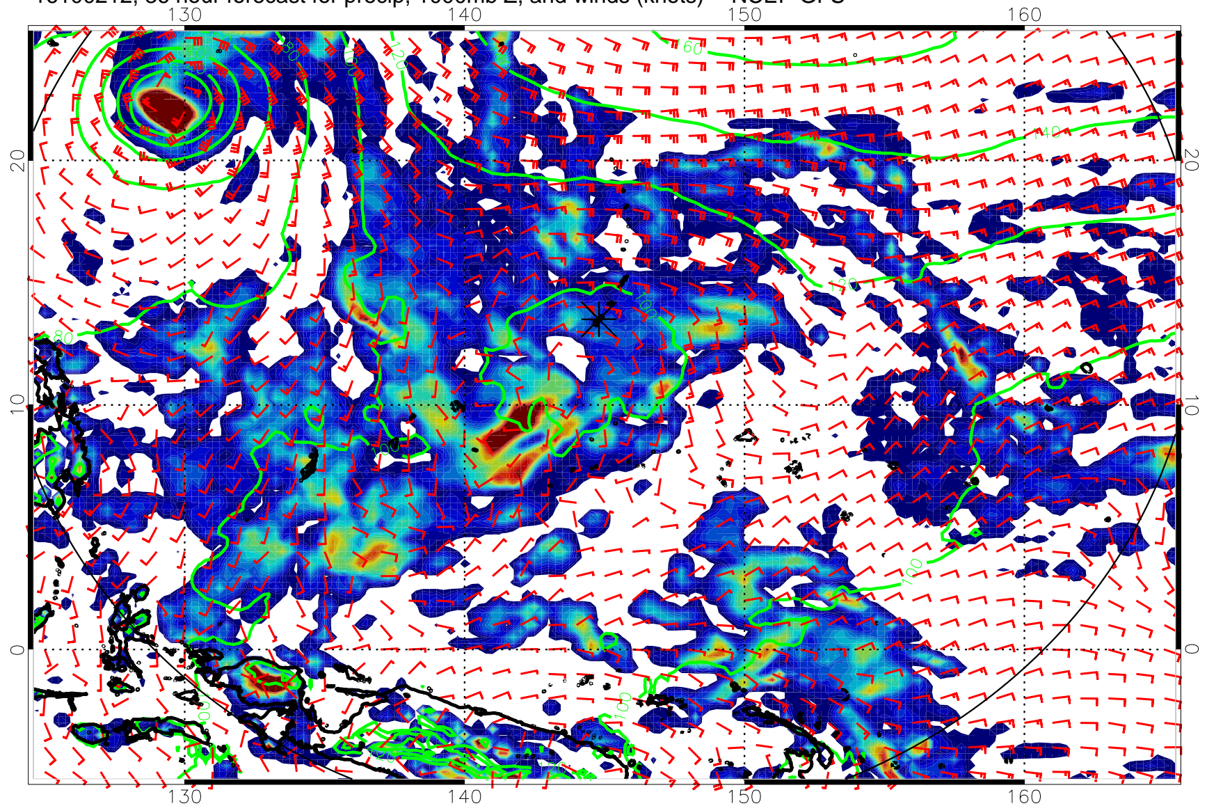
16100212, 36 hour forecast for precip, 1000mb Z, and winds (knots) -- NCEP GFS
