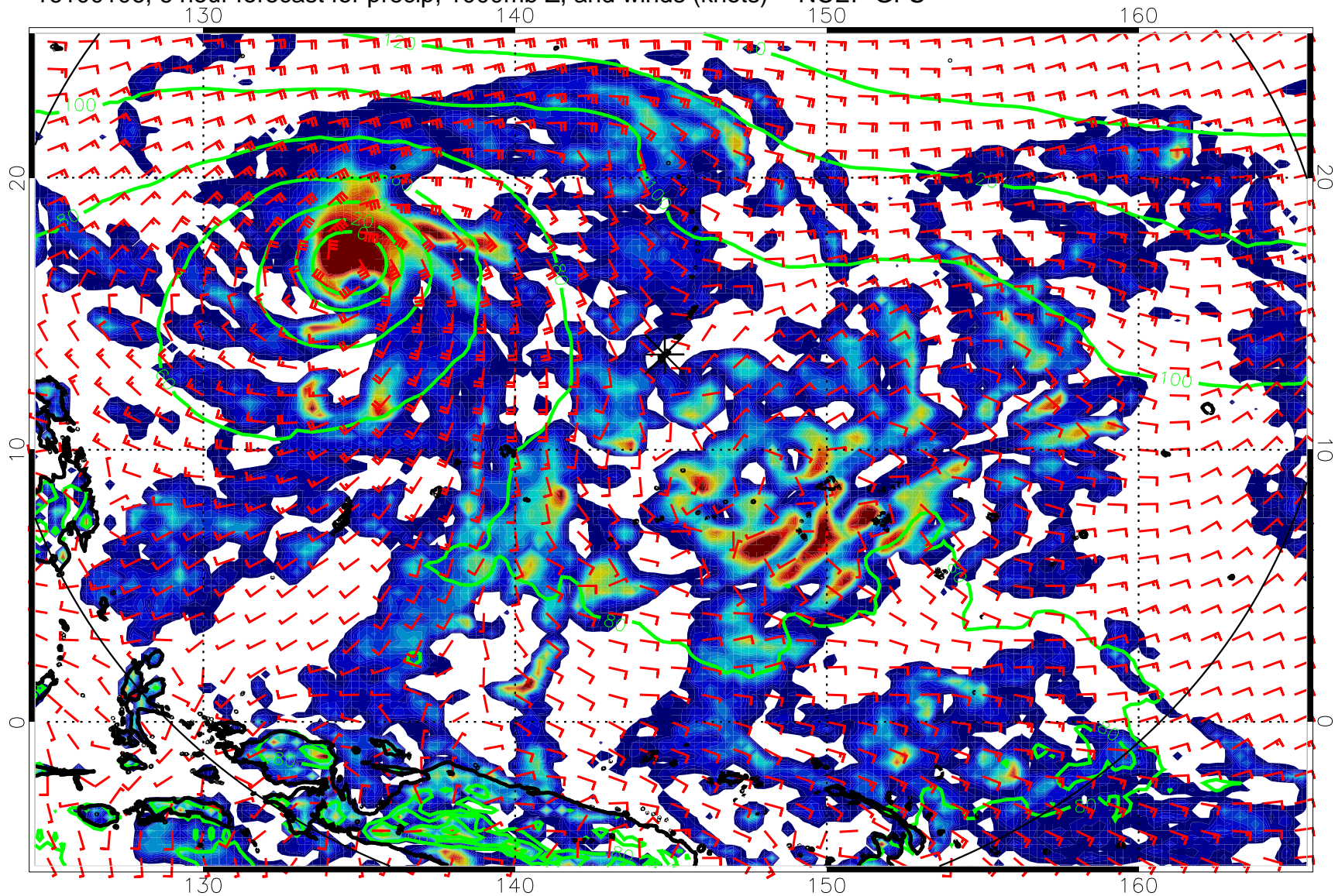
16100106, 6 hour forecast for precip, 1000mb Z, and winds (knots) -- NCEP GFS
