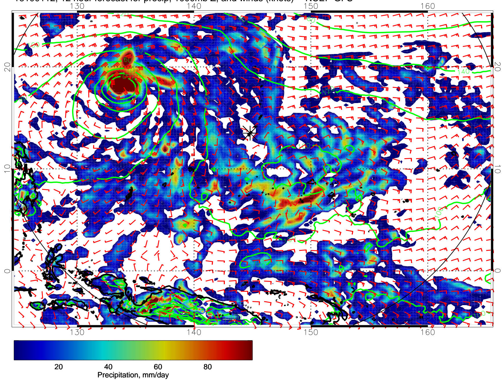
16100112, 12 hour forecast for precip, 1000mb Z, and winds (knots) -- NCEP GFS
