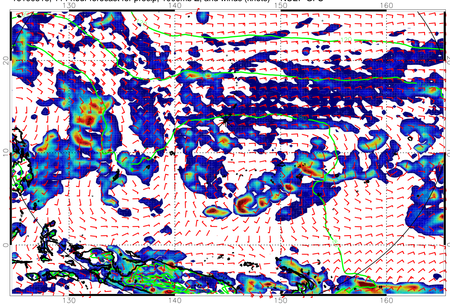
16100518, 114 hour forecast for precip, 1000mb Z, and winds (knots) -- NCEP GFS
