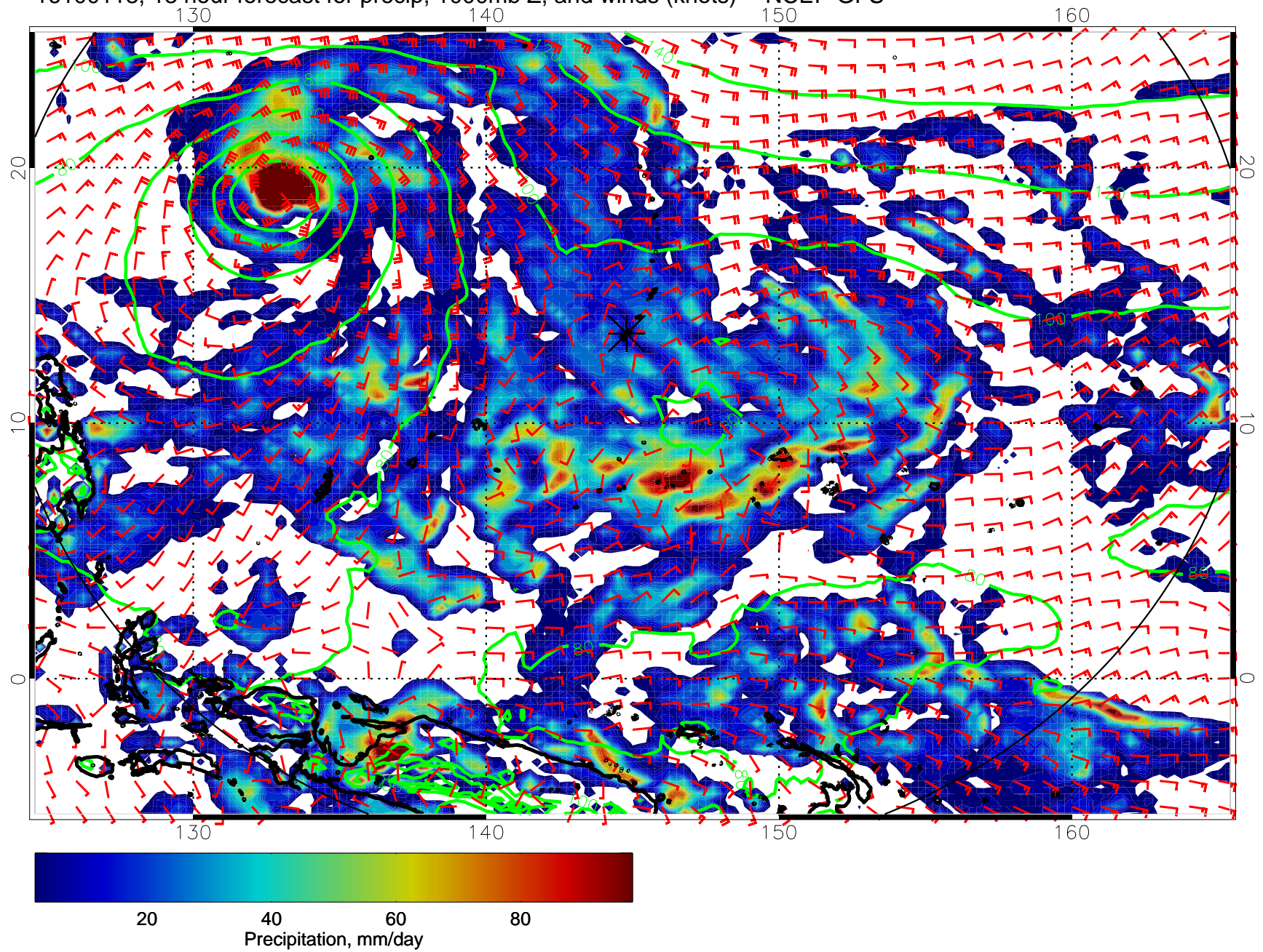
16100118, 18 hour forecast for precip, 1000mb Z, and winds (knots) -- NCEP GFS
