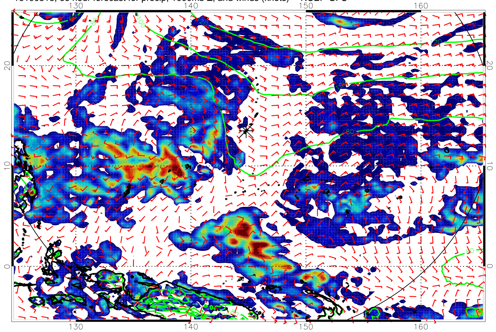
16100318, 66 hour forecast for precip, 1000mb Z, and winds (knots) -- NCEP GFS
