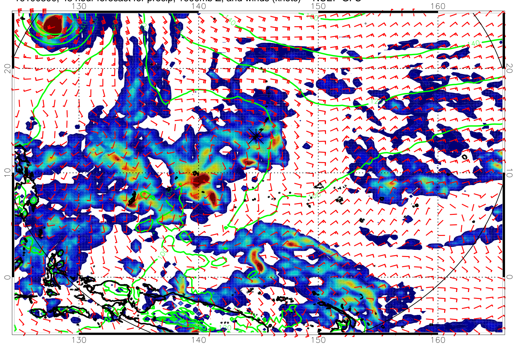
16100300, 48 hour forecast for precip, 1000mb Z, and winds (knots) -- NCEP GFS
