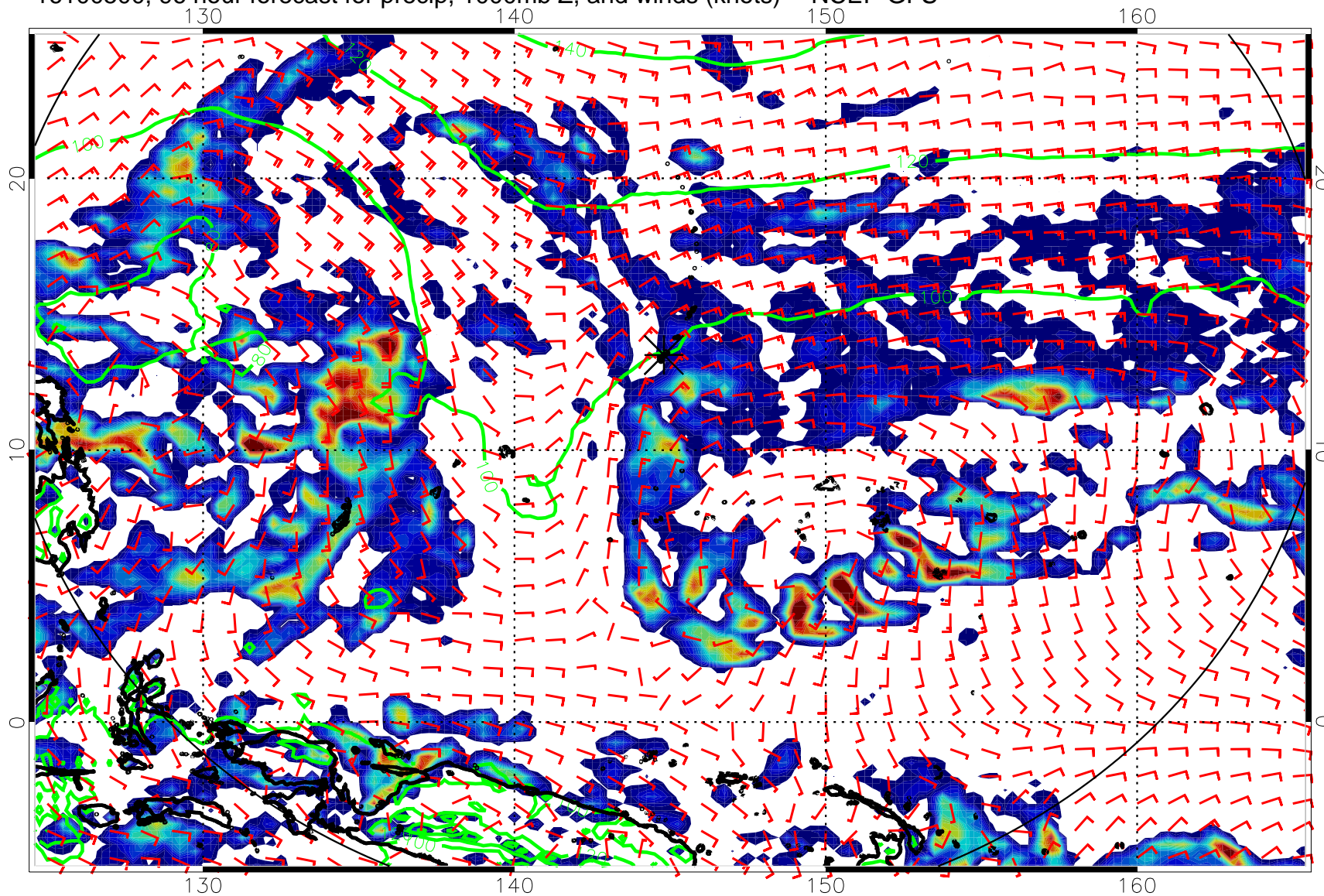
16100500, 96 hour forecast for precip, 1000mb Z, and winds (knots) -- NCEP GFS
