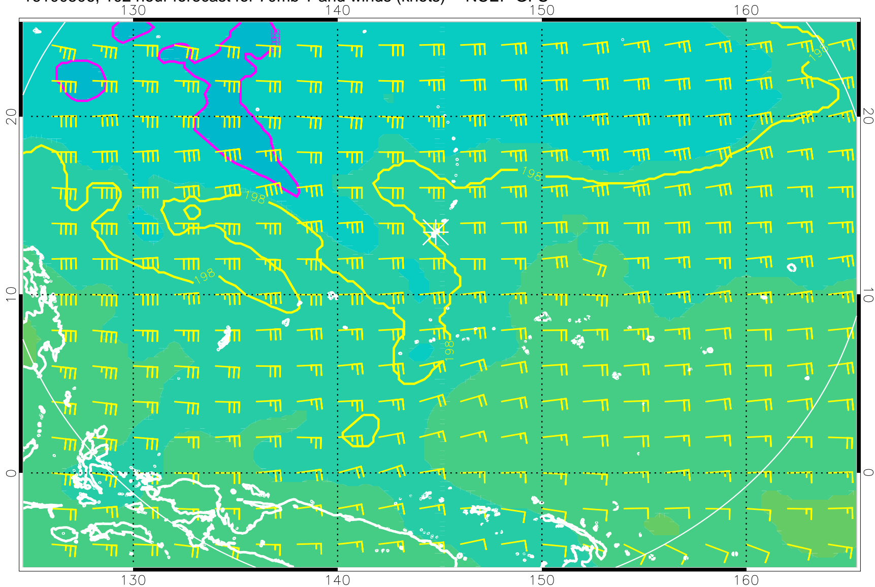
16100506, 102 hour forecast for 70mb T and winds (knots) -- NCEP GFS
