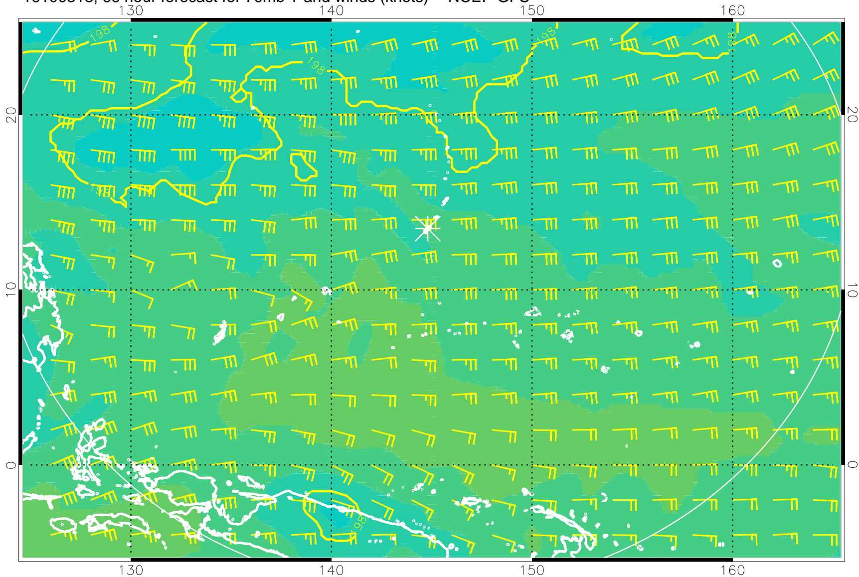
16100318, 66 hour forecast for 70mb T and winds (knots) -- NCEP GFS
