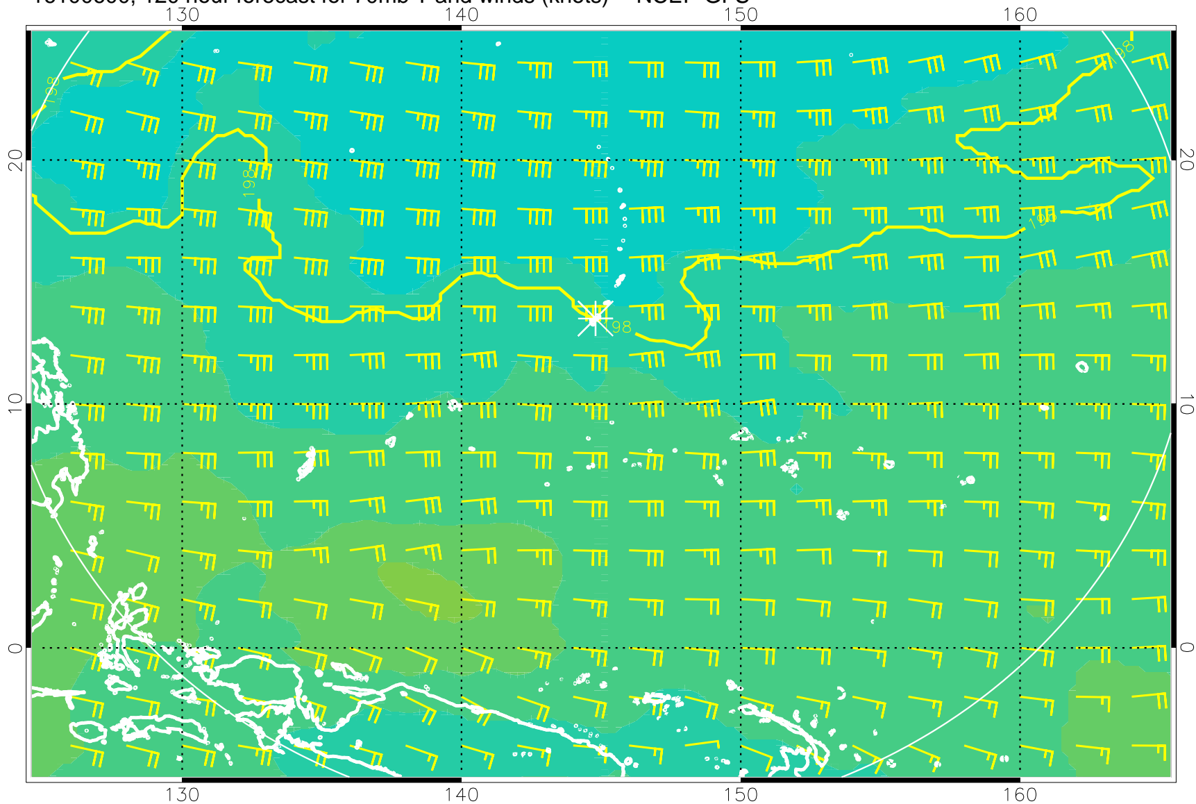
16100600, 120 hour forecast for 70mb T and winds (knots) -- NCEP GFS
