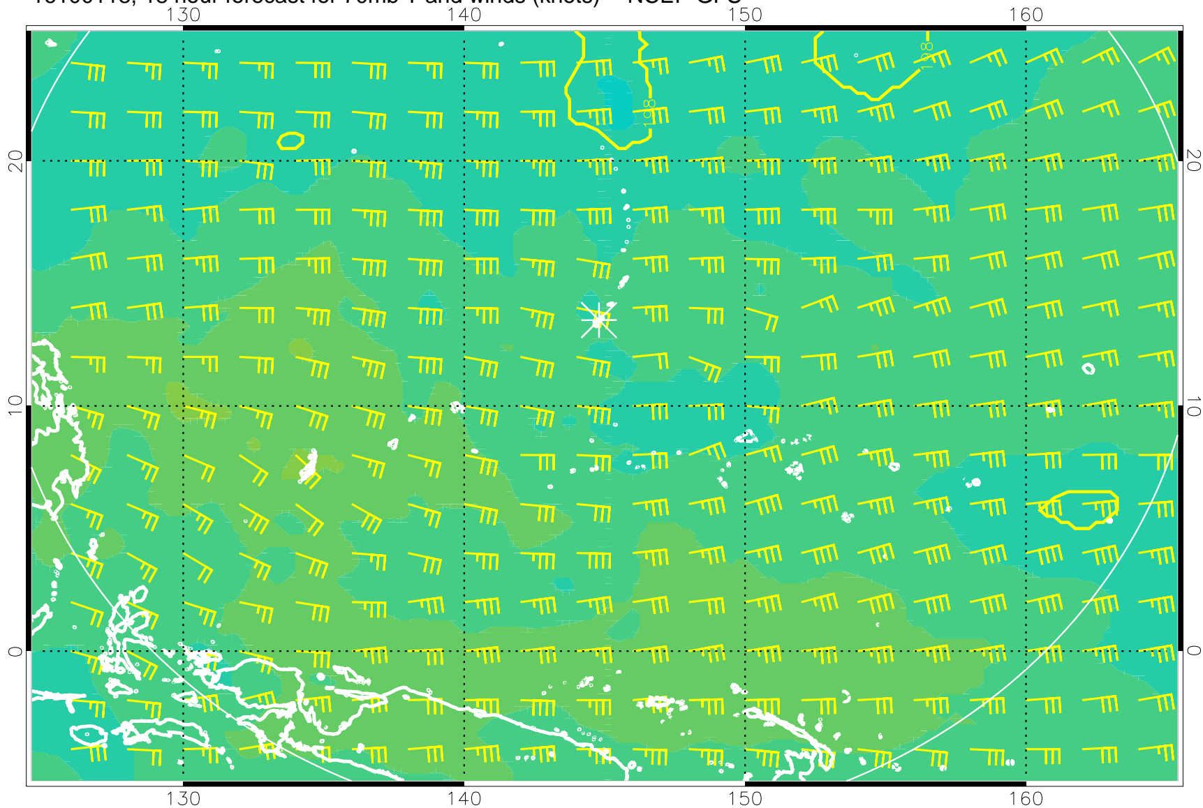
16100118, 18 hour forecast for 70mb T and winds (knots) -- NCEP GFS
