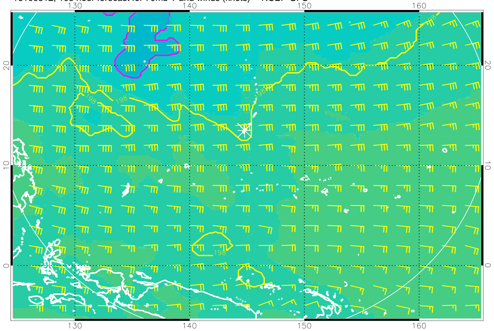
16100512, 108 hour forecast for 70mb T and winds (knots) -- NCEP GFS
