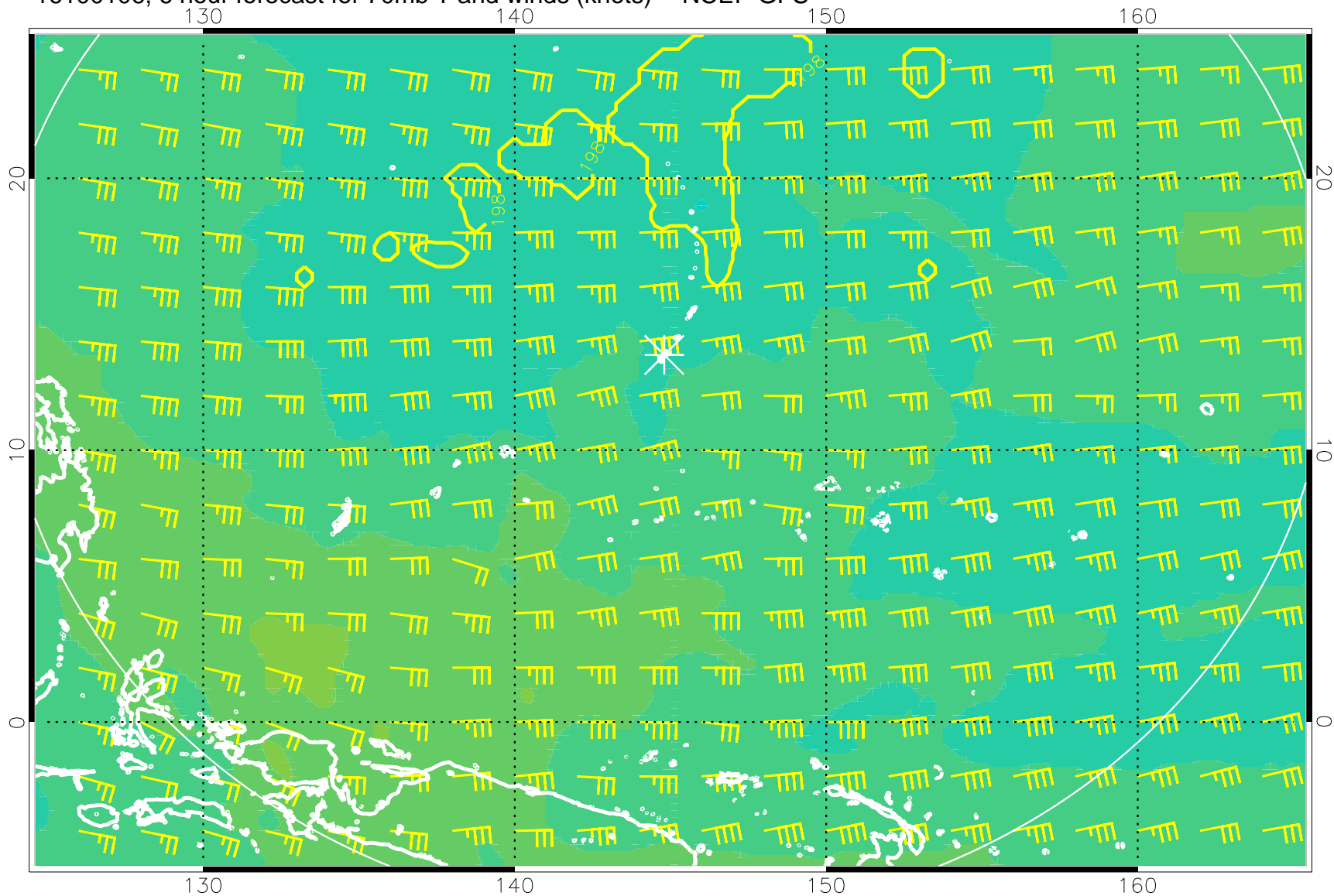
16100106, 6 hour forecast for 70mb T and winds (knots) -- NCEP GFS
