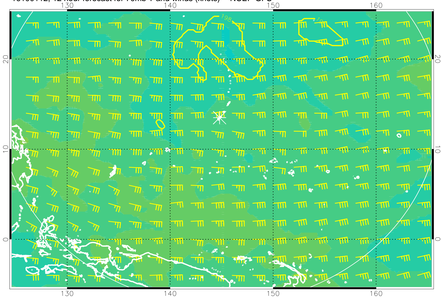
16100112, 12 hour forecast for 70mb T and winds (knots) -- NCEP GFS
