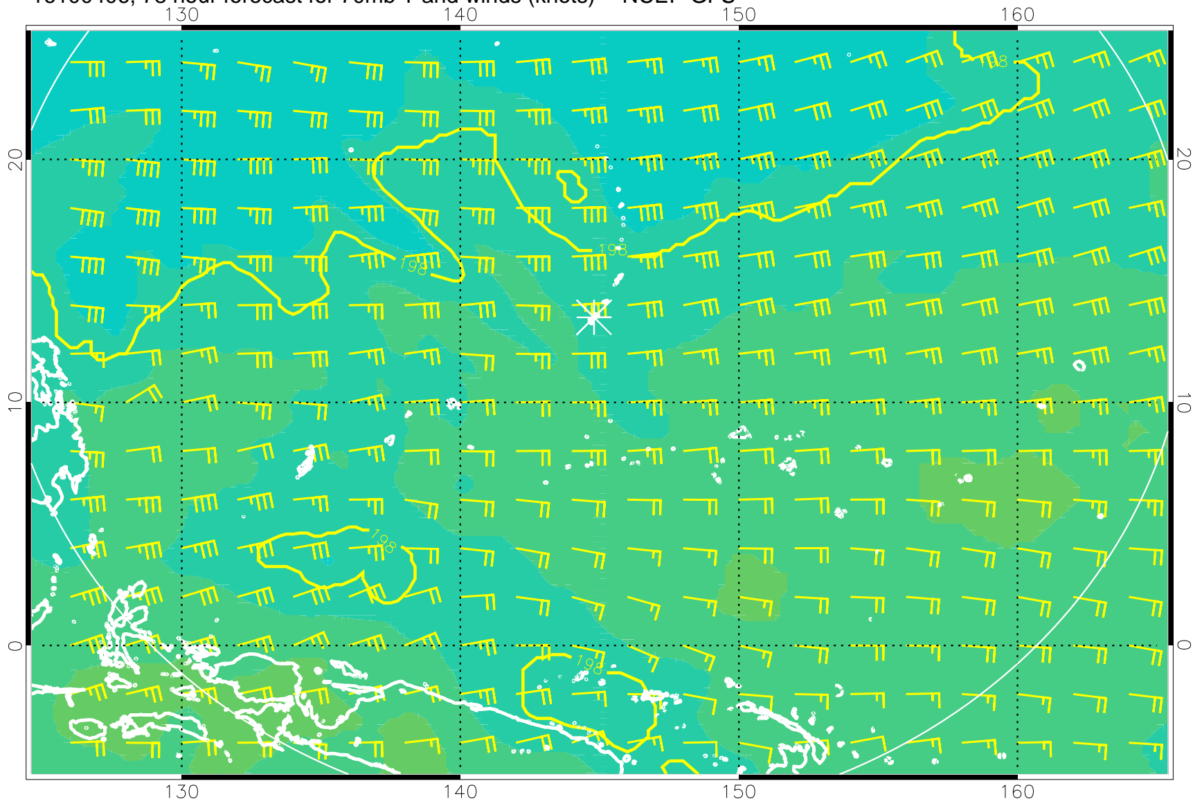
16100406, 78 hour forecast for 70mb T and winds (knots) -- NCEP GFS
