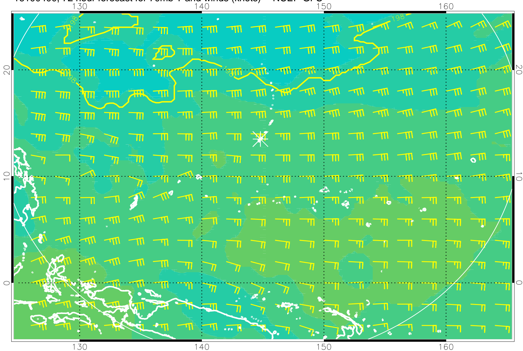
16100400, 72 hour forecast for 70mb T and winds (knots) -- NCEP GFS
