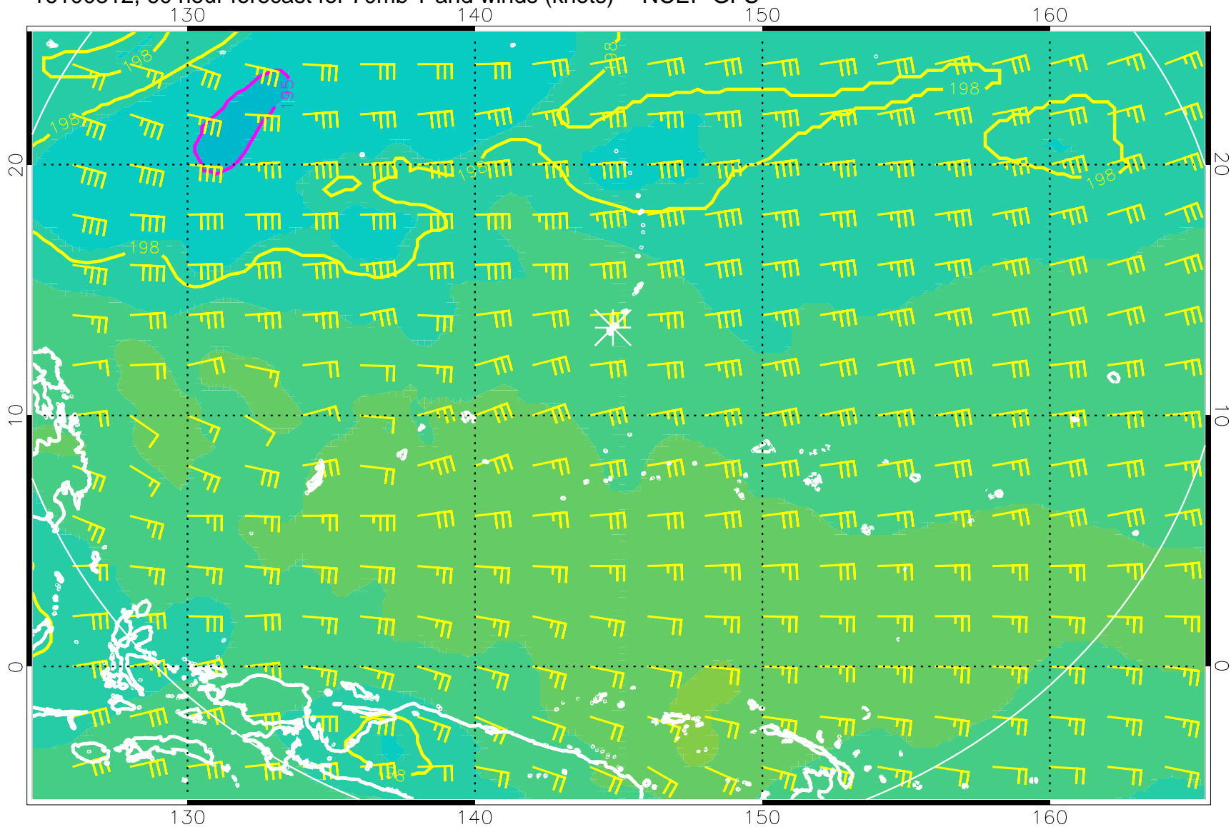
16100312, 60 hour forecast for 70mb T and winds (knots) -- NCEP GFS
