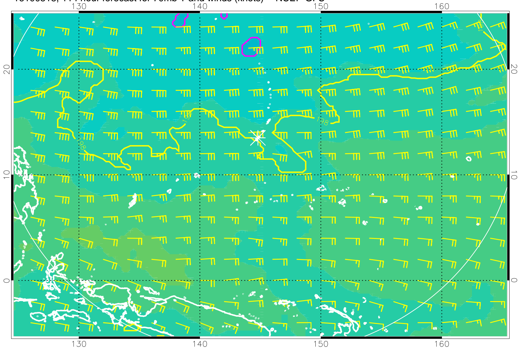
16100518, 114 hour forecast for 70mb T and winds (knots) -- NCEP GFS
