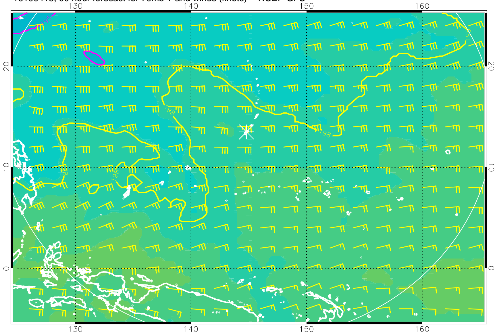
16100418, 90 hour forecast for 70mb T and winds (knots) -- NCEP GFS
