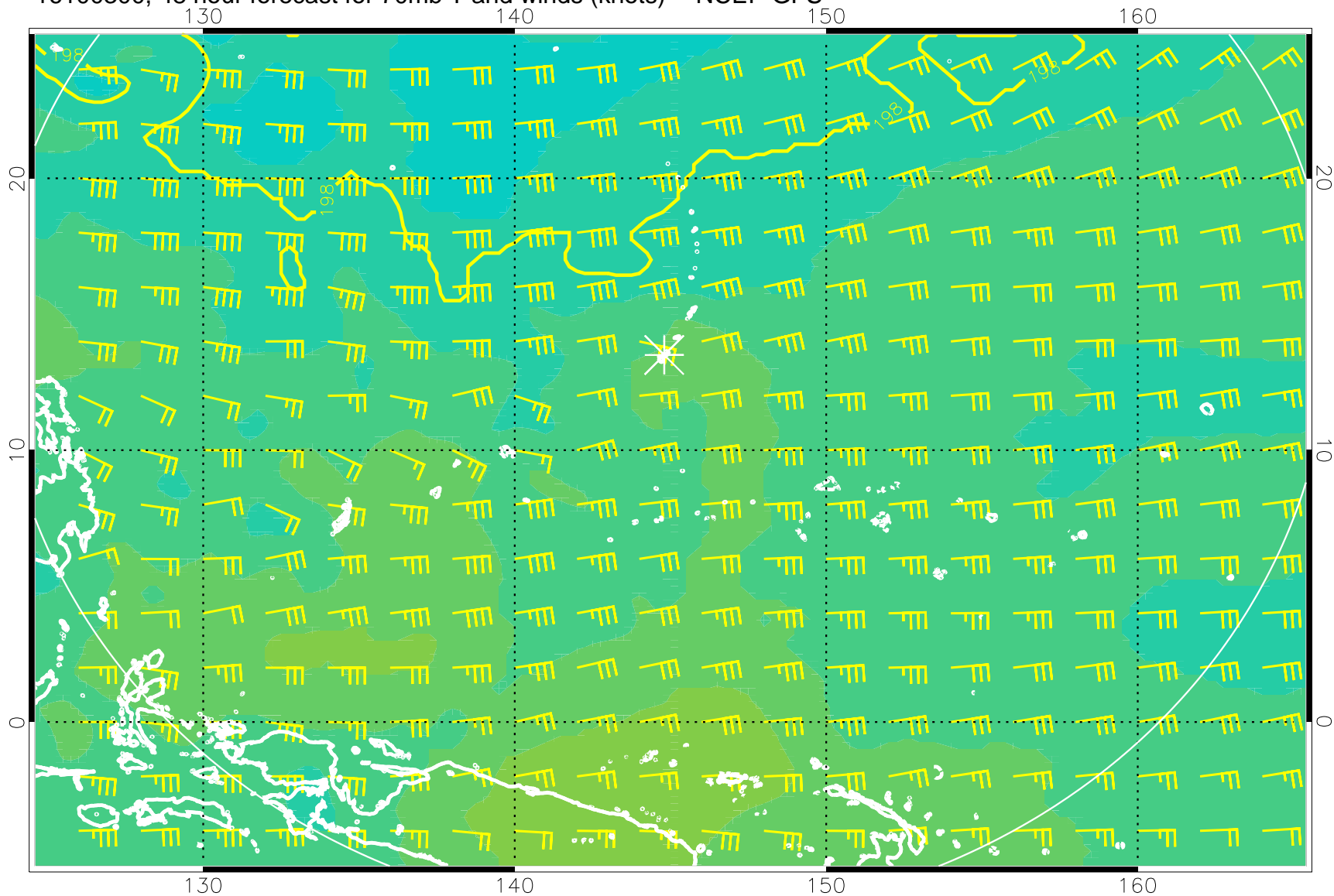
16100300, 48 hour forecast for 70mb T and winds (knots) -- NCEP GFS
