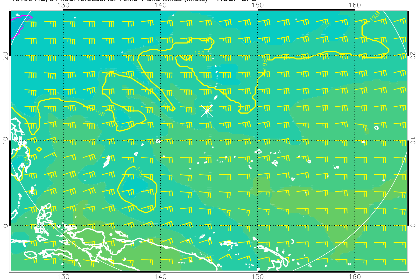
16100412, 84 hour forecast for 70mb T and winds (knots) -- NCEP GFS
