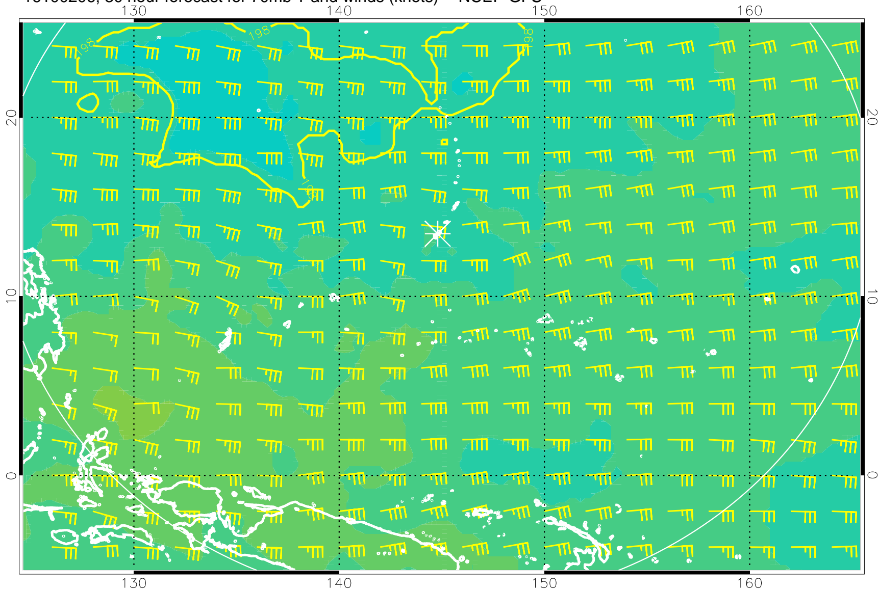
16100206, 30 hour forecast for 70mb T and winds (knots) -- NCEP GFS
