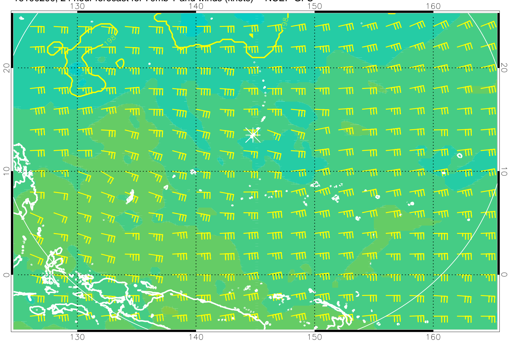
16100200, 24 hour forecast for 70mb T and winds (knots) -- NCEP GFS
