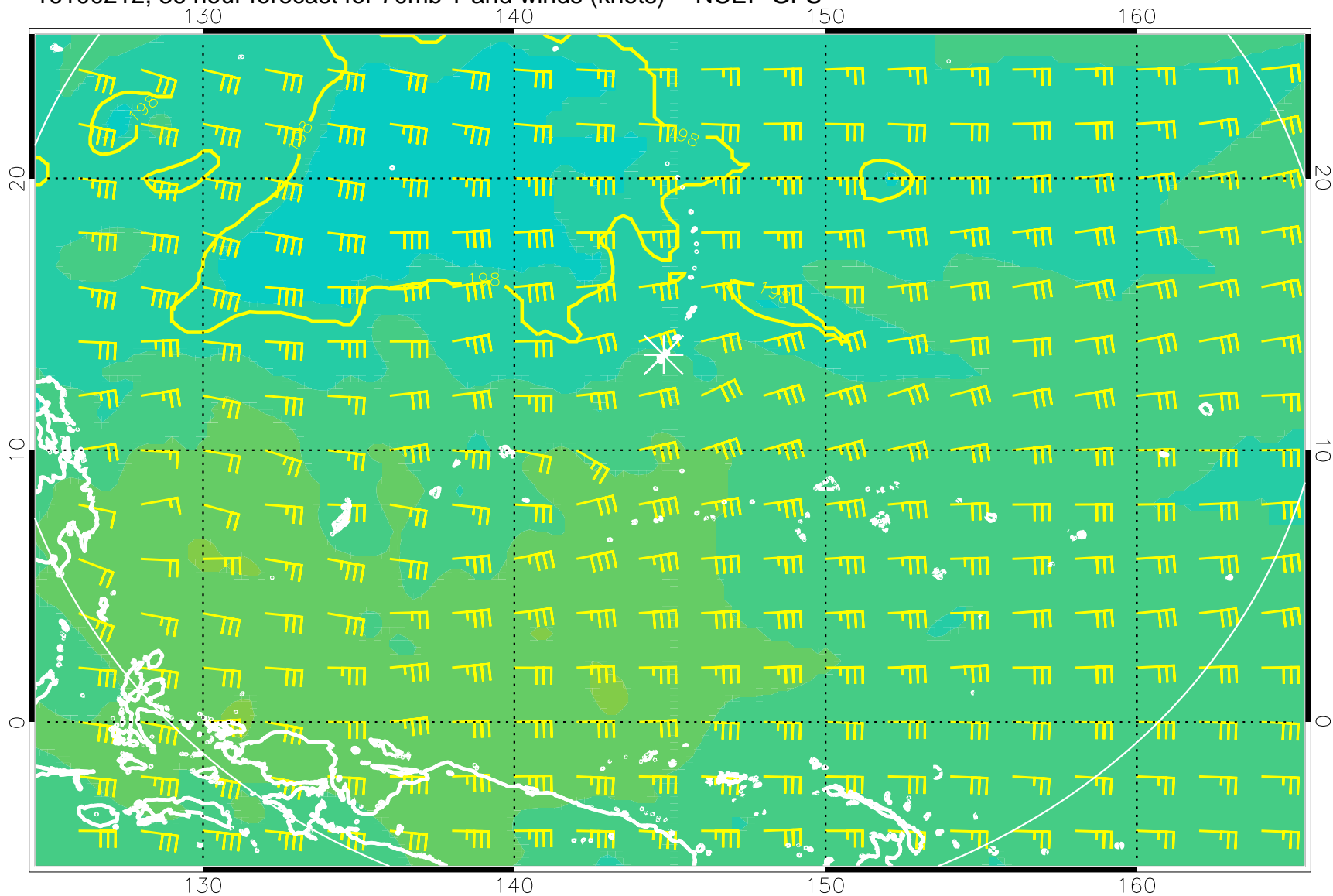
16100212, 36 hour forecast for 70mb T and winds (knots) -- NCEP GFS
