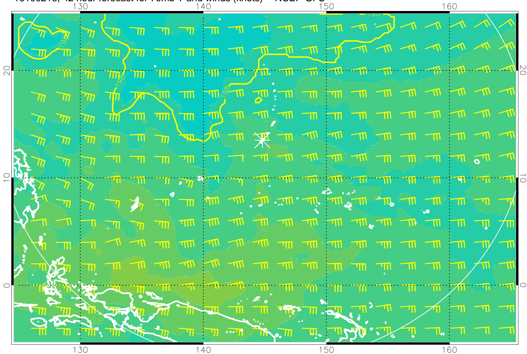
16100218, 42 hour forecast for 70mb T and winds (knots) -- NCEP GFS
