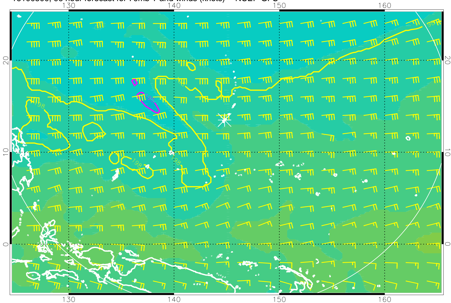
16100500, 96 hour forecast for 70mb T and winds (knots) -- NCEP GFS
