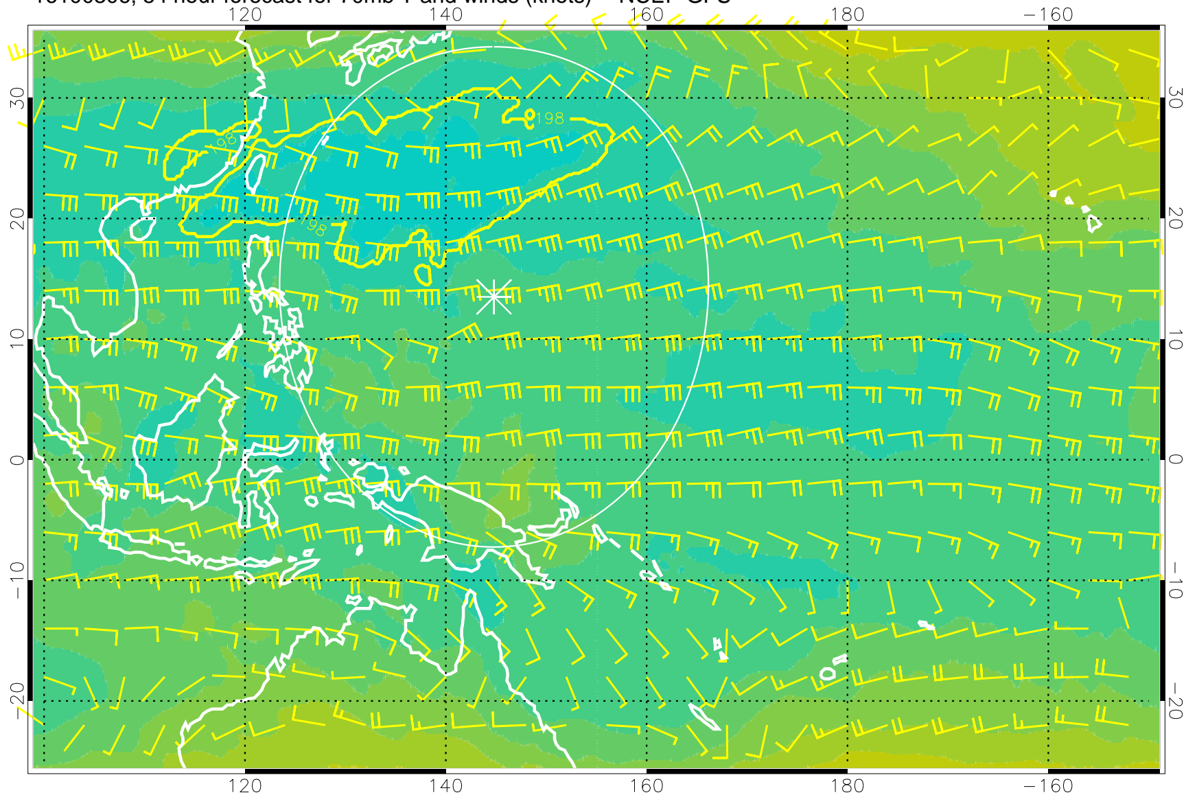
16100306, 54 hour forecast for 70mb T and winds (knots) -- NCEP GFS
