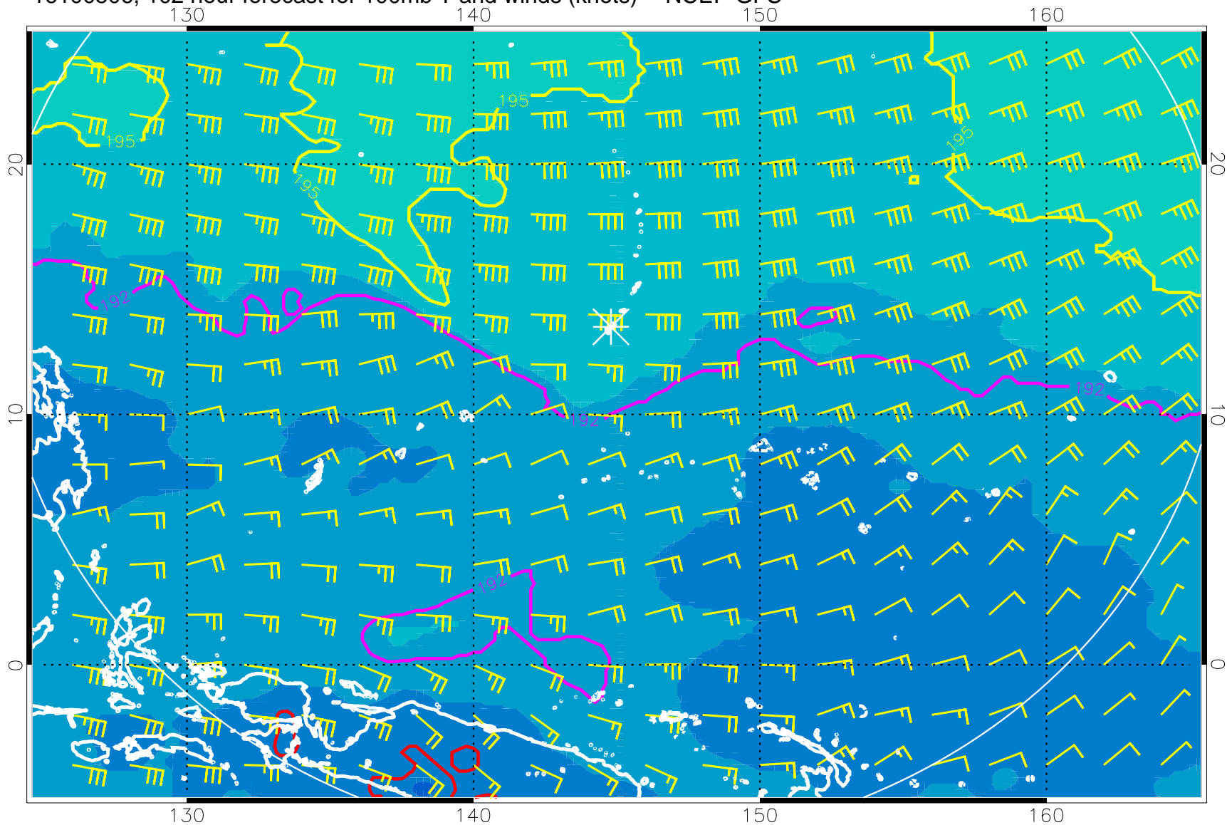
16100506, 102 hour forecast for 100mb T and winds (knots) -- NCEP GFS
