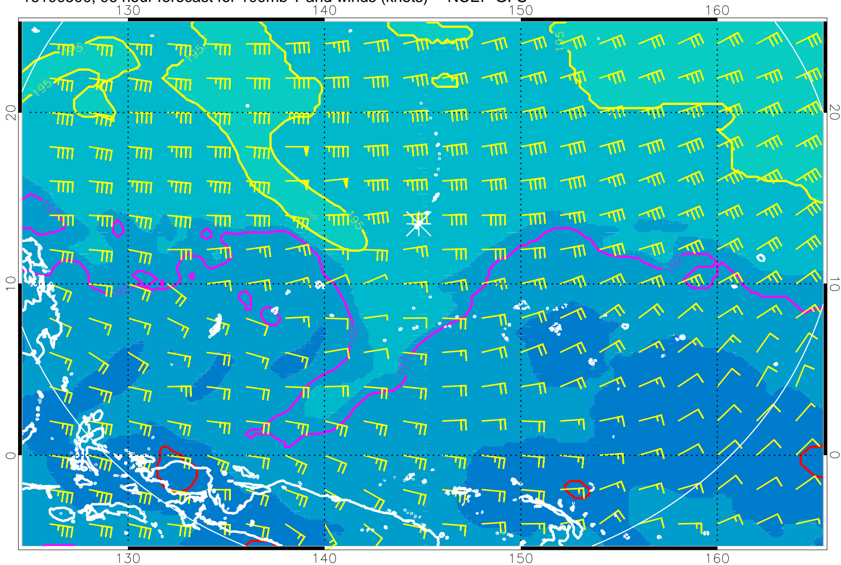
16100500, 96 hour forecast for 100mb T and winds (knots) -- NCEP GFS
