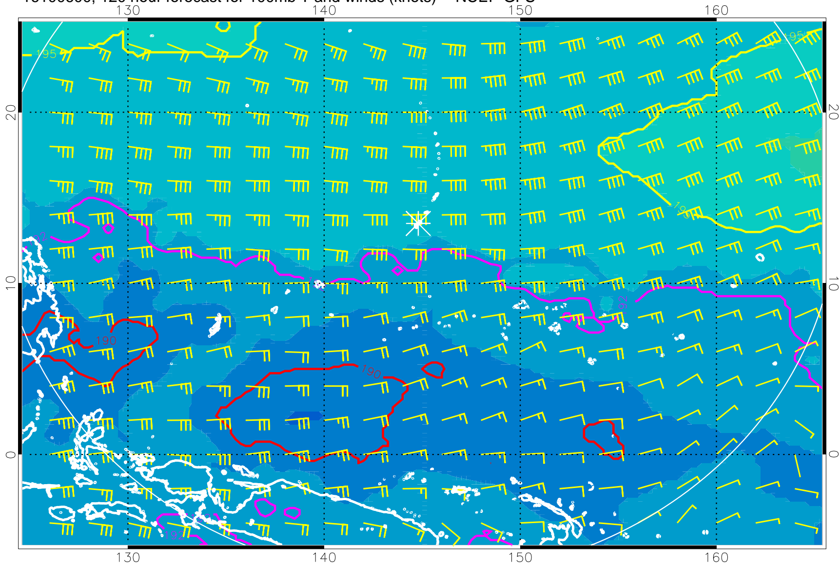
16100600, 120 hour forecast for 100mb T and winds (knots) -- NCEP GFS
