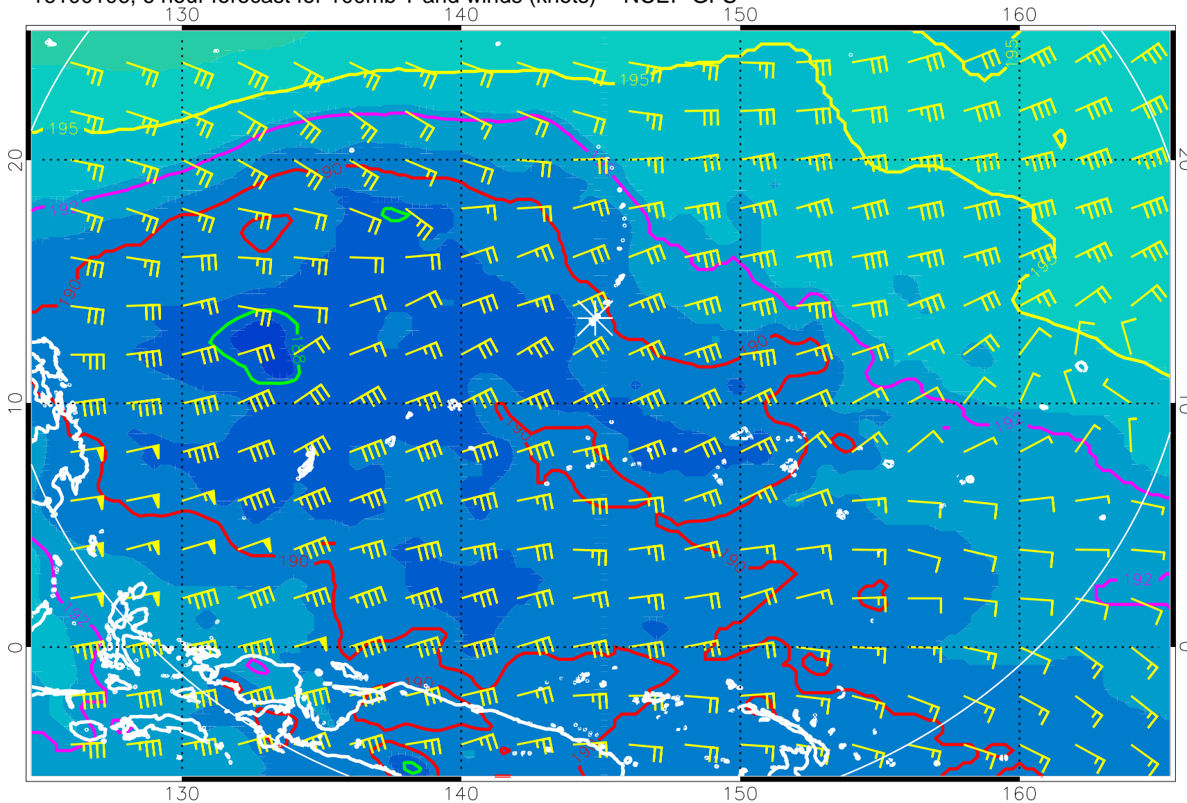
16100106, 6 hour forecast for 100mb T and winds (knots) -- NCEP GFS
