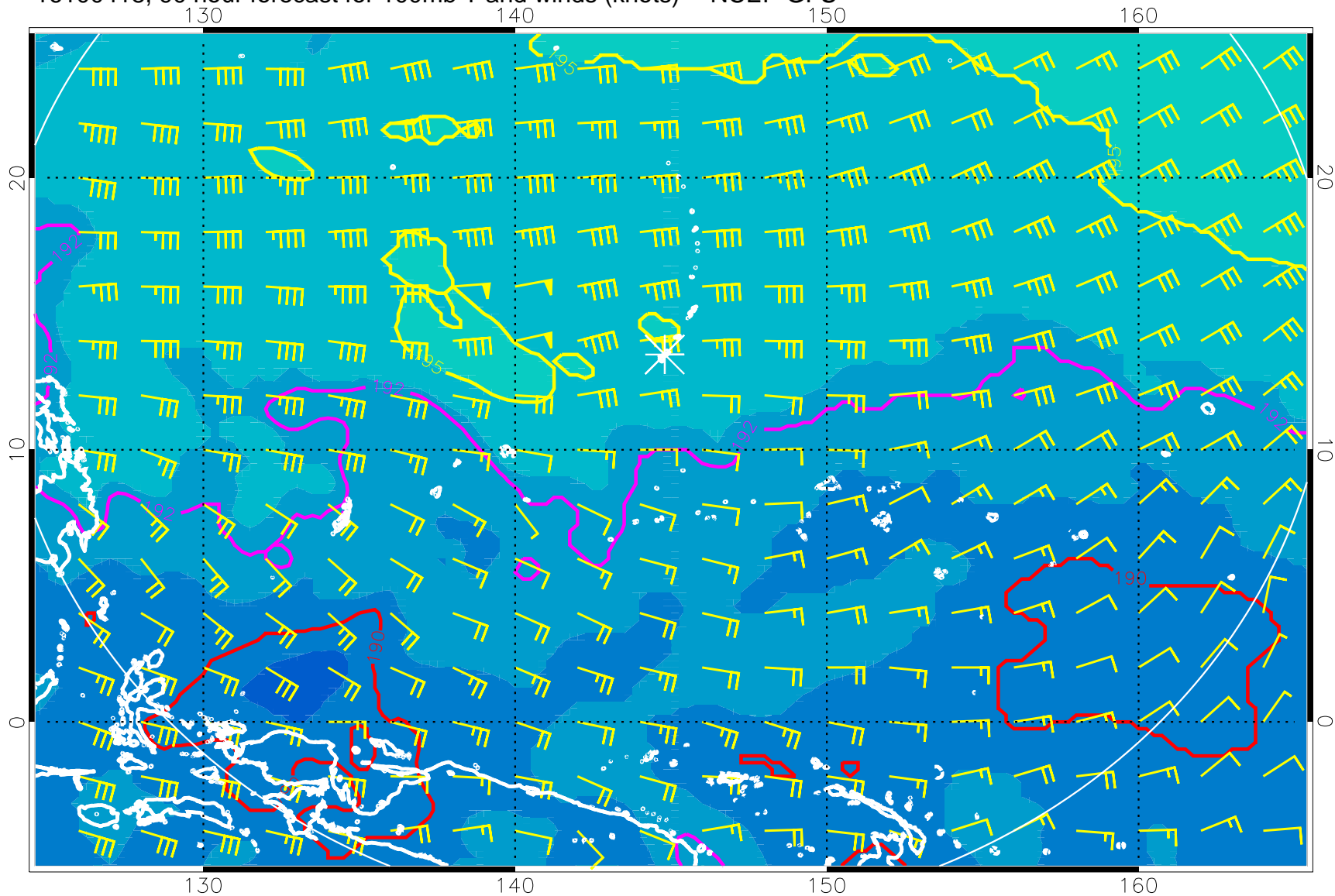
16100418, 90 hour forecast for 100mb T and winds (knots) -- NCEP GFS
