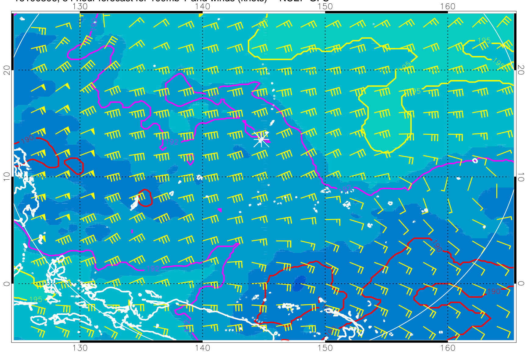
16100306, 54 hour forecast for 100mb T and winds (knots) -- NCEP GFS
