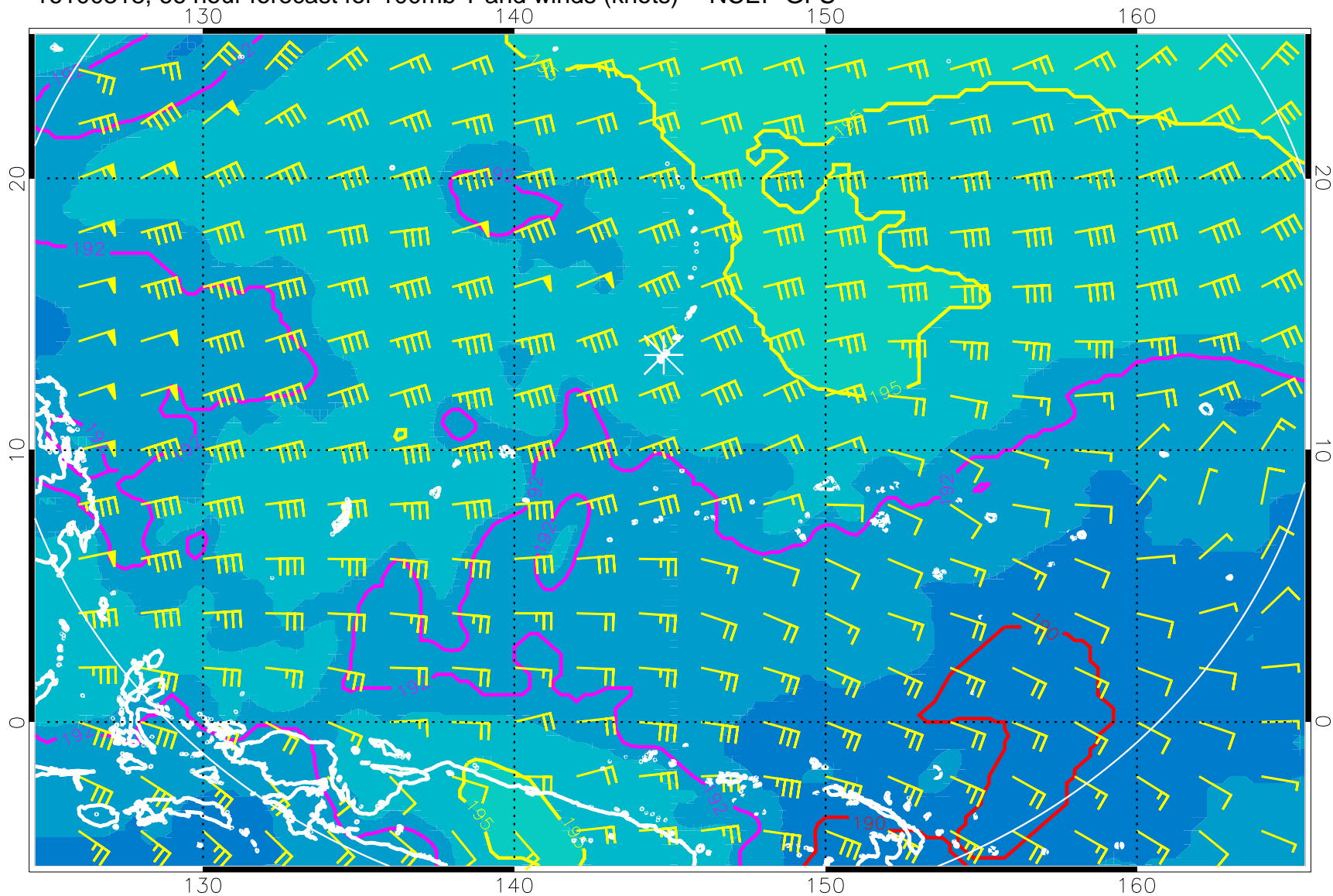
16100318, 66 hour forecast for 100mb T and winds (knots) -- NCEP GFS
