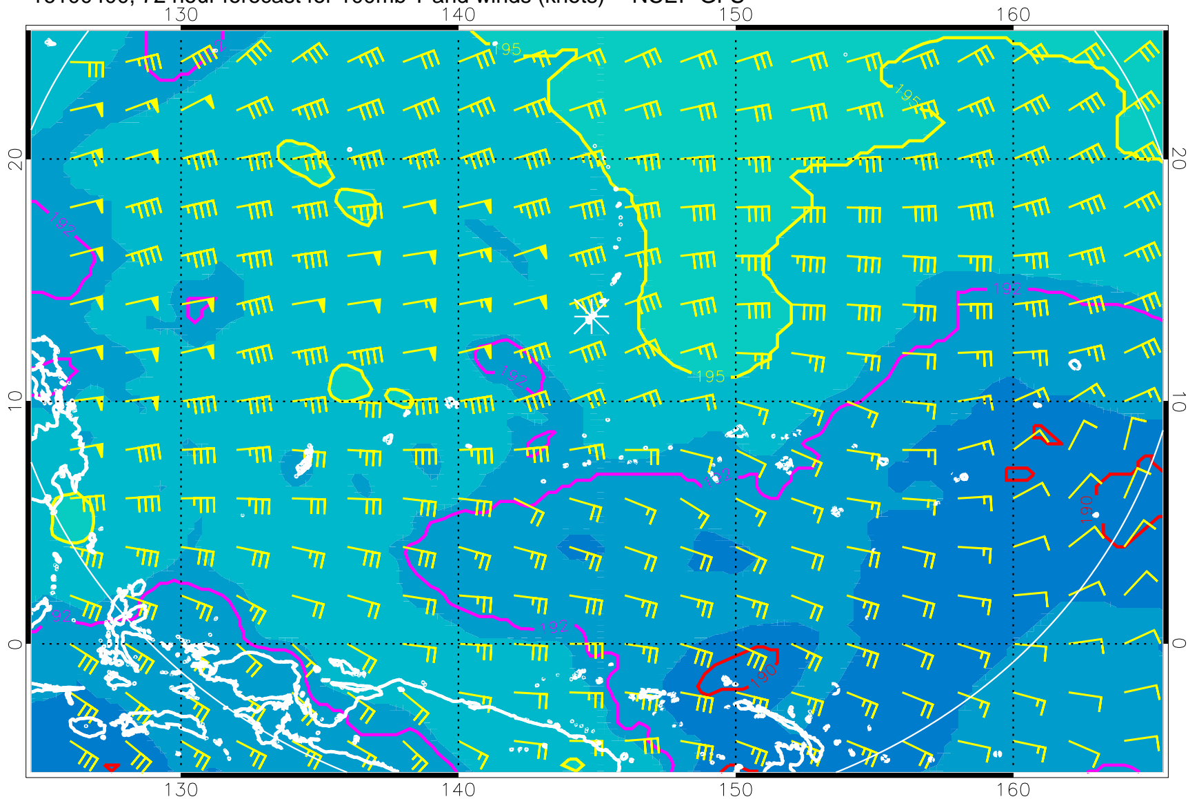
16100400, 72 hour forecast for 100mb T and winds (knots) -- NCEP GFS
