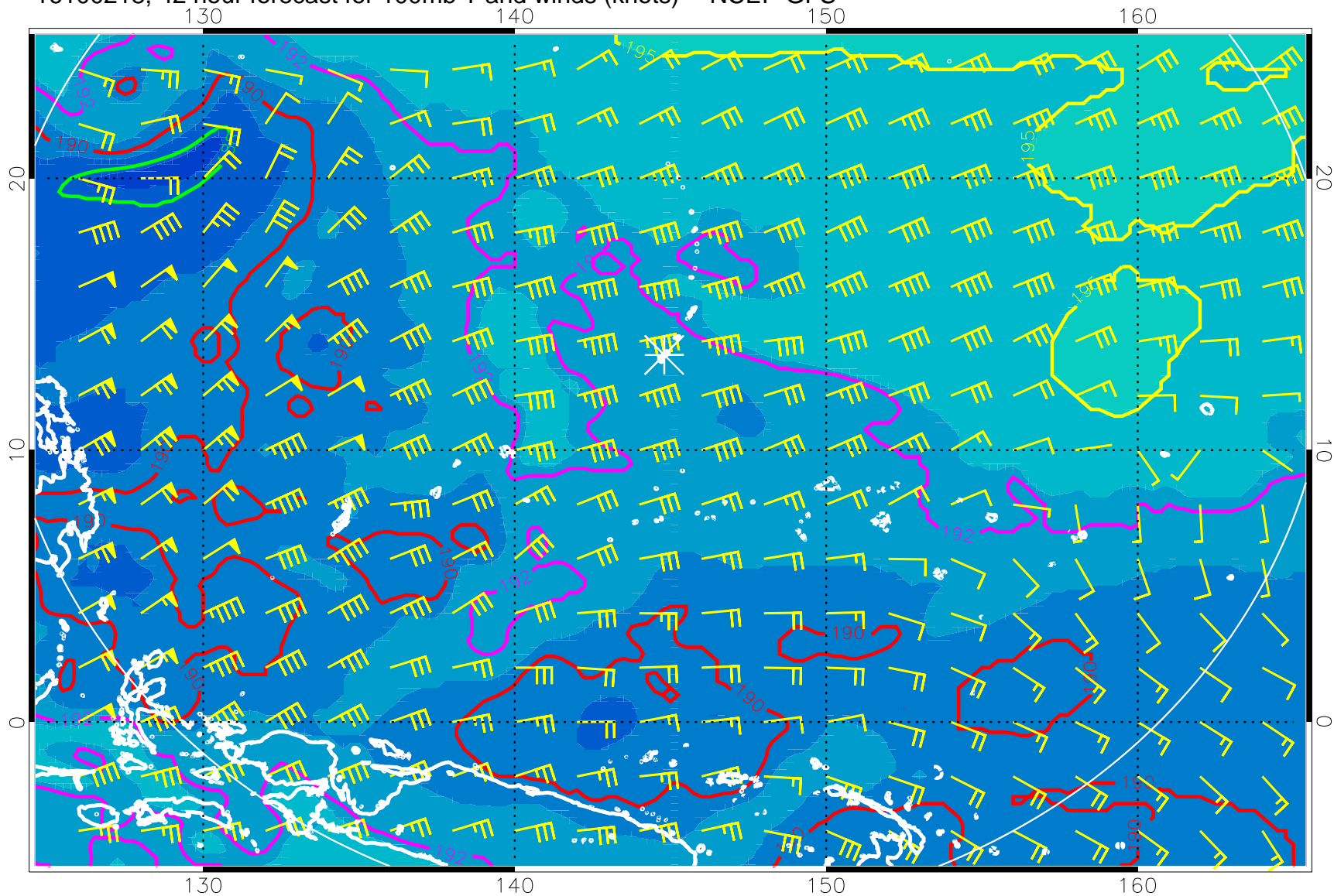
16100218, 42 hour forecast for 100mb T and winds (knots) -- NCEP GFS
