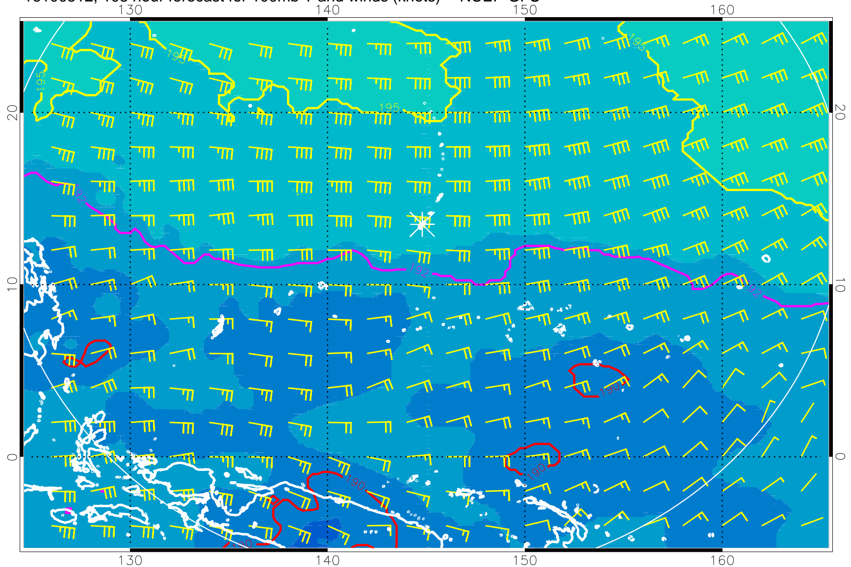
16100512, 108 hour forecast for 100mb T and winds (knots) -- NCEP GFS
