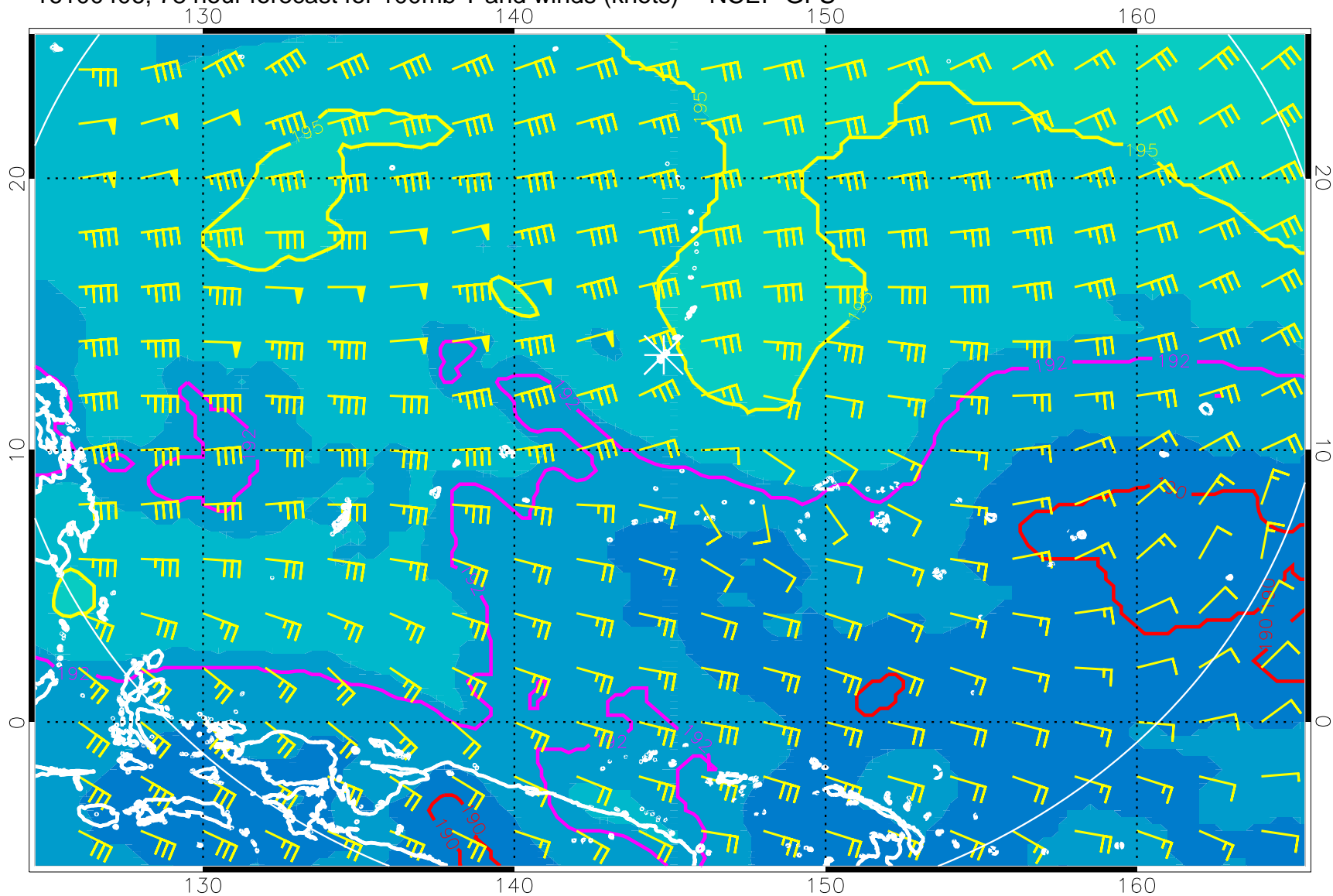
16100406, 78 hour forecast for 100mb T and winds (knots) -- NCEP GFS
