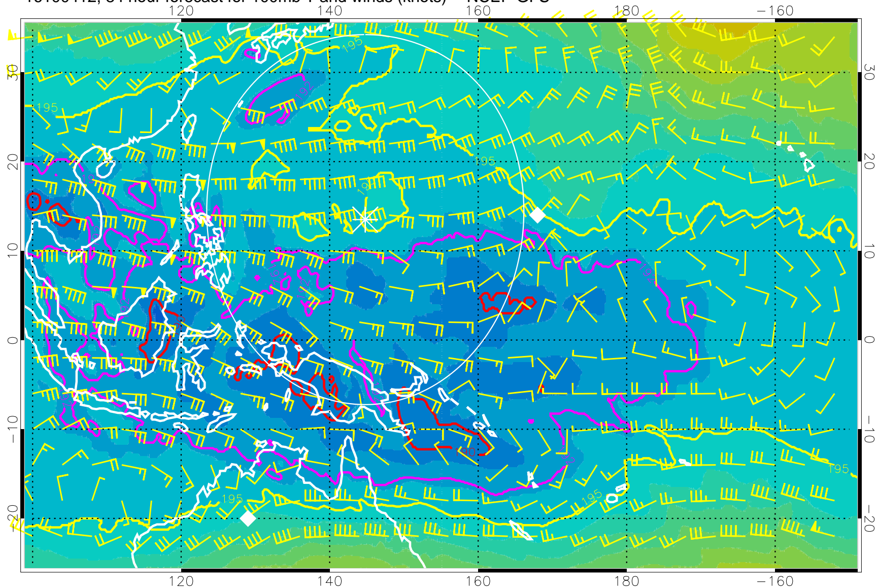
16100412, 84 hour forecast for 100mb T and winds (knots) -- NCEP GFS
