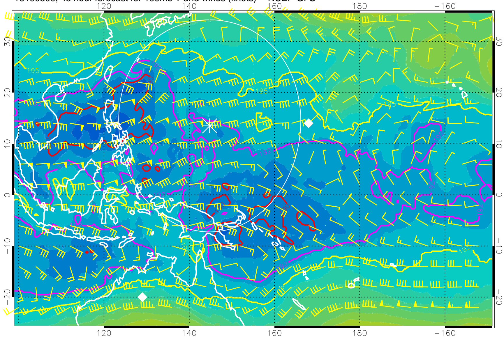
16100300, 48 hour forecast for 100mb T and winds (knots) -- NCEP GFS
