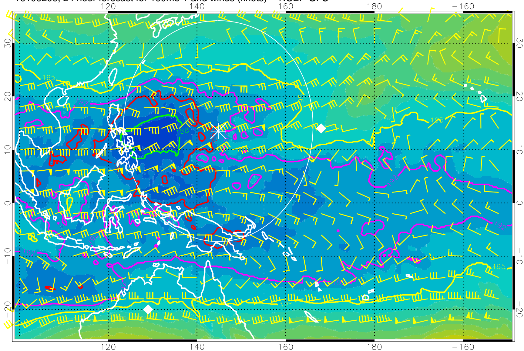
16100200, 24 hour forecast for 100mb T and winds (knots) -- NCEP GFS
