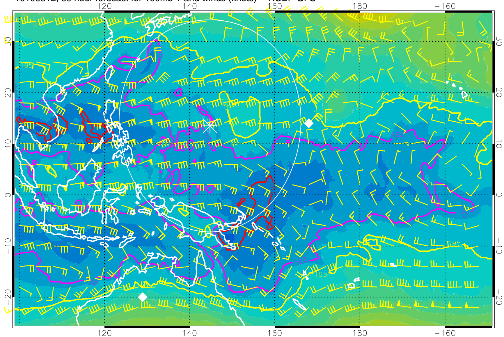
16100312, 60 hour forecast for 100mb T and winds (knots) -- NCEP GFS
