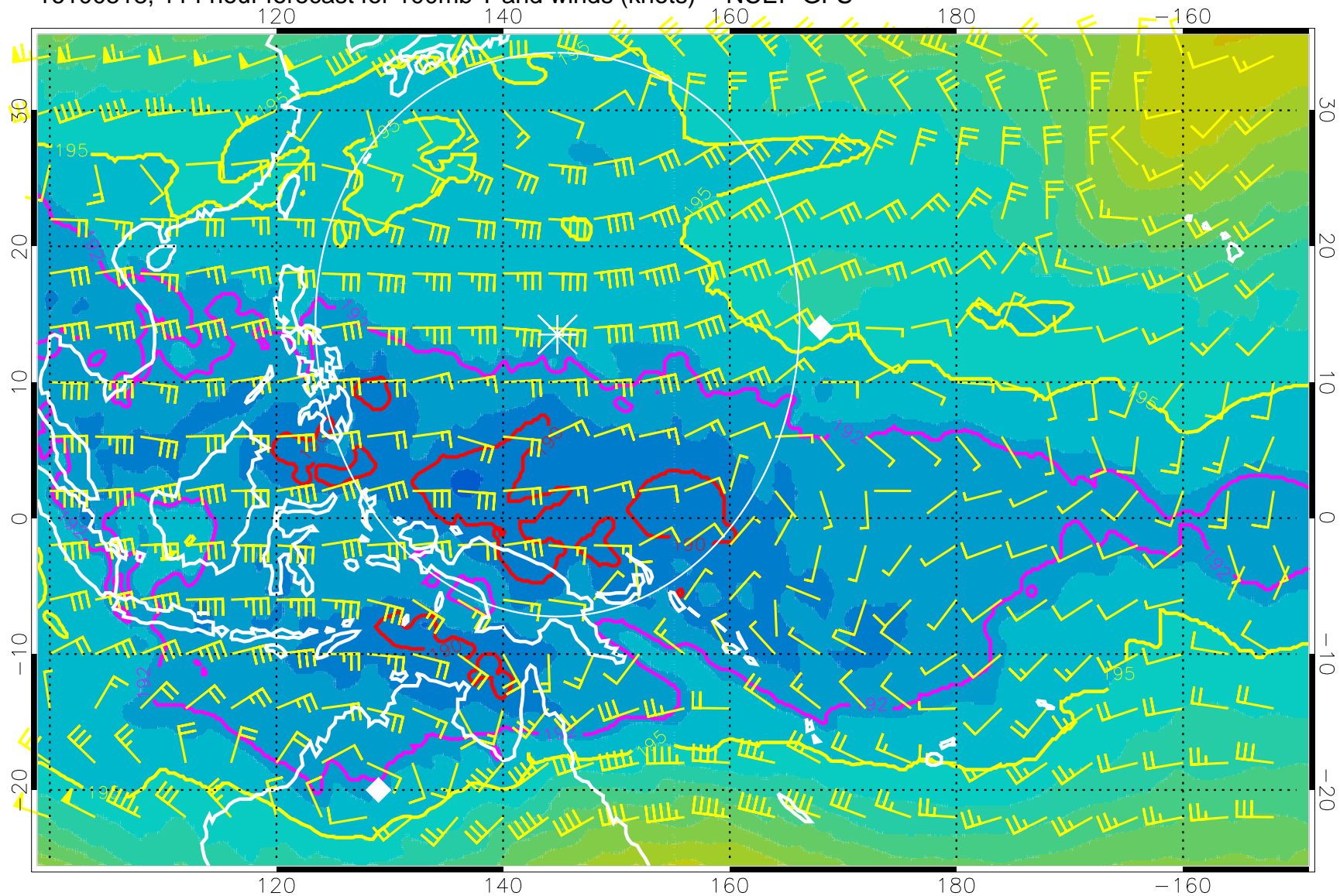
16100518, 114 hour forecast for 100mb T and winds (knots) -- NCEP GFS
