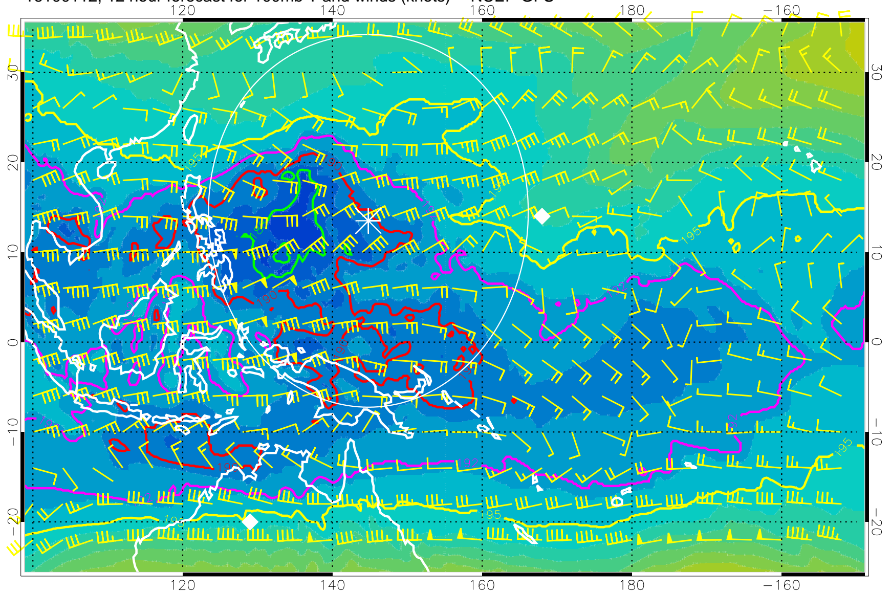
16100112, 12 hour forecast for 100mb T and winds (knots) -- NCEP GFS
