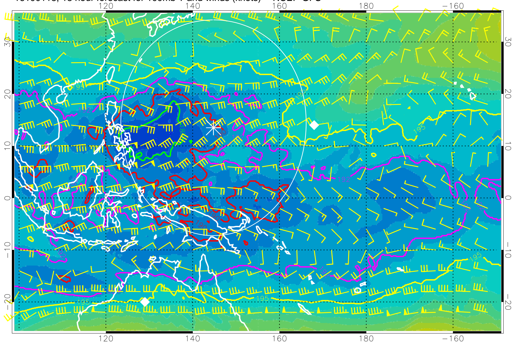
16100118, 18 hour forecast for 100mb T and winds (knots) -- NCEP GFS
