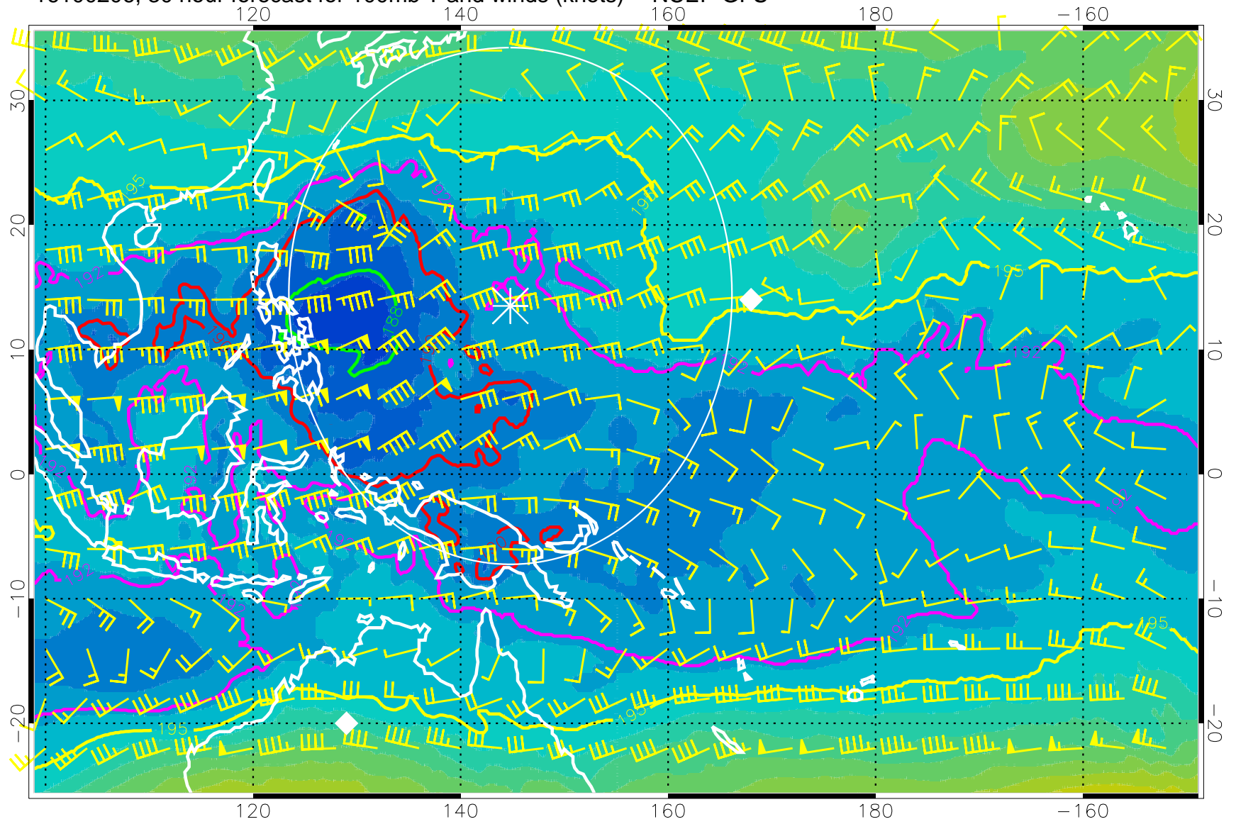
16100206, 30 hour forecast for 100mb T and winds (knots) -- NCEP GFS
