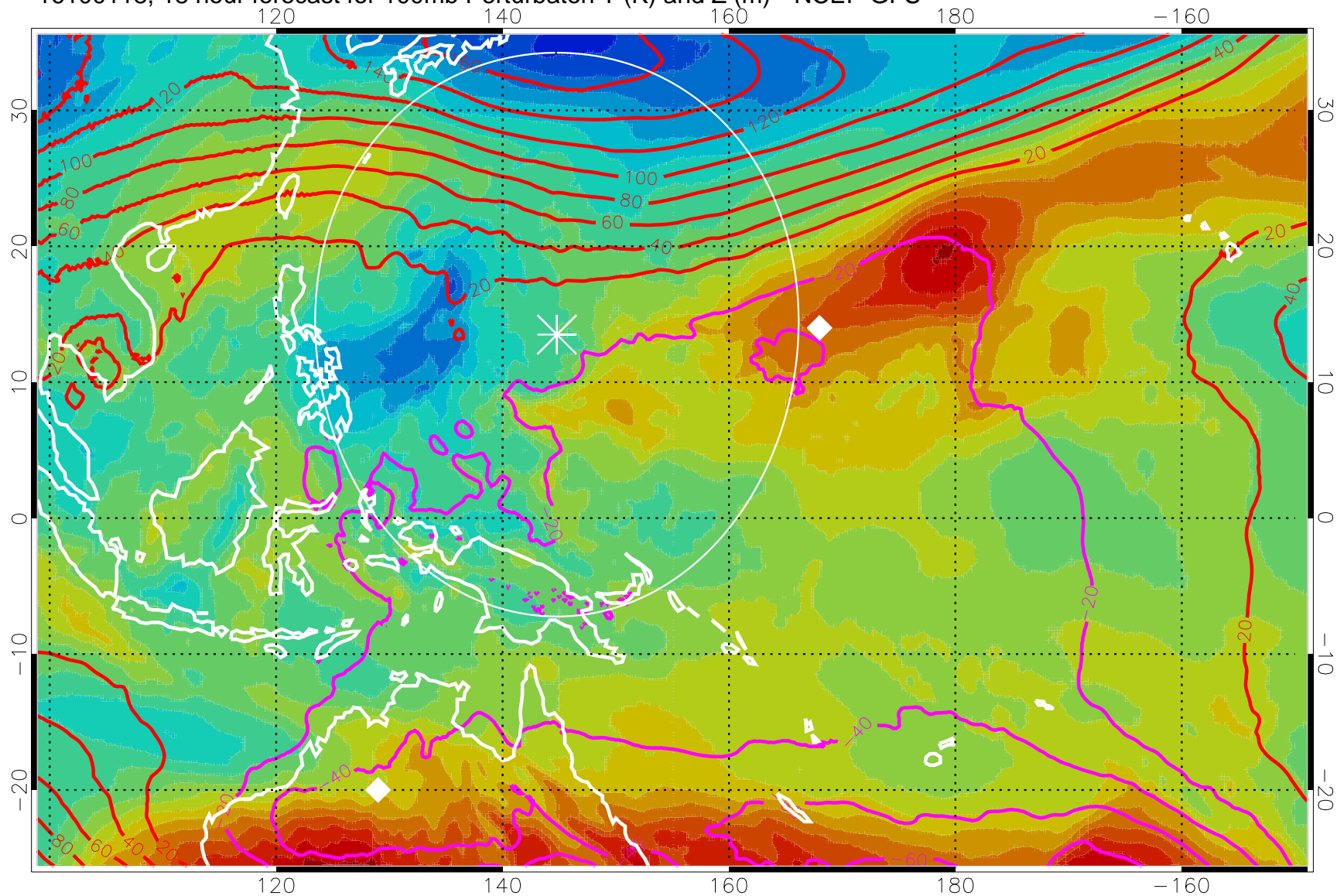
16100118, 18 hour forecast for 100mb Perturbaton T (K) and Z (m)-- NCEP GFS
