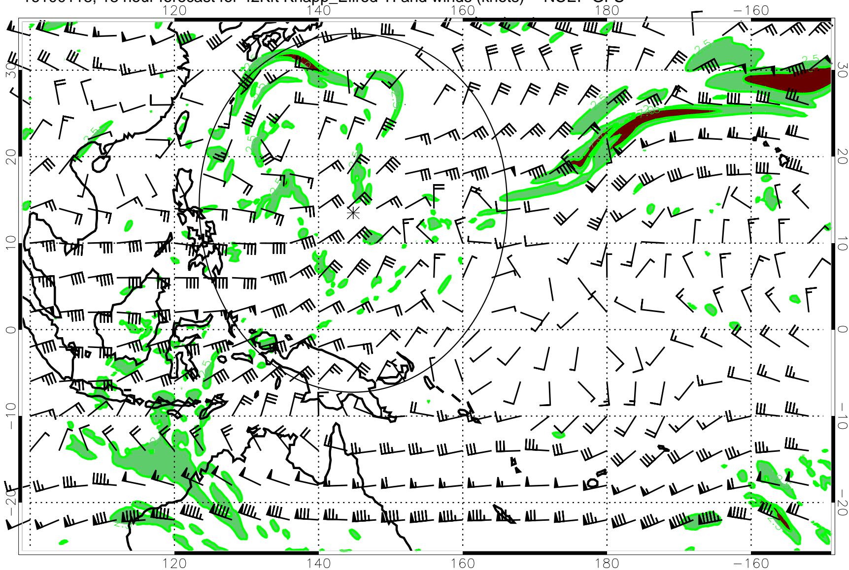
16100118, 18 hour forecast for 42Kft Knapp_Ellrod TI and winds (knots) -- NCEP GFS
