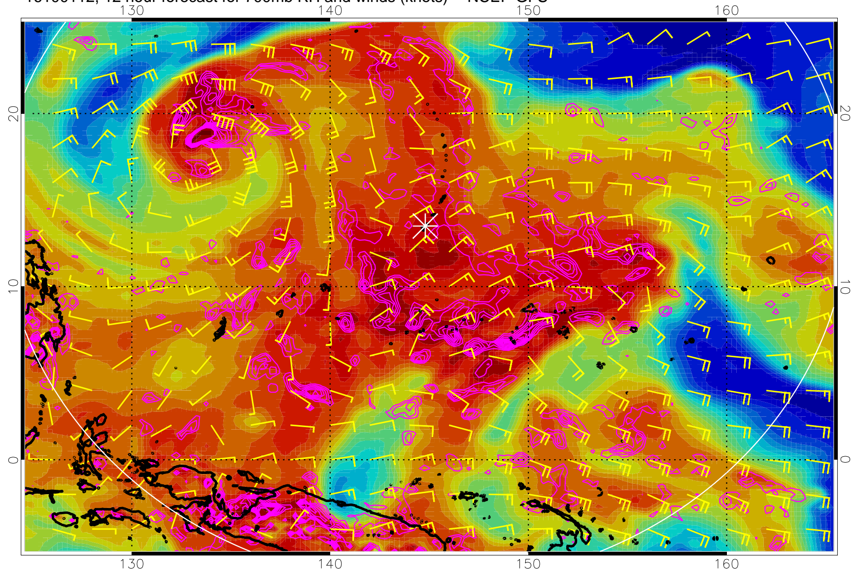
16100112, 12 hour forecast for 700mb RH and winds (knots) -- NCEP GFS
