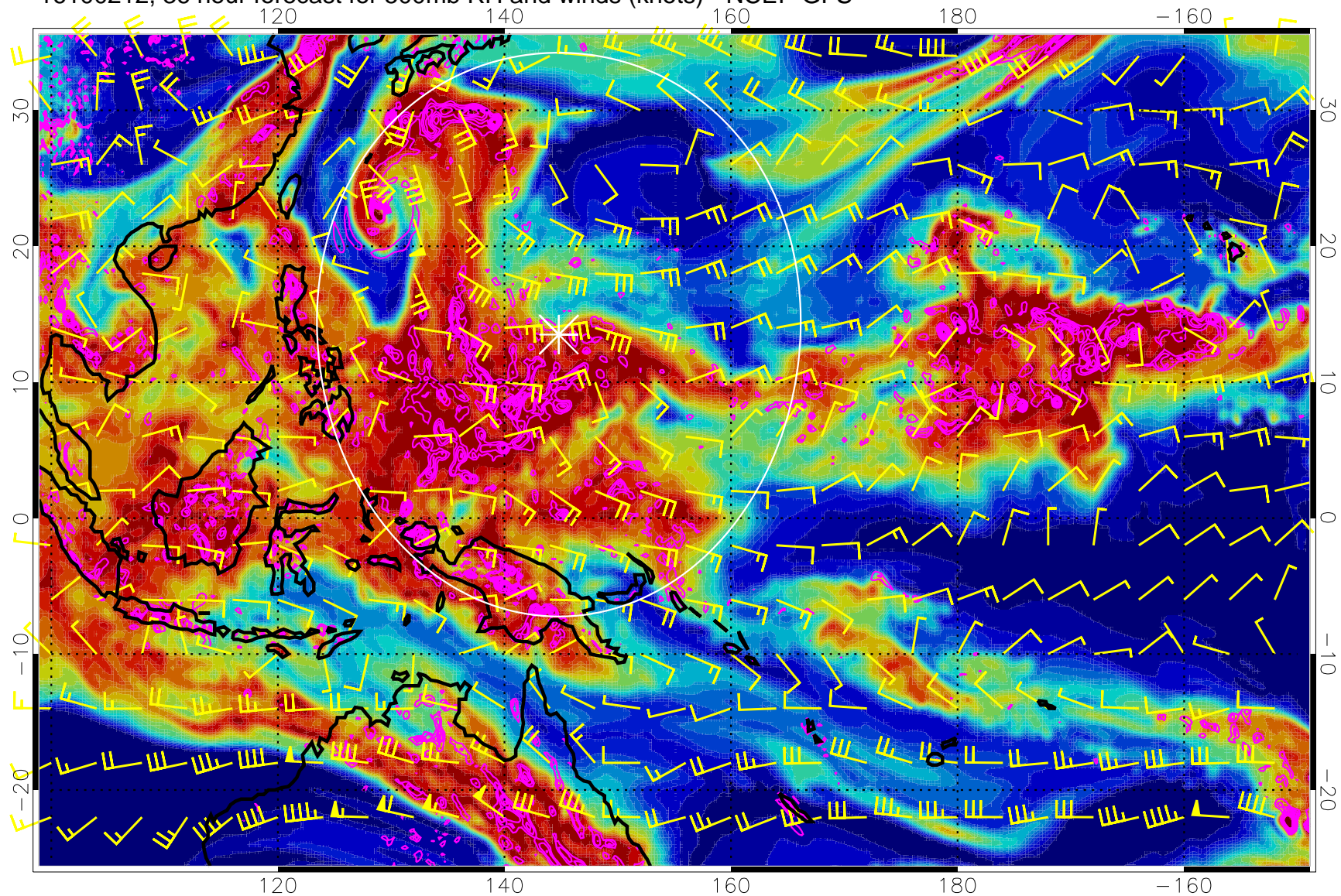
16100212, 36 hour forecast for 500mb RH and winds (knots) - NCEP GFS
