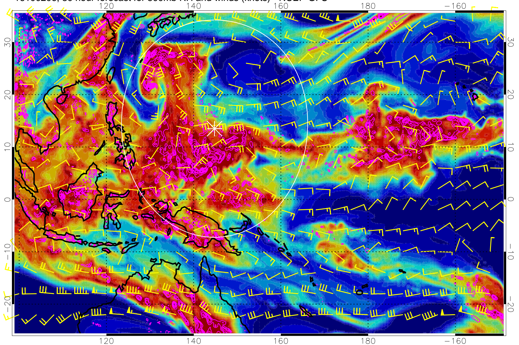
16100206, 30 hour forecast for 500mb RH and winds (knots) - NCEP GFS
