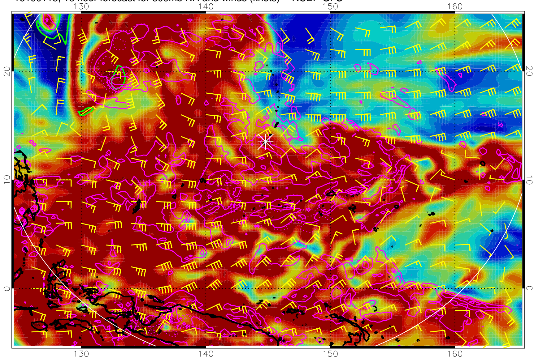
16100118, 18 hour forecast for 300mb RH and winds (knots) -- NCEP GFS
