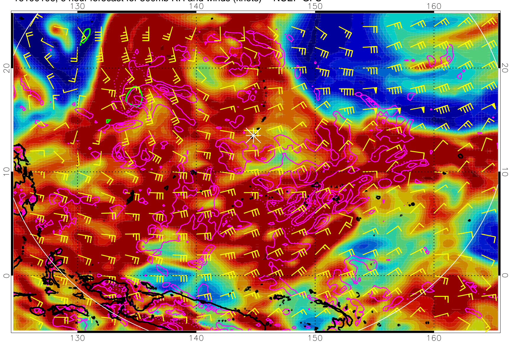
16100106, 6 hour forecast for 300mb RH and winds (knots) -- NCEP GFS
