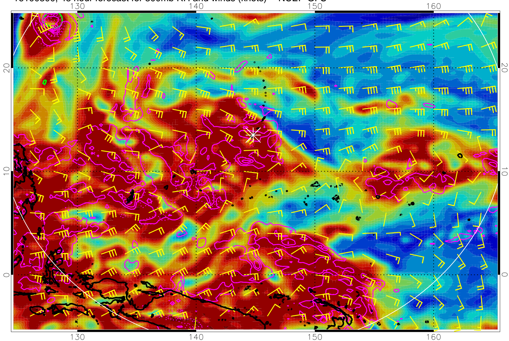
16100300, 48 hour forecast for 300mb RH and winds (knots) -- NCEP GFS
