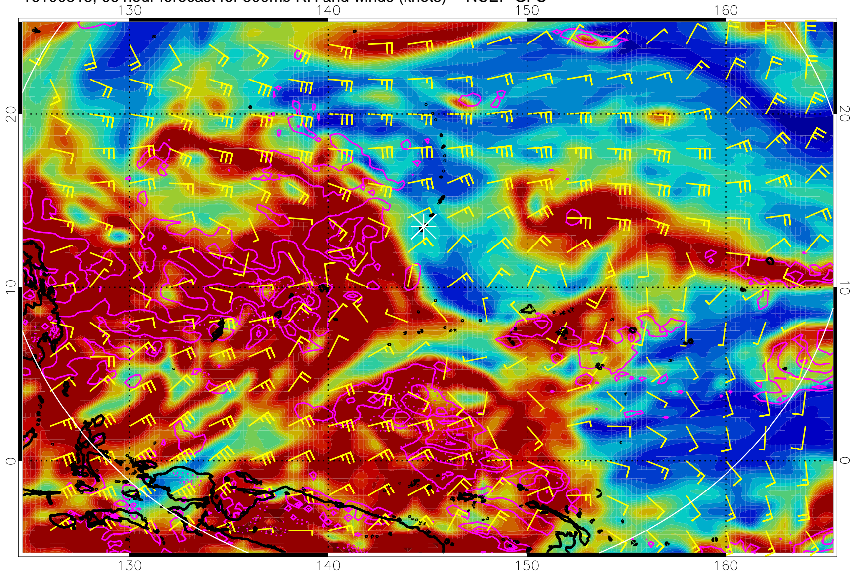
16100318, 66 hour forecast for 300mb RH and winds (knots) -- NCEP GFS
