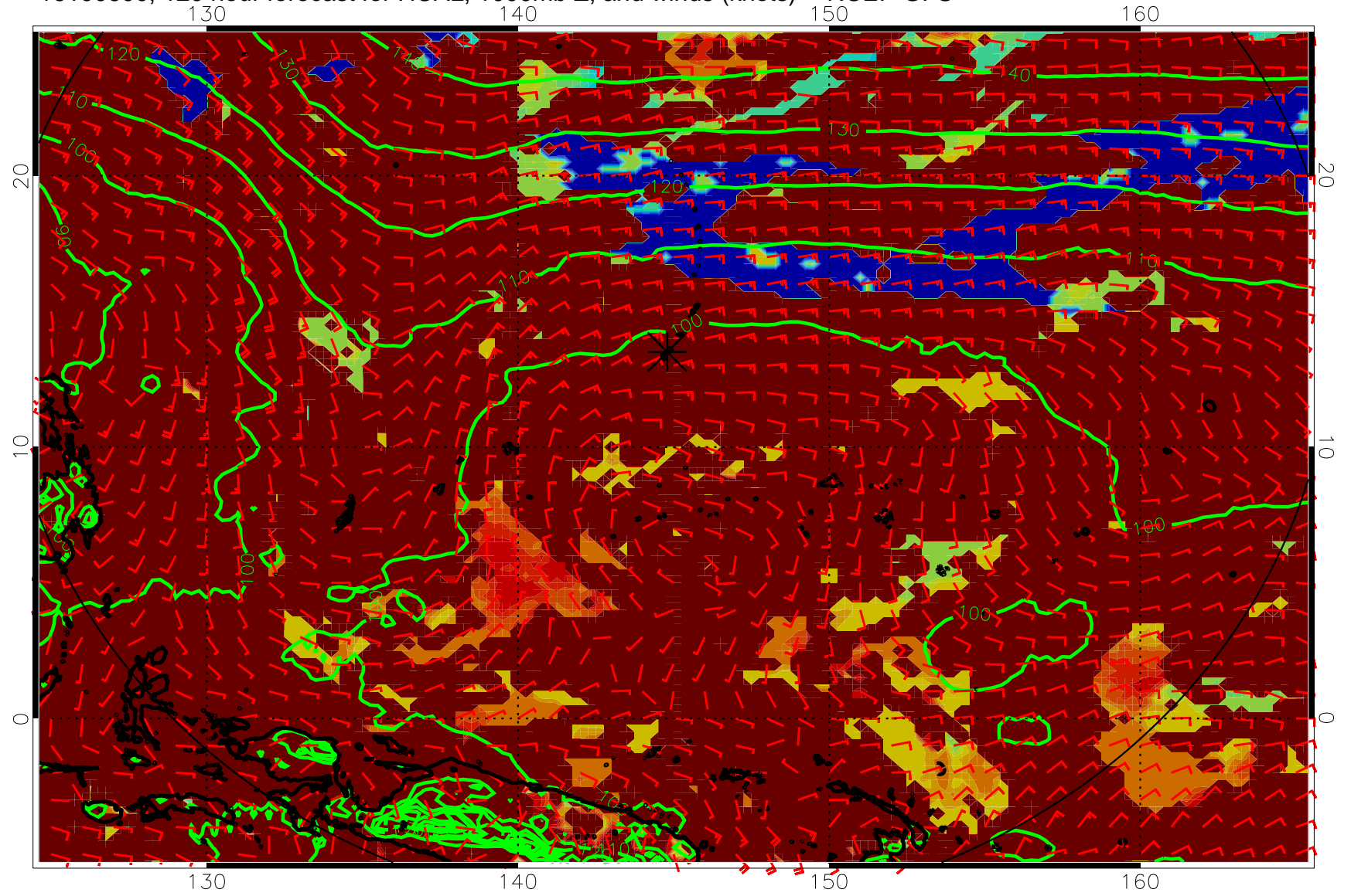
16100600, 120 hour forecast for HCAL, 1000mb Z, and winds (knots) -- NCEP GFS
