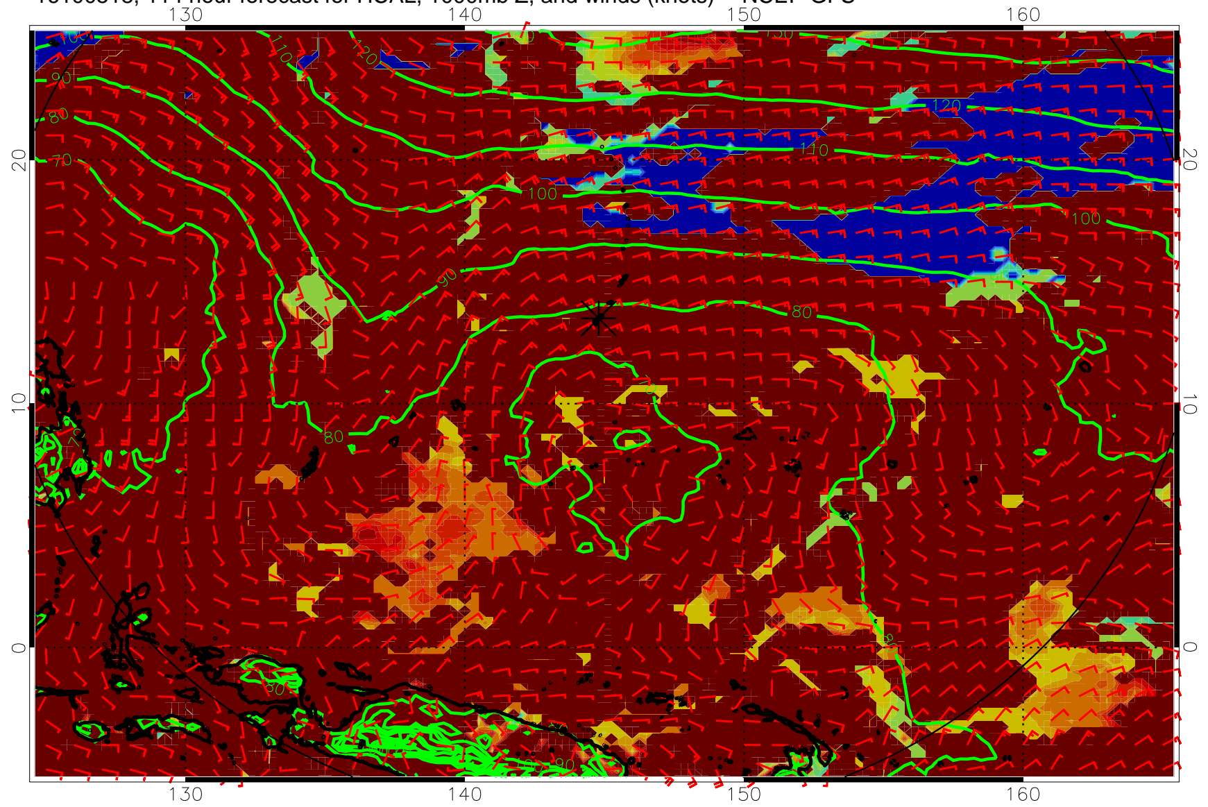
16100518, 114 hour forecast for HCAL, 1000mb Z, and winds (knots) -- NCEP GFS
