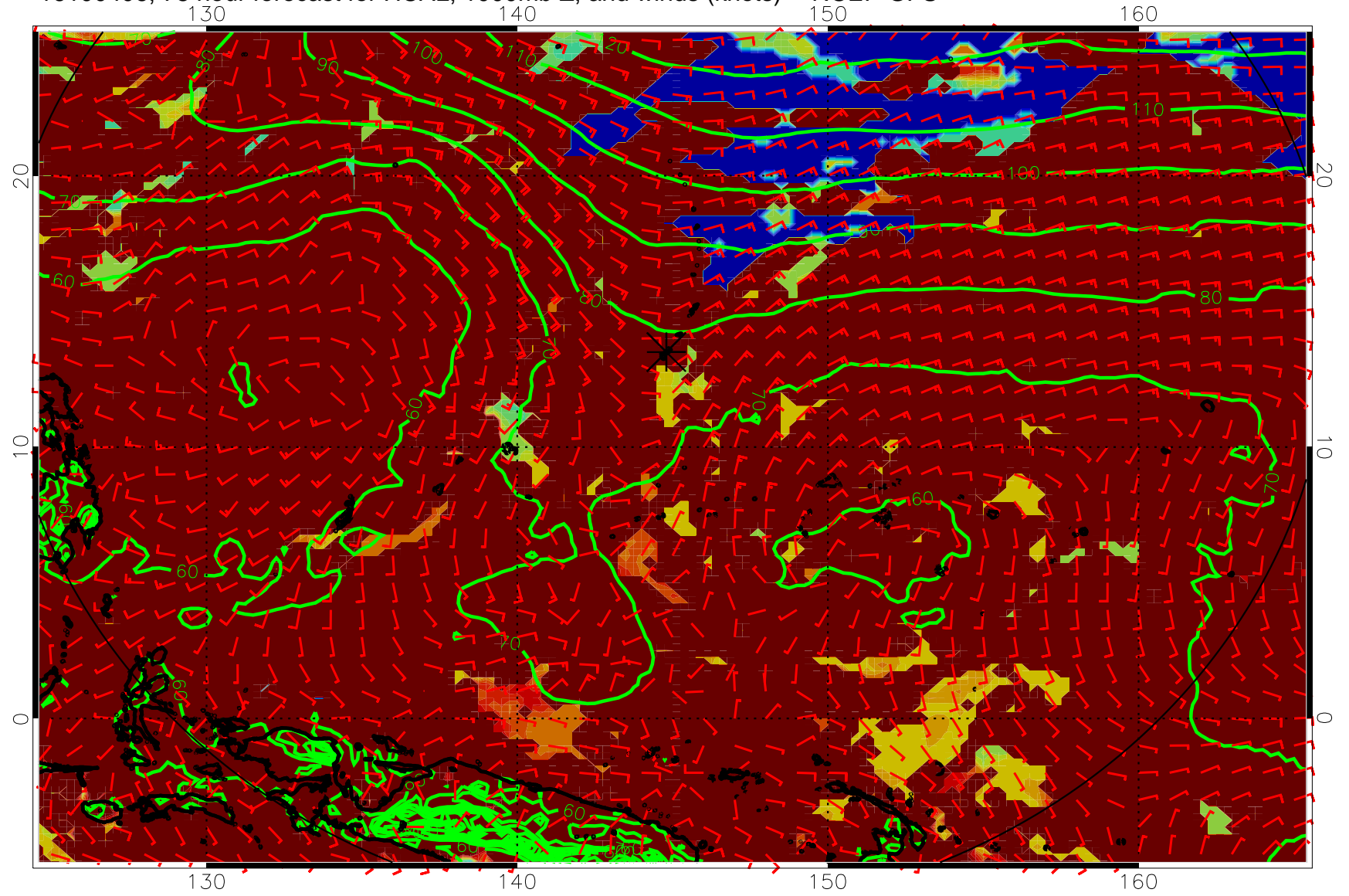
16100406, 78 hour forecast for HCAL, 1000mb Z, and winds (knots) -- NCEP GFS
