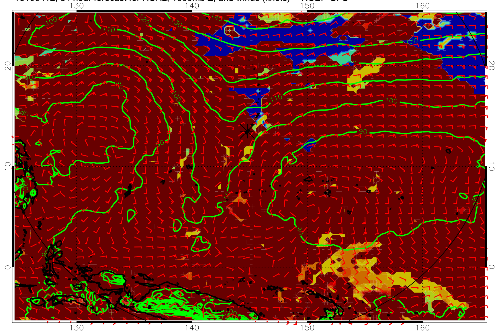
16100412, 84 hour forecast for HCAL, 1000mb Z, and winds (knots) -- NCEP GFS
