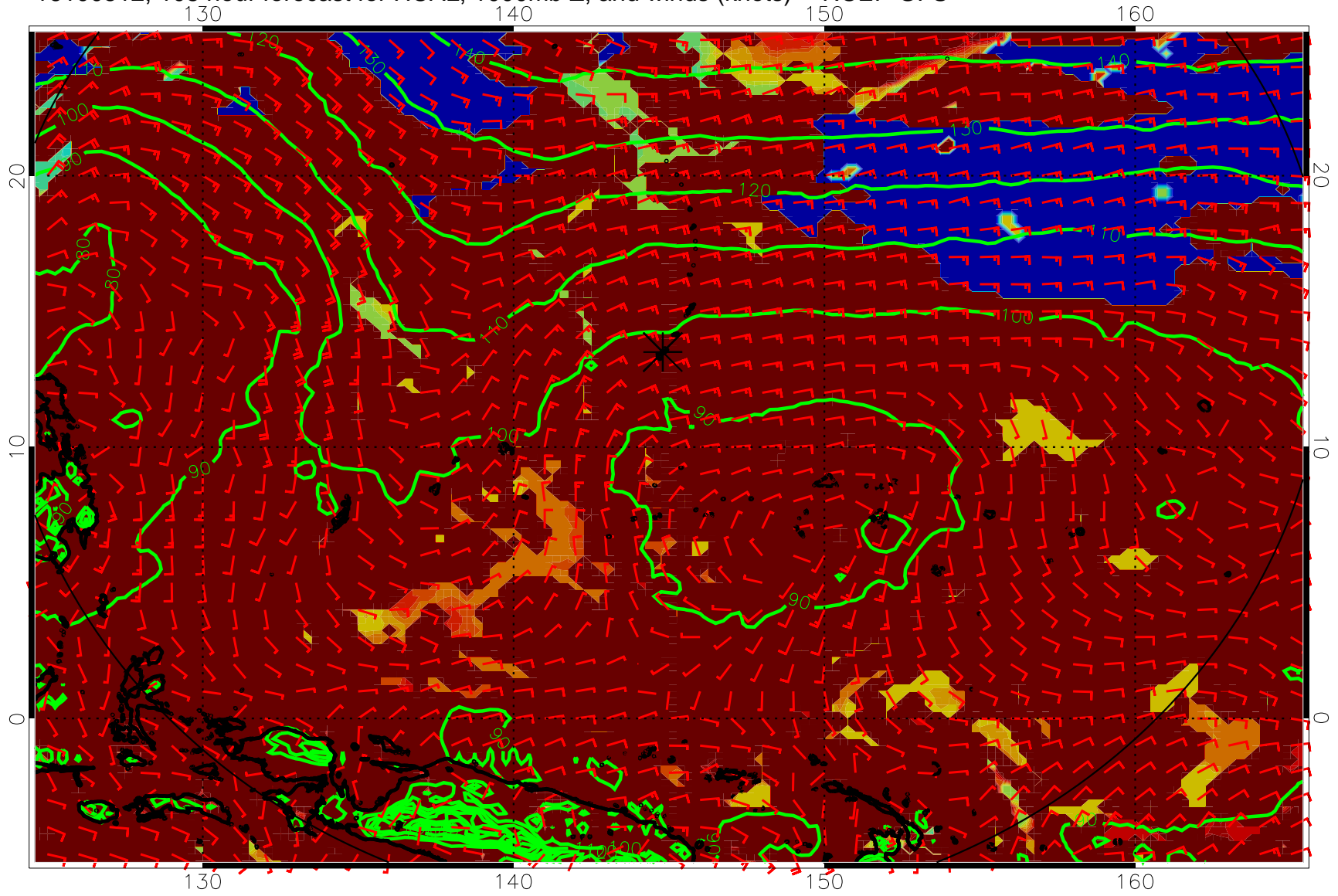
16100512, 108 hour forecast for HCAL, 1000mb Z, and winds (knots) -- NCEP GFS
