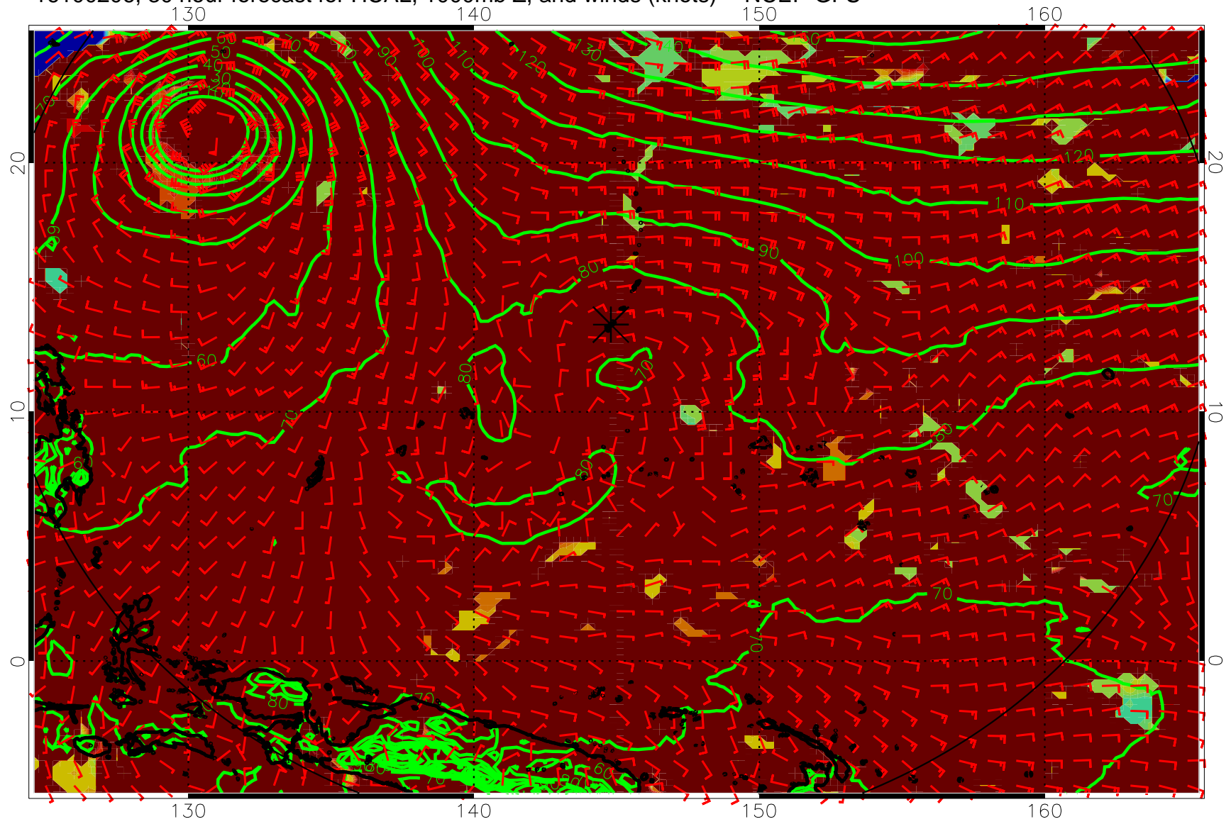
16100206, 30 hour forecast for HCAL, 1000mb Z, and winds (knots) -- NCEP GFS
