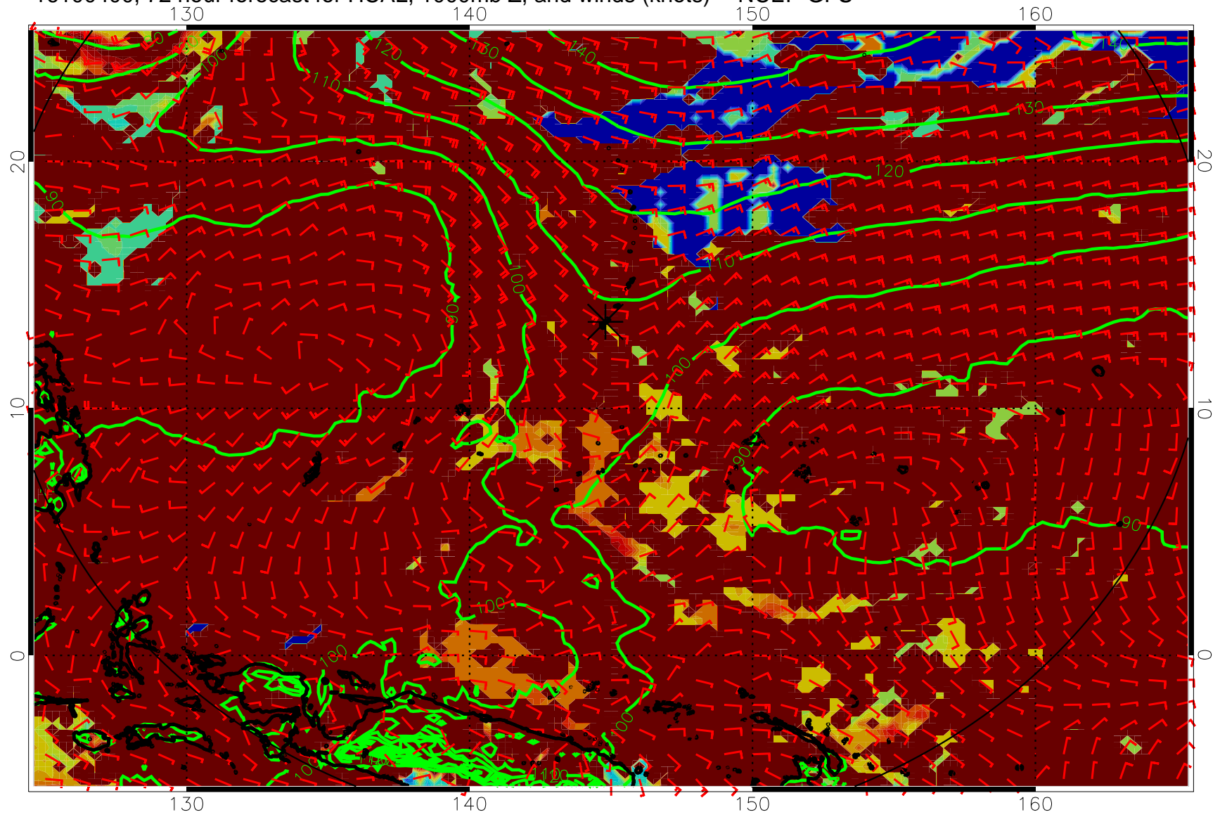
16100400, 72 hour forecast for HCAL, 1000mb Z, and winds (knots) -- NCEP GFS
