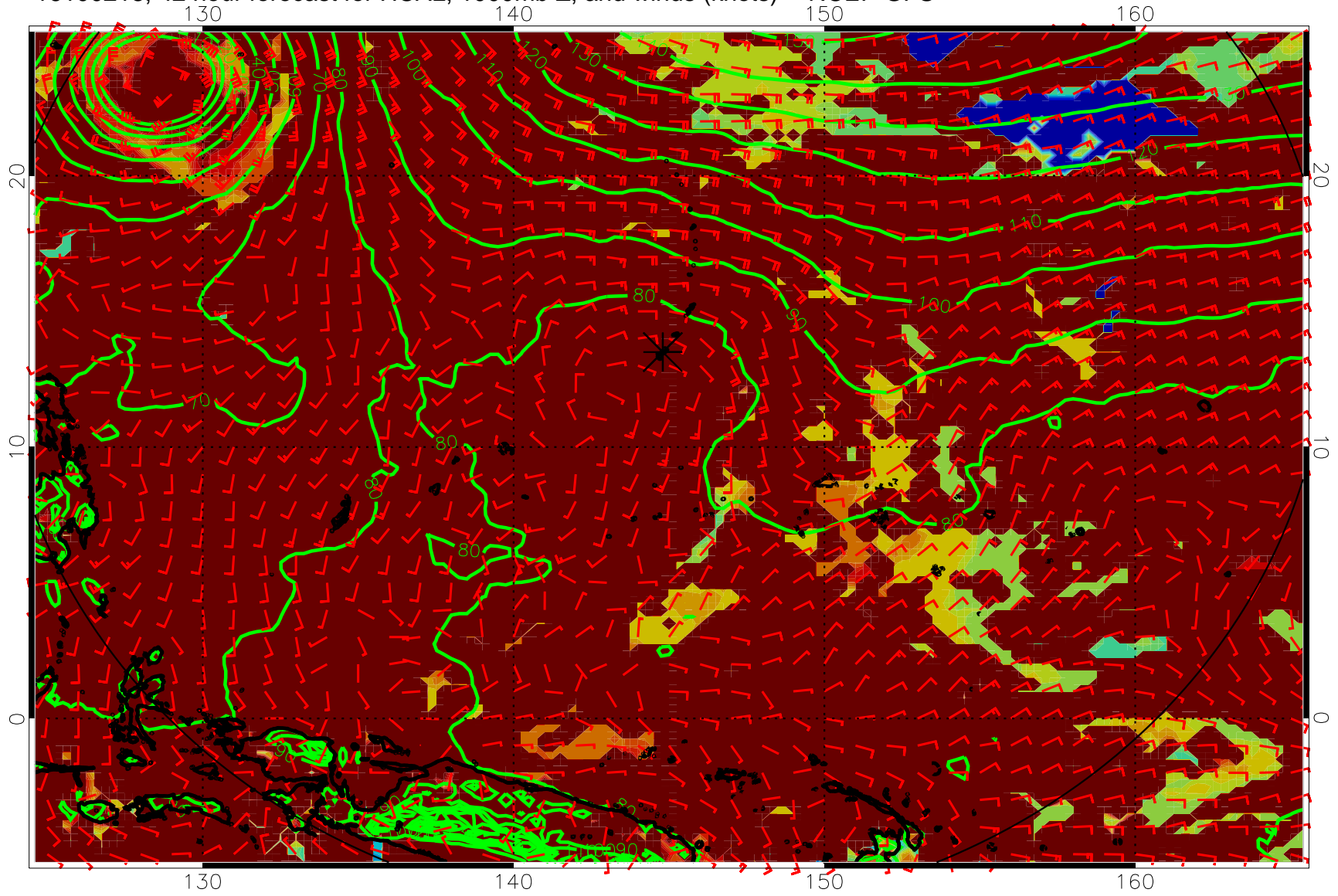
16100218, 42 hour forecast for HCAL, 1000mb Z, and winds (knots) -- NCEP GFS
