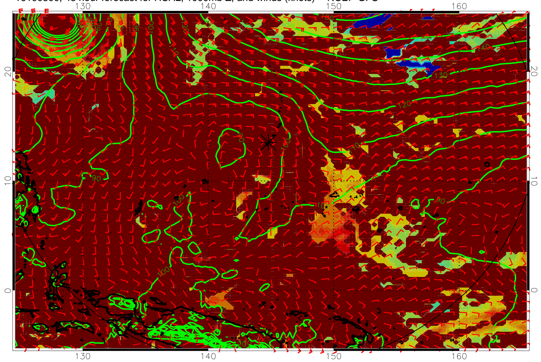
16100300, 48 hour forecast for HCAL, 1000mb Z, and winds (knots) -- NCEP GFS
