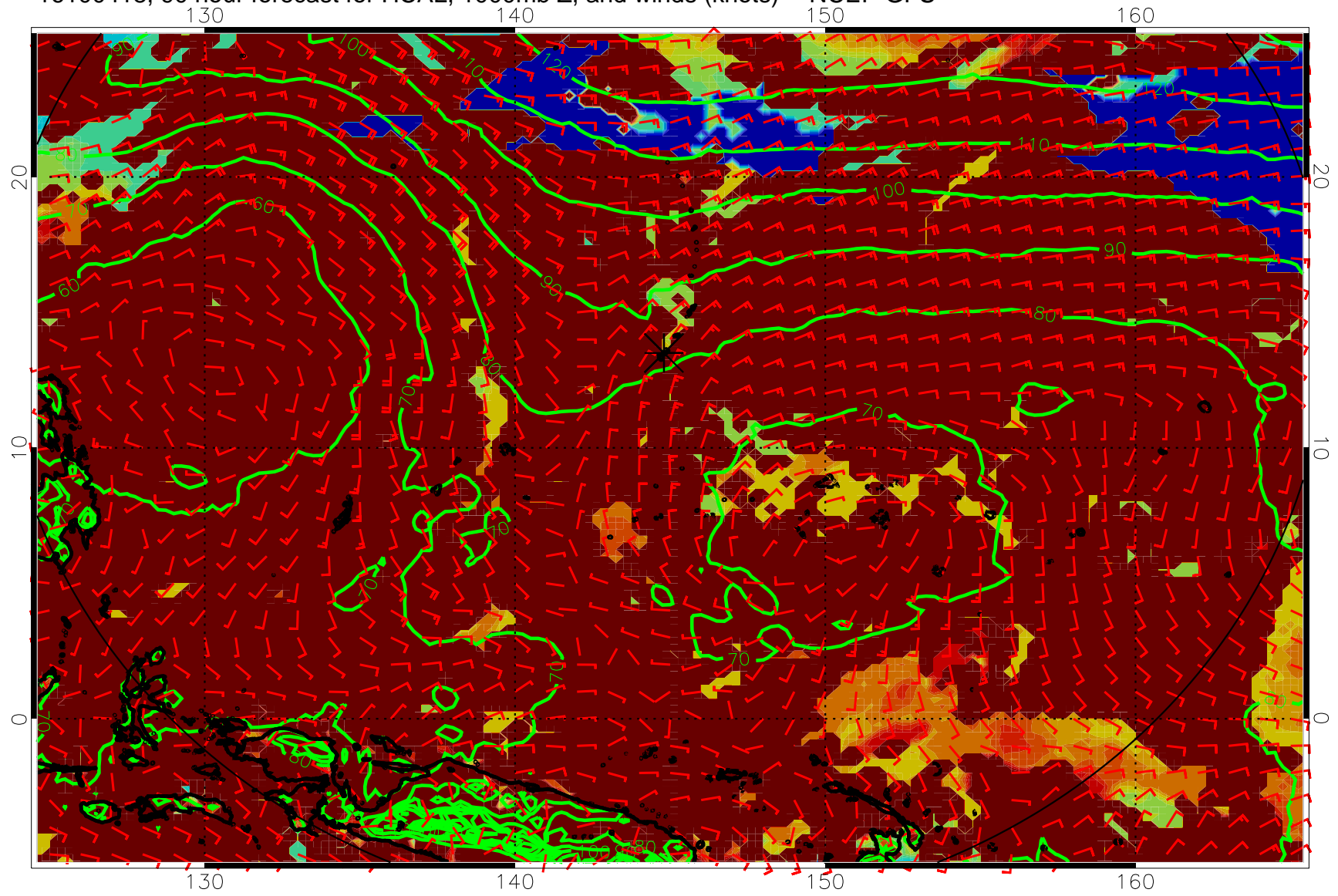
16100418, 90 hour forecast for HCAL, 1000mb Z, and winds (knots) -- NCEP GFS
