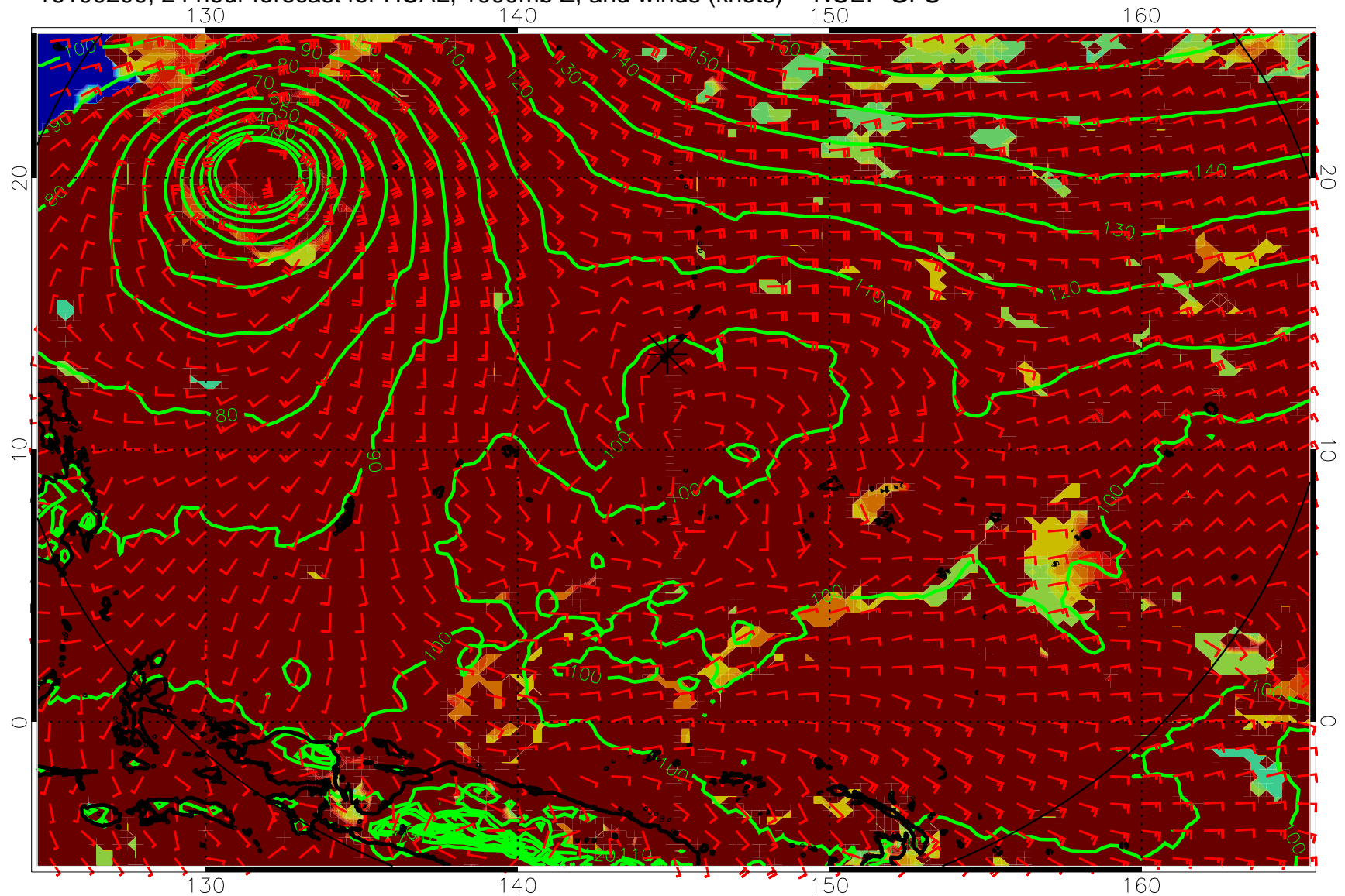
16100200, 24 hour forecast for HCAL, 1000mb Z, and winds (knots) -- NCEP GFS
