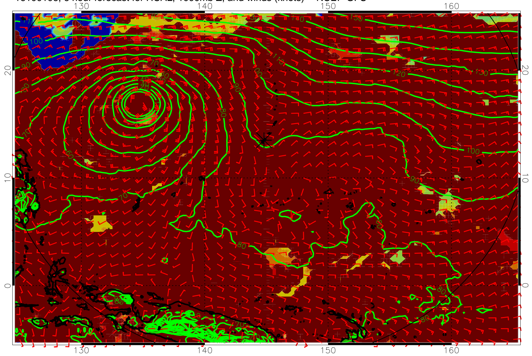
16100106, 6 hour forecast for HCAL, 1000mb Z, and winds (knots) -- NCEP GFS
