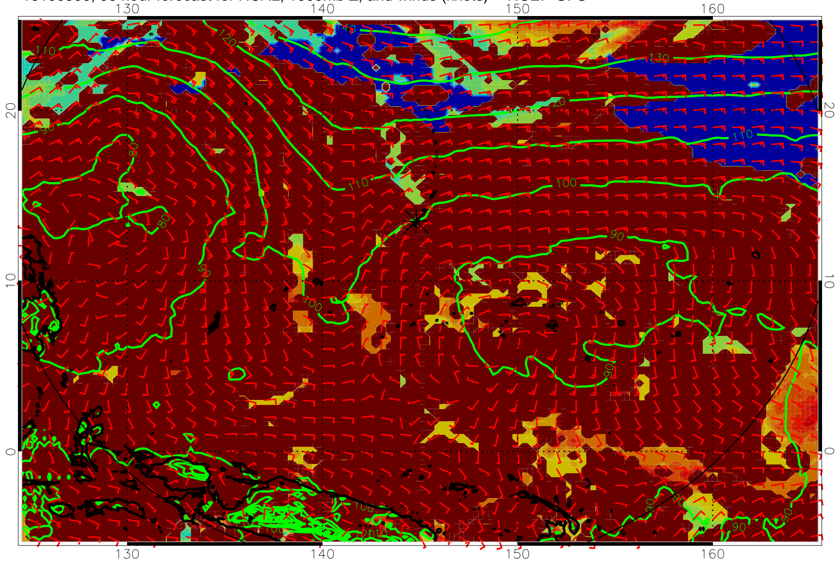
16100500, 96 hour forecast for HCAL, 1000mb Z, and winds (knots) -- NCEP GFS
