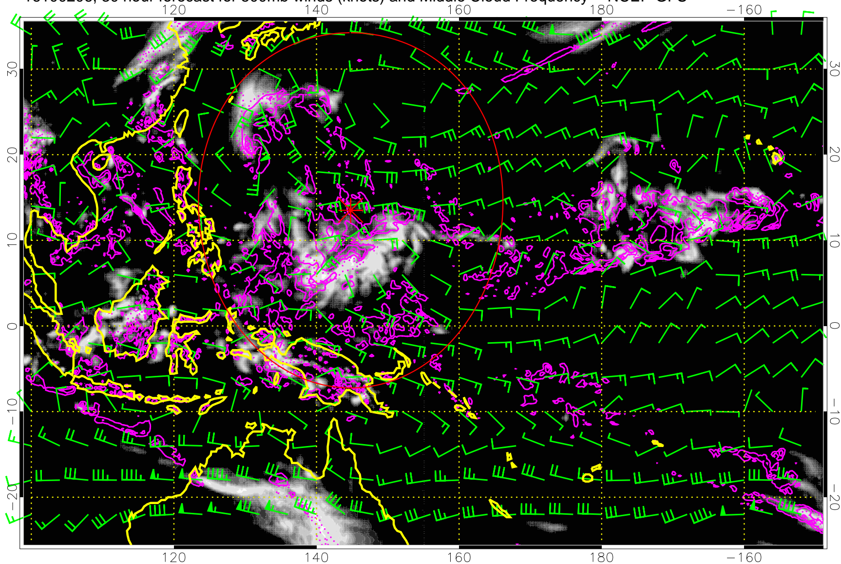
16100206, 30 hour forecast for 500mb winds (knots) and Middle Cloud Frequency -- NCEP GFS
