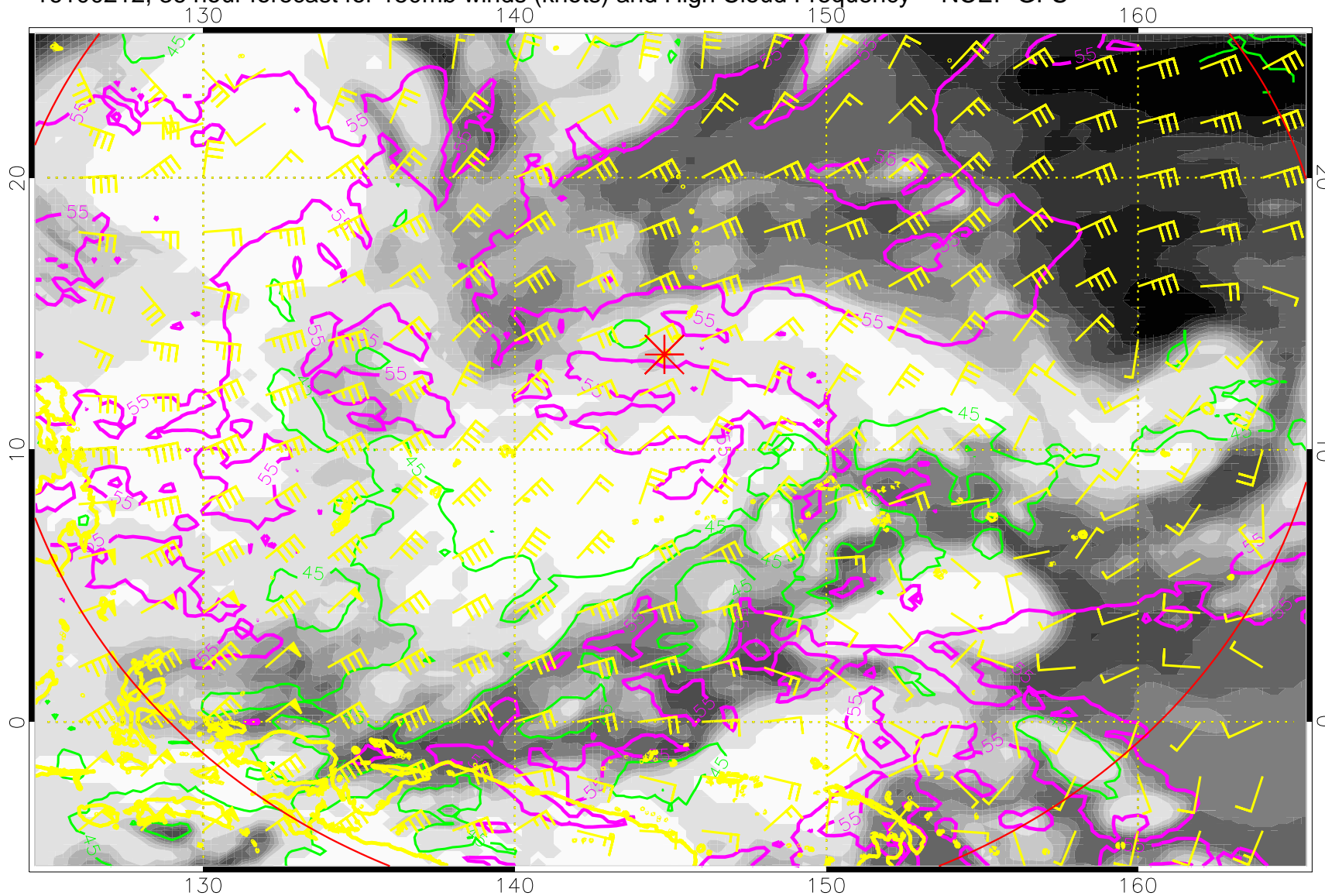
16100212, 36 hour forecast for 150mb winds (knots) and High Cloud Frequency -- NCEP GFS
