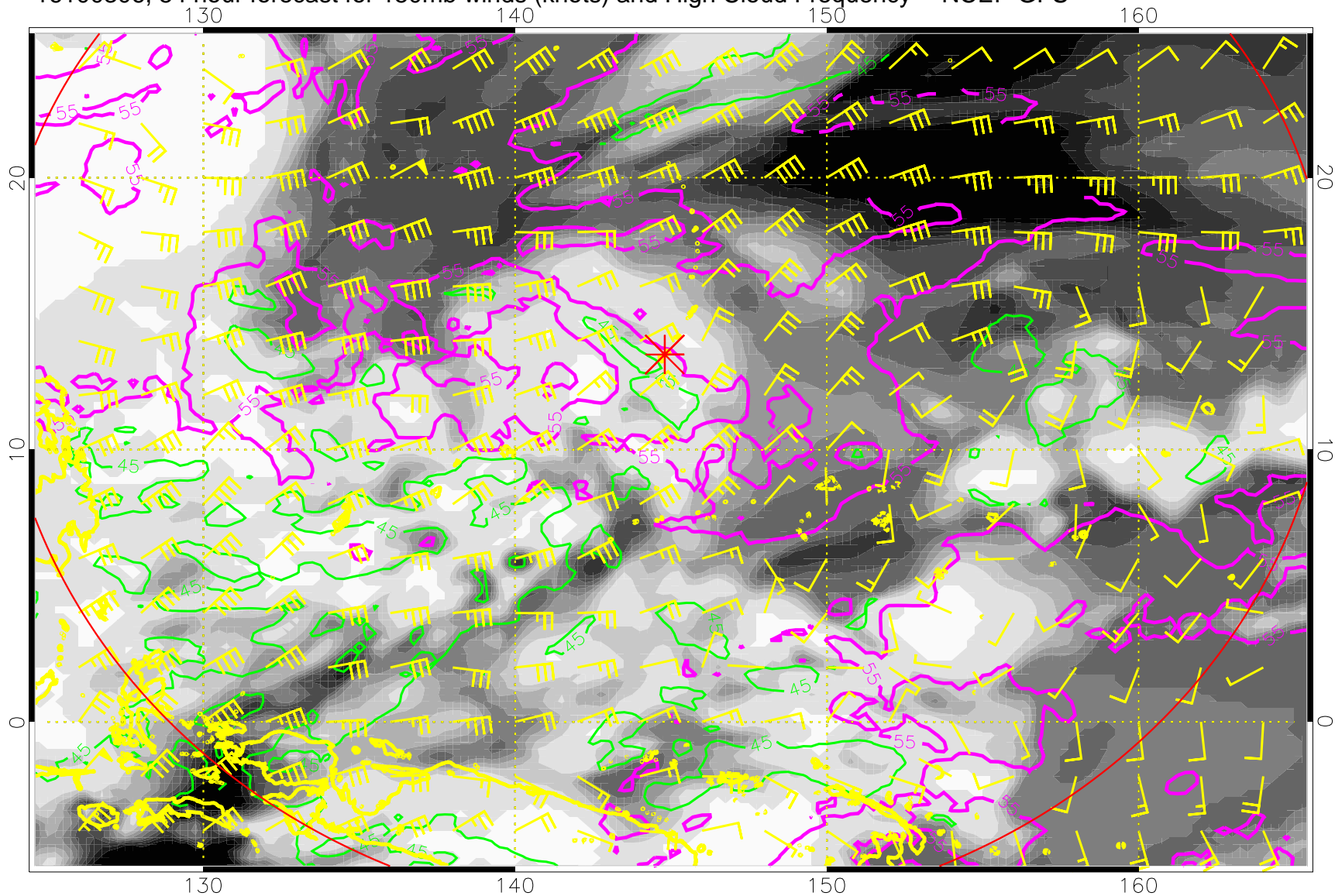
16100306, 54 hour forecast for 150mb winds (knots) and High Cloud Frequency -- NCEP GFS
