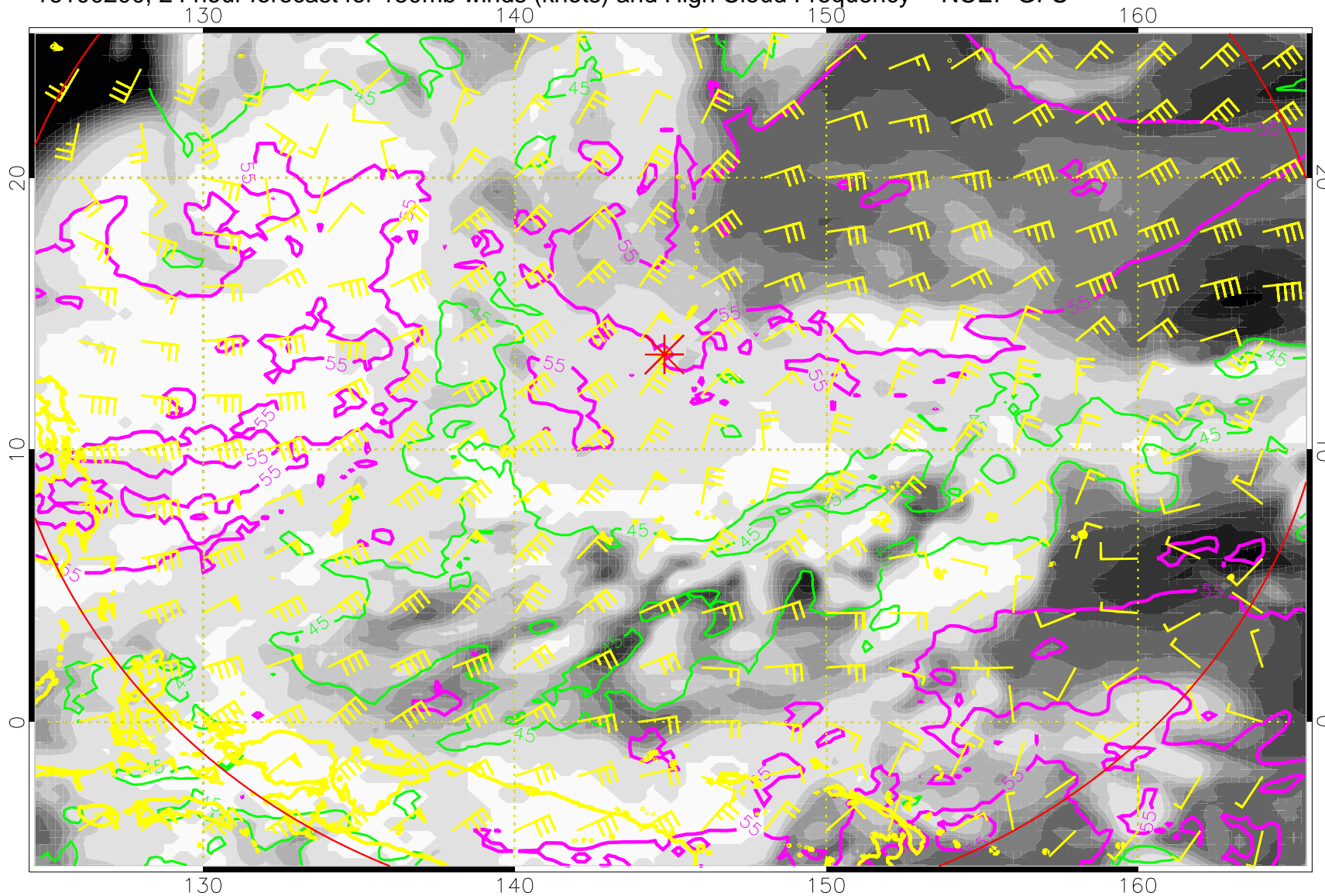
16100200, 24 hour forecast for 150mb winds (knots) and High Cloud Frequency -- NCEP GFS
