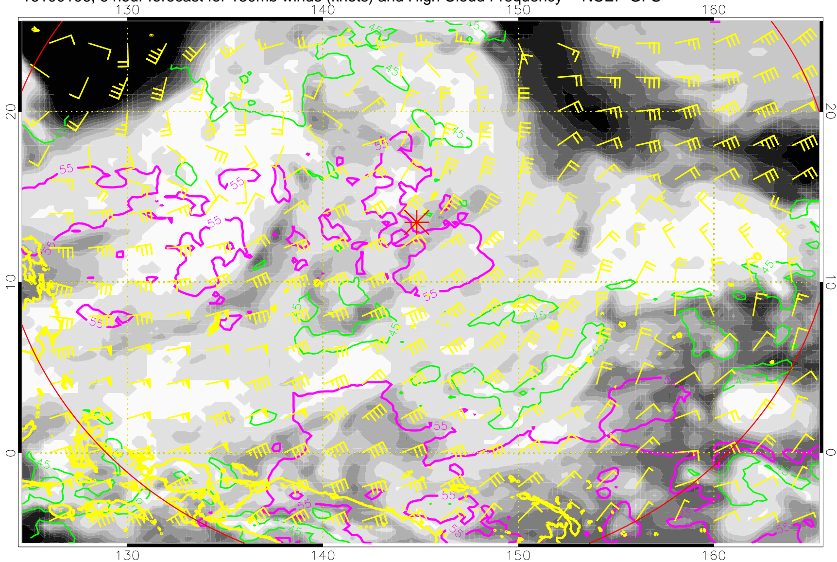
16100106, 6 hour forecast for 150mb winds (knots) and High Cloud Frequency -- NCEP GFS
