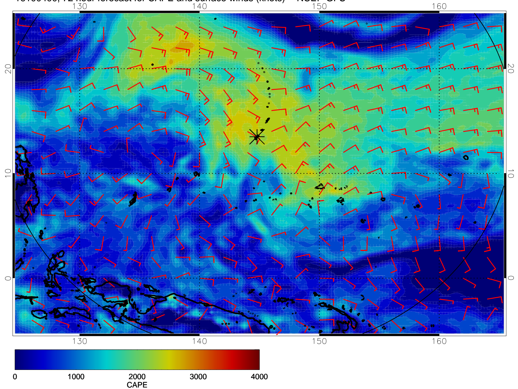
16100400, 72 hour forecast for CAPE and surface winds (knots) -- NCEP GFS
