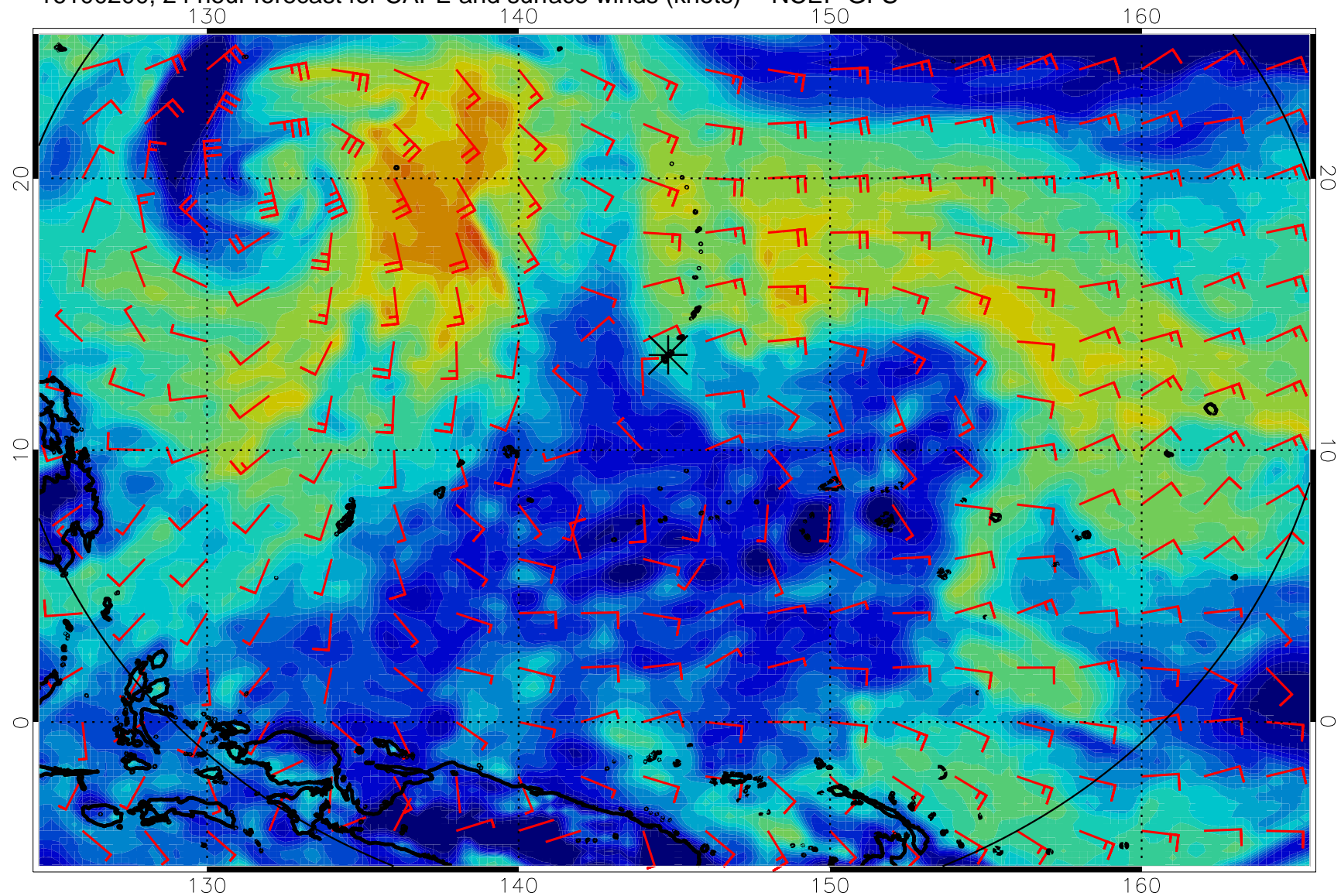
16100200, 24 hour forecast for CAPE and surface winds (knots) -- NCEP GFS
