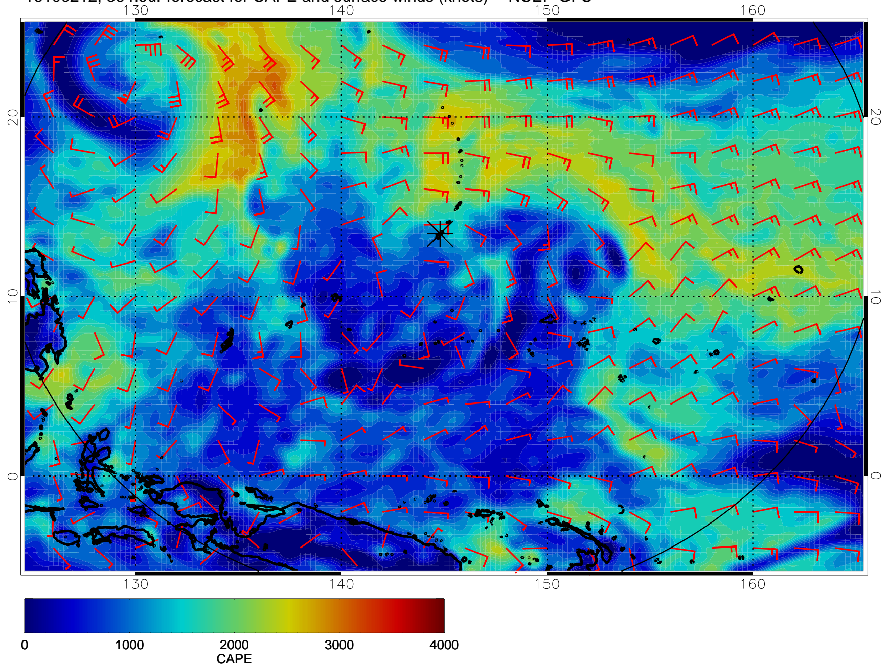
16100212, 36 hour forecast for CAPE and surface winds (knots) -- NCEP GFS
