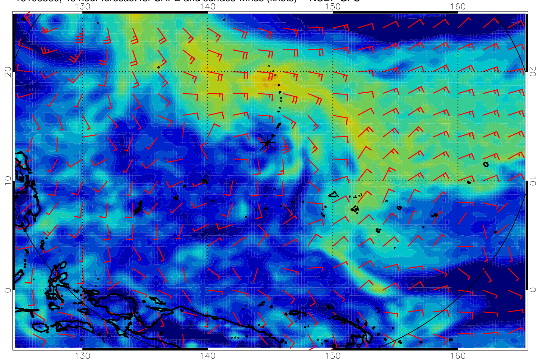
16100300, 48 hour forecast for CAPE and surface winds (knots) -- NCEP GFS
