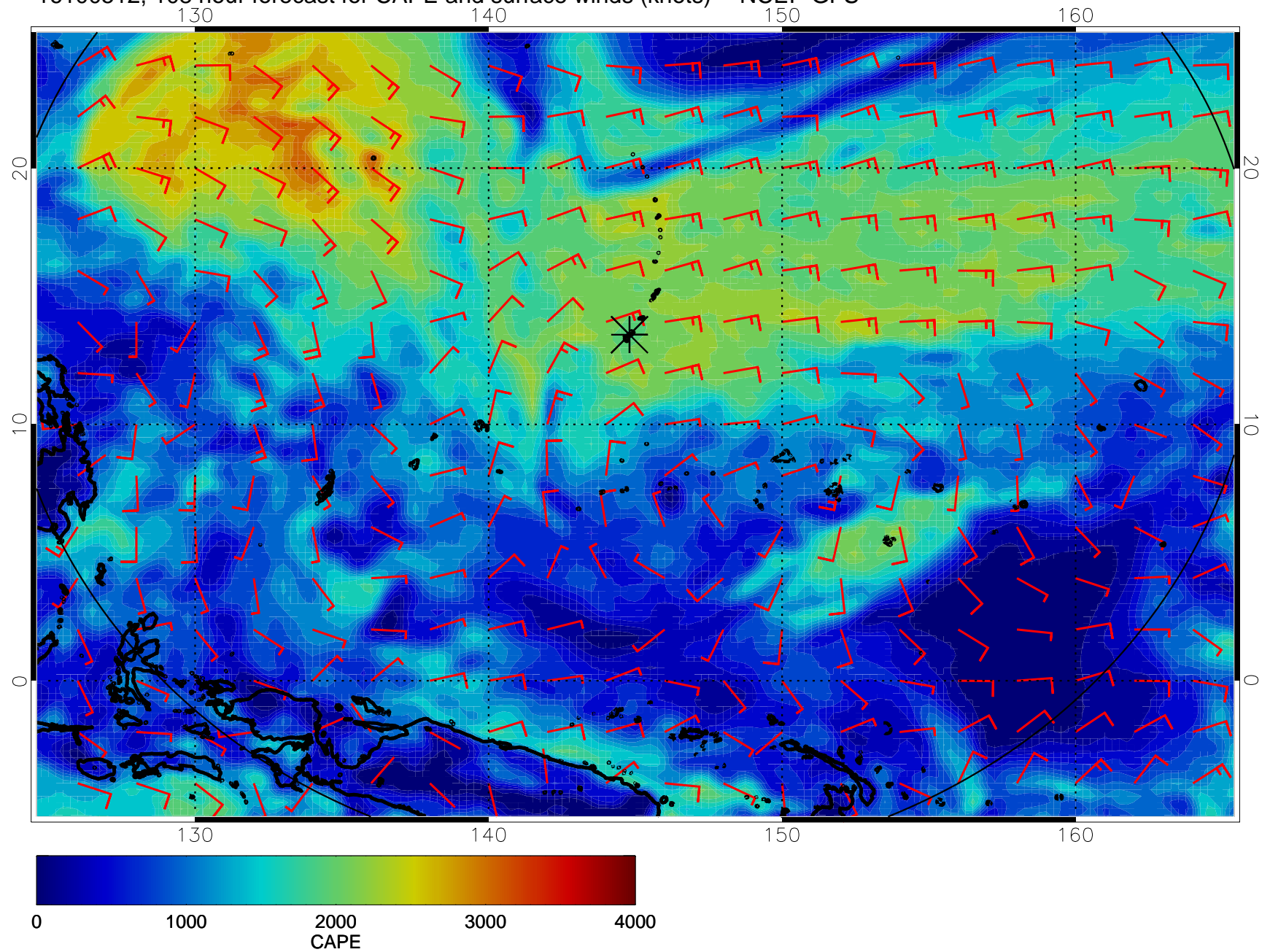
16100512, 108 hour forecast for CAPE and surface winds (knots) -- NCEP GFS
