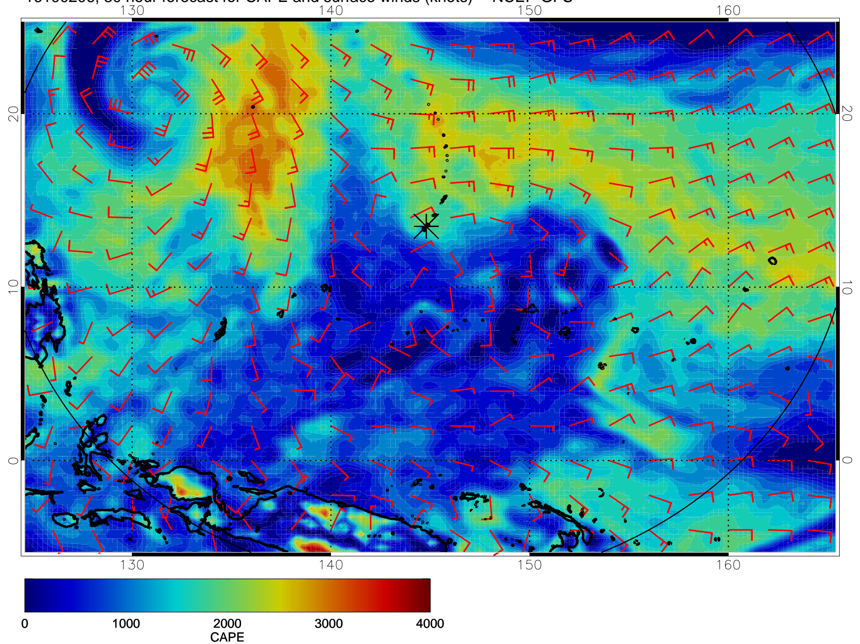
16100206, 30 hour forecast for CAPE and surface winds (knots) -- NCEP GFS
