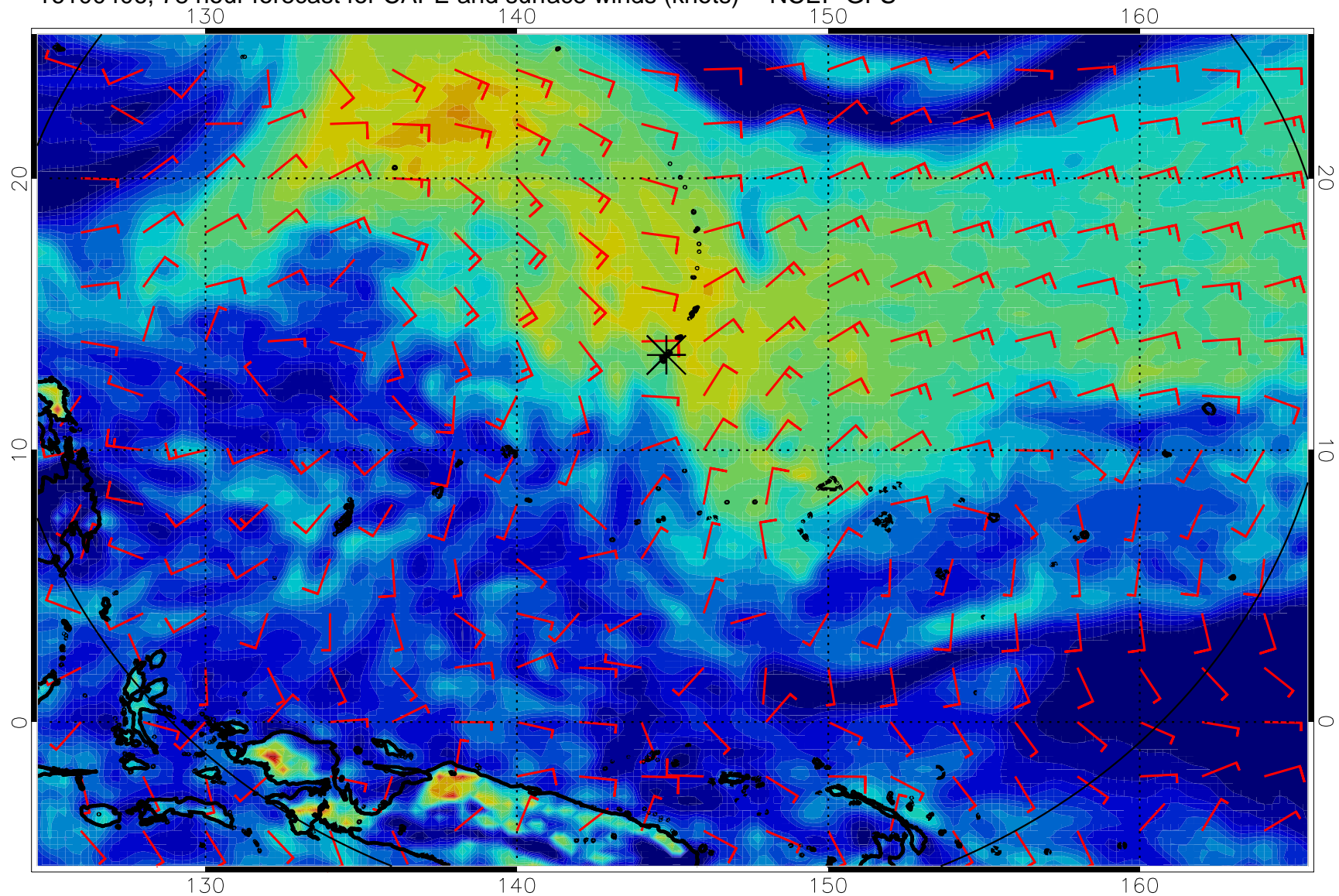
16100406, 78 hour forecast for CAPE and surface winds (knots) -- NCEP GFS
