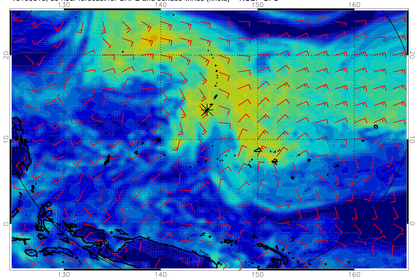
16100318, 66 hour forecast for CAPE and surface winds (knots) -- NCEP GFS
