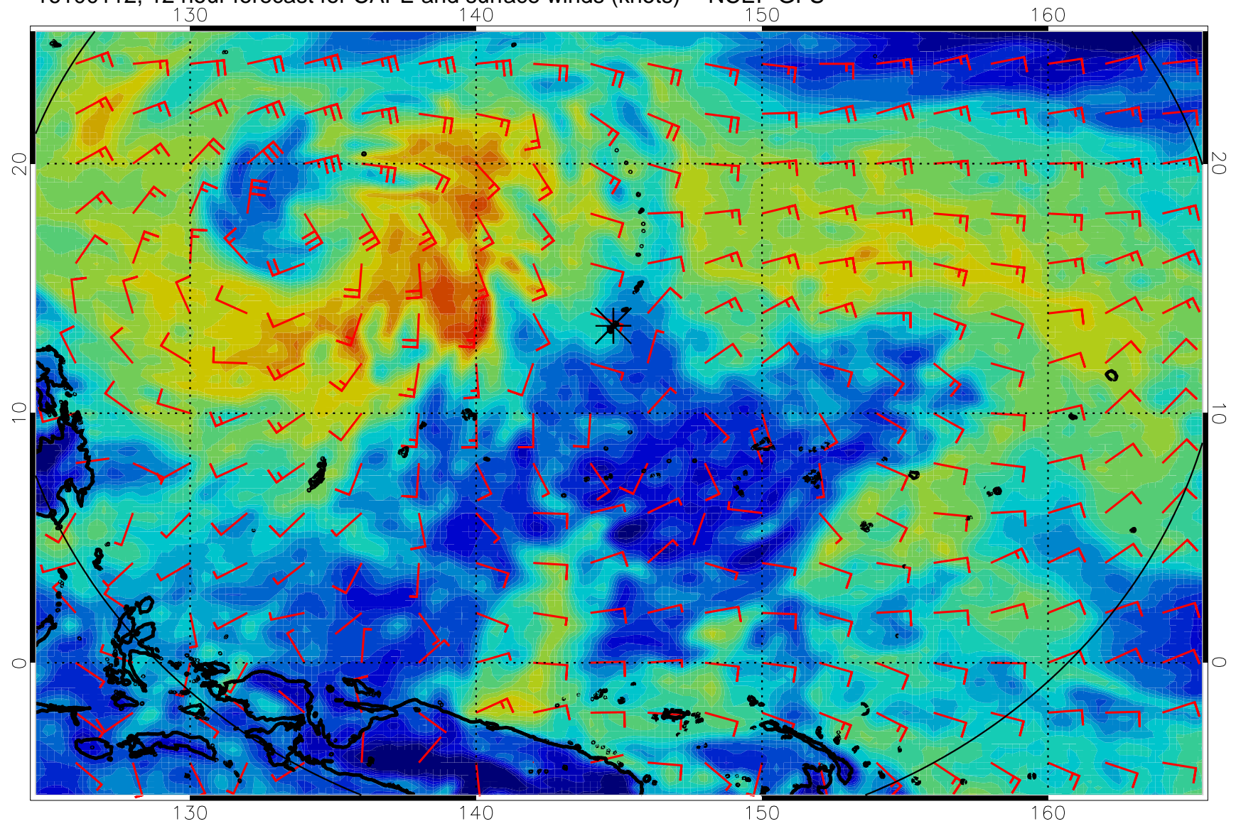
16100112, 12 hour forecast for CAPE and surface winds (knots) -- NCEP GFS
