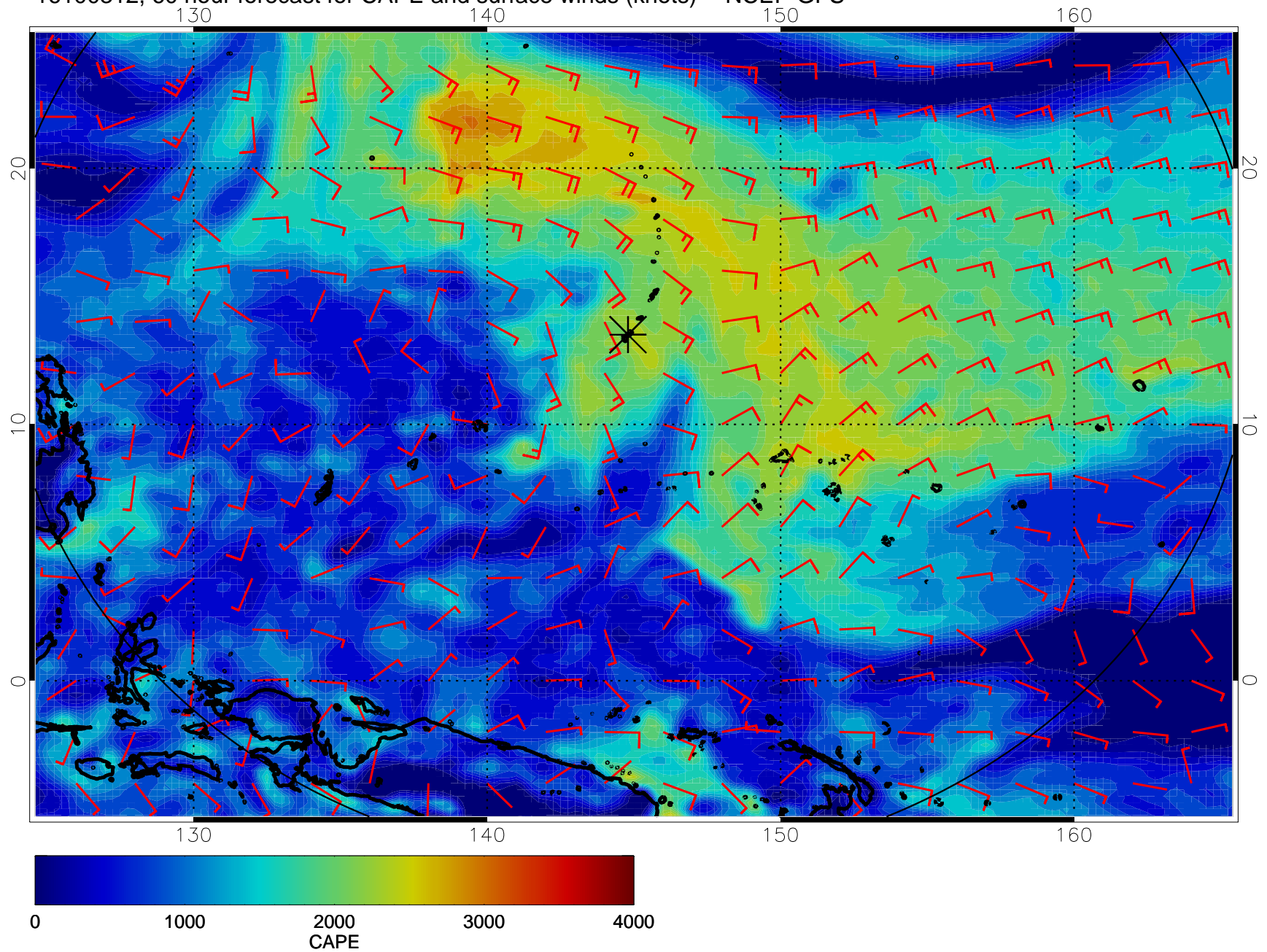
16100312, 60 hour forecast for CAPE and surface winds (knots) -- NCEP GFS
