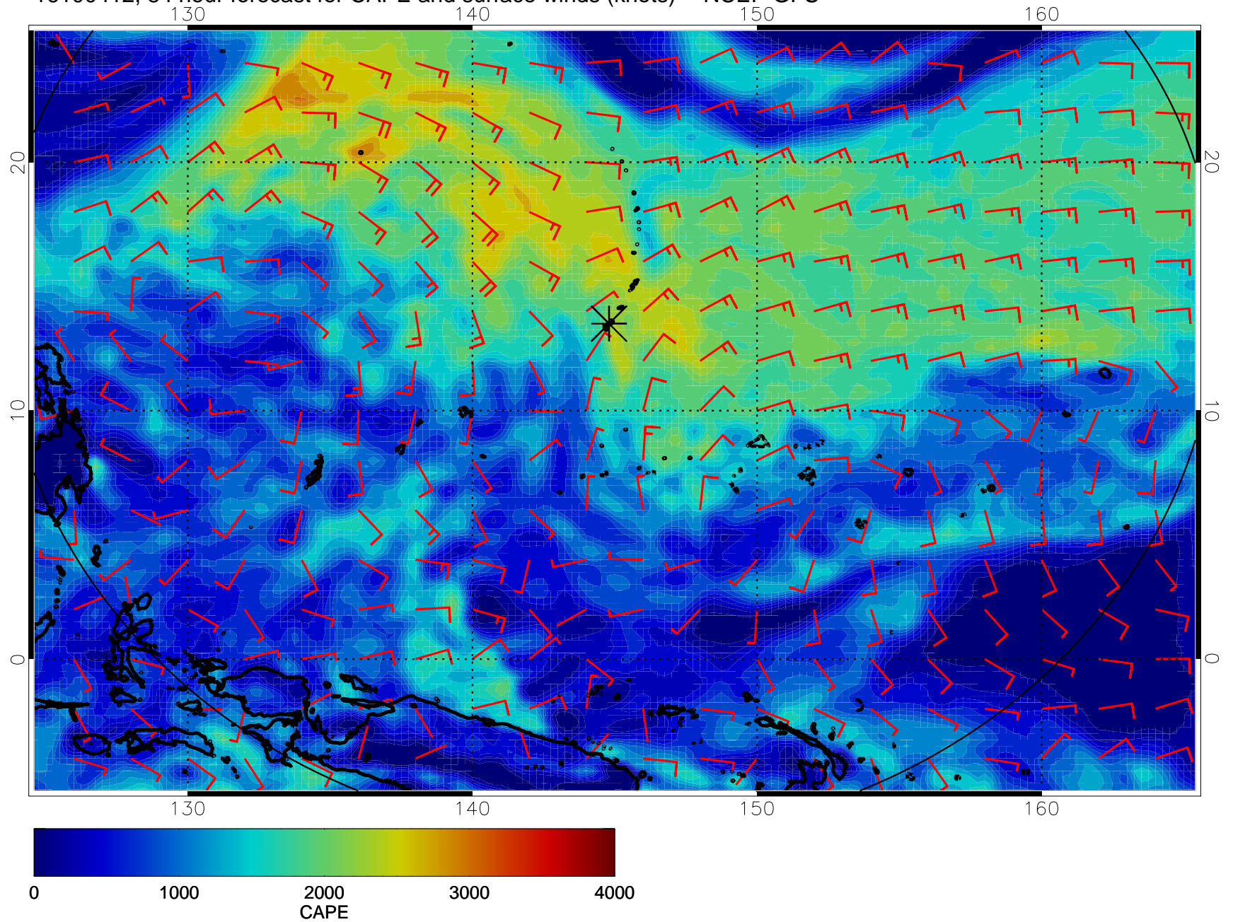
16100412, 84 hour forecast for CAPE and surface winds (knots) -- NCEP GFS
