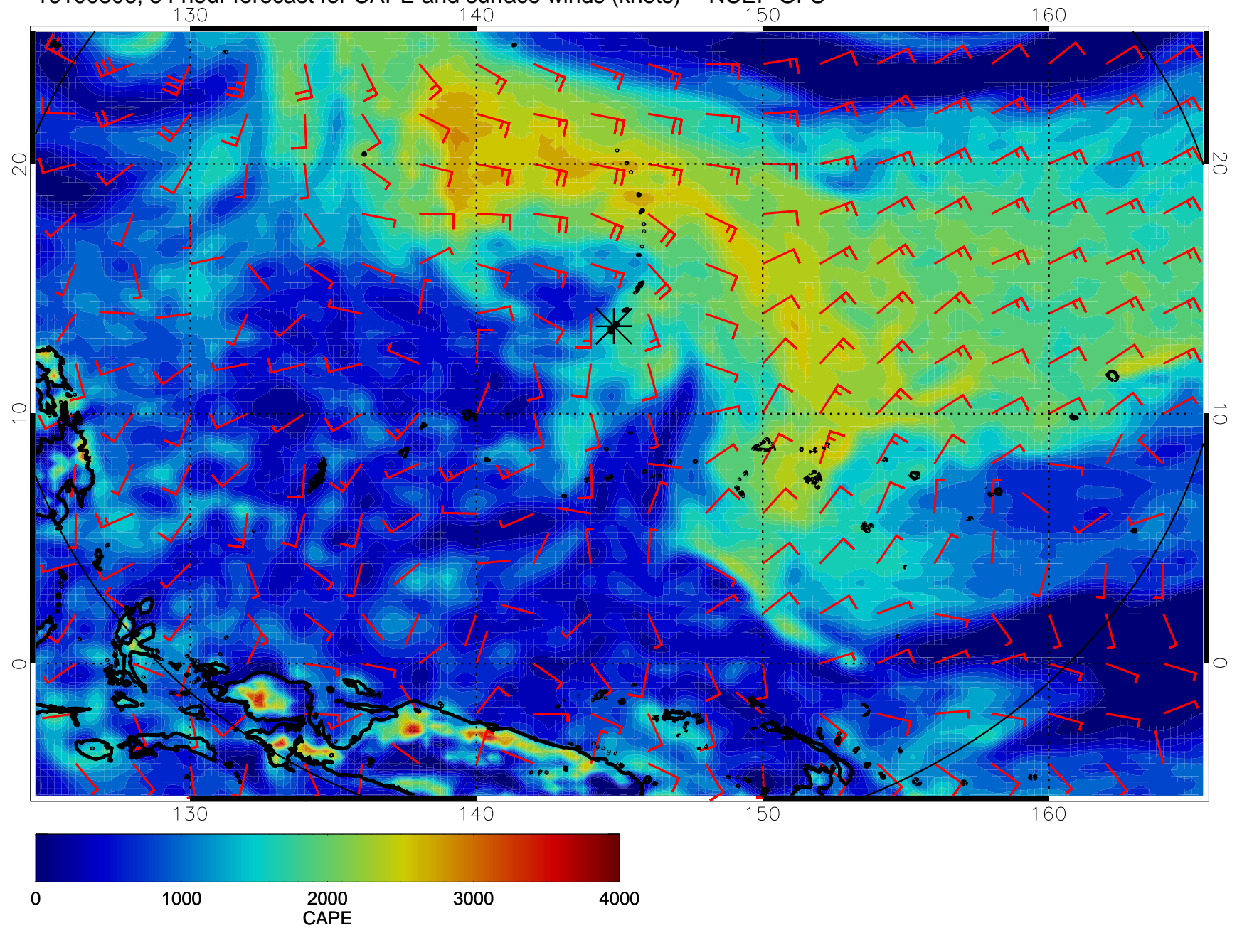
16100306, 54 hour forecast for CAPE and surface winds (knots) -- NCEP GFS
