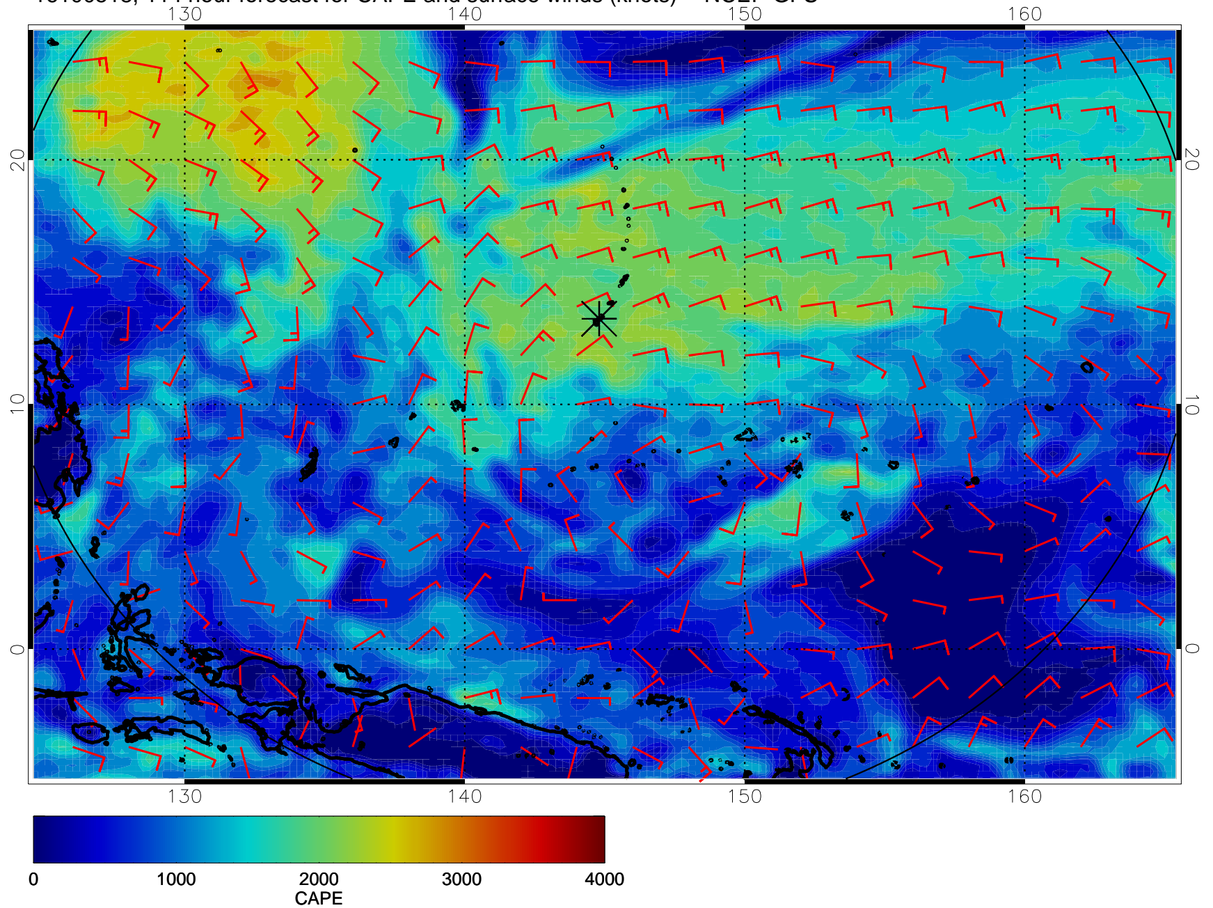
16100518, 114 hour forecast for CAPE and surface winds (knots) -- NCEP GFS
