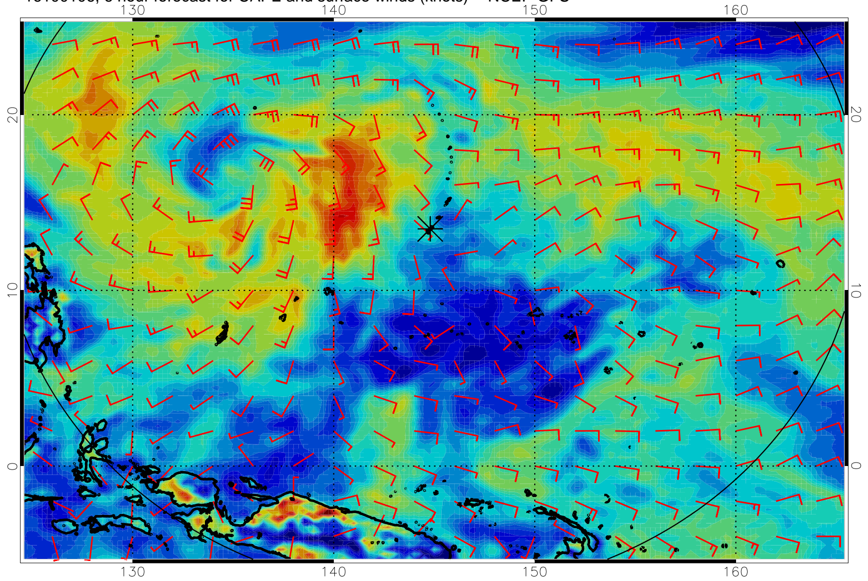
16100106, 6 hour forecast for CAPE and surface winds (knots) -- NCEP GFS
