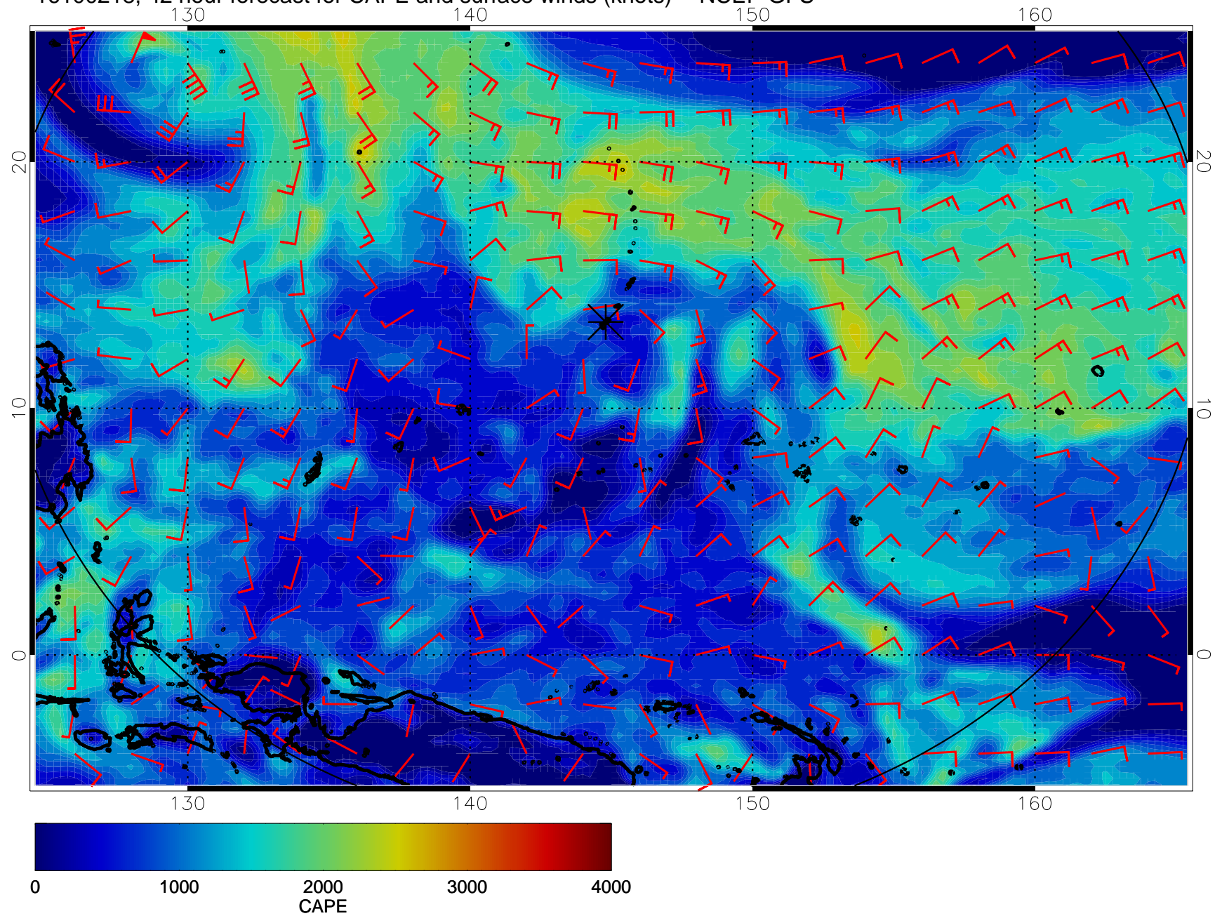
16100218, 42 hour forecast for CAPE and surface winds (knots) -- NCEP GFS
