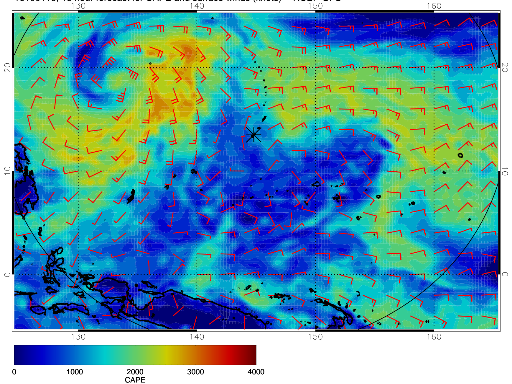
16100118, 18 hour forecast for CAPE and surface winds (knots) -- NCEP GFS
