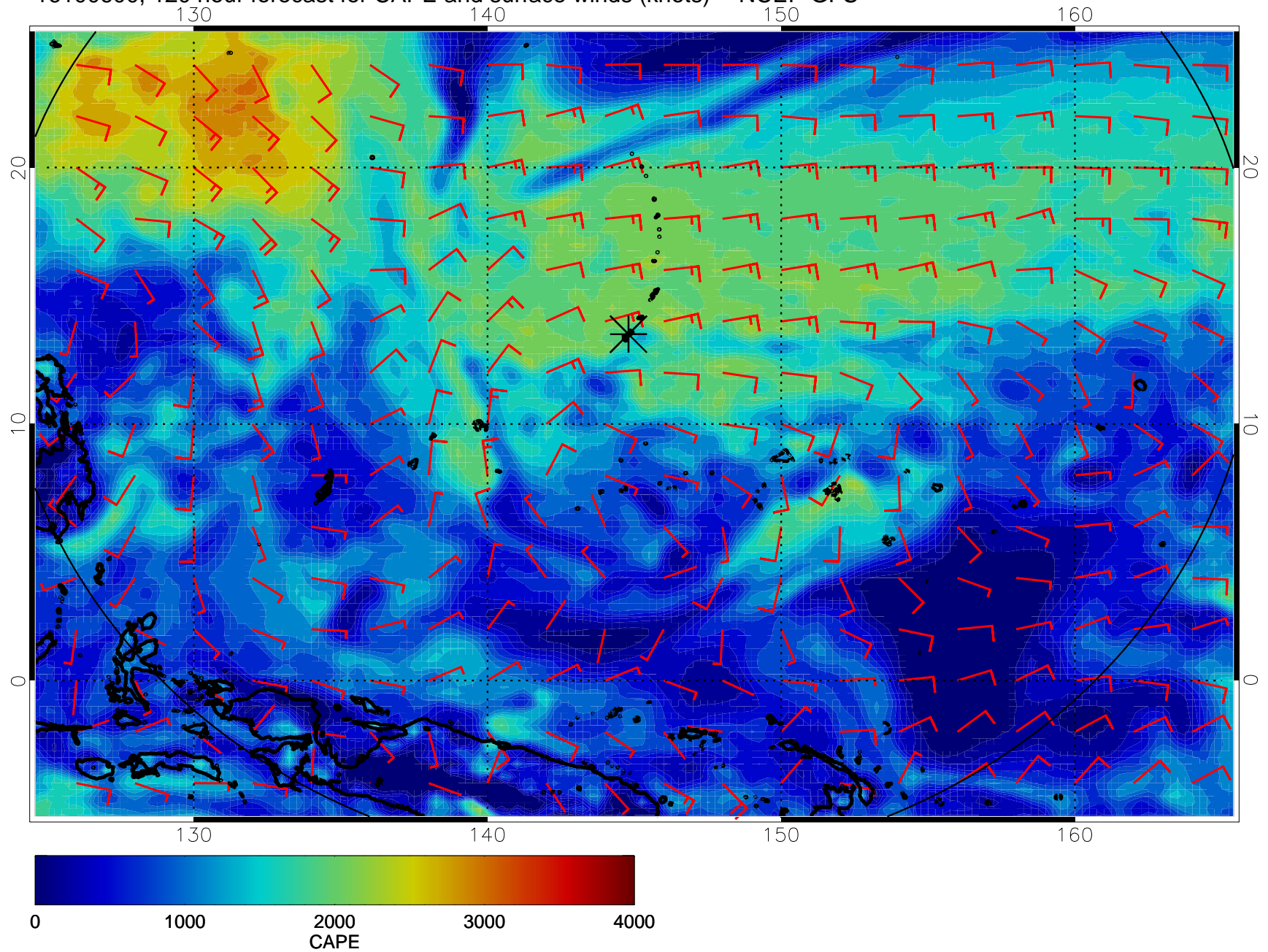
16100600, 120 hour forecast for CAPE and surface winds (knots) -- NCEP GFS
