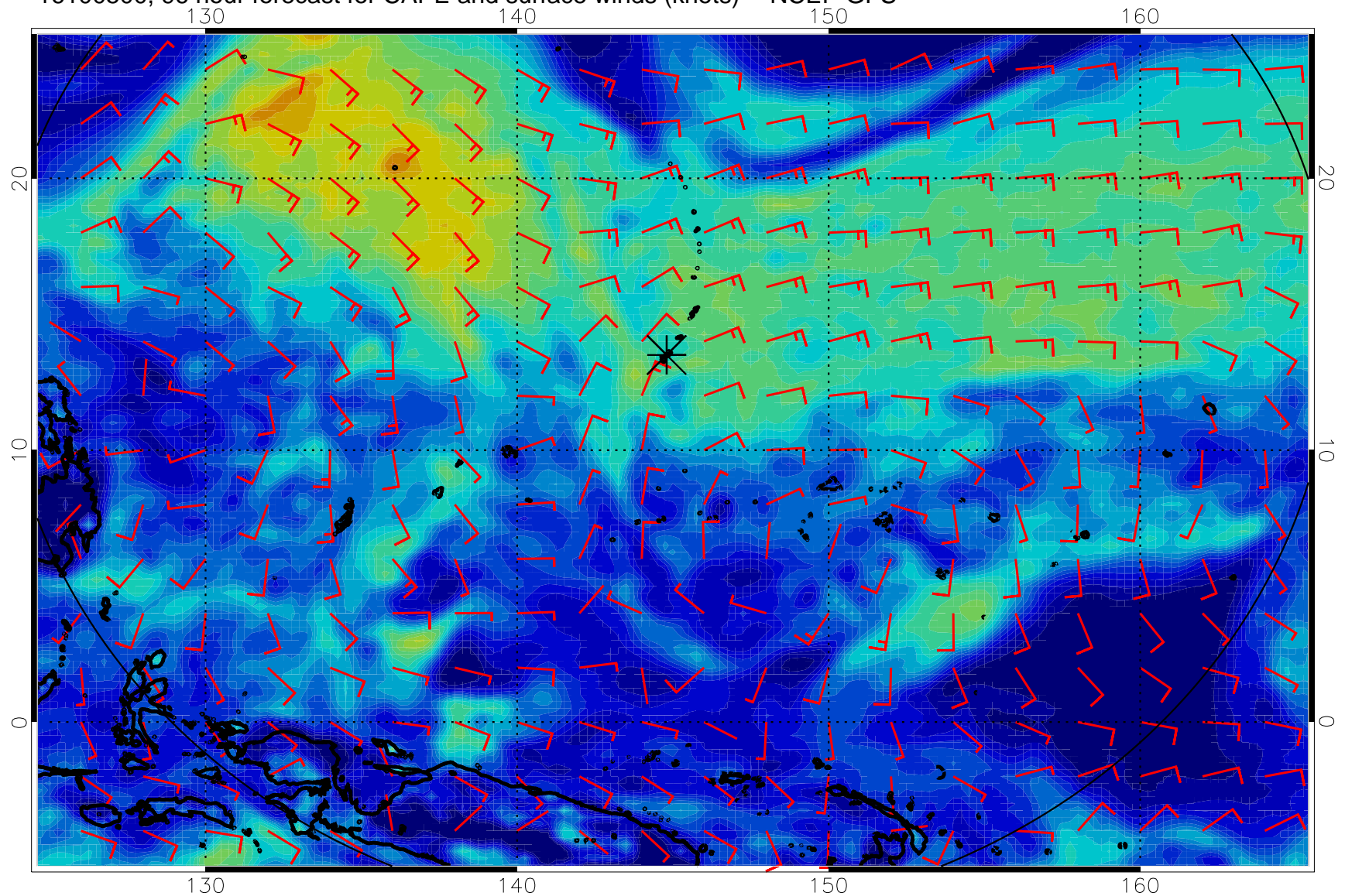
16100500, 96 hour forecast for CAPE and surface winds (knots) -- NCEP GFS
